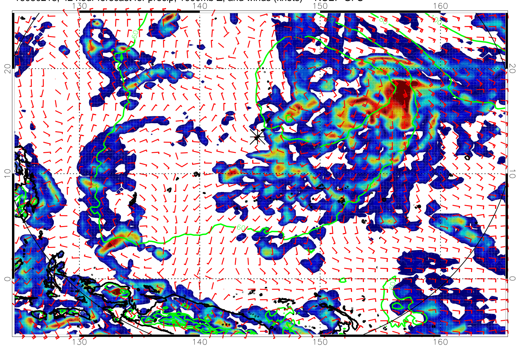
16080218, 42 hour forecast for precip, 1000mb Z, and winds (knots) -- NCEP GFS
