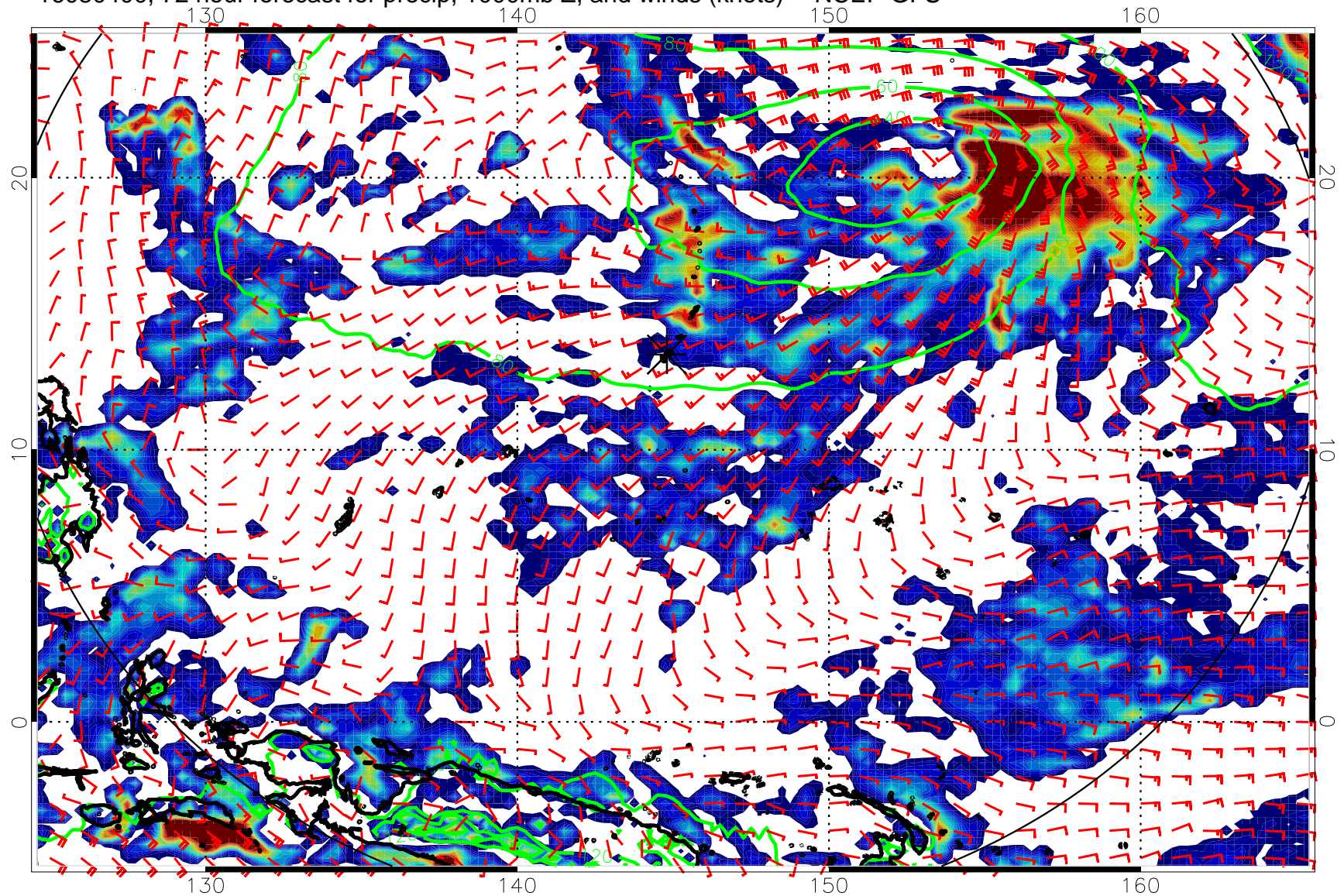
16080400, 72 hour forecast for precip, 1000mb Z, and winds (knots) -- NCEP GFS
