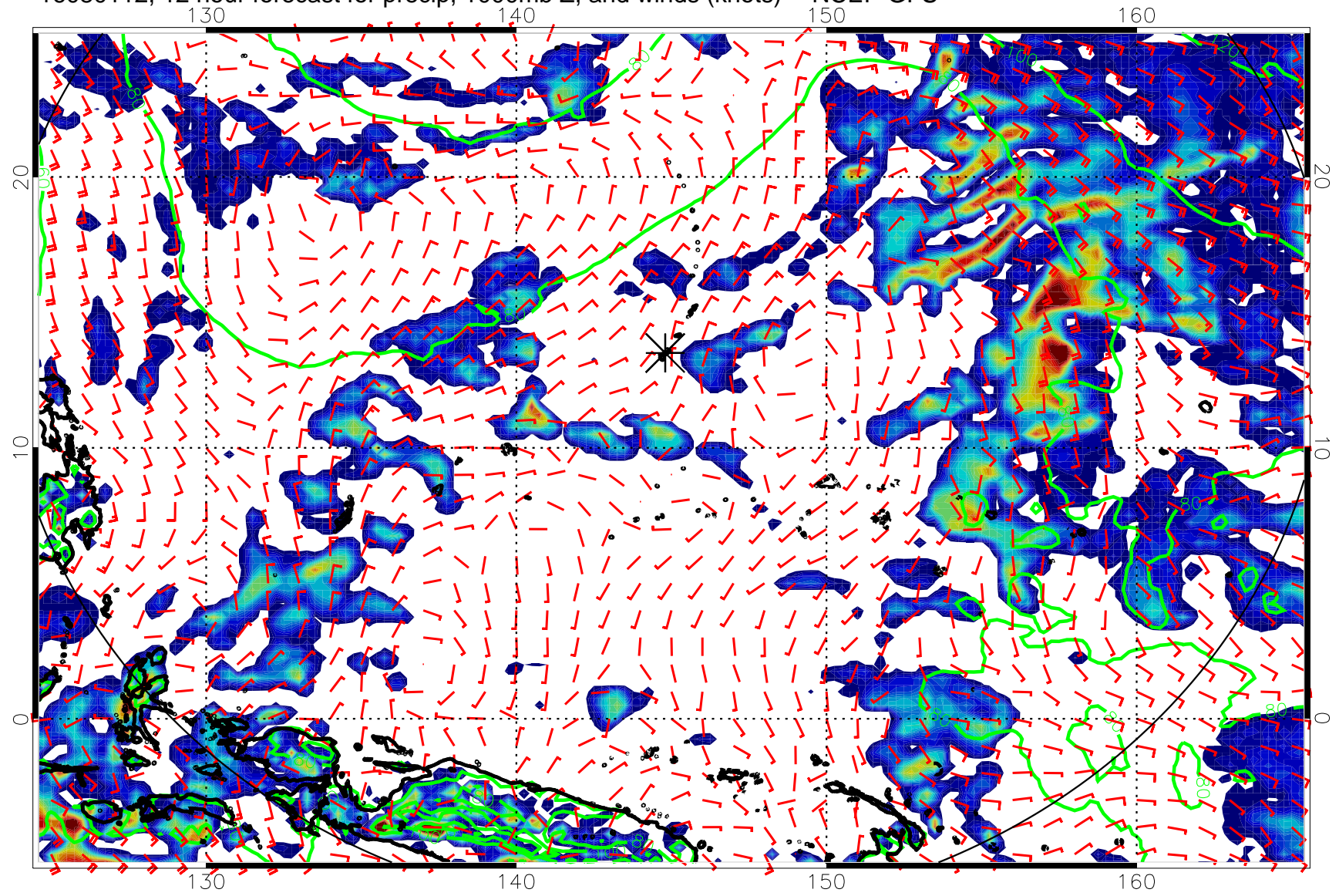
16080112, 12 hour forecast for precip, 1000mb Z, and winds (knots) -- NCEP GFS
