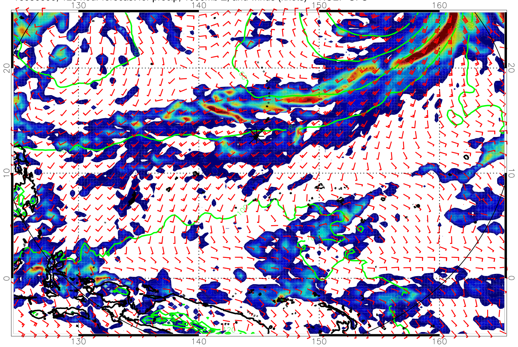
16080600, 120 hour forecast for precip, 1000mb Z, and winds (knots) -- NCEP GFS
