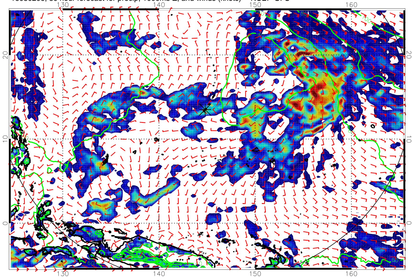
16080206, 30 hour forecast for precip, 1000mb Z, and winds (knots) -- NCEP GFS
