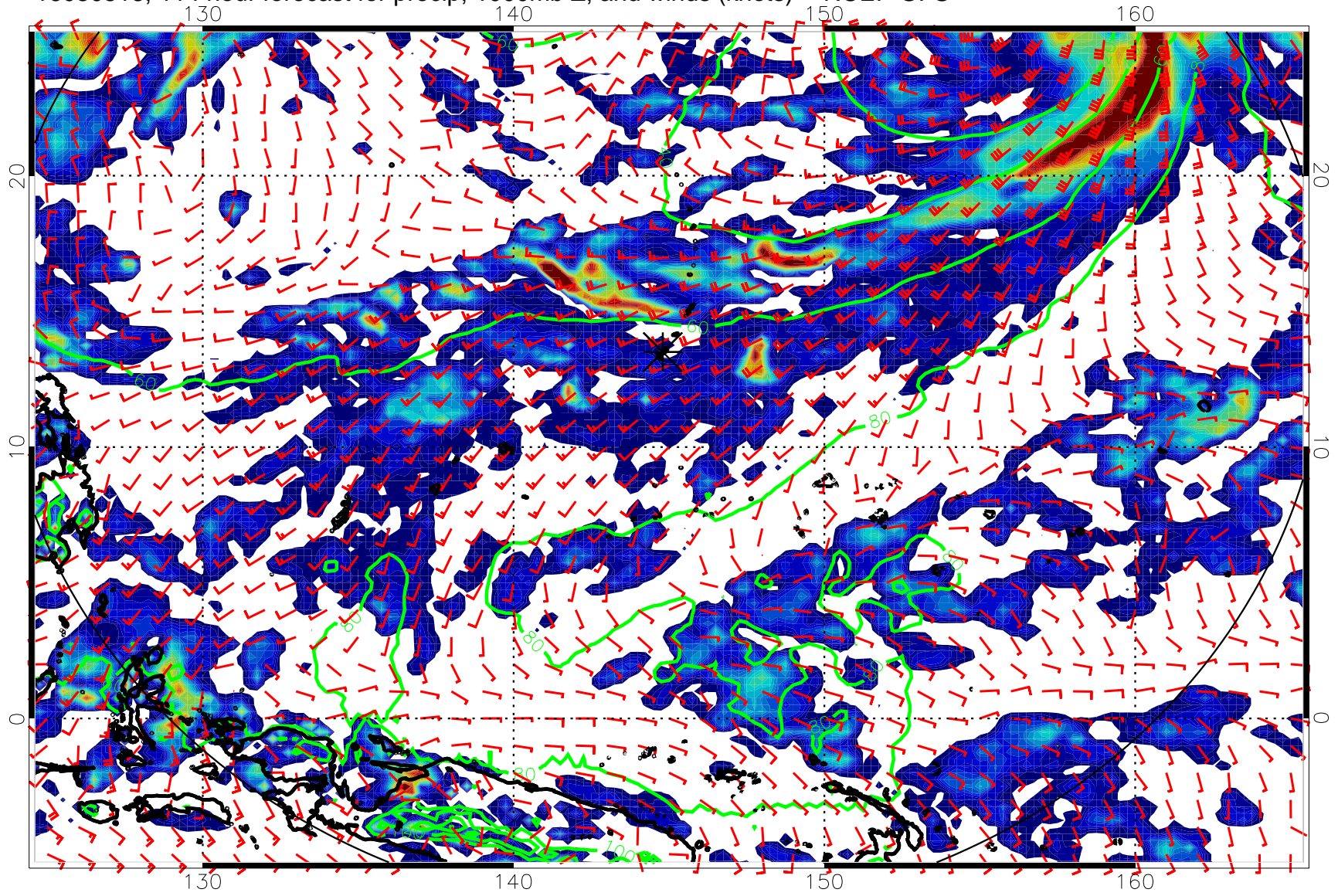
16080518, 114 hour forecast for precip, 1000mb Z, and winds (knots) -- NCEP GFS
