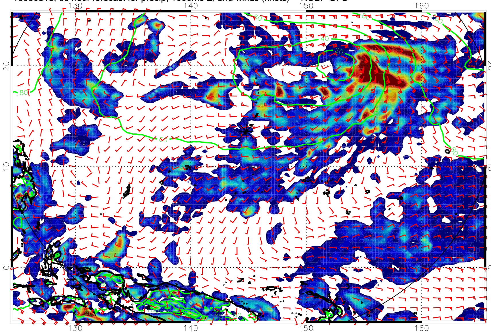
16080318, 66 hour forecast for precip, 1000mb Z, and winds (knots) -- NCEP GFS
