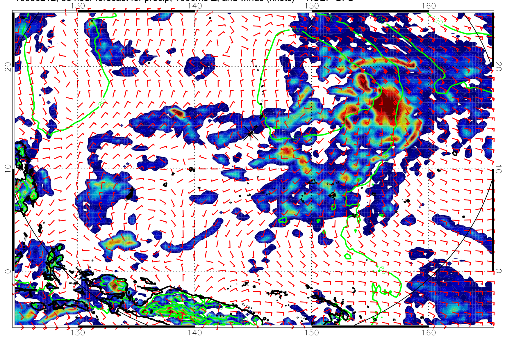
16080212, 36 hour forecast for precip, 1000mb Z, and winds (knots) -- NCEP GFS
