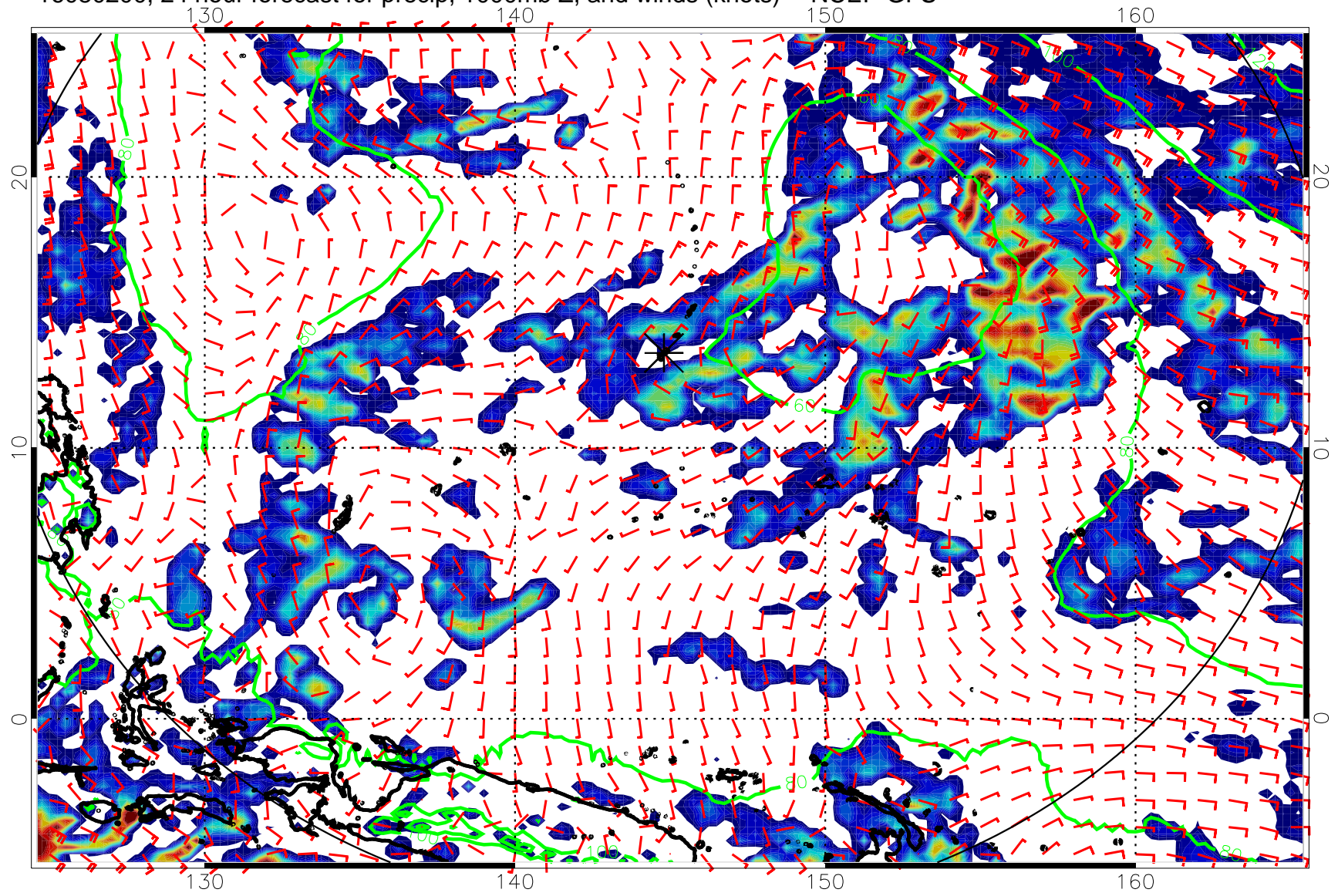
16080200, 24 hour forecast for precip, 1000mb Z, and winds (knots) -- NCEP GFS
