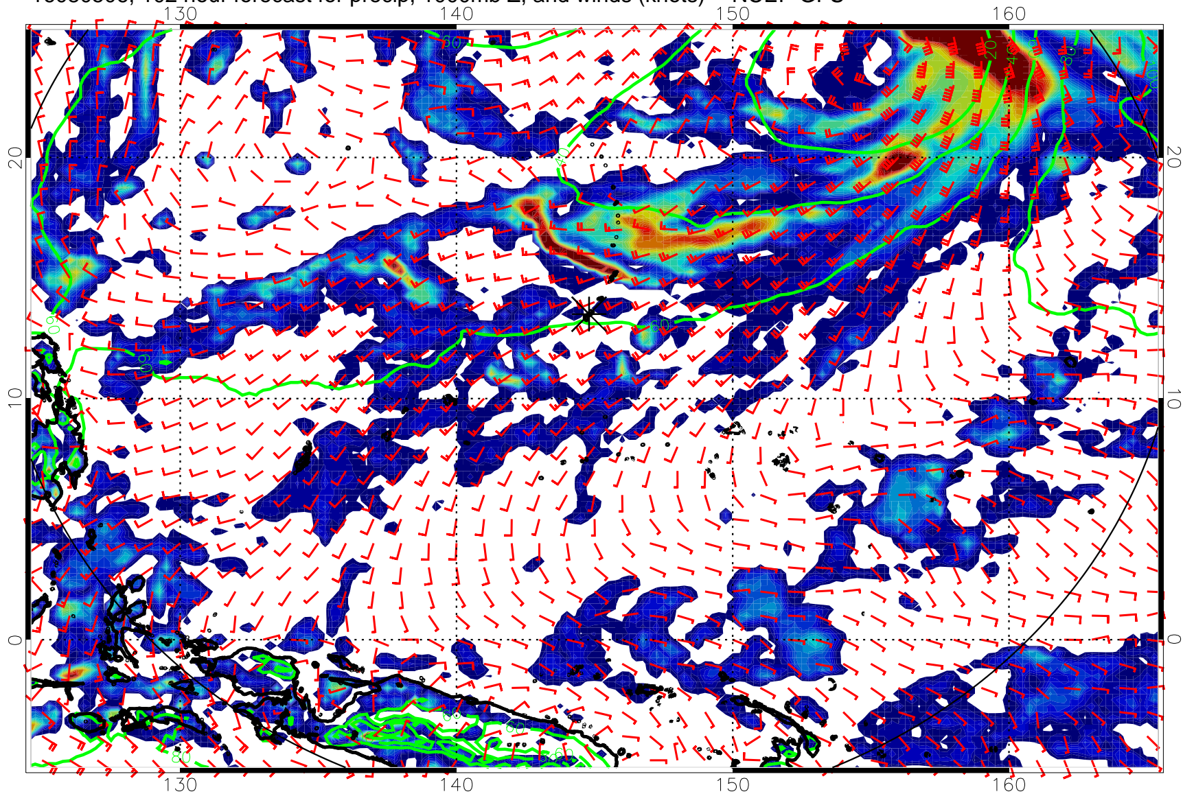
16080506, 102 hour forecast for precip, 1000mb Z, and winds (knots) -- NCEP GFS
