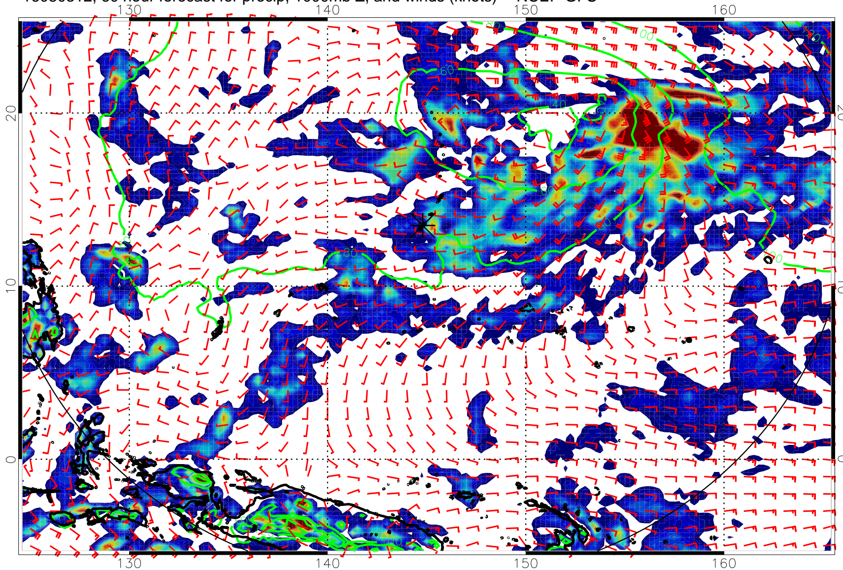
16080312, 60 hour forecast for precip, 1000mb Z, and winds (knots) -- NCEP GFS
