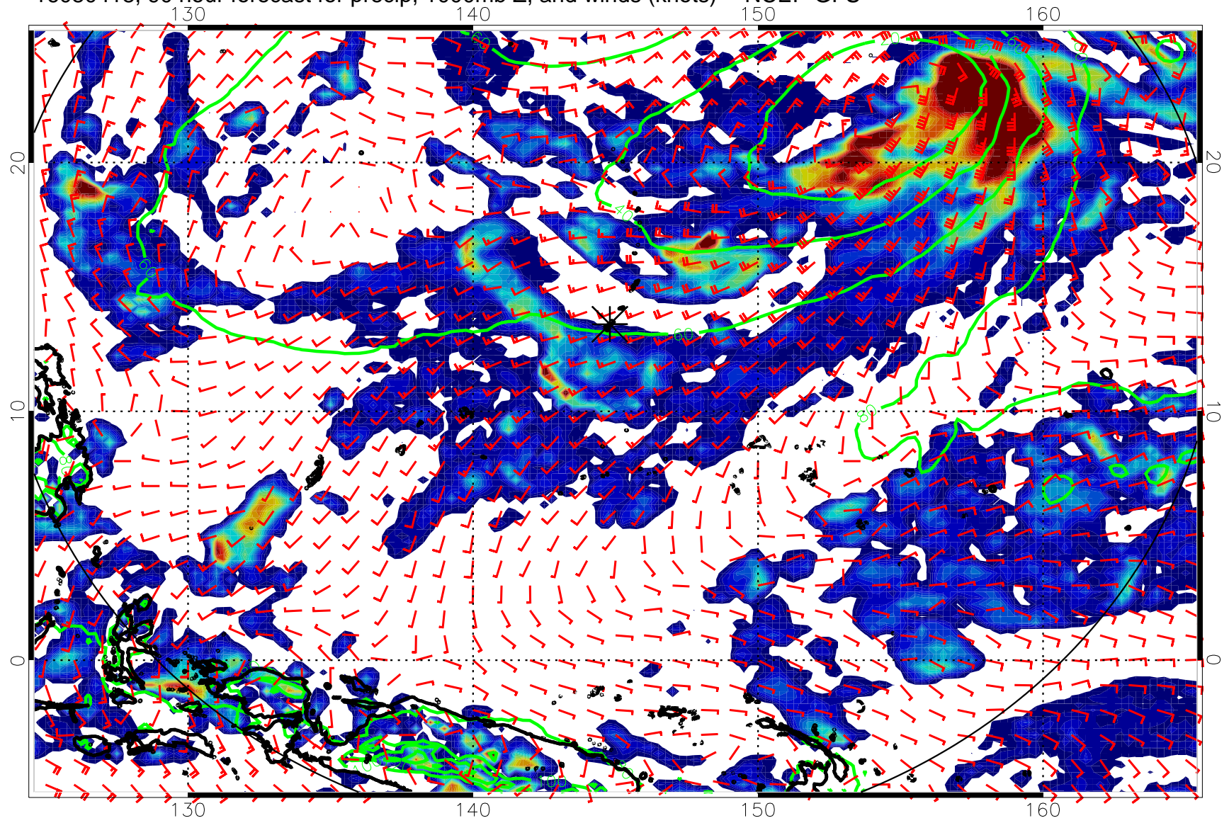
16080418, 90 hour forecast for precip, 1000mb Z, and winds (knots) -- NCEP GFS
