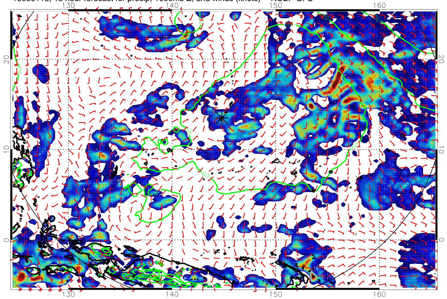
16080118, 18 hour forecast for precip, 1000mb Z, and winds (knots) -- NCEP GFS
