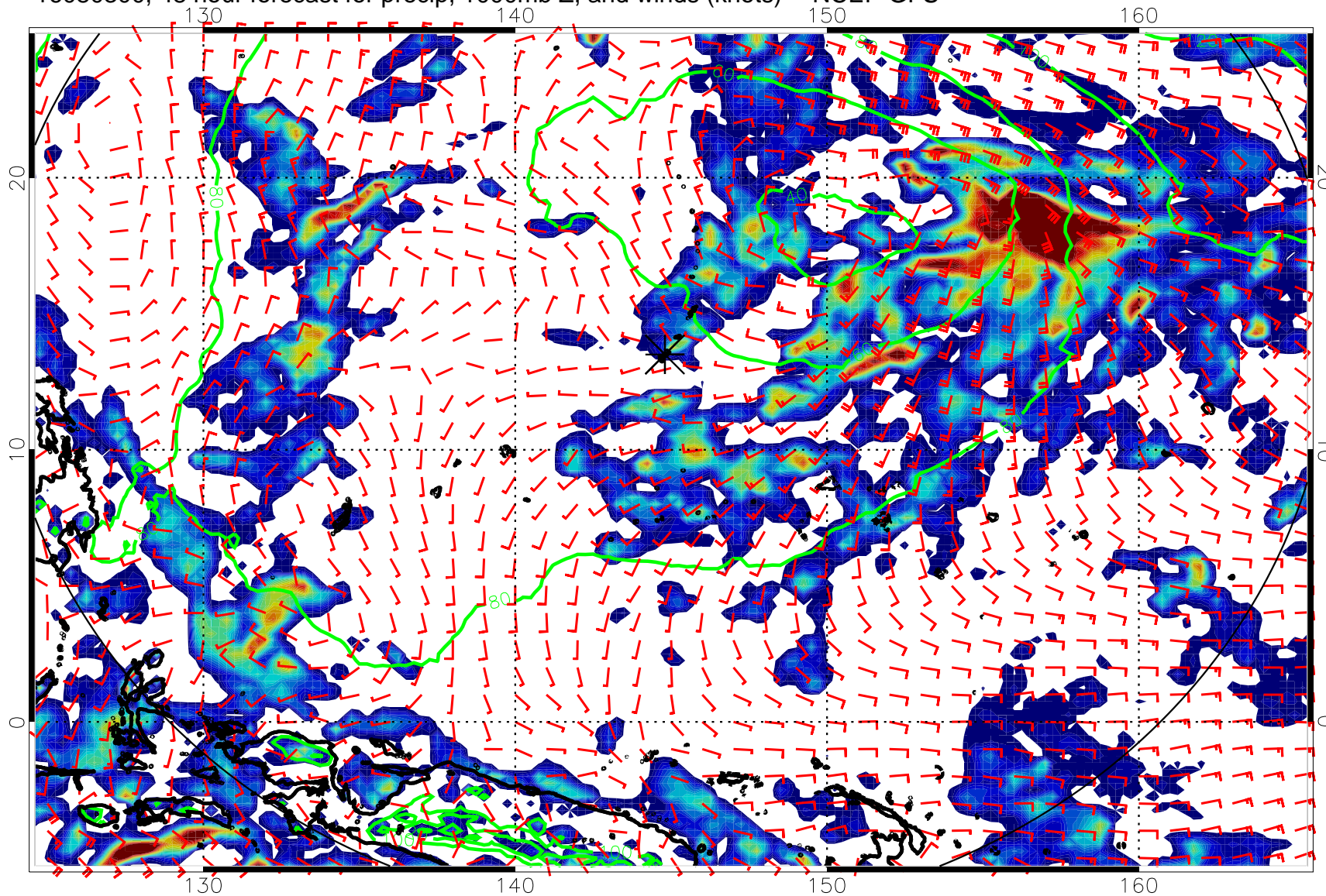
16080300, 48 hour forecast for precip, 1000mb Z, and winds (knots) -- NCEP GFS
