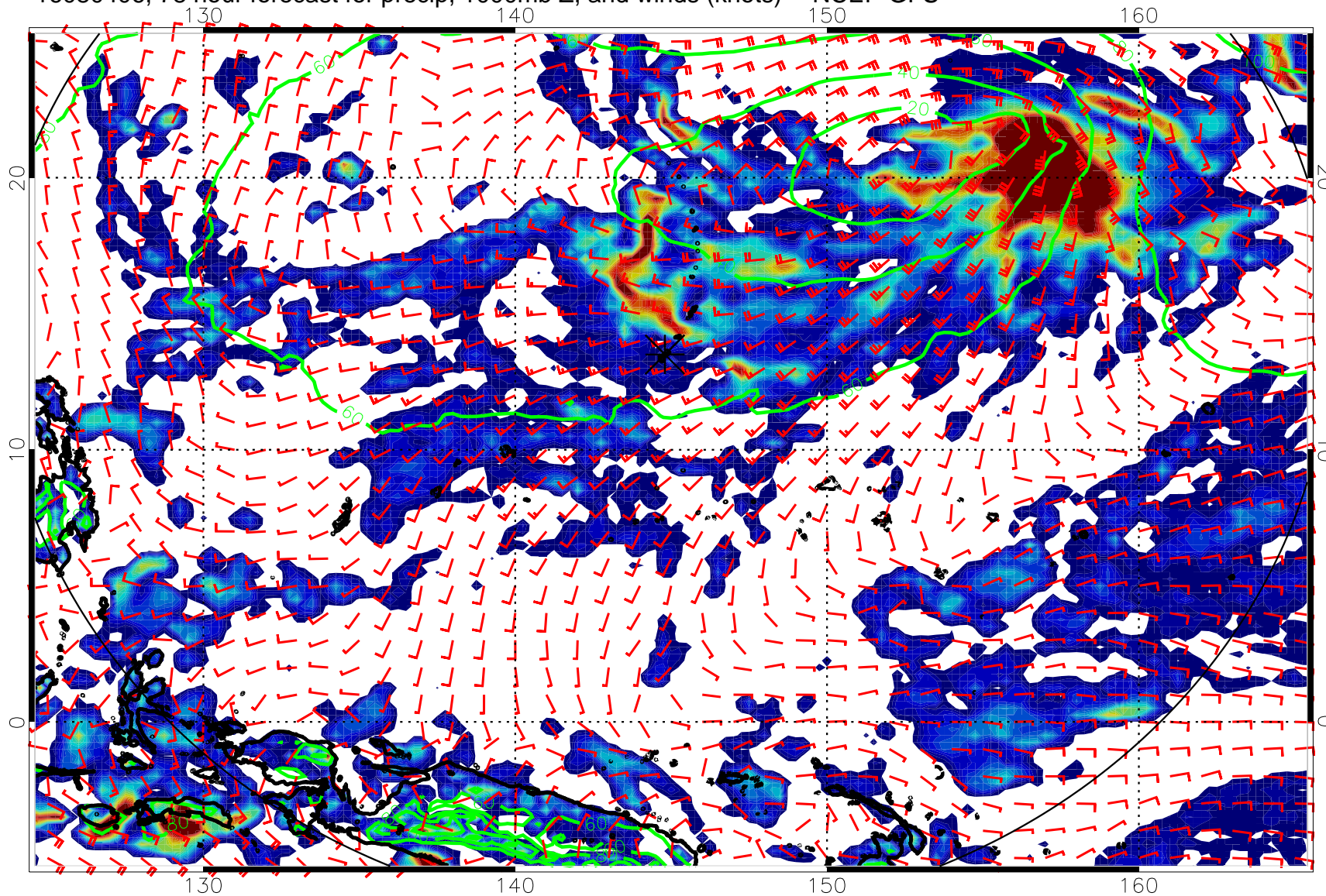
16080406, 78 hour forecast for precip, 1000mb Z, and winds (knots) -- NCEP GFS
