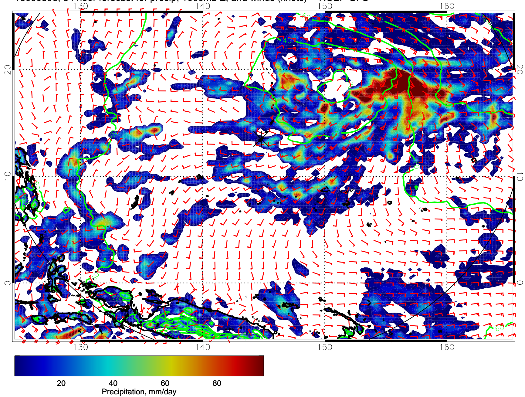
16080306, 54 hour forecast for precip, 1000mb Z, and winds (knots) -- NCEP GFS
