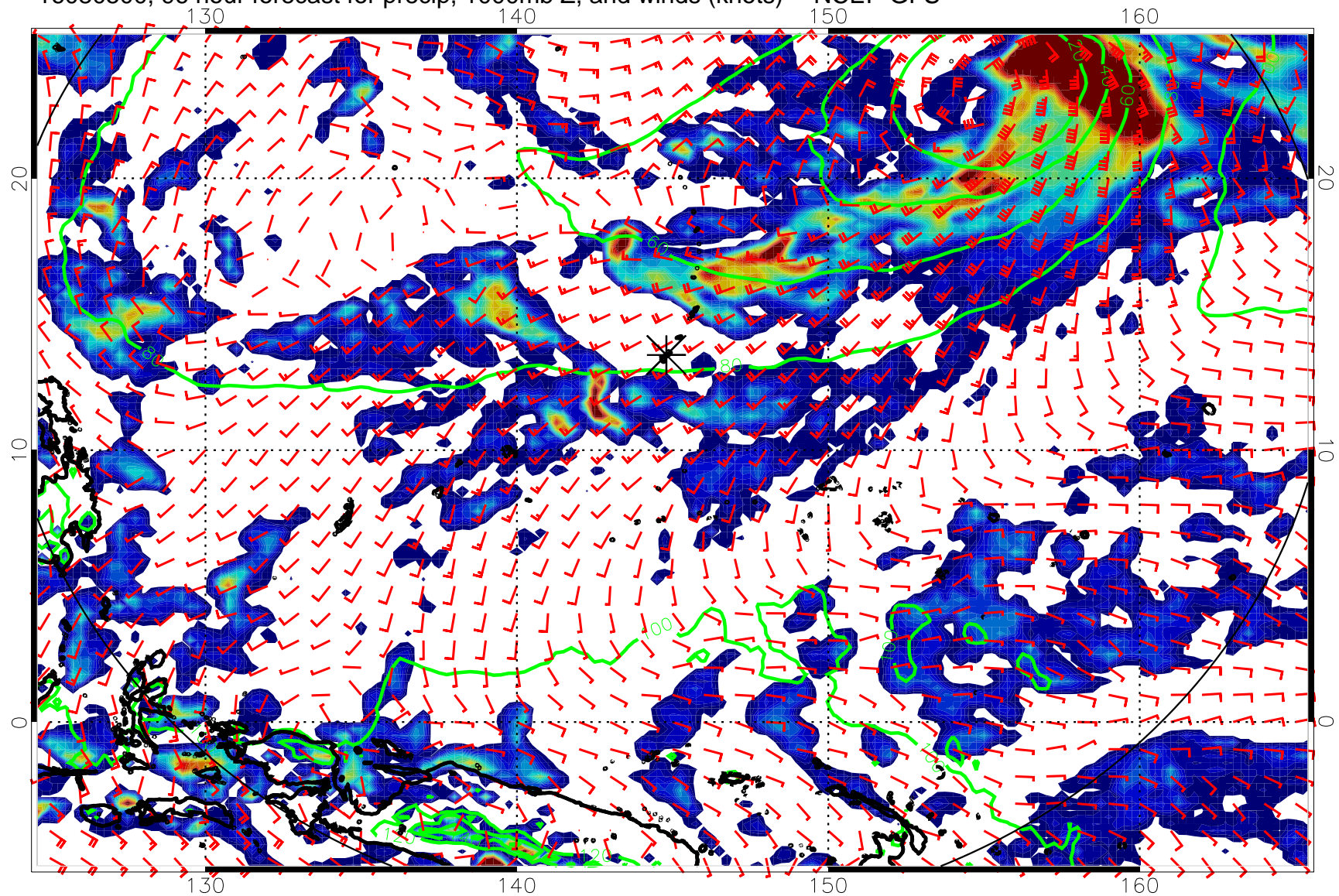
16080500, 96 hour forecast for precip, 1000mb Z, and winds (knots) -- NCEP GFS
