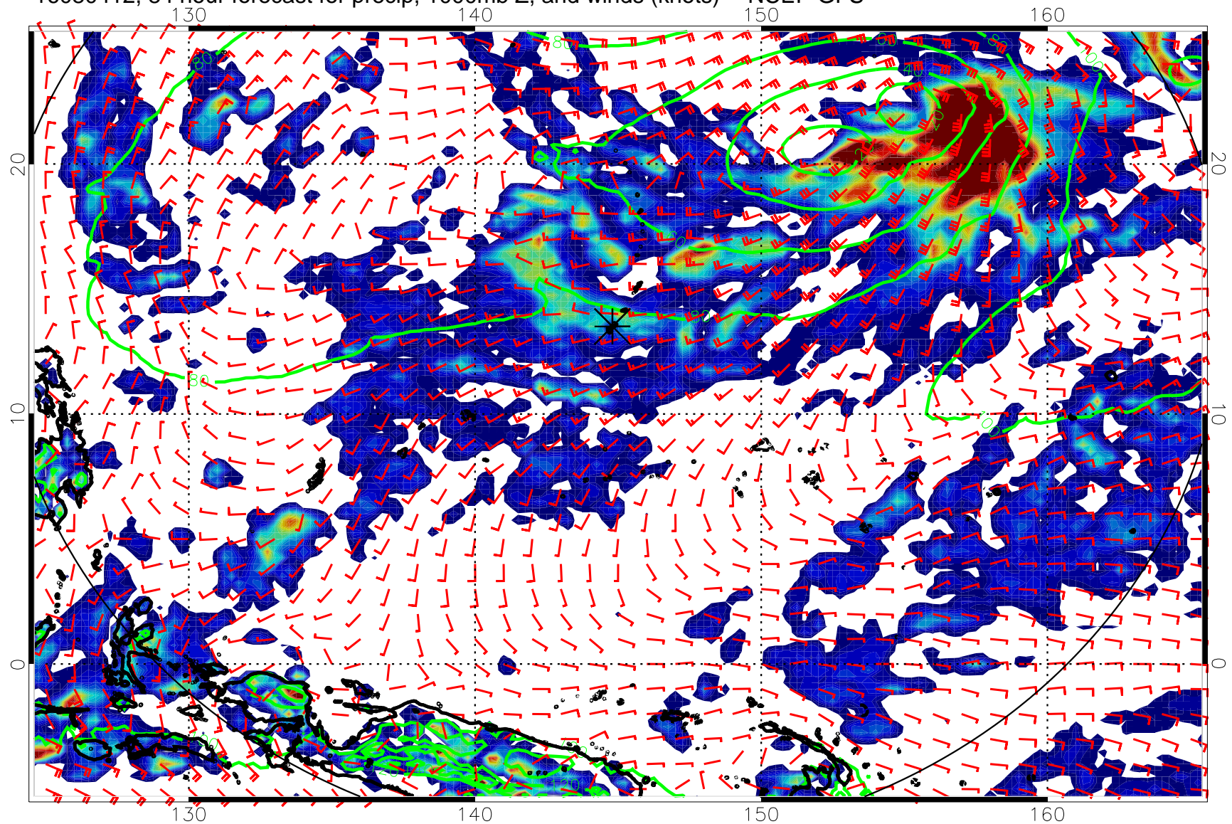
16080412, 84 hour forecast for precip, 1000mb Z, and winds (knots) -- NCEP GFS
