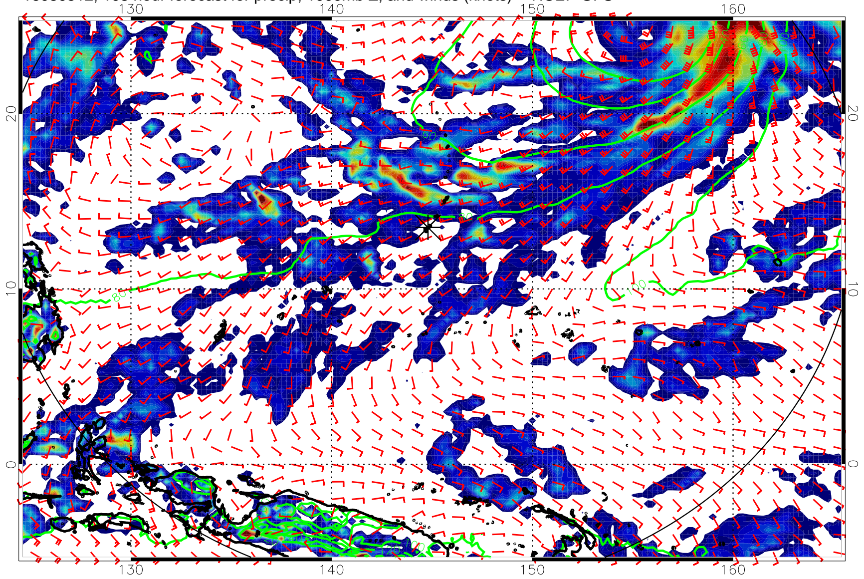
16080512, 108 hour forecast for precip, 1000mb Z, and winds (knots) -- NCEP GFS
