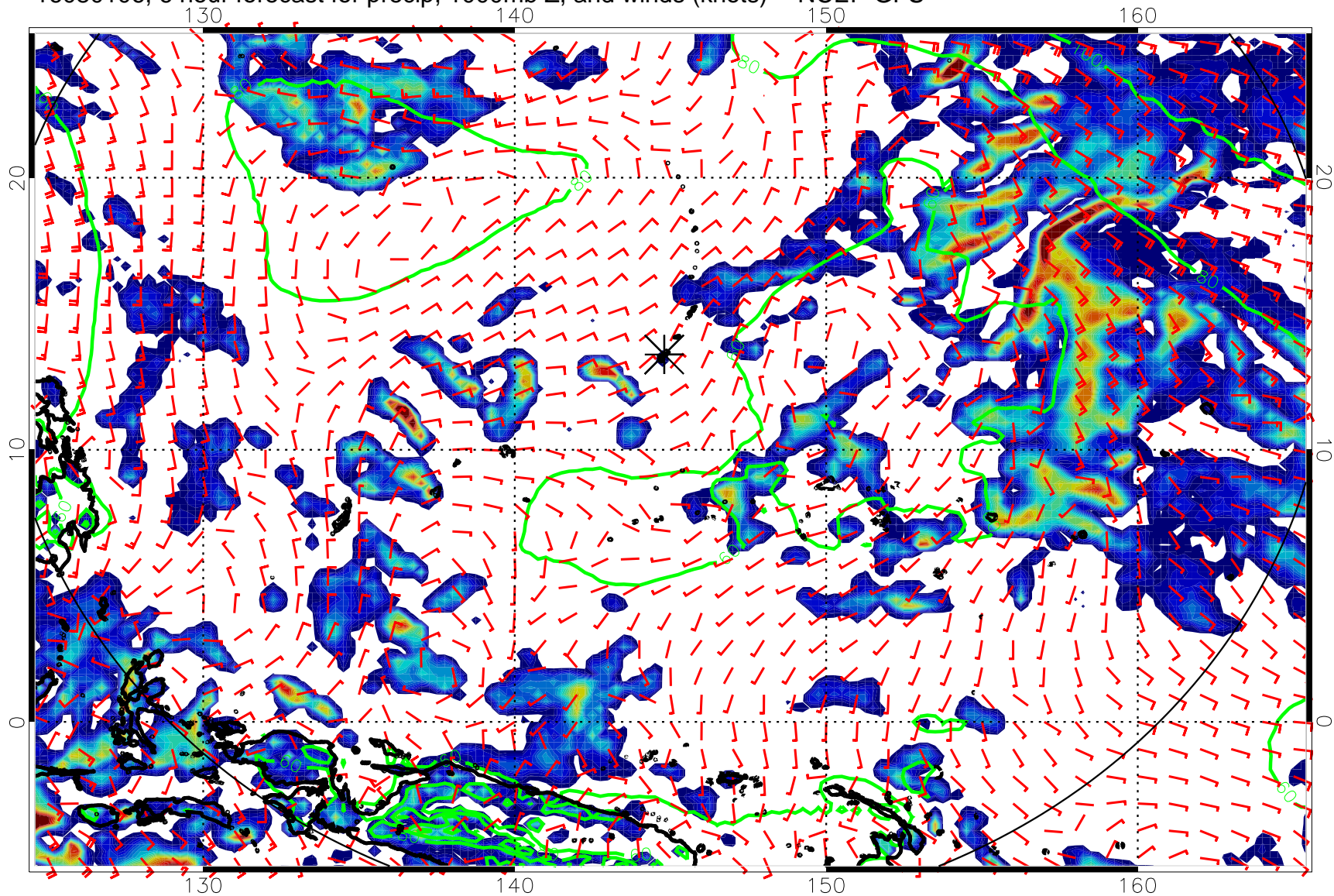
16080106, 6 hour forecast for precip, 1000mb Z, and winds (knots) -- NCEP GFS
