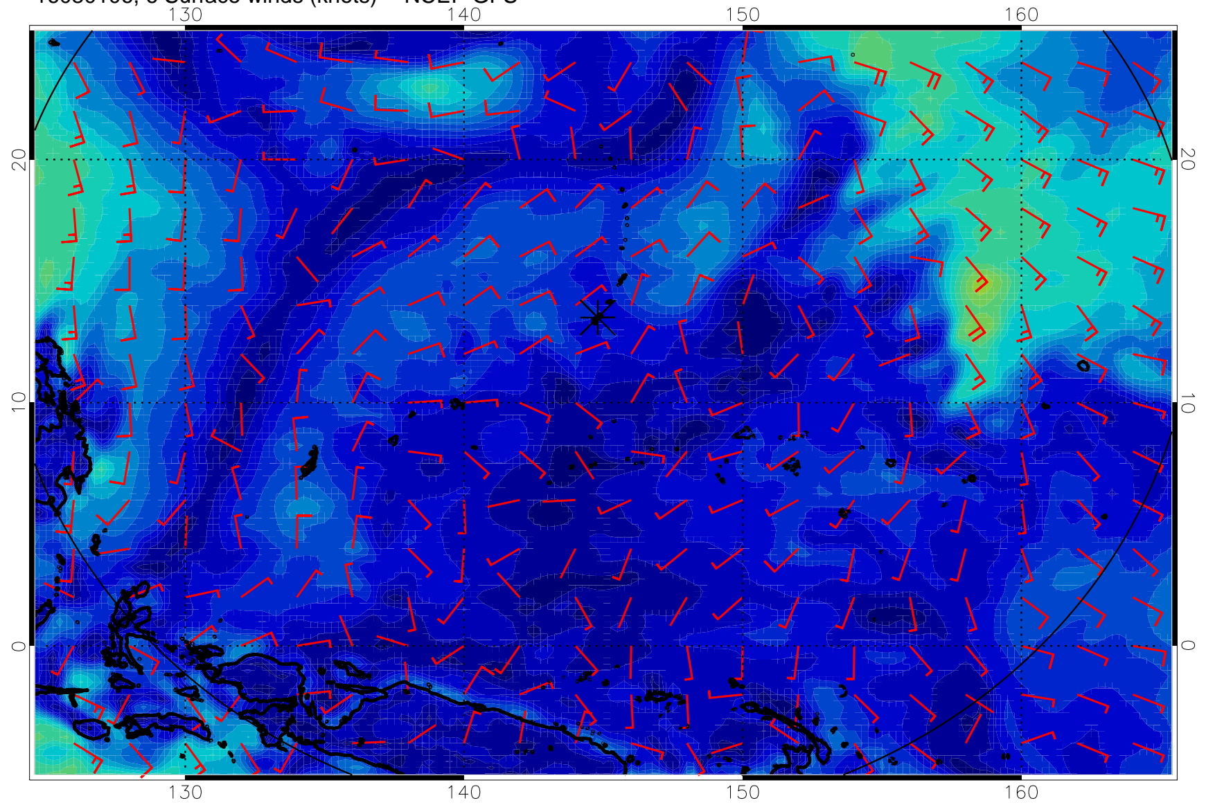
16080106, 6 Surface winds (knots) -- NCEP GFS
