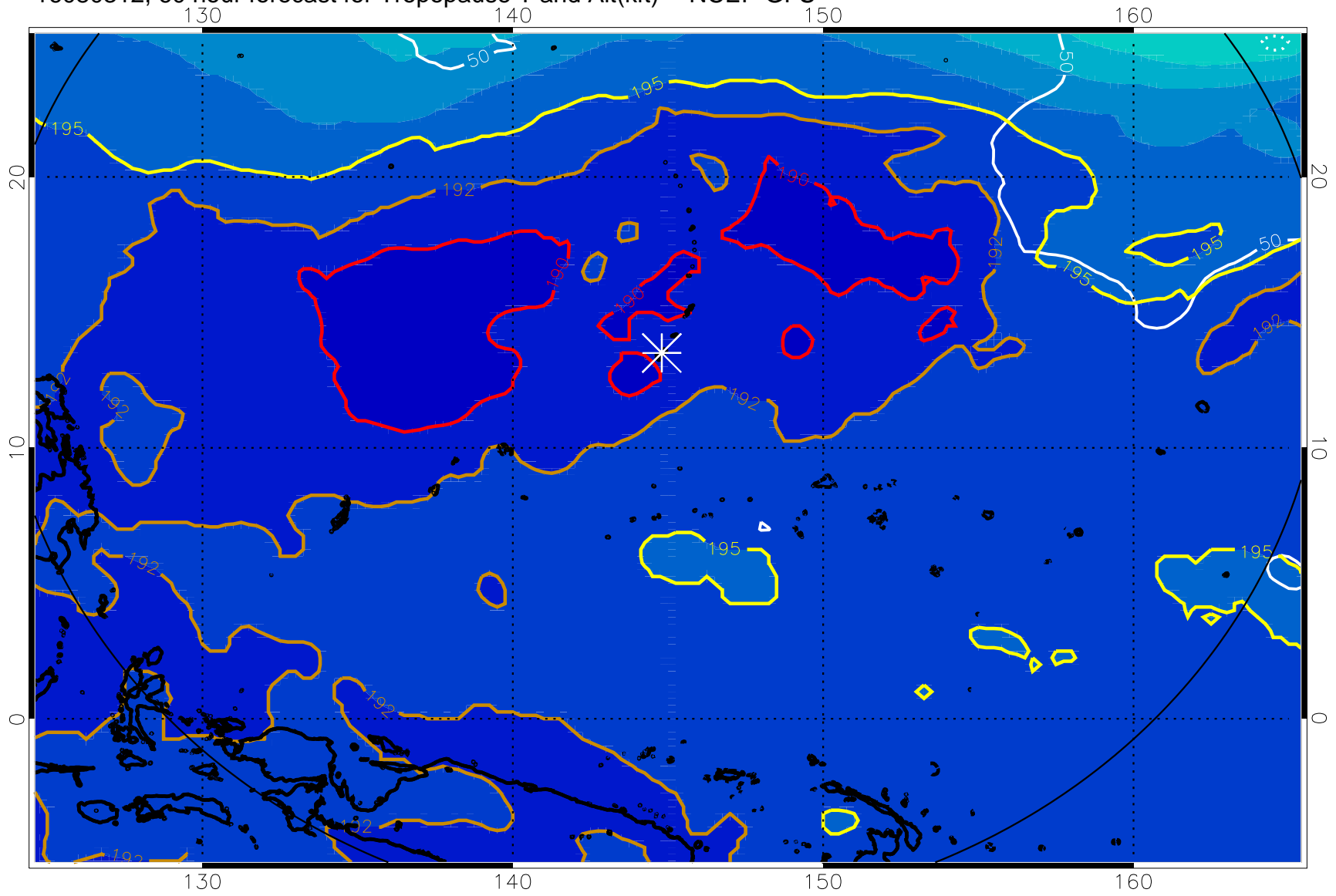
16080312, 60 hour forecast for Tropopause T and Alt(kft) -- NCEP GFS
