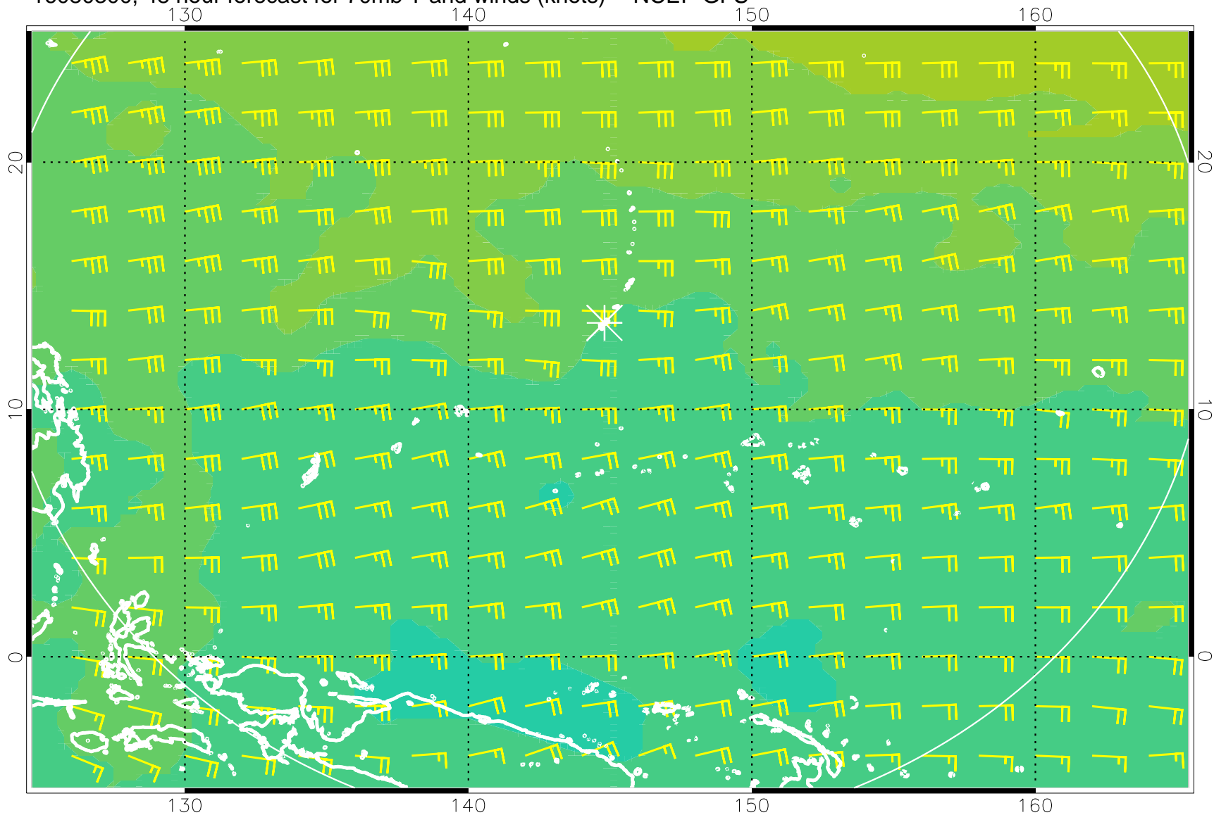
16080300, 48 hour forecast for 70mb T and winds (knots) -- NCEP GFS
