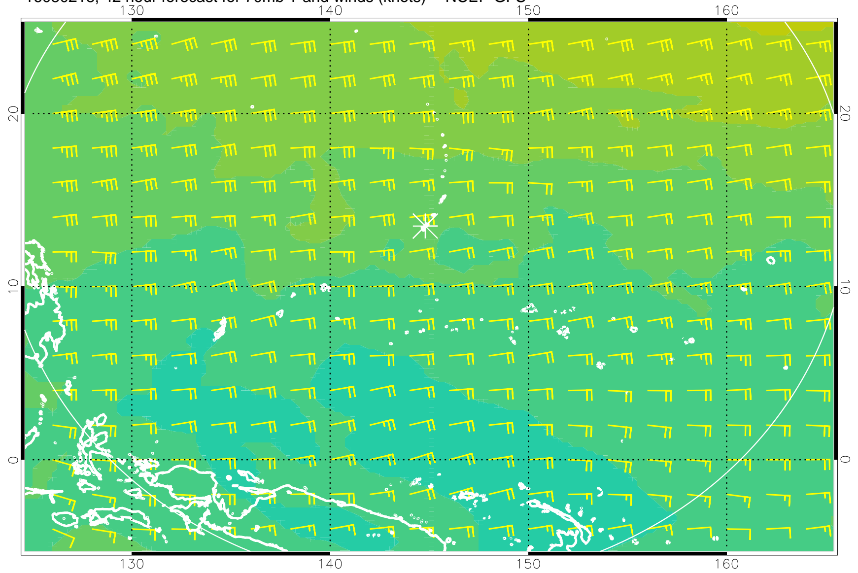
16080218, 42 hour forecast for 70mb T and winds (knots) -- NCEP GFS
