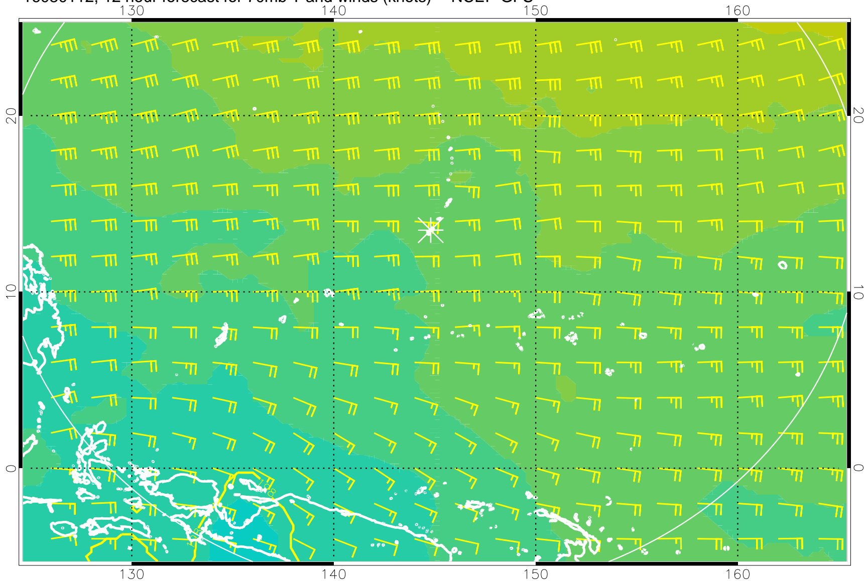
16080112, 12 hour forecast for 70mb T and winds (knots) -- NCEP GFS
