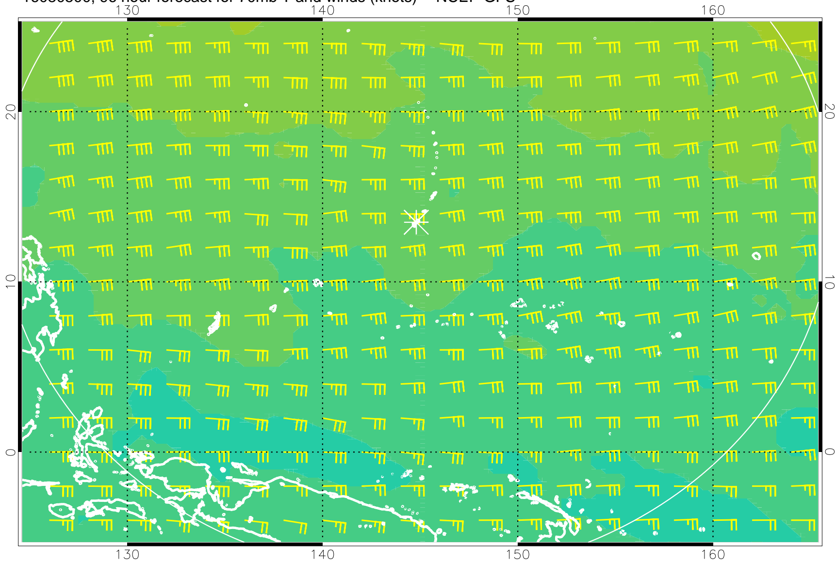
16080500, 96 hour forecast for 70mb T and winds (knots) -- NCEP GFS
