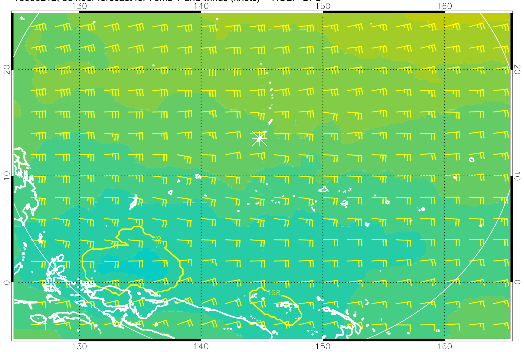
16080212, 36 hour forecast for 70mb T and winds (knots) -- NCEP GFS
