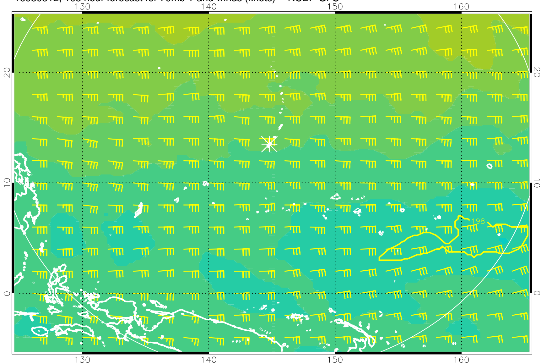
16080512, 108 hour forecast for 70mb T and winds (knots) -- NCEP GFS
