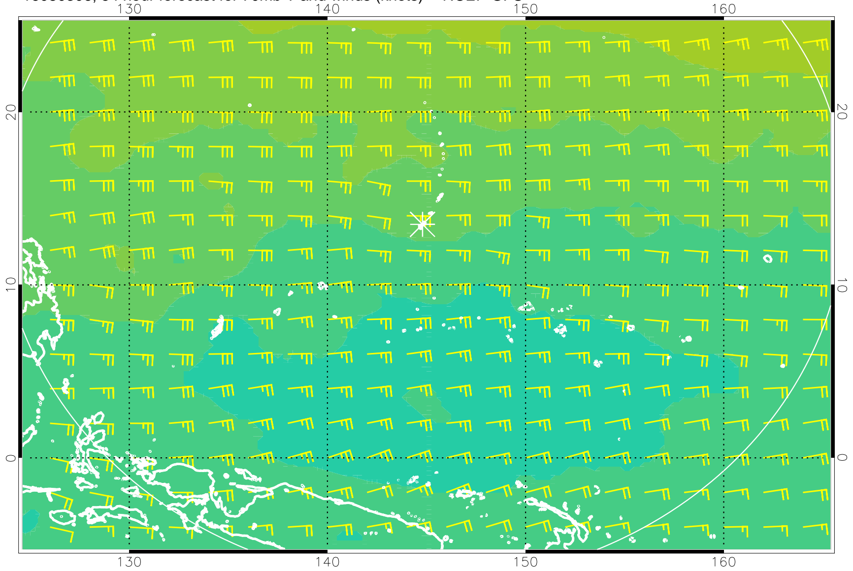
16080306, 54 hour forecast for 70mb T and winds (knots) -- NCEP GFS
