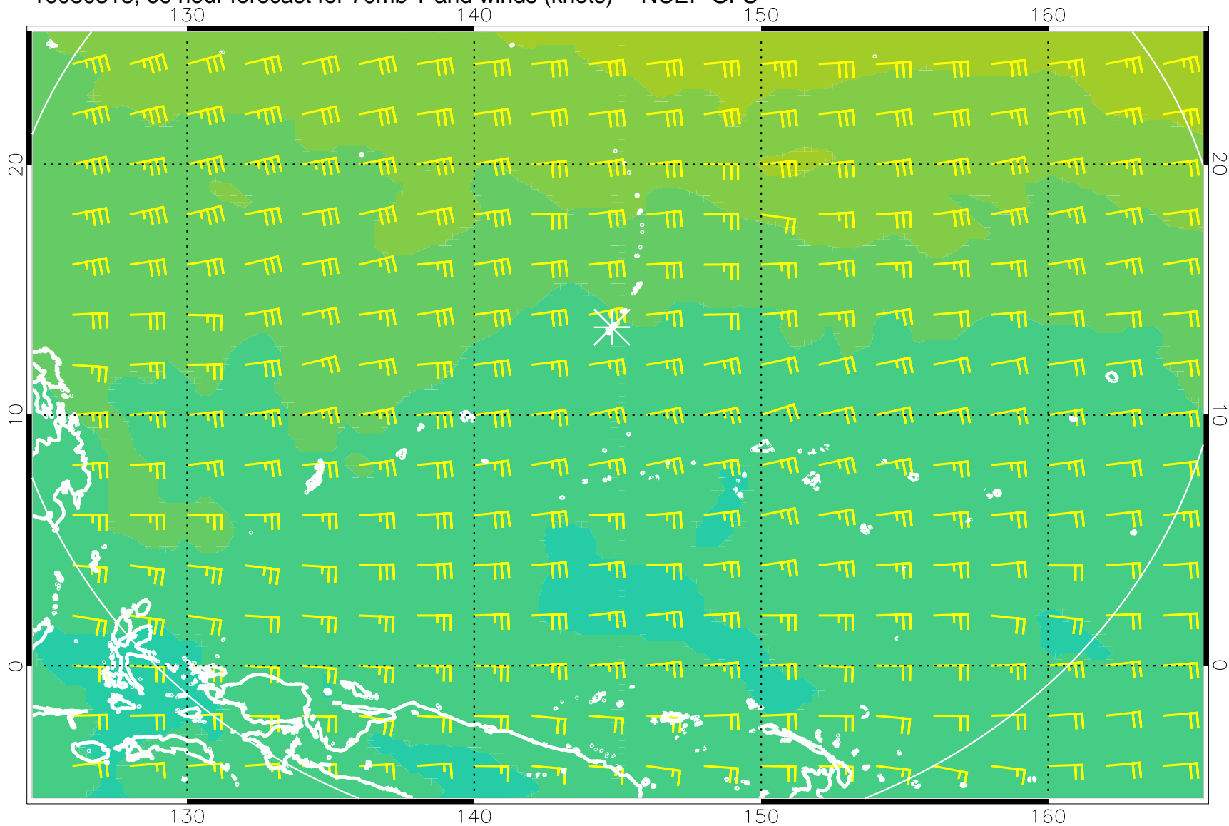
16080318, 66 hour forecast for 70mb T and winds (knots) -- NCEP GFS
