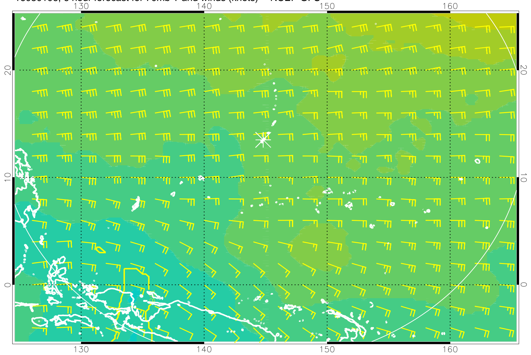
16080106, 6 hour forecast for 70mb T and winds (knots) -- NCEP GFS
