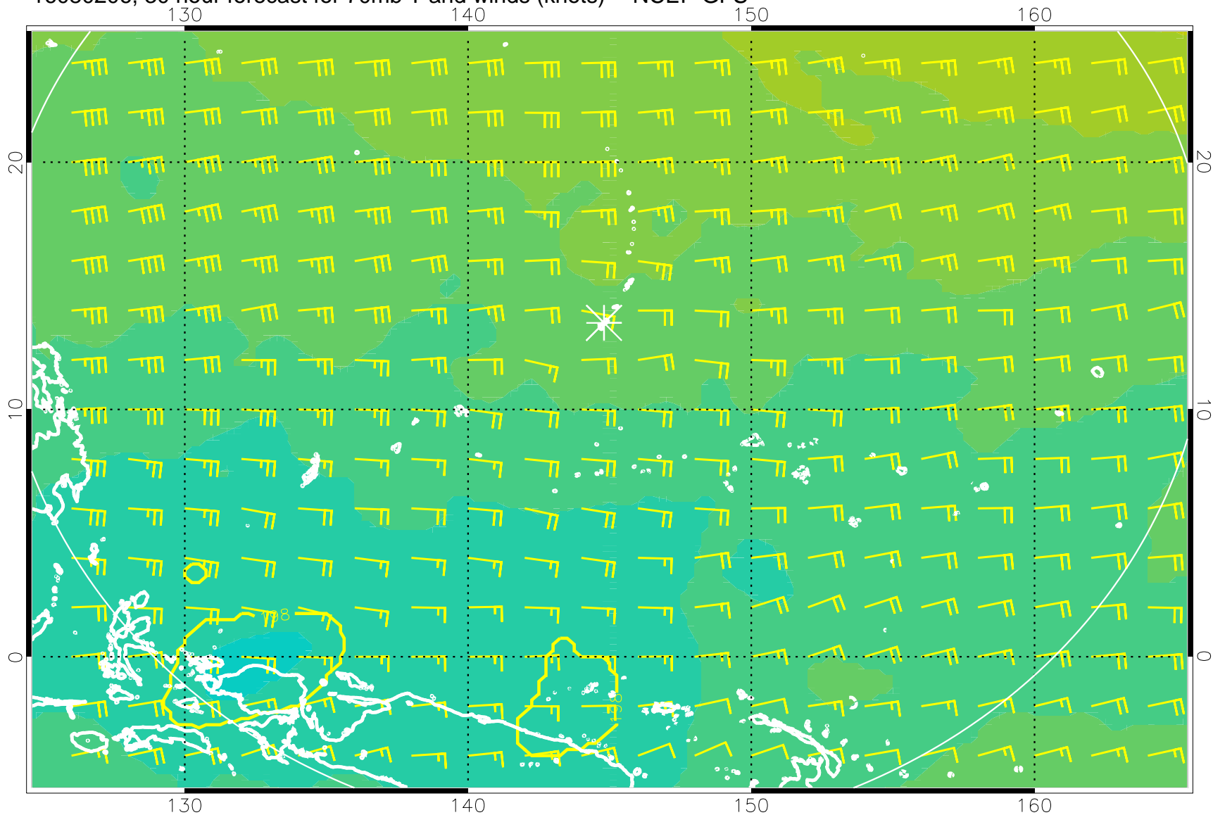
16080206, 30 hour forecast for 70mb T and winds (knots) -- NCEP GFS
