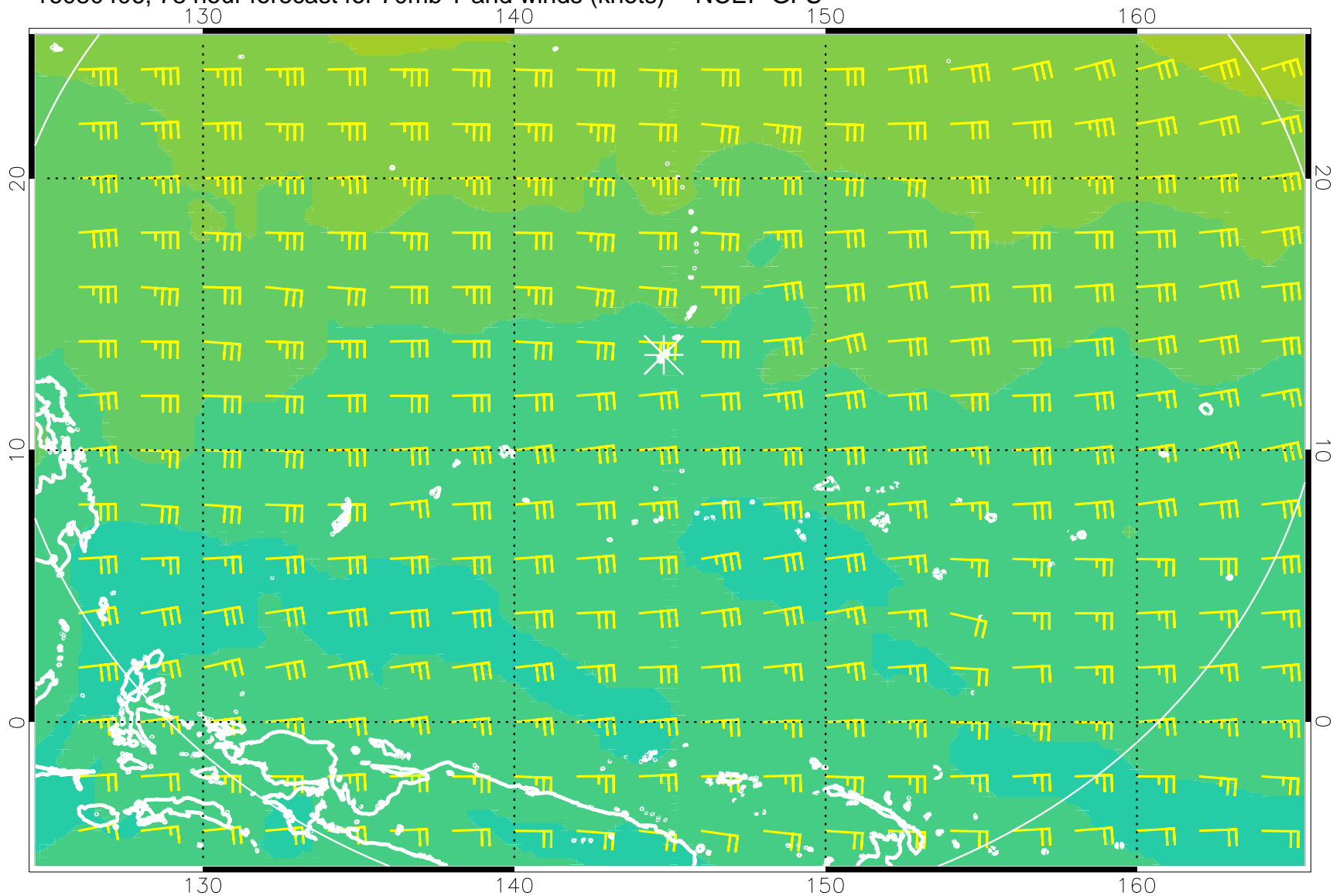
16080406, 78 hour forecast for 70mb T and winds (knots) -- NCEP GFS
