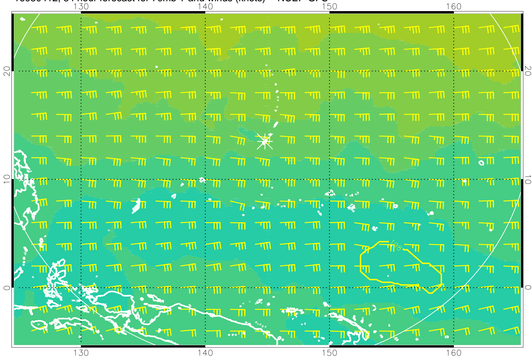
16080412, 84 hour forecast for 70mb T and winds (knots) -- NCEP GFS
