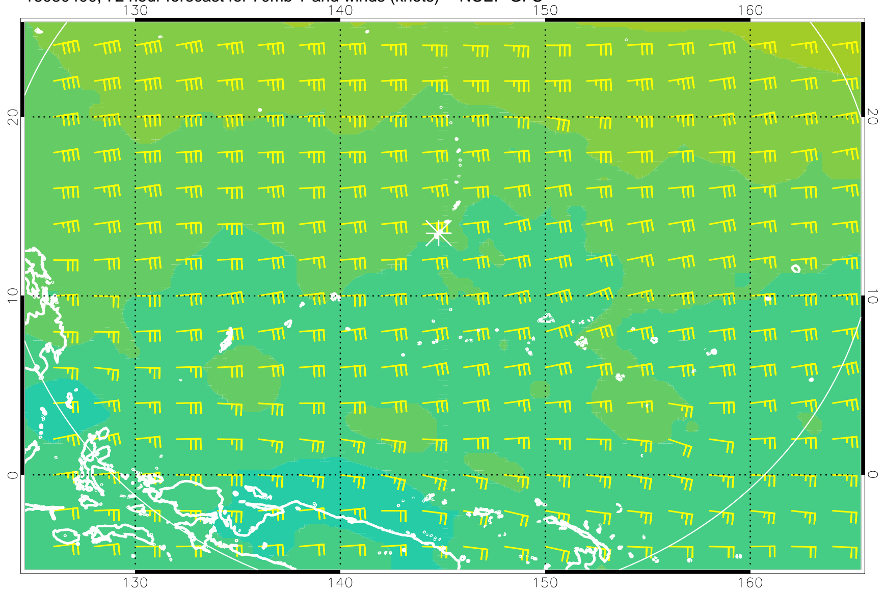
16080400, 72 hour forecast for 70mb T and winds (knots) -- NCEP GFS
