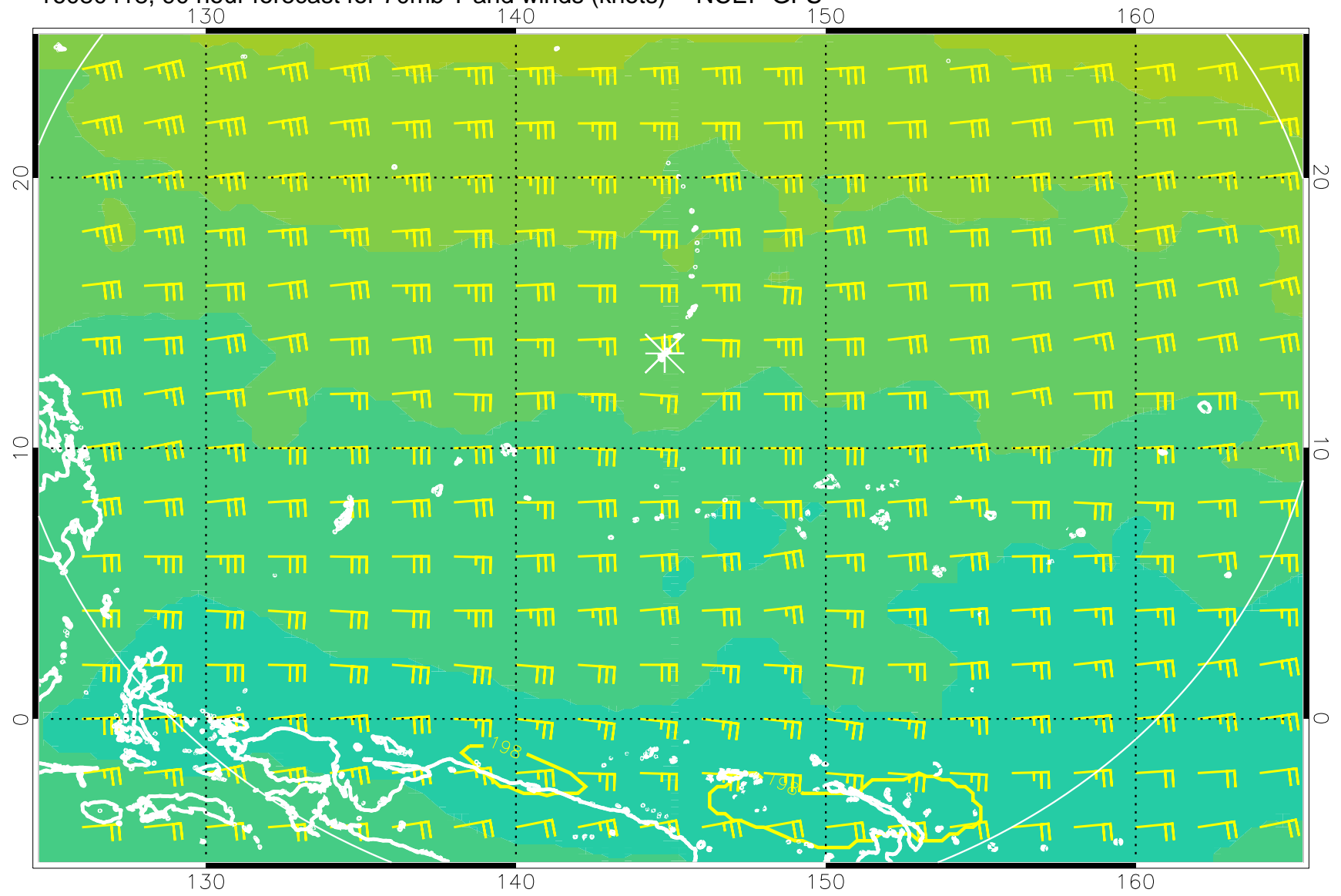
16080418, 90 hour forecast for 70mb T and winds (knots) -- NCEP GFS
