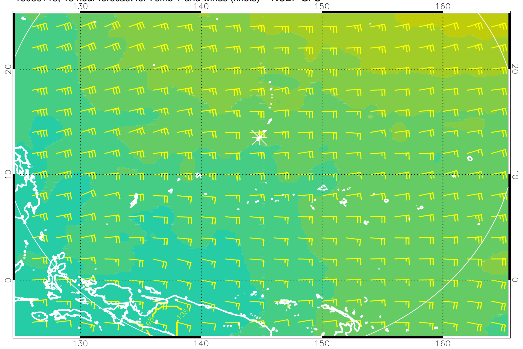
16080118, 18 hour forecast for 70mb T and winds (knots) -- NCEP GFS
