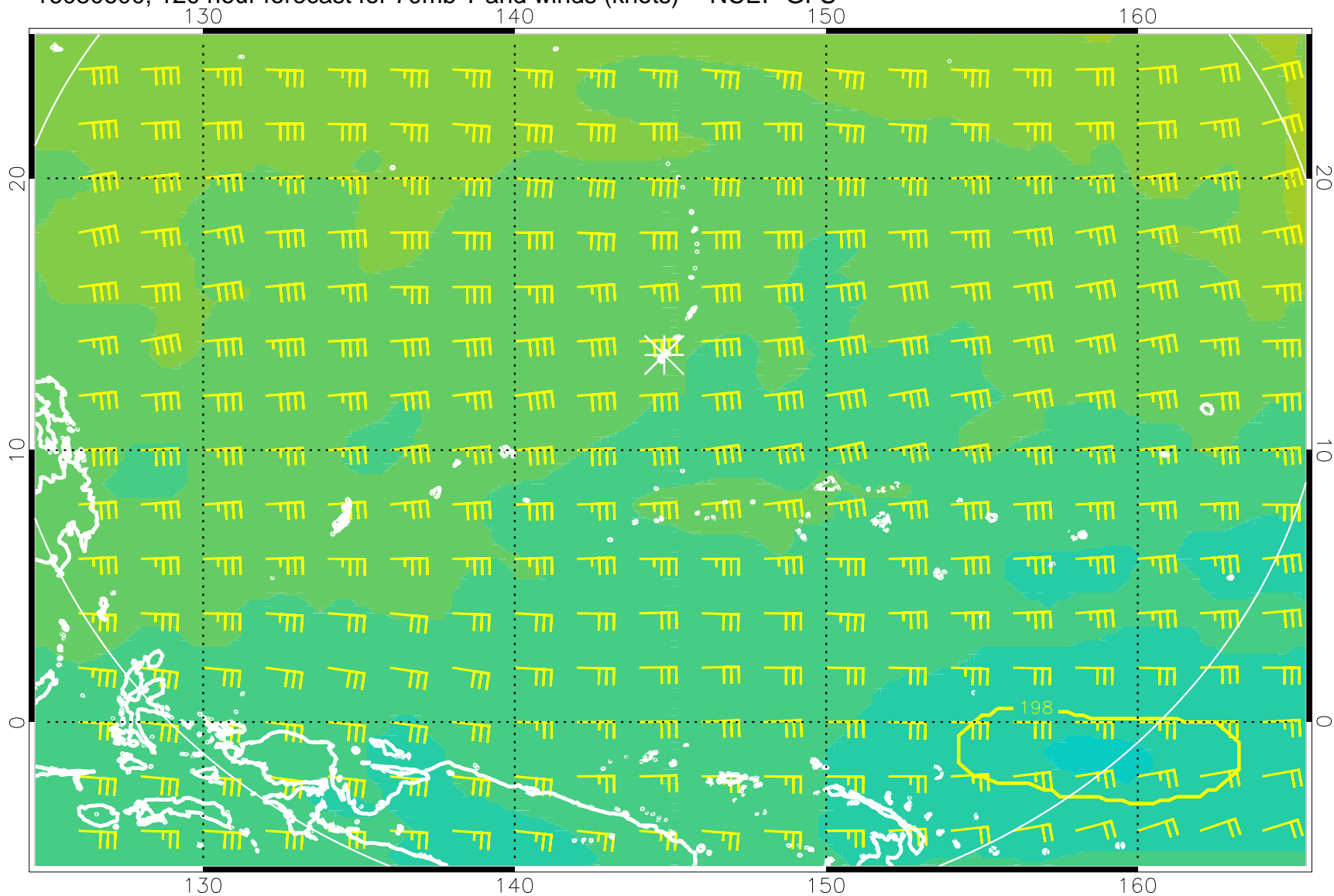
16080600, 120 hour forecast for 70mb T and winds (knots) -- NCEP GFS
