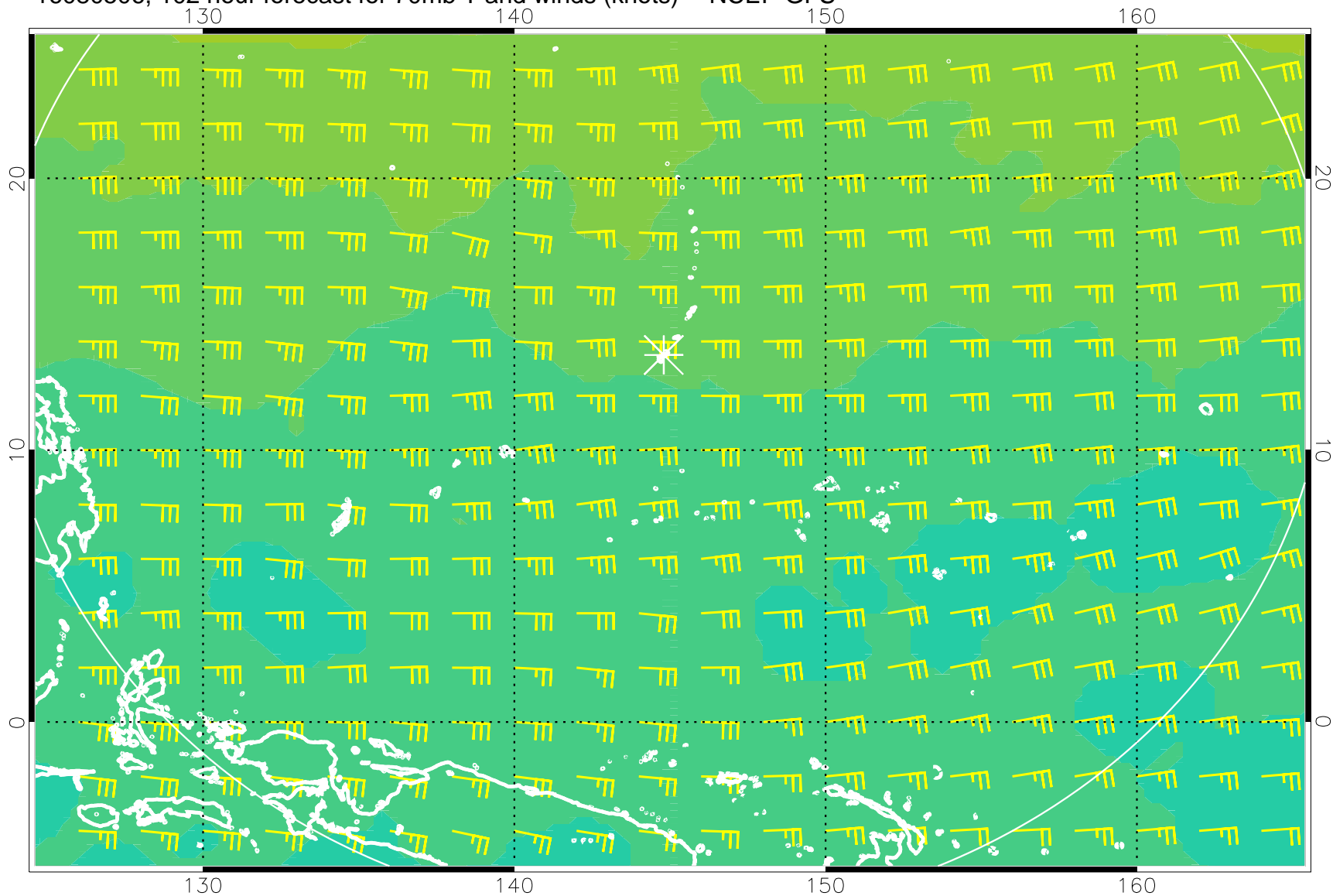
16080506, 102 hour forecast for 70mb T and winds (knots) -- NCEP GFS
