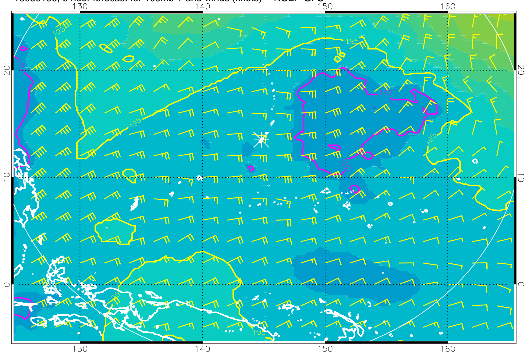
16080106, 6 hour forecast for 100mb T and winds (knots) -- NCEP GFS
