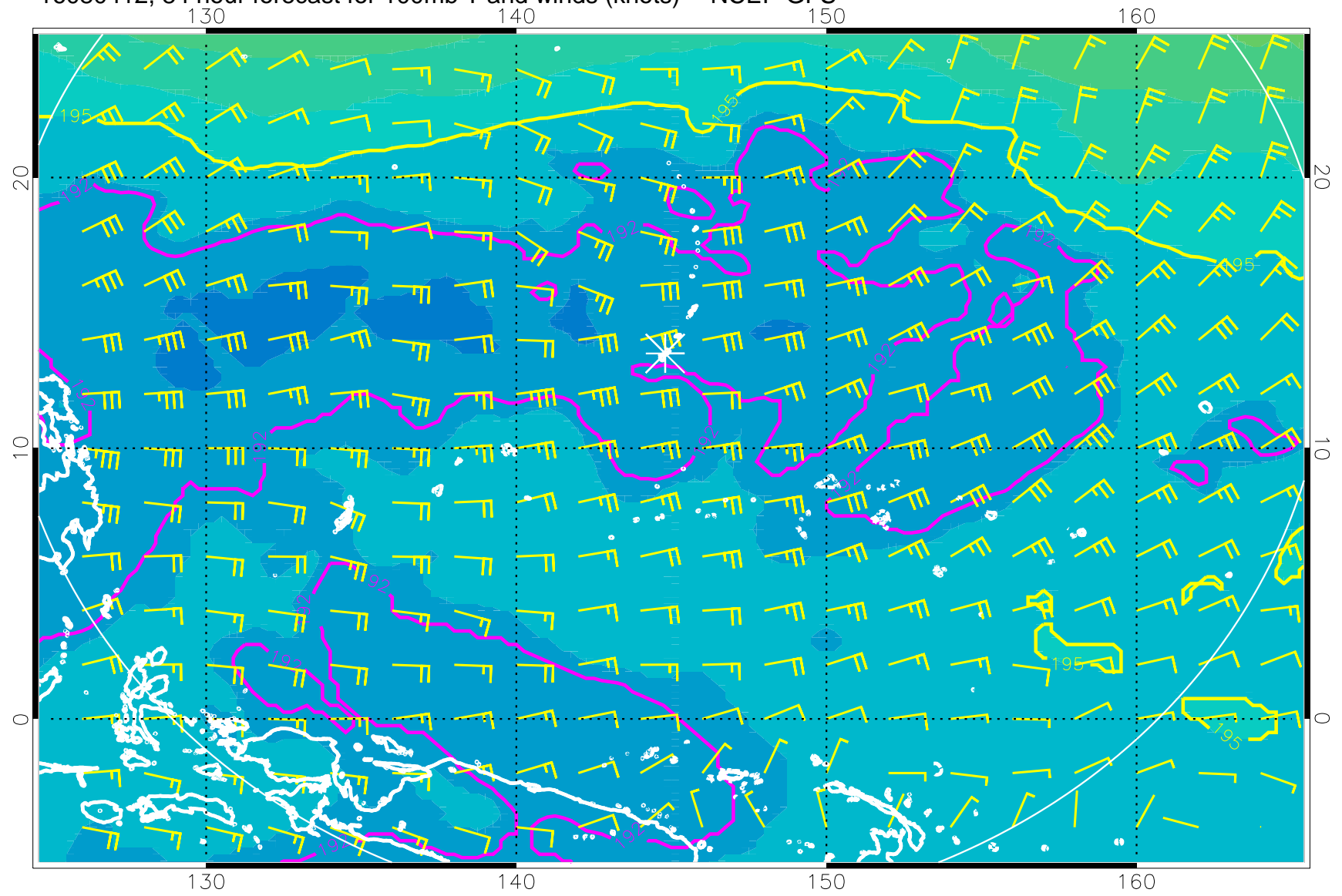
16080412, 84 hour forecast for 100mb T and winds (knots) -- NCEP GFS
