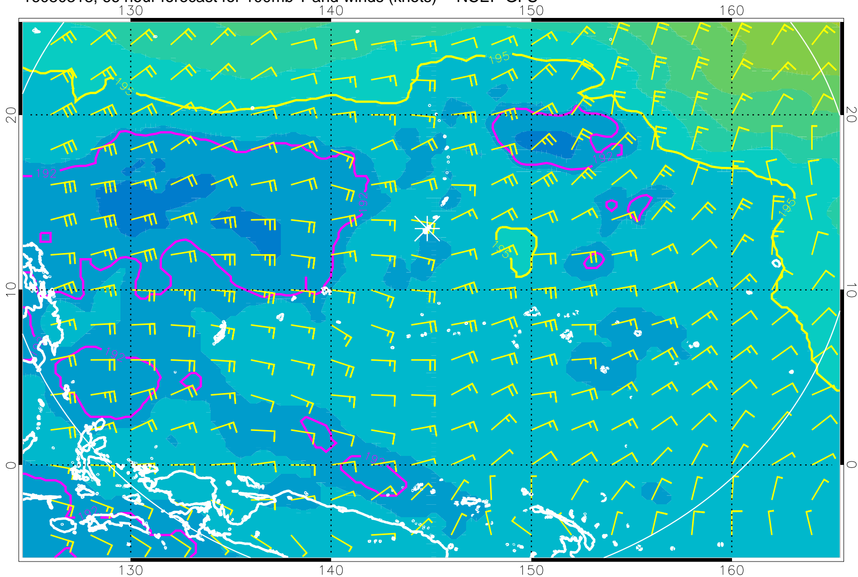
16080318, 66 hour forecast for 100mb T and winds (knots) -- NCEP GFS
