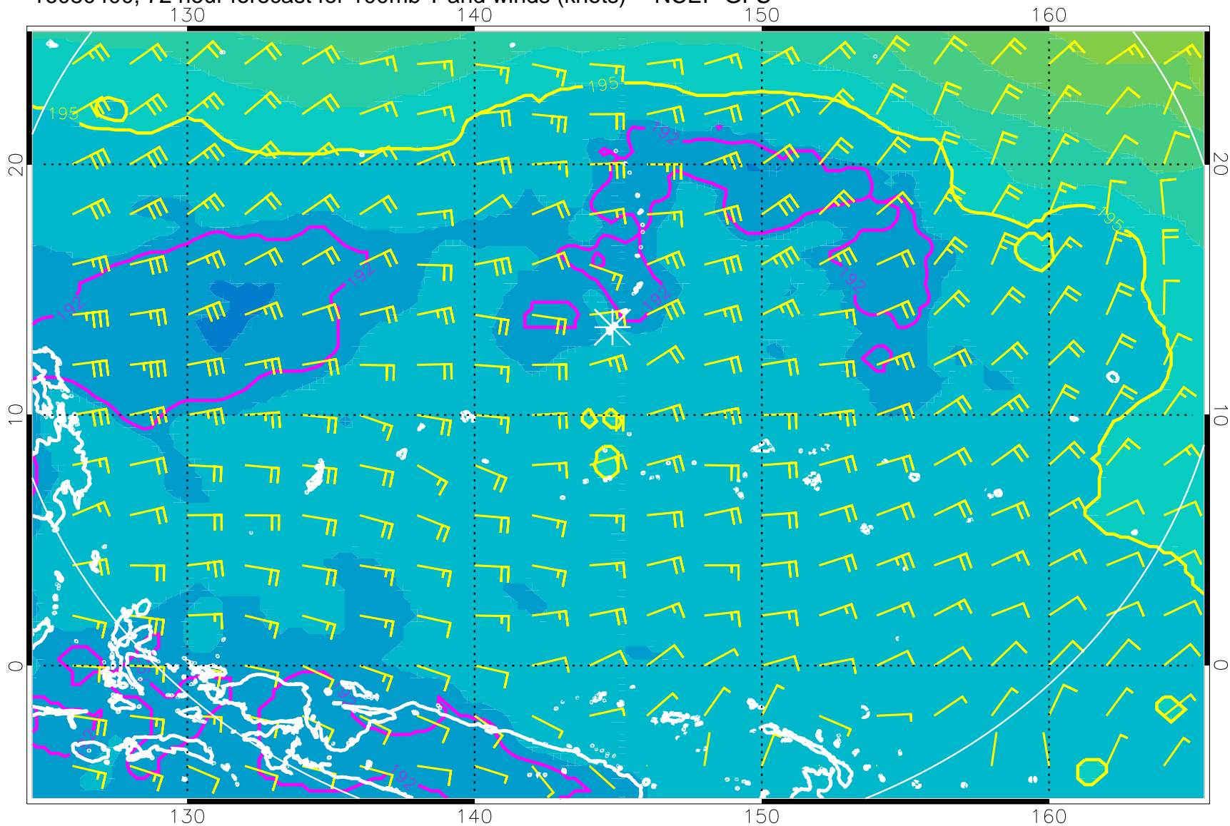
16080400, 72 hour forecast for 100mb T and winds (knots) -- NCEP GFS
