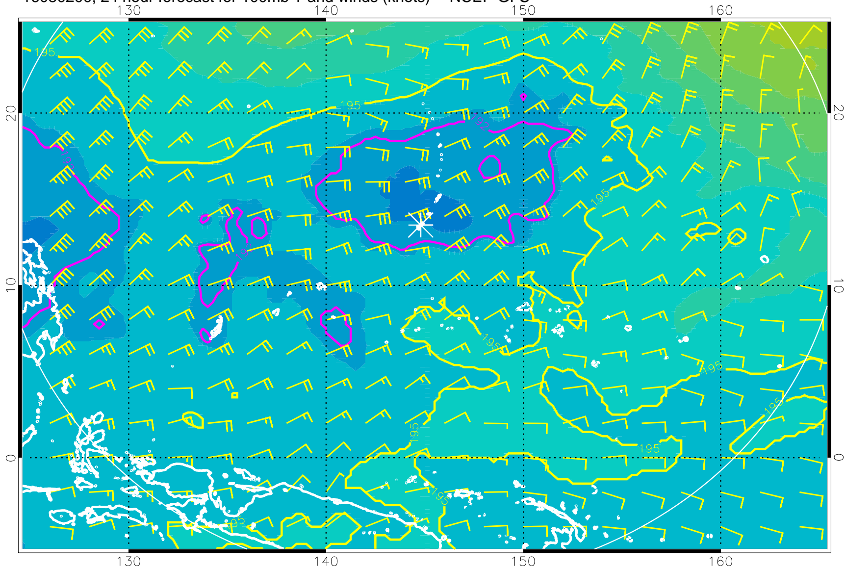
16080200, 24 hour forecast for 100mb T and winds (knots) -- NCEP GFS
