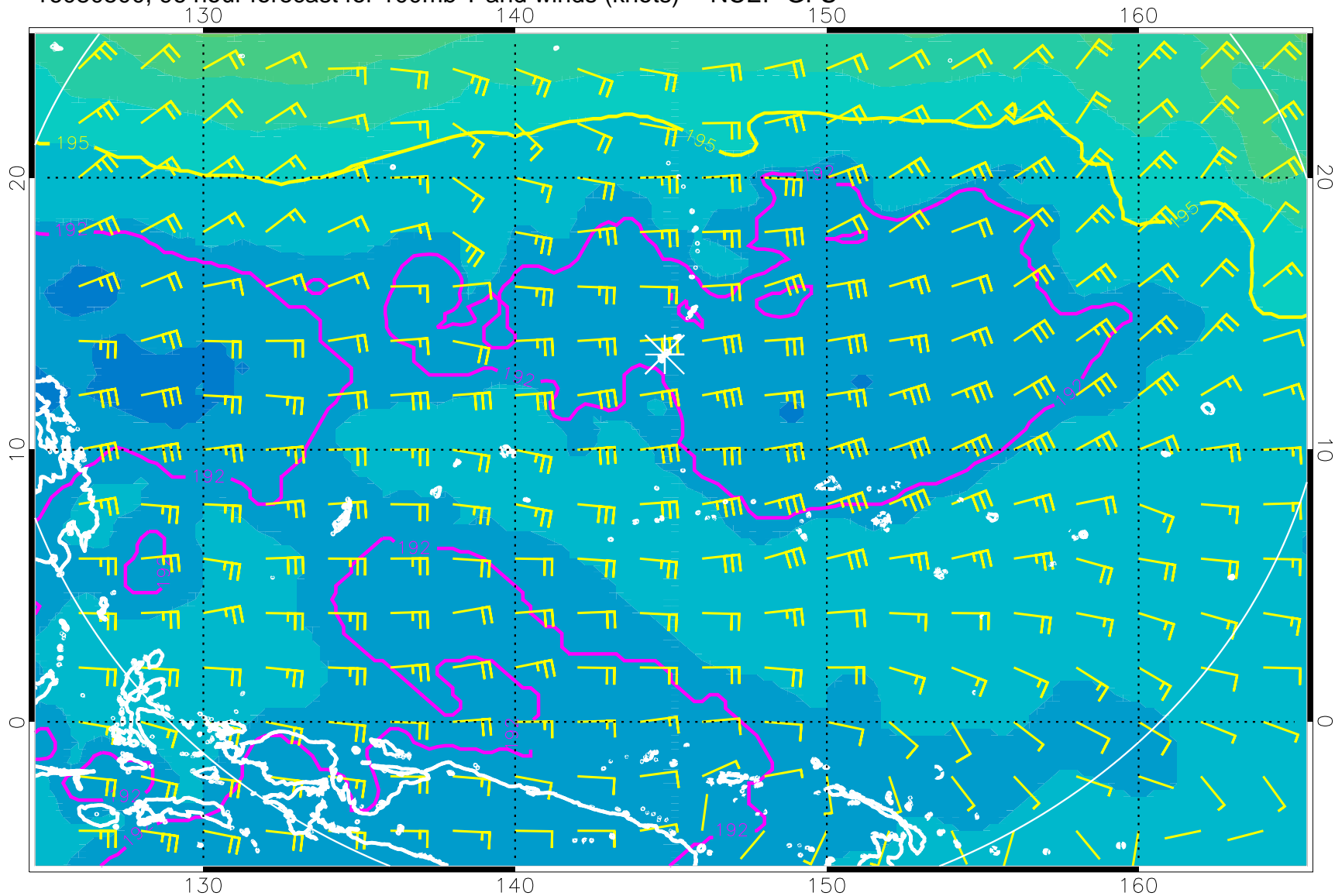
16080500, 96 hour forecast for 100mb T and winds (knots) -- NCEP GFS
