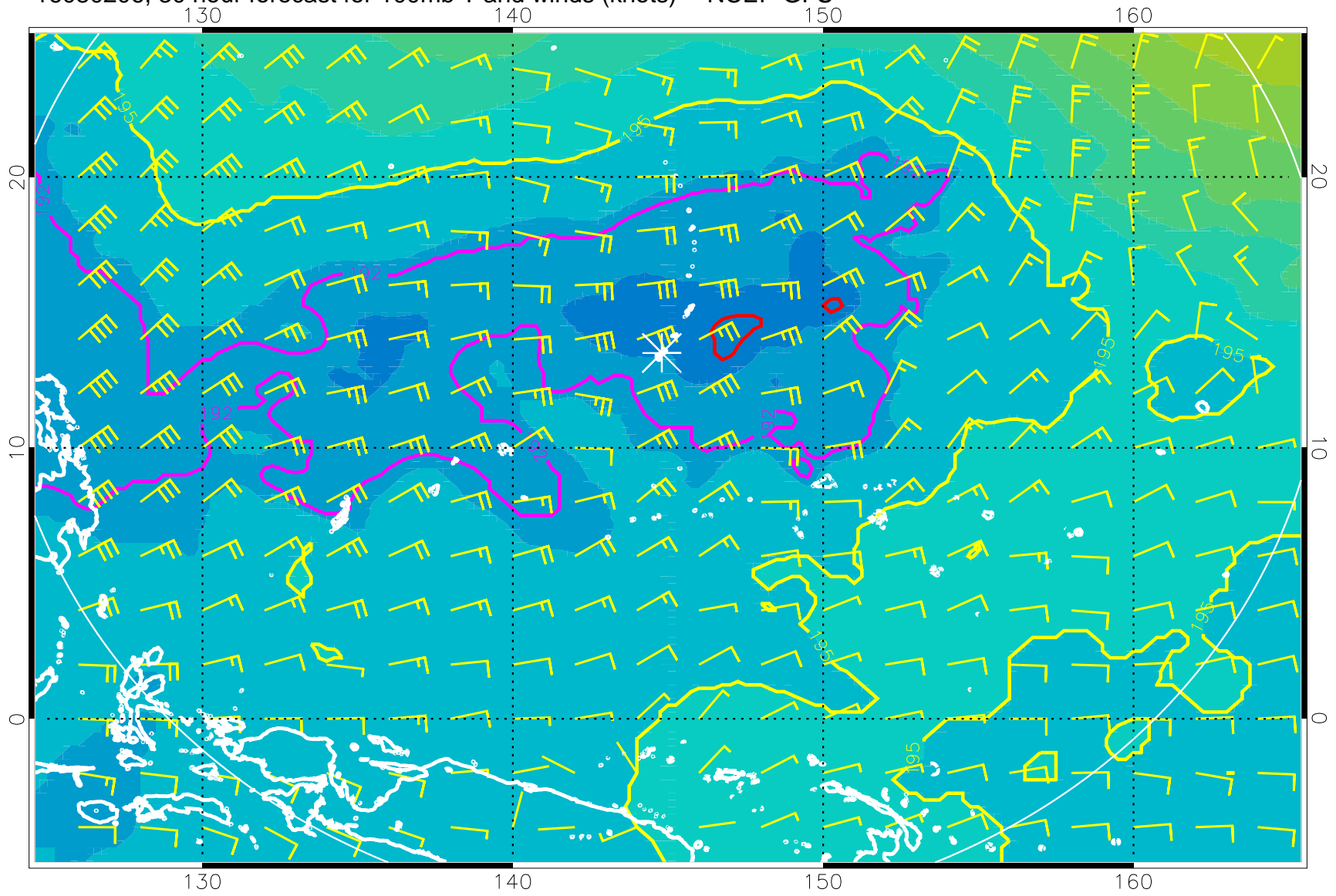
16080206, 30 hour forecast for 100mb T and winds (knots) -- NCEP GFS
