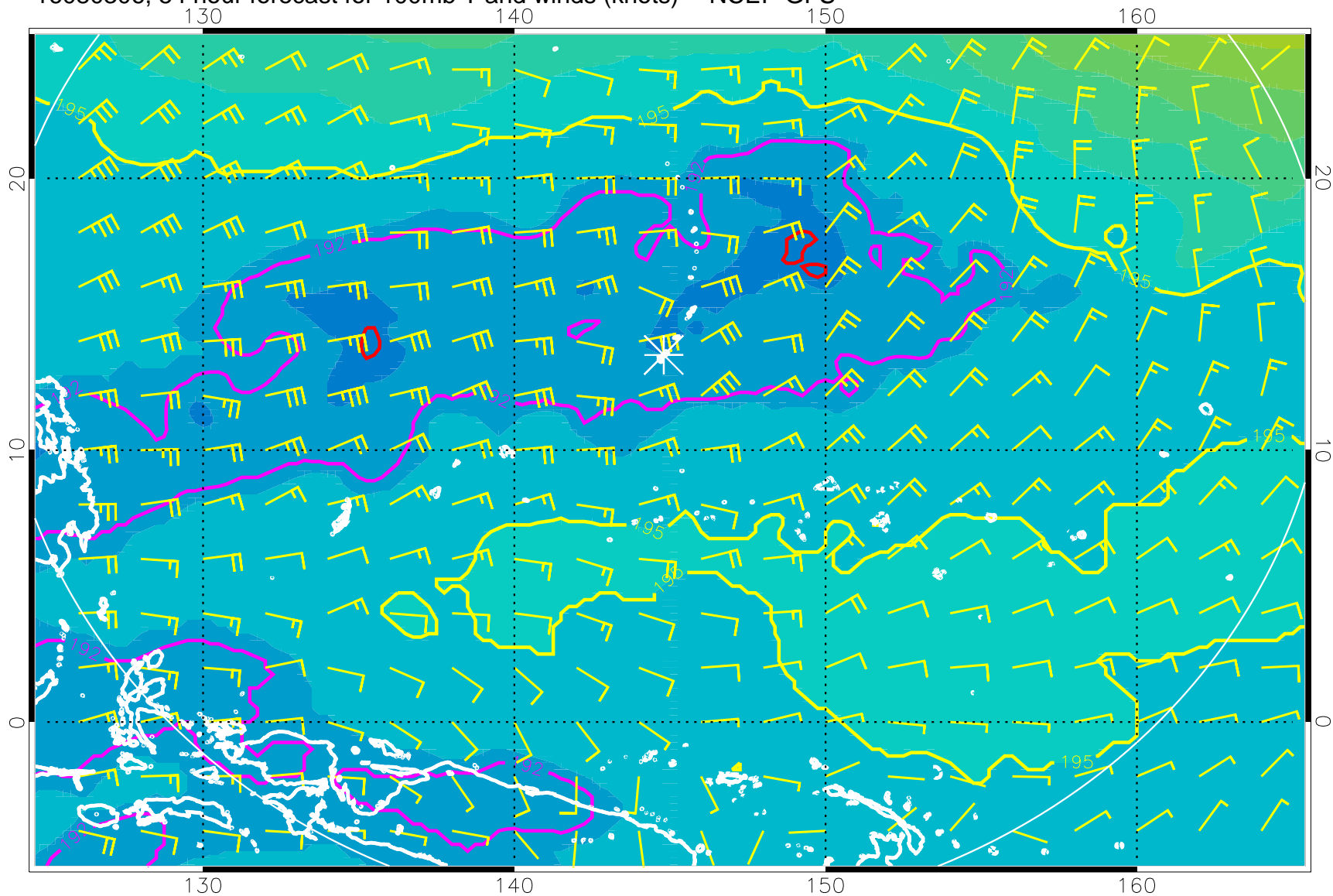
16080306, 54 hour forecast for 100mb T and winds (knots) -- NCEP GFS
