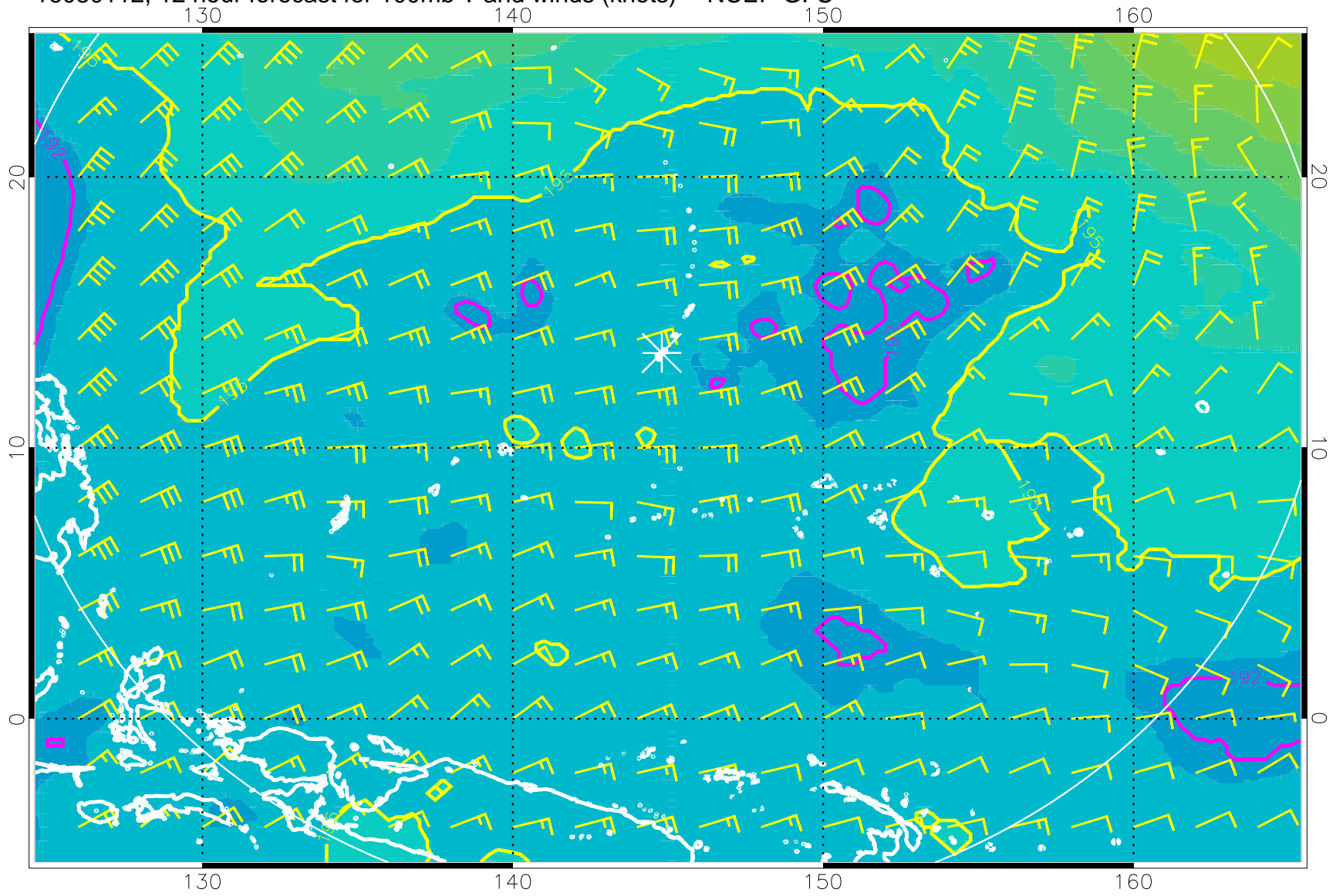
16080112, 12 hour forecast for 100mb T and winds (knots) -- NCEP GFS
