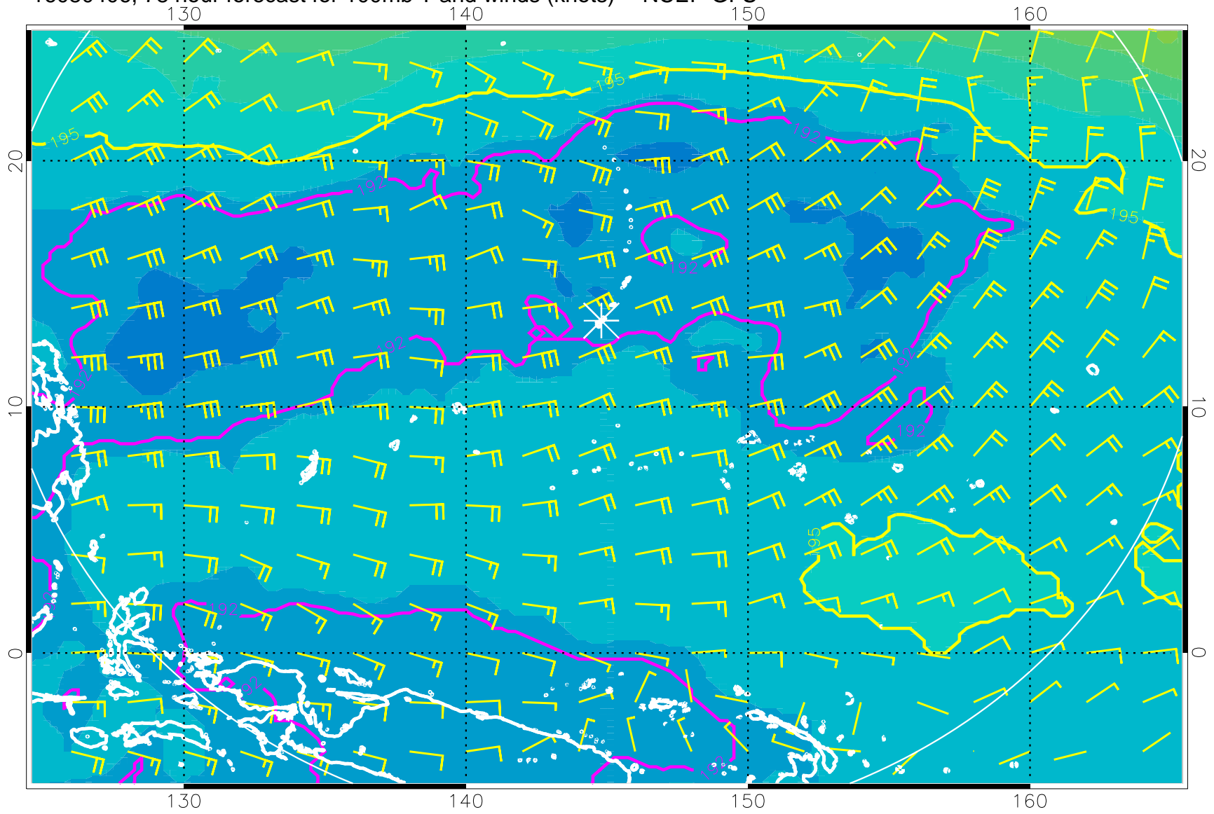
16080406, 78 hour forecast for 100mb T and winds (knots) -- NCEP GFS
