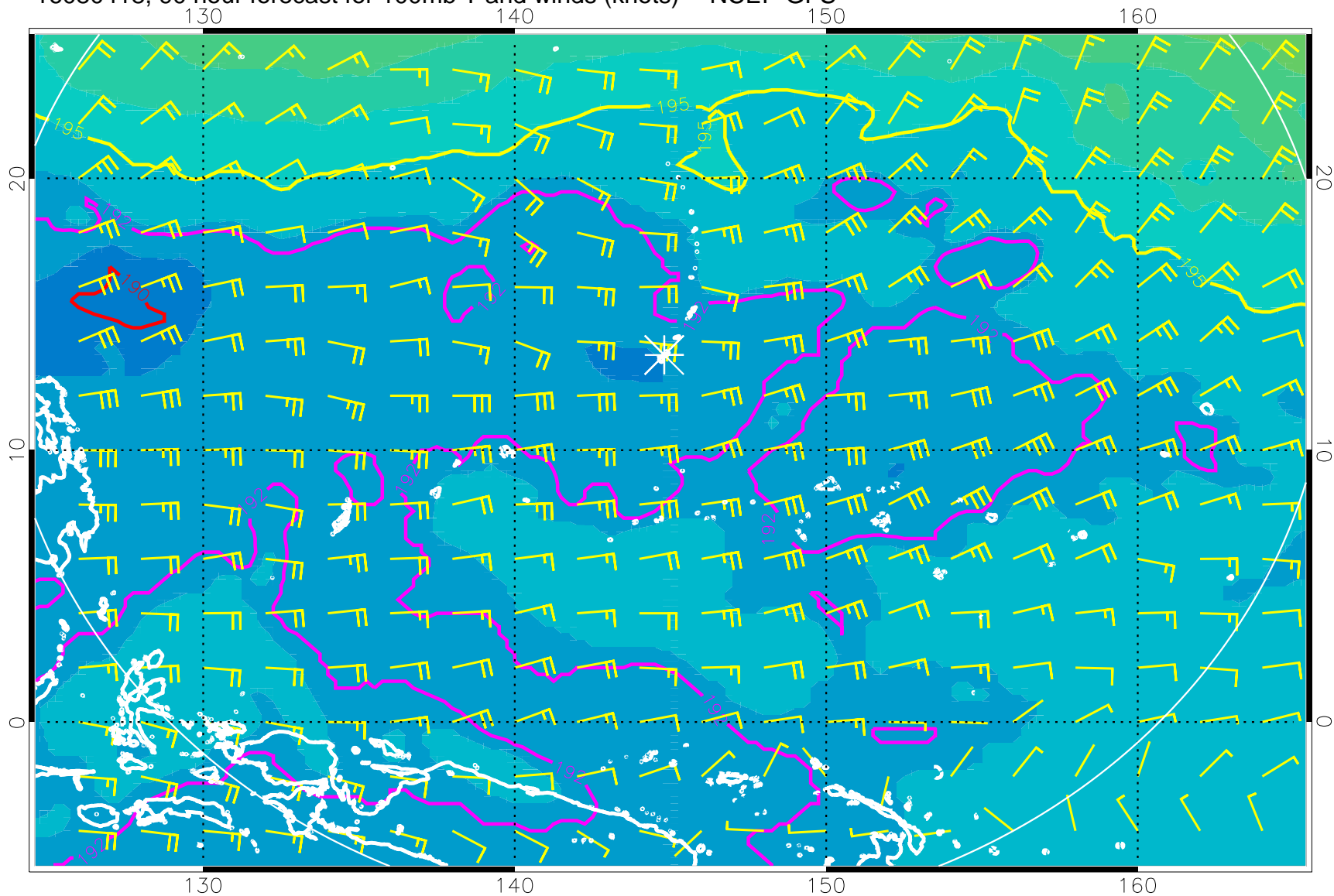
16080418, 90 hour forecast for 100mb T and winds (knots) -- NCEP GFS
