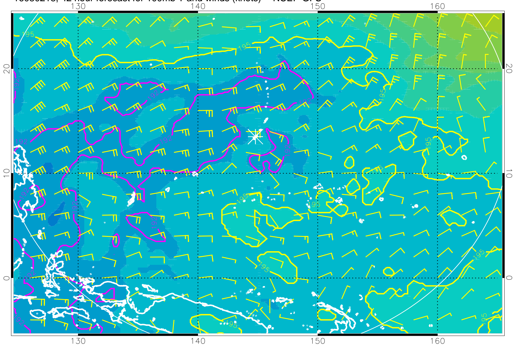
16080218, 42 hour forecast for 100mb T and winds (knots) -- NCEP GFS
