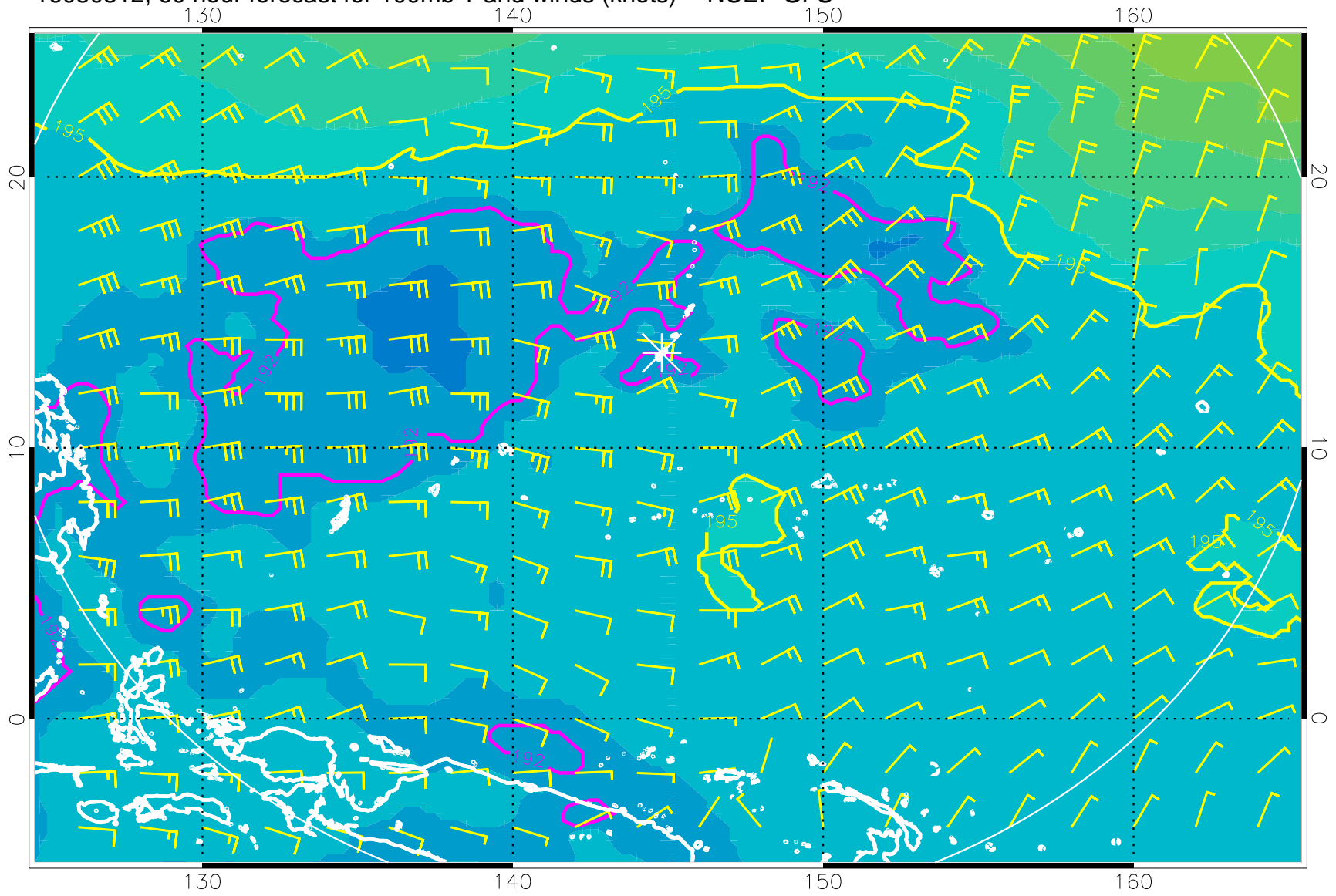
16080312, 60 hour forecast for 100mb T and winds (knots) -- NCEP GFS
