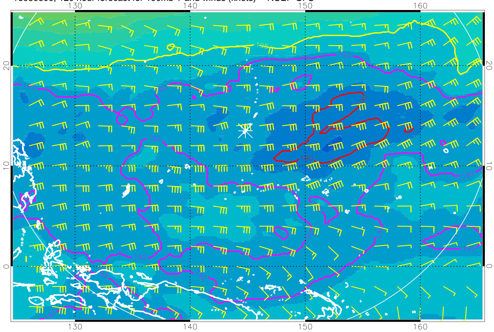
16080600, 120 hour forecast for 100mb T and winds (knots) -- NCEP GFS
