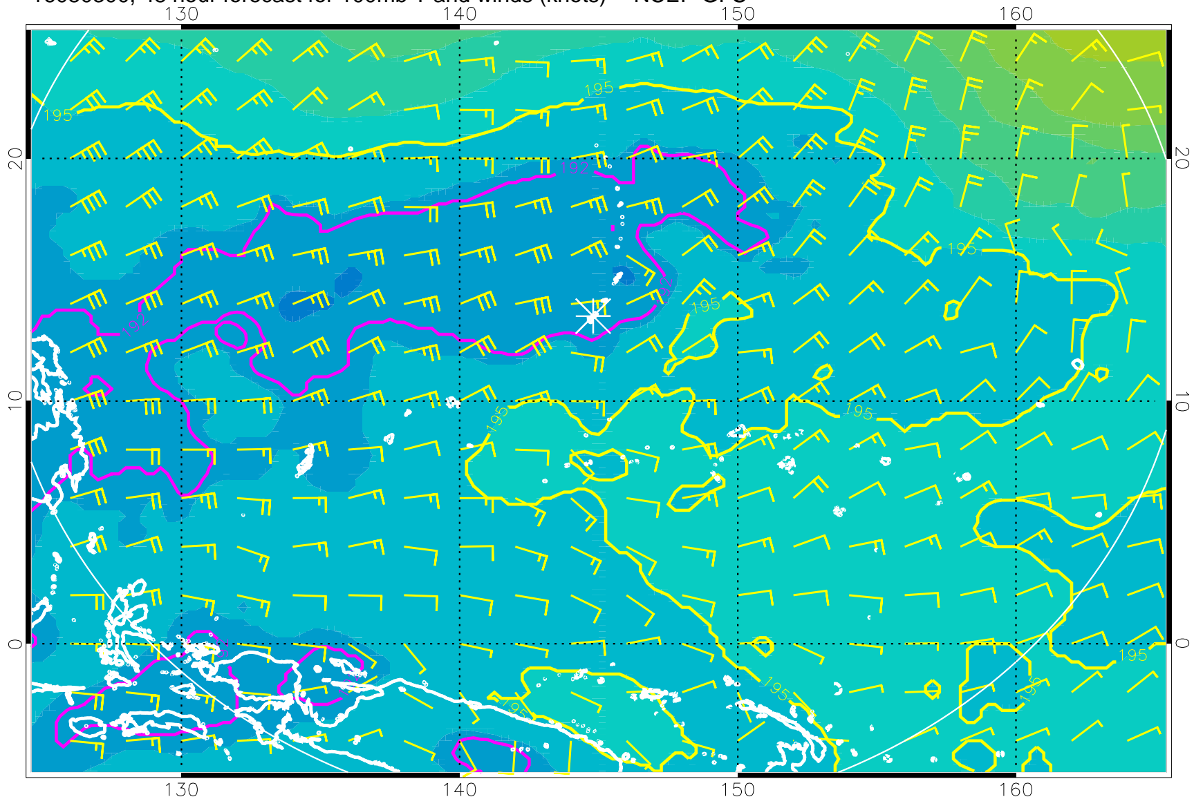
16080300, 48 hour forecast for 100mb T and winds (knots) -- NCEP GFS
