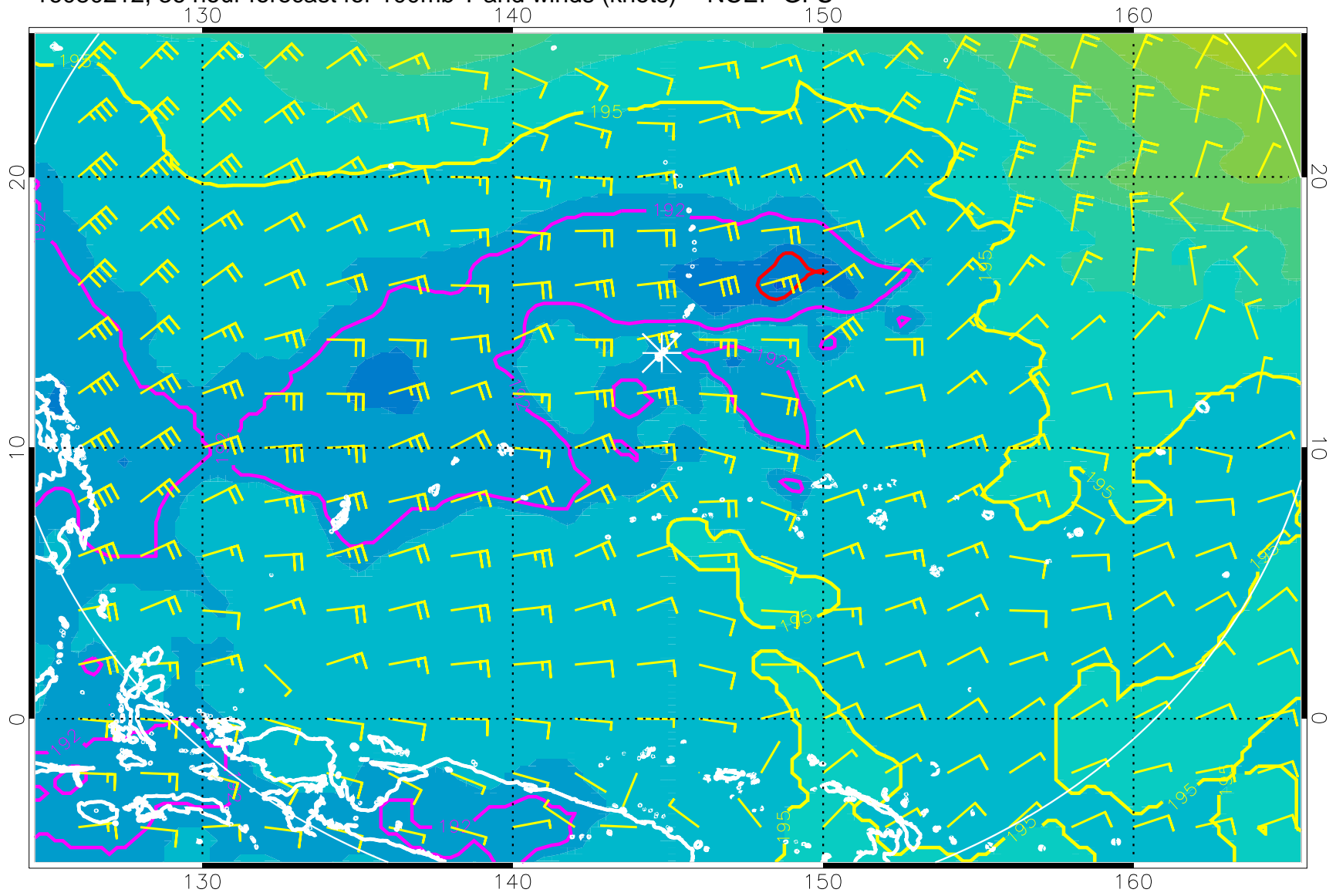
16080212, 36 hour forecast for 100mb T and winds (knots) -- NCEP GFS
