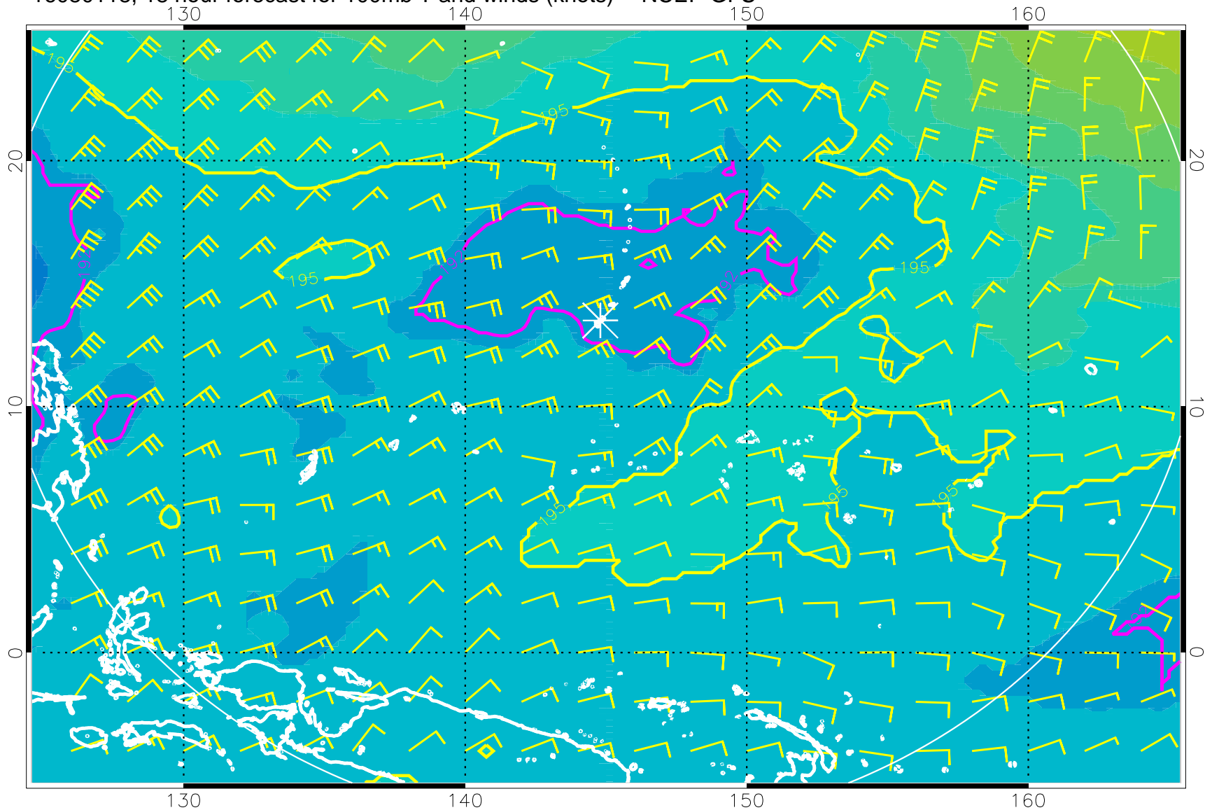
16080118, 18 hour forecast for 100mb T and winds (knots) -- NCEP GFS
