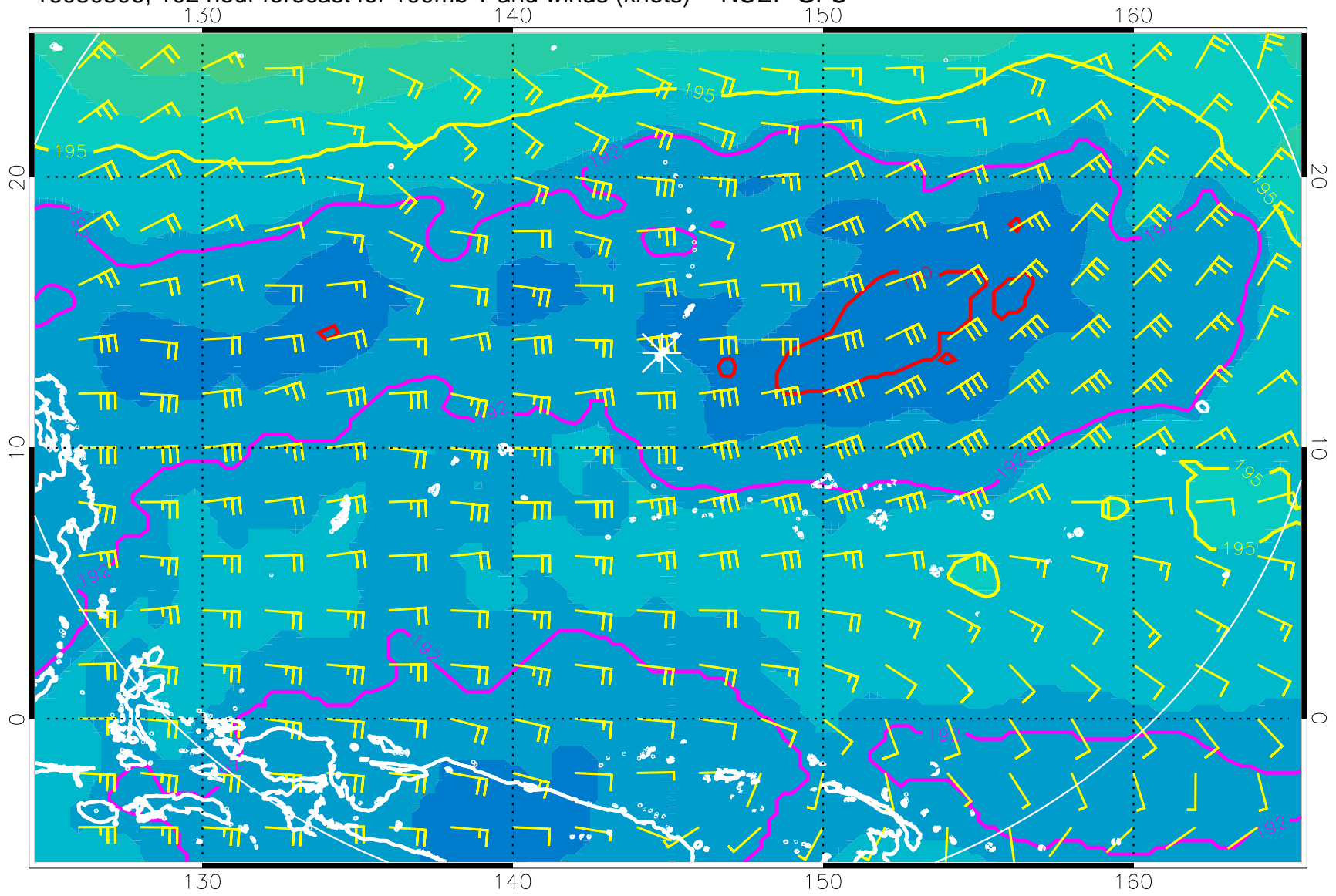
16080506, 102 hour forecast for 100mb T and winds (knots) -- NCEP GFS
