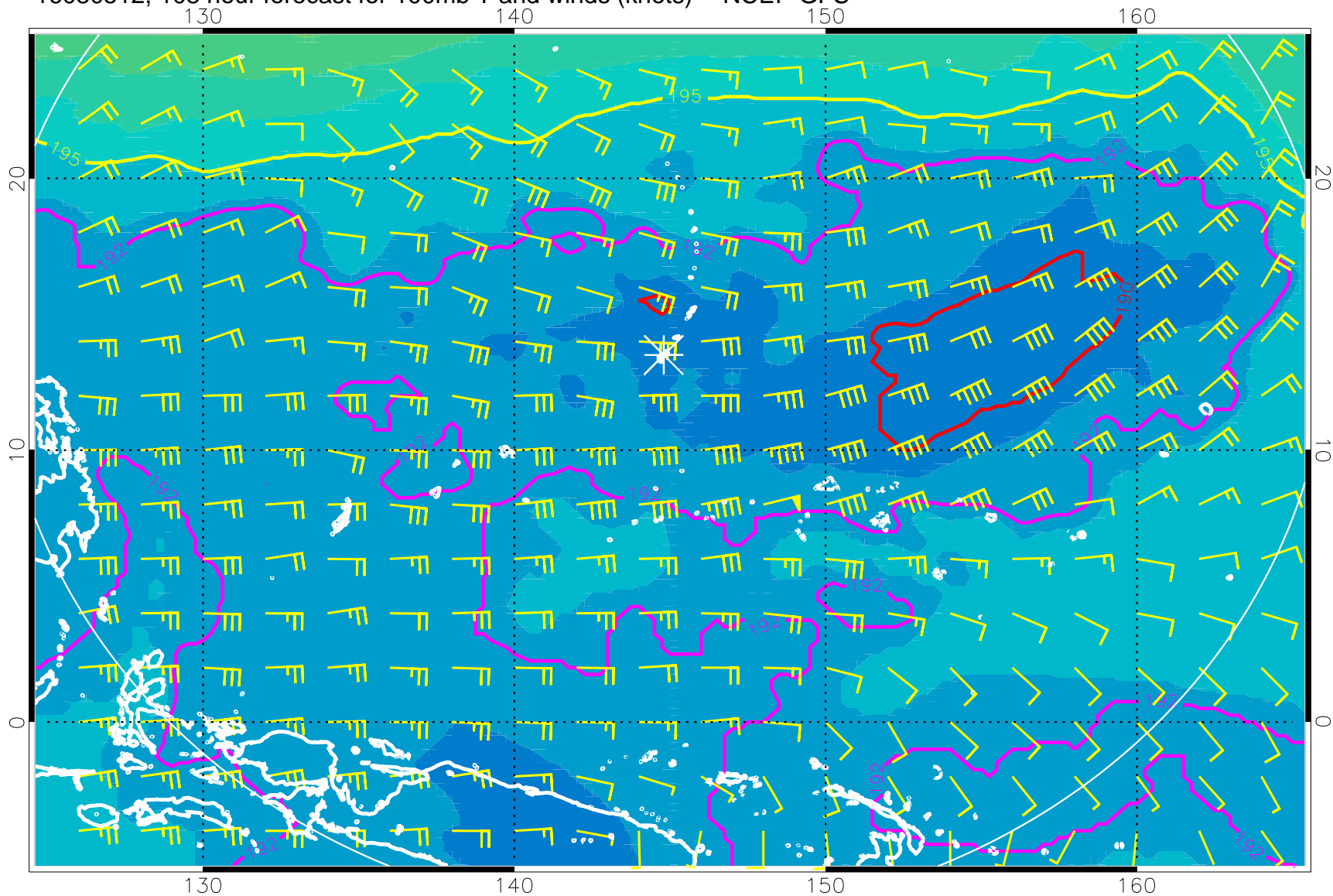
16080512, 108 hour forecast for 100mb T and winds (knots) -- NCEP GFS
