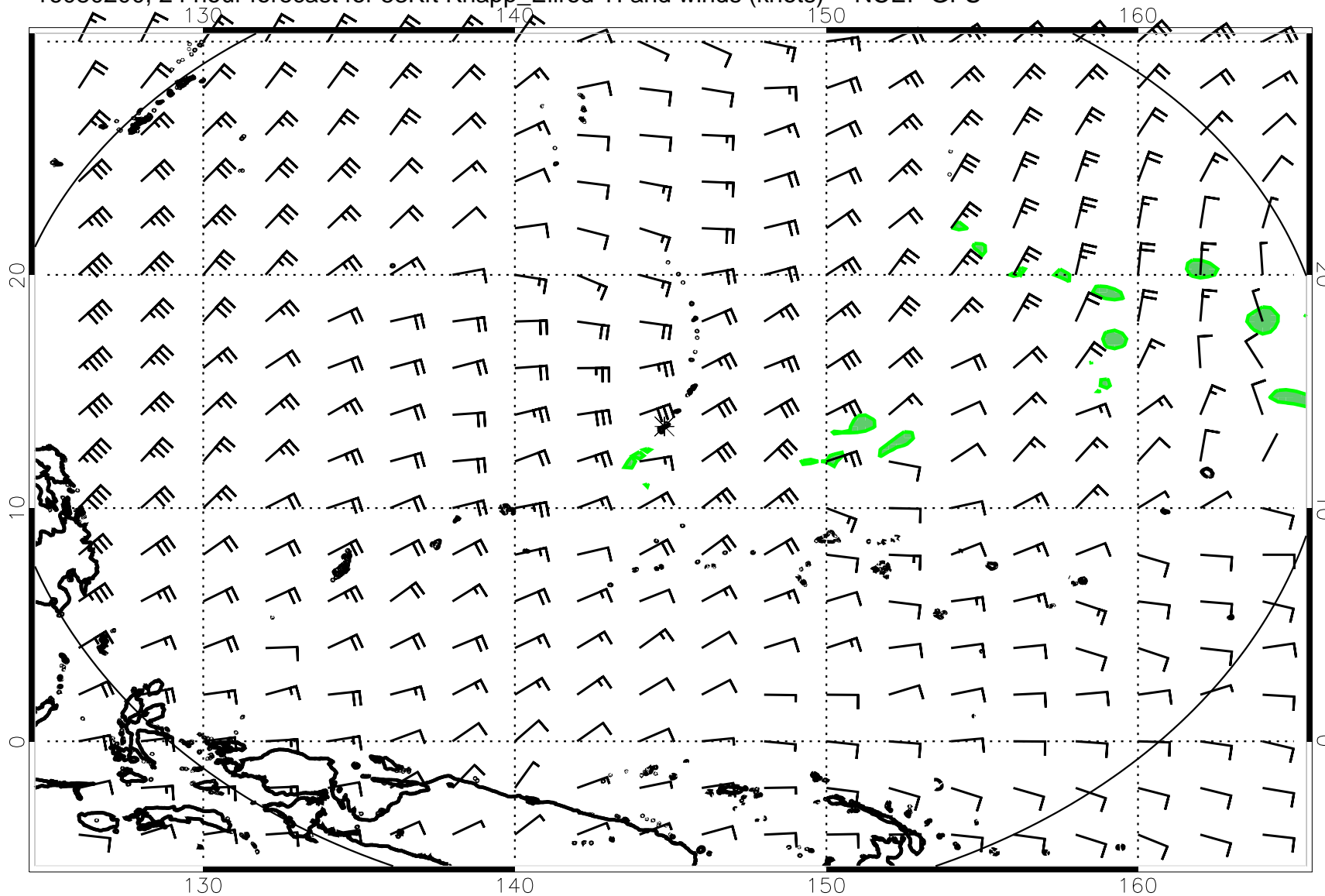
16080200, 24 hour forecast for 53Kft Knapp_Ellrod TI and winds (knots) -- NCEP GFS
