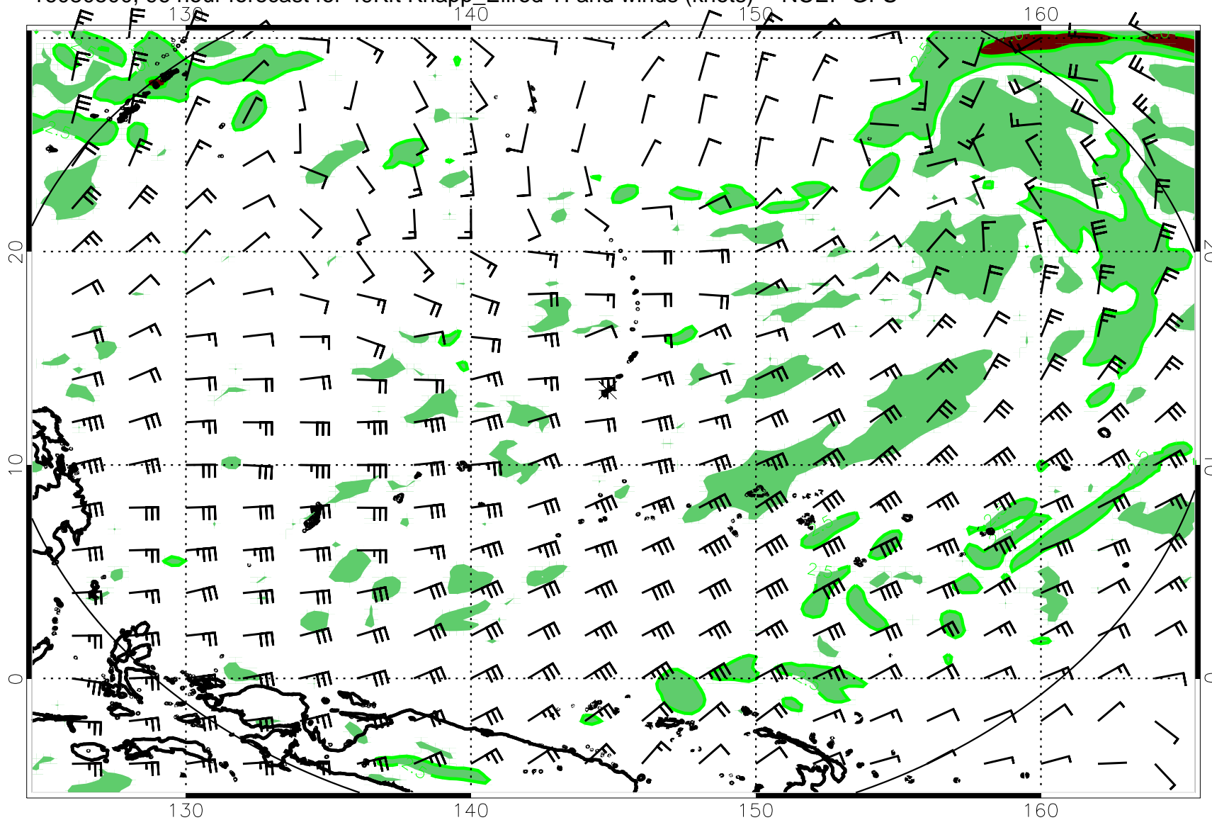
16080500, 96 hour forecast for 49Kft Knapp_Ellrod TI and winds (knots) -- NCEP GFS
