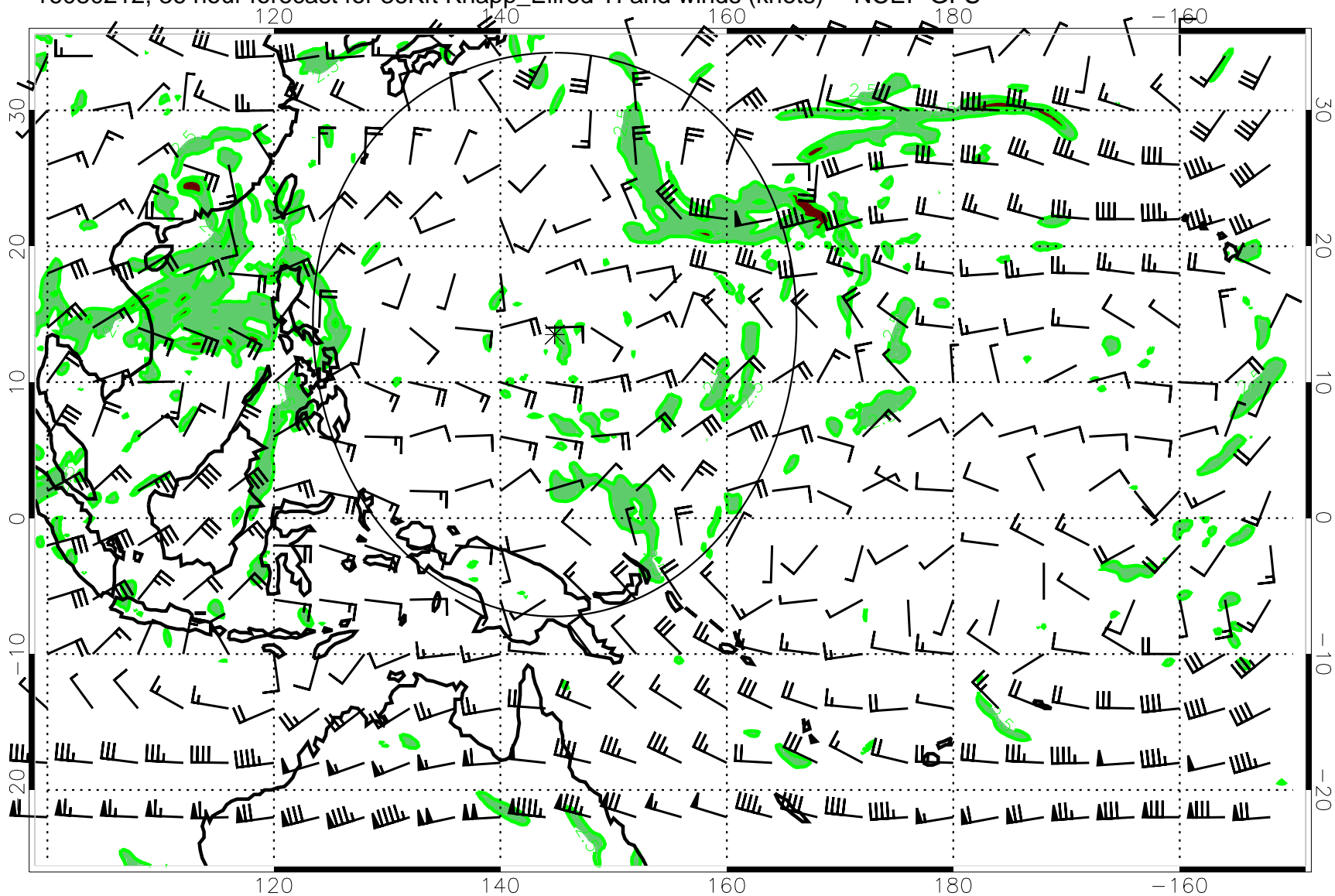
16080212, 36 hour forecast for 36Kft Knapp_Ellrod TI and winds (knots) -- NCEP GFS
