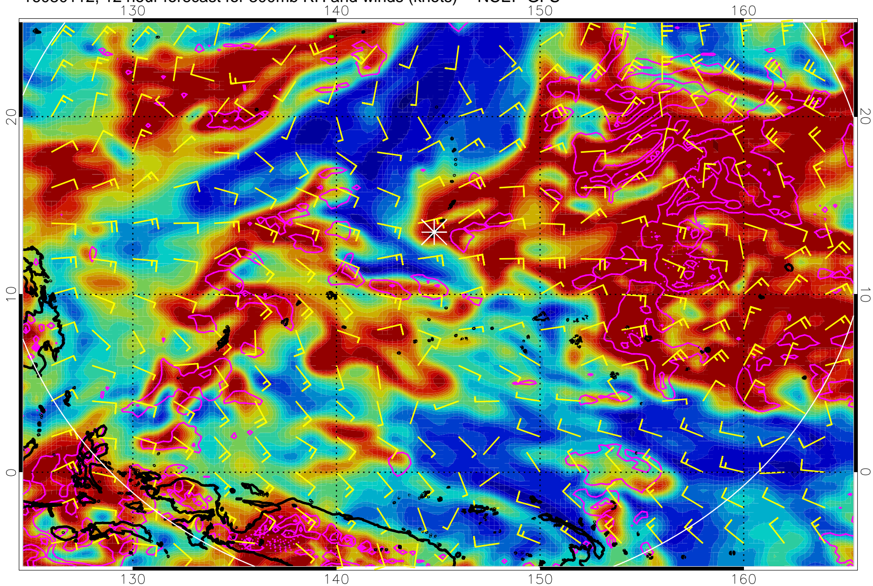
16080112, 12 hour forecast for 300mb RH and winds (knots) -- NCEP GFS
