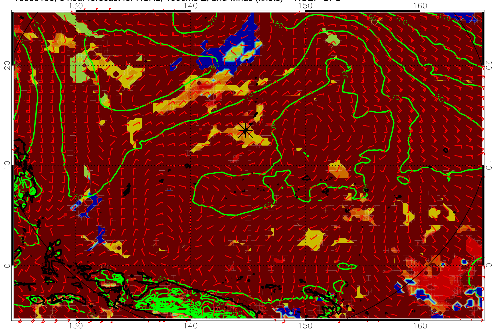
16080106, 6 hour forecast for HCAL, 1000mb Z, and winds (knots) -- NCEP GFS
