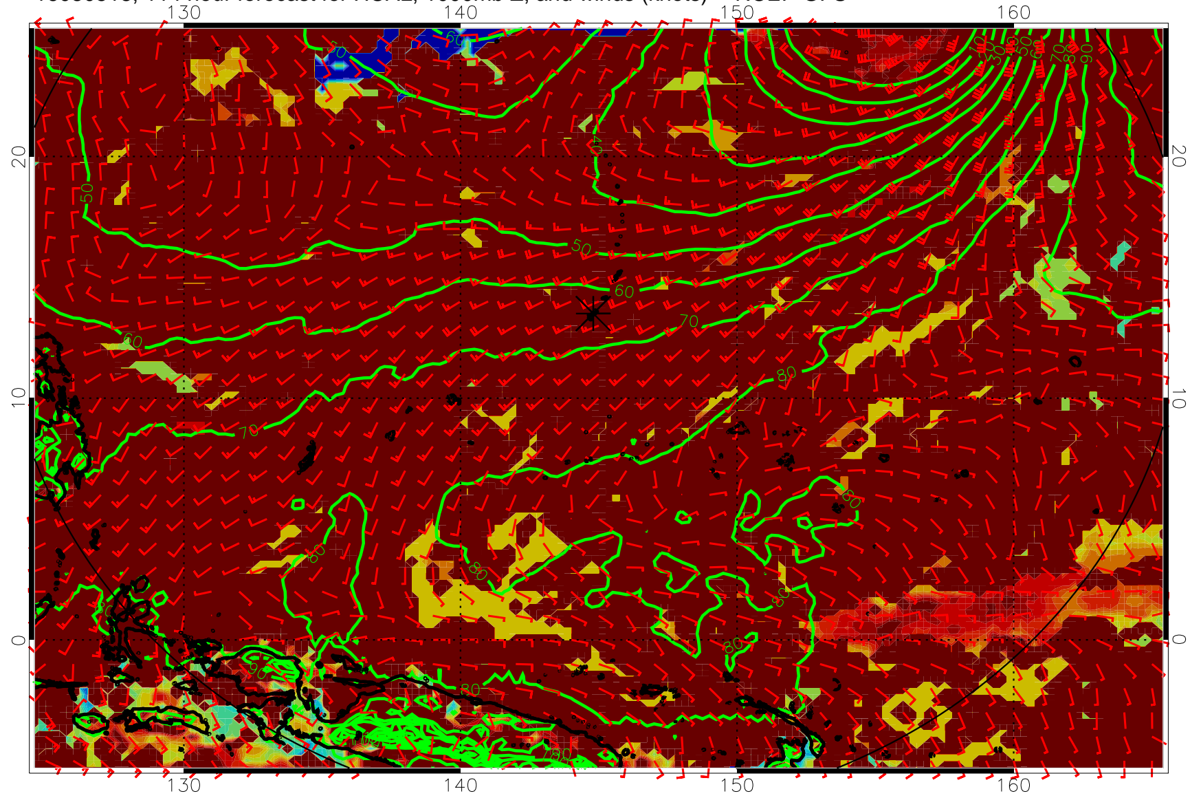
16080518, 114 hour forecast for HCAL, 1000mb Z, and winds (knots) -- NCEP GFS
