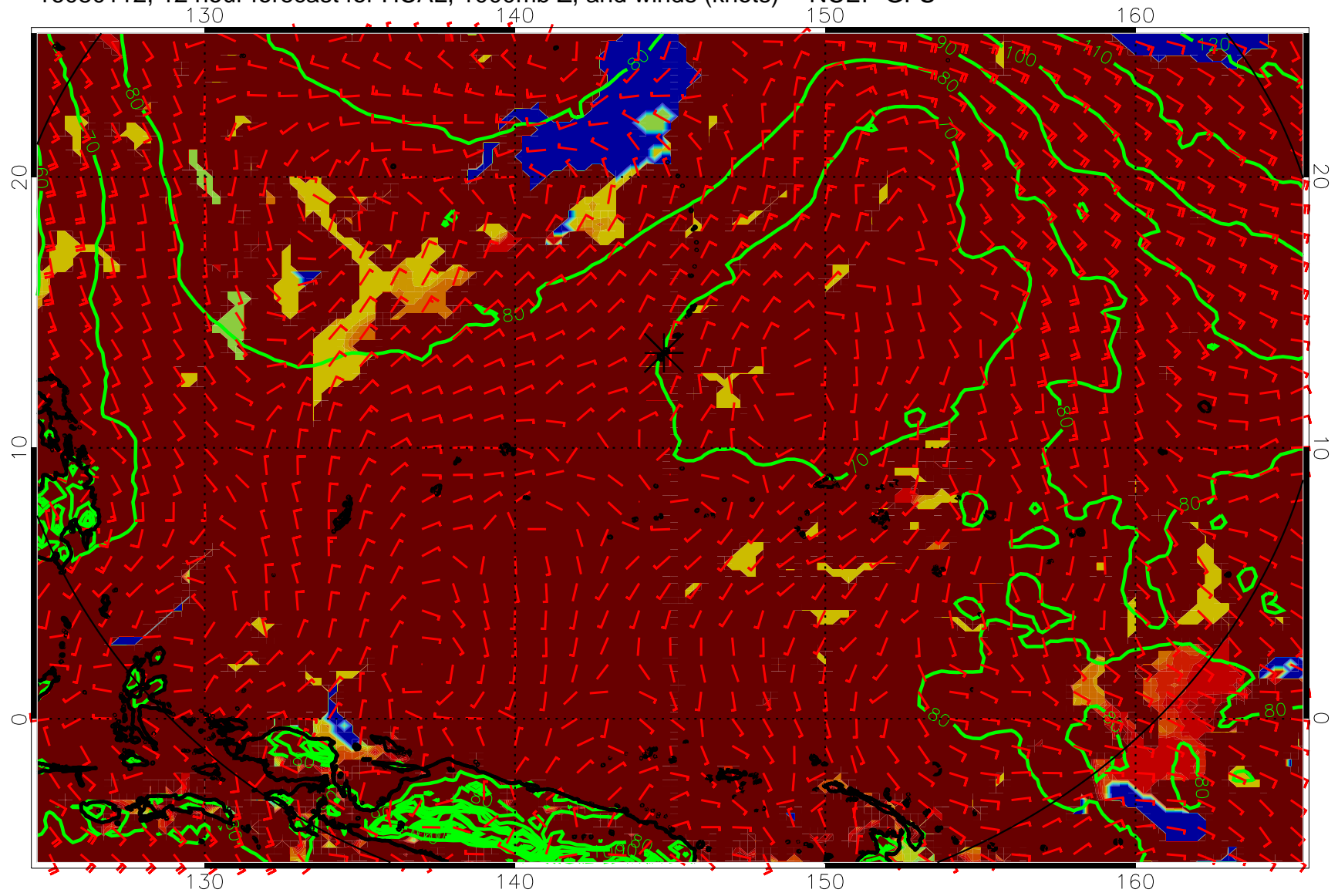
16080112, 12 hour forecast for HCAL, 1000mb Z, and winds (knots) -- NCEP GFS
