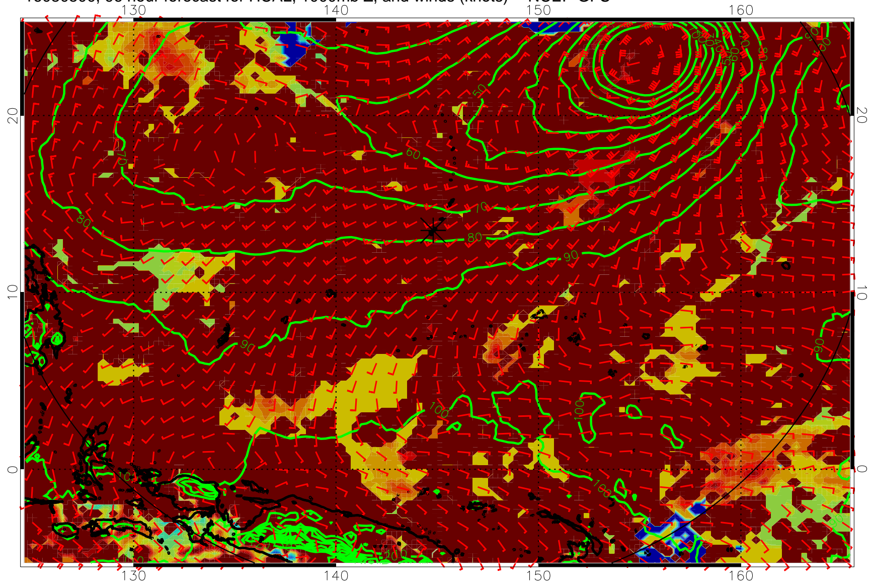
16080500, 96 hour forecast for HCAL, 1000mb Z, and winds (knots) -- NCEP GFS
