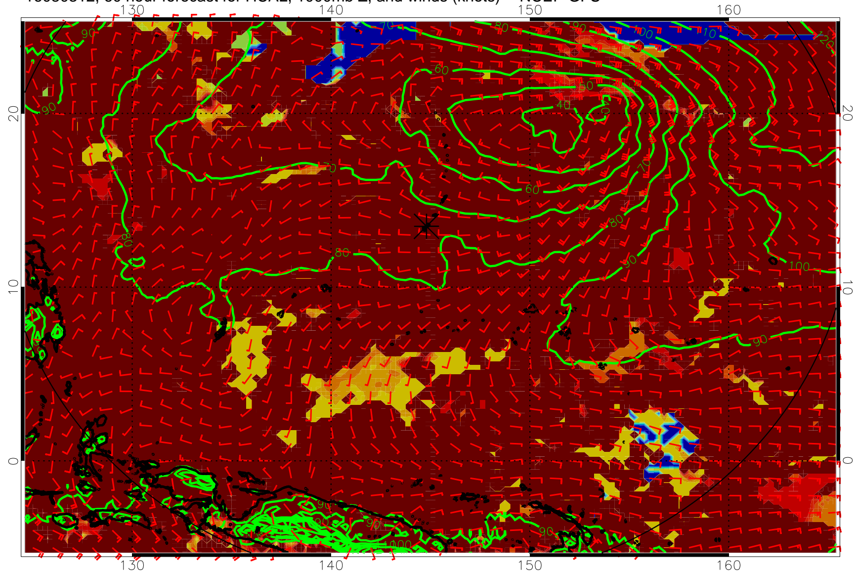
16080312, 60 hour forecast for HCAL, 1000mb Z, and winds (knots) -- NCEP GFS
