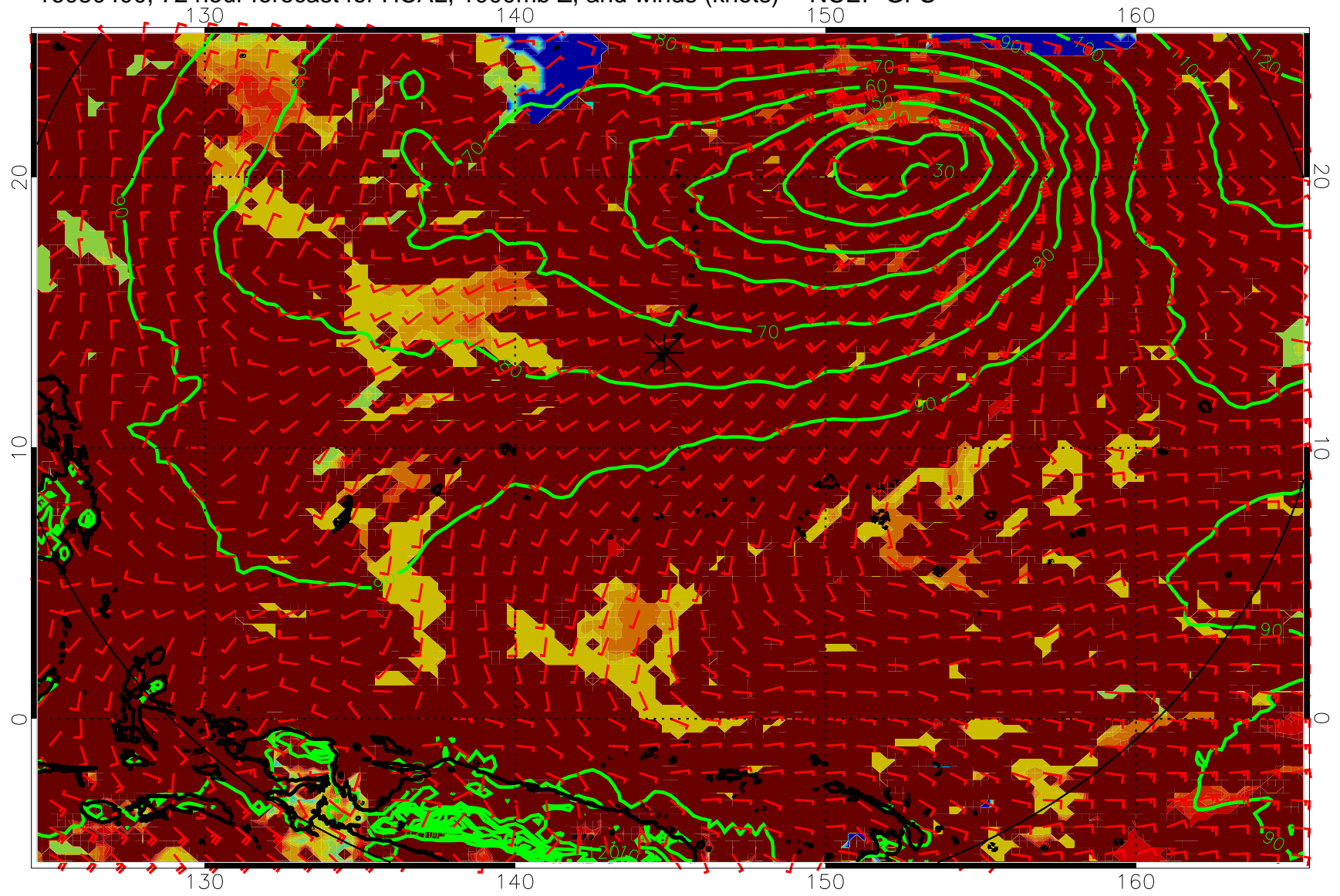
16080400, 72 hour forecast for HCAL, 1000mb Z, and winds (knots) -- NCEP GFS
