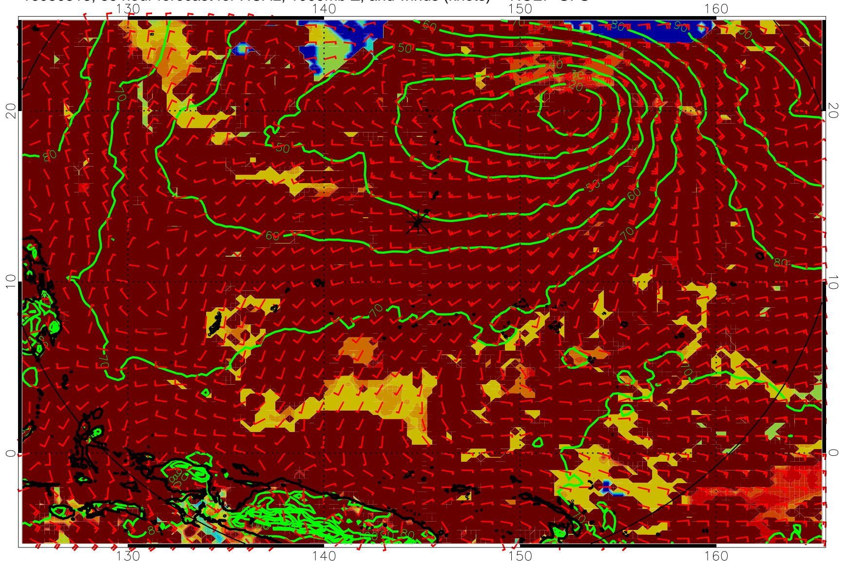
16080318, 66 hour forecast for HCAL, 1000mb Z, and winds (knots) -- NCEP GFS
