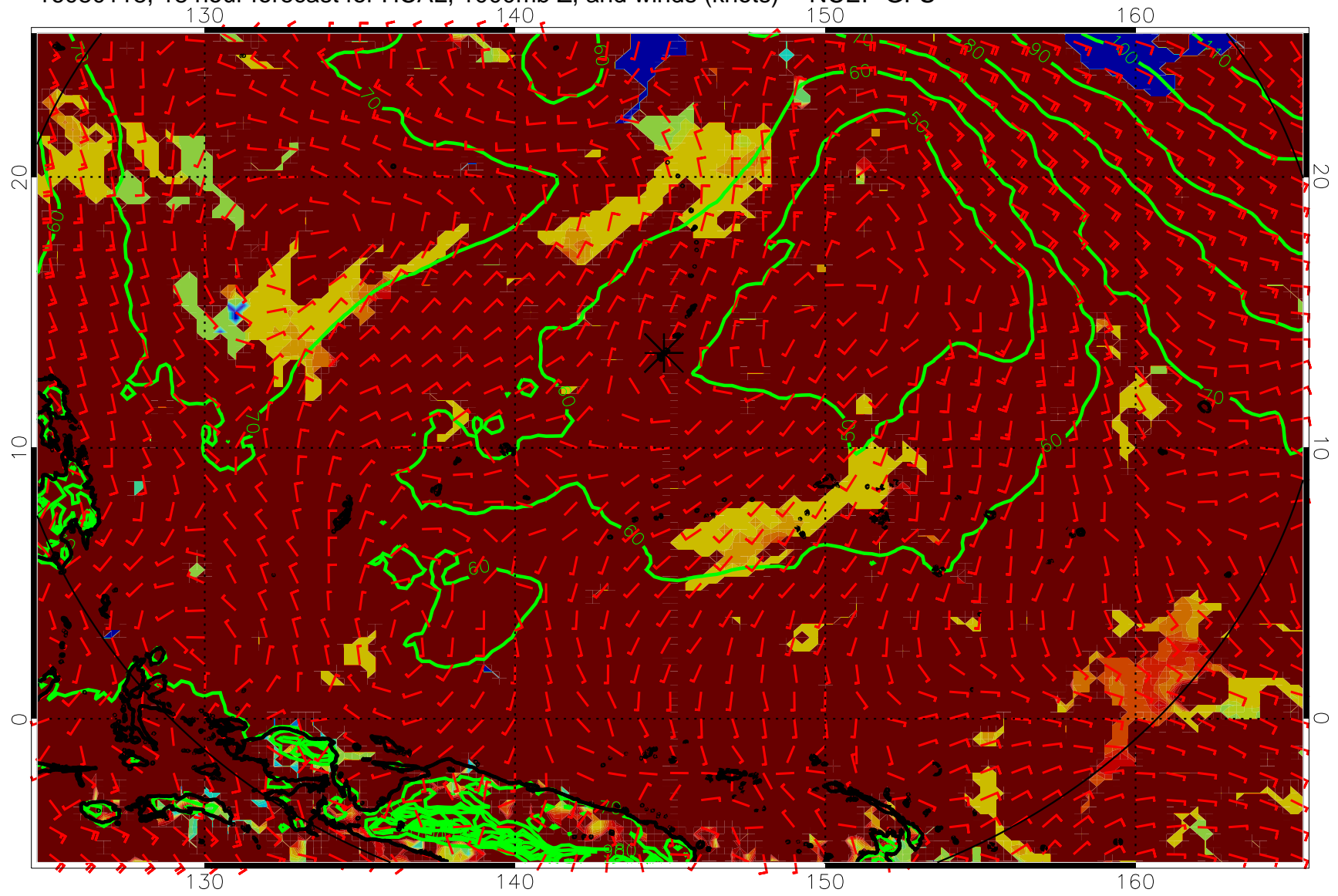
16080118, 18 hour forecast for HCAL, 1000mb Z, and winds (knots) -- NCEP GFS
