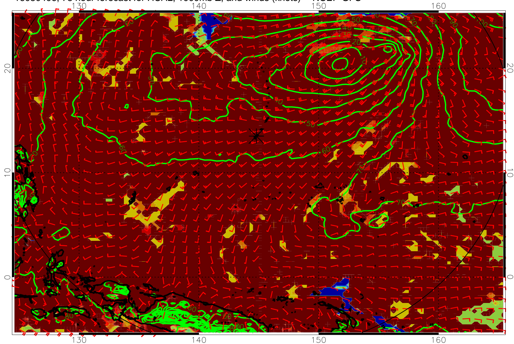
16080406, 78 hour forecast for HCAL, 1000mb Z, and winds (knots) -- NCEP GFS
