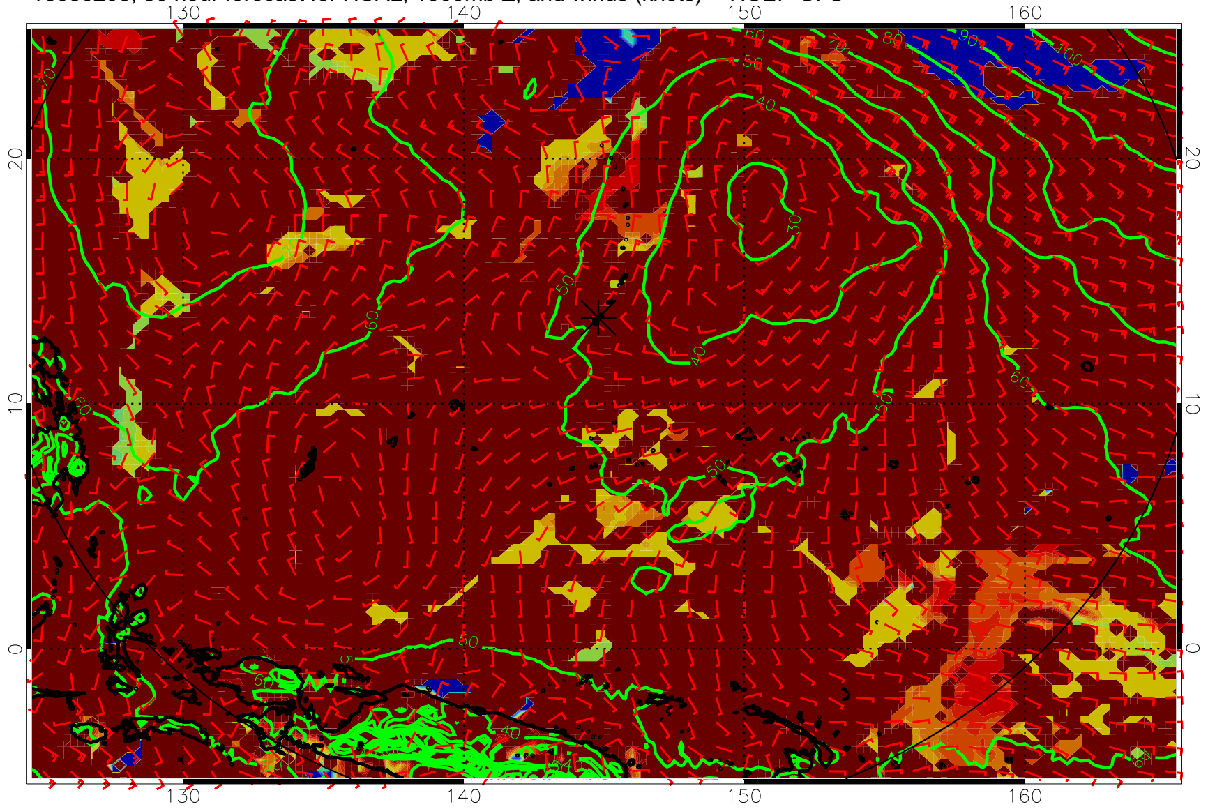
16080206, 30 hour forecast for HCAL, 1000mb Z, and winds (knots) -- NCEP GFS
