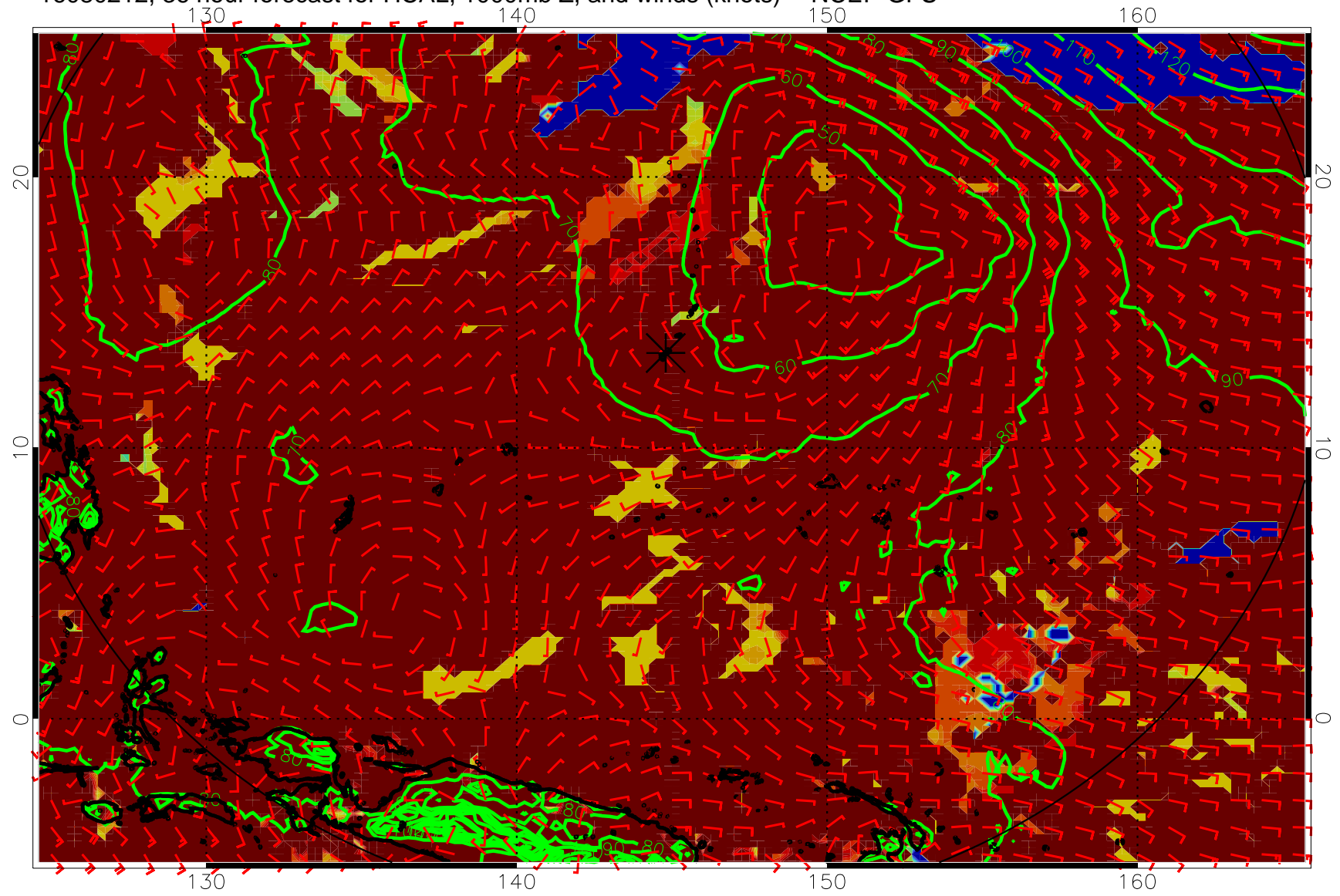
16080212, 36 hour forecast for HCAL, 1000mb Z, and winds (knots) -- NCEP GFS
