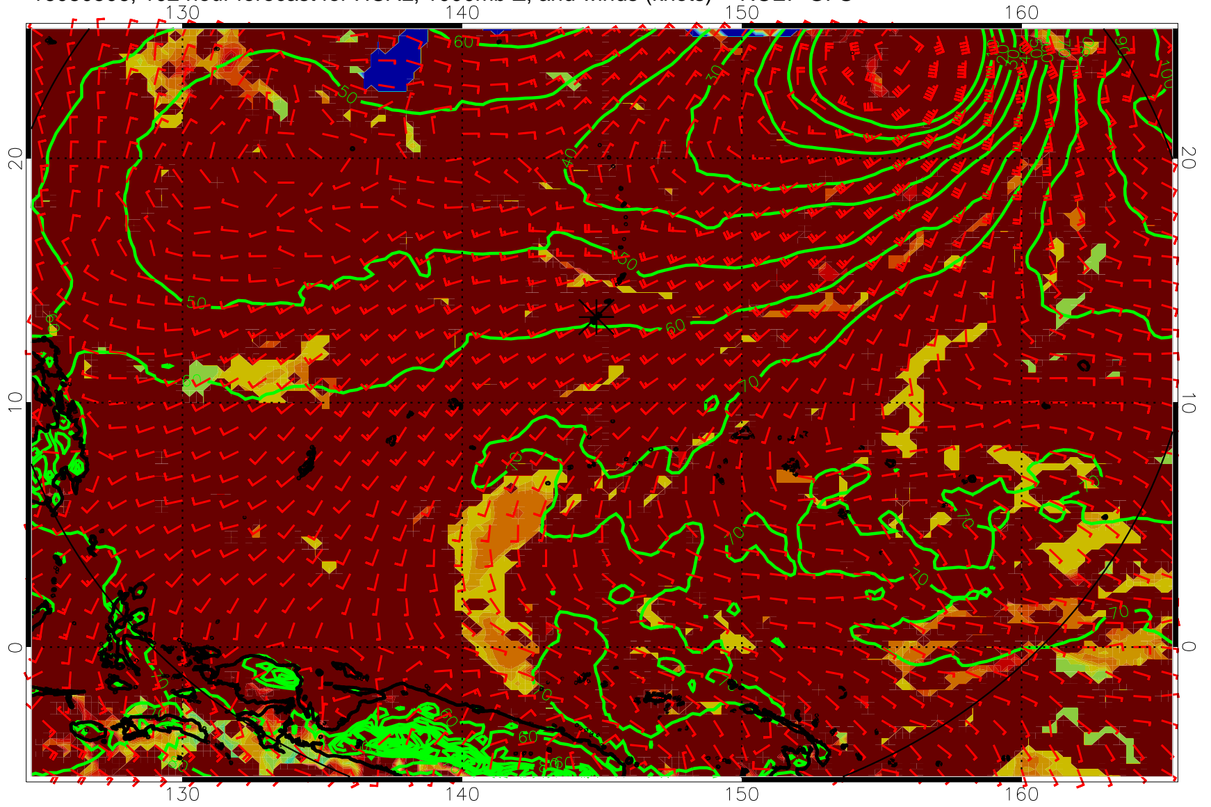
16080506, 102 hour forecast for HCAL, 1000mb Z, and winds (knots) -- NCEP GFS
