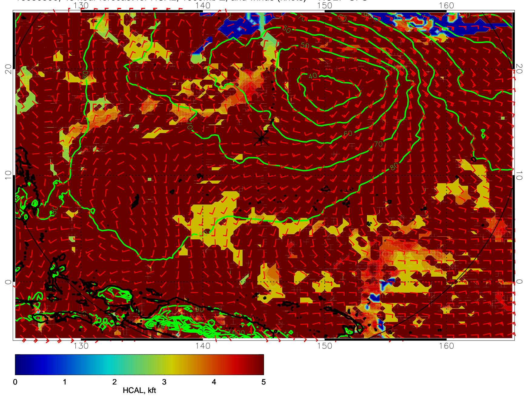
16080300, 48 hour forecast for HCAL, 1000mb Z, and winds (knots) -- NCEP GFS
