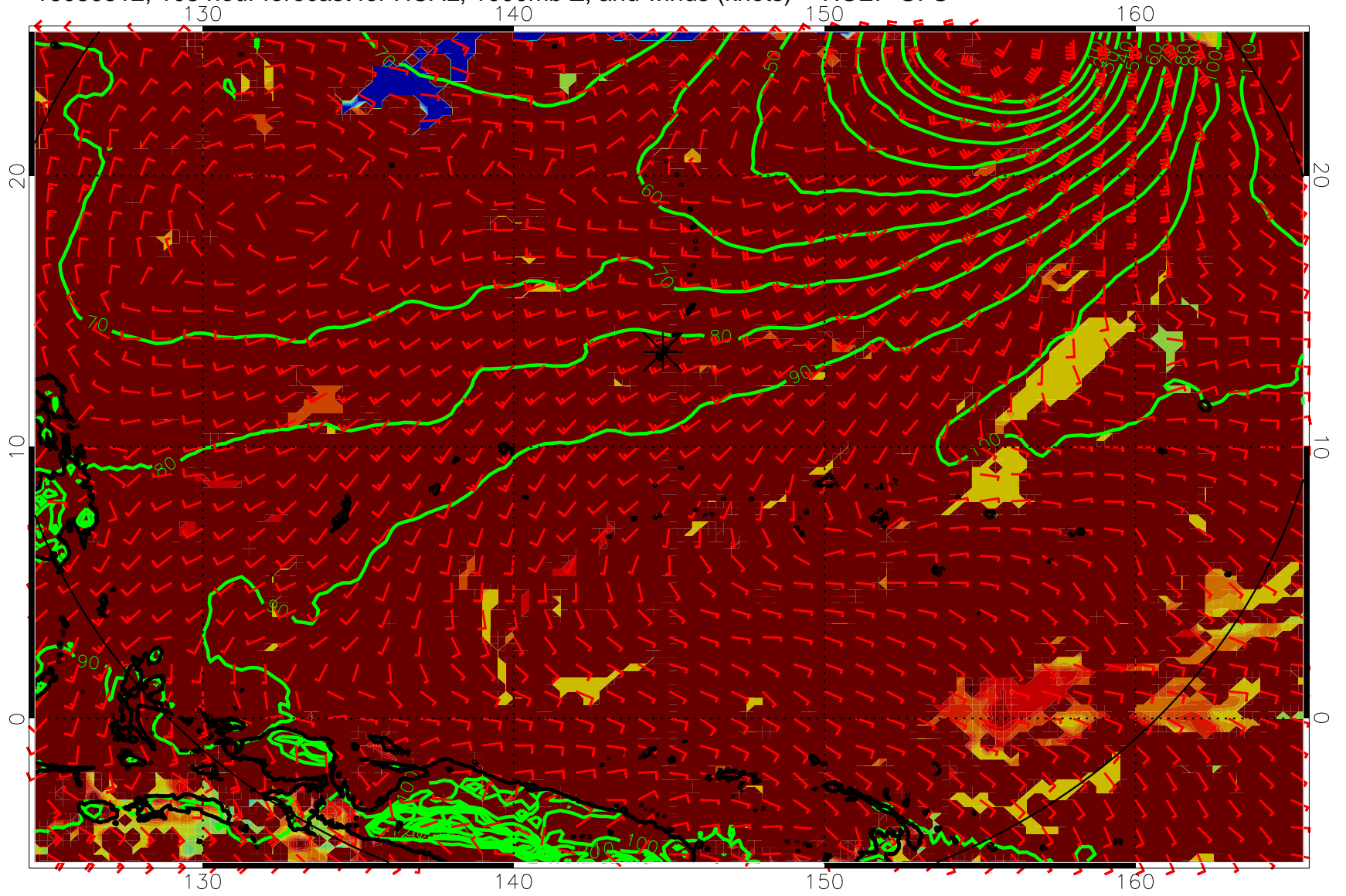
16080512, 108 hour forecast for HCAL, 1000mb Z, and winds (knots) -- NCEP GFS
