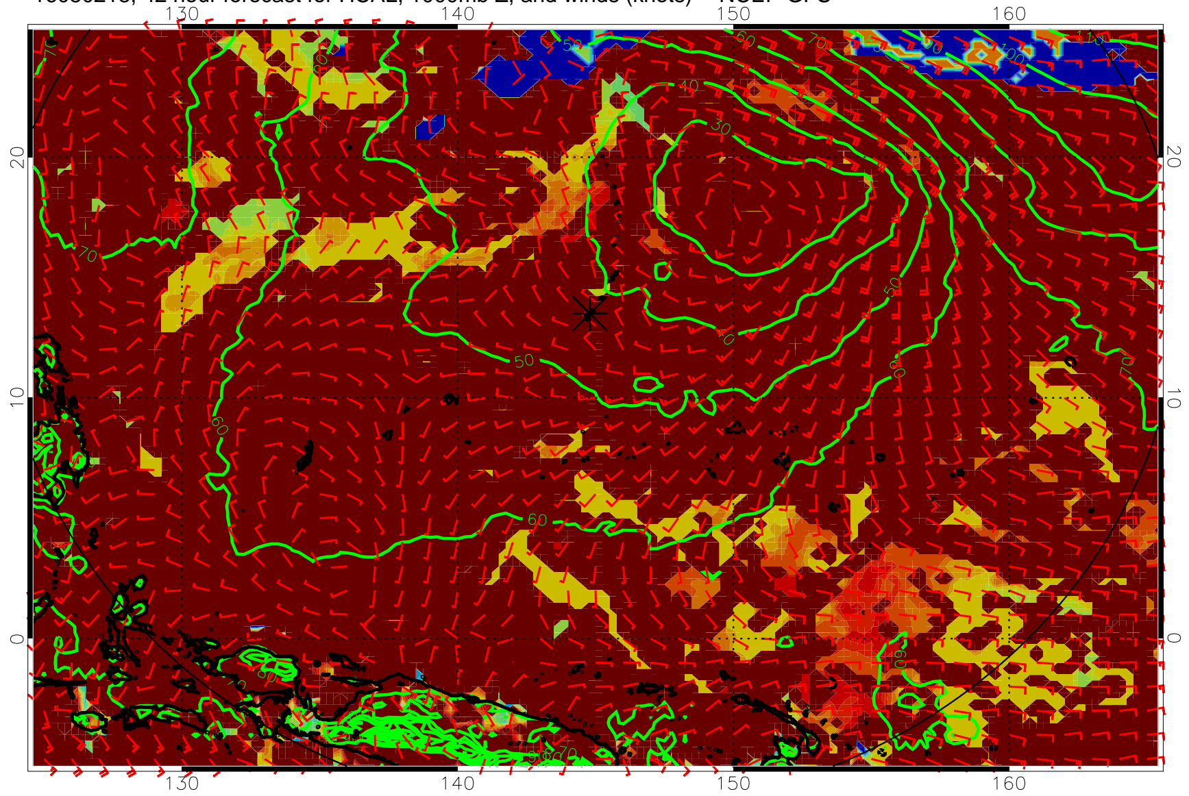
16080218, 42 hour forecast for HCAL, 1000mb Z, and winds (knots) -- NCEP GFS
