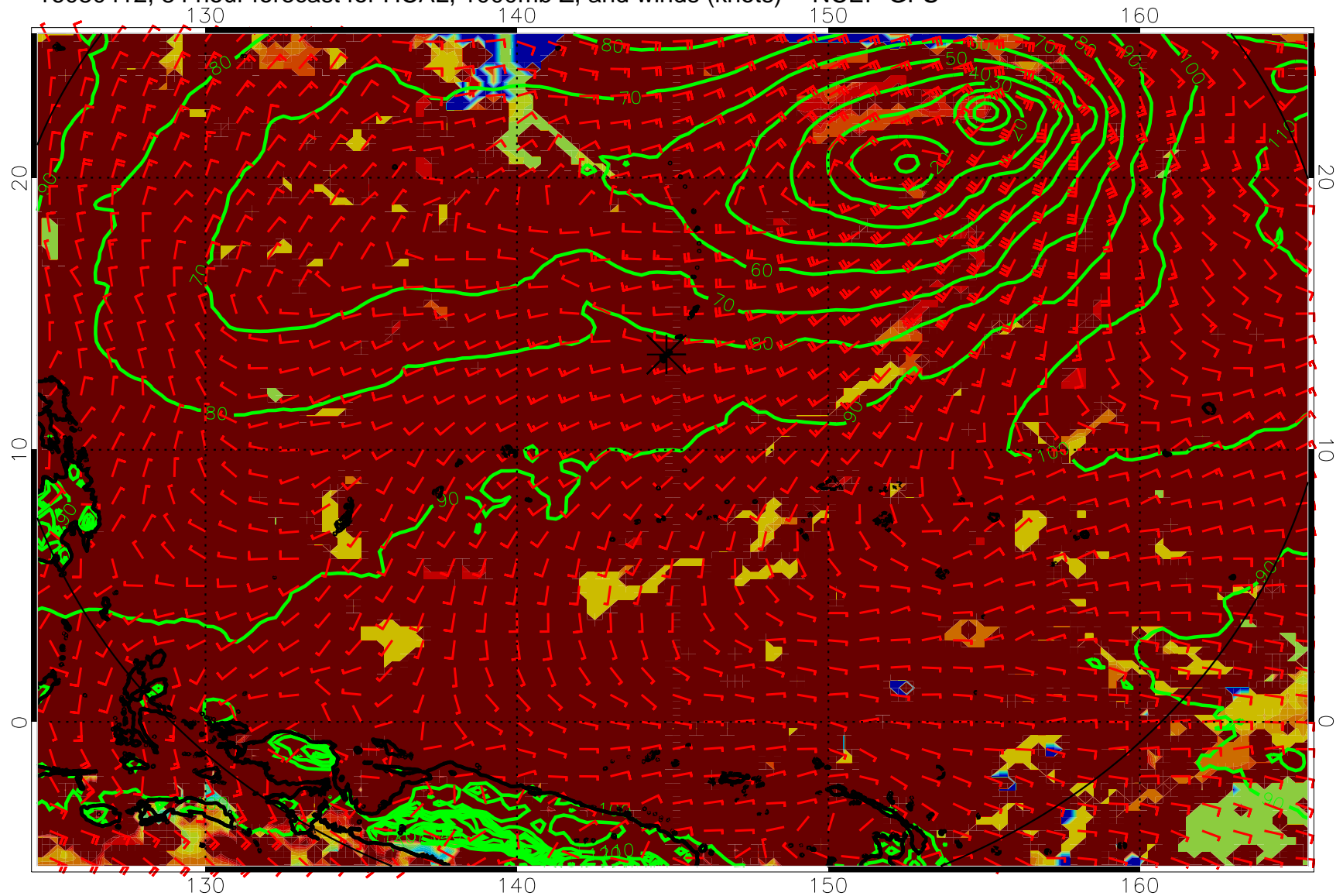
16080412, 84 hour forecast for HCAL, 1000mb Z, and winds (knots) -- NCEP GFS
