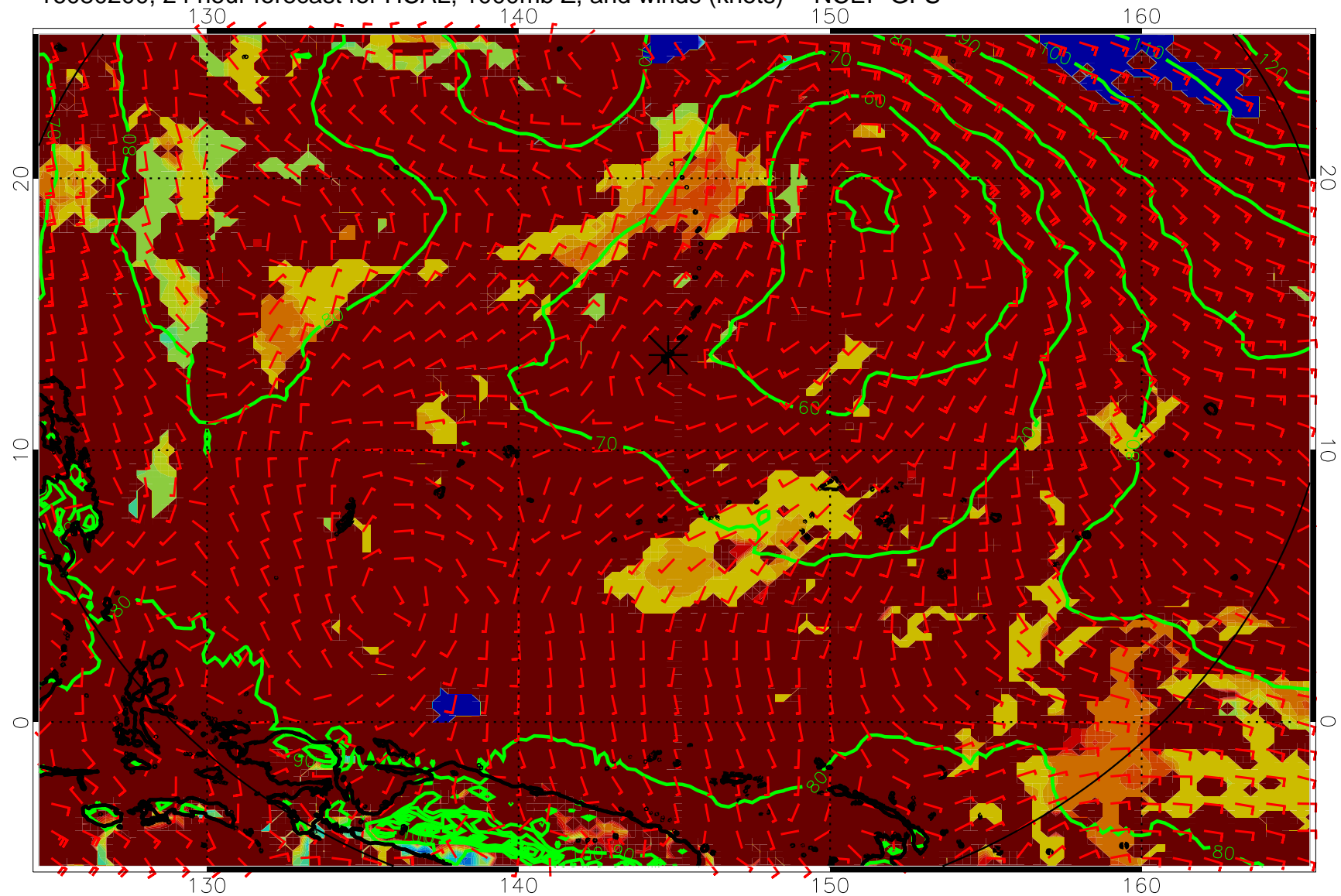
16080200, 24 hour forecast for HCAL, 1000mb Z, and winds (knots) -- NCEP GFS
