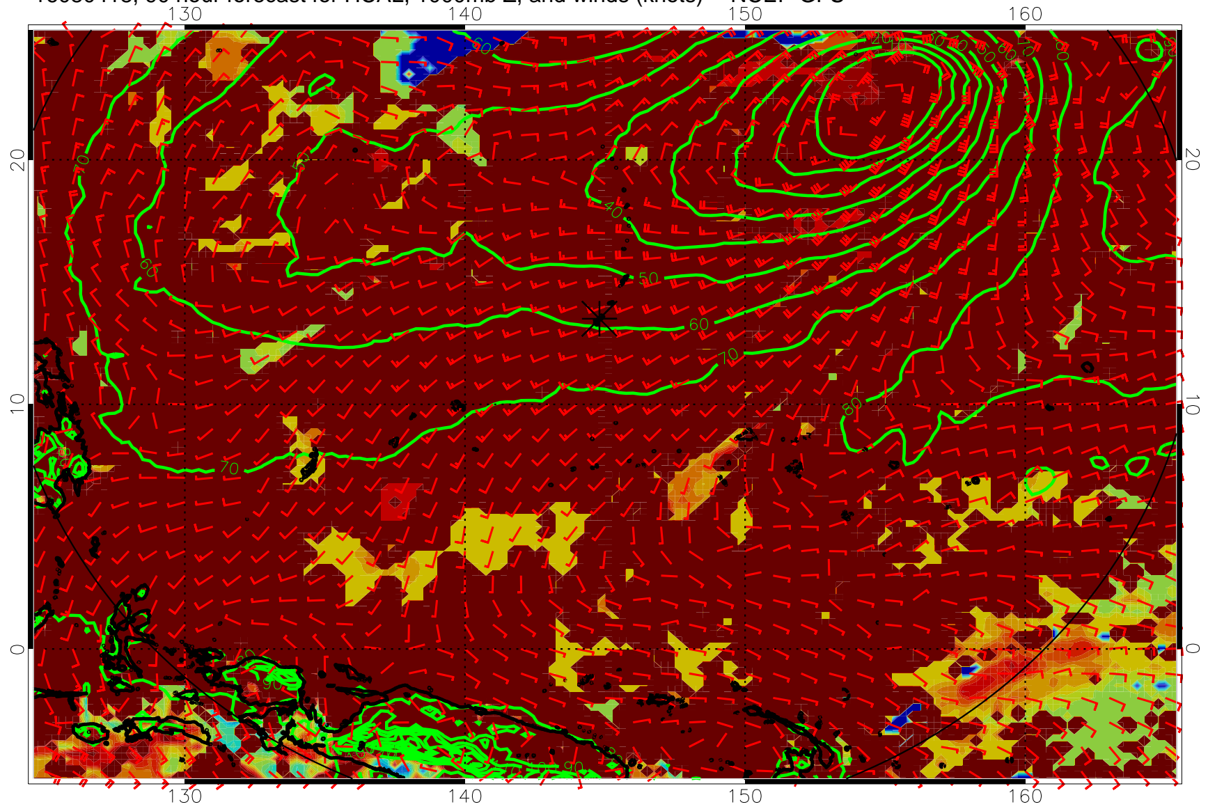
16080418, 90 hour forecast for HCAL, 1000mb Z, and winds (knots) -- NCEP GFS
