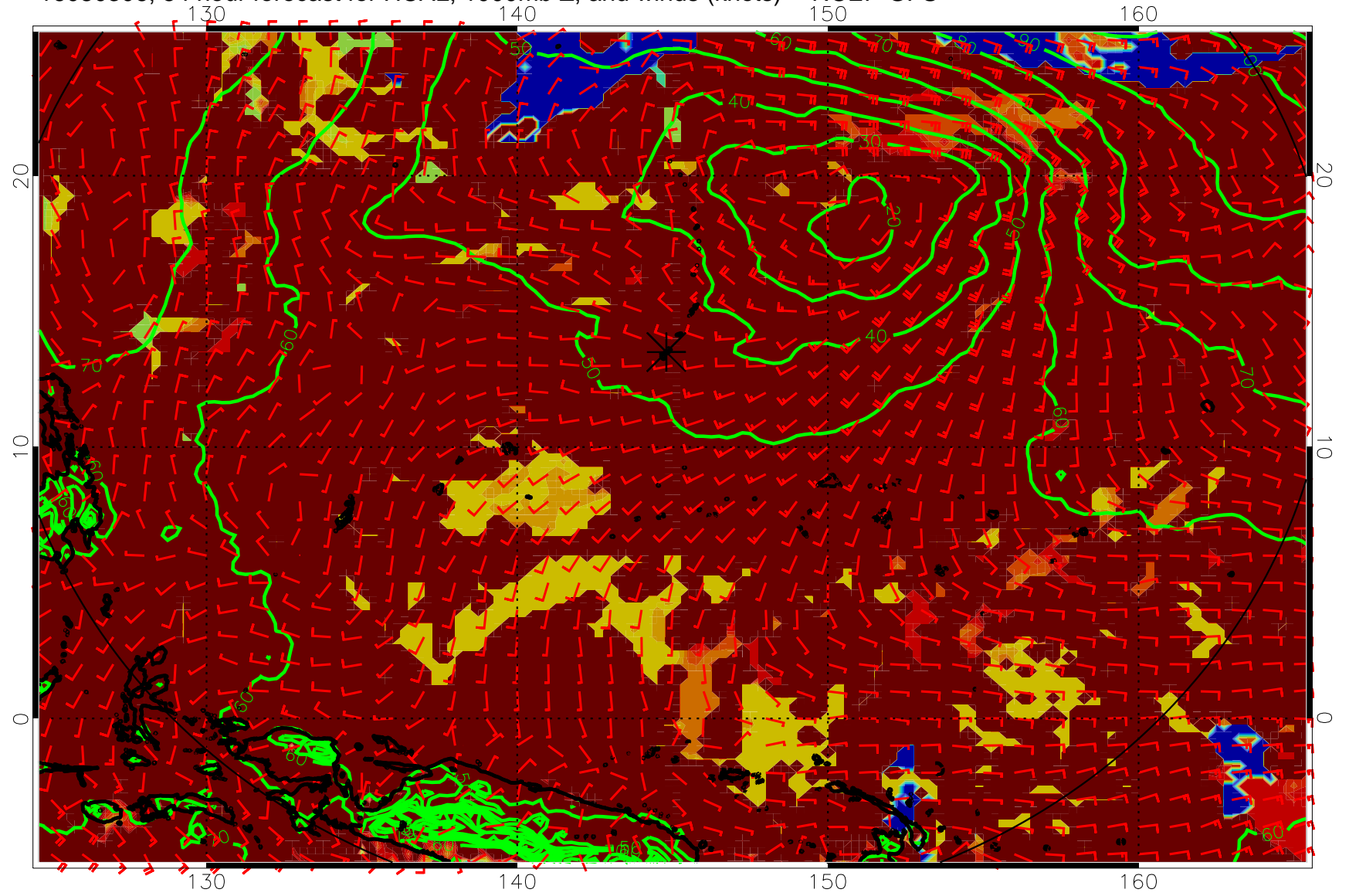
16080306, 54 hour forecast for HCAL, 1000mb Z, and winds (knots) -- NCEP GFS
