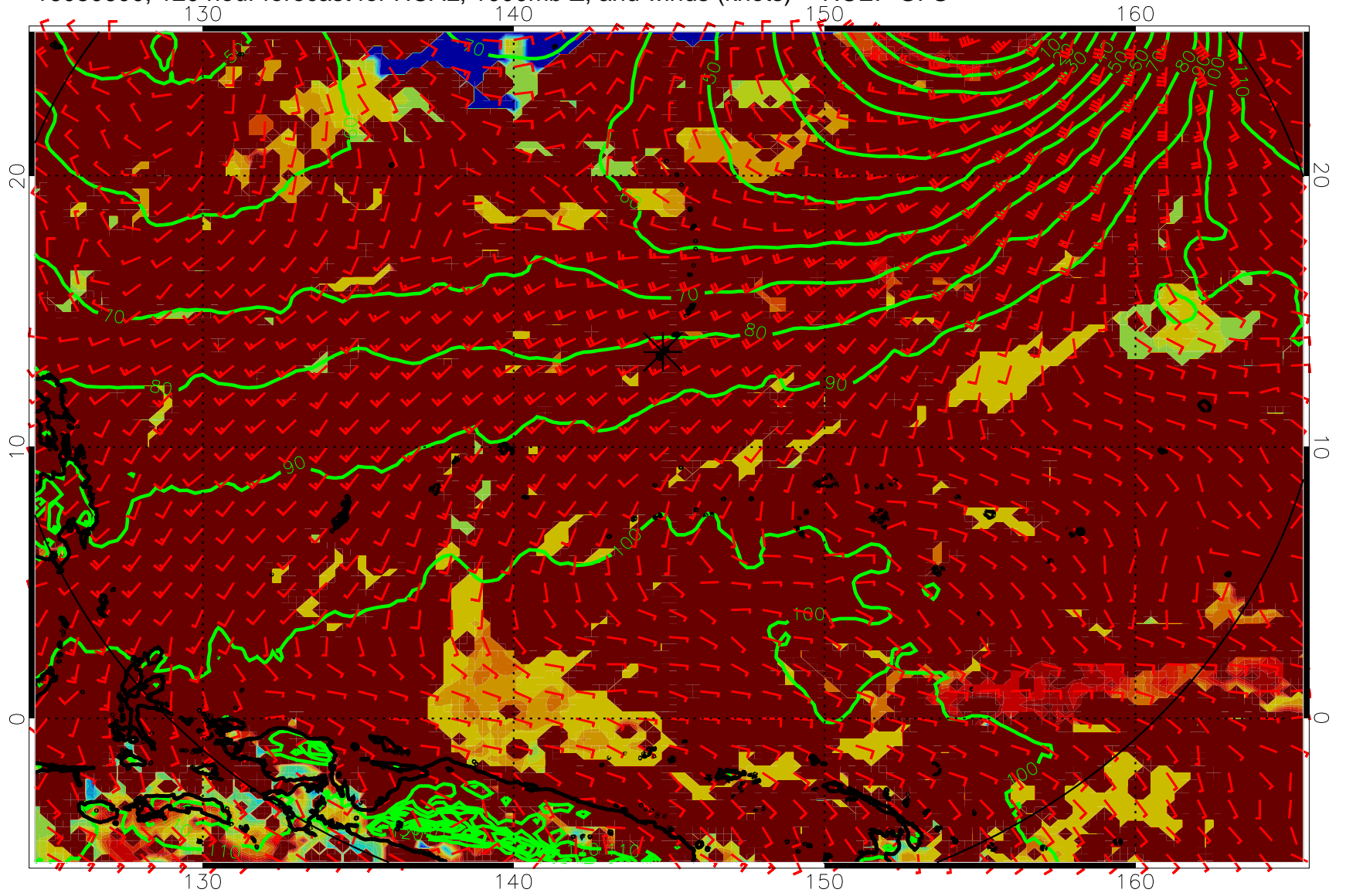
16080600, 120 hour forecast for HCAL, 1000mb Z, and winds (knots) -- NCEP GFS
