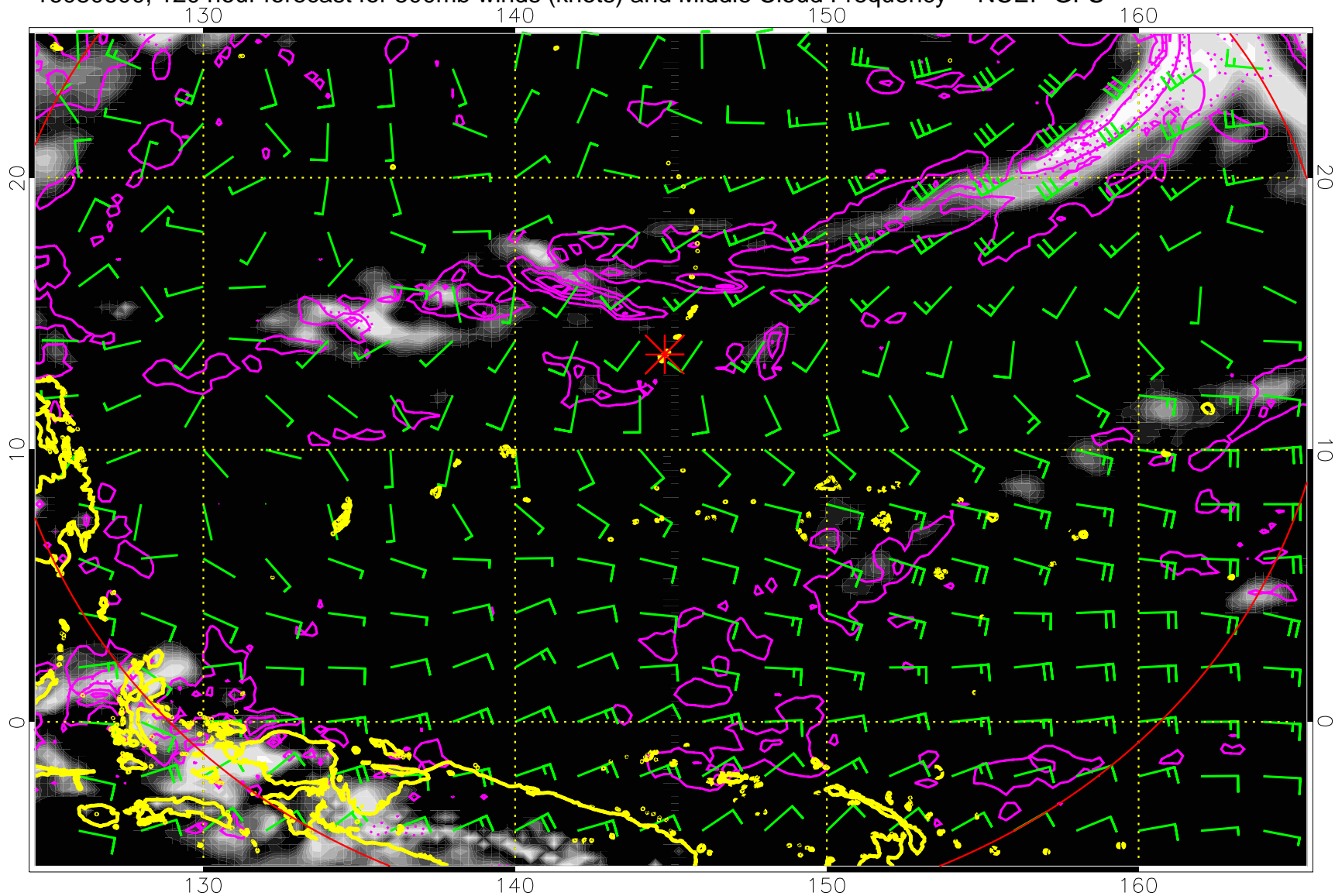
16080600, 120 hour forecast for 500mb winds (knots) and Middle Cloud Frequency -- NCEP GFS
