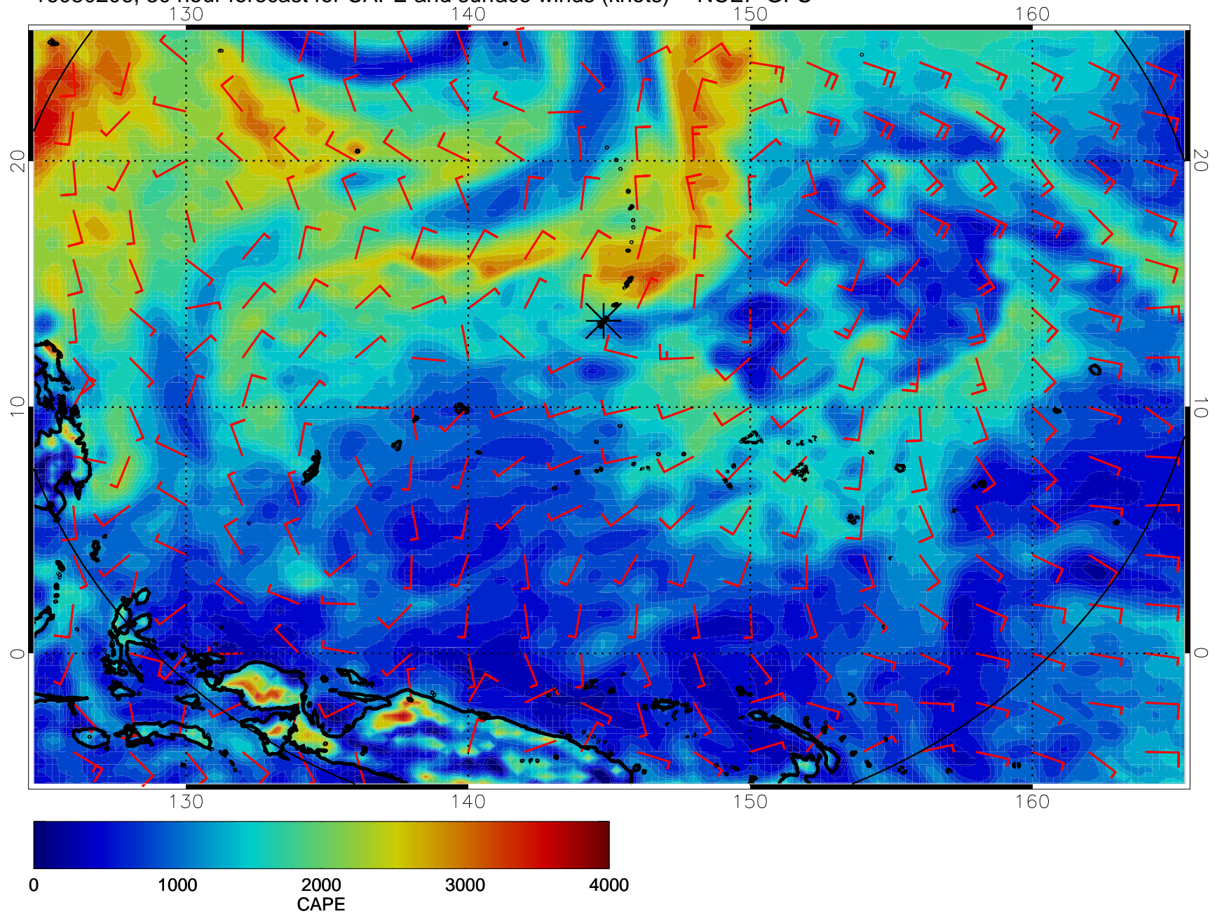
16080206, 30 hour forecast for CAPE and surface winds (knots) -- NCEP GFS
