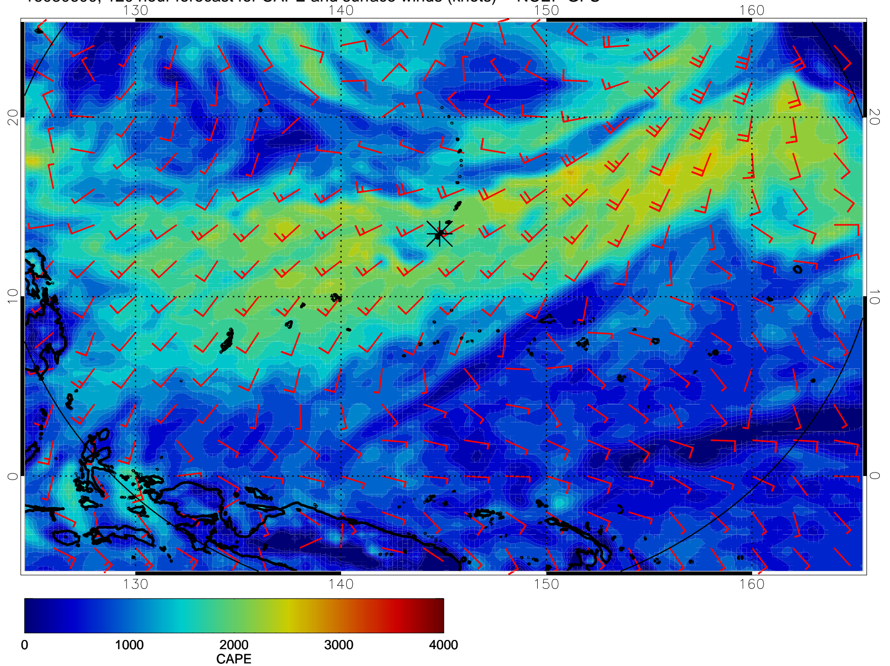
16080600, 120 hour forecast for CAPE and surface winds (knots) -- NCEP GFS
