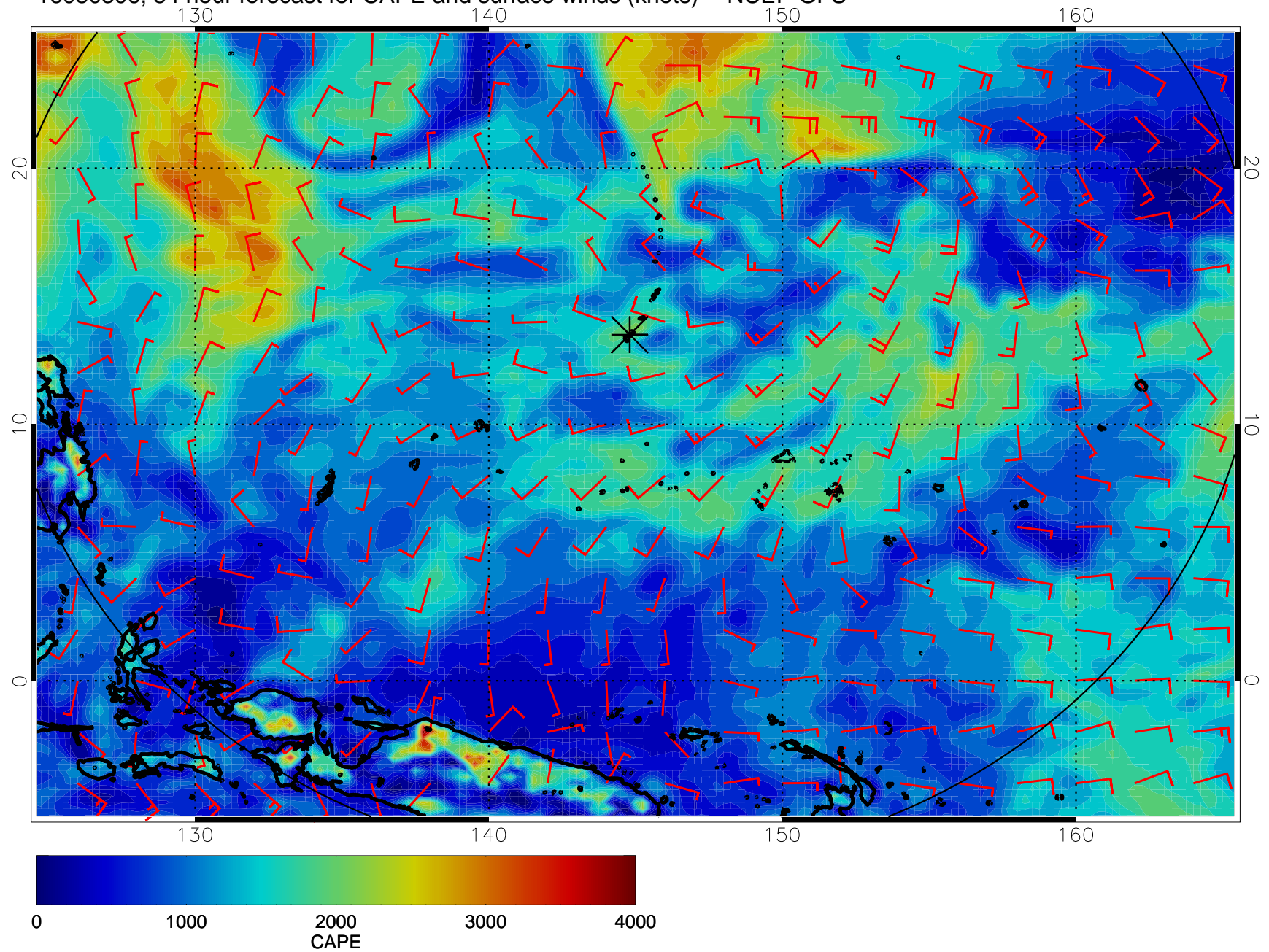
16080306, 54 hour forecast for CAPE and surface winds (knots) -- NCEP GFS
