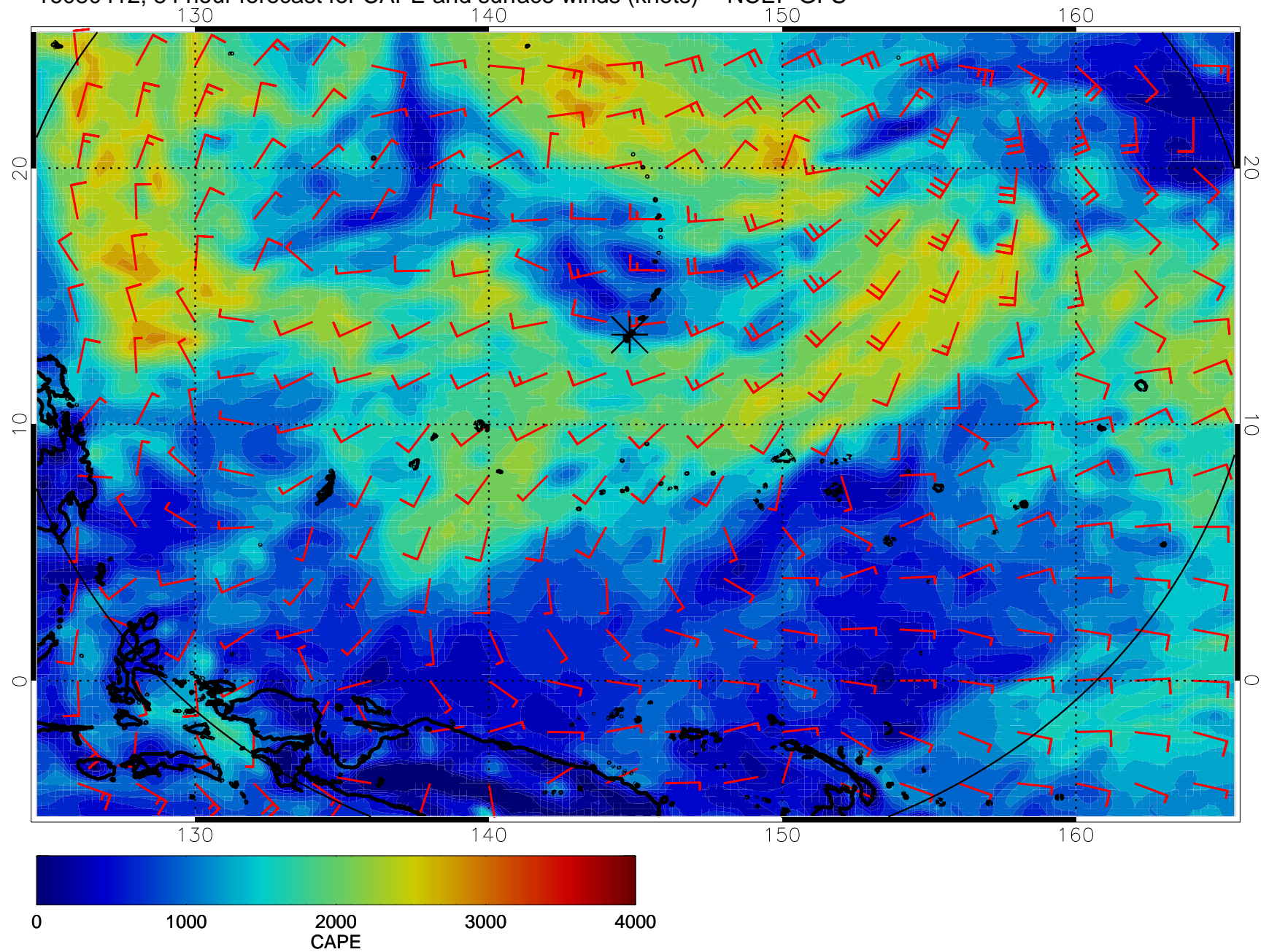
16080412, 84 hour forecast for CAPE and surface winds (knots) -- NCEP GFS
