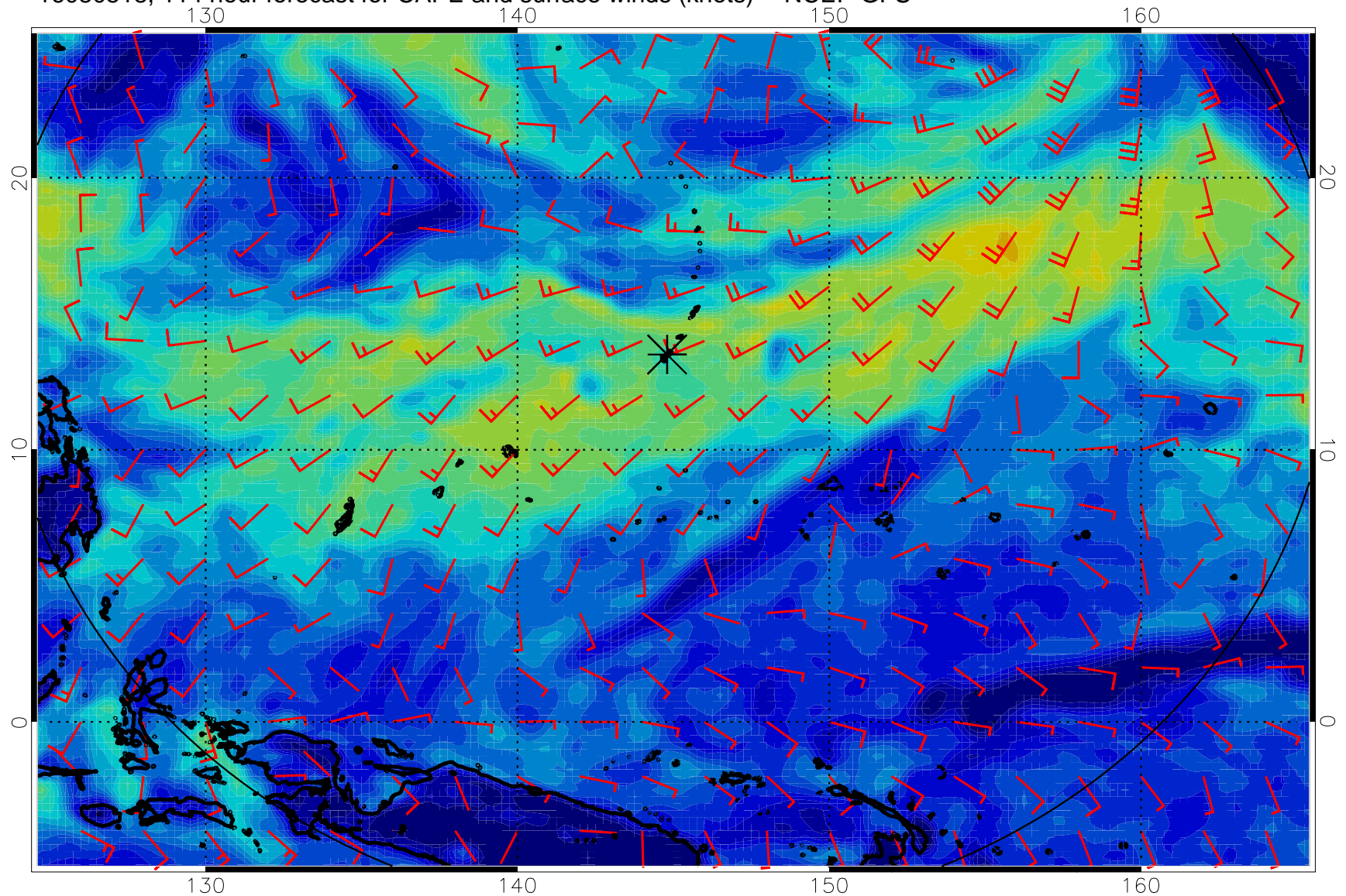
16080518, 114 hour forecast for CAPE and surface winds (knots) -- NCEP GFS
