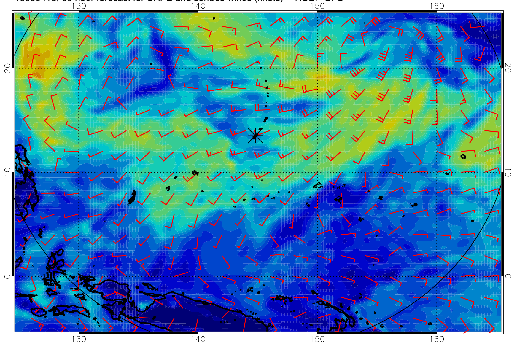
16080418, 90 hour forecast for CAPE and surface winds (knots) -- NCEP GFS
