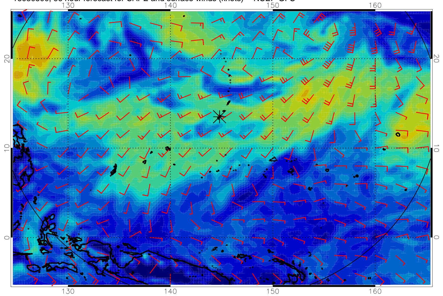
16080500, 96 hour forecast for CAPE and surface winds (knots) -- NCEP GFS
