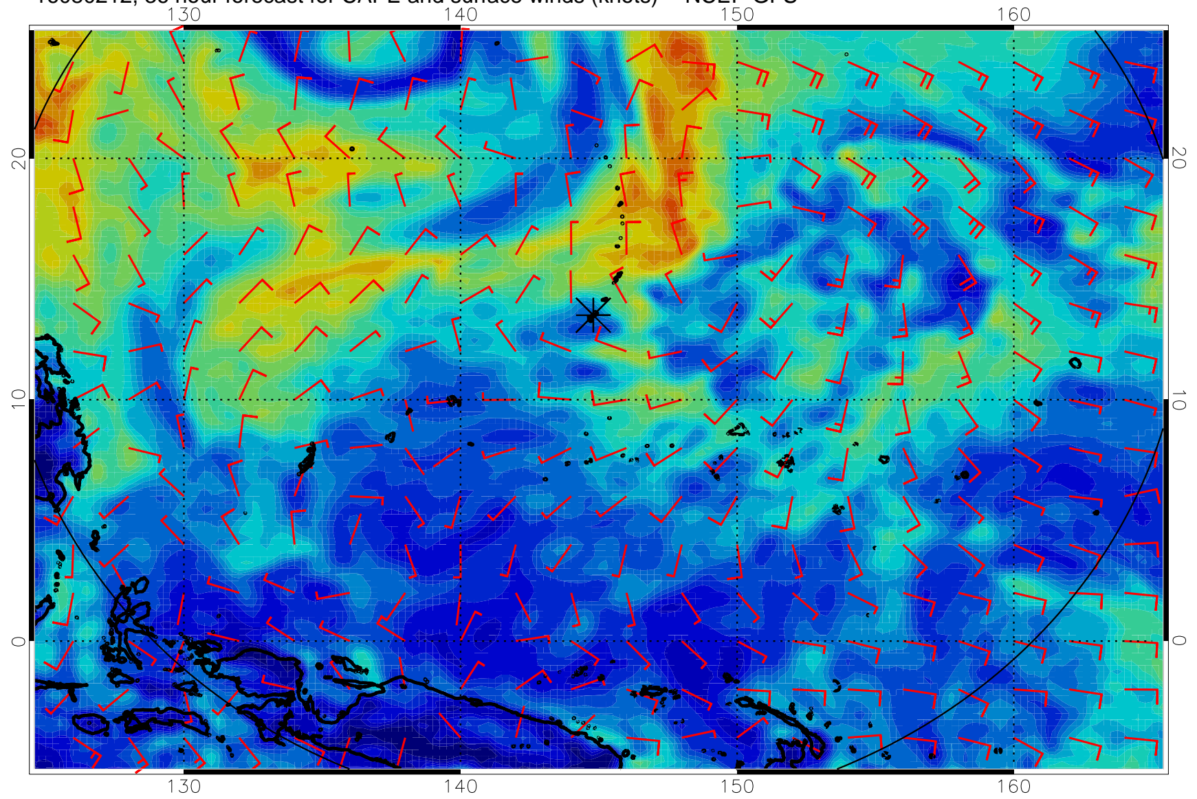
16080212, 36 hour forecast for CAPE and surface winds (knots) -- NCEP GFS
