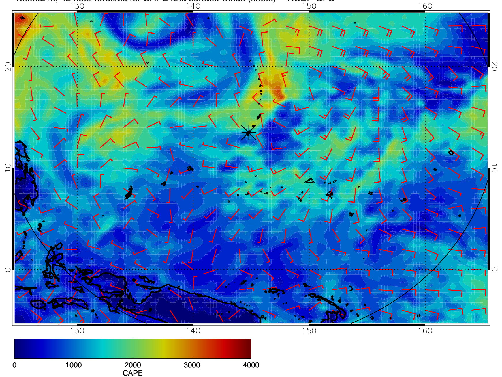
16080218, 42 hour forecast for CAPE and surface winds (knots) -- NCEP GFS
