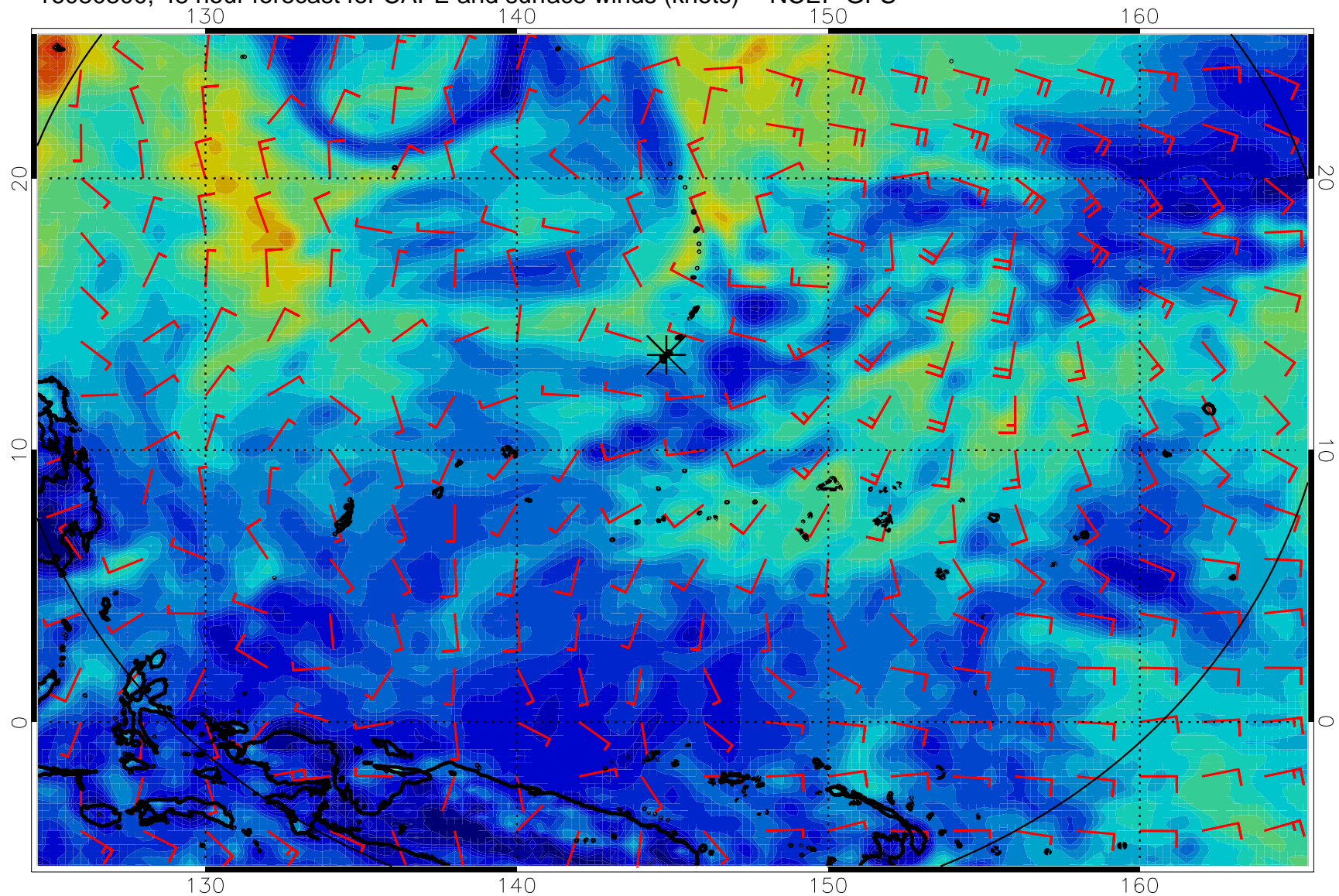
16080300, 48 hour forecast for CAPE and surface winds (knots) -- NCEP GFS
