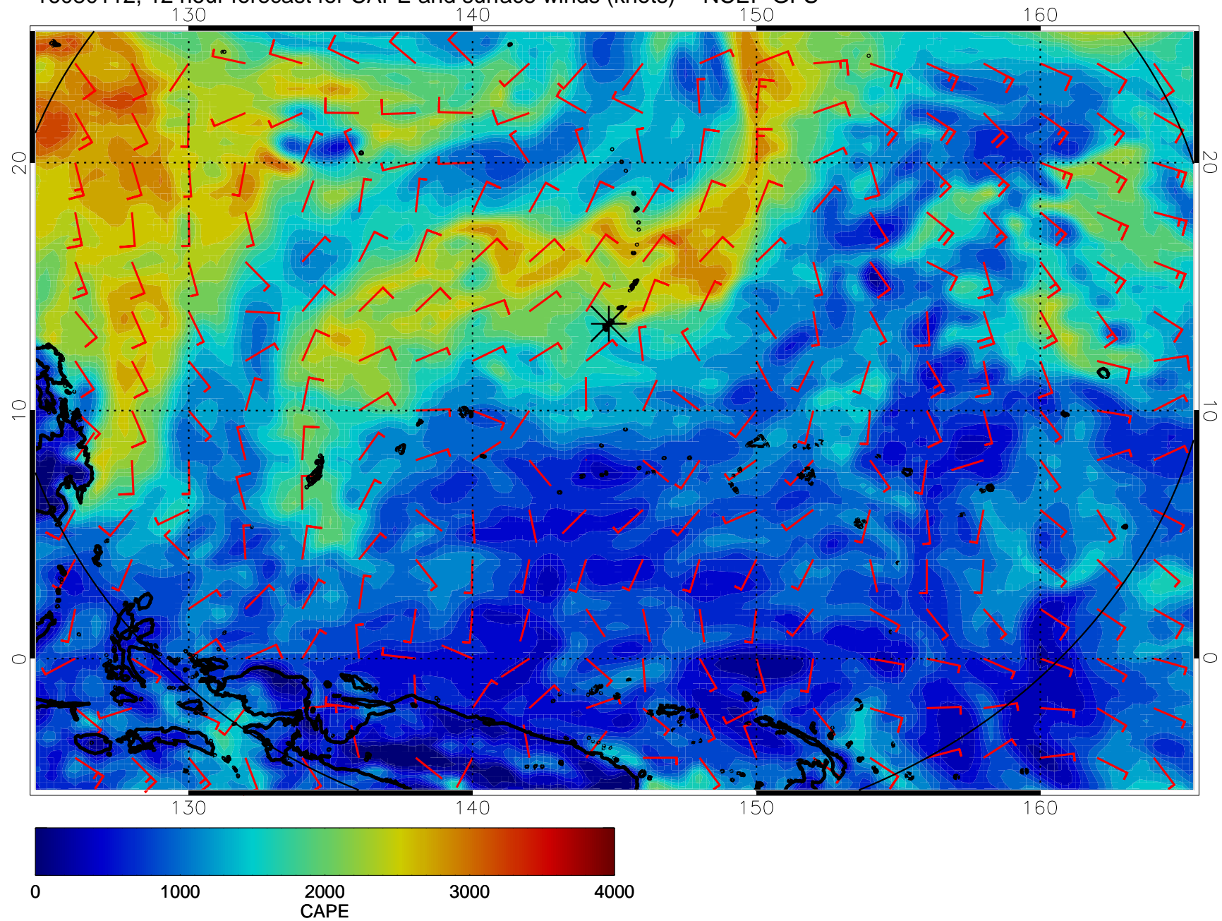
16080112, 12 hour forecast for CAPE and surface winds (knots) -- NCEP GFS
