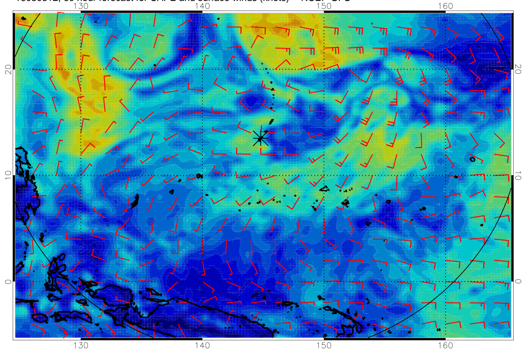
16080312, 60 hour forecast for CAPE and surface winds (knots) -- NCEP GFS
