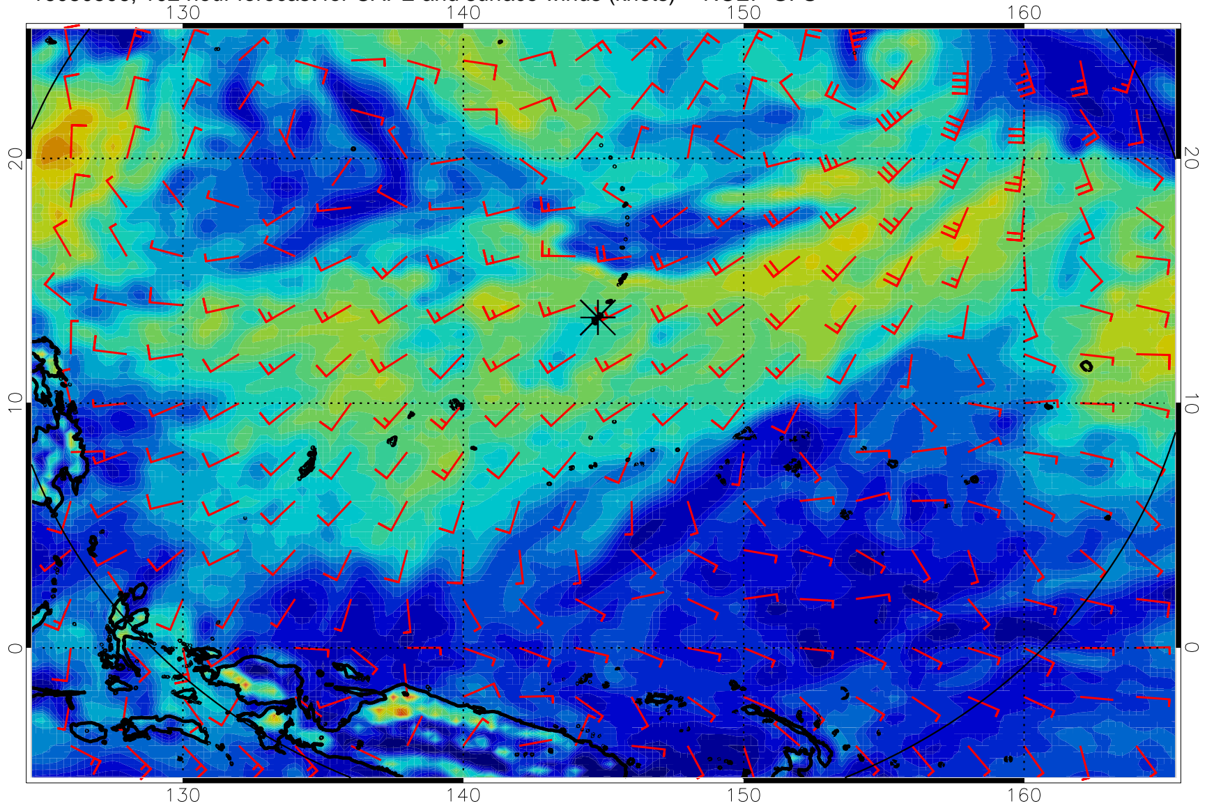
16080506, 102 hour forecast for CAPE and surface winds (knots) -- NCEP GFS
