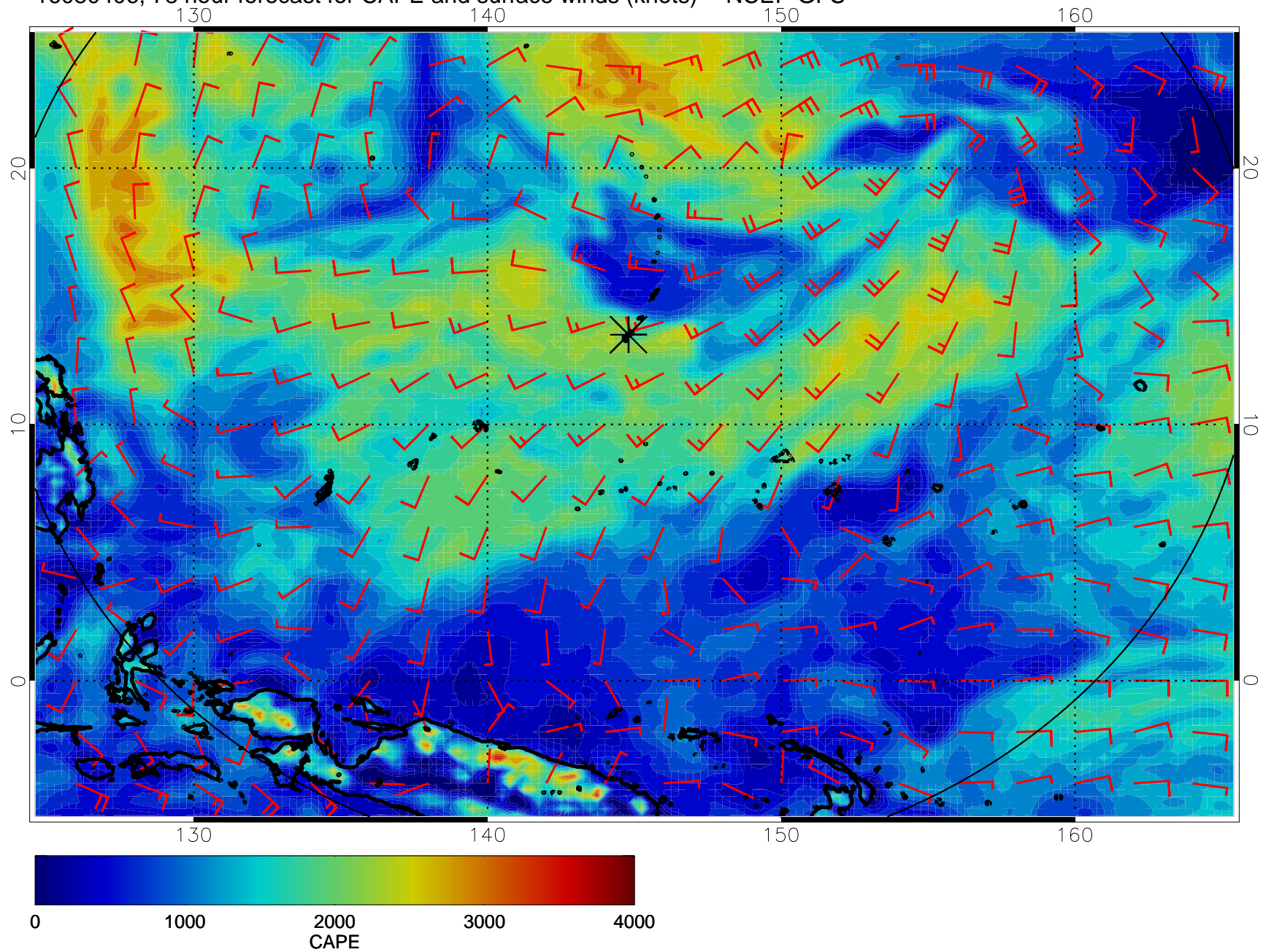
16080406, 78 hour forecast for CAPE and surface winds (knots) -- NCEP GFS
