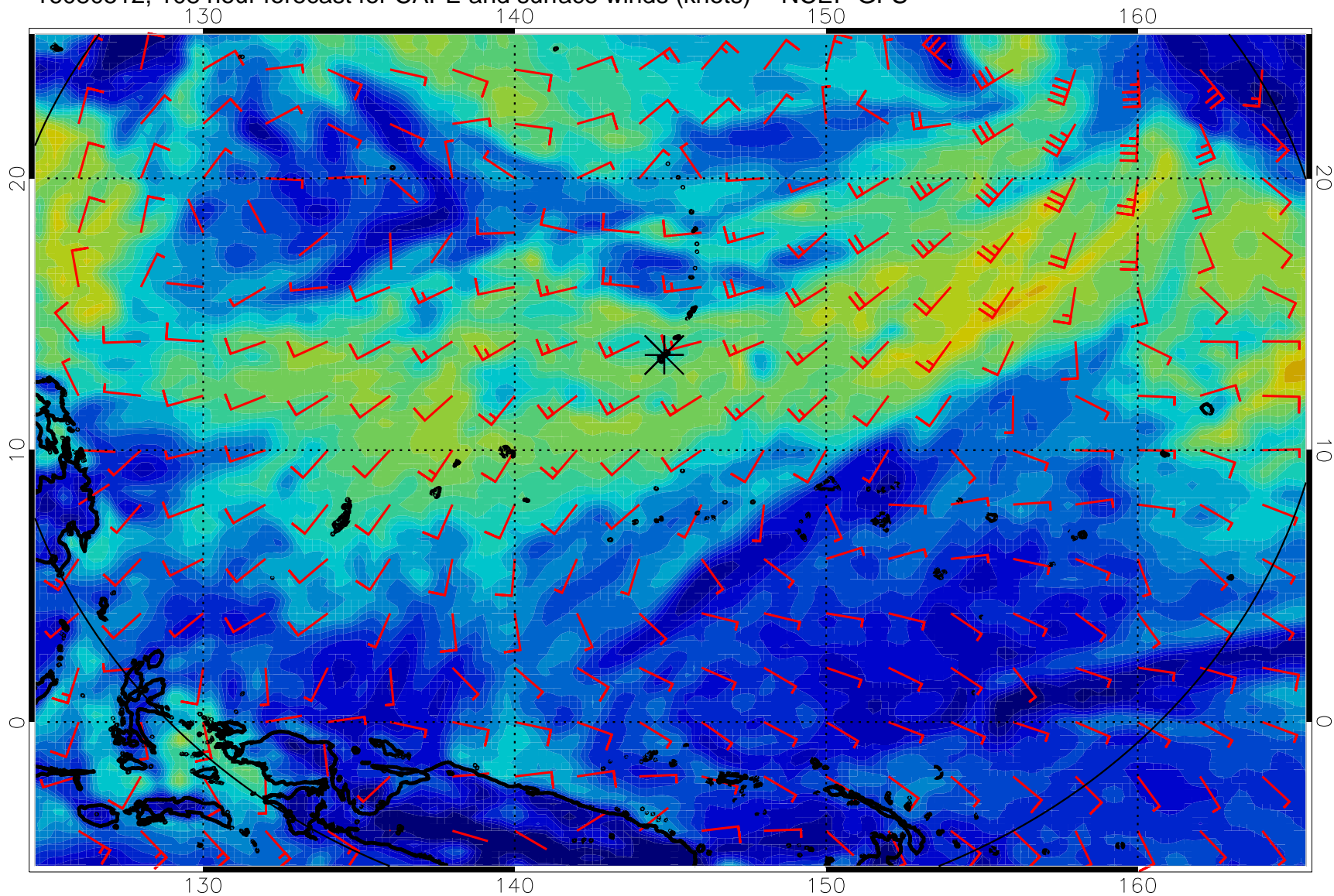
16080512, 108 hour forecast for CAPE and surface winds (knots) -- NCEP GFS
