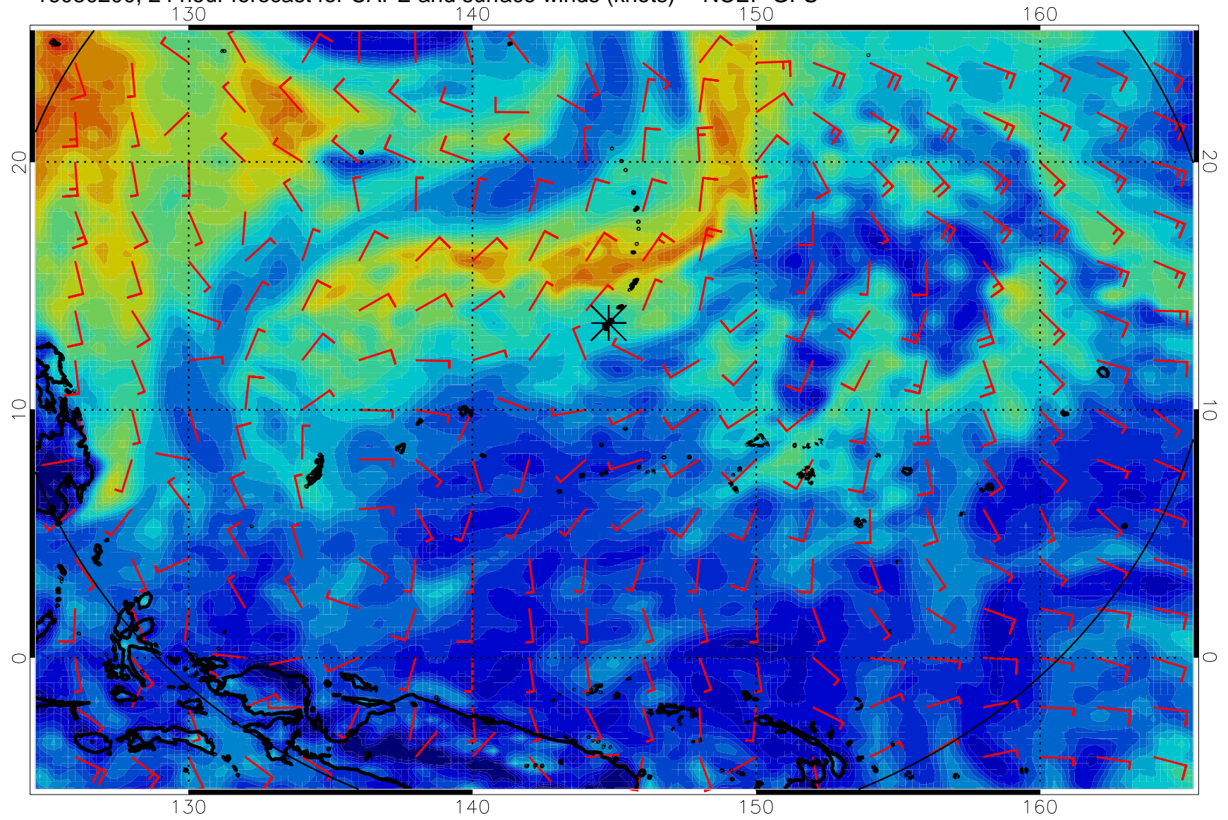
16080200, 24 hour forecast for CAPE and surface winds (knots) -- NCEP GFS
