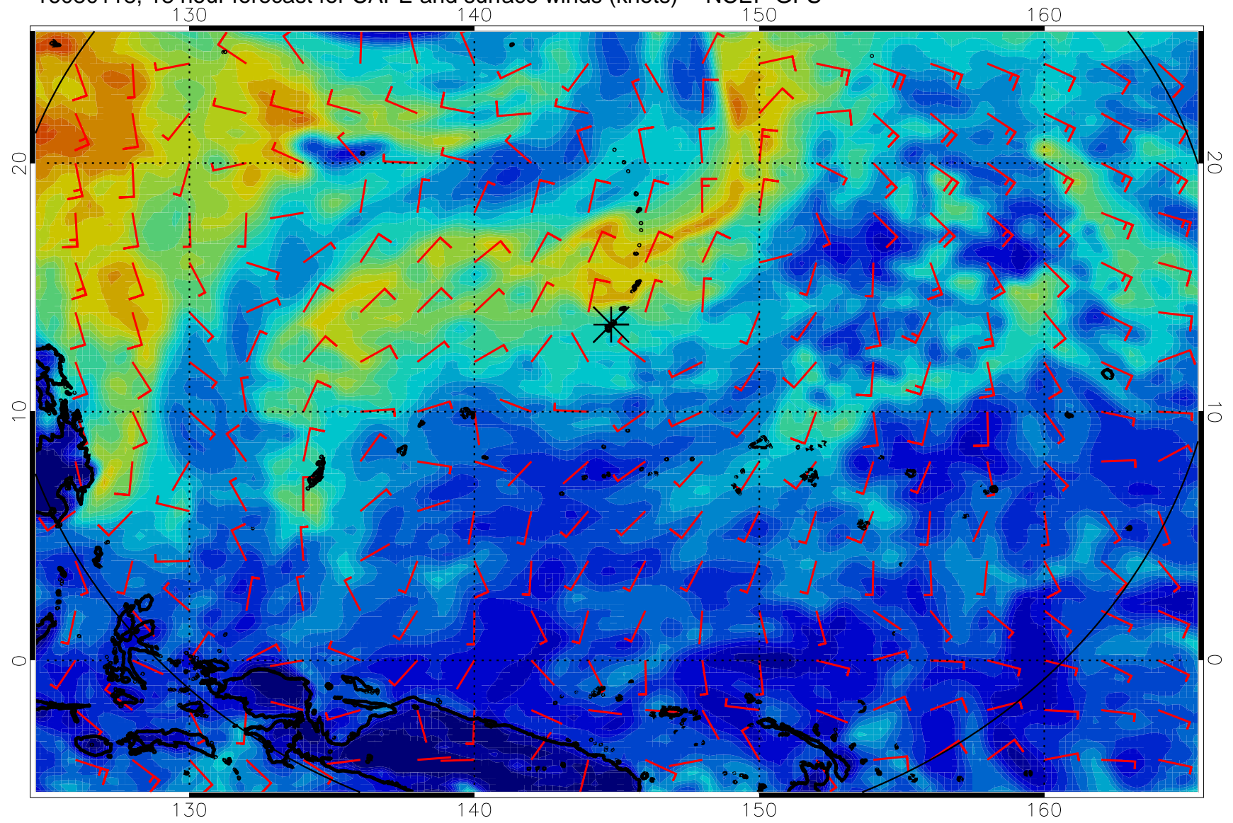
16080118, 18 hour forecast for CAPE and surface winds (knots) -- NCEP GFS
