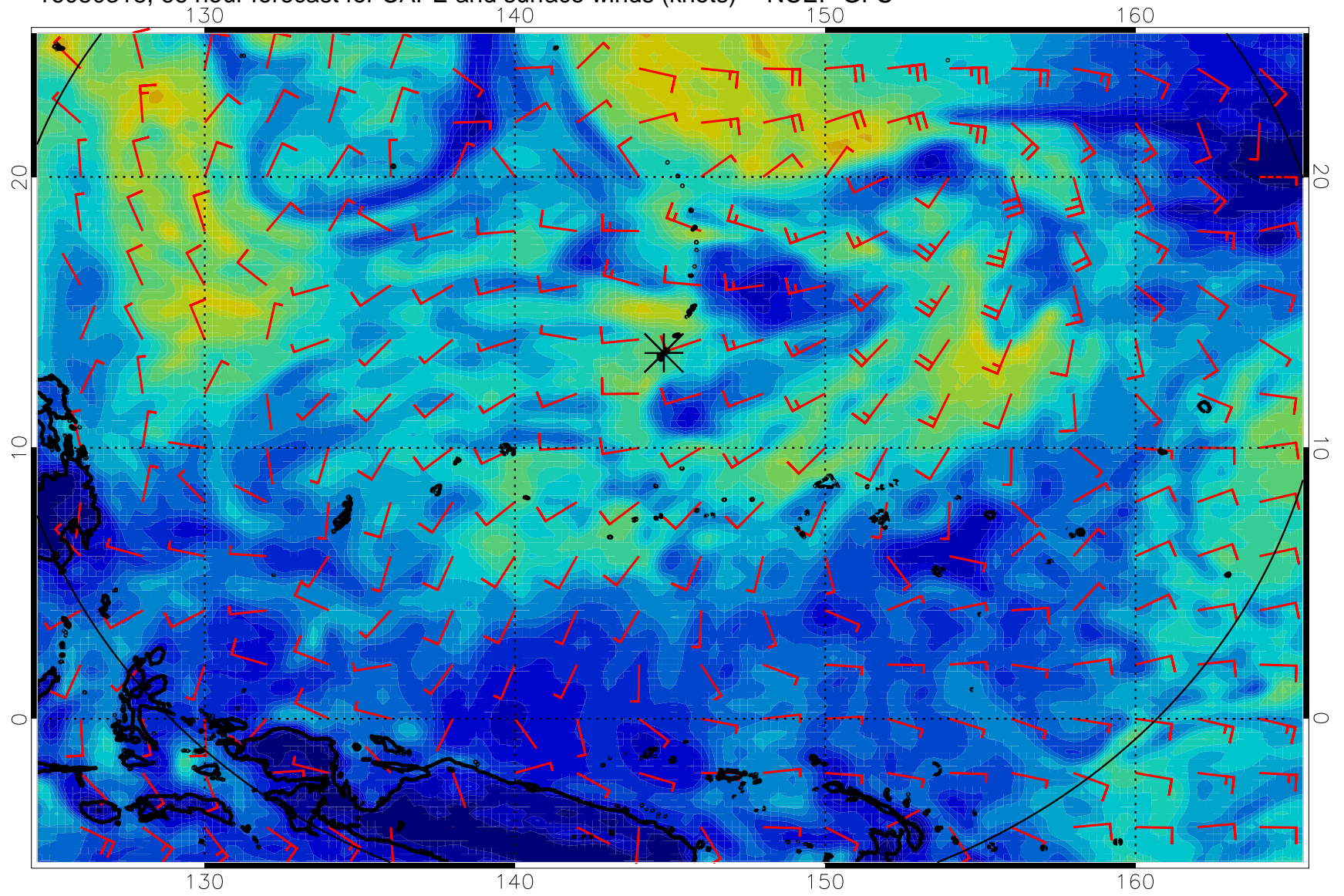
16080318, 66 hour forecast for CAPE and surface winds (knots) -- NCEP GFS
