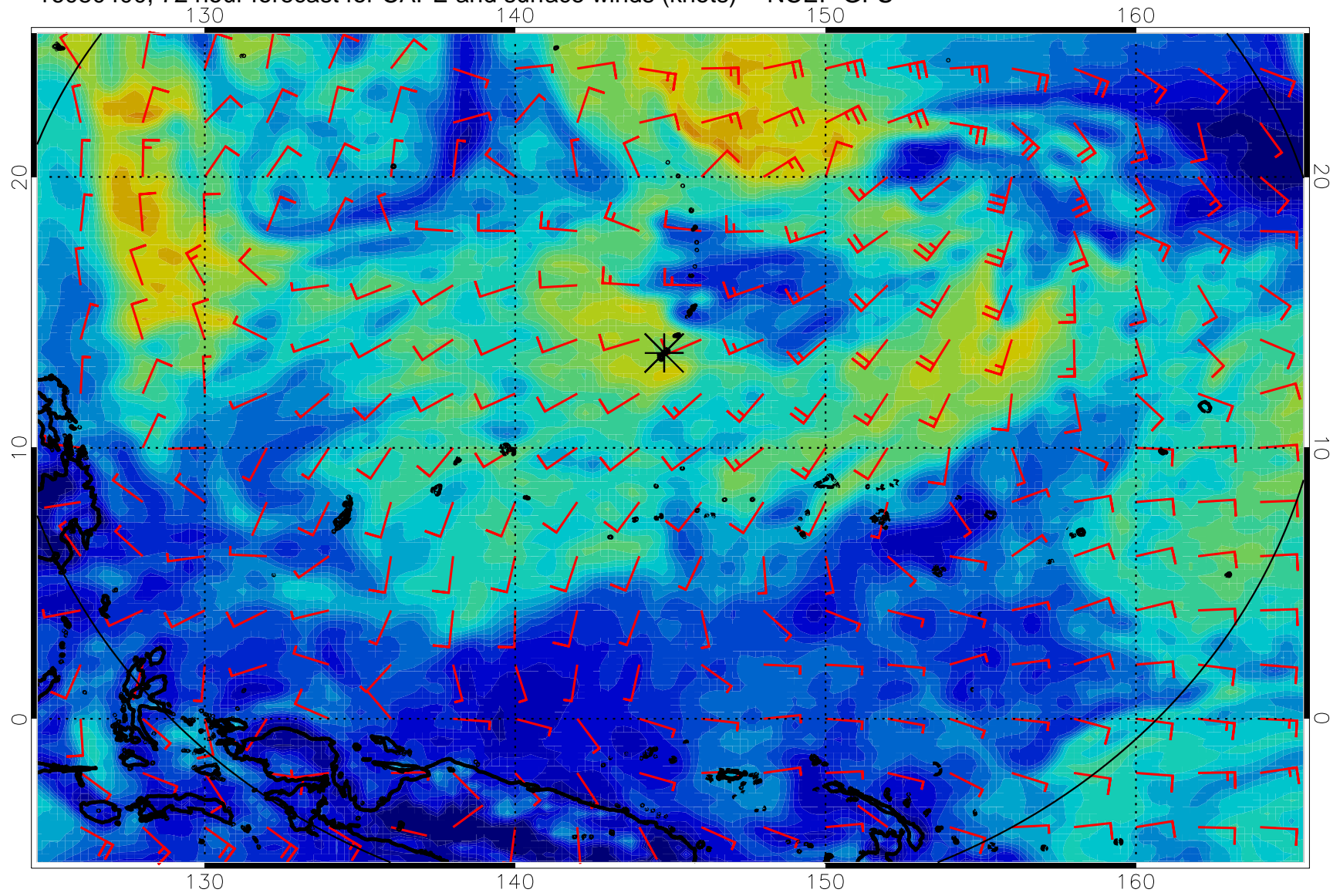
16080400, 72 hour forecast for CAPE and surface winds (knots) -- NCEP GFS
