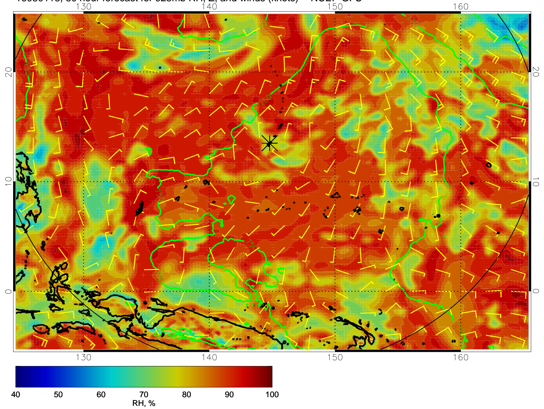
16080118, 30 hour forecast for 925mb RH, Z, and winds (knots) -- NCEP GFS
