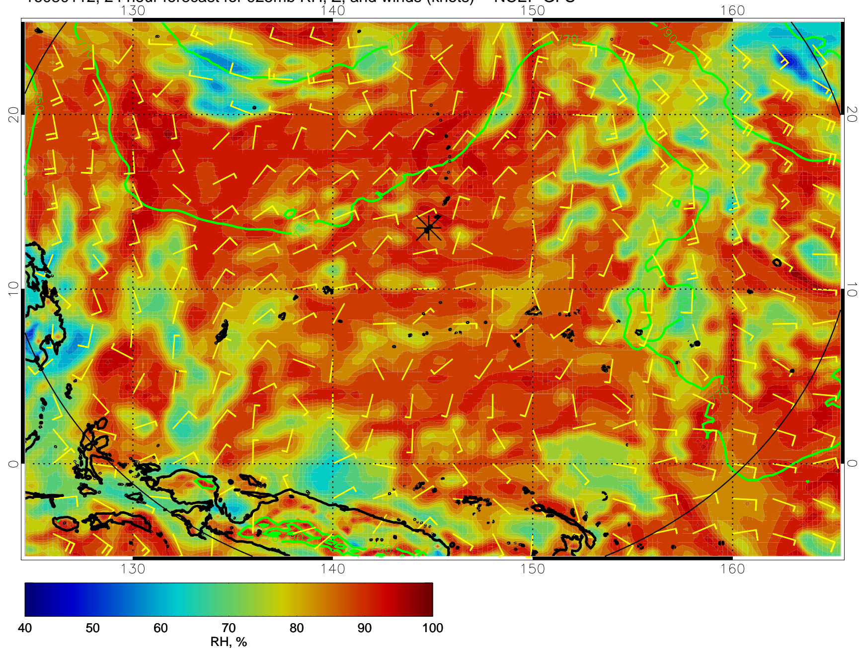
16080112, 24 hour forecast for 925mb RH, Z, and winds (knots) -- NCEP GFS
