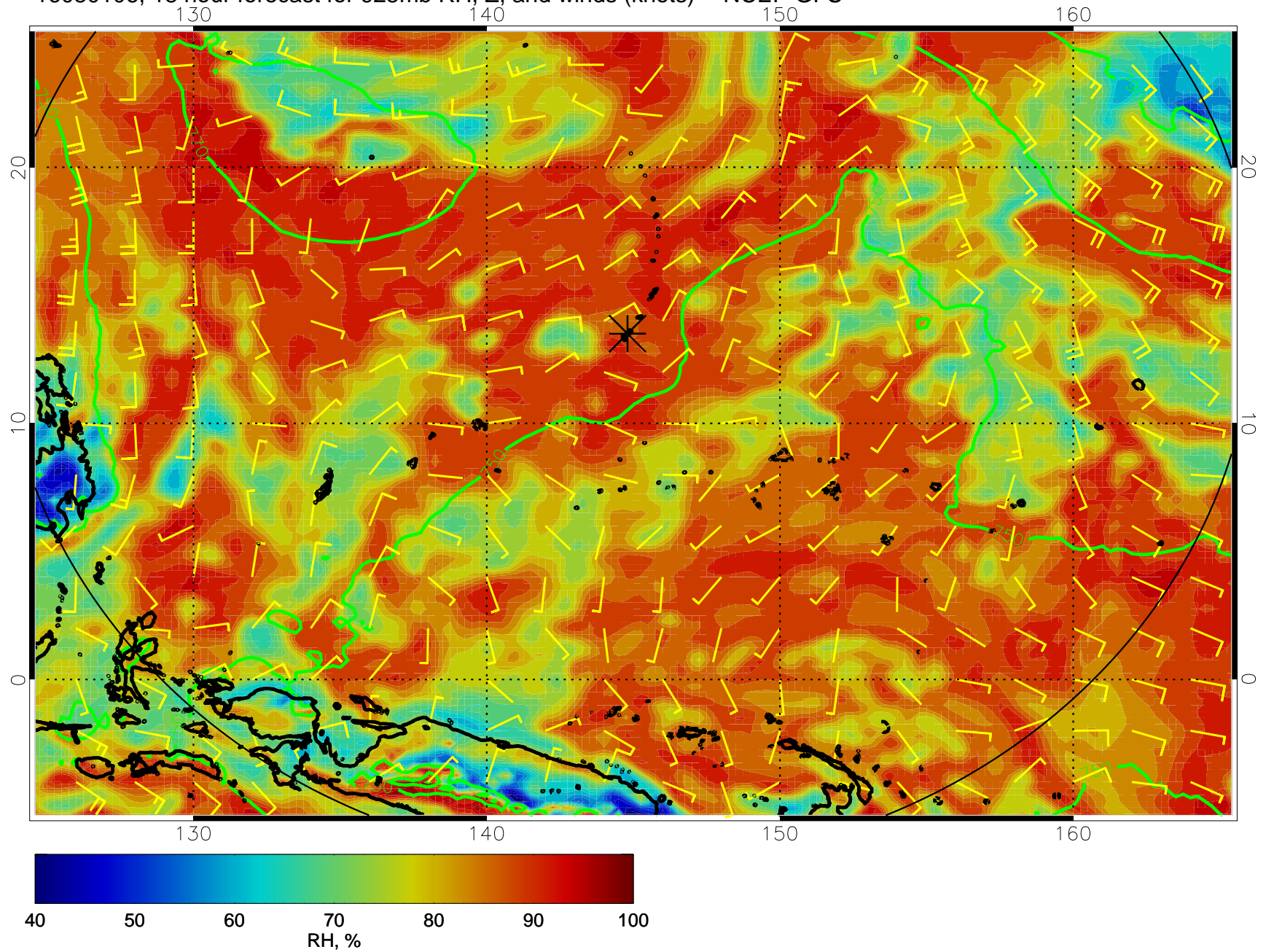
16080106, 18 hour forecast for 925mb RH, Z, and winds (knots) -- NCEP GFS
