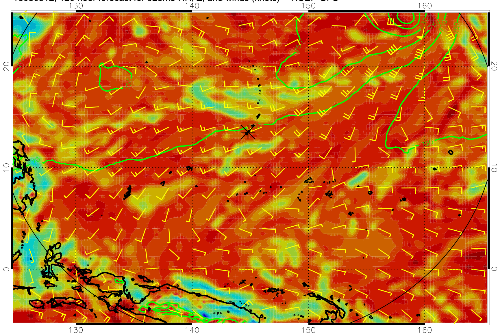
16080512, 120 hour forecast for 925mb RH, Z, and winds (knots) -- NCEP GFS
