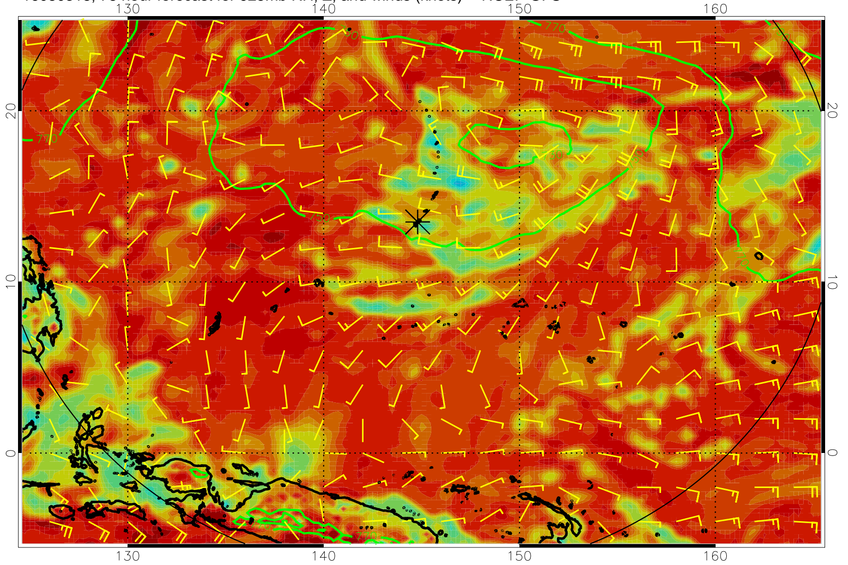
16080318, 78 hour forecast for 925mb RH, Z, and winds (knots) -- NCEP GFS
