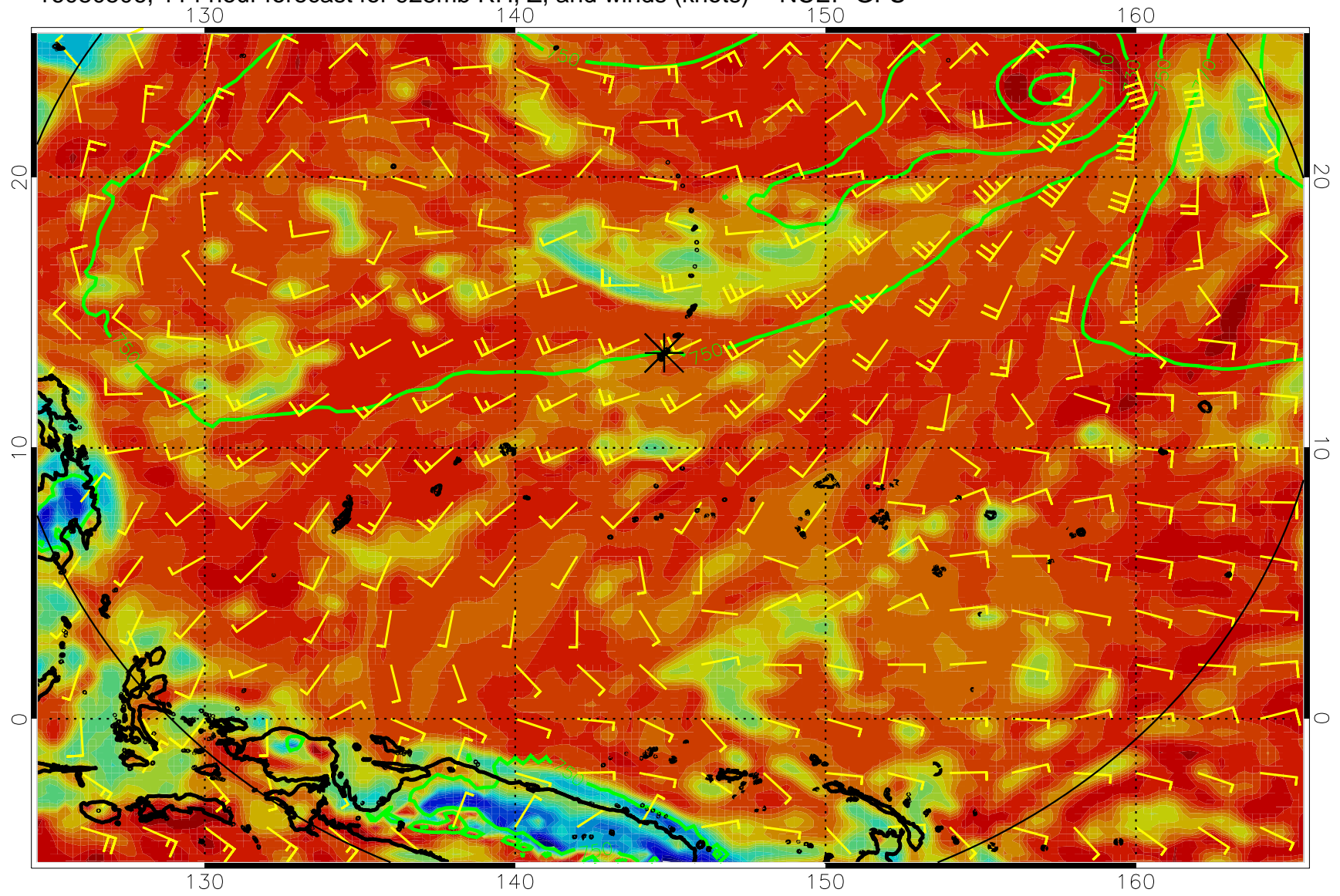
16080506, 114 hour forecast for 925mb RH, Z, and winds (knots) -- NCEP GFS
