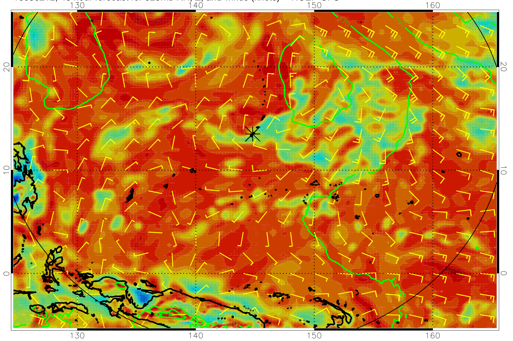
16080212, 48 hour forecast for 925mb RH, Z, and winds (knots) -- NCEP GFS
