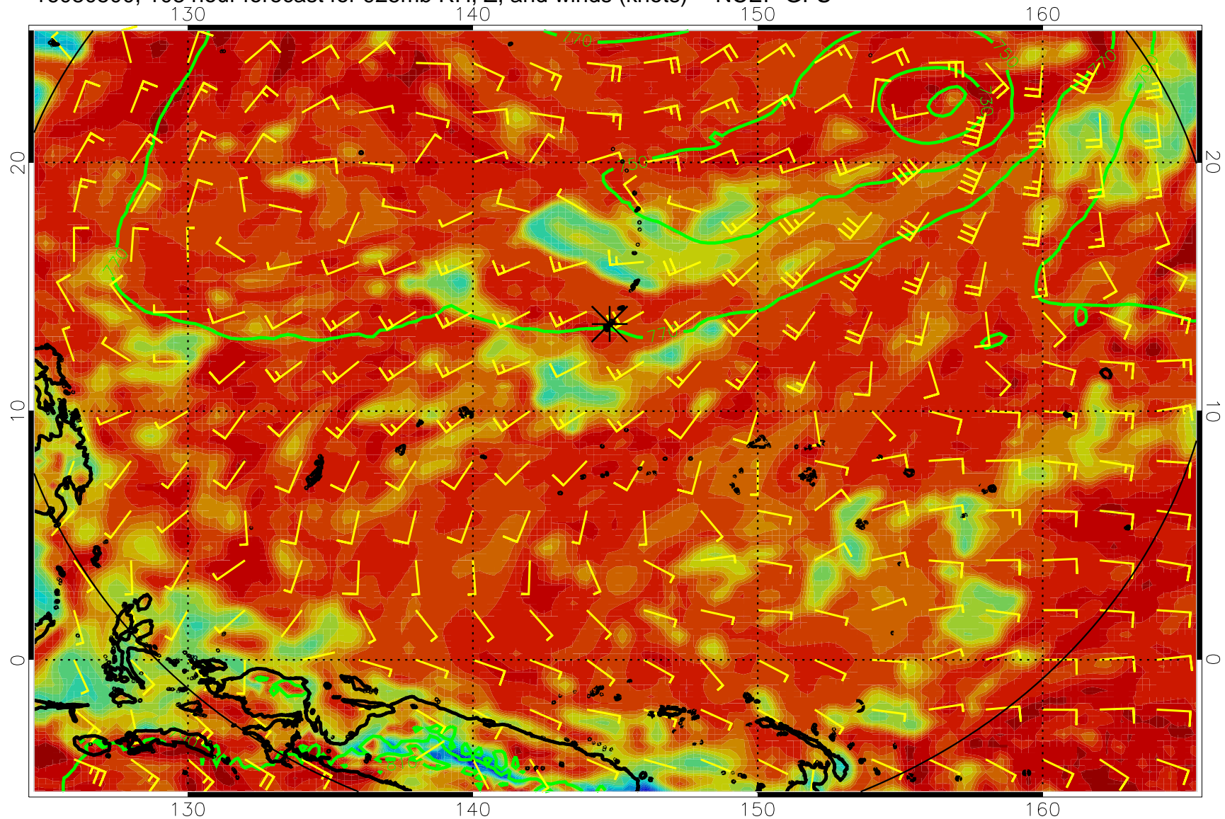
16080500, 108 hour forecast for 925mb RH, Z, and winds (knots) -- NCEP GFS
