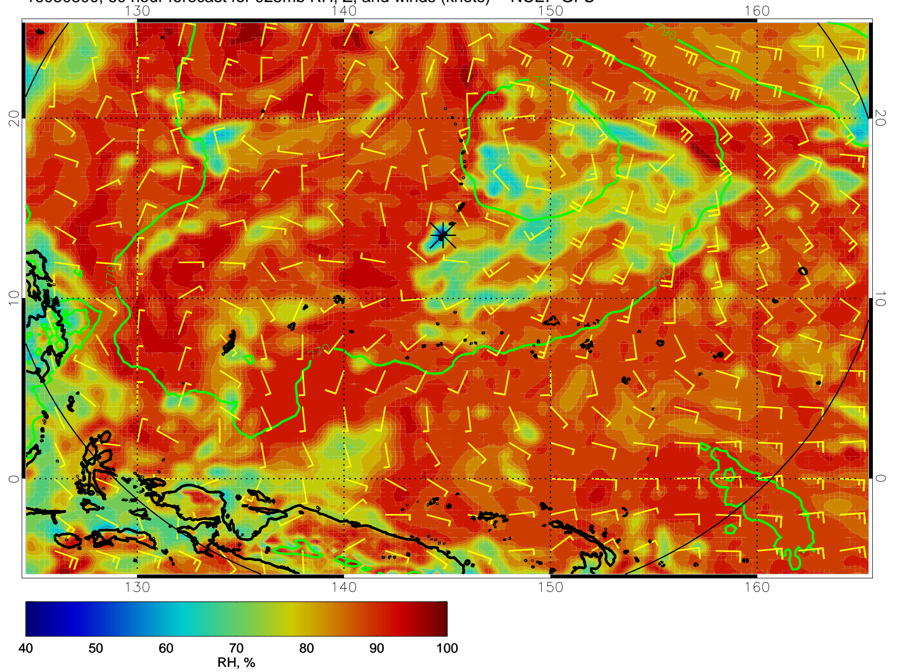
16080300, 60 hour forecast for 925mb RH, Z, and winds (knots) -- NCEP GFS
