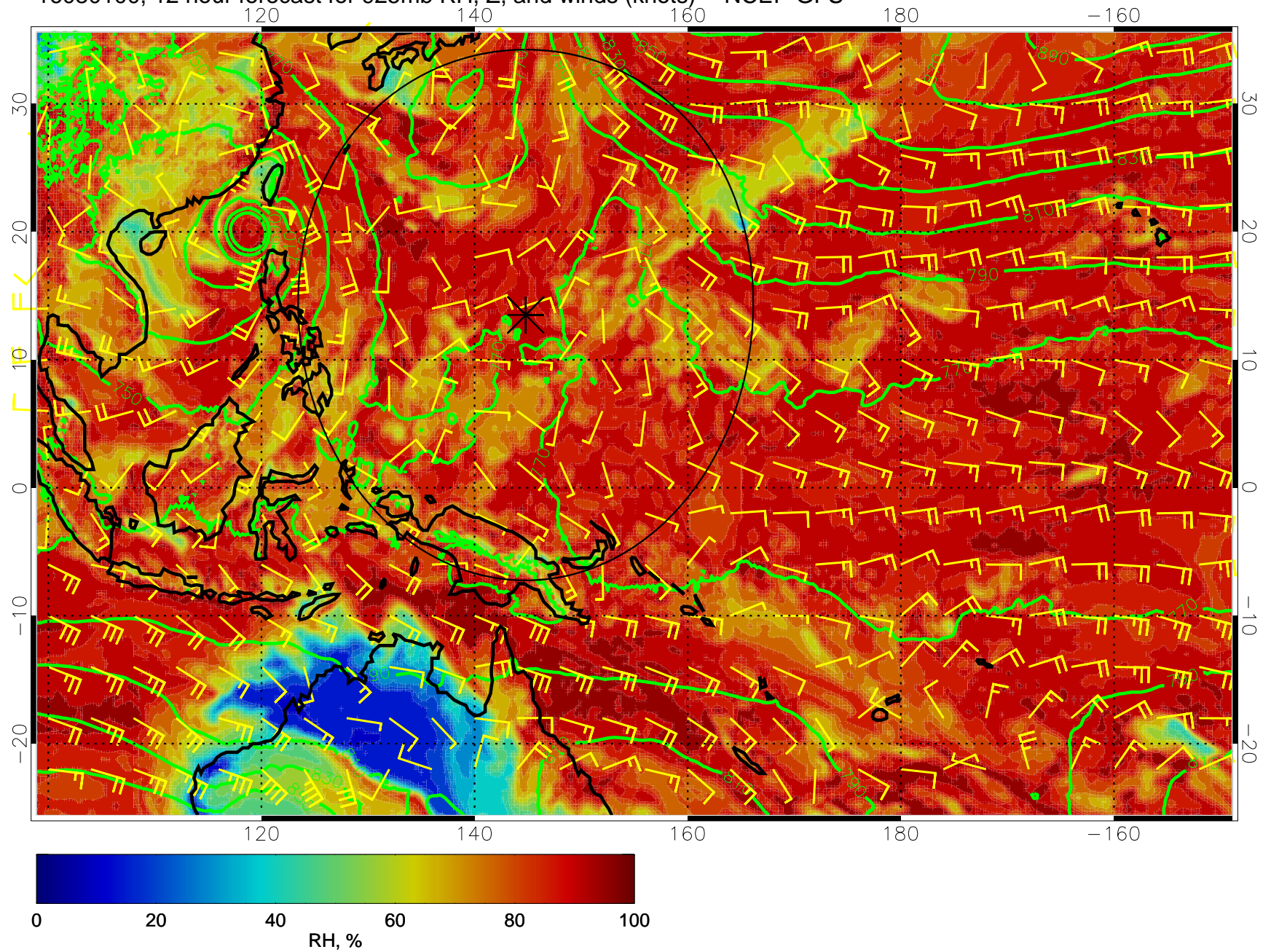
16080100, 12 hour forecast for 925mb RH, Z, and winds (knots) -- NCEP GFS
