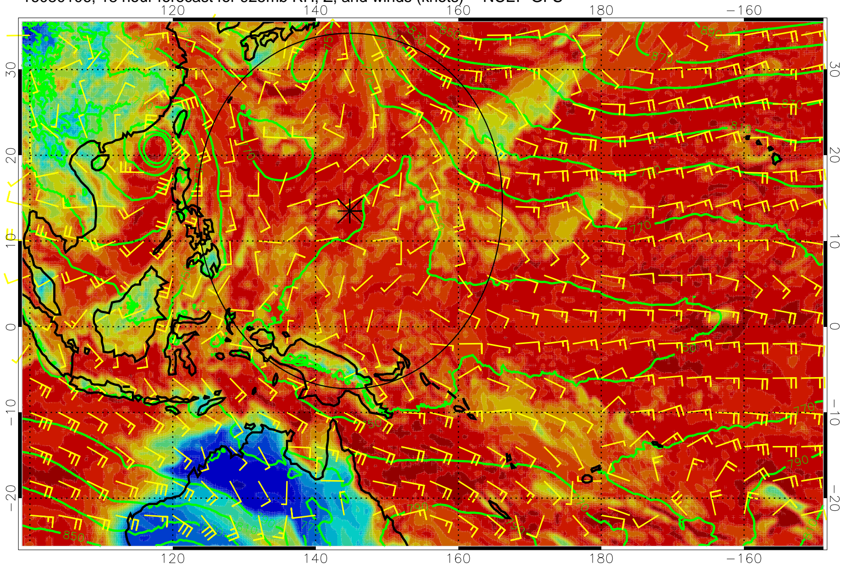
16080106, 18 hour forecast for 925mb RH, Z, and winds (knots) -- NCEP GFS
