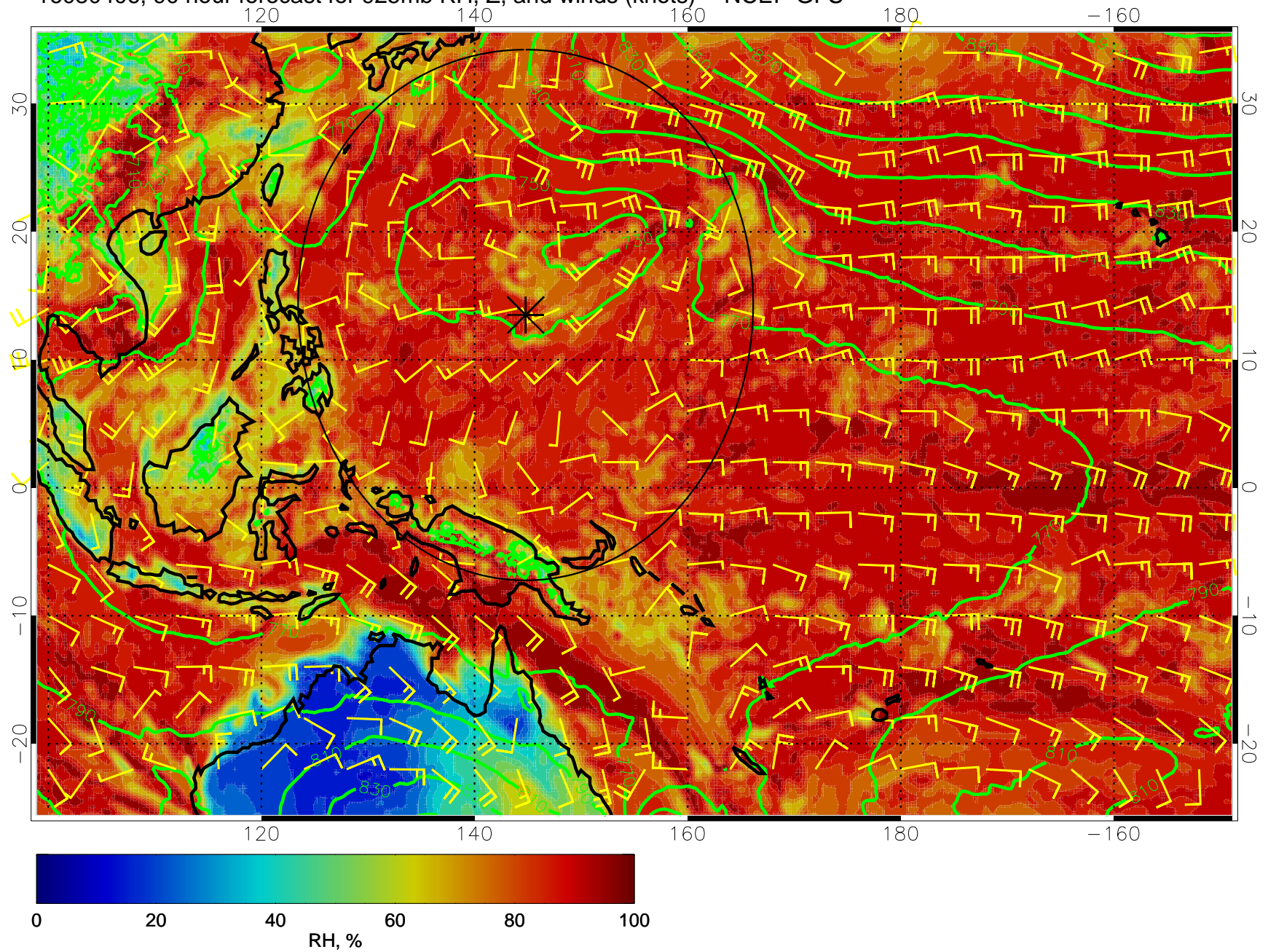
16080406, 90 hour forecast for 925mb RH, Z, and winds (knots) -- NCEP GFS
