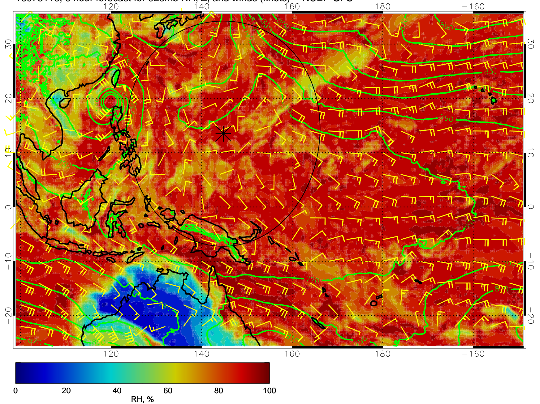
16073118, 6 hour forecast for 925mb RH, Z, and winds (knots) -- NCEP GFS
