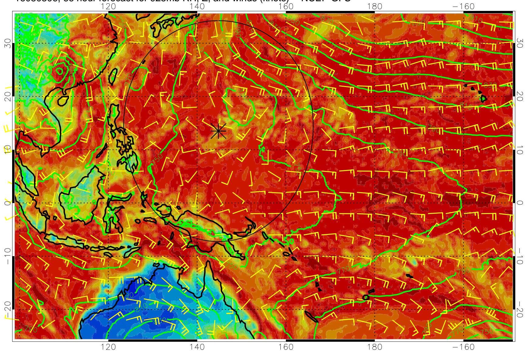
16080306, 66 hour forecast for 925mb RH, Z, and winds (knots) -- NCEP GFS
