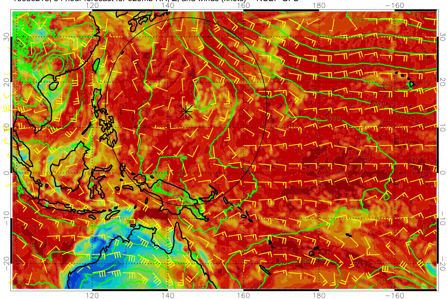
16080218, 54 hour forecast for 925mb RH, Z, and winds (knots) -- NCEP GFS
