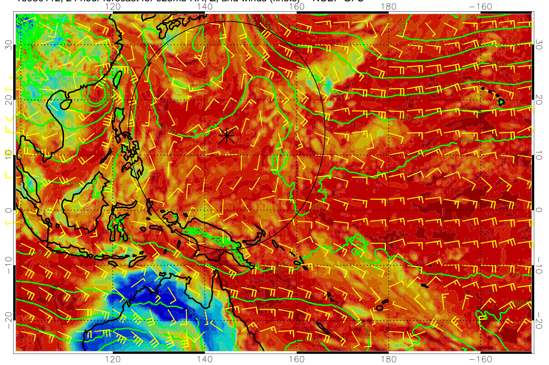
16080112, 24 hour forecast for 925mb RH, Z, and winds (knots) -- NCEP GFS
