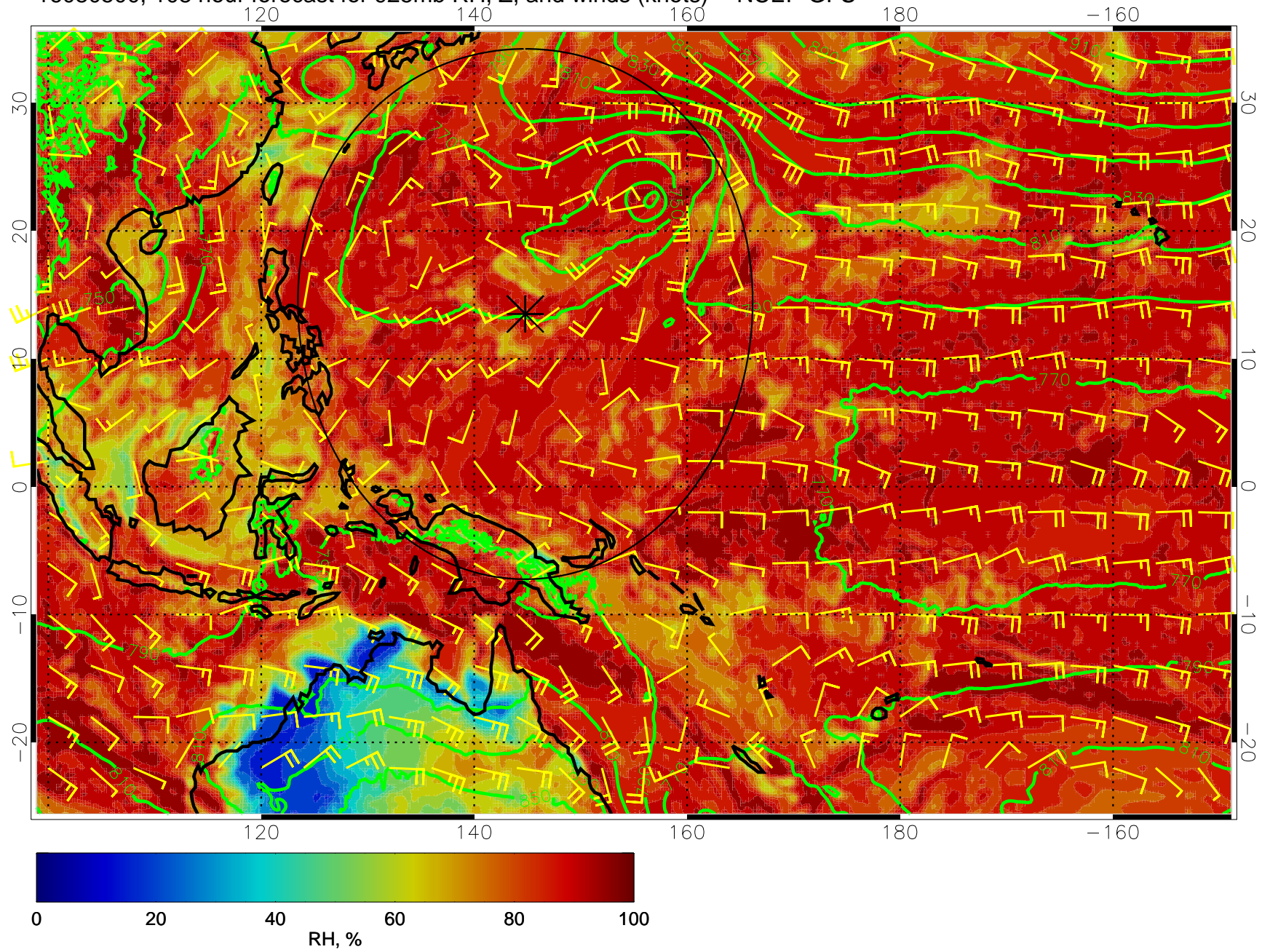
16080500, 108 hour forecast for 925mb RH, Z, and winds (knots) -- NCEP GFS
