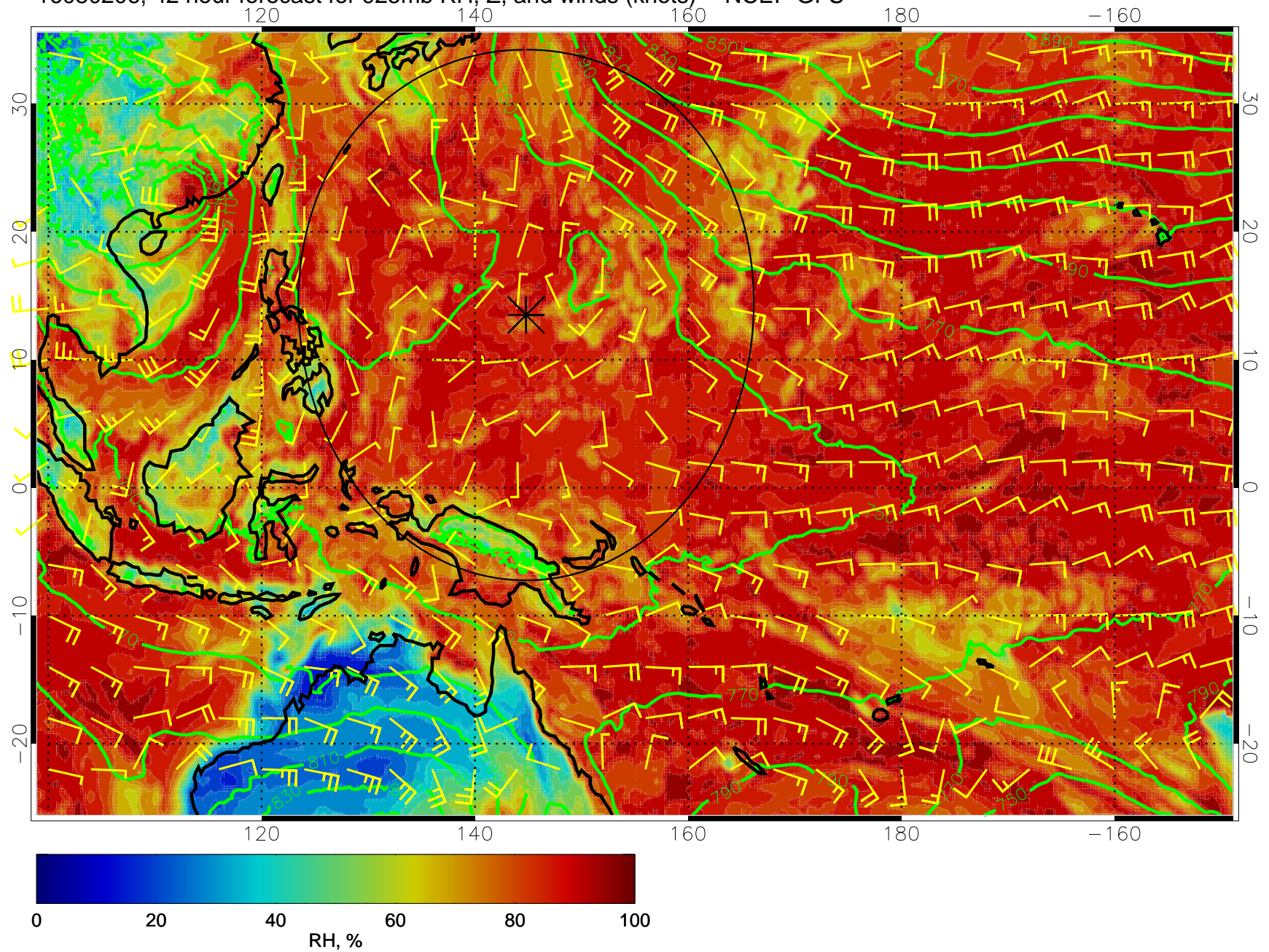
16080206, 42 hour forecast for 925mb RH, Z, and winds (knots) -- NCEP GFS
