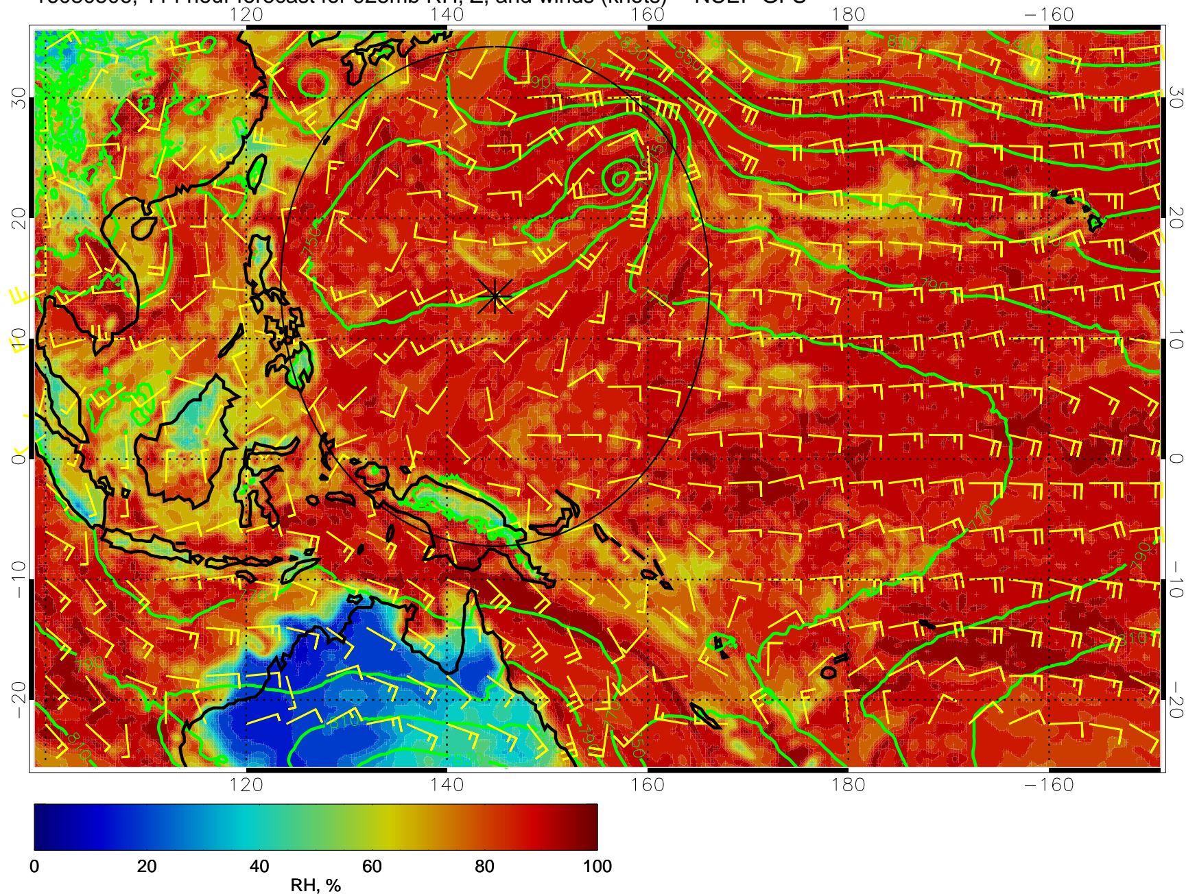
16080506, 114 hour forecast for 925mb RH, Z, and winds (knots) -- NCEP GFS
