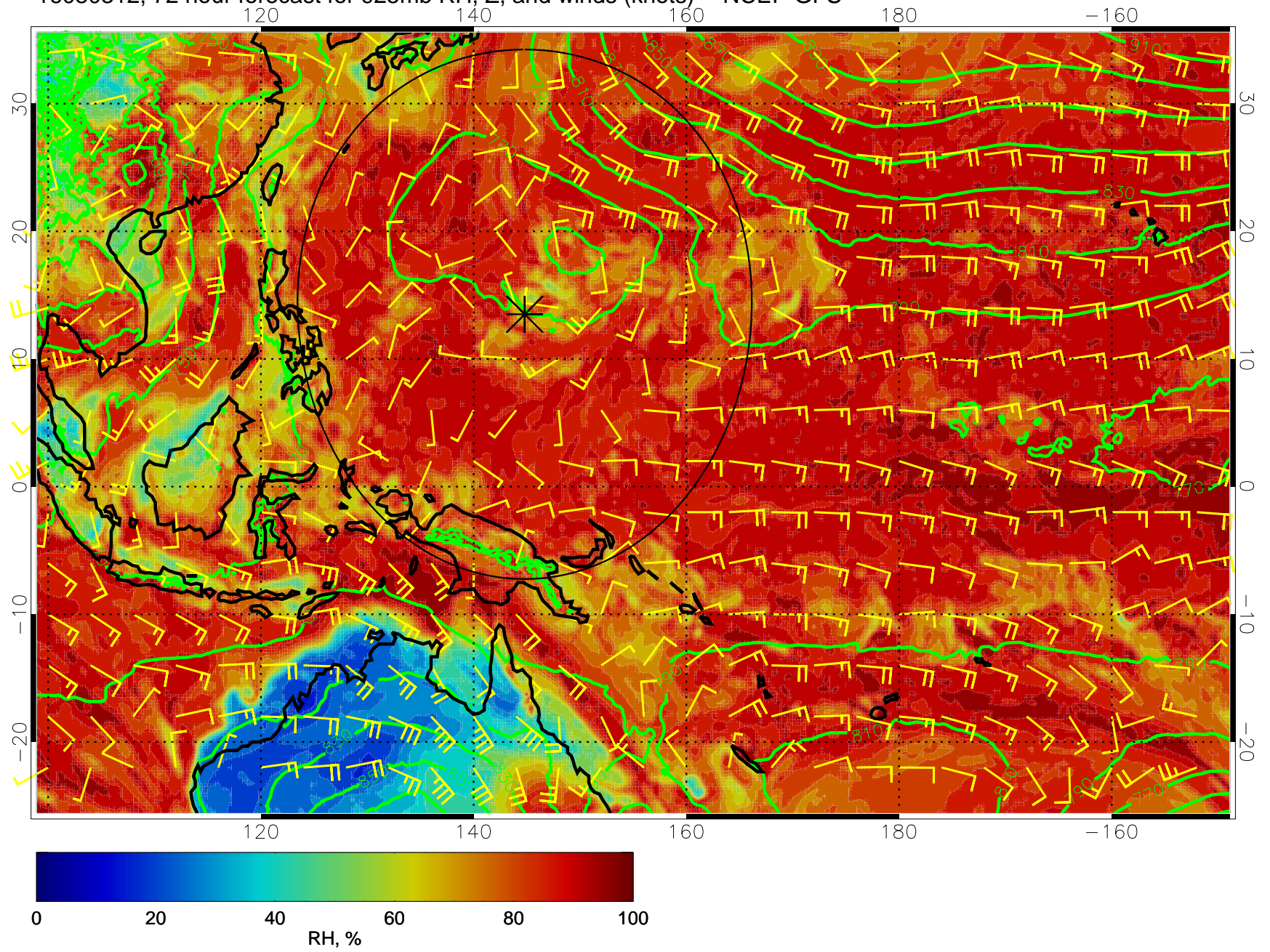
16080312, 72 hour forecast for 925mb RH, Z, and winds (knots) -- NCEP GFS
