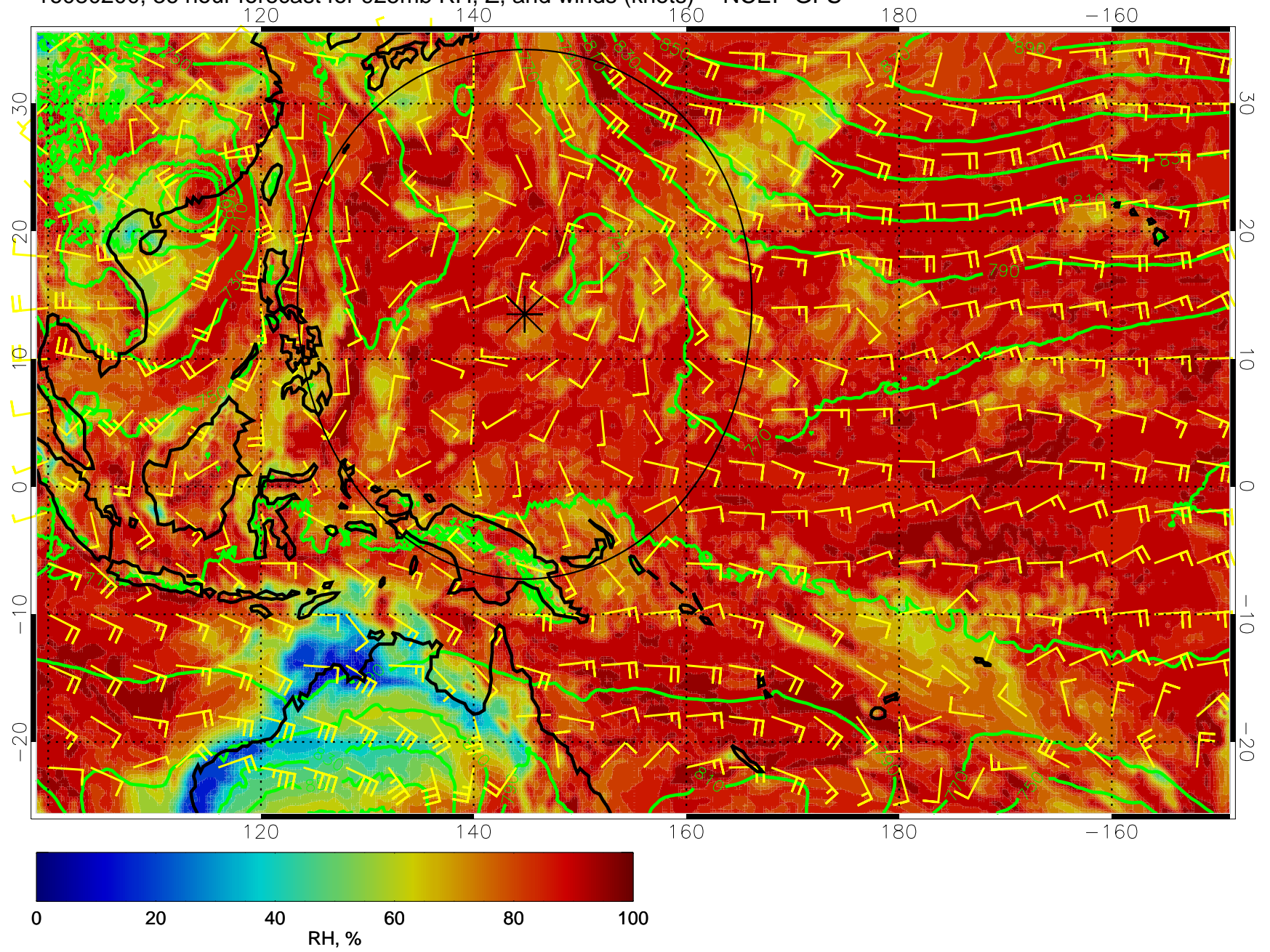
16080200, 36 hour forecast for 925mb RH, Z, and winds (knots) -- NCEP GFS
