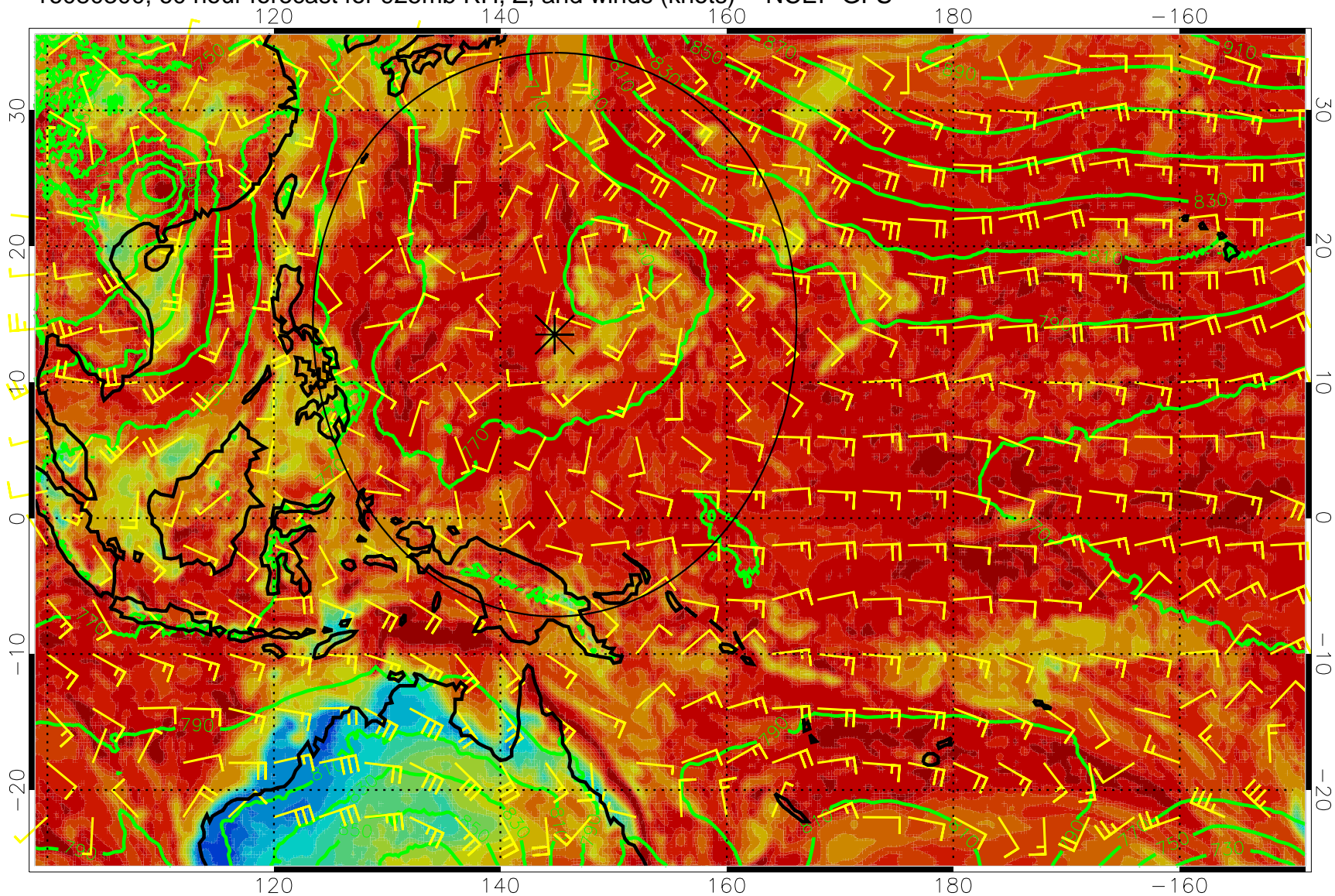
16080300, 60 hour forecast for 925mb RH, Z, and winds (knots) -- NCEP GFS
