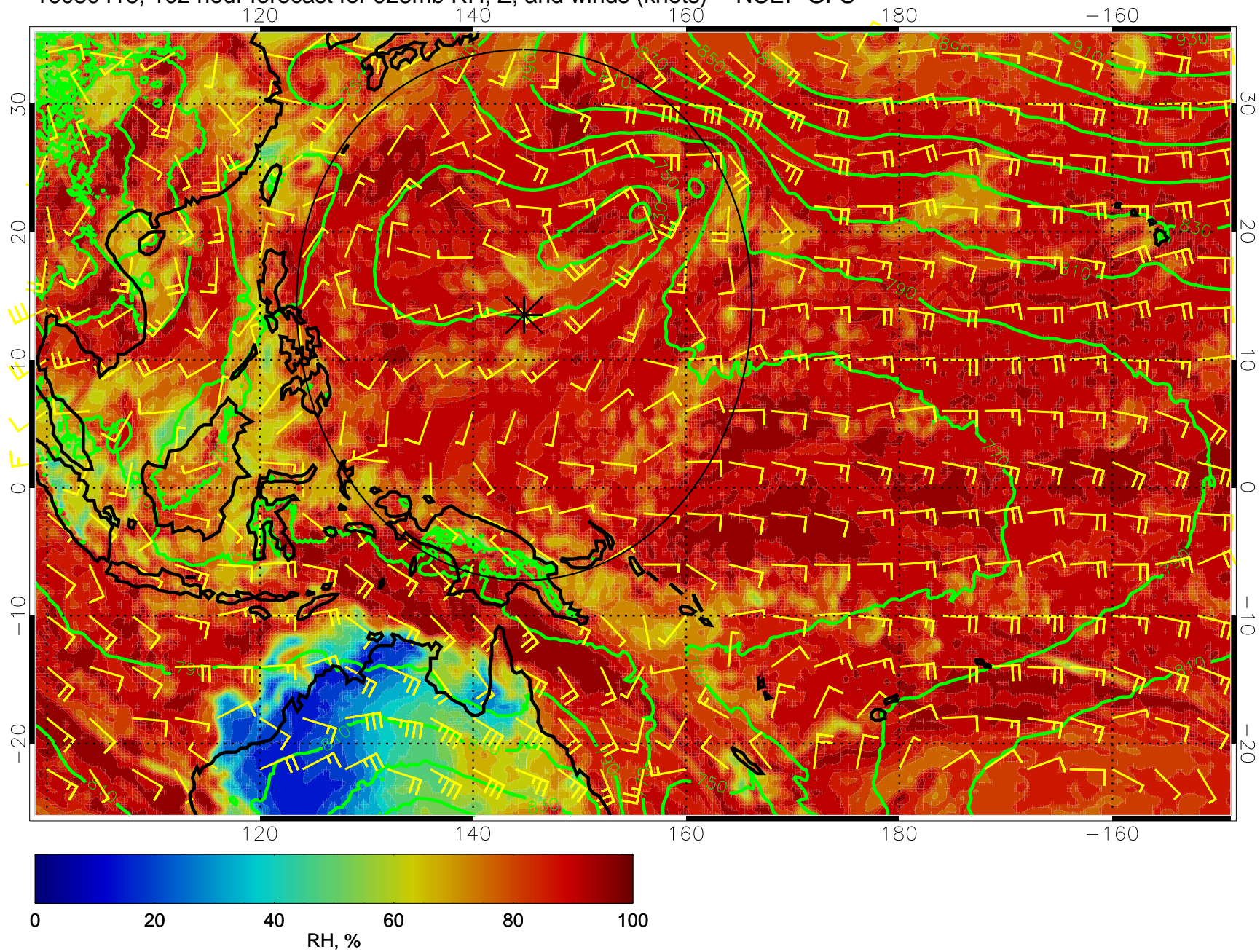
16080418, 102 hour forecast for 925mb RH, Z, and winds (knots) -- NCEP GFS
