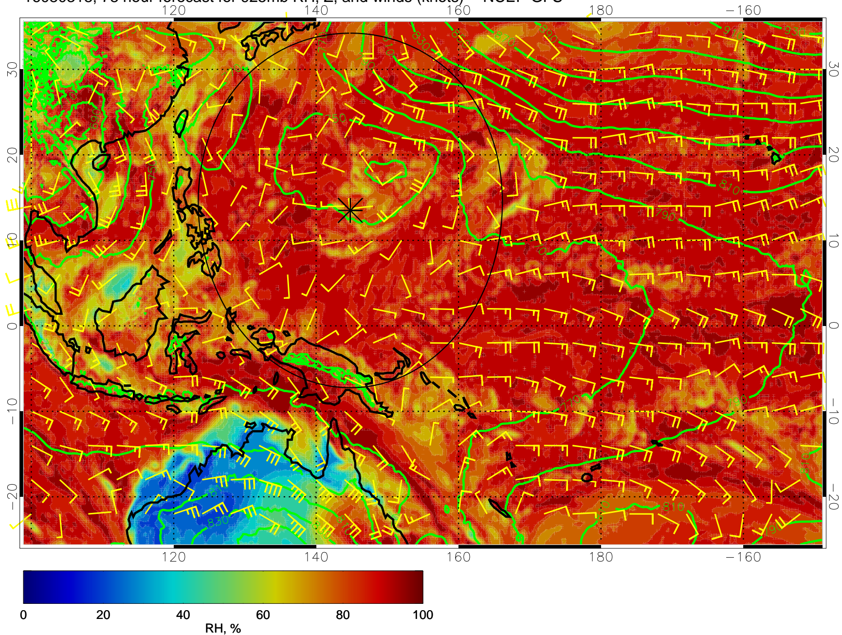
16080318, 78 hour forecast for 925mb RH, Z, and winds (knots) -- NCEP GFS
