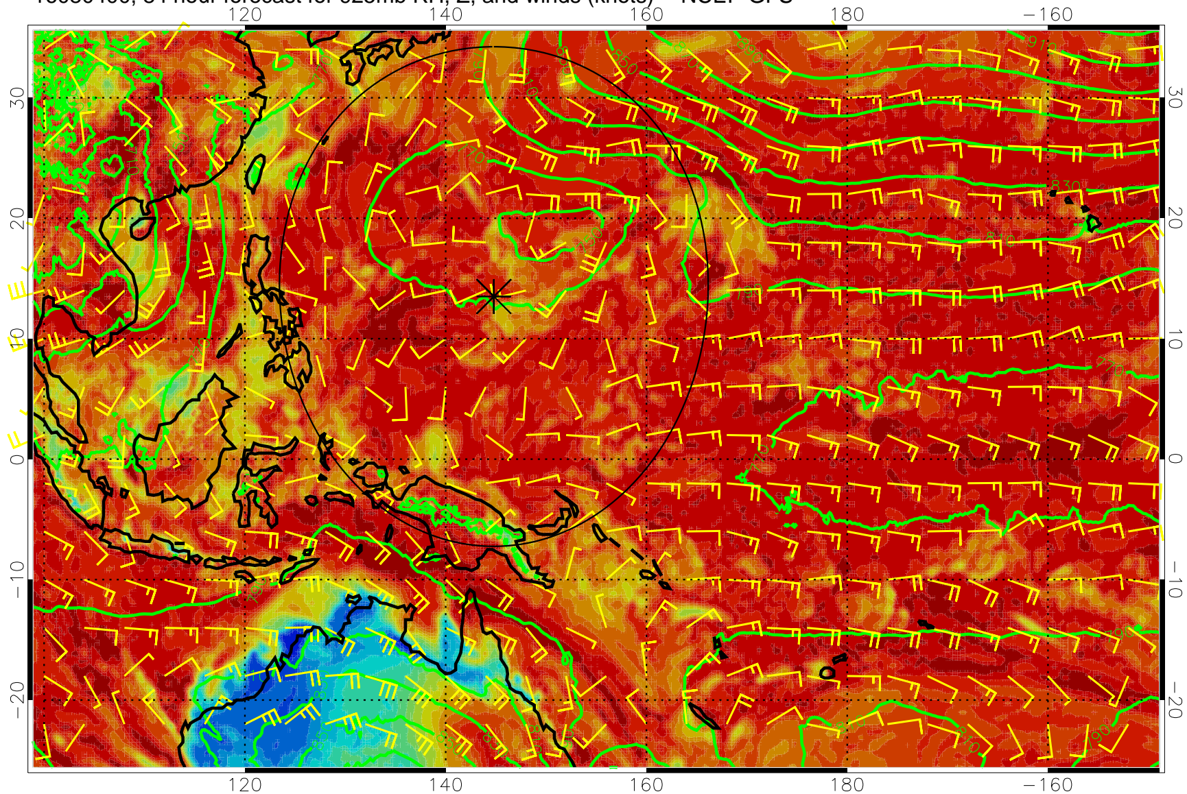
16080400, 84 hour forecast for 925mb RH, Z, and winds (knots) -- NCEP GFS
