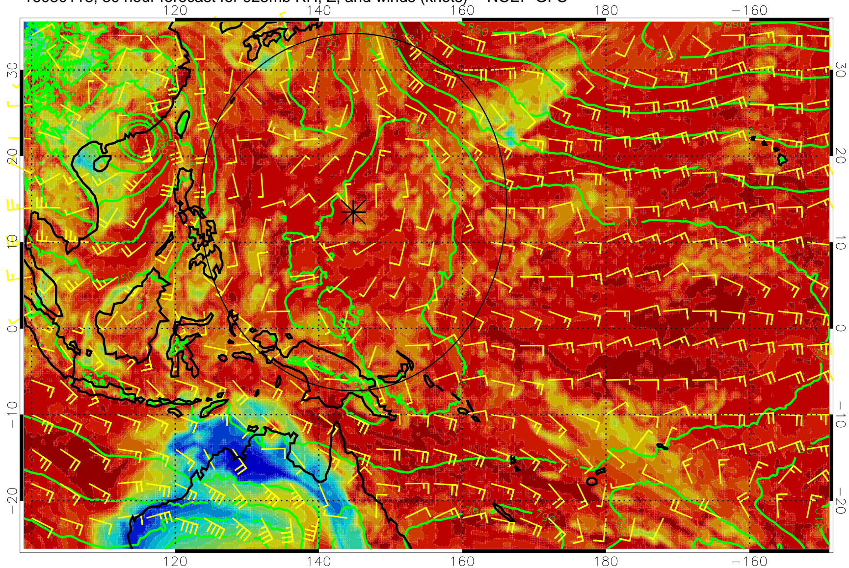
16080118, 30 hour forecast for 925mb RH, Z, and winds (knots) -- NCEP GFS
