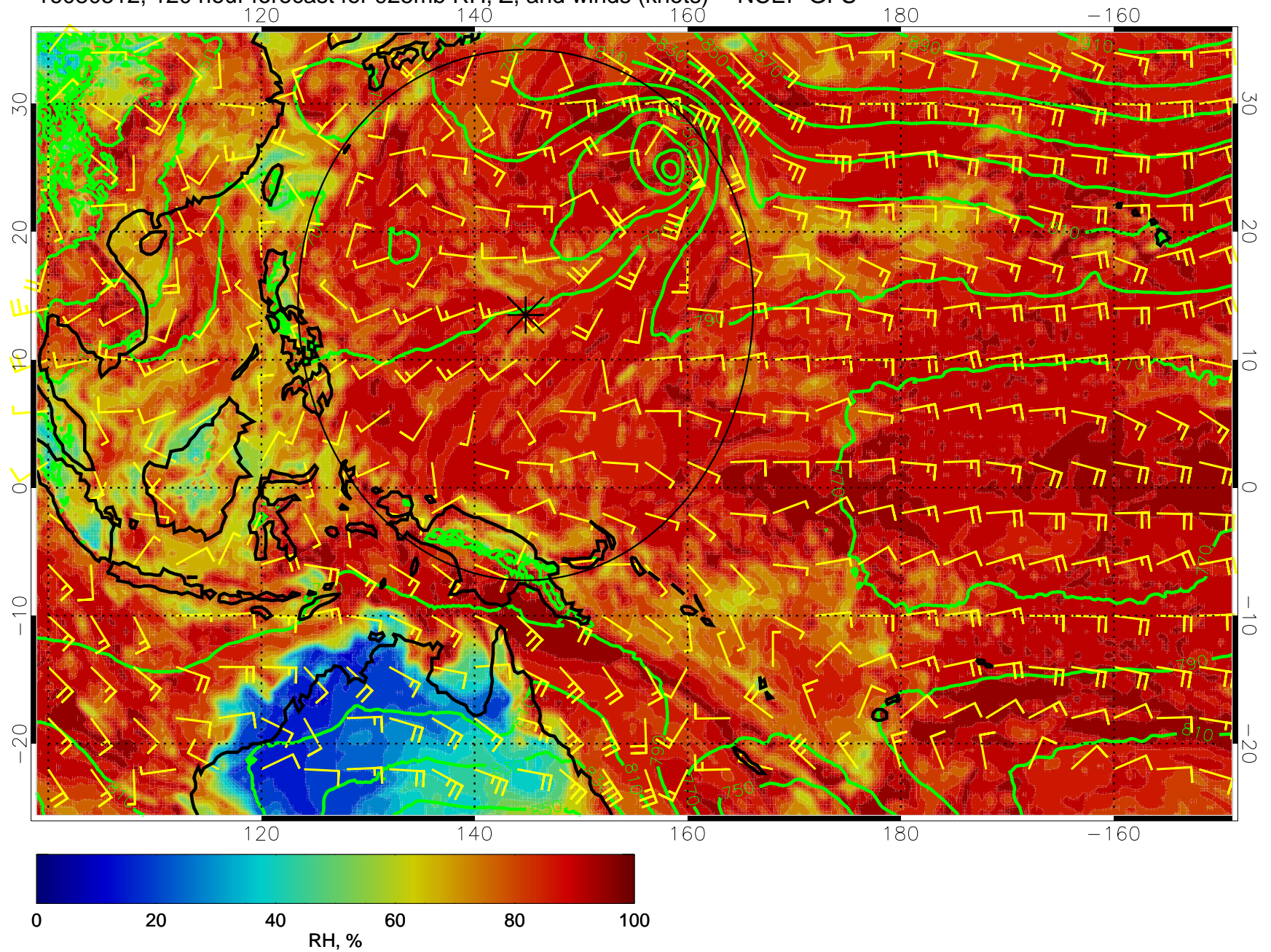
16080512, 120 hour forecast for 925mb RH, Z, and winds (knots) -- NCEP GFS
