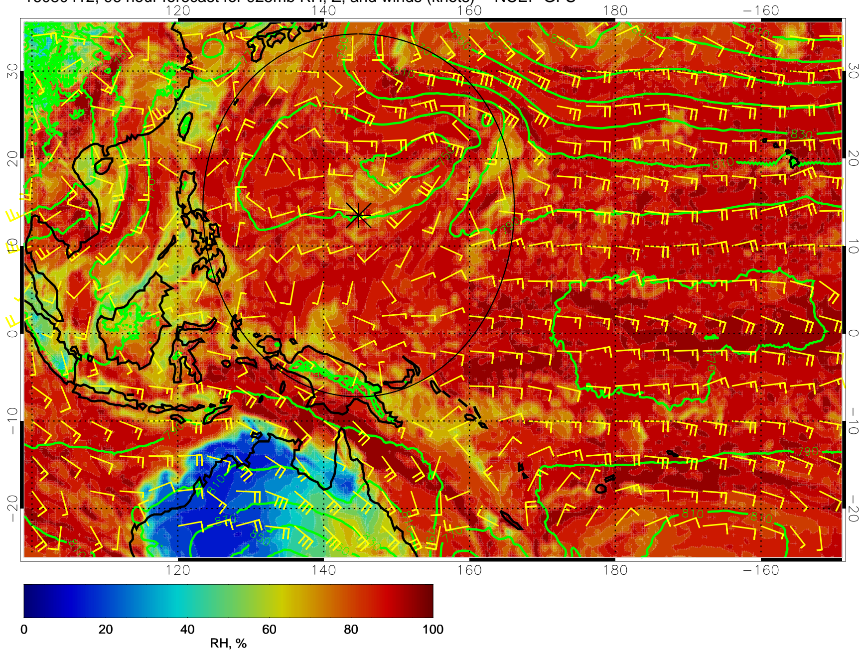
16080412, 96 hour forecast for 925mb RH, Z, and winds (knots) -- NCEP GFS
