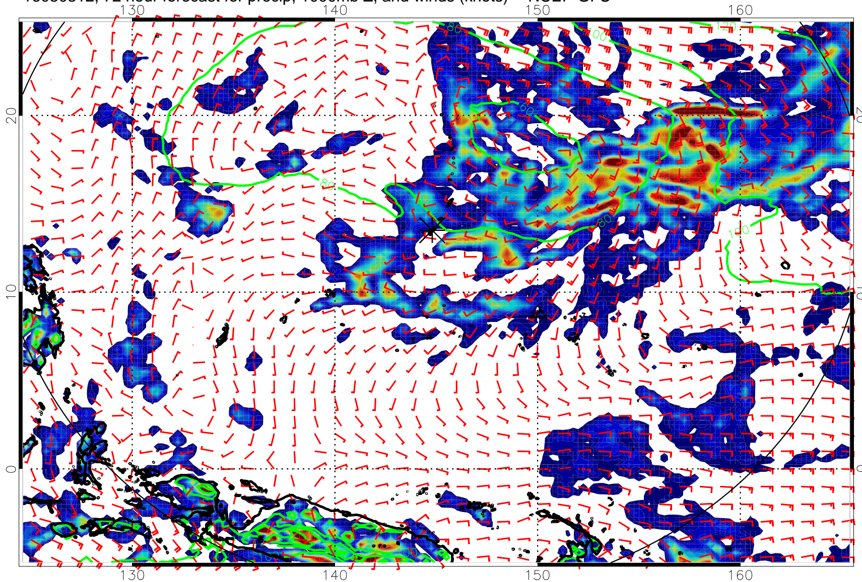
16080312, 72 hour forecast for precip, 1000mb Z, and winds (knots) -- NCEP GFS
