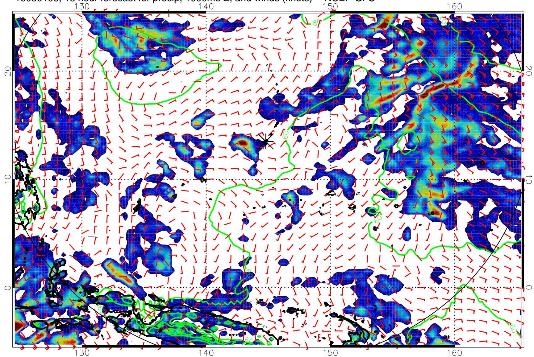
16080106, 18 hour forecast for precip, 1000mb Z, and winds (knots) -- NCEP GFS
