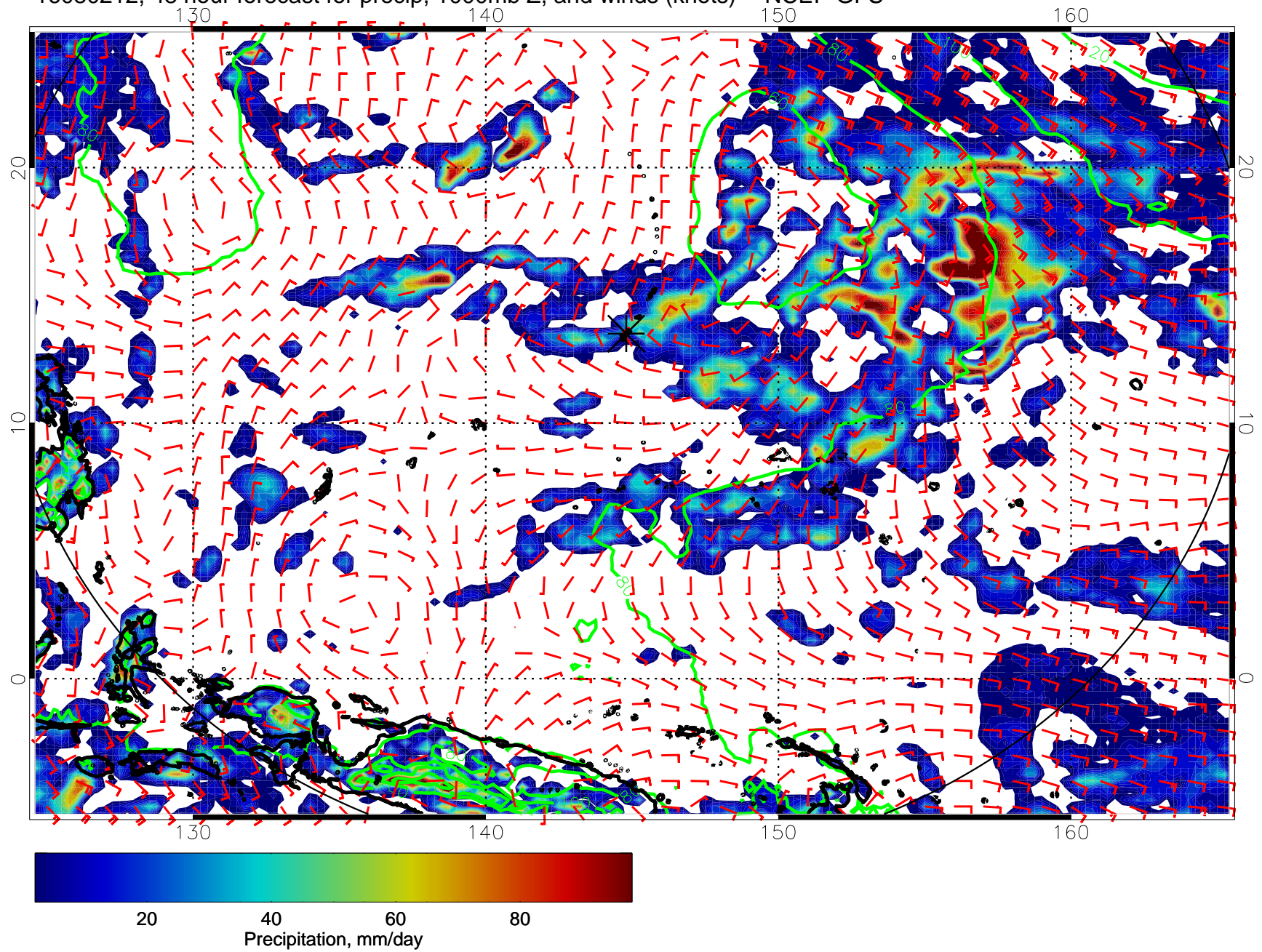
16080212, 48 hour forecast for precip, 1000mb Z, and winds (knots) -- NCEP GFS
