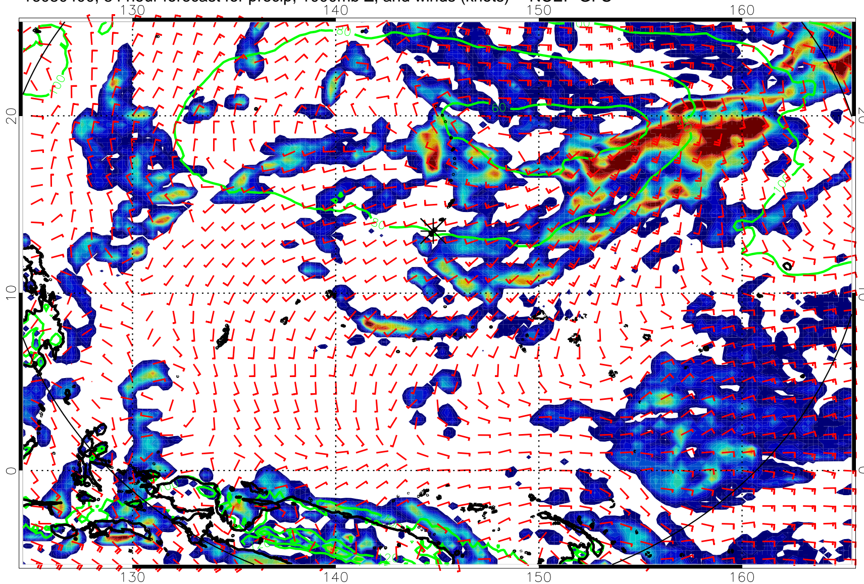
16080400, 84 hour forecast for precip, 1000mb Z, and winds (knots) -- NCEP GFS
