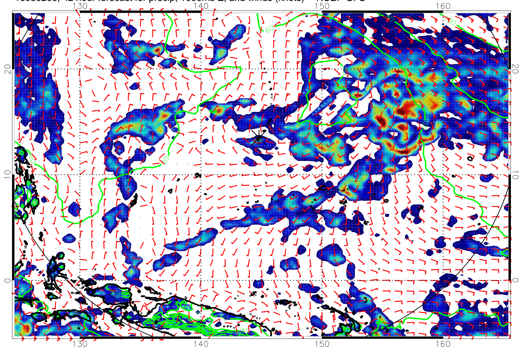
16080206, 42 hour forecast for precip, 1000mb Z, and winds (knots) -- NCEP GFS
