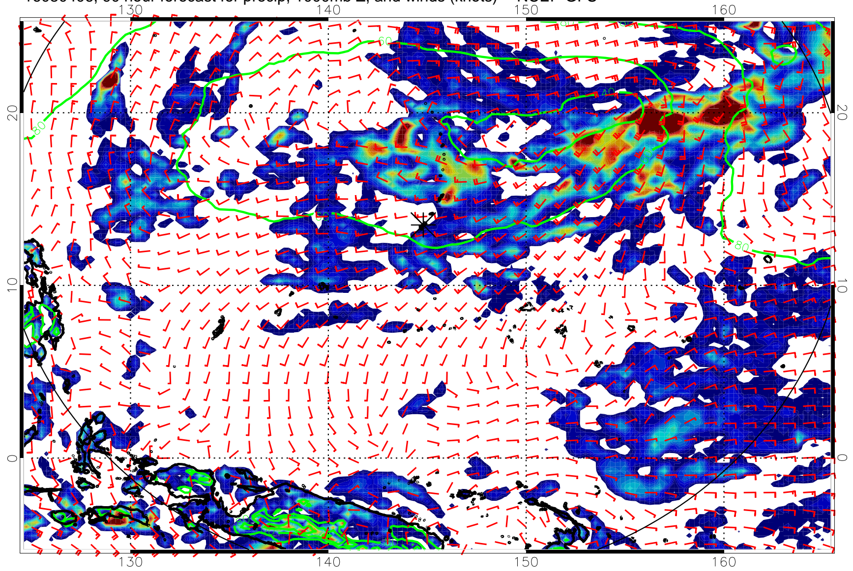
16080406, 90 hour forecast for precip, 1000mb Z, and winds (knots) -- NCEP GFS
