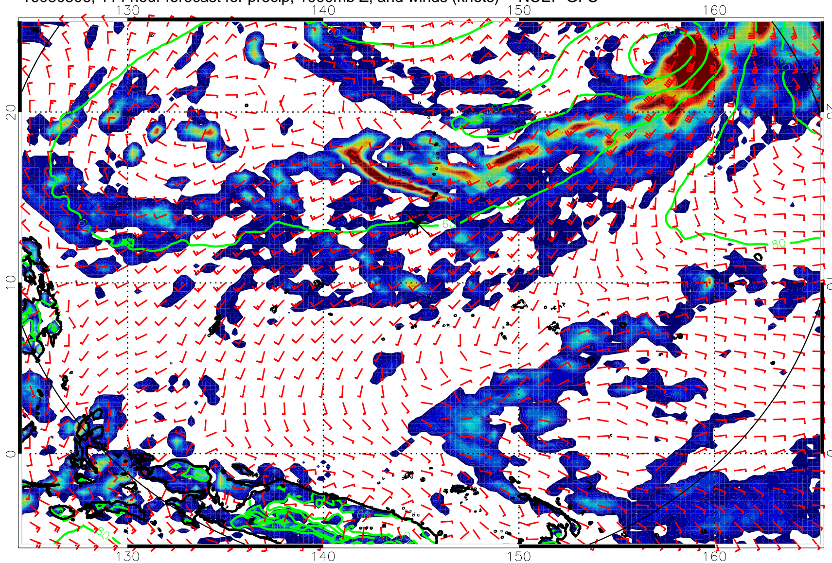
16080506, 114 hour forecast for precip, 1000mb Z, and winds (knots) -- NCEP GFS
