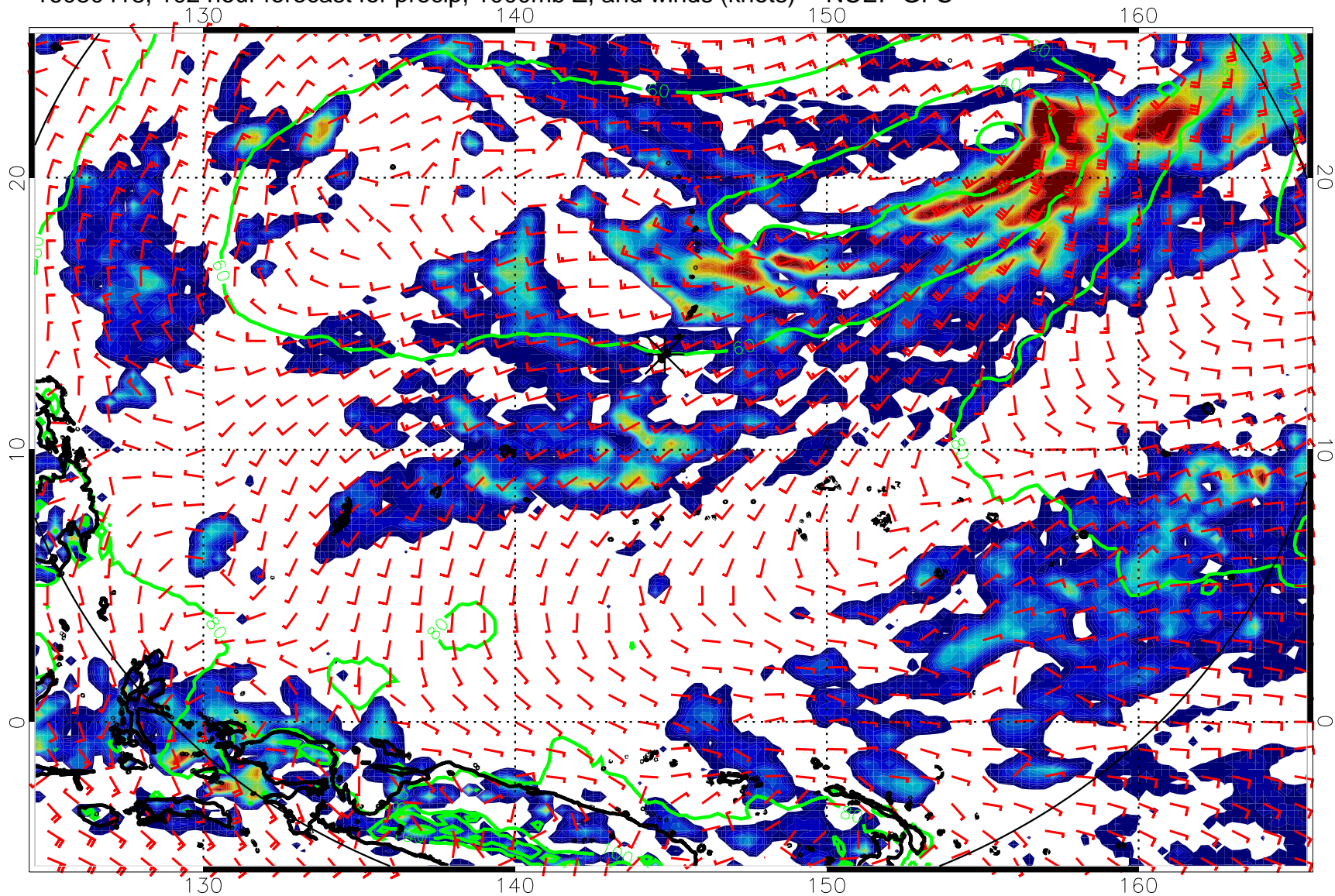
16080418, 102 hour forecast for precip, 1000mb Z, and winds (knots) -- NCEP GFS
