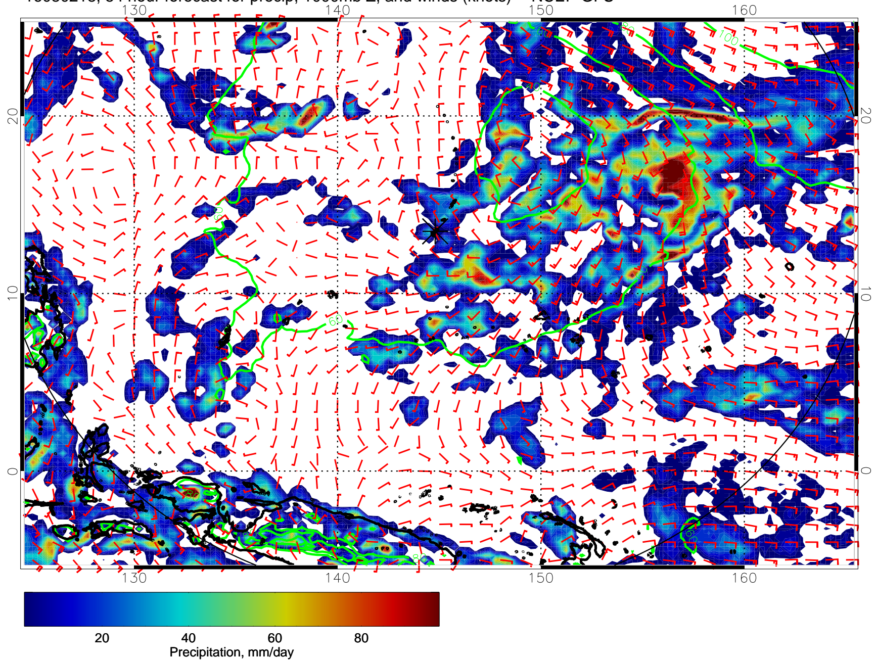
16080218, 54 hour forecast for precip, 1000mb Z, and winds (knots) -- NCEP GFS
