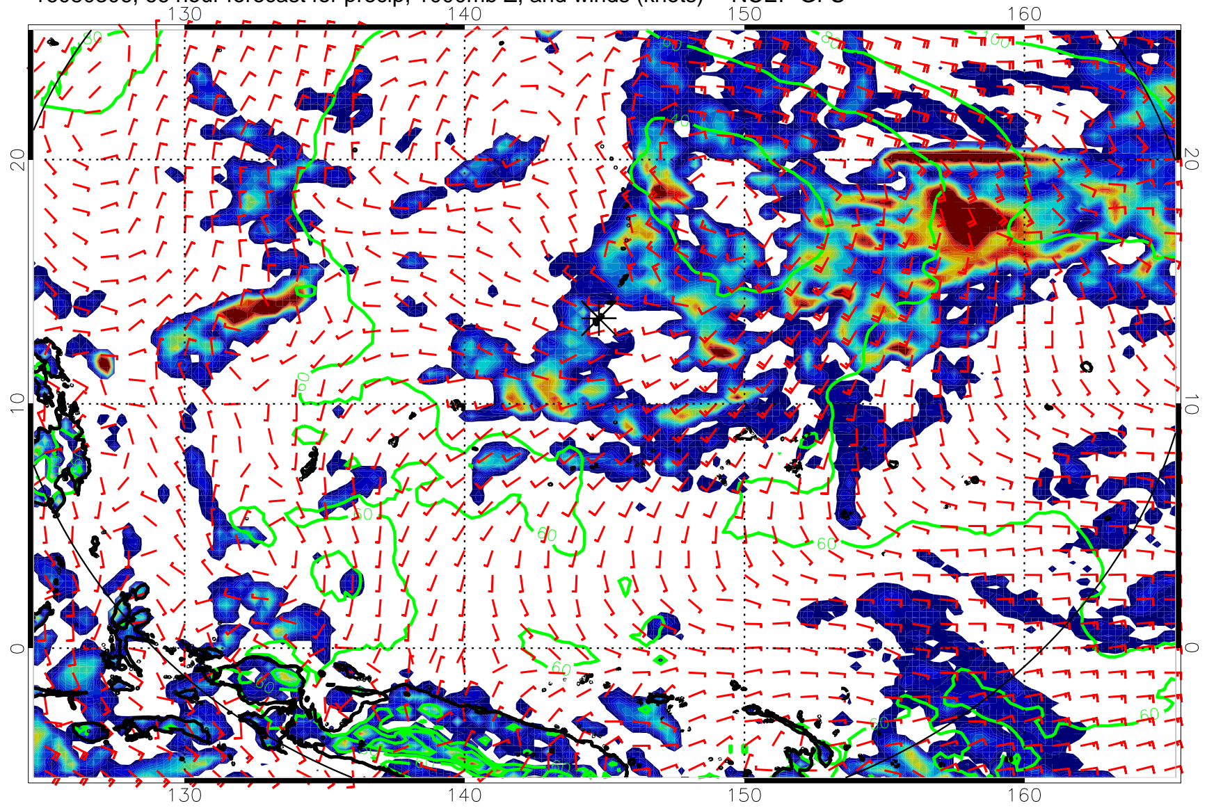
16080306, 66 hour forecast for precip, 1000mb Z, and winds (knots) -- NCEP GFS
