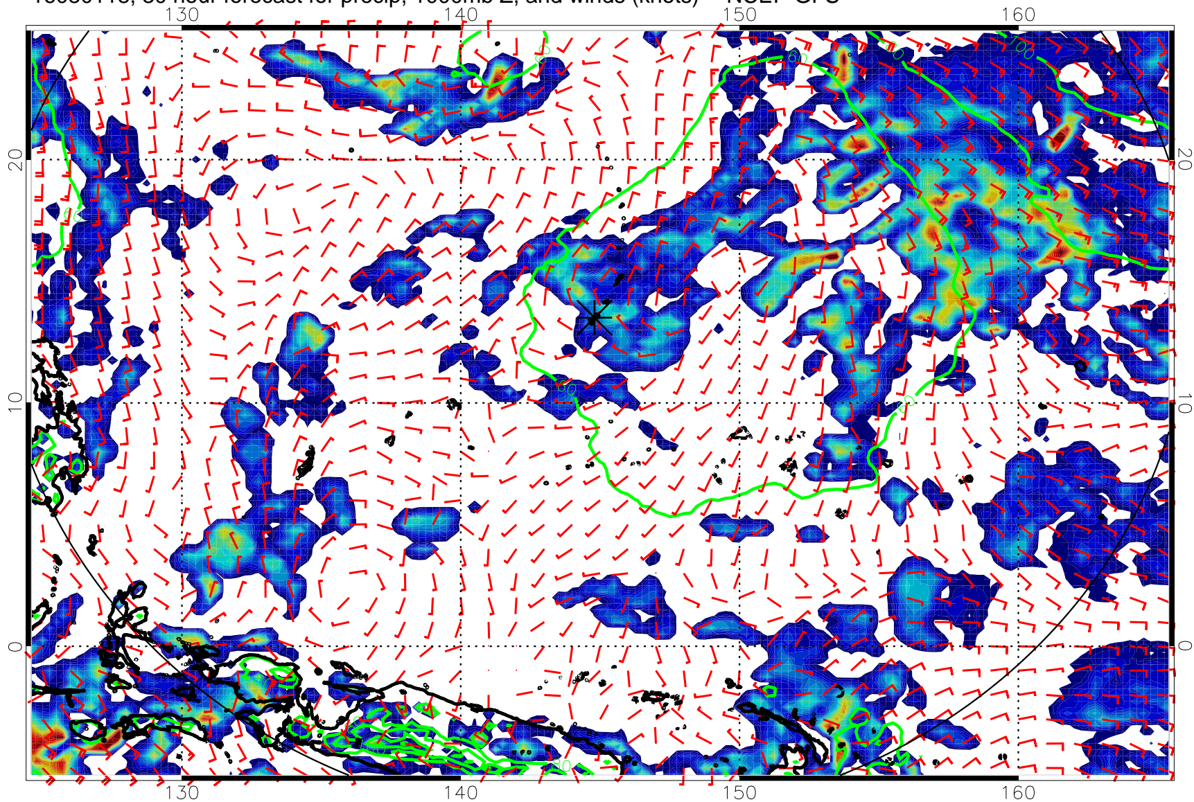
16080118, 30 hour forecast for precip, 1000mb Z, and winds (knots) -- NCEP GFS
