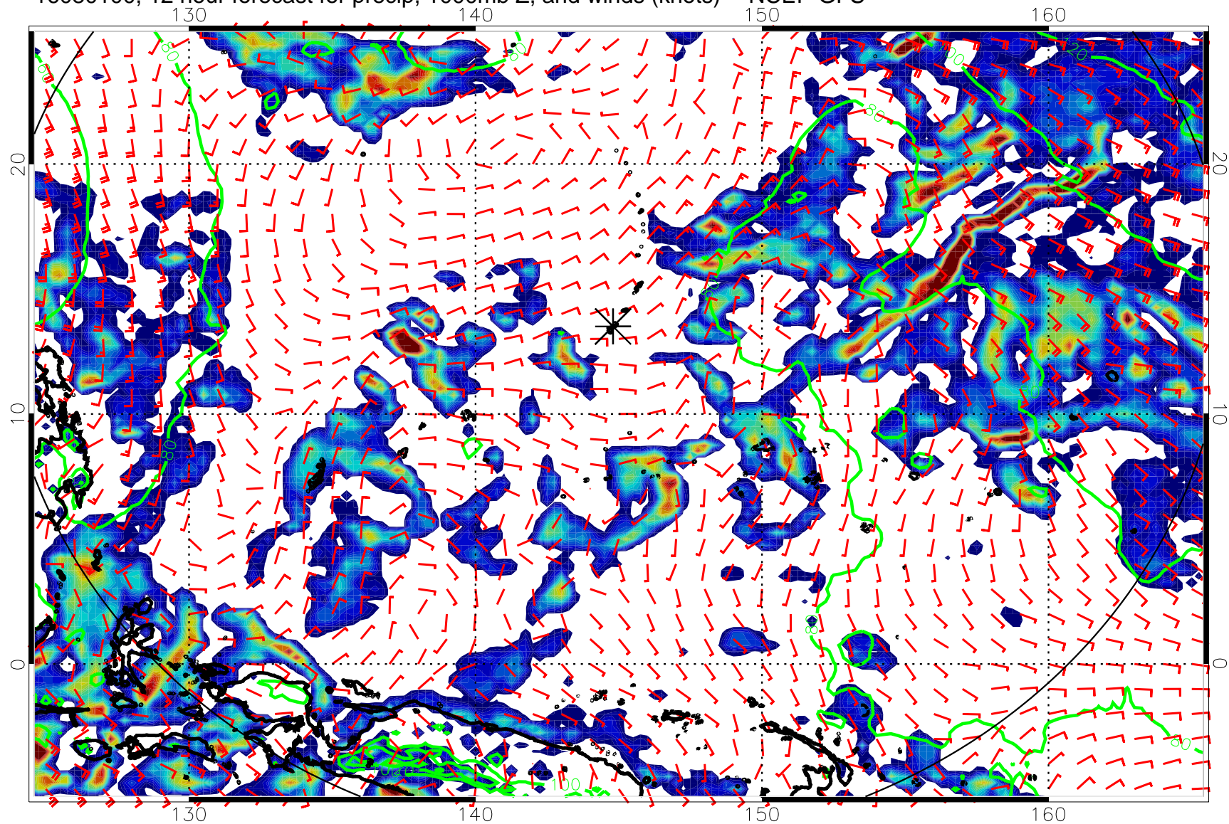
16080100, 12 hour forecast for precip, 1000mb Z, and winds (knots) -- NCEP GFS
