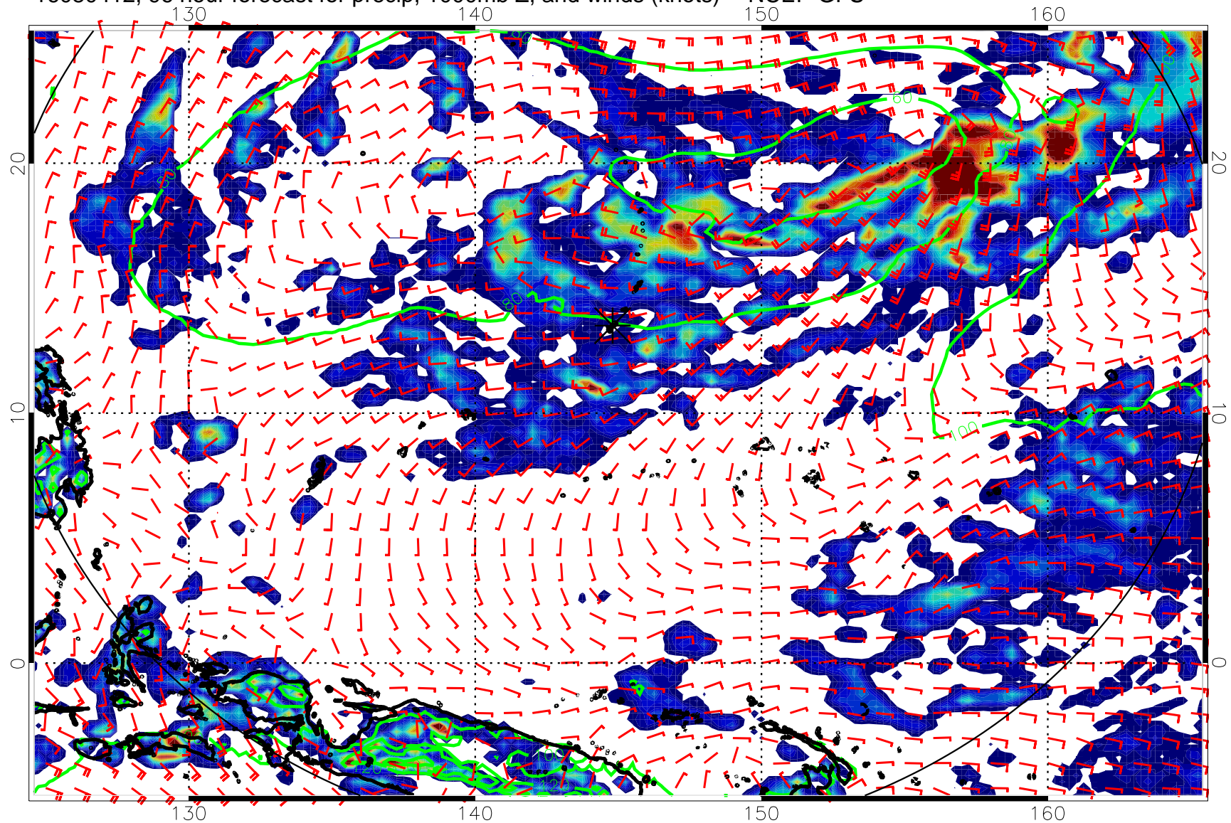
16080412, 96 hour forecast for precip, 1000mb Z, and winds (knots) -- NCEP GFS
