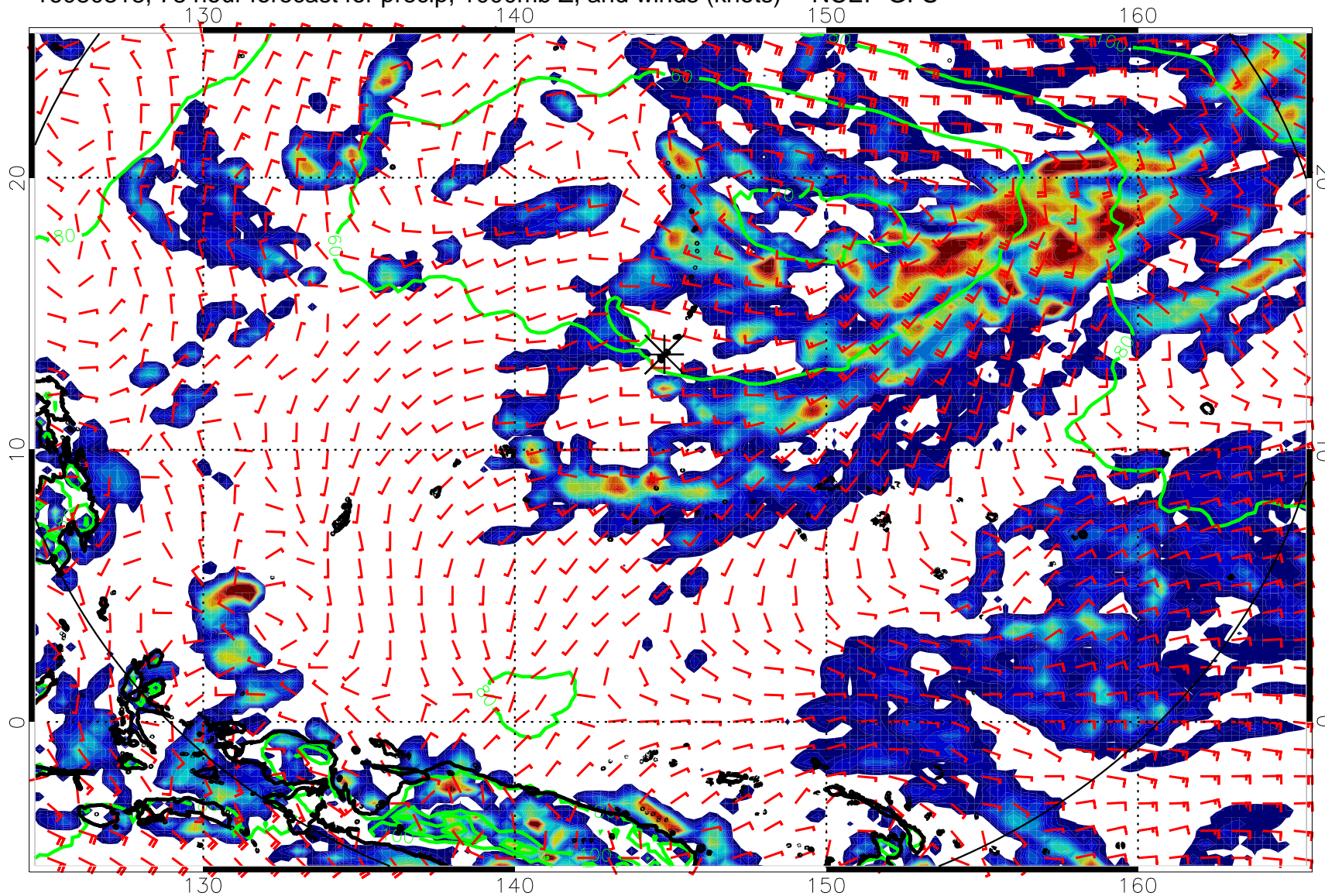
16080318, 78 hour forecast for precip, 1000mb Z, and winds (knots) -- NCEP GFS
