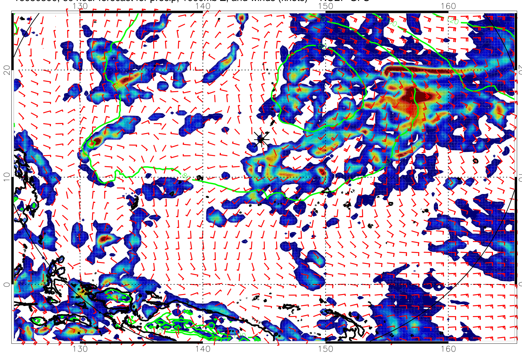
16080300, 60 hour forecast for precip, 1000mb Z, and winds (knots) -- NCEP GFS
