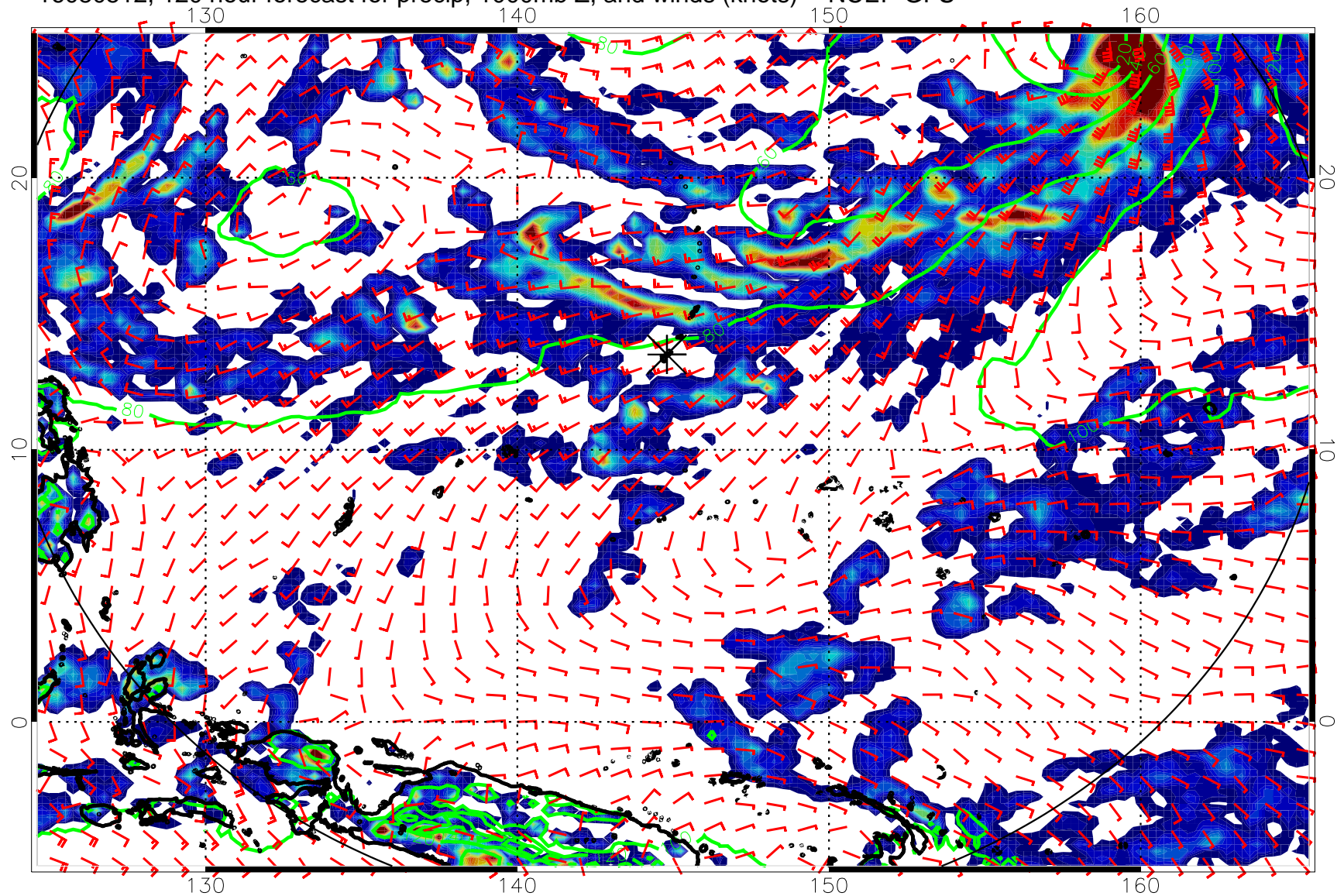
16080512, 120 hour forecast for precip, 1000mb Z, and winds (knots) -- NCEP GFS
