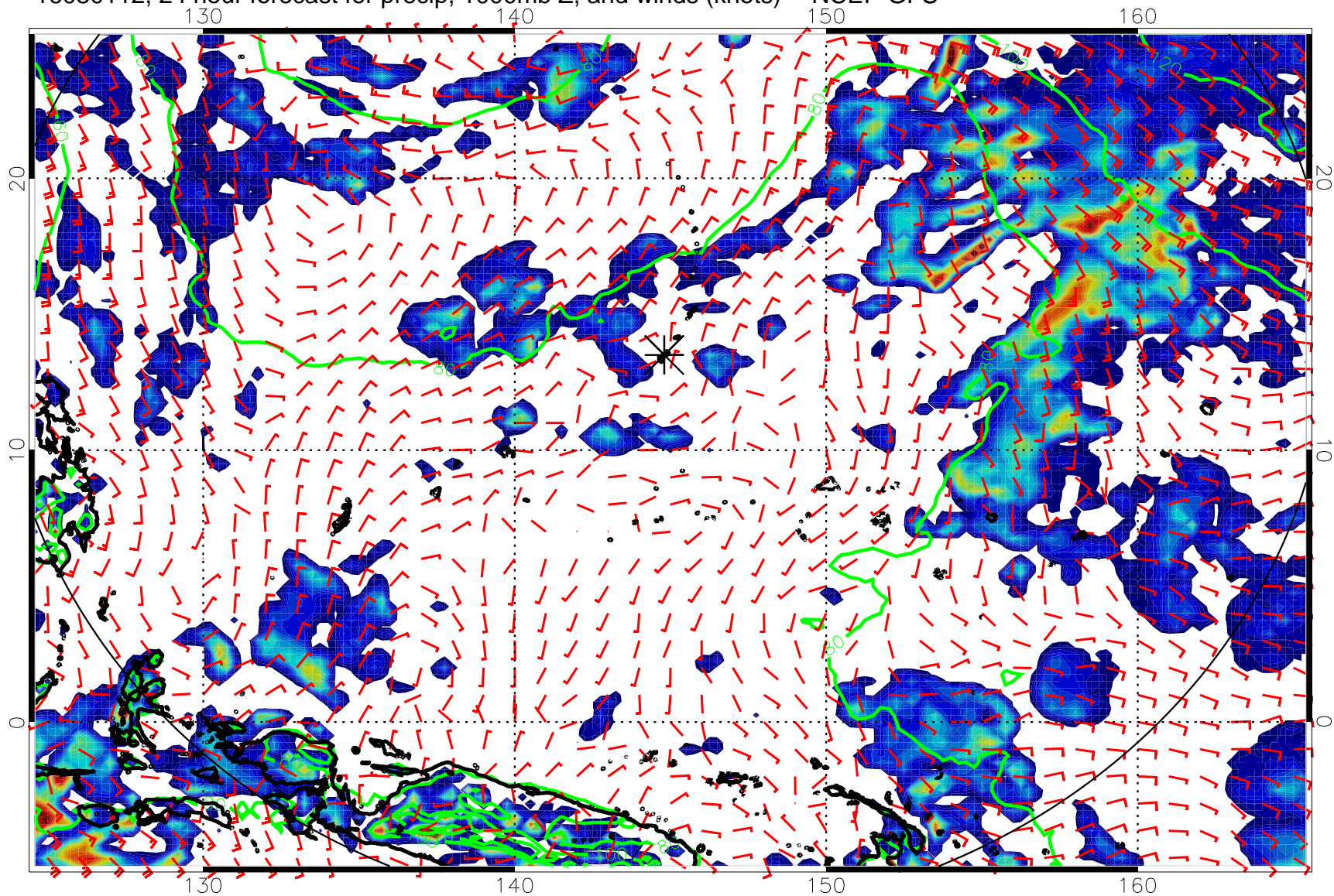
16080112, 24 hour forecast for precip, 1000mb Z, and winds (knots) -- NCEP GFS
