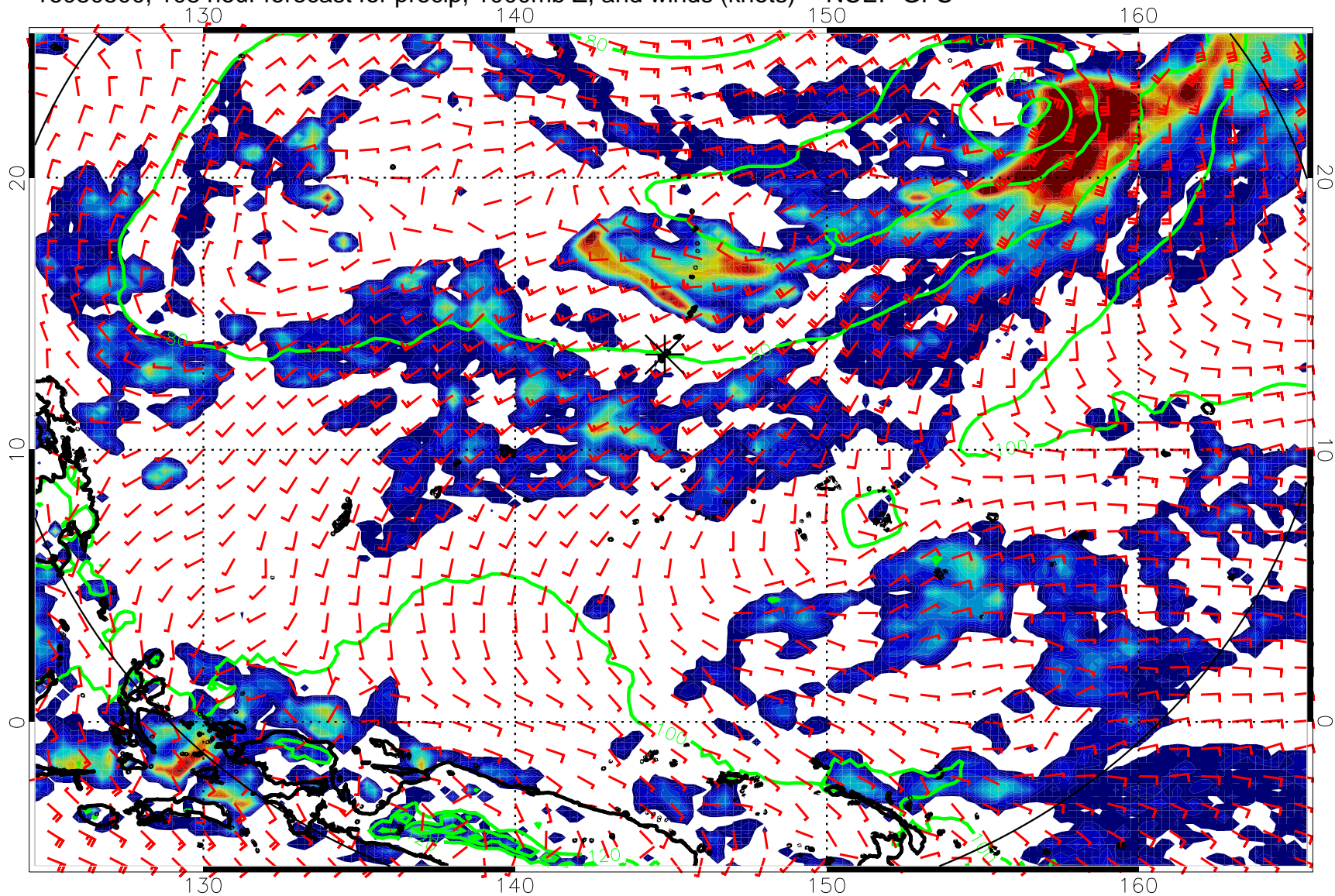
16080500, 108 hour forecast for precip, 1000mb Z, and winds (knots) -- NCEP GFS
