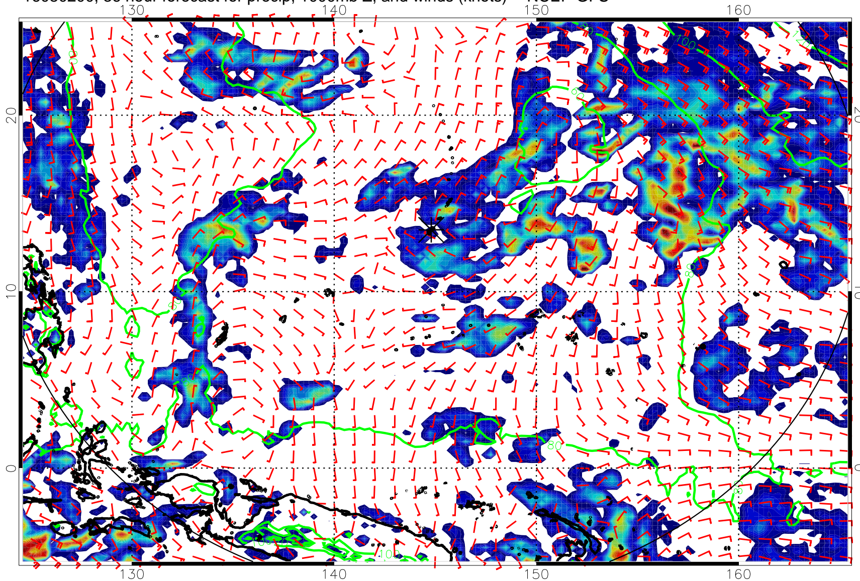
16080200, 36 hour forecast for precip, 1000mb Z, and winds (knots) -- NCEP GFS
