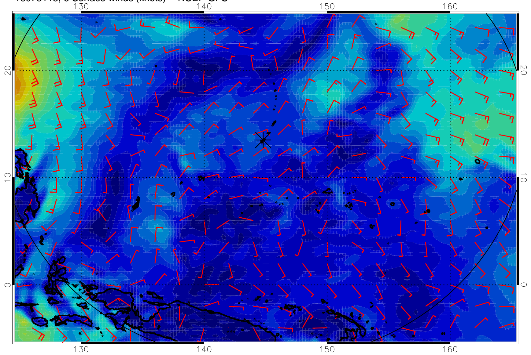
16073118, 6 Surface winds (knots) -- NCEP GFS
