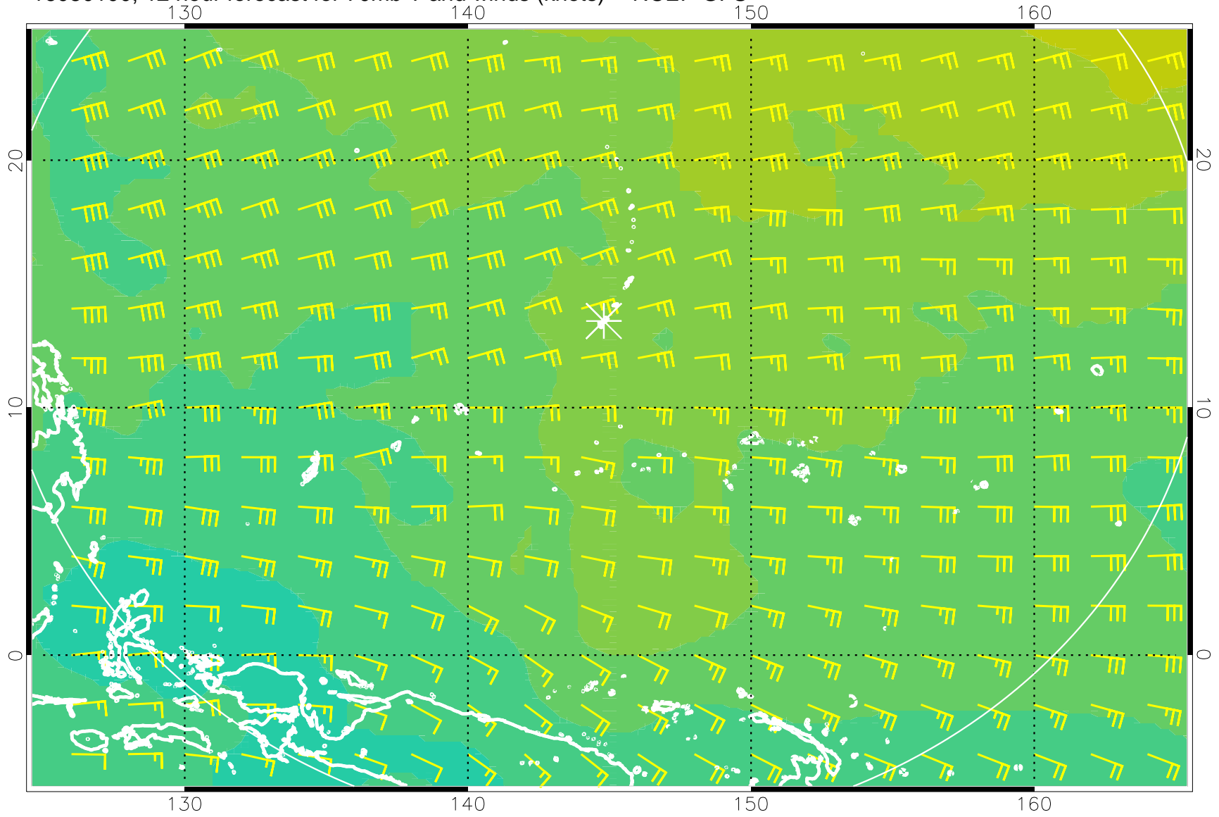
16080100, 12 hour forecast for 70mb T and winds (knots) -- NCEP GFS
