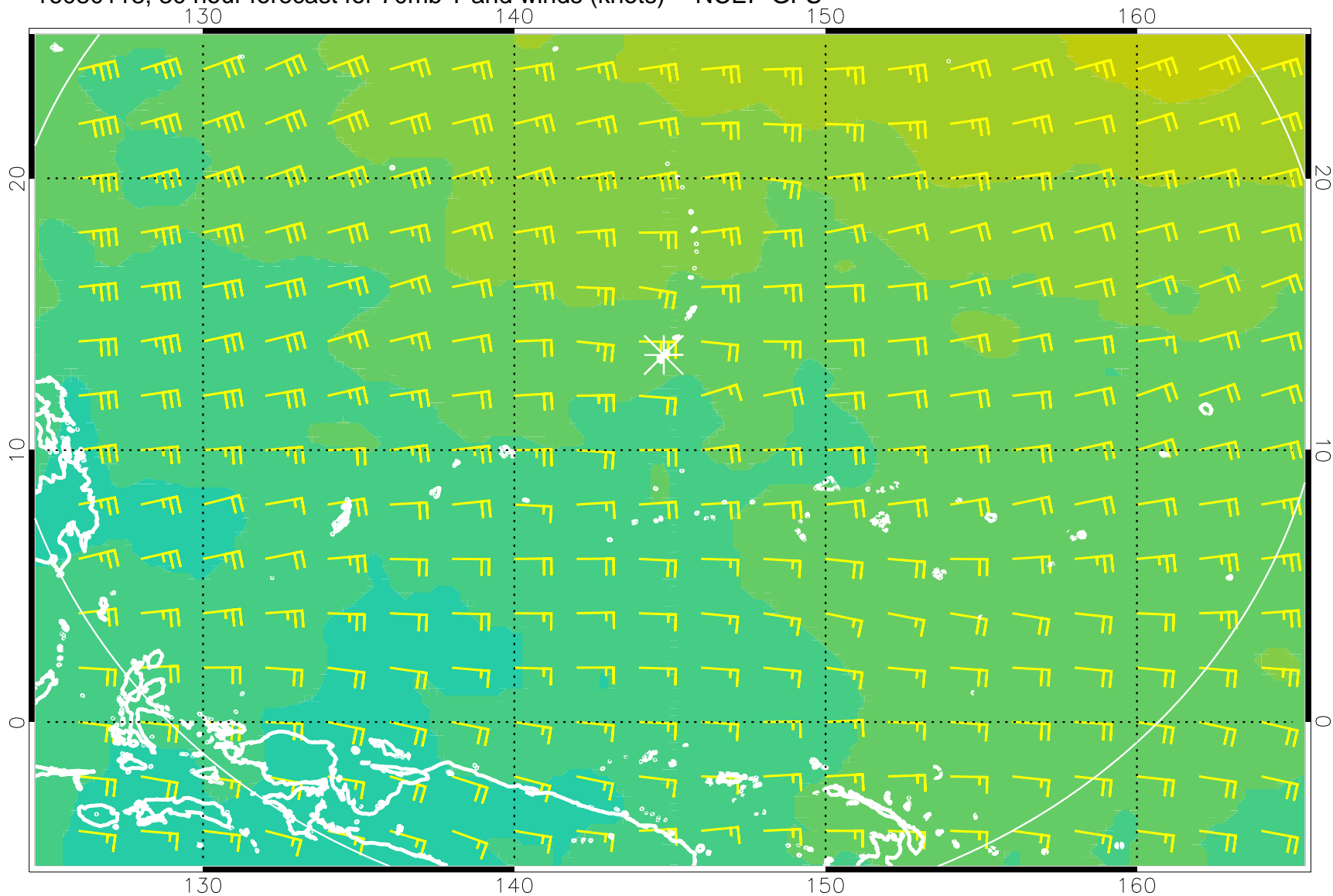
16080118, 30 hour forecast for 70mb T and winds (knots) -- NCEP GFS
