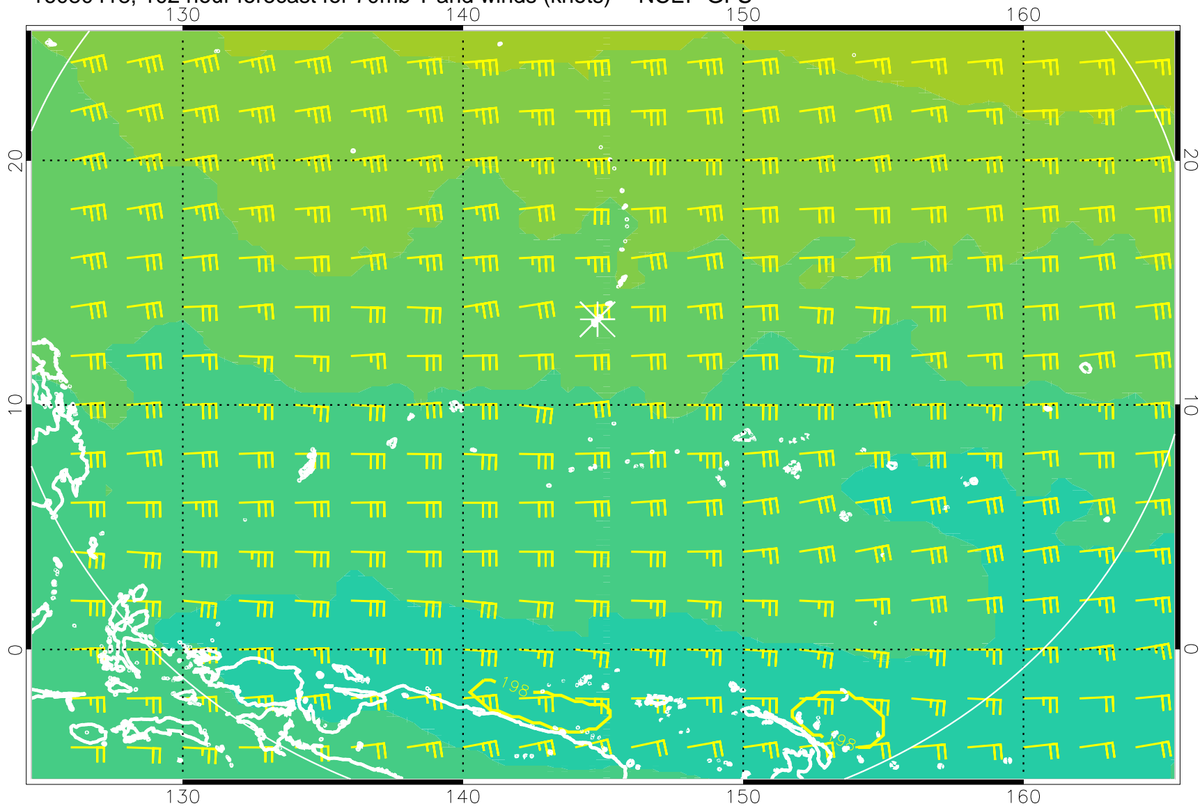
16080418, 102 hour forecast for 70mb T and winds (knots) -- NCEP GFS
