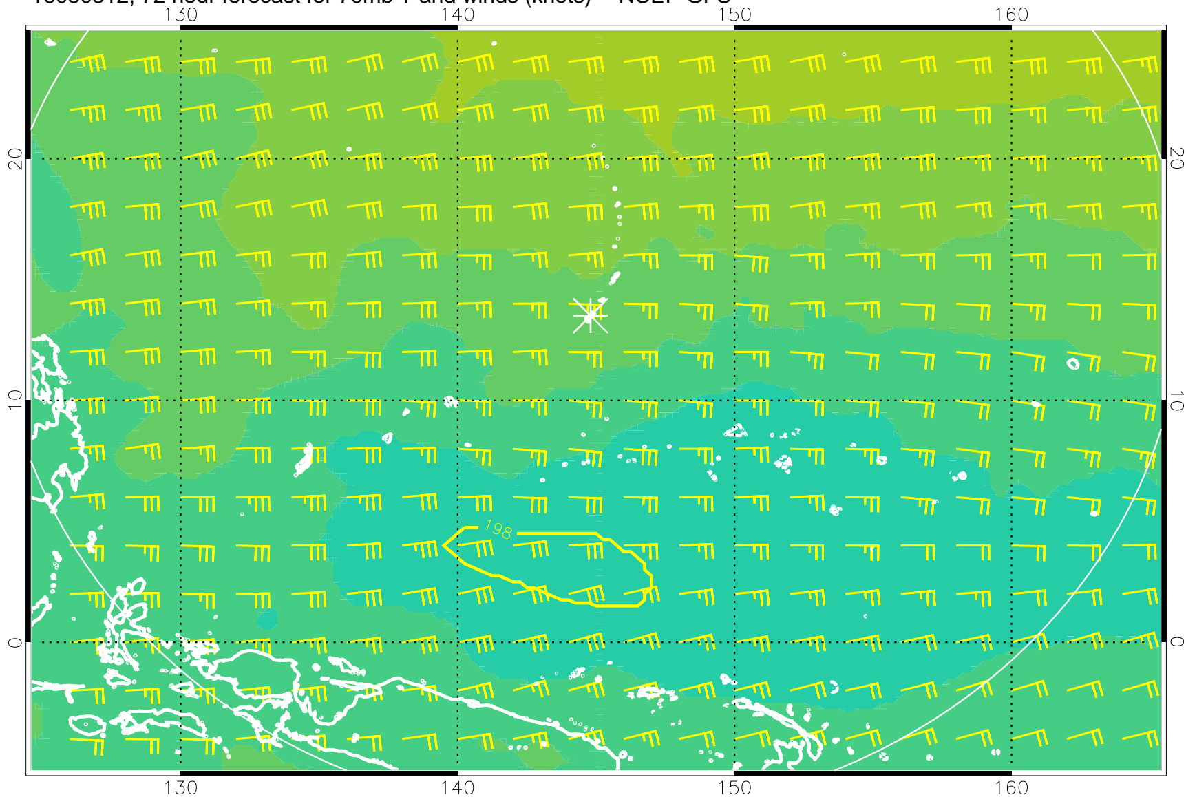
16080312, 72 hour forecast for 70mb T and winds (knots) -- NCEP GFS
