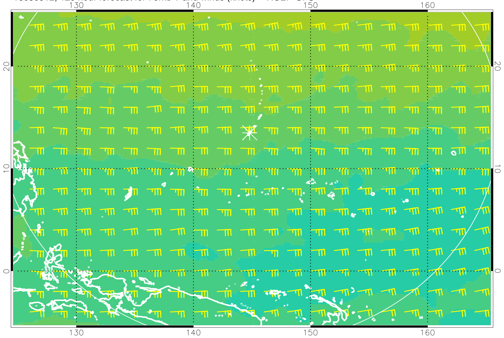
16080512, 120 hour forecast for 70mb T and winds (knots) -- NCEP GFS
