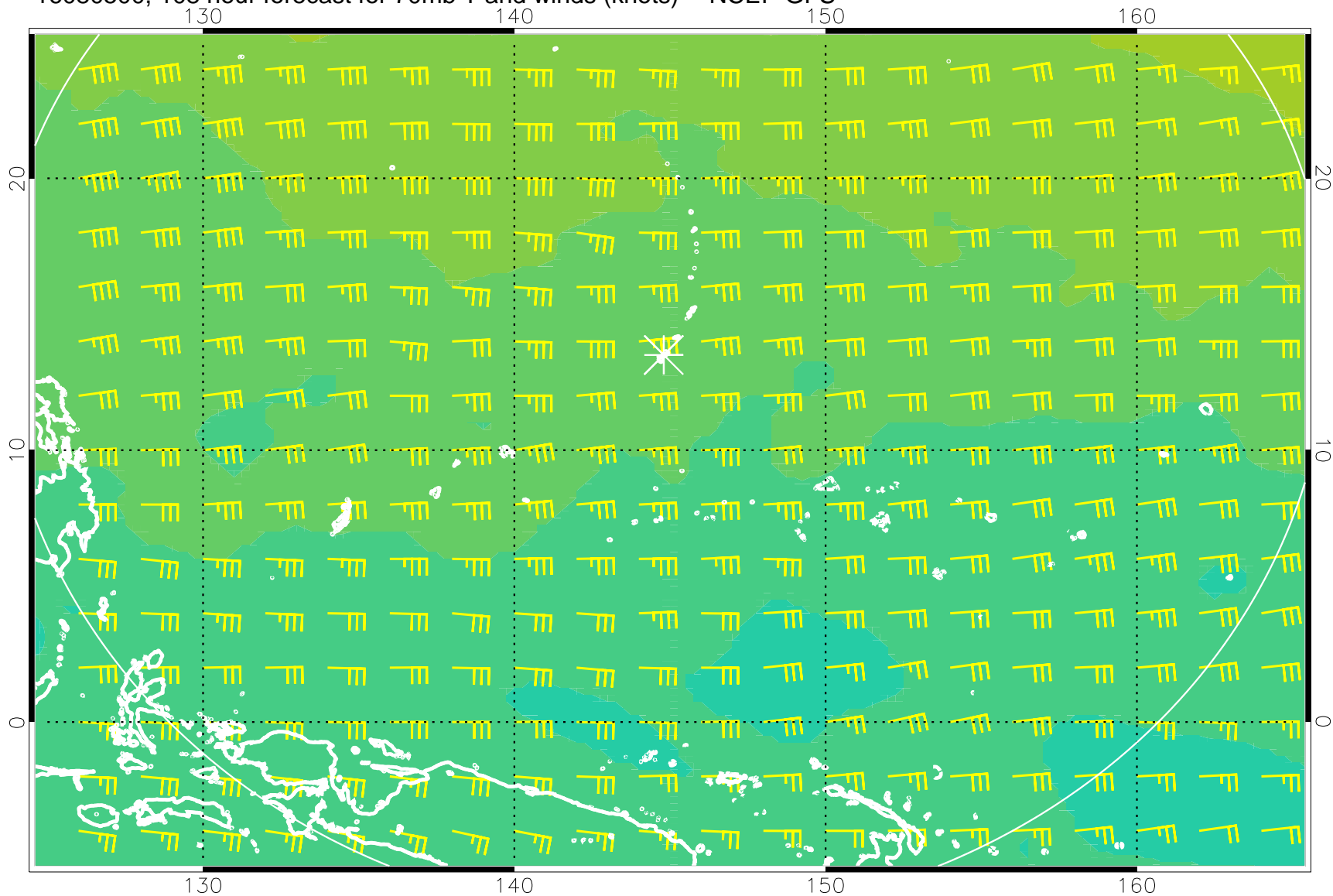
16080500, 108 hour forecast for 70mb T and winds (knots) -- NCEP GFS
