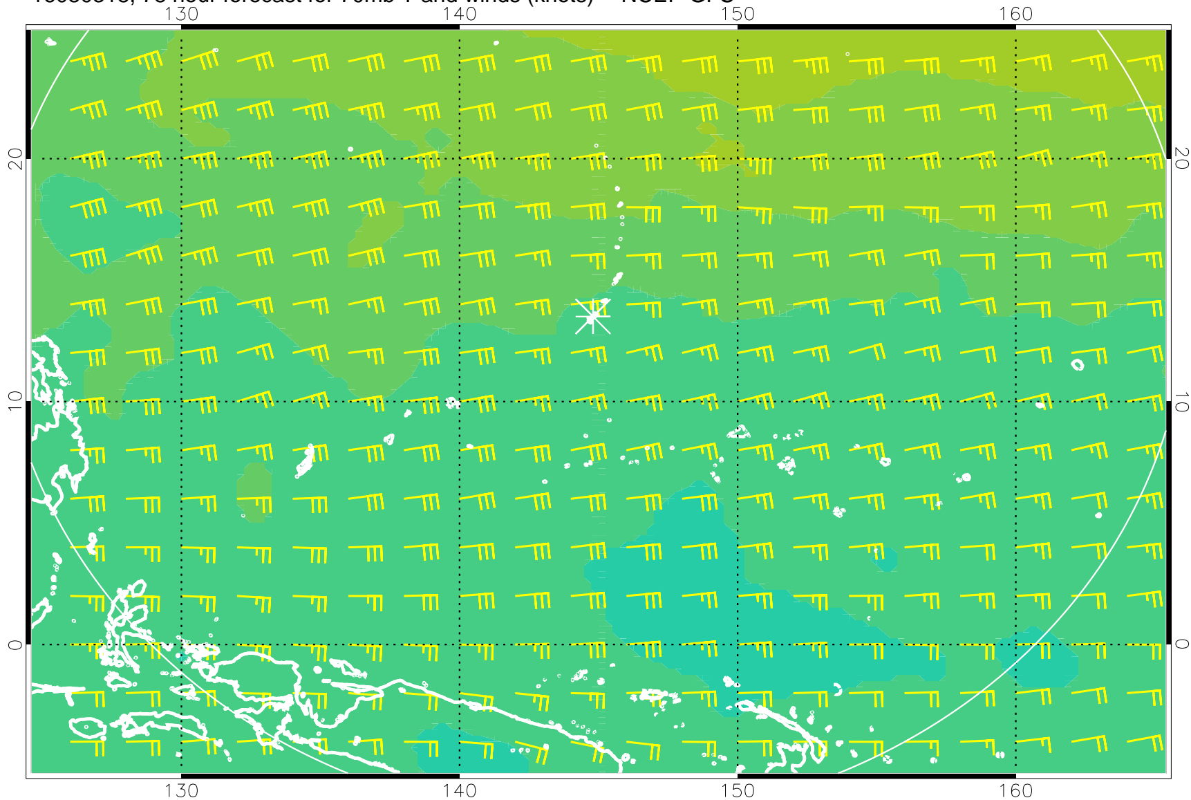
16080318, 78 hour forecast for 70mb T and winds (knots) -- NCEP GFS
