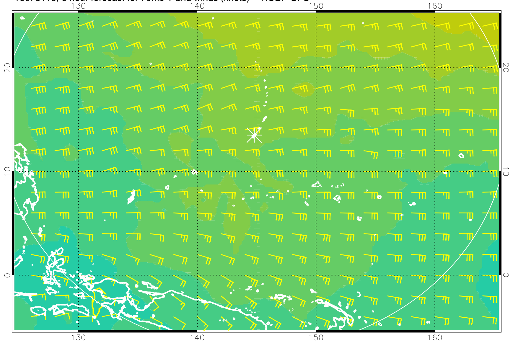
16073118, 6 hour forecast for 70mb T and winds (knots) -- NCEP GFS
