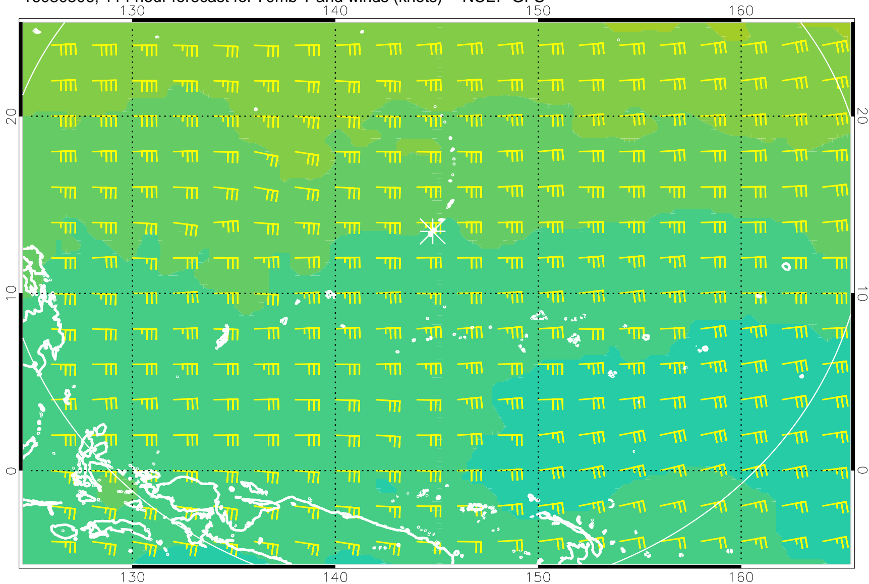
16080506, 114 hour forecast for 70mb T and winds (knots) -- NCEP GFS
