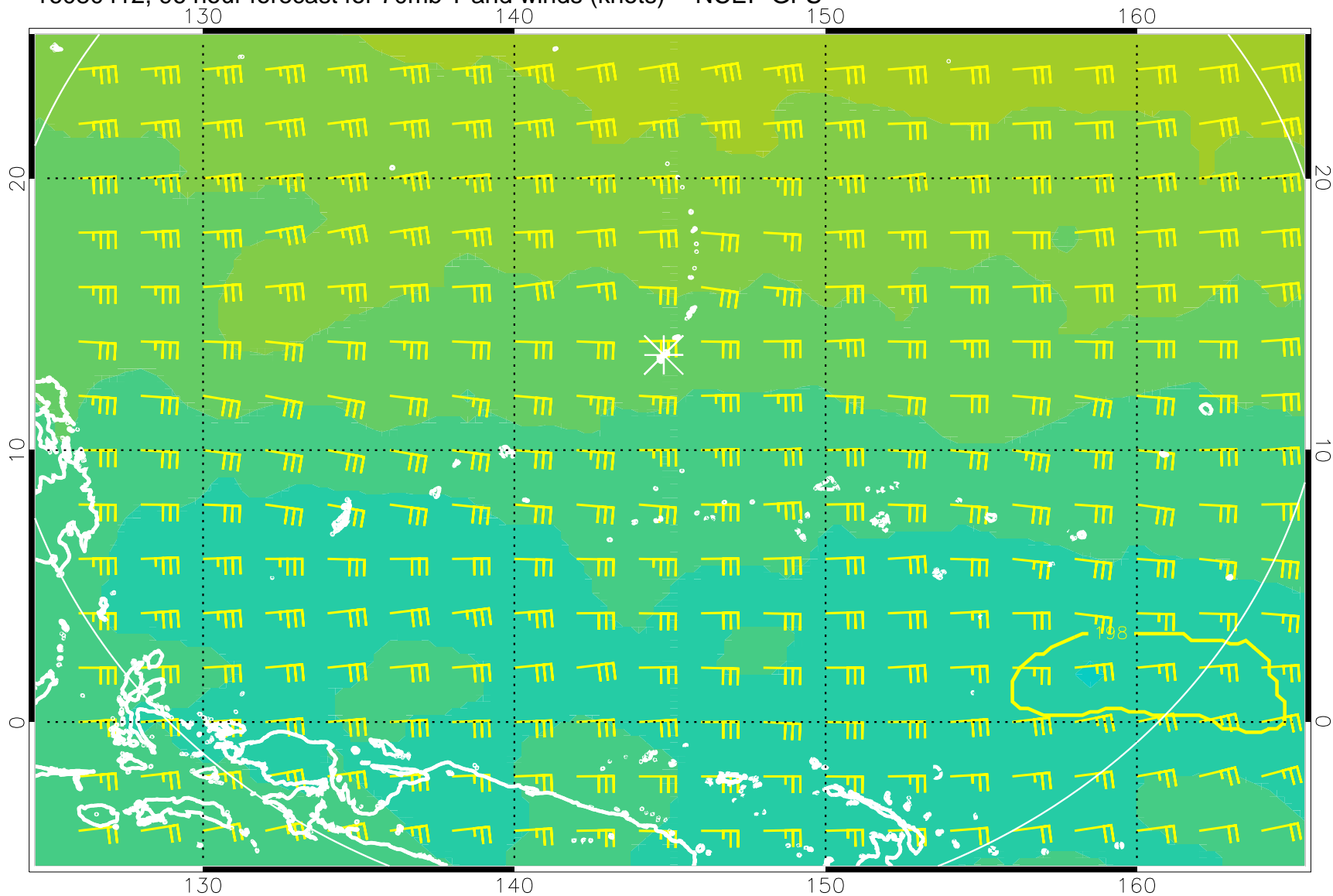
16080412, 96 hour forecast for 70mb T and winds (knots) -- NCEP GFS
