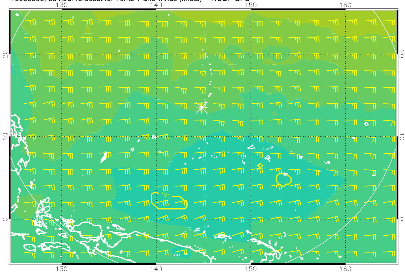
16080306, 66 hour forecast for 70mb T and winds (knots) -- NCEP GFS
