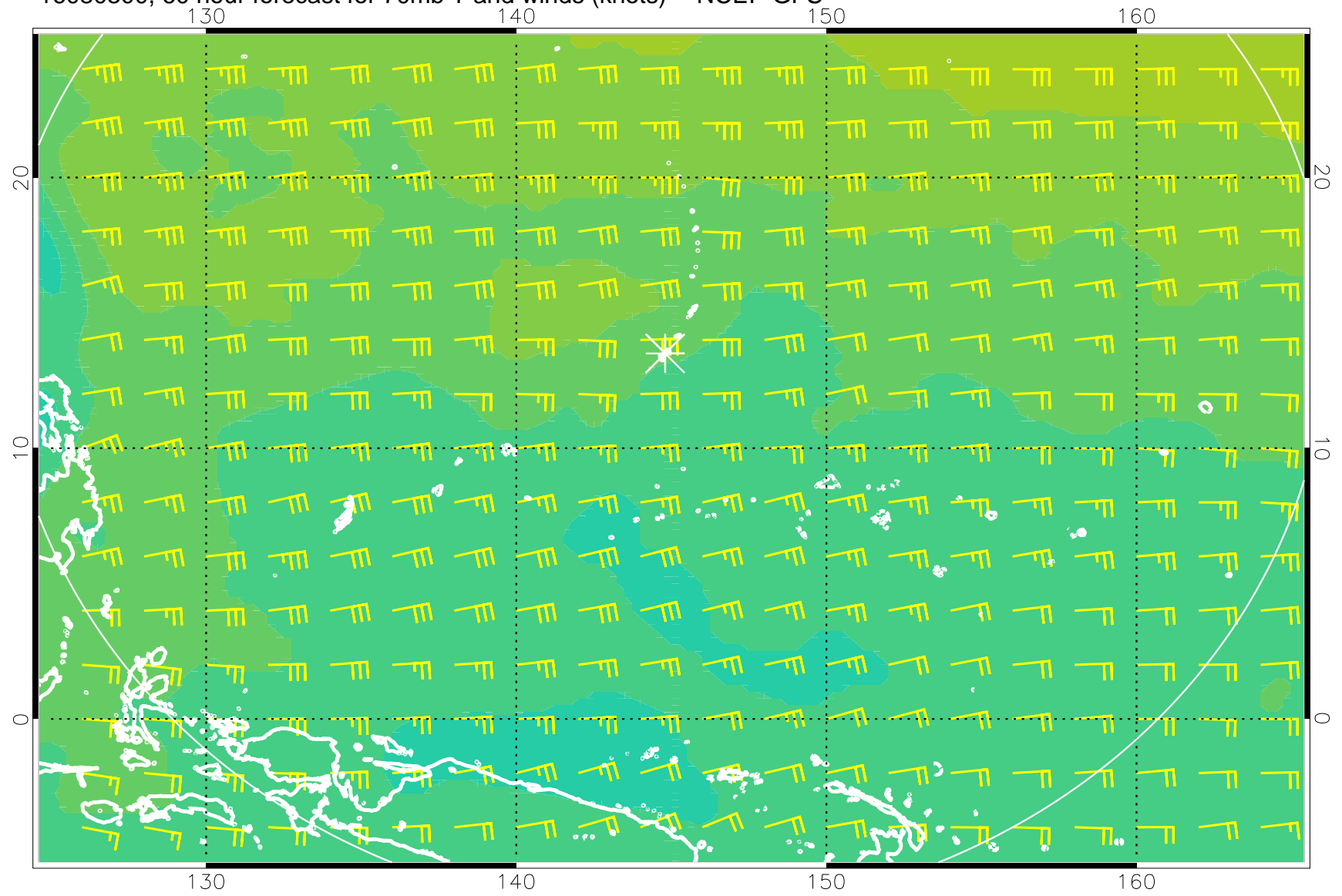
16080300, 60 hour forecast for 70mb T and winds (knots) -- NCEP GFS
