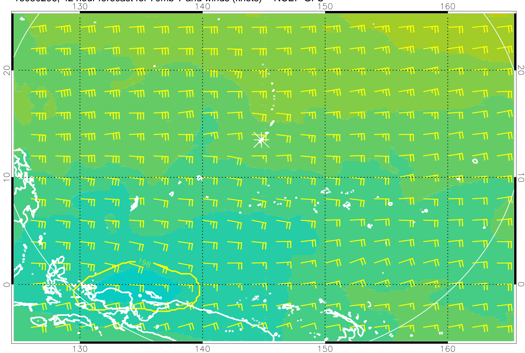
16080206, 42 hour forecast for 70mb T and winds (knots) -- NCEP GFS
