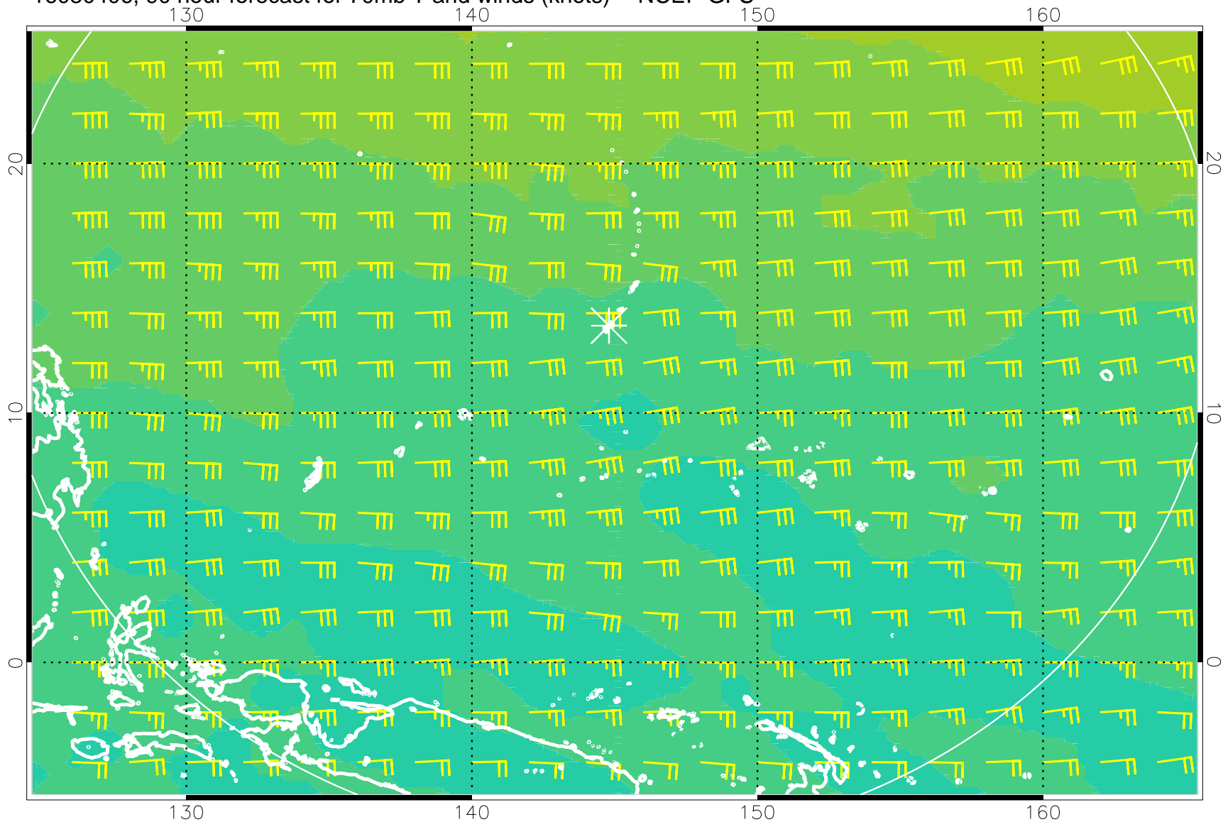
16080406, 90 hour forecast for 70mb T and winds (knots) -- NCEP GFS
