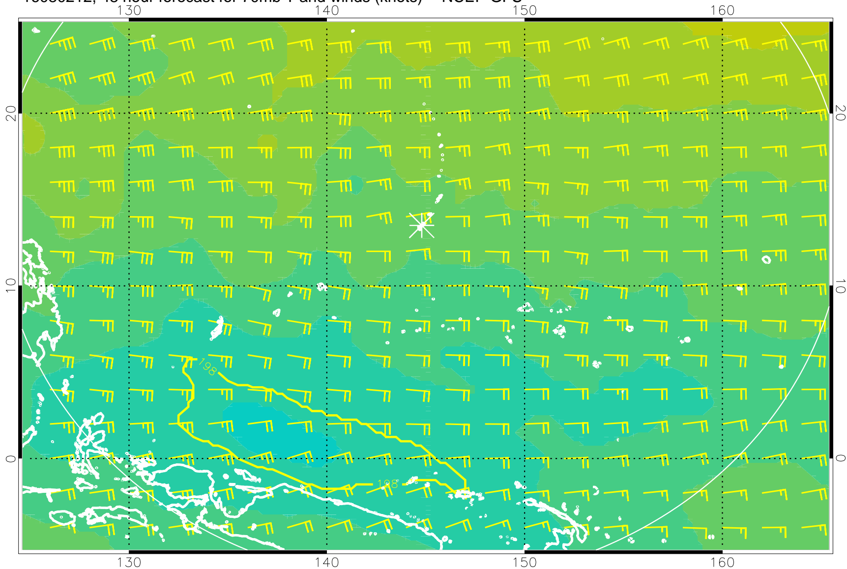
16080212, 48 hour forecast for 70mb T and winds (knots) -- NCEP GFS
