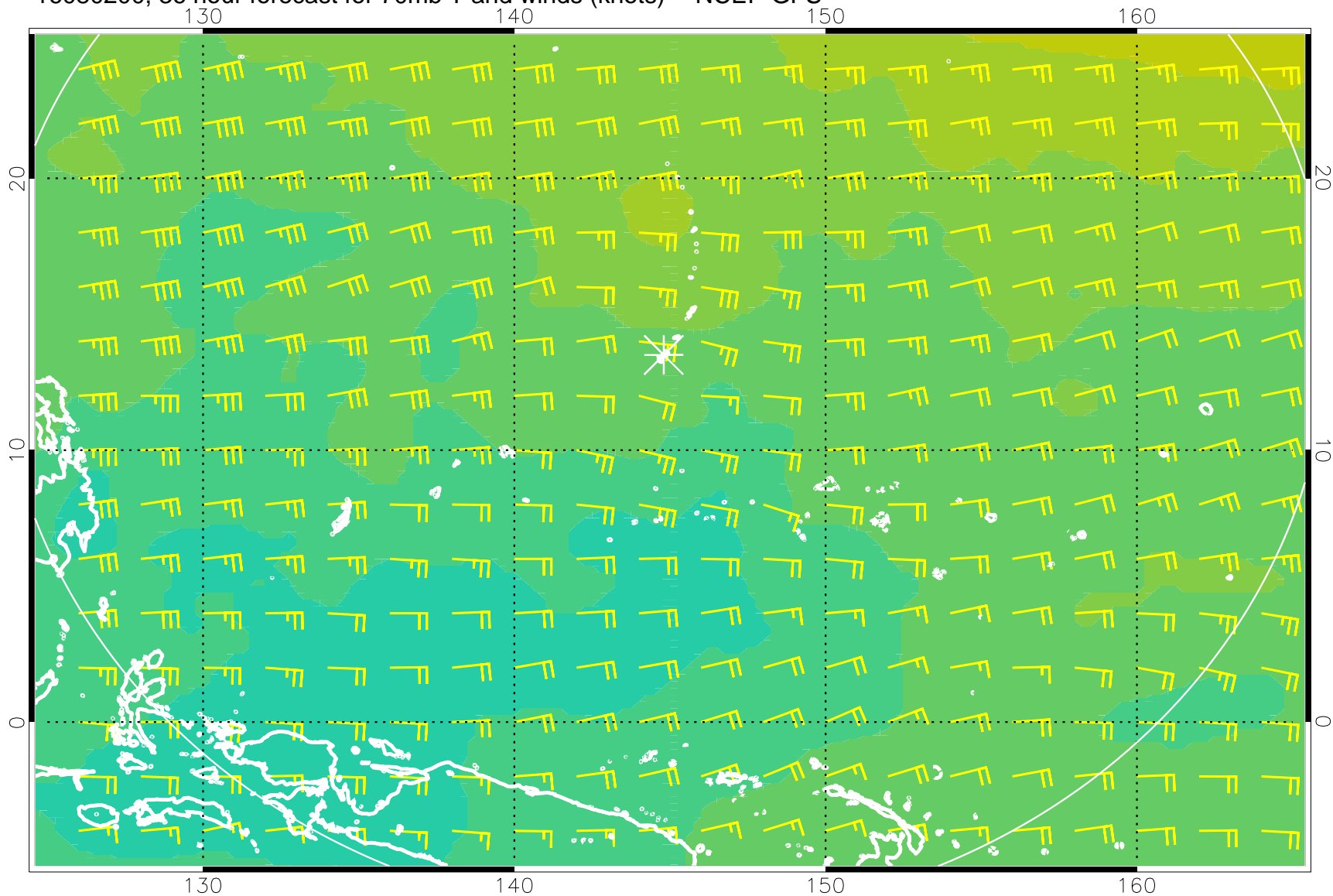
16080200, 36 hour forecast for 70mb T and winds (knots) -- NCEP GFS
