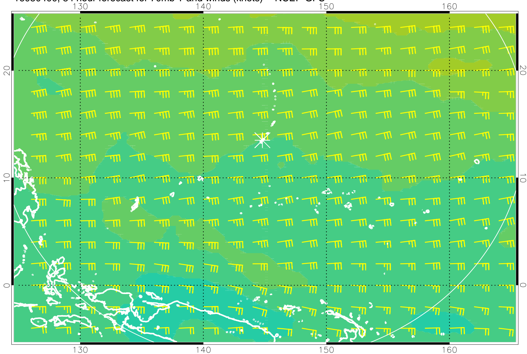
16080400, 84 hour forecast for 70mb T and winds (knots) -- NCEP GFS
