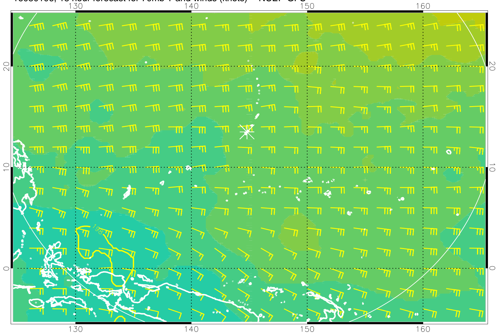
16080106, 18 hour forecast for 70mb T and winds (knots) -- NCEP GFS
