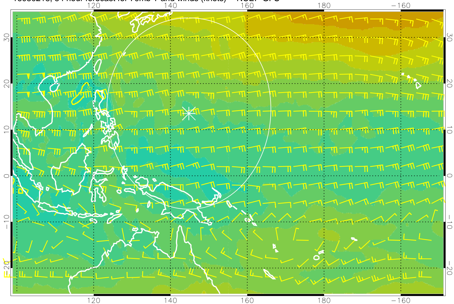
16080218, 54 hour forecast for 70mb T and winds (knots) -- NCEP GFS
