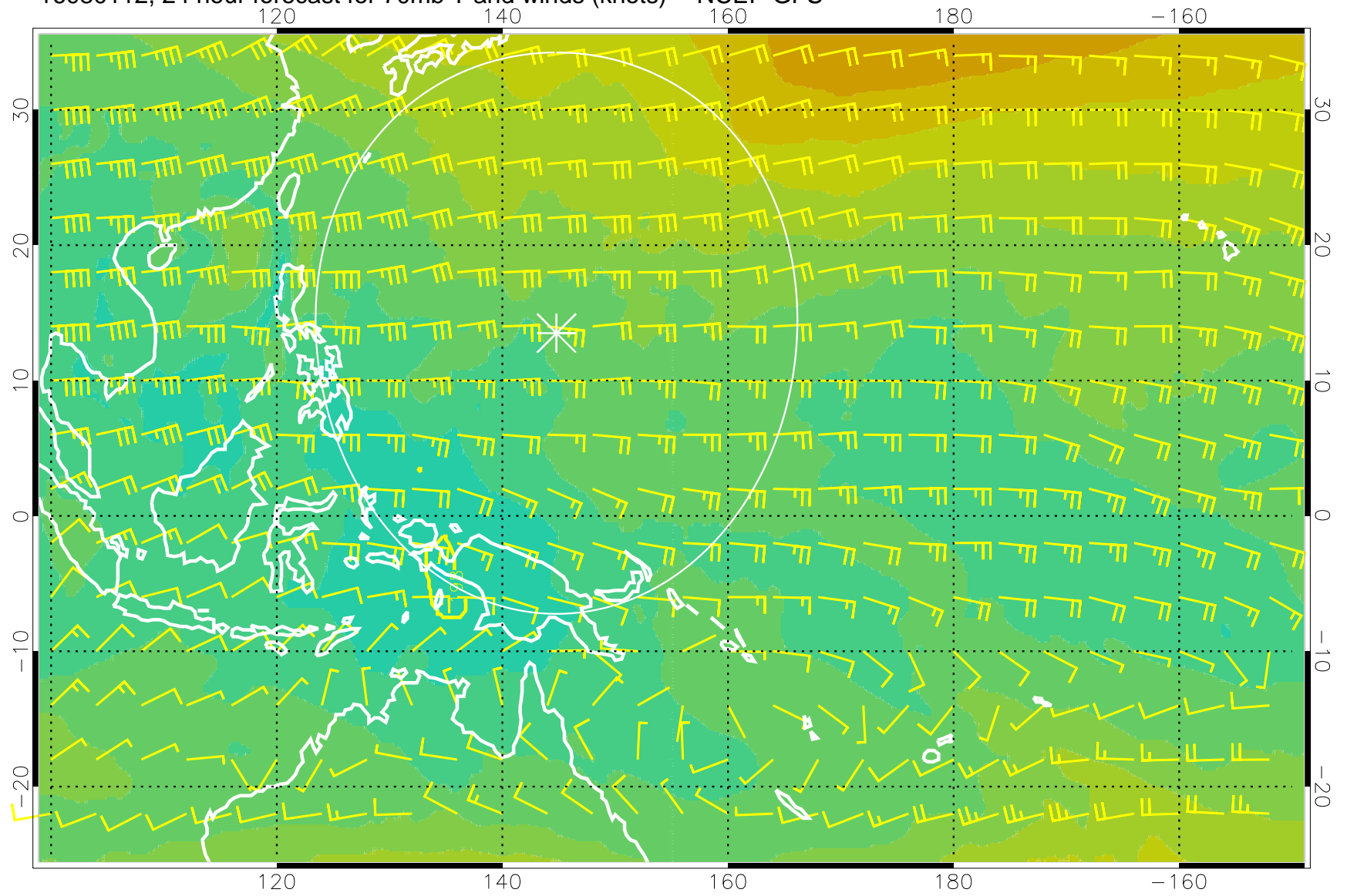
16080112, 24 hour forecast for 70mb T and winds (knots) -- NCEP GFS
