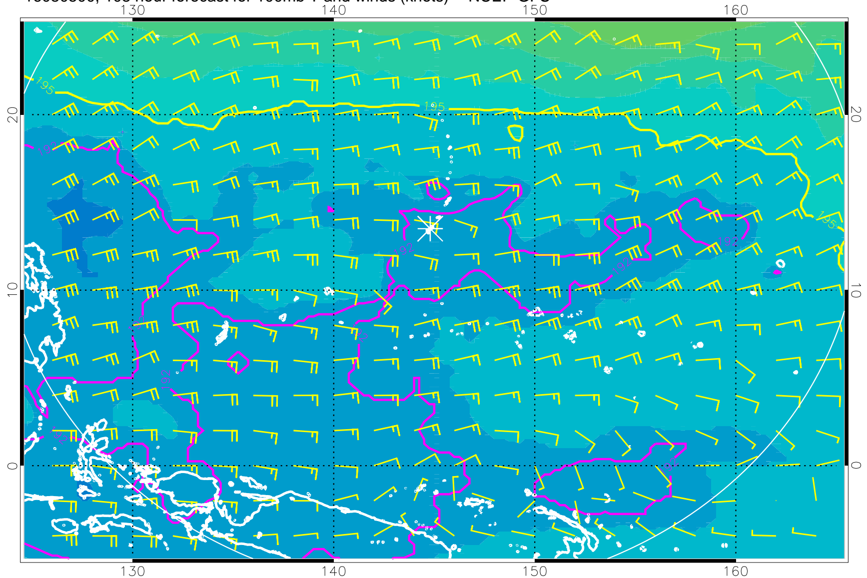
16080500, 108 hour forecast for 100mb T and winds (knots) -- NCEP GFS
