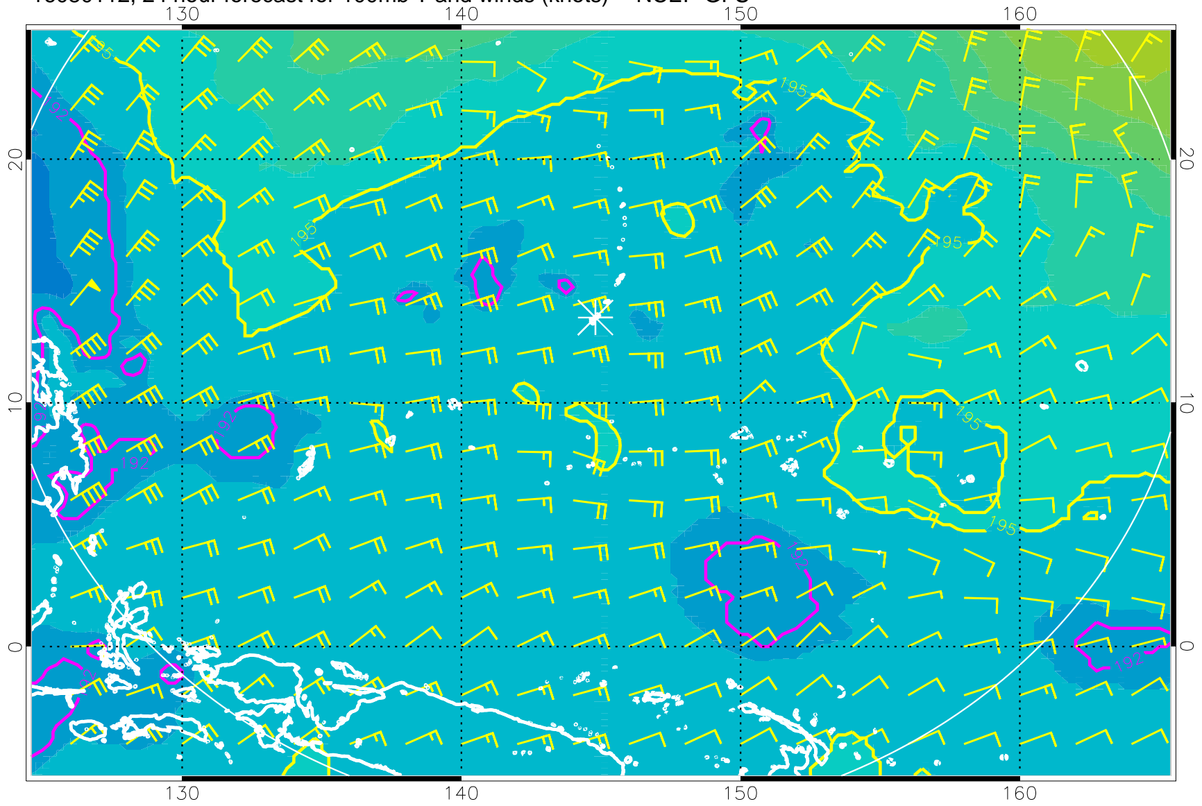
16080112, 24 hour forecast for 100mb T and winds (knots) -- NCEP GFS
