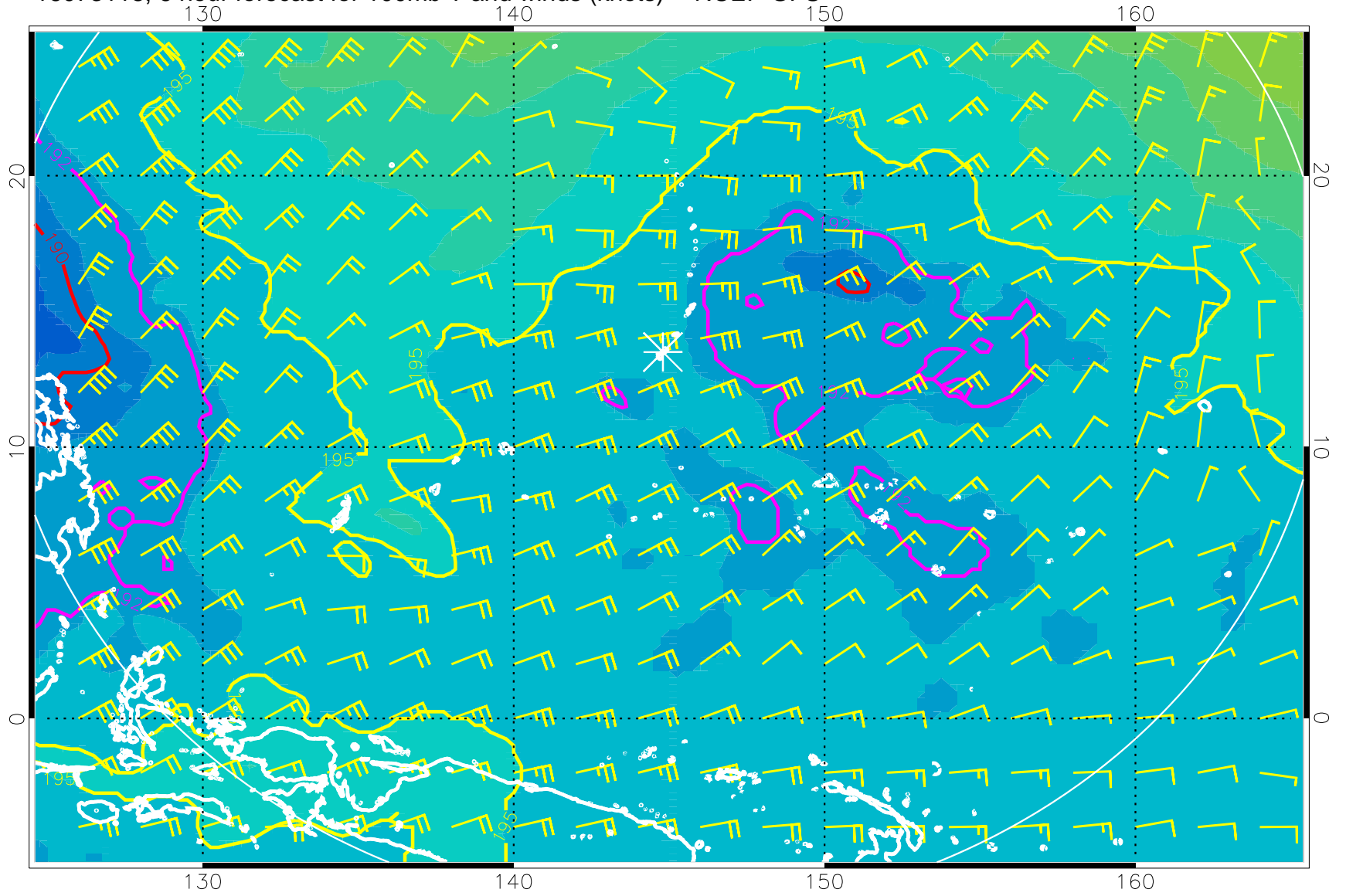
16073118, 6 hour forecast for 100mb T and winds (knots) -- NCEP GFS
