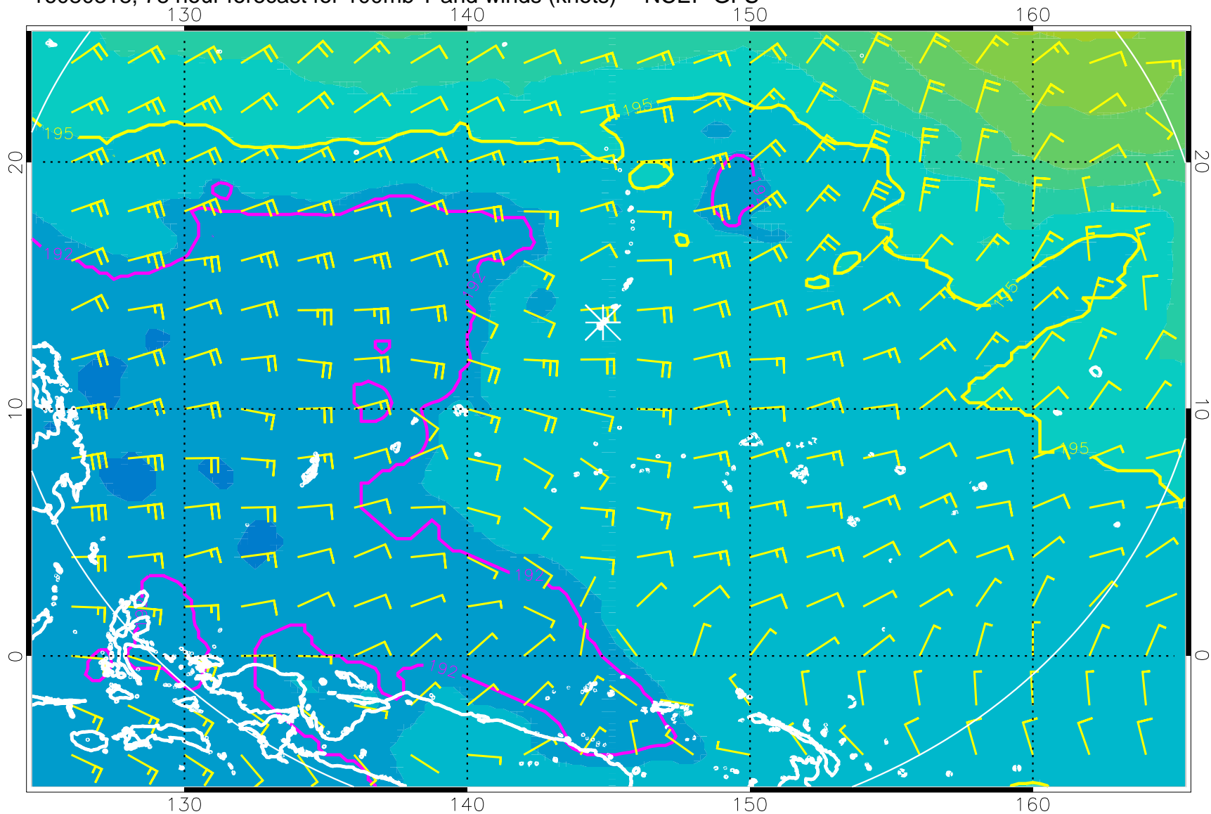
16080318, 78 hour forecast for 100mb T and winds (knots) -- NCEP GFS
