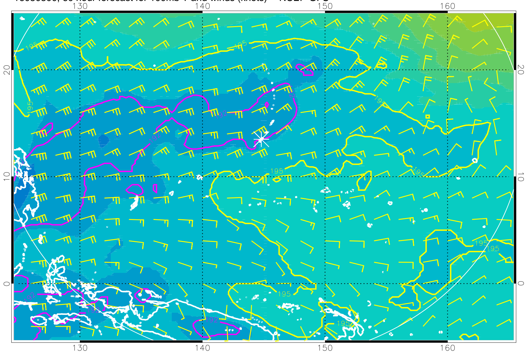
16080300, 60 hour forecast for 100mb T and winds (knots) -- NCEP GFS
