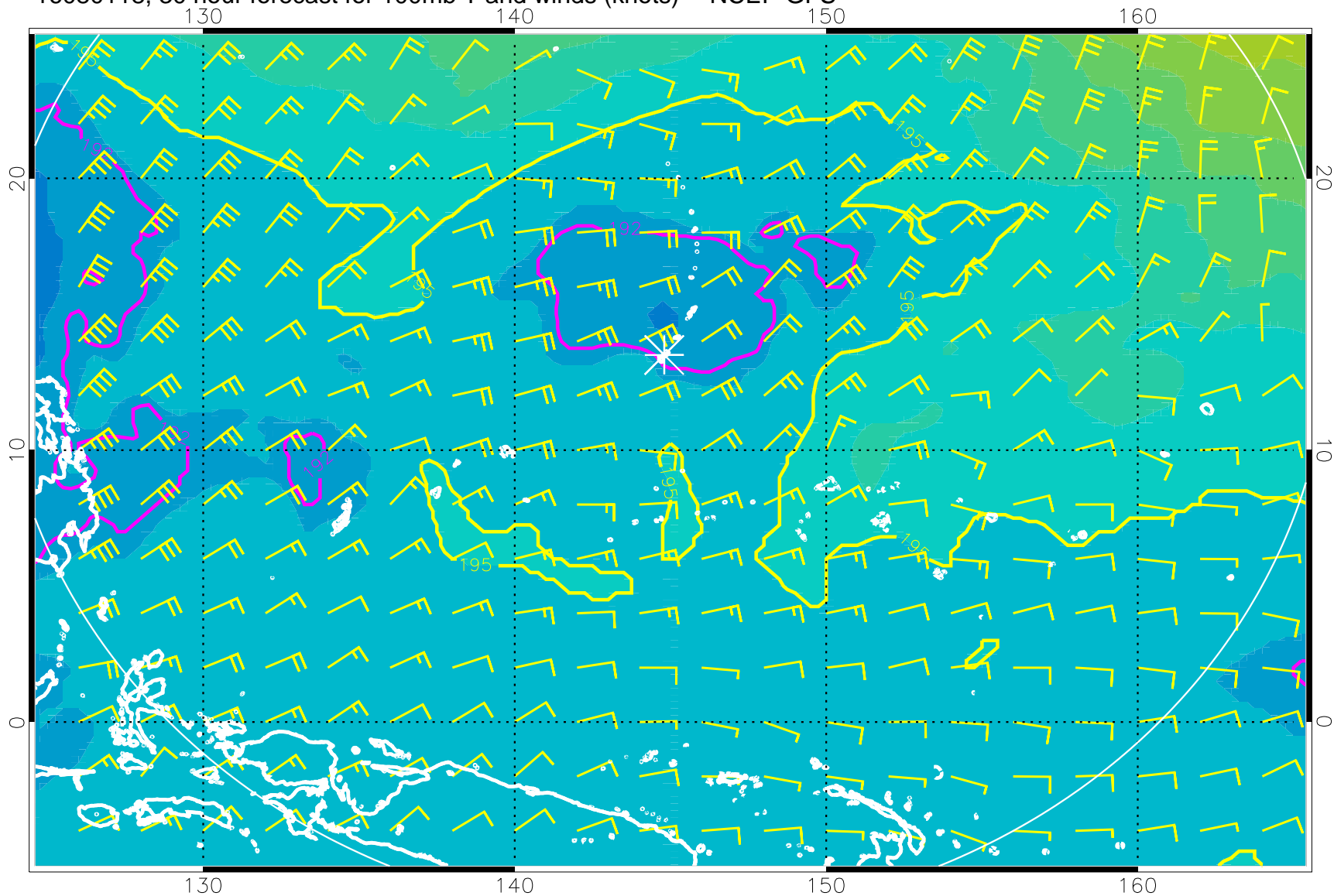
16080118, 30 hour forecast for 100mb T and winds (knots) -- NCEP GFS
