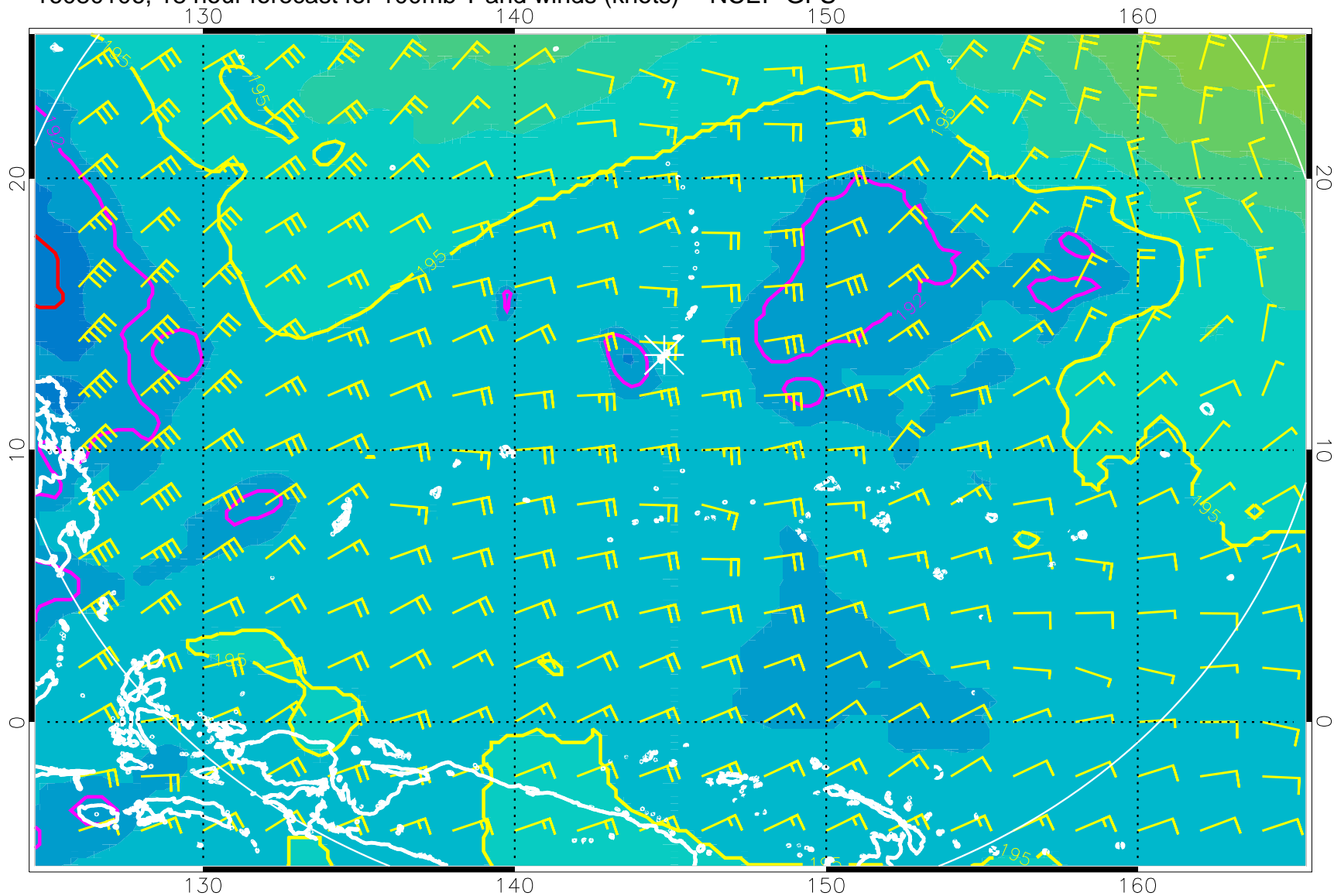
16080106, 18 hour forecast for 100mb T and winds (knots) -- NCEP GFS
