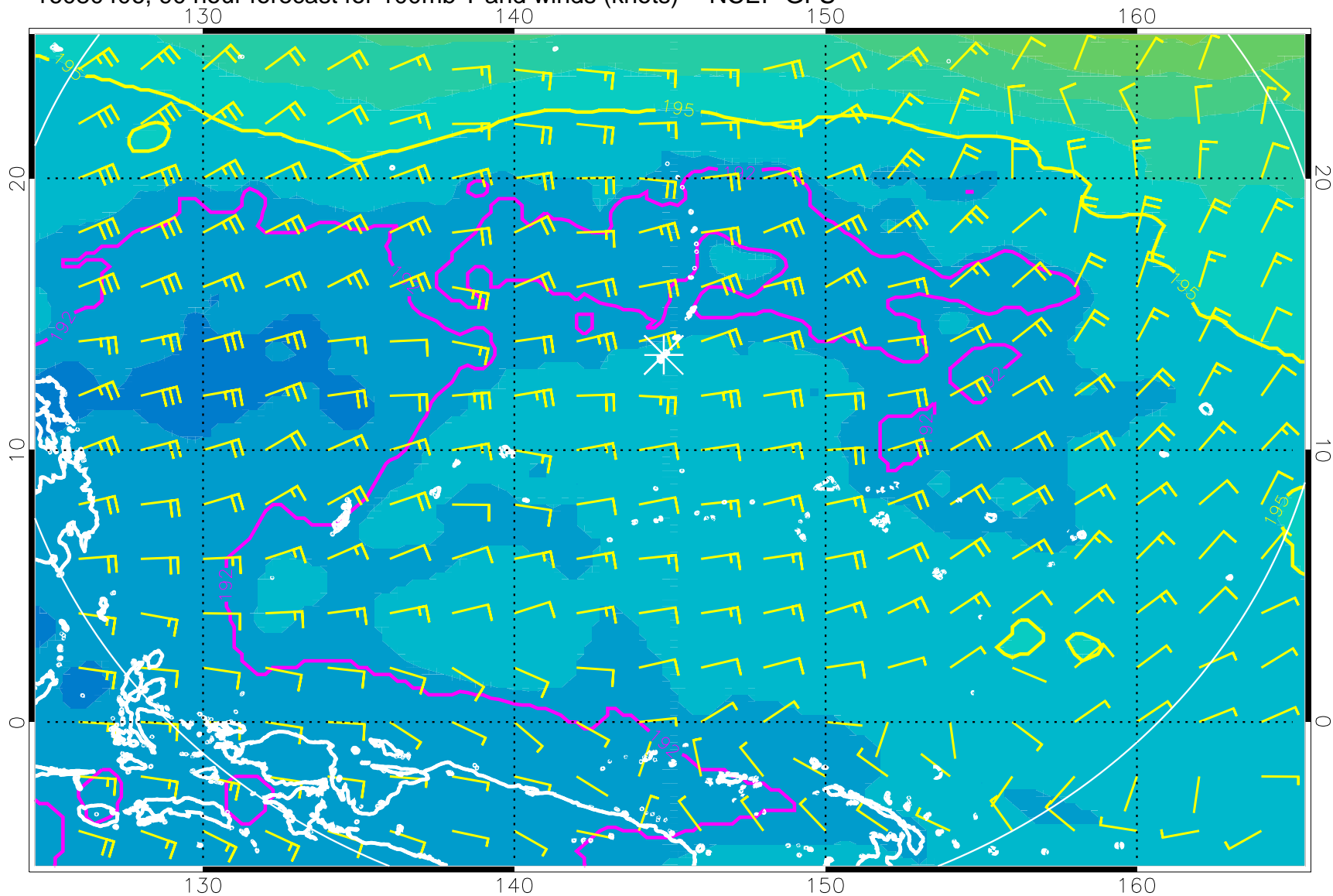
16080406, 90 hour forecast for 100mb T and winds (knots) -- NCEP GFS
