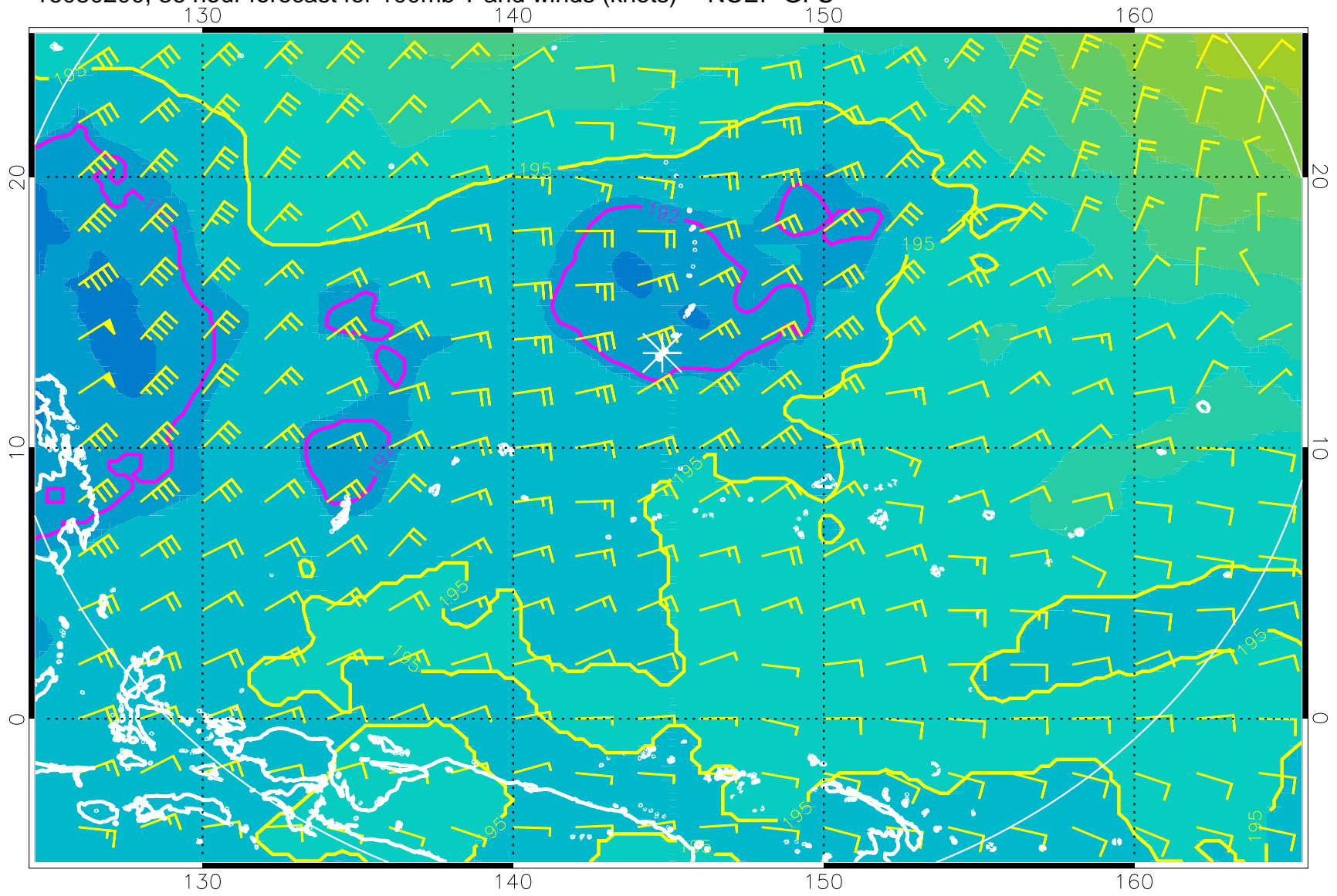
16080200, 36 hour forecast for 100mb T and winds (knots) -- NCEP GFS
