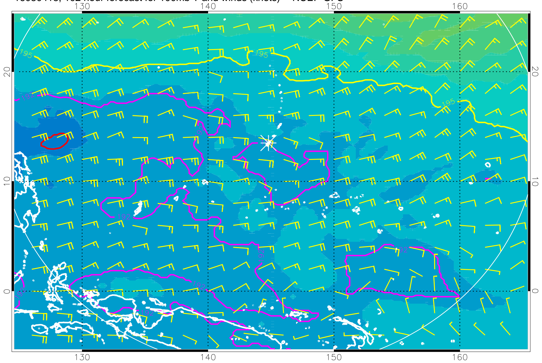
16080418, 102 hour forecast for 100mb T and winds (knots) -- NCEP GFS
