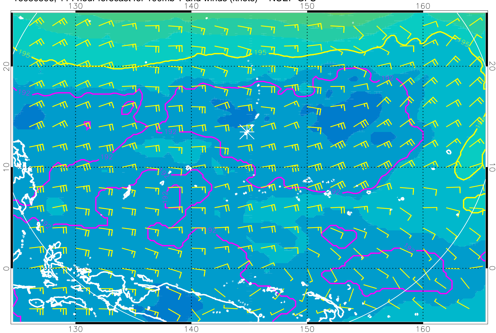
16080506, 114 hour forecast for 100mb T and winds (knots) -- NCEP GFS
