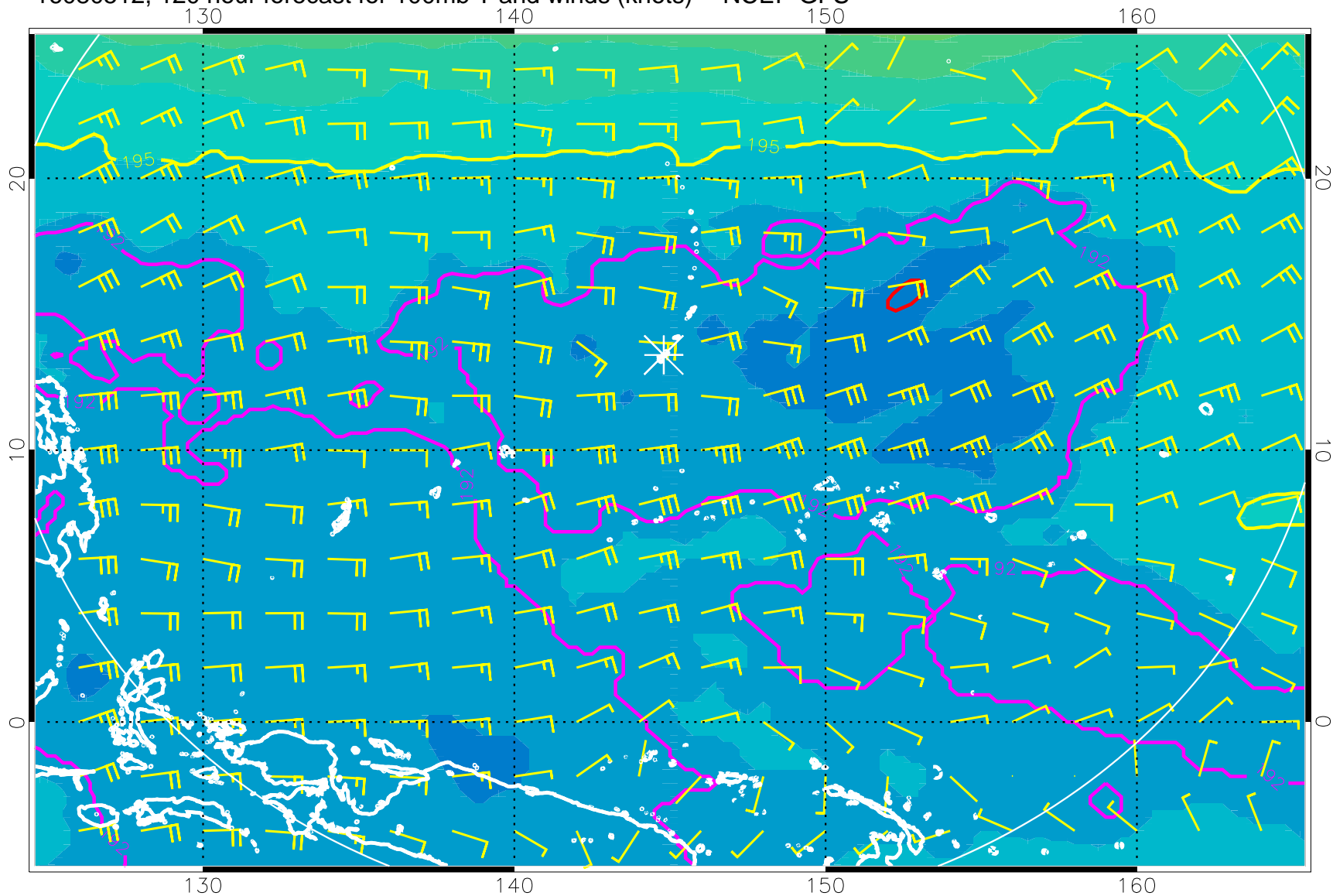
16080512, 120 hour forecast for 100mb T and winds (knots) -- NCEP GFS
