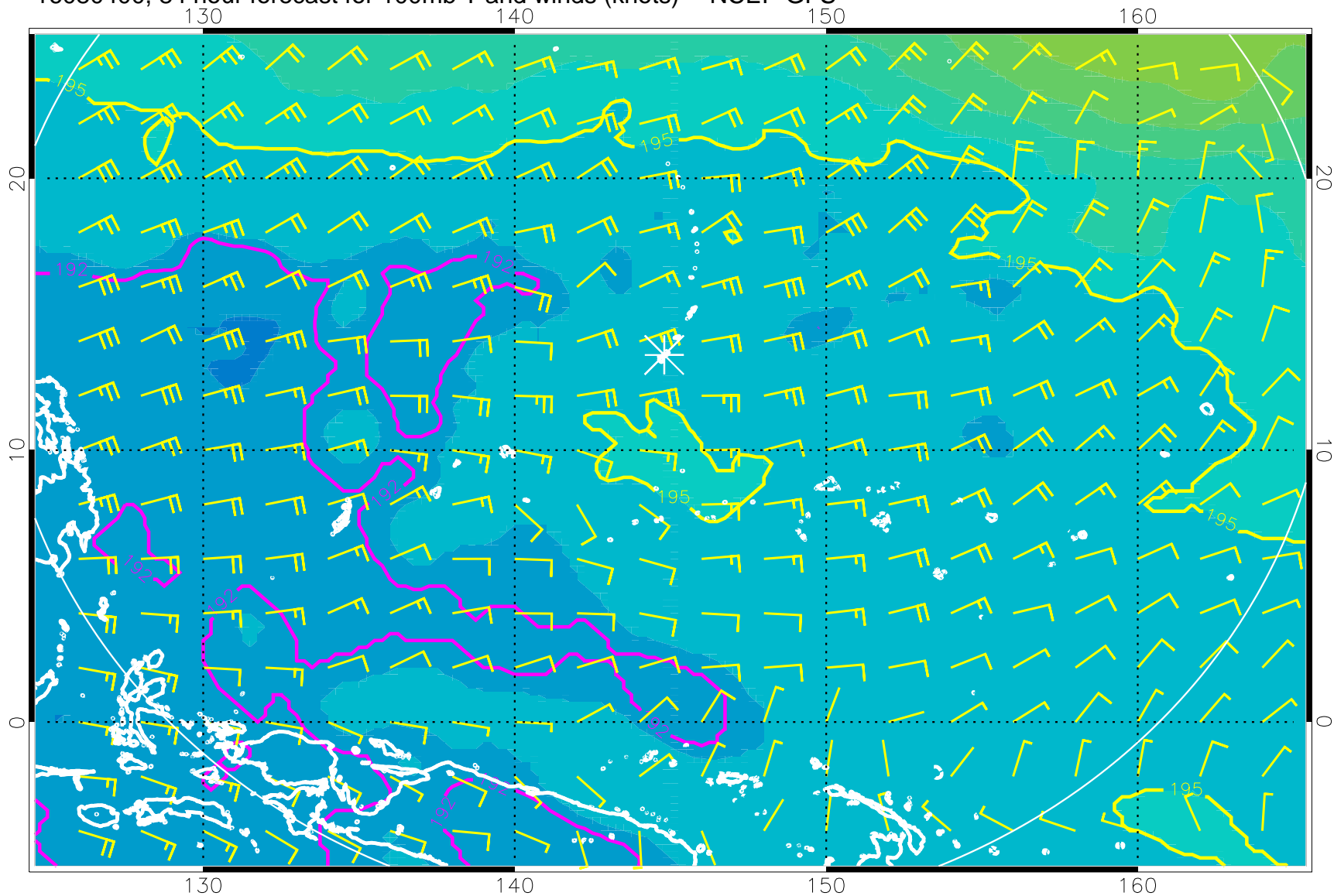
16080400, 84 hour forecast for 100mb T and winds (knots) -- NCEP GFS
