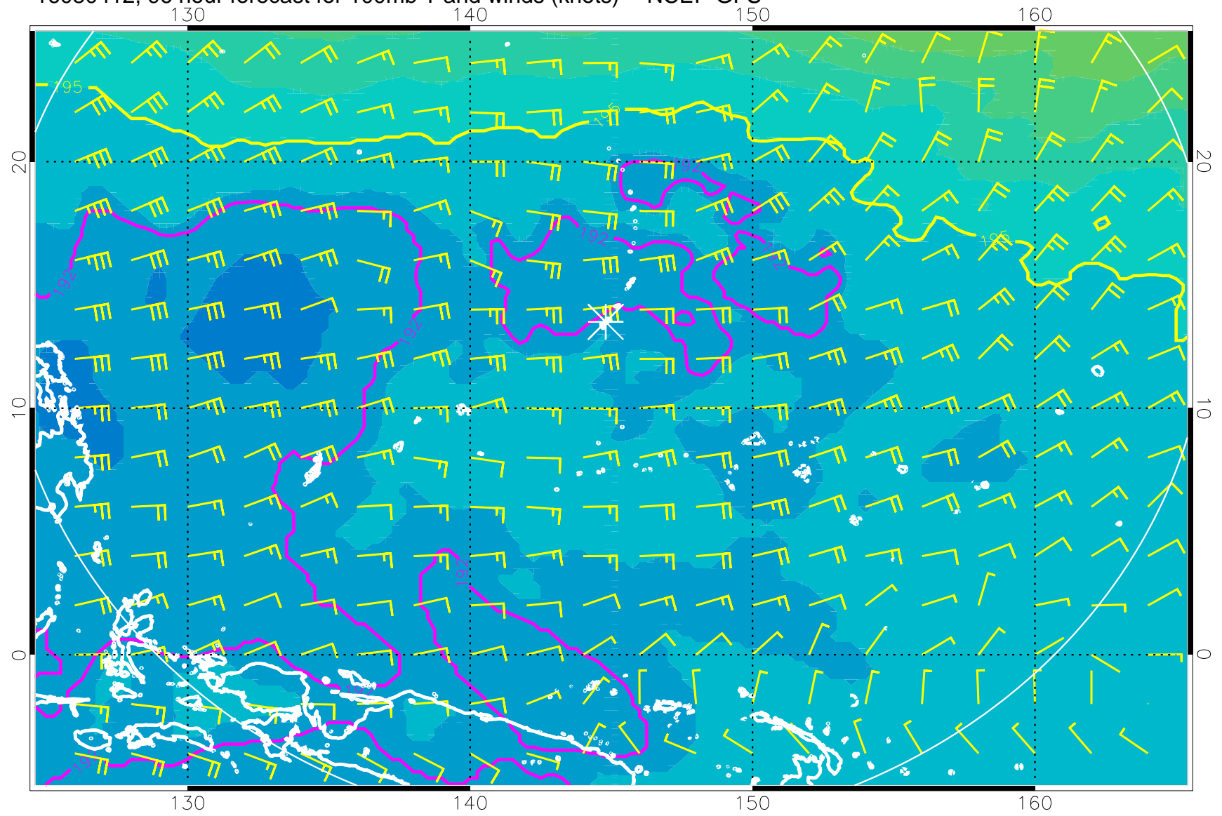
16080412, 96 hour forecast for 100mb T and winds (knots) -- NCEP GFS
