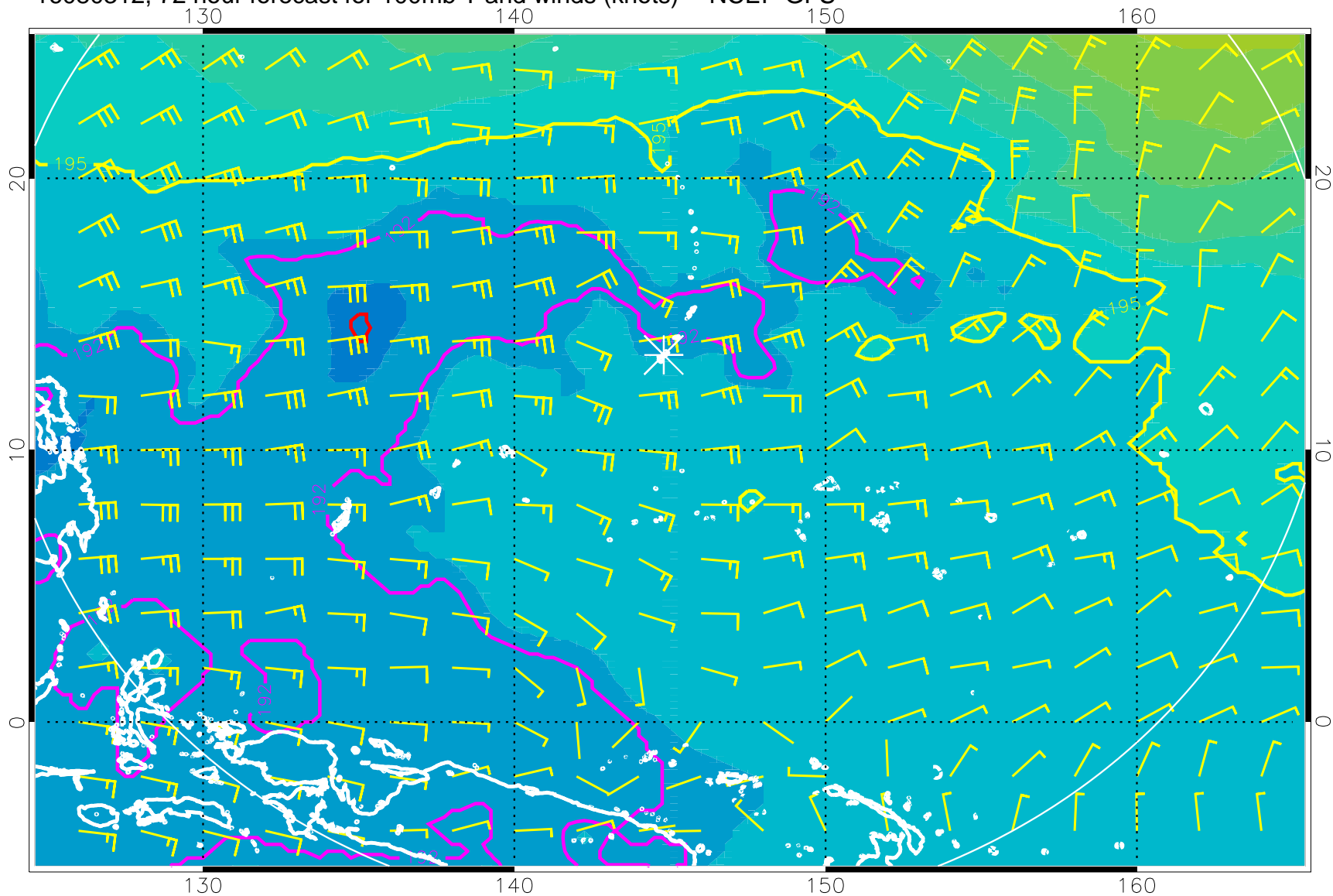
16080312, 72 hour forecast for 100mb T and winds (knots) -- NCEP GFS
