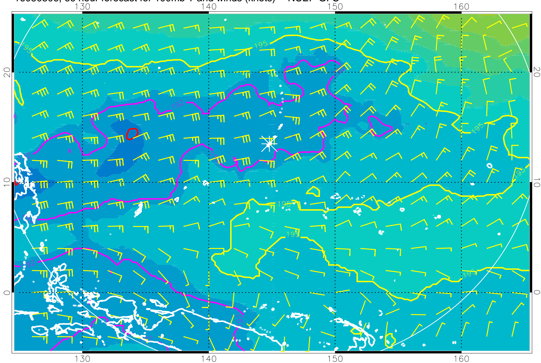
16080306, 66 hour forecast for 100mb T and winds (knots) -- NCEP GFS
