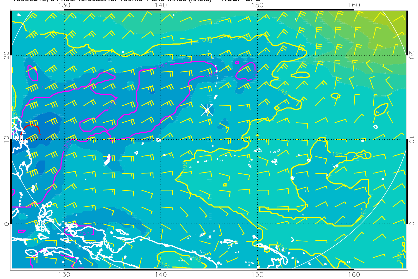
16080218, 54 hour forecast for 100mb T and winds (knots) -- NCEP GFS
