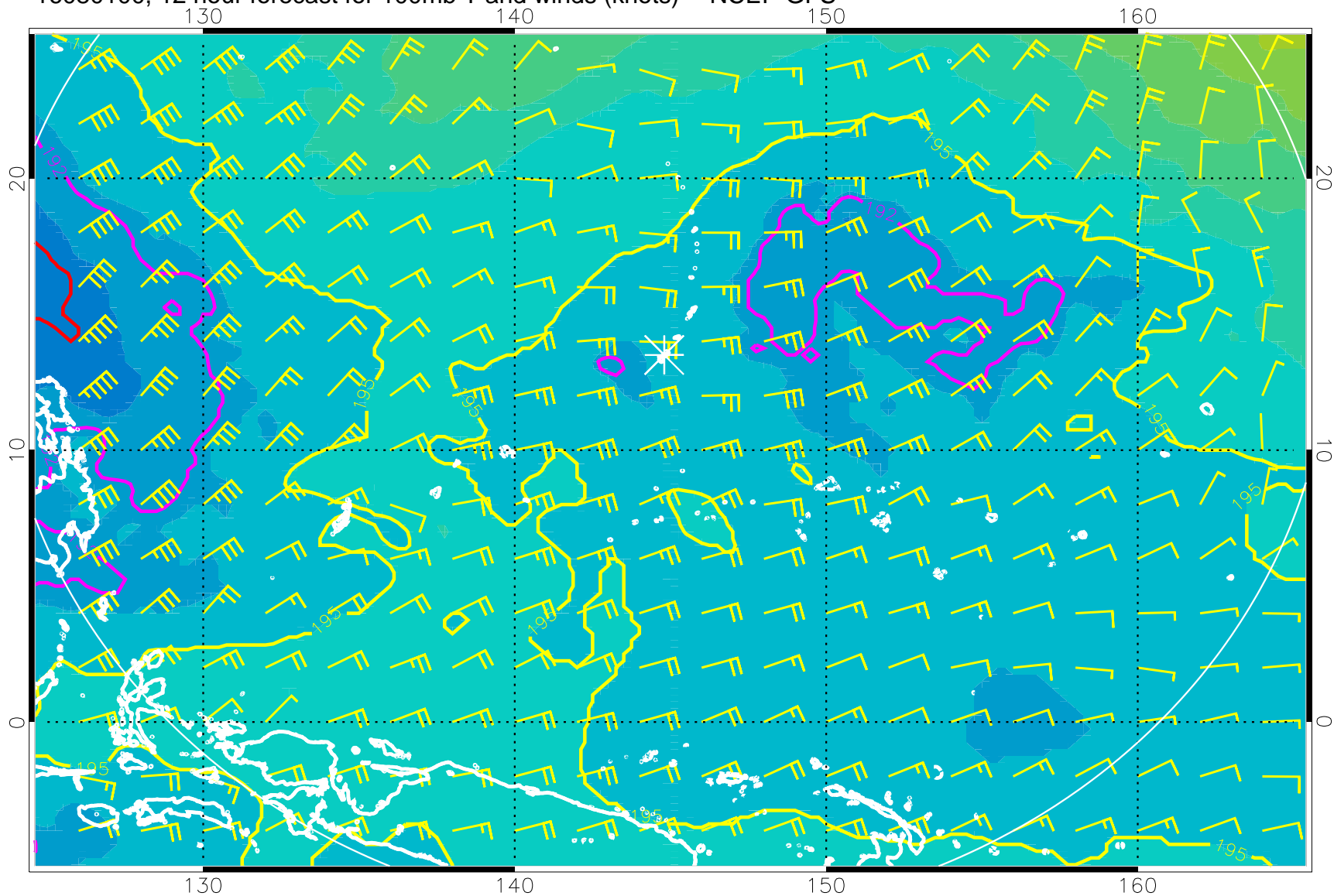
16080100, 12 hour forecast for 100mb T and winds (knots) -- NCEP GFS
