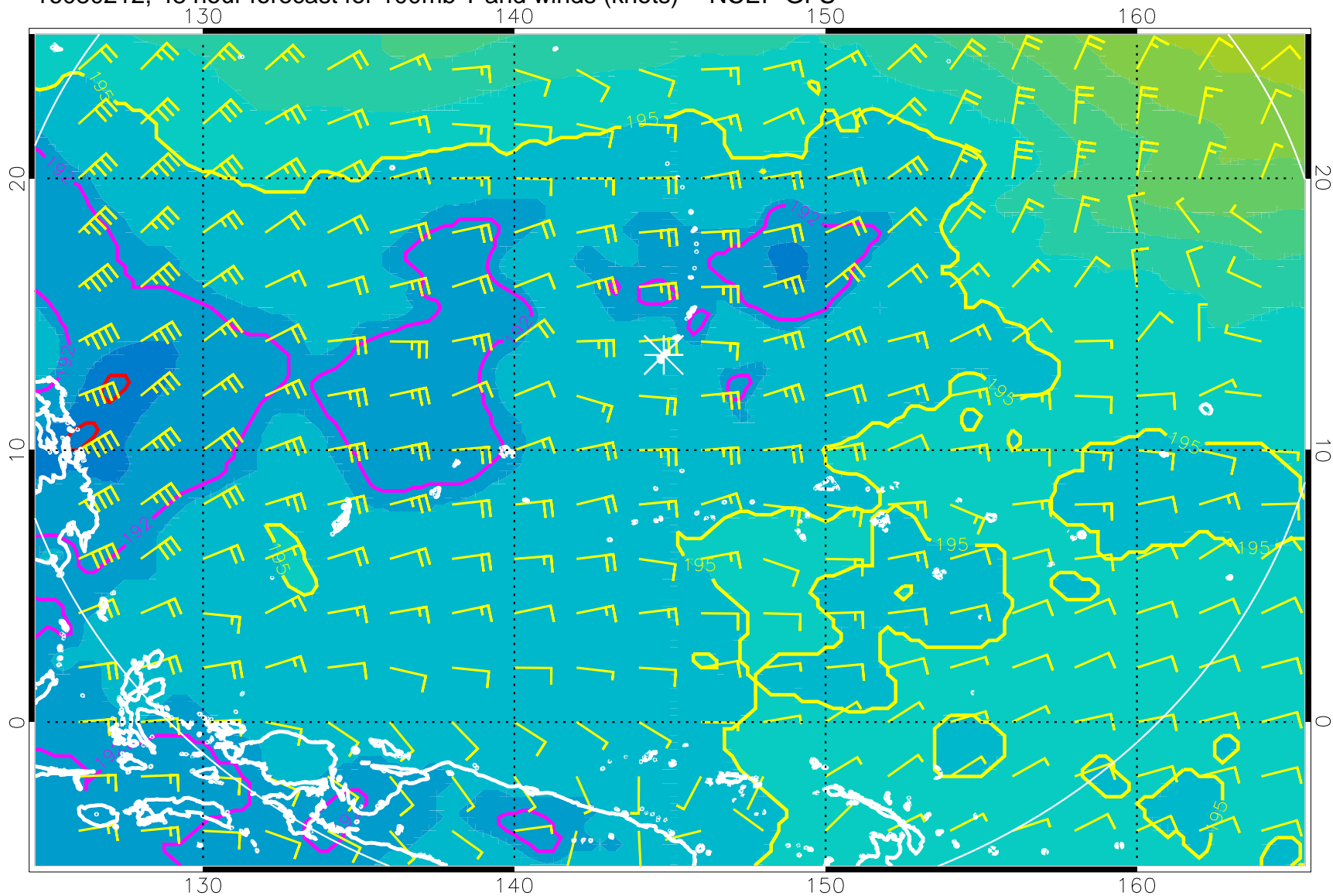
16080212, 48 hour forecast for 100mb T and winds (knots) -- NCEP GFS
