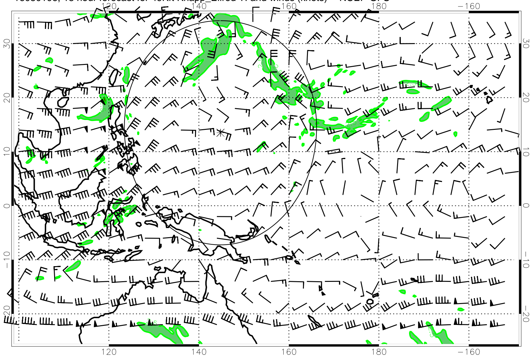
16080106, 18 hour forecast for 49Kft Knapp_Ellrod TI and winds (knots) -- NCEP GFS
