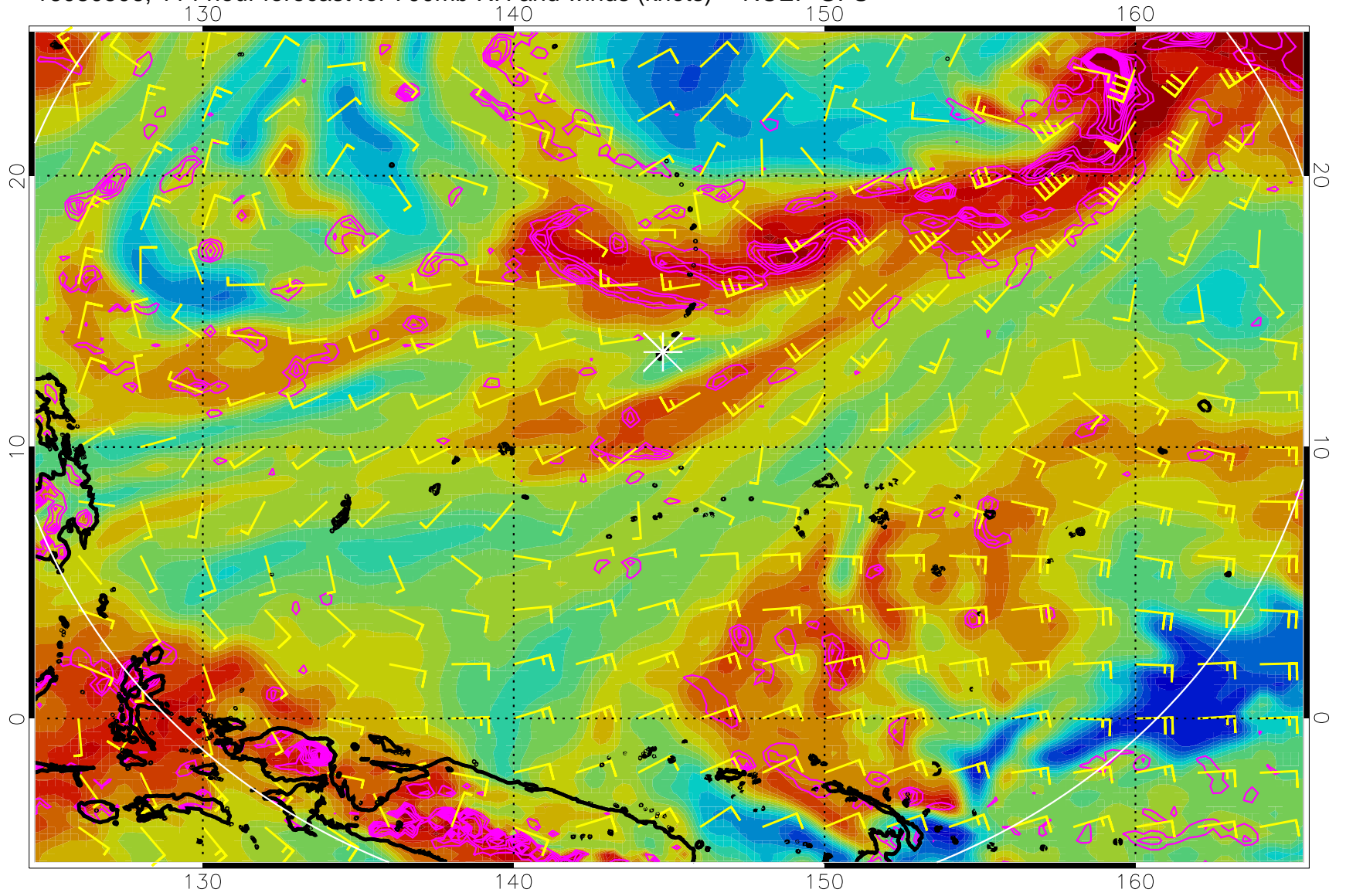
16080506, 114 hour forecast for 700mb RH and winds (knots) -- NCEP GFS
