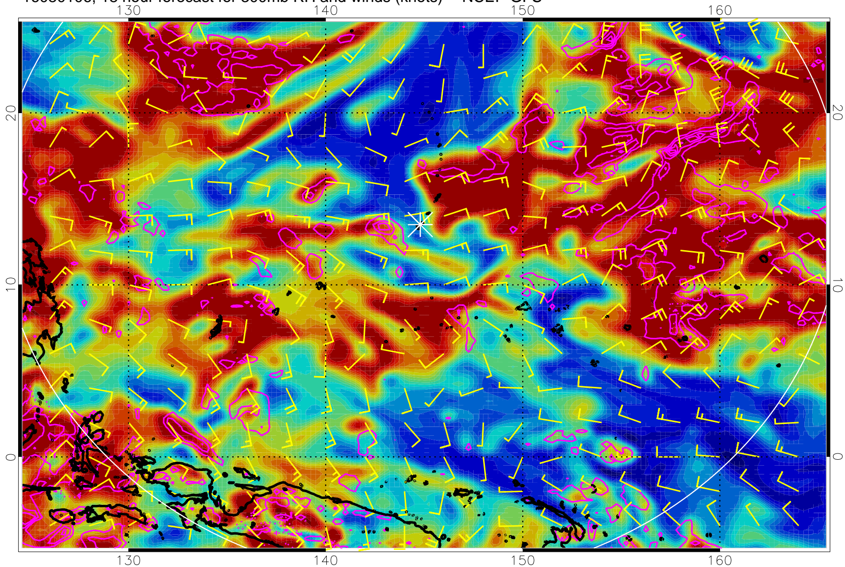
16080106, 18 hour forecast for 300mb RH and winds (knots) -- NCEP GFS
