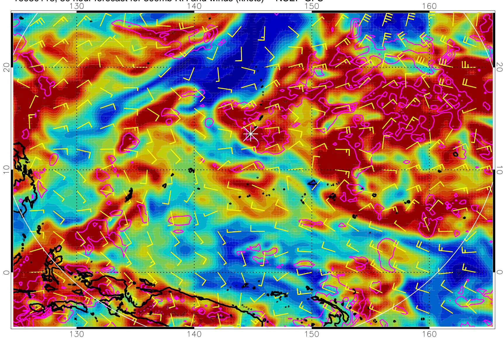
16080118, 30 hour forecast for 300mb RH and winds (knots) -- NCEP GFS
