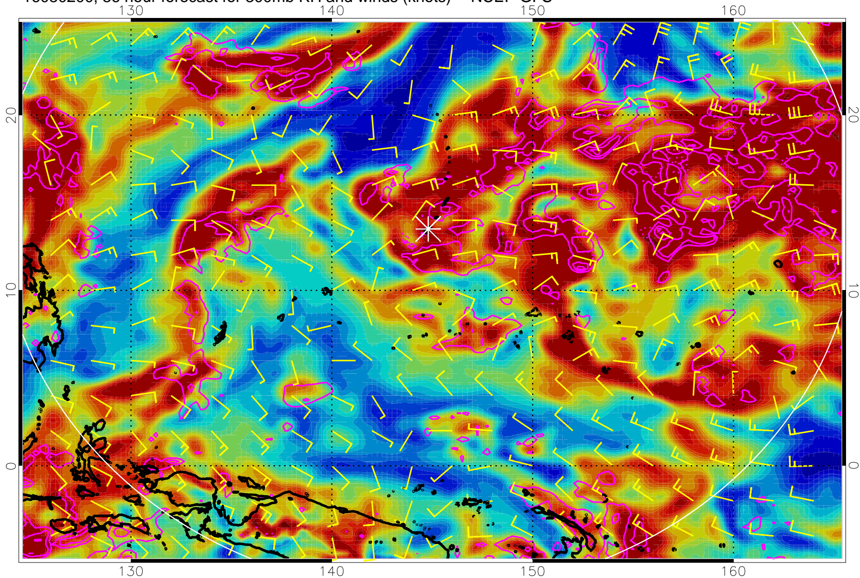
16080200, 36 hour forecast for 300mb RH and winds (knots) -- NCEP GFS
