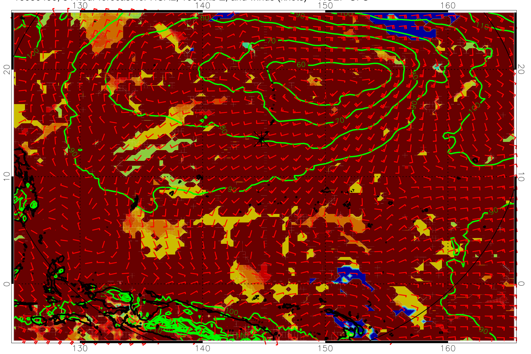
16080400, 84 hour forecast for HCAL, 1000mb Z, and winds (knots) -- NCEP GFS
