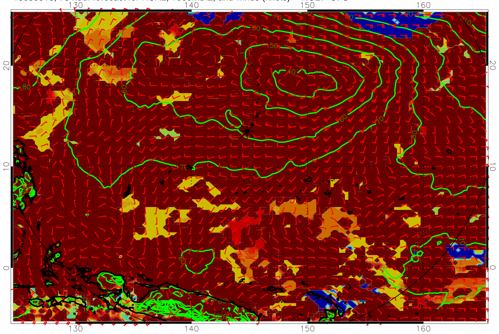
16080318, 78 hour forecast for HCAL, 1000mb Z, and winds (knots) -- NCEP GFS
