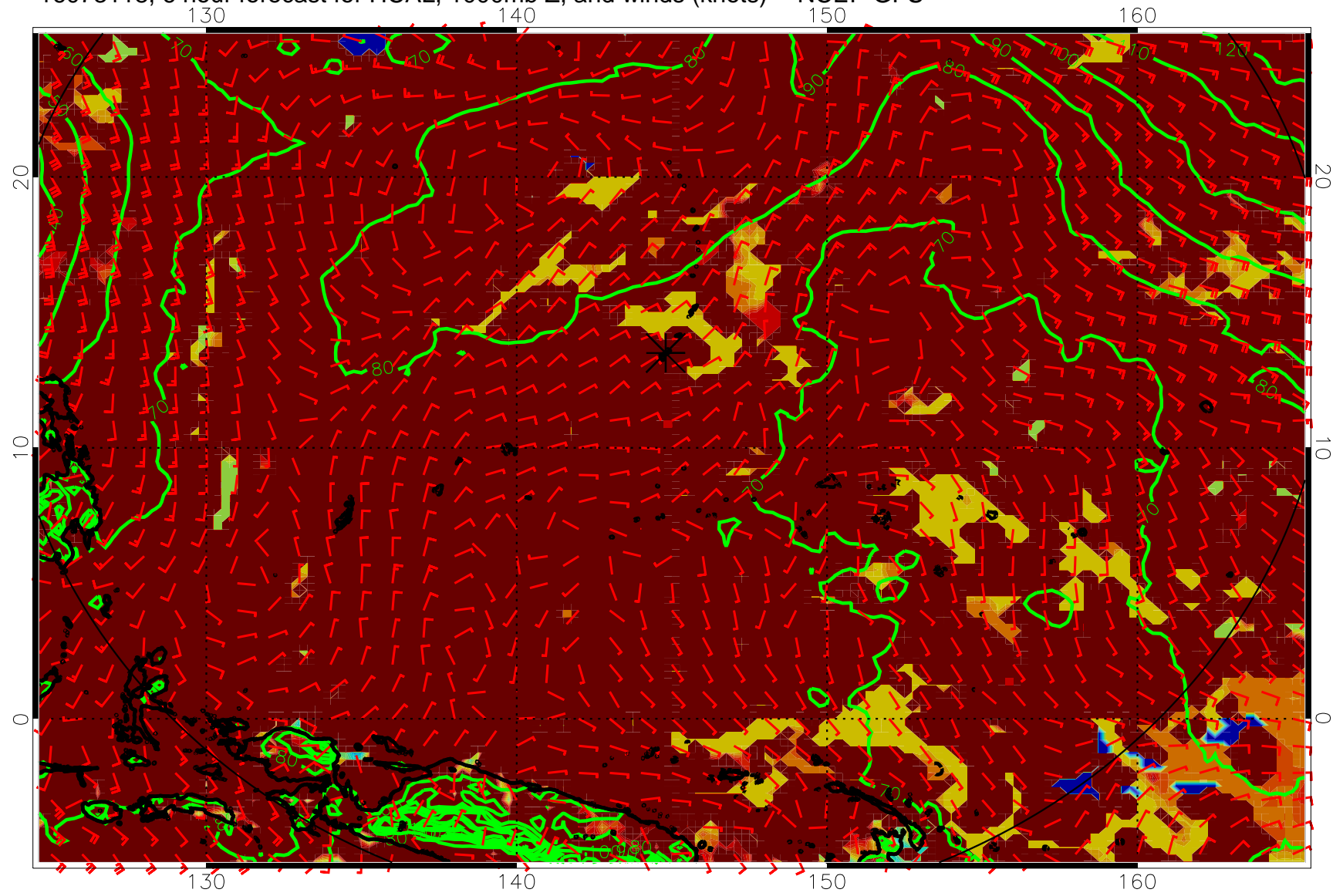
16073118, 6 hour forecast for HCAL, 1000mb Z, and winds (knots) -- NCEP GFS
