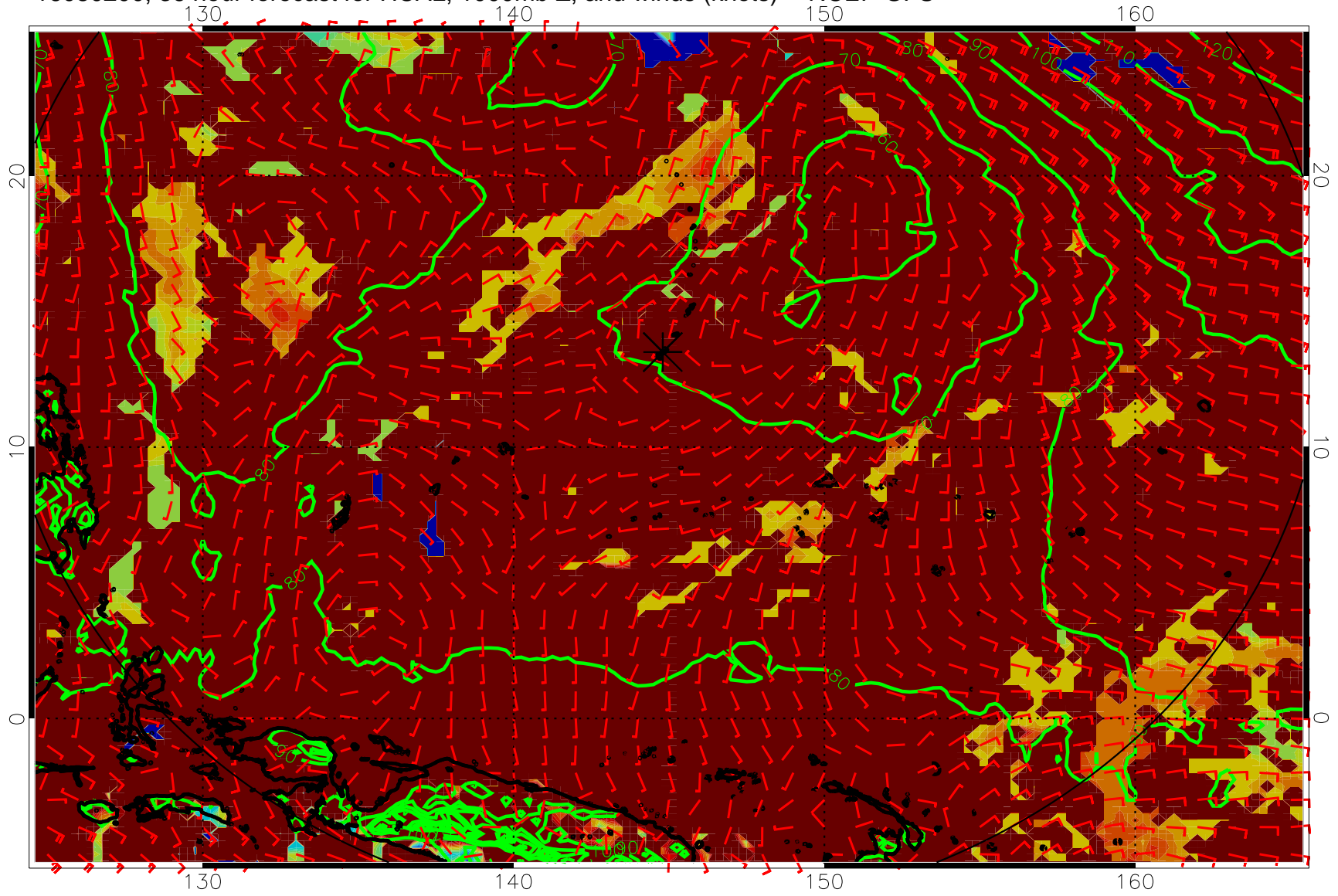
16080200, 36 hour forecast for HCAL, 1000mb Z, and winds (knots) -- NCEP GFS
