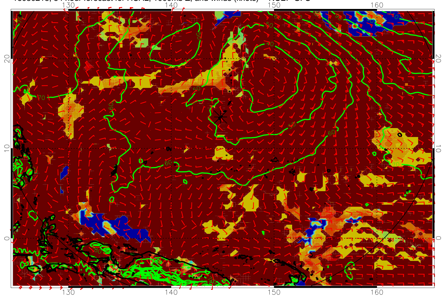
16080218, 54 hour forecast for HCAL, 1000mb Z, and winds (knots) -- NCEP GFS
