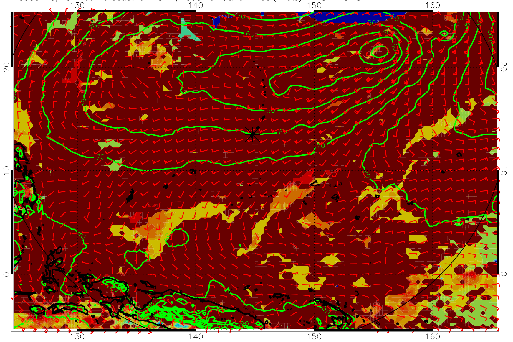
16080418, 102 hour forecast for HCAL, 1000mb Z, and winds (knots) -- NCEP GFS
