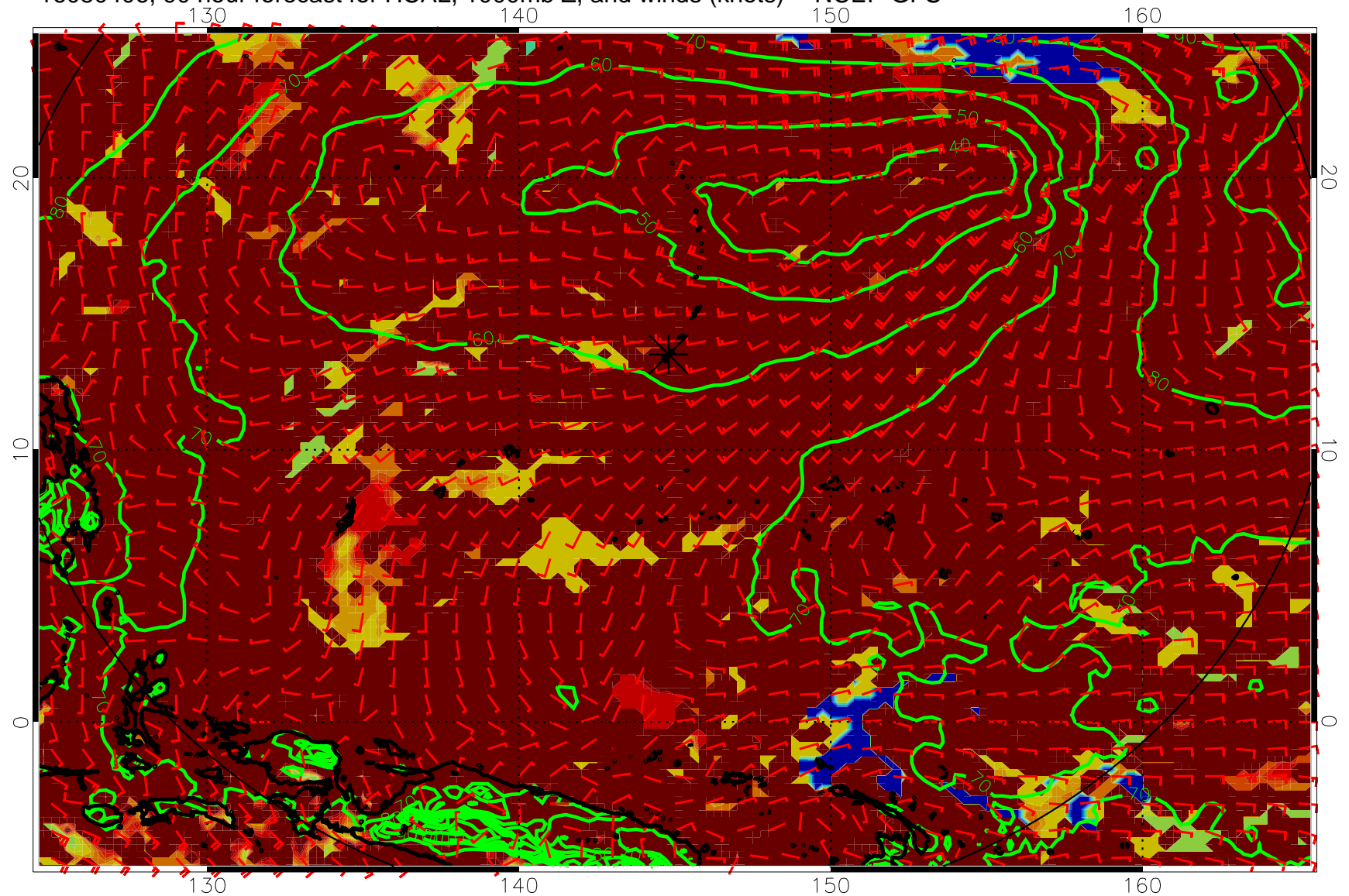
16080406, 90 hour forecast for HCAL, 1000mb Z, and winds (knots) -- NCEP GFS
