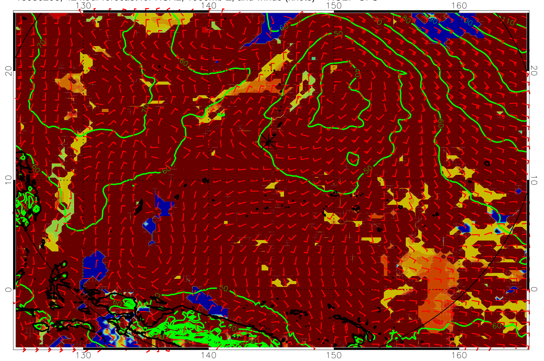
16080206, 42 hour forecast for HCAL, 1000mb Z, and winds (knots) -- NCEP GFS
