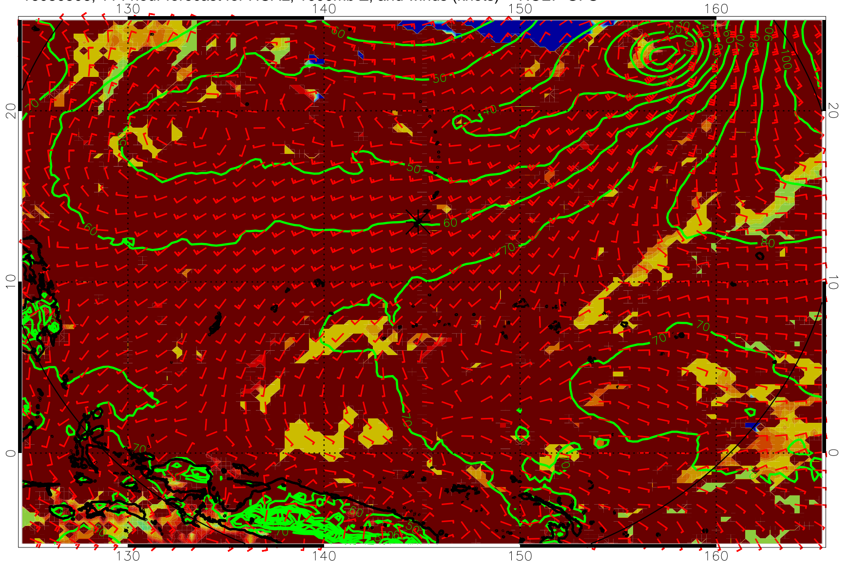
16080506, 114 hour forecast for HCAL, 1000mb Z, and winds (knots) -- NCEP GFS
