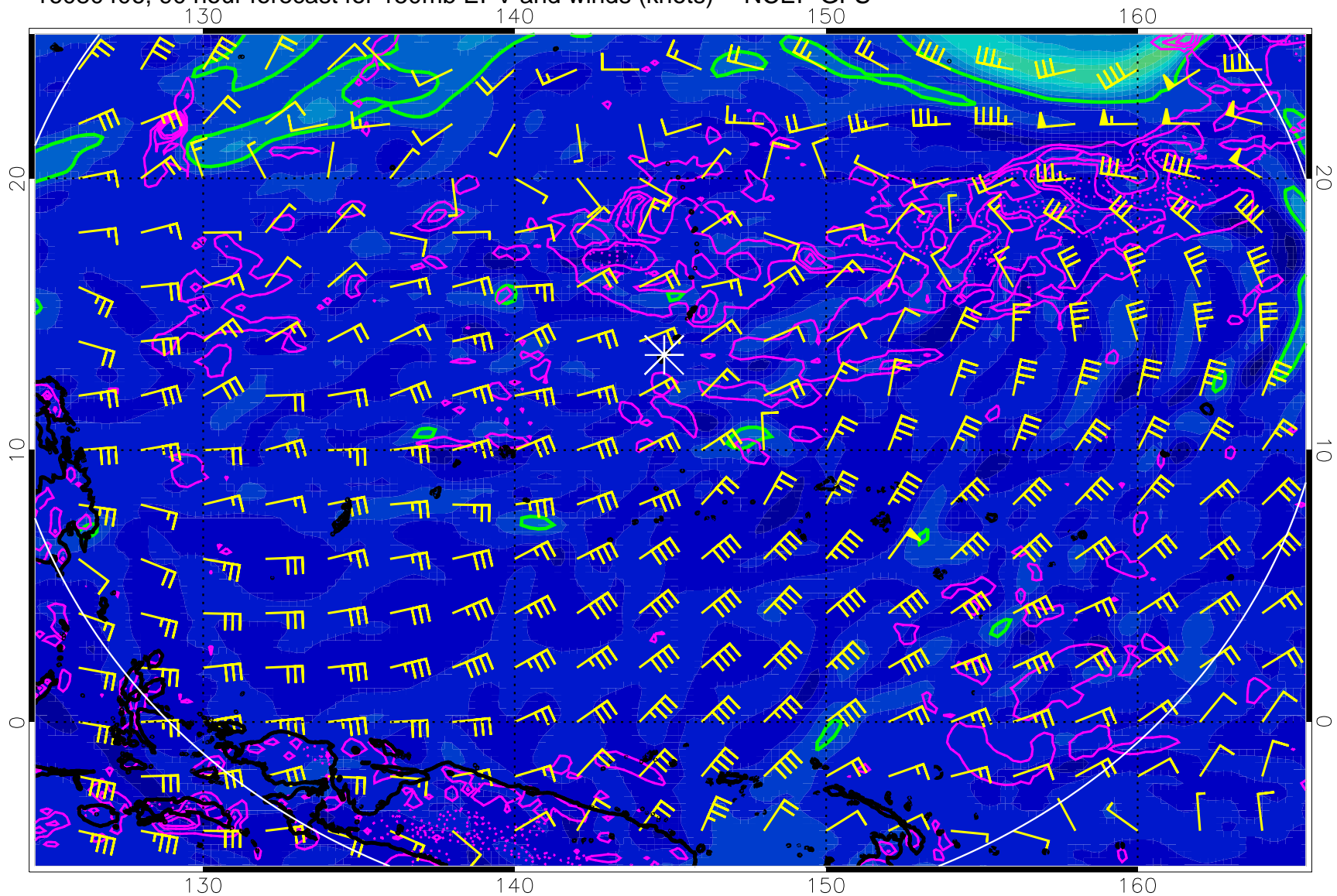
16080406, 90 hour forecast for 150mb EPV and winds (knots) -- NCEP GFS
