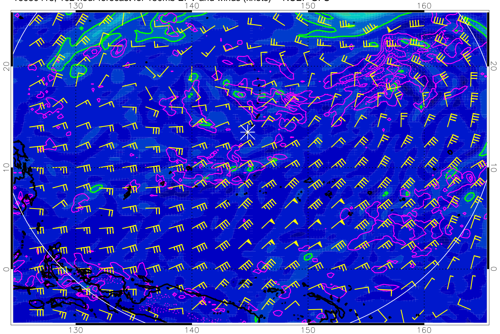
16080418, 102 hour forecast for 150mb EPV and winds (knots) -- NCEP GFS
