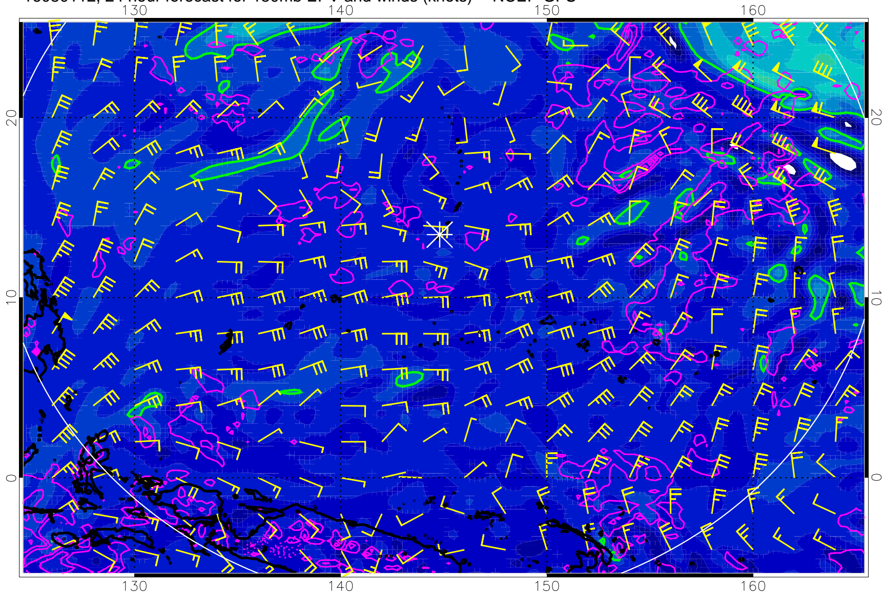
16080112, 24 hour forecast for 150mb EPV and winds (knots) -- NCEP GFS
