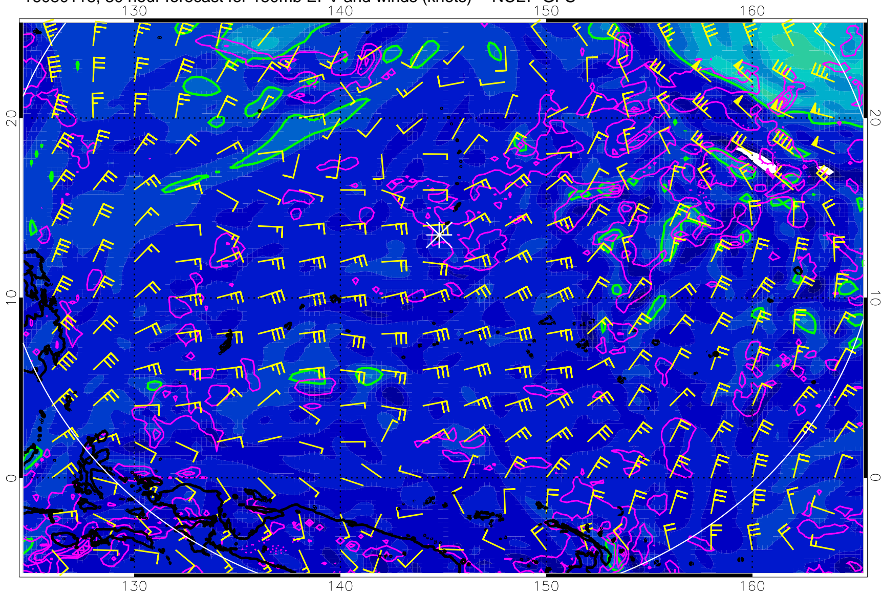
16080118, 30 hour forecast for 150mb EPV and winds (knots) -- NCEP GFS
