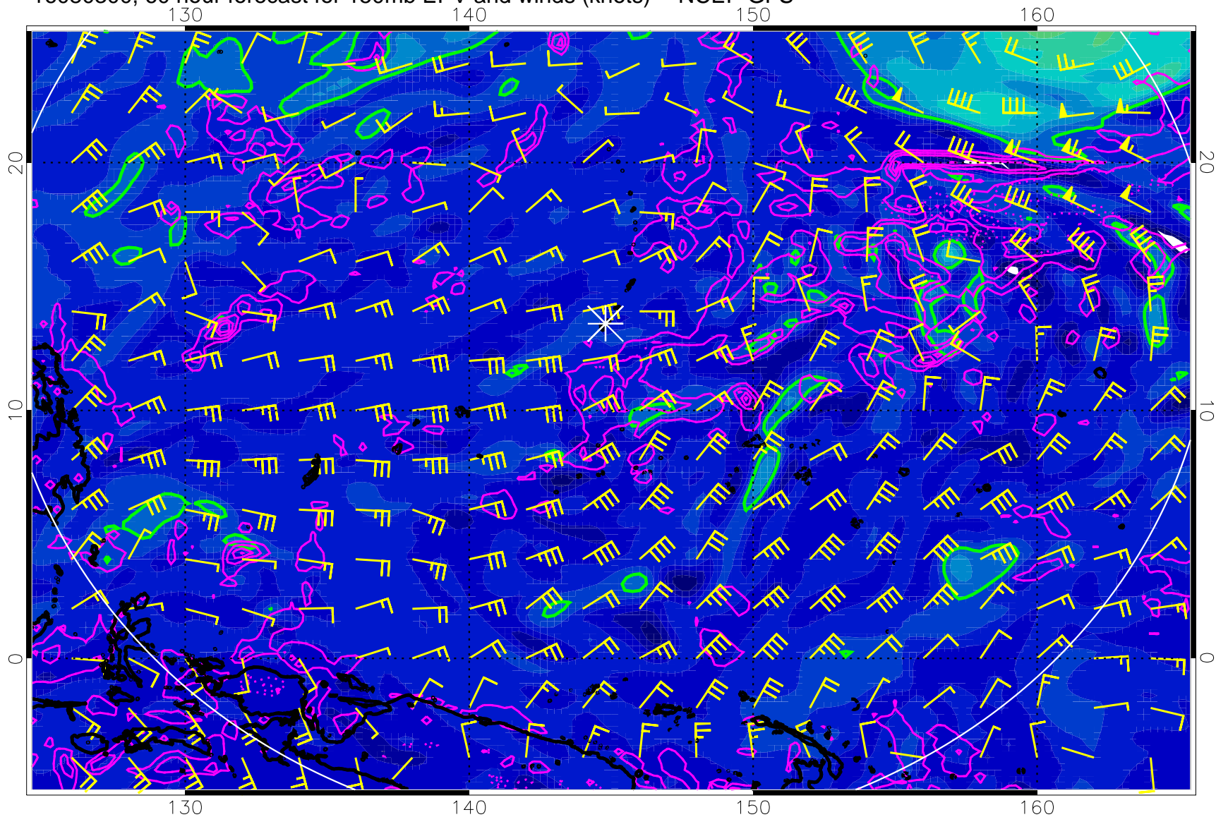
16080300, 60 hour forecast for 150mb EPV and winds (knots) -- NCEP GFS
