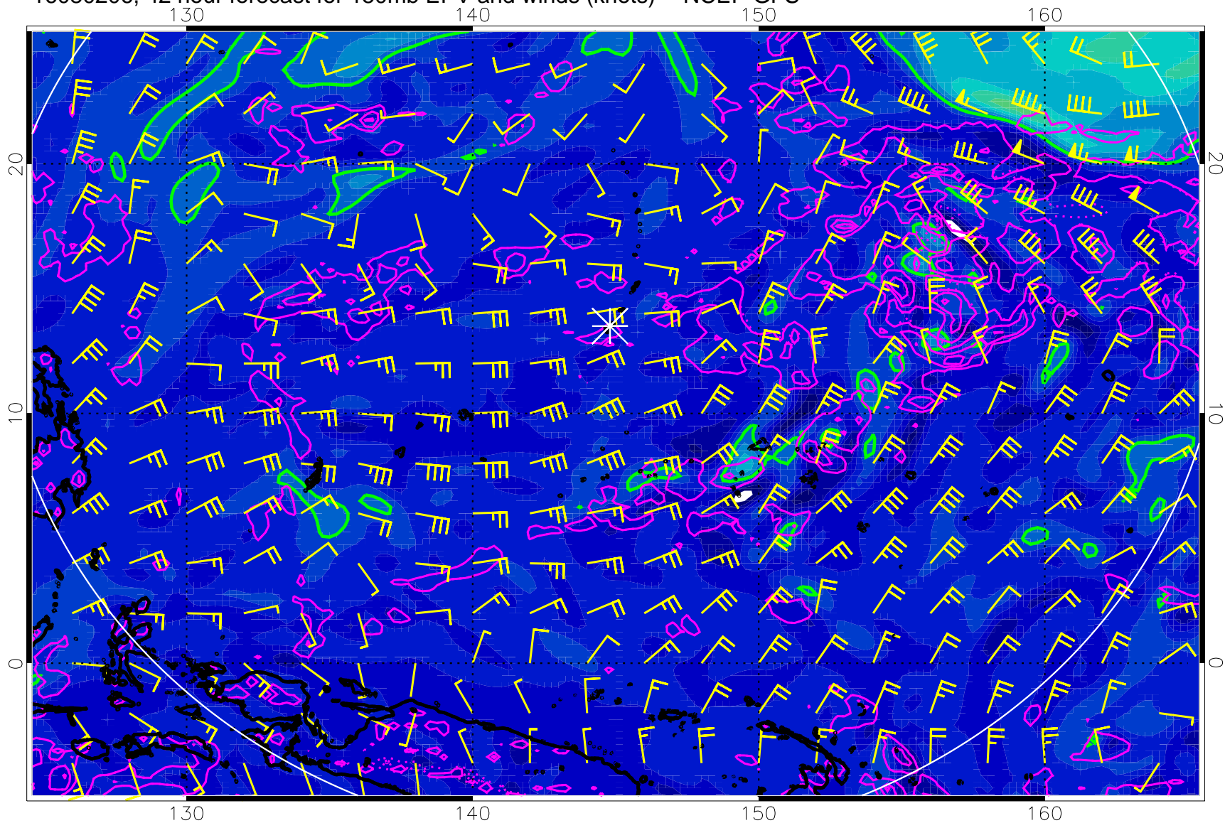
16080206, 42 hour forecast for 150mb EPV and winds (knots) -- NCEP GFS
