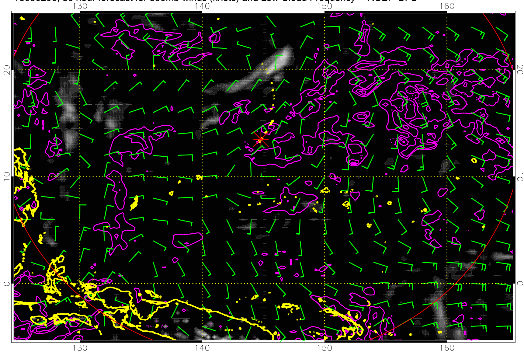
16080200, 36 hour forecast for 850mb winds (knots) and Low Cloud Frequency -- NCEP GFS
