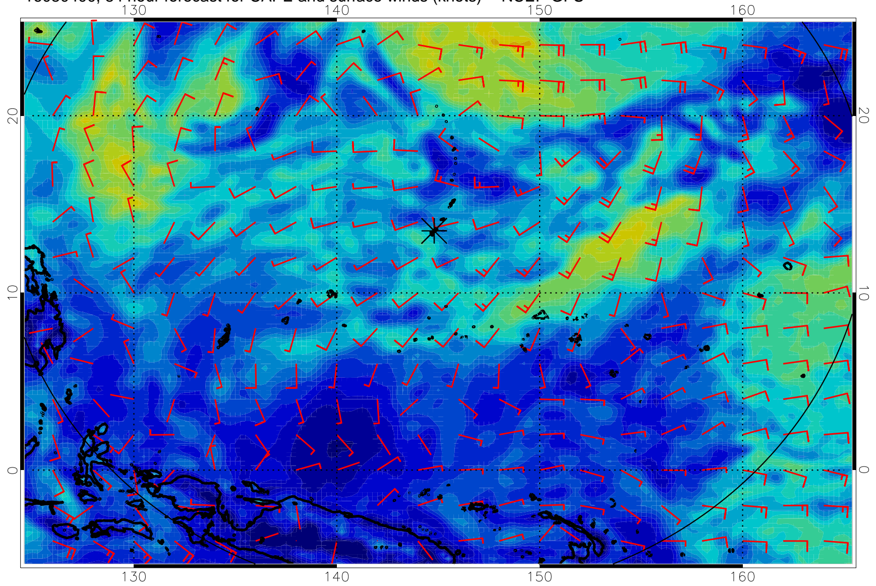
16080400, 84 hour forecast for CAPE and surface winds (knots) -- NCEP GFS
