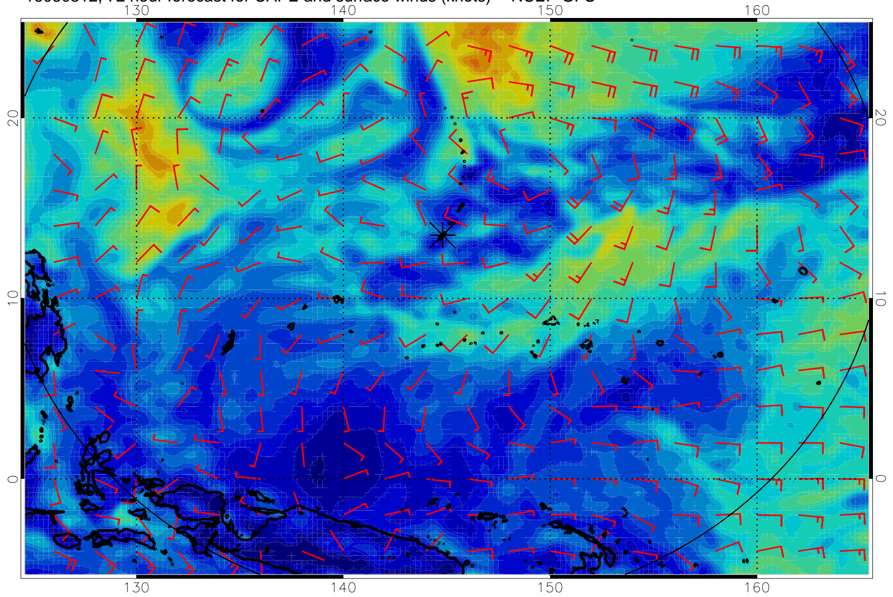
16080312, 72 hour forecast for CAPE and surface winds (knots) -- NCEP GFS
