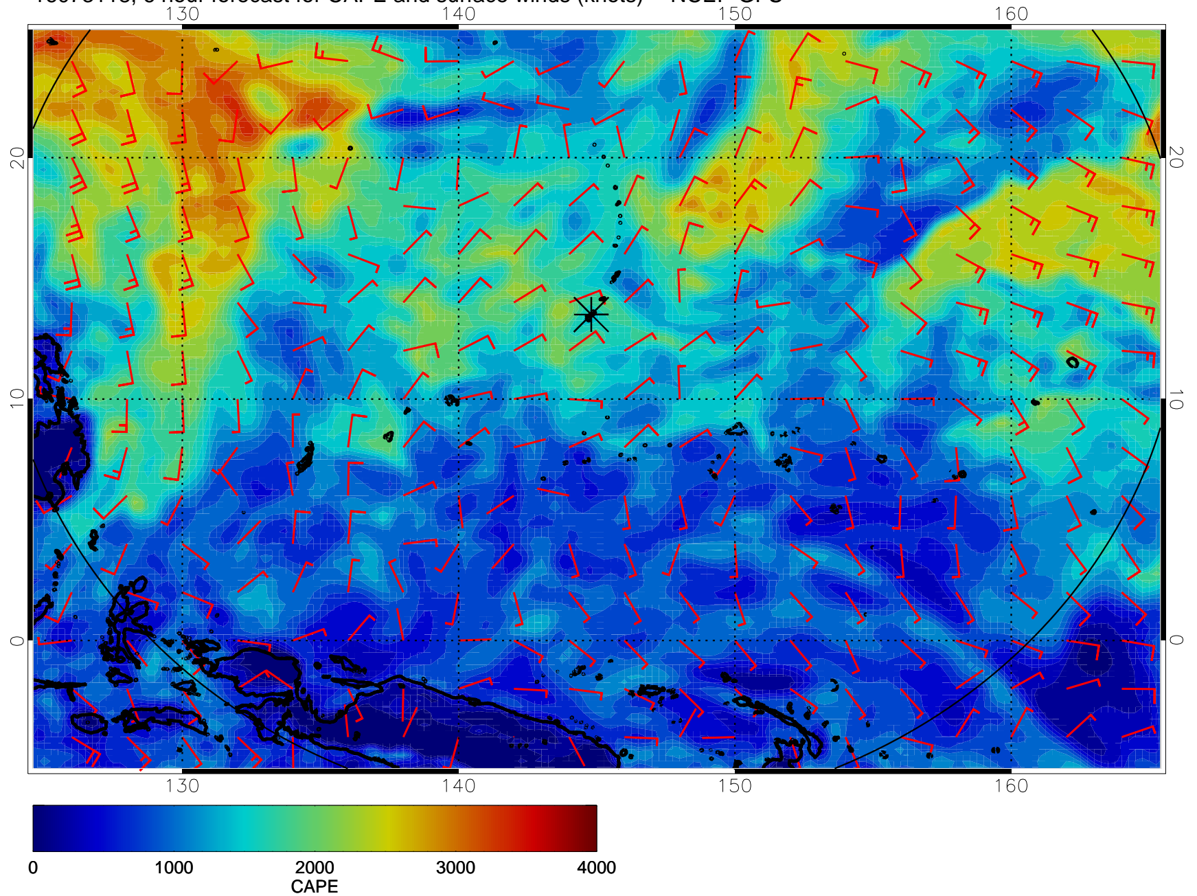
16073118, 6 hour forecast for CAPE and surface winds (knots) -- NCEP GFS
