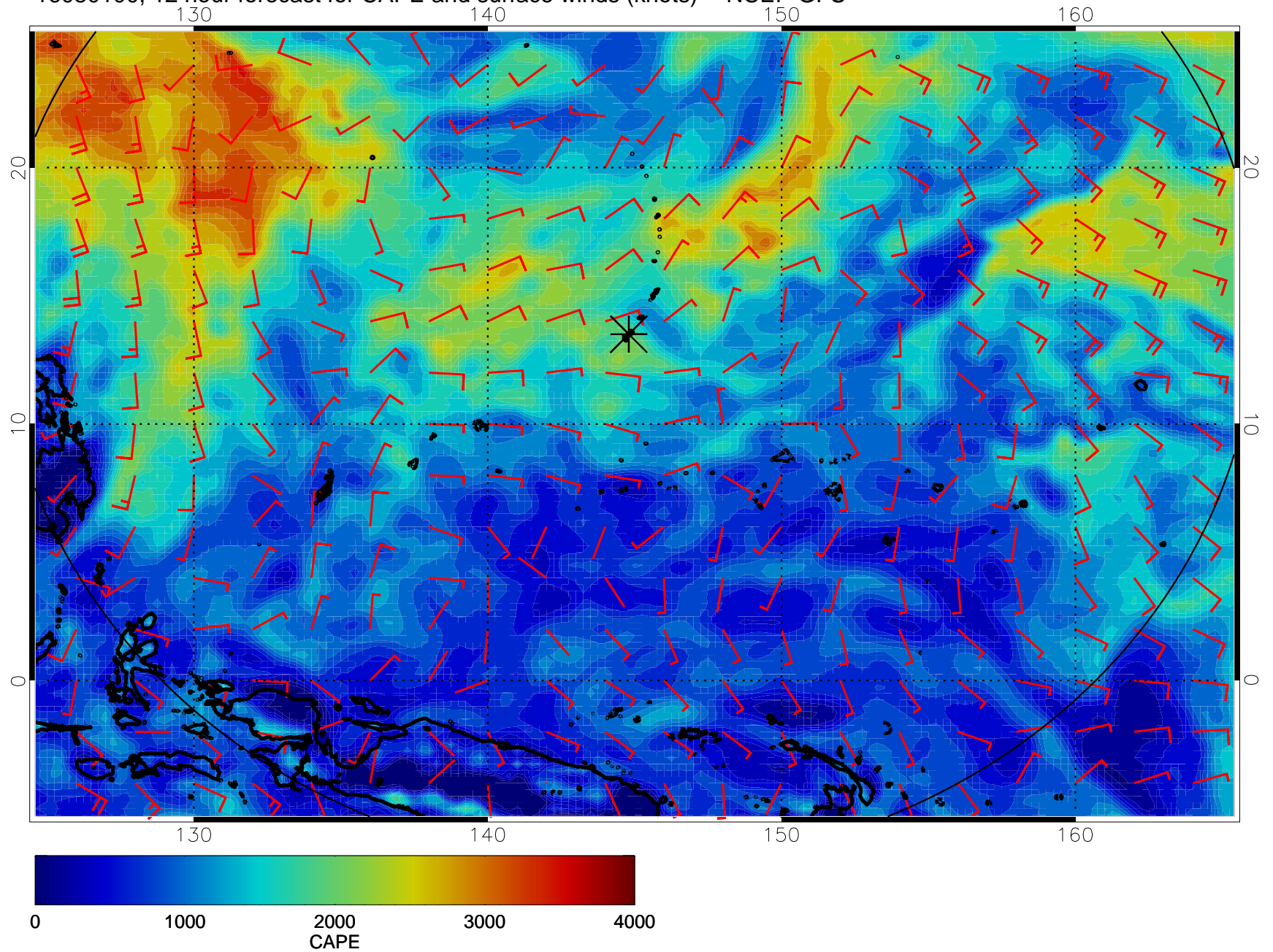
16080100, 12 hour forecast for CAPE and surface winds (knots) -- NCEP GFS
