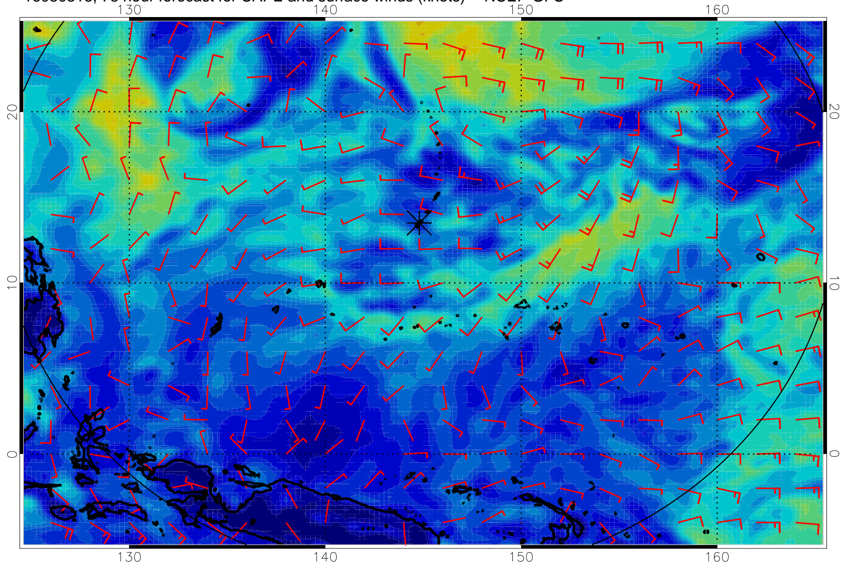
16080318, 78 hour forecast for CAPE and surface winds (knots) -- NCEP GFS
