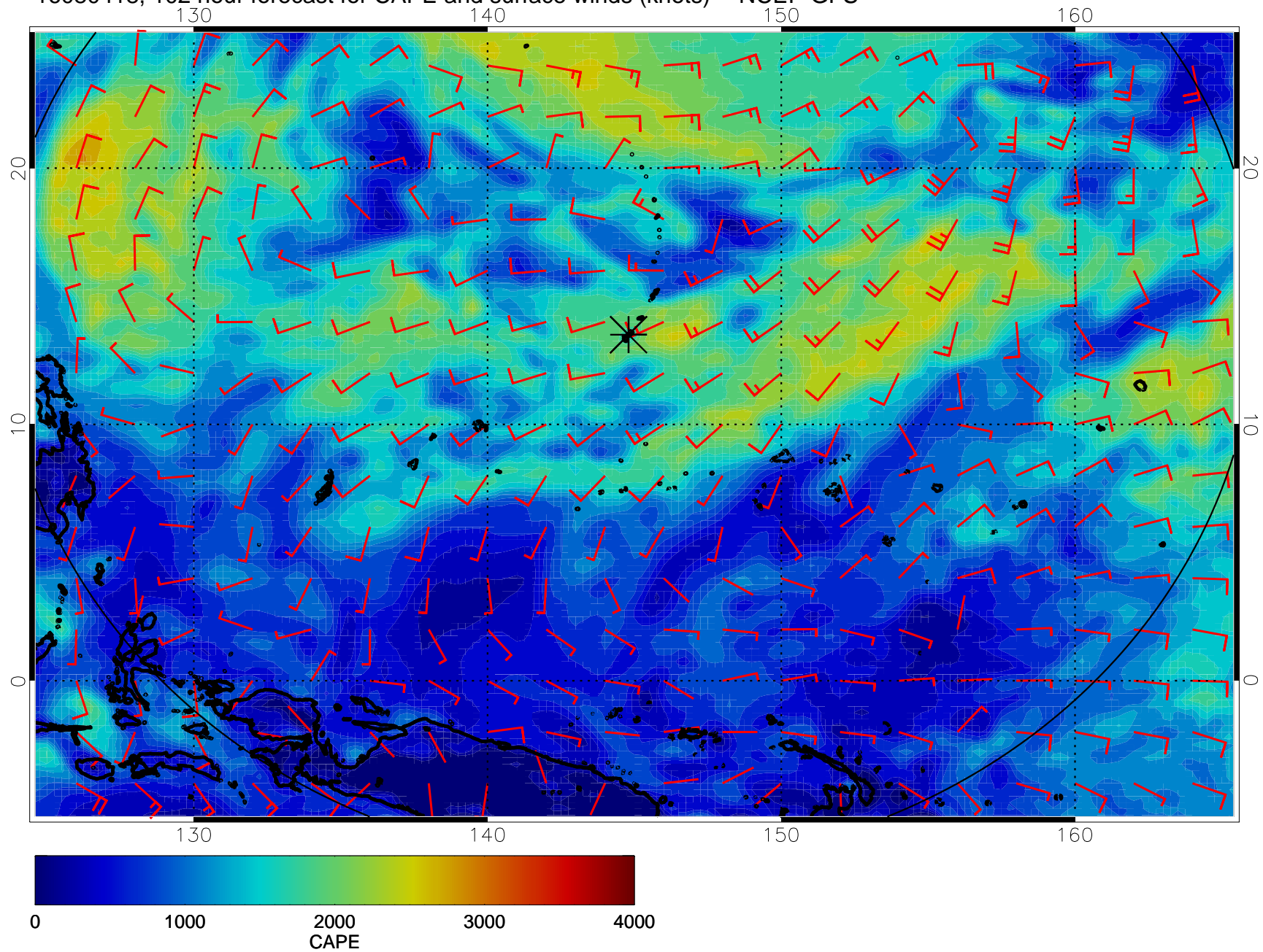
16080418, 102 hour forecast for CAPE and surface winds (knots) -- NCEP GFS
