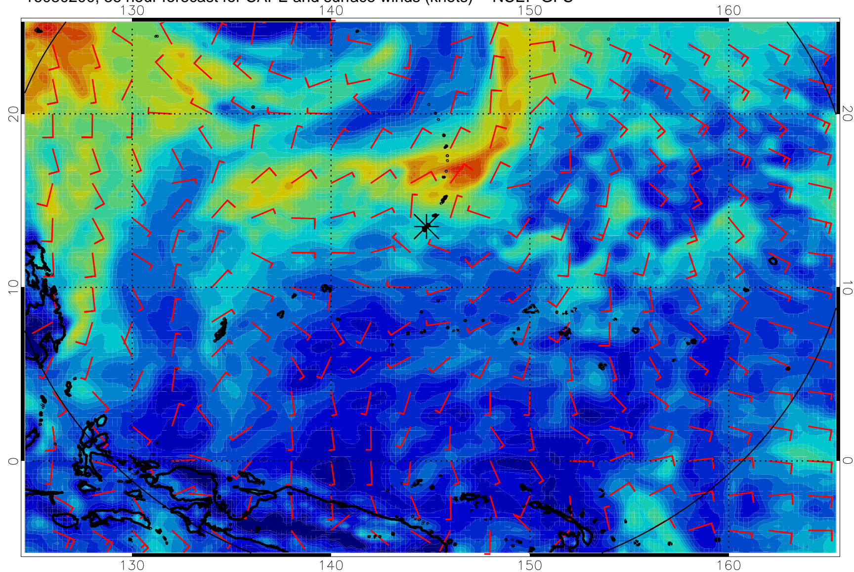
16080200, 36 hour forecast for CAPE and surface winds (knots) -- NCEP GFS
