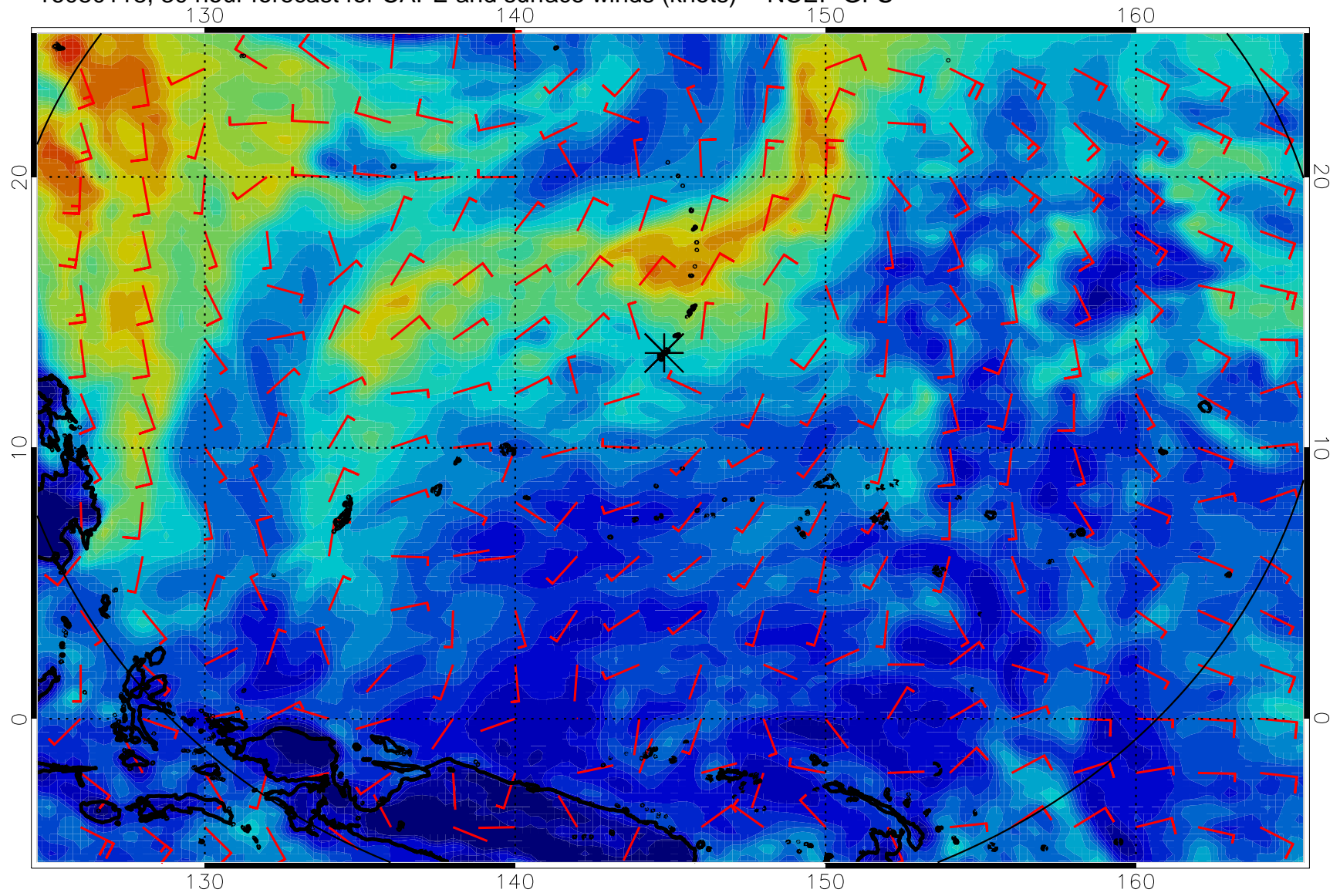
16080118, 30 hour forecast for CAPE and surface winds (knots) -- NCEP GFS
