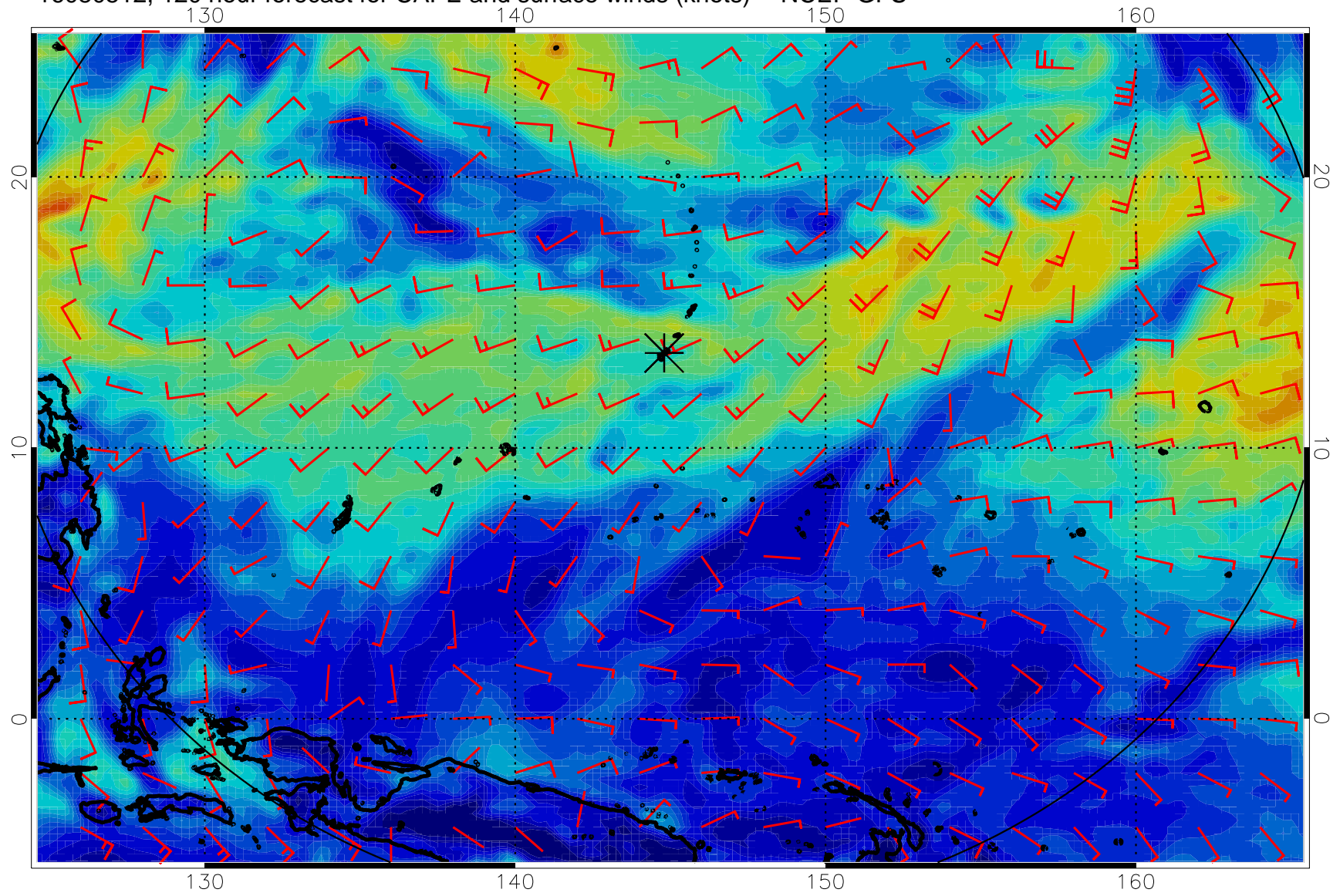
16080512, 120 hour forecast for CAPE and surface winds (knots) -- NCEP GFS
