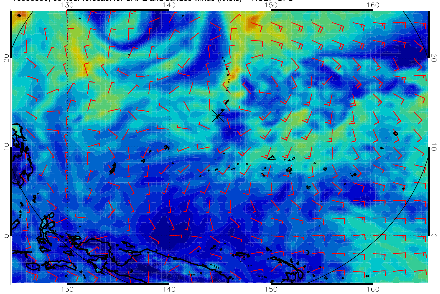
16080300, 60 hour forecast for CAPE and surface winds (knots) -- NCEP GFS
