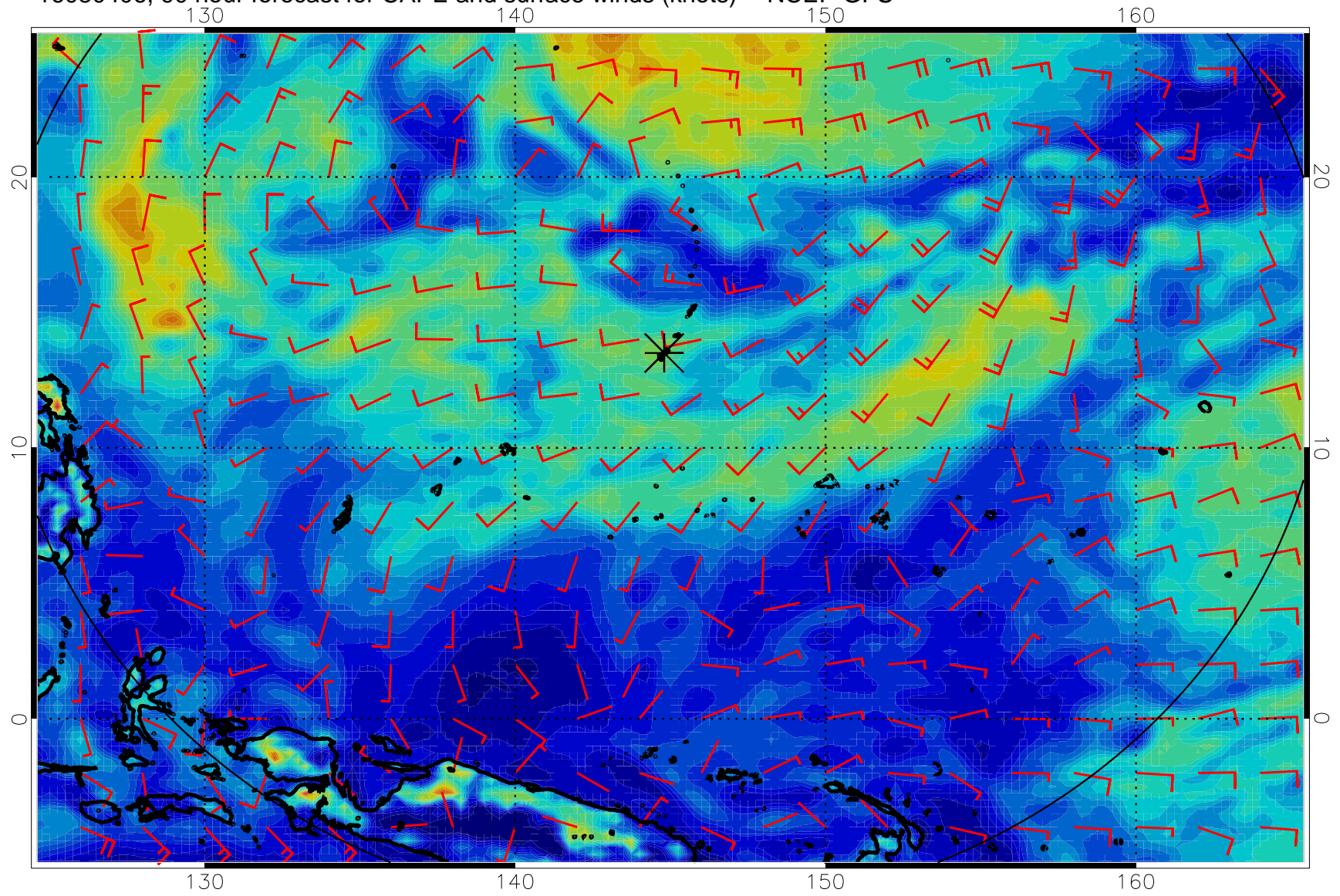
16080406, 90 hour forecast for CAPE and surface winds (knots) -- NCEP GFS
