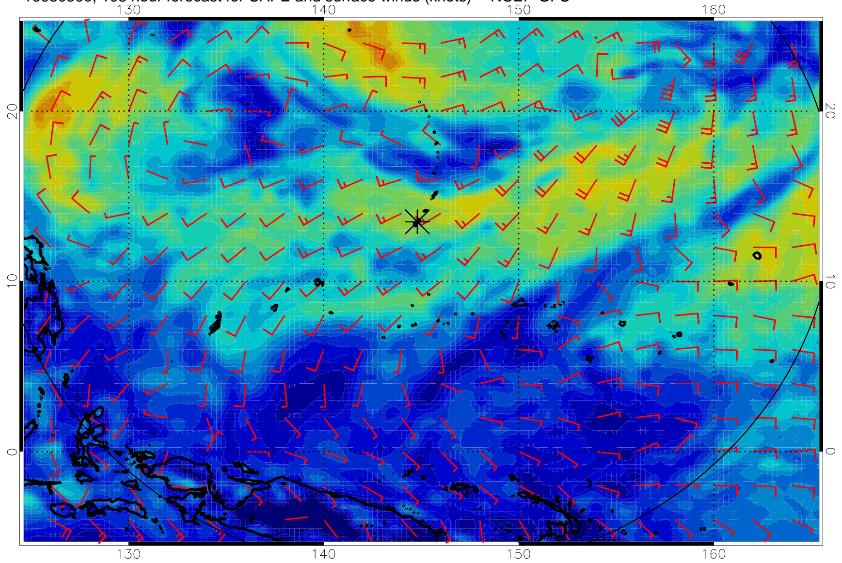
16080500, 108 hour forecast for CAPE and surface winds (knots) -- NCEP GFS
