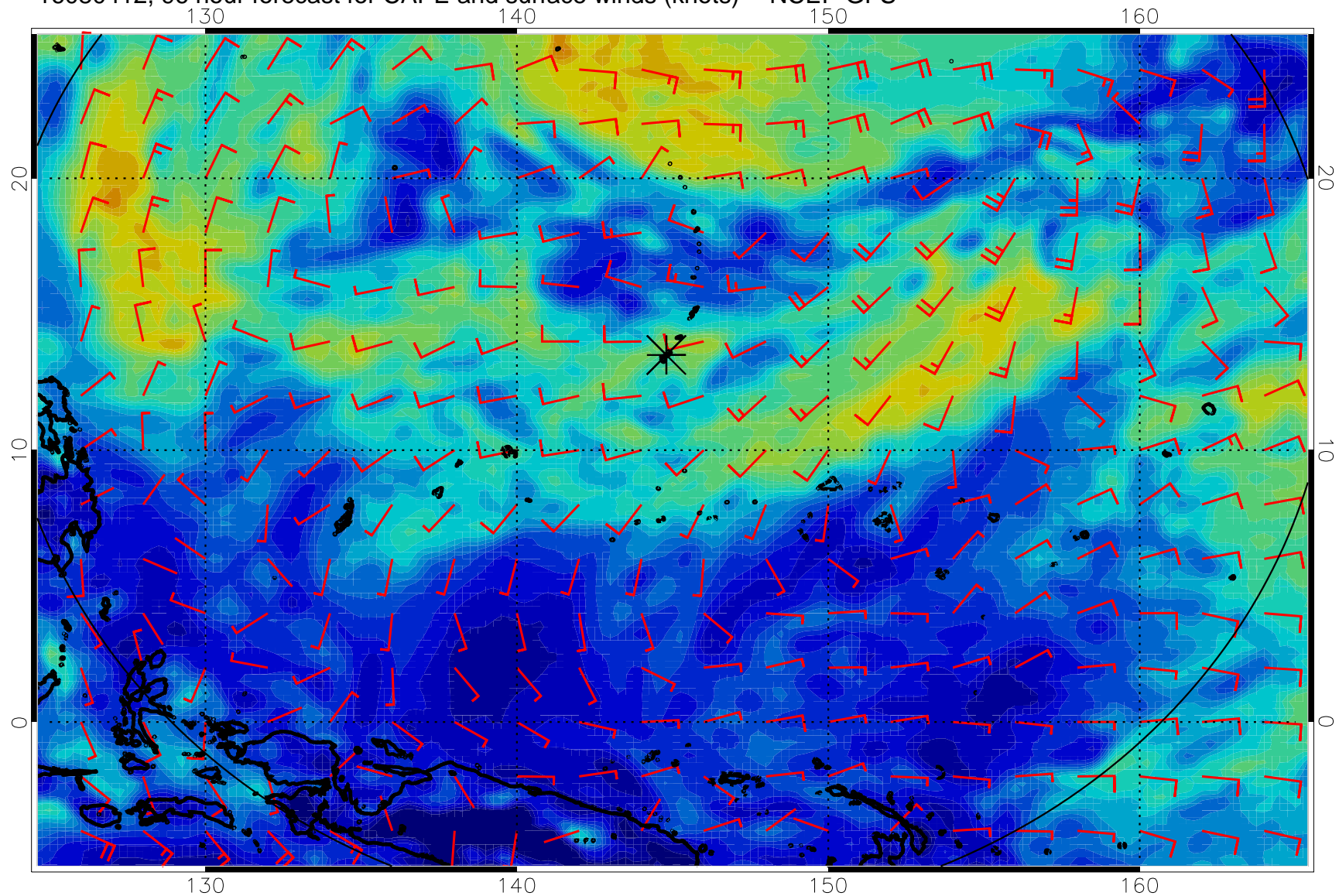
16080412, 96 hour forecast for CAPE and surface winds (knots) -- NCEP GFS
