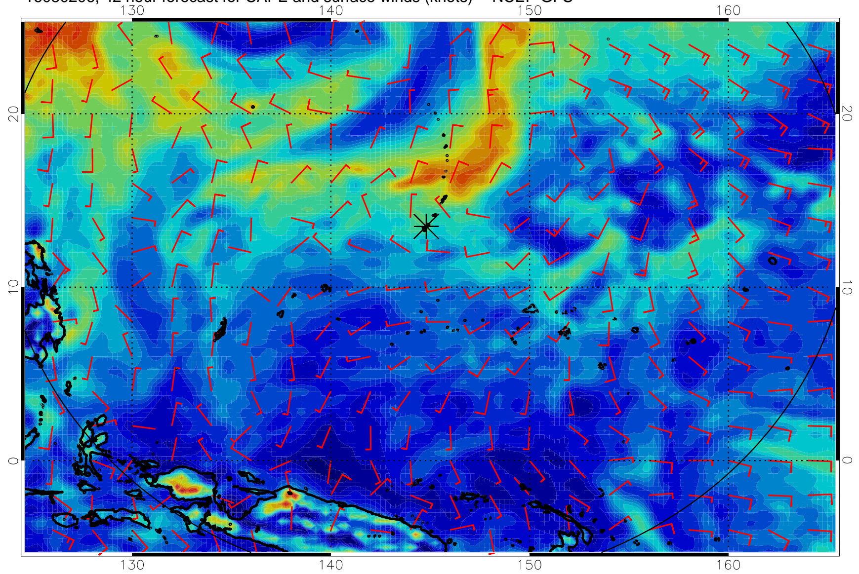
16080206, 42 hour forecast for CAPE and surface winds (knots) -- NCEP GFS
