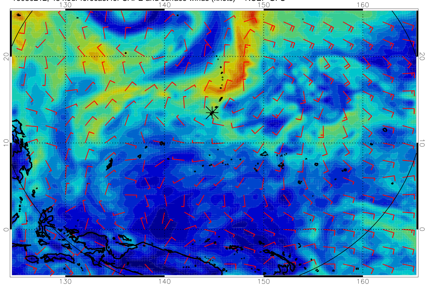
16080212, 48 hour forecast for CAPE and surface winds (knots) -- NCEP GFS
