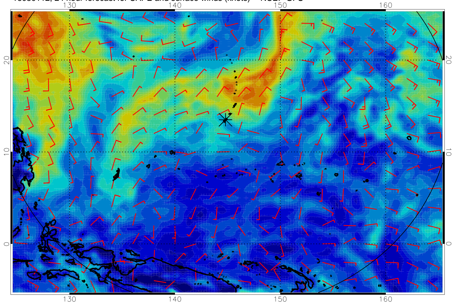
16080112, 24 hour forecast for CAPE and surface winds (knots) -- NCEP GFS
