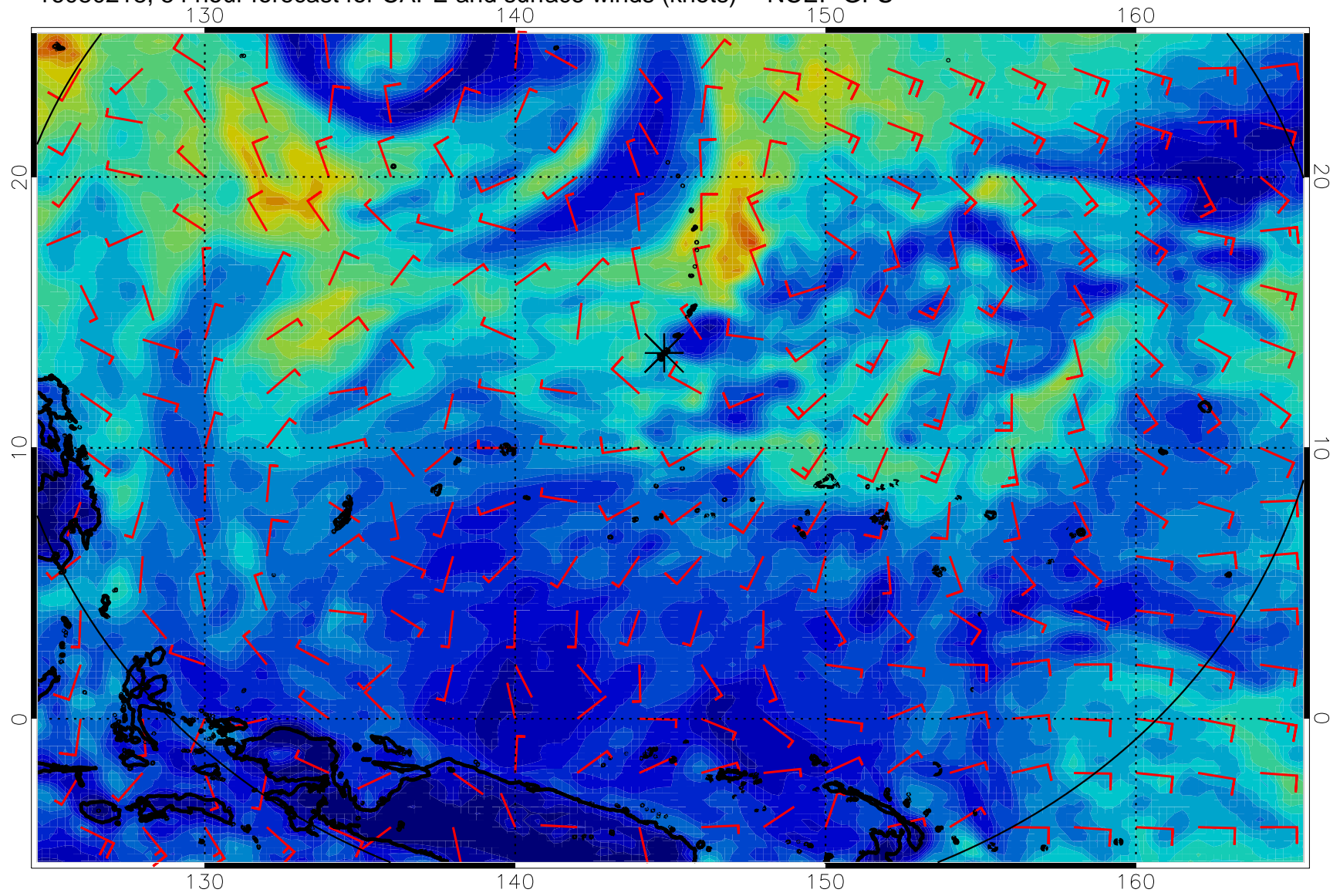
16080218, 54 hour forecast for CAPE and surface winds (knots) -- NCEP GFS
