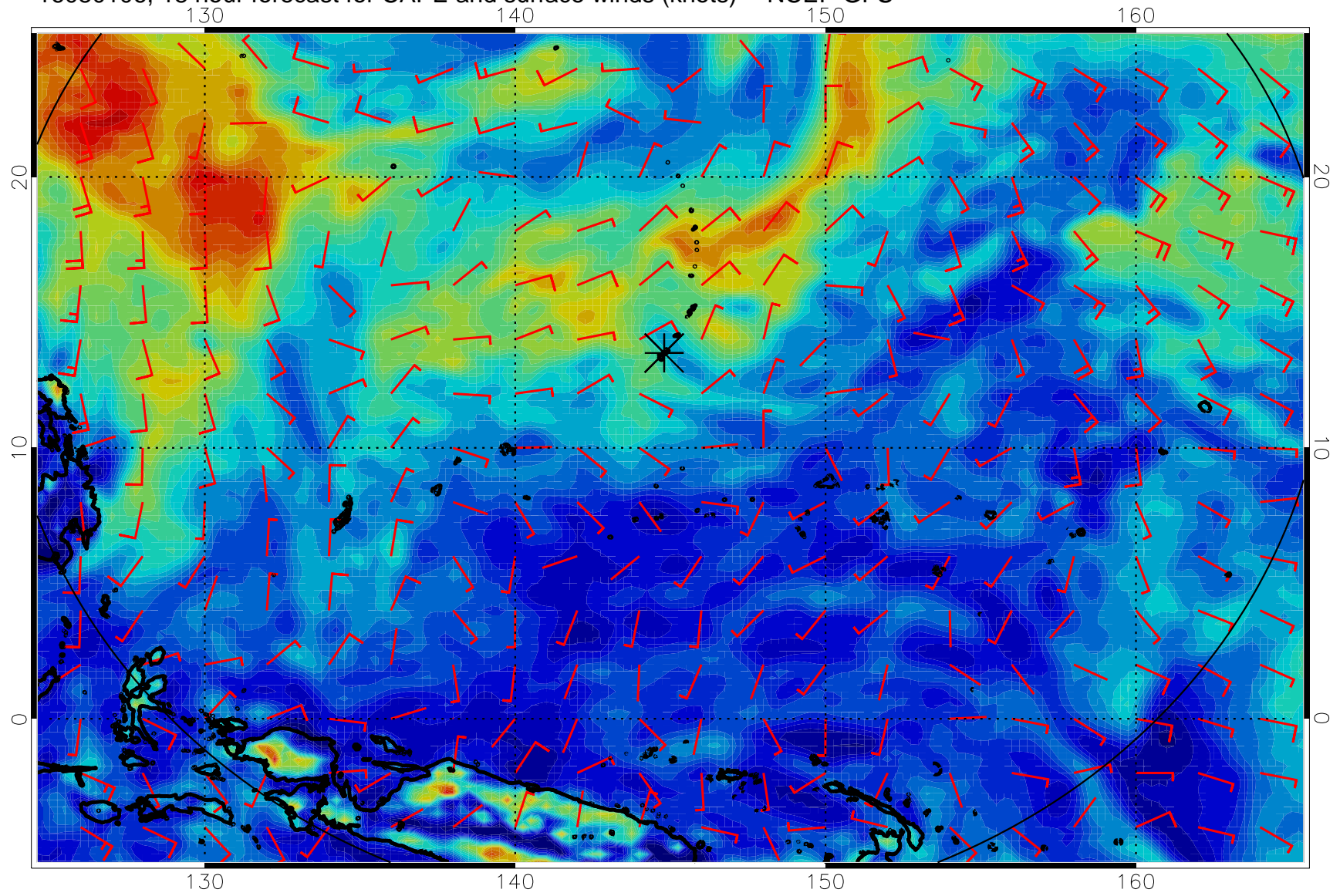
16080106, 18 hour forecast for CAPE and surface winds (knots) -- NCEP GFS
