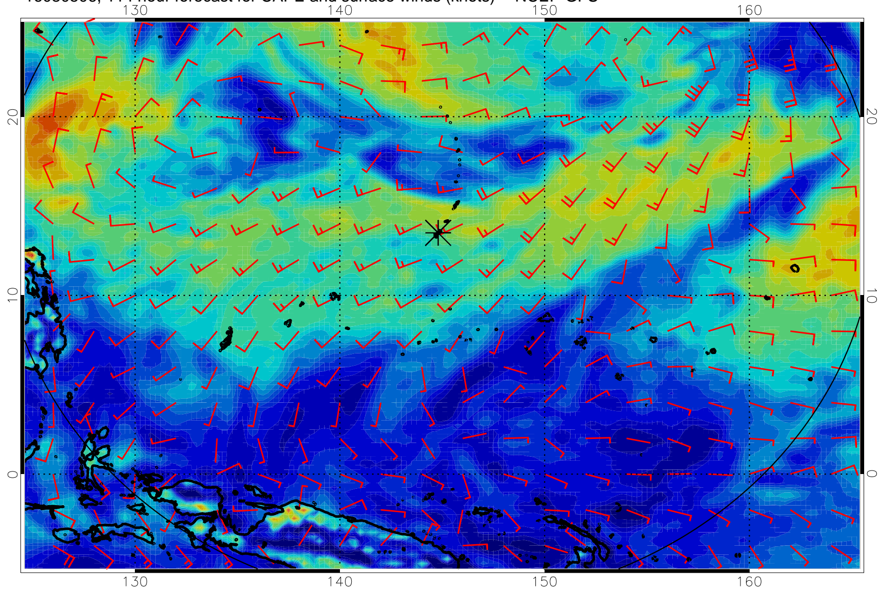
16080506, 114 hour forecast for CAPE and surface winds (knots) -- NCEP GFS
