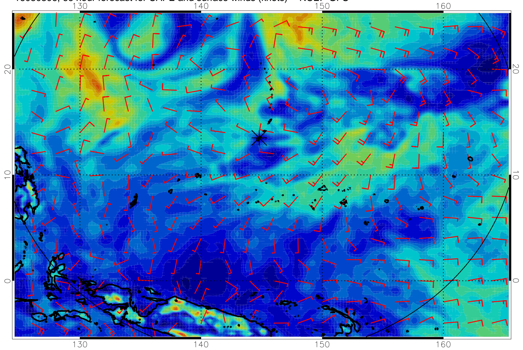
16080306, 66 hour forecast for CAPE and surface winds (knots) -- NCEP GFS
