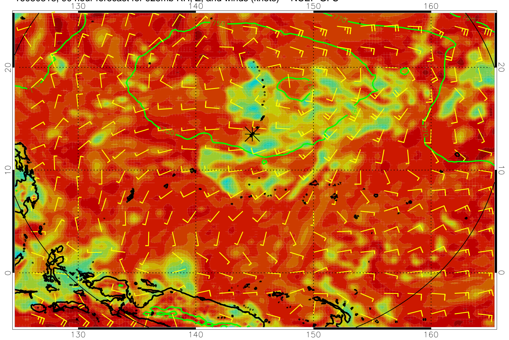
16080318, 90 hour forecast for 925mb RH, Z, and winds (knots) -- NCEP GFS
