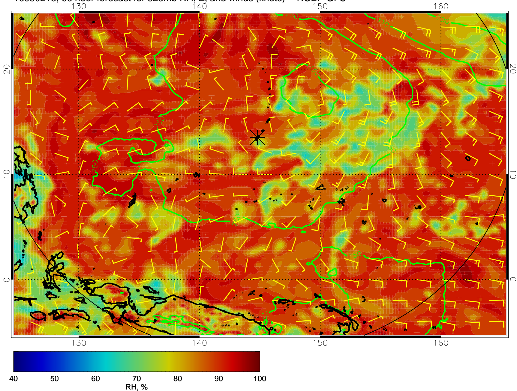
16080218, 66 hour forecast for 925mb RH, Z, and winds (knots) -- NCEP GFS
