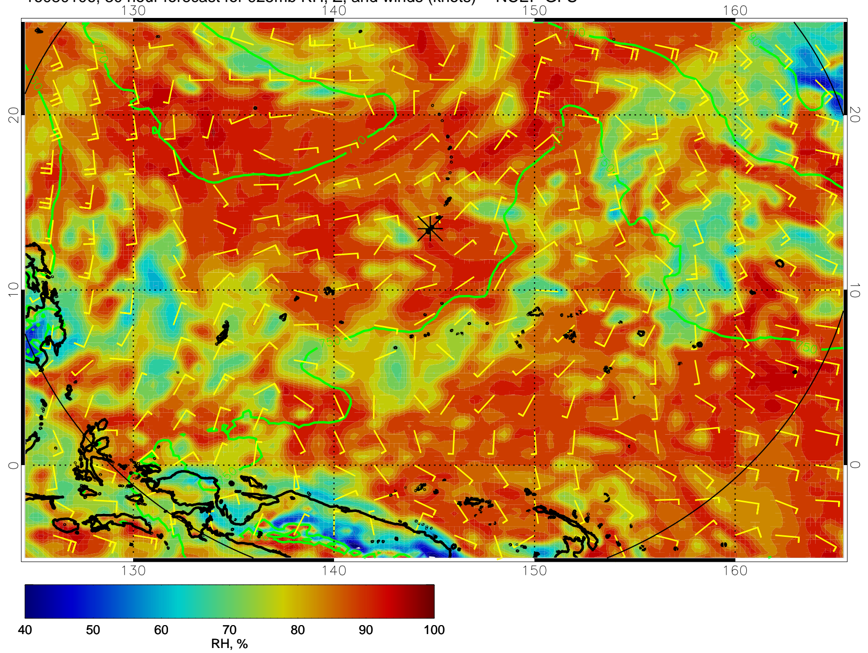
16080106, 30 hour forecast for 925mb RH, Z, and winds (knots) -- NCEP GFS
