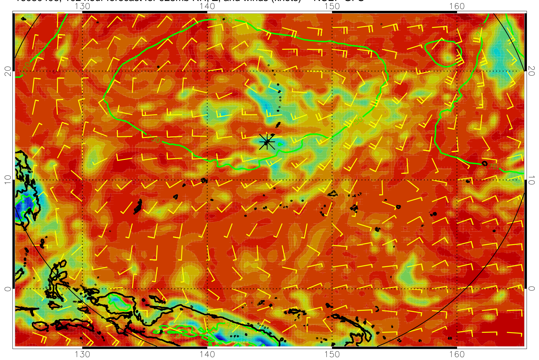
16080406, 102 hour forecast for 925mb RH, Z, and winds (knots) -- NCEP GFS
