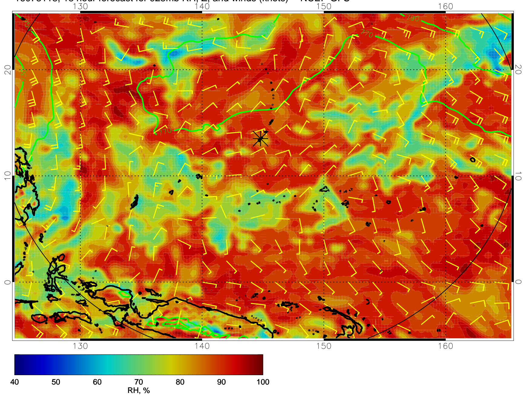
16073118, 18 hour forecast for 925mb RH, Z, and winds (knots) -- NCEP GFS
