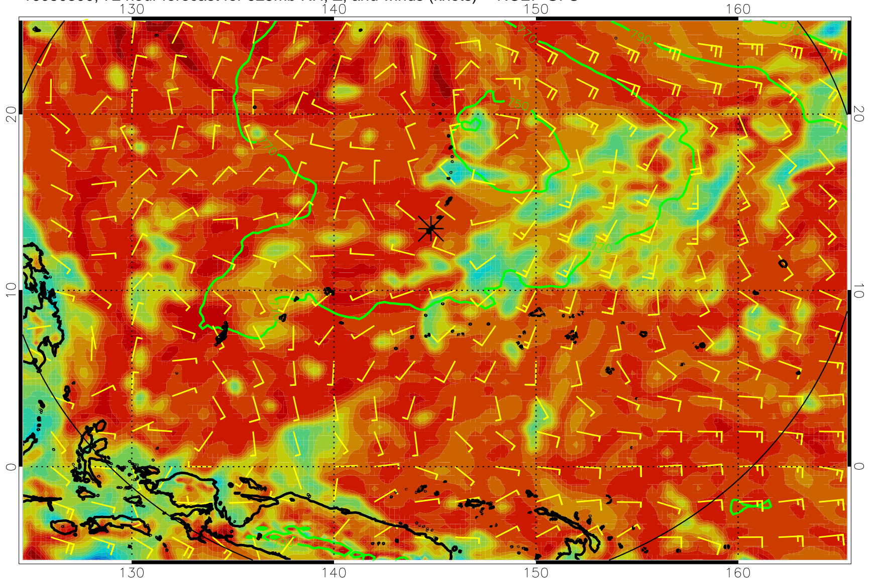
16080300, 72 hour forecast for 925mb RH, Z, and winds (knots) -- NCEP GFS
