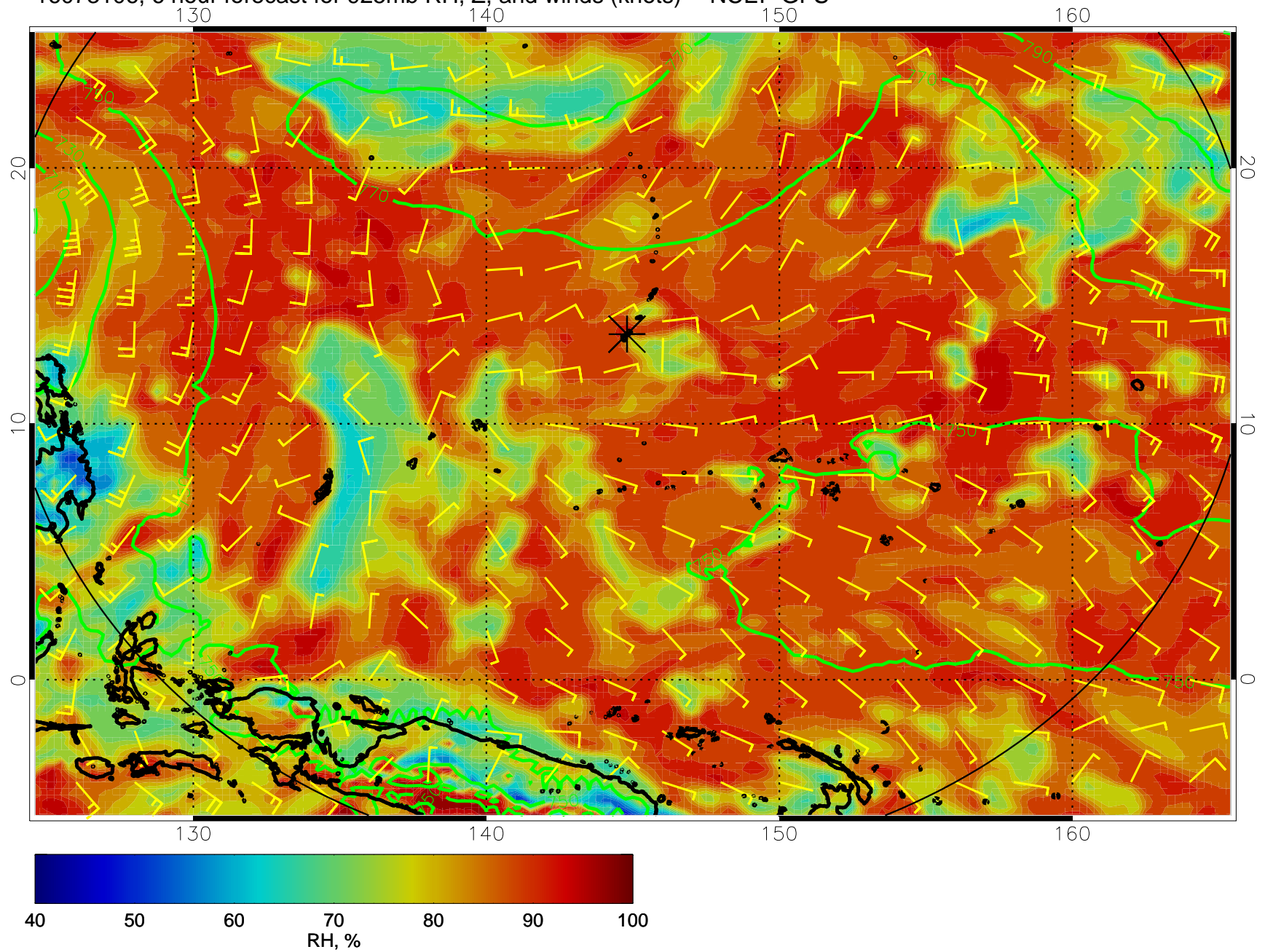
16073106, 6 hour forecast for 925mb RH, Z, and winds (knots) -- NCEP GFS
