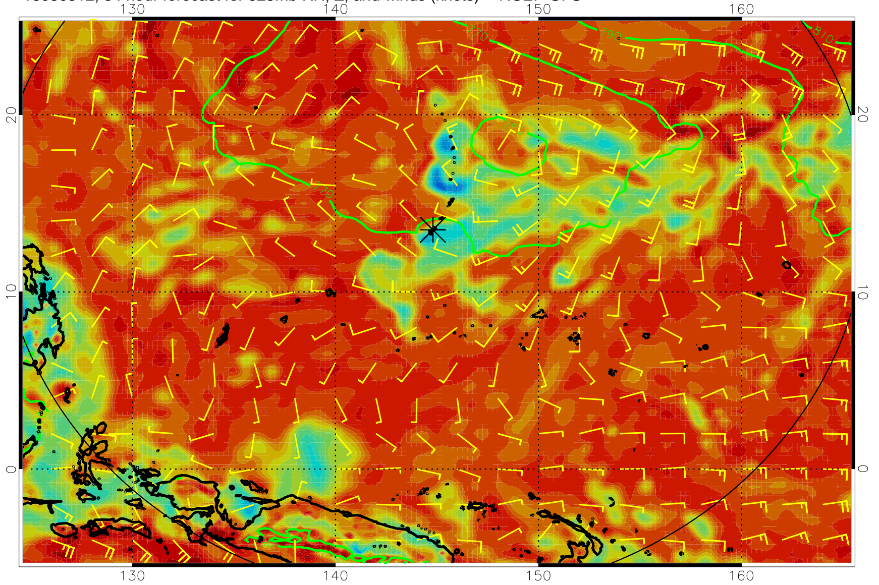
16080312, 84 hour forecast for 925mb RH, Z, and winds (knots) -- NCEP GFS
