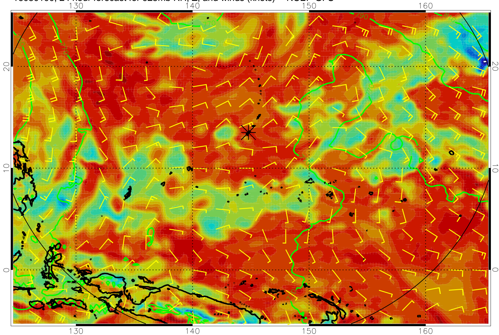
16080100, 24 hour forecast for 925mb RH, Z, and winds (knots) -- NCEP GFS
