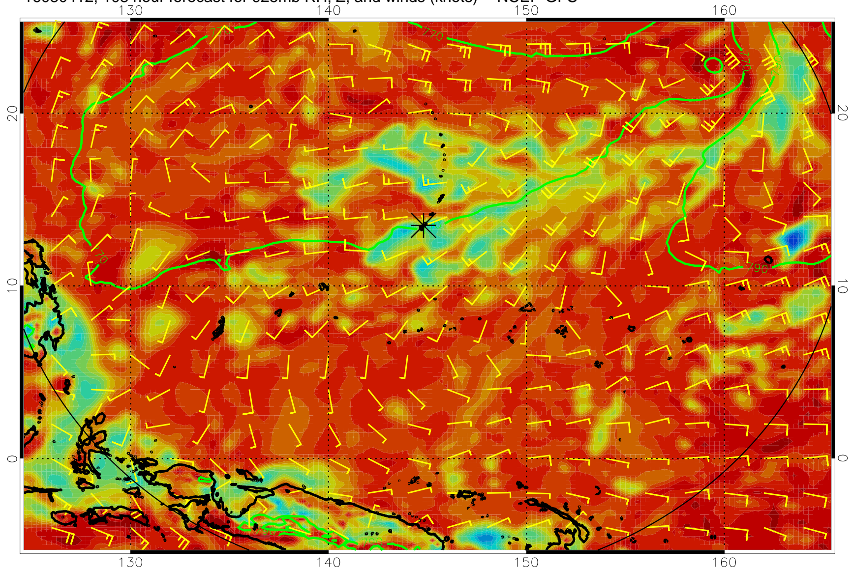
16080412, 108 hour forecast for 925mb RH, Z, and winds (knots) -- NCEP GFS
