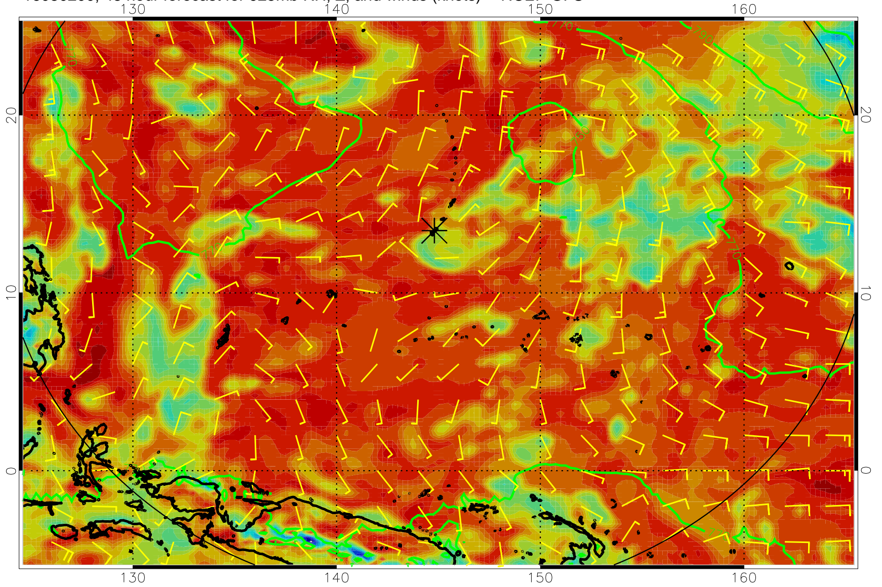
16080200, 48 hour forecast for 925mb RH, Z, and winds (knots) -- NCEP GFS
