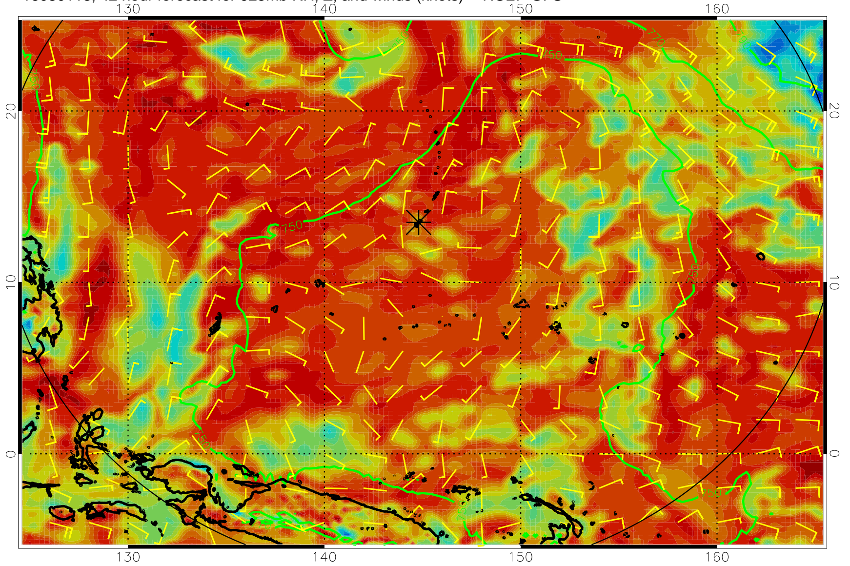
16080118, 42 hour forecast for 925mb RH, Z, and winds (knots) -- NCEP GFS
