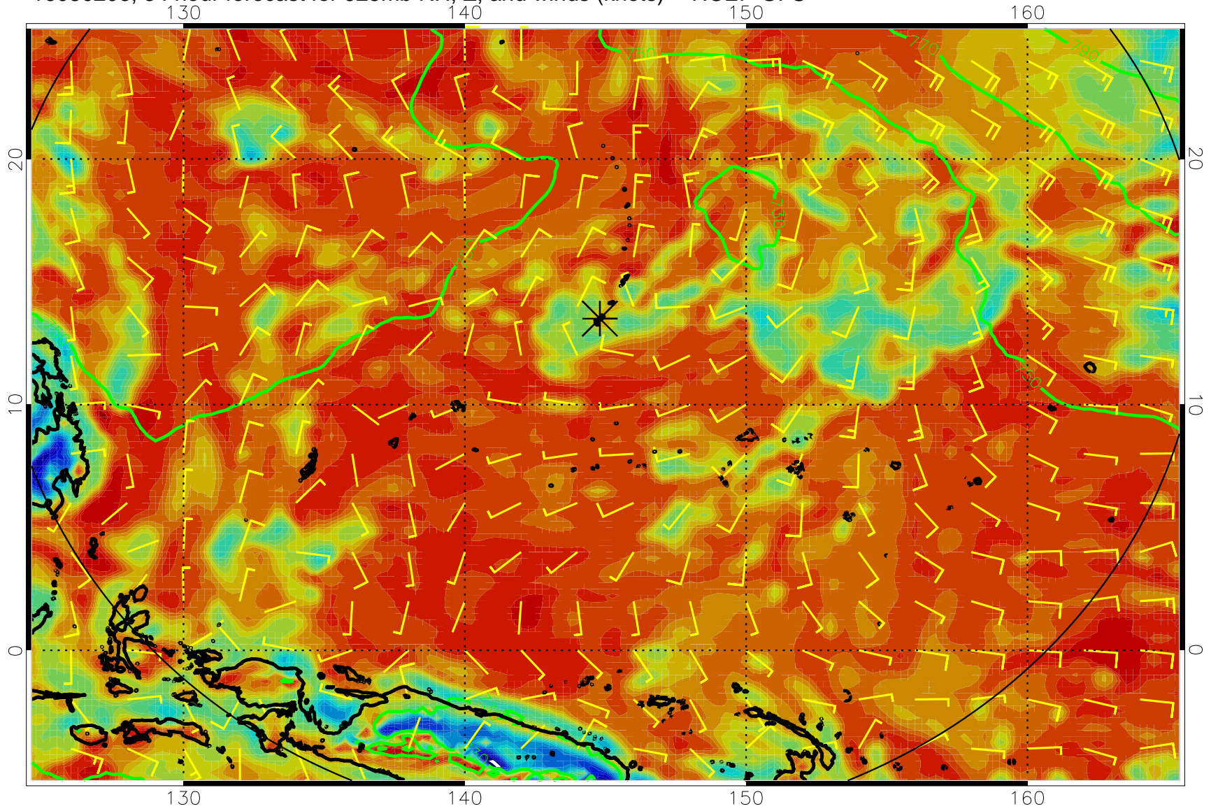
16080206, 54 hour forecast for 925mb RH, Z, and winds (knots) -- NCEP GFS
