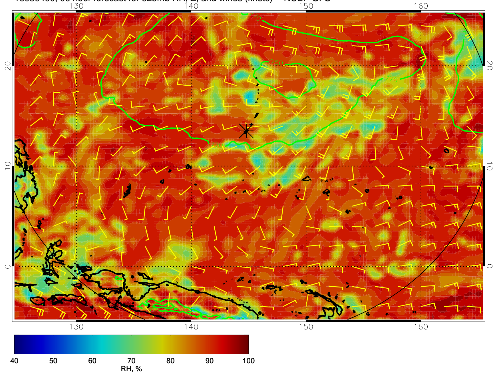
16080400, 96 hour forecast for 925mb RH, Z, and winds (knots) -- NCEP GFS
