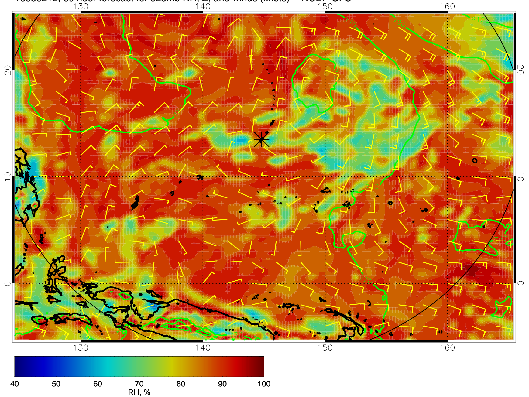
16080212, 60 hour forecast for 925mb RH, Z, and winds (knots) -- NCEP GFS
