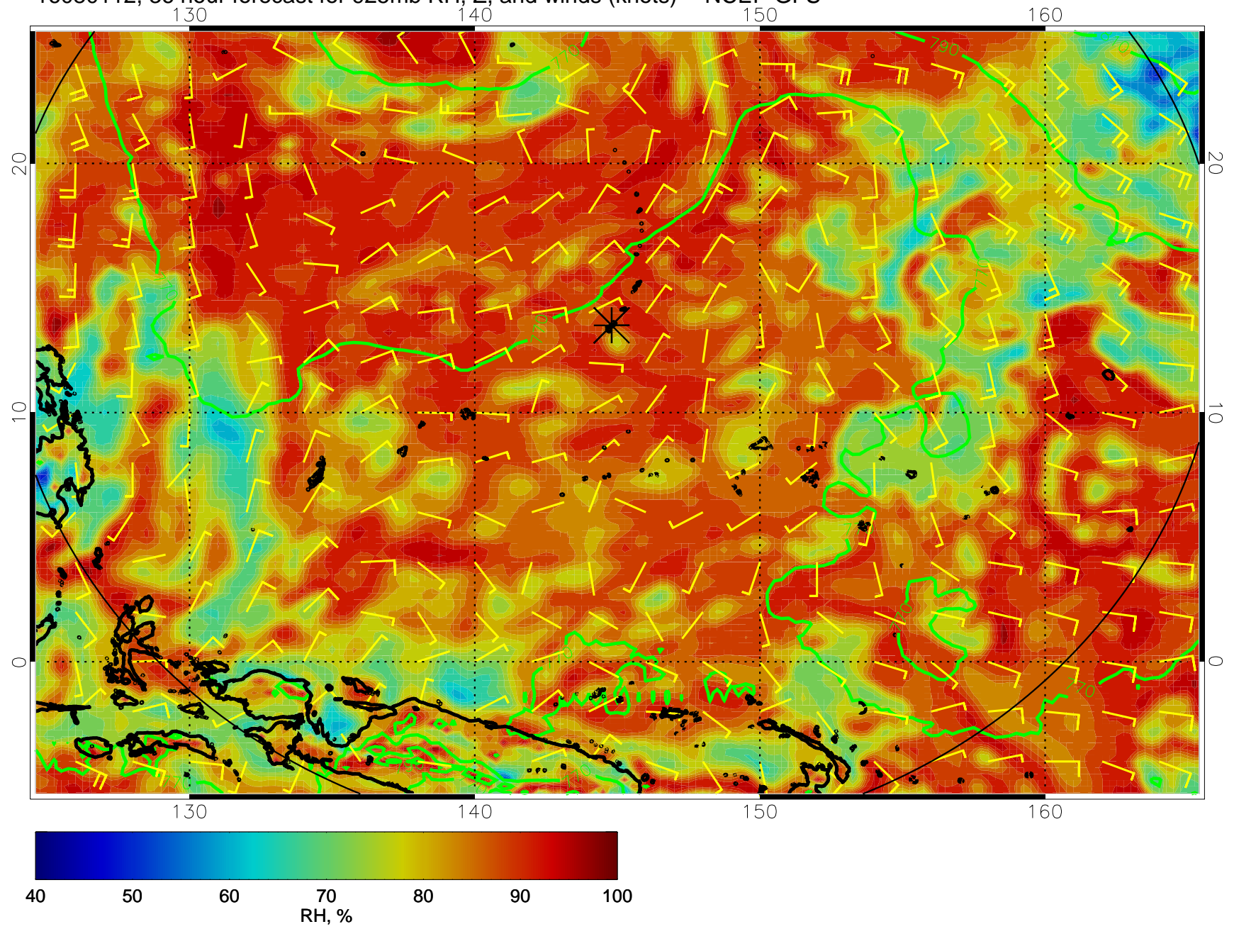
16080112, 36 hour forecast for 925mb RH, Z, and winds (knots) -- NCEP GFS
