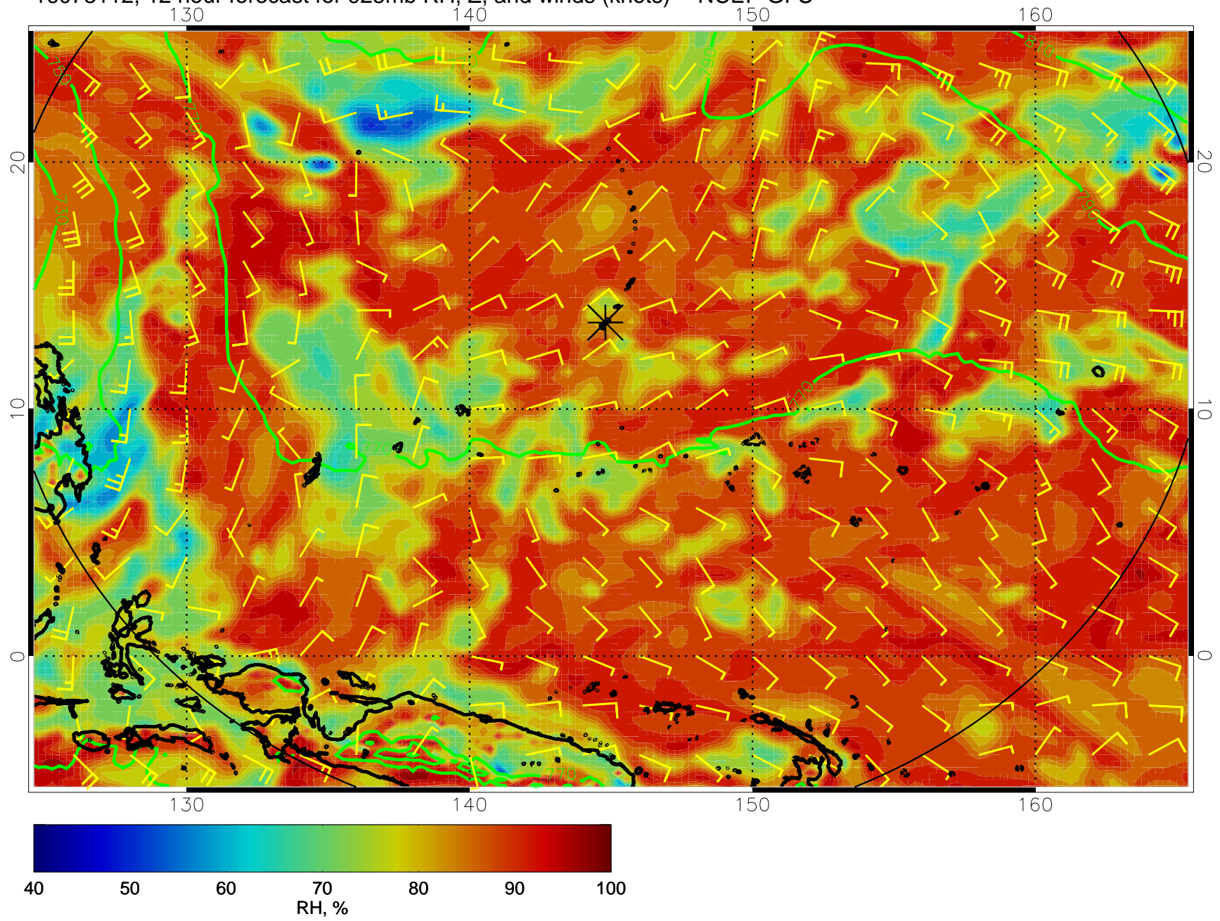
16073112, 12 hour forecast for 925mb RH, Z, and winds (knots) -- NCEP GFS
