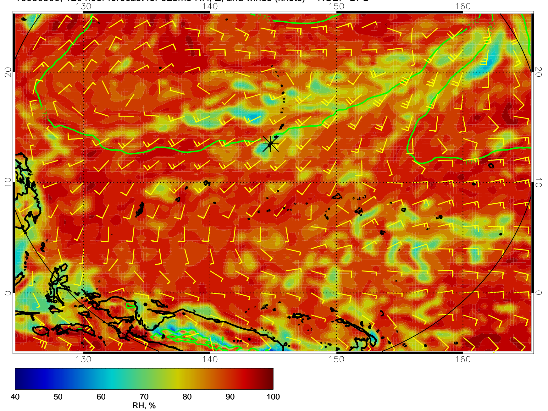
16080500, 120 hour forecast for 925mb RH, Z, and winds (knots) -- NCEP GFS
