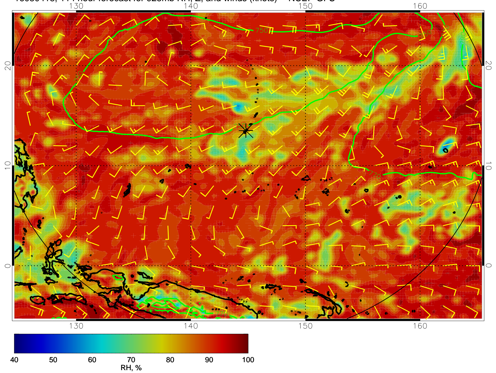
16080418, 114 hour forecast for 925mb RH, Z, and winds (knots) -- NCEP GFS
