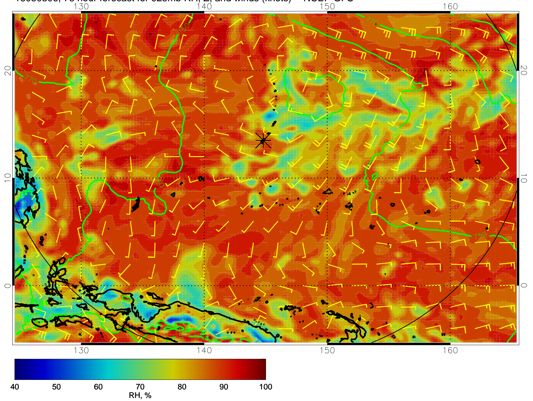
16080306, 78 hour forecast for 925mb RH, Z, and winds (knots) -- NCEP GFS
