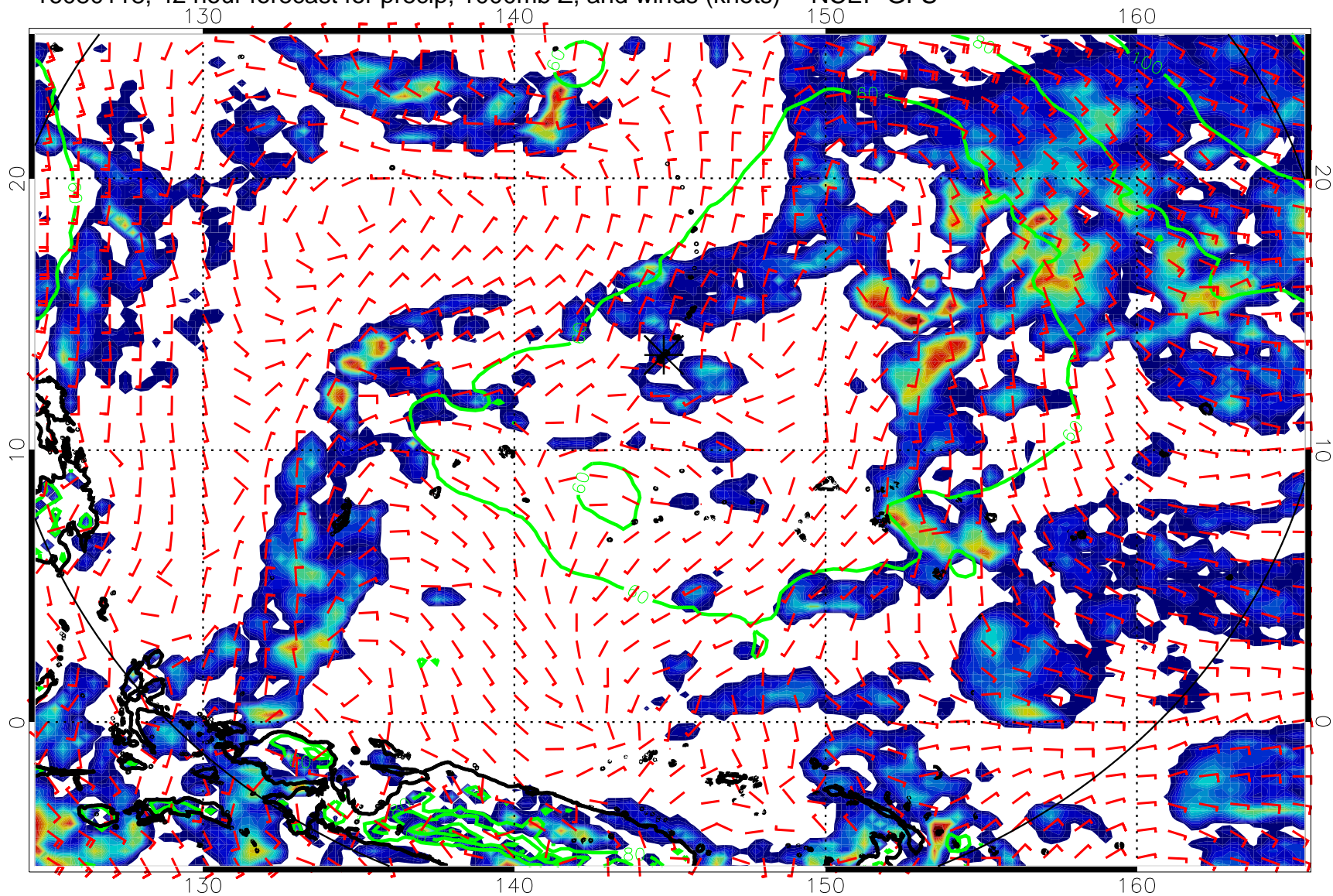
16080118, 42 hour forecast for precip, 1000mb Z, and winds (knots) -- NCEP GFS
