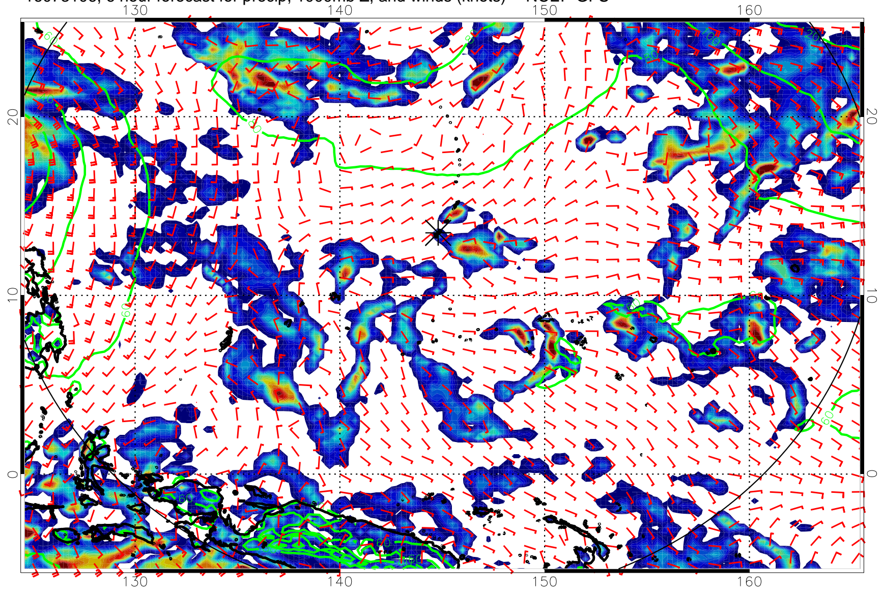
16073106, 6 hour forecast for precip, 1000mb Z, and winds (knots) -- NCEP GFS
