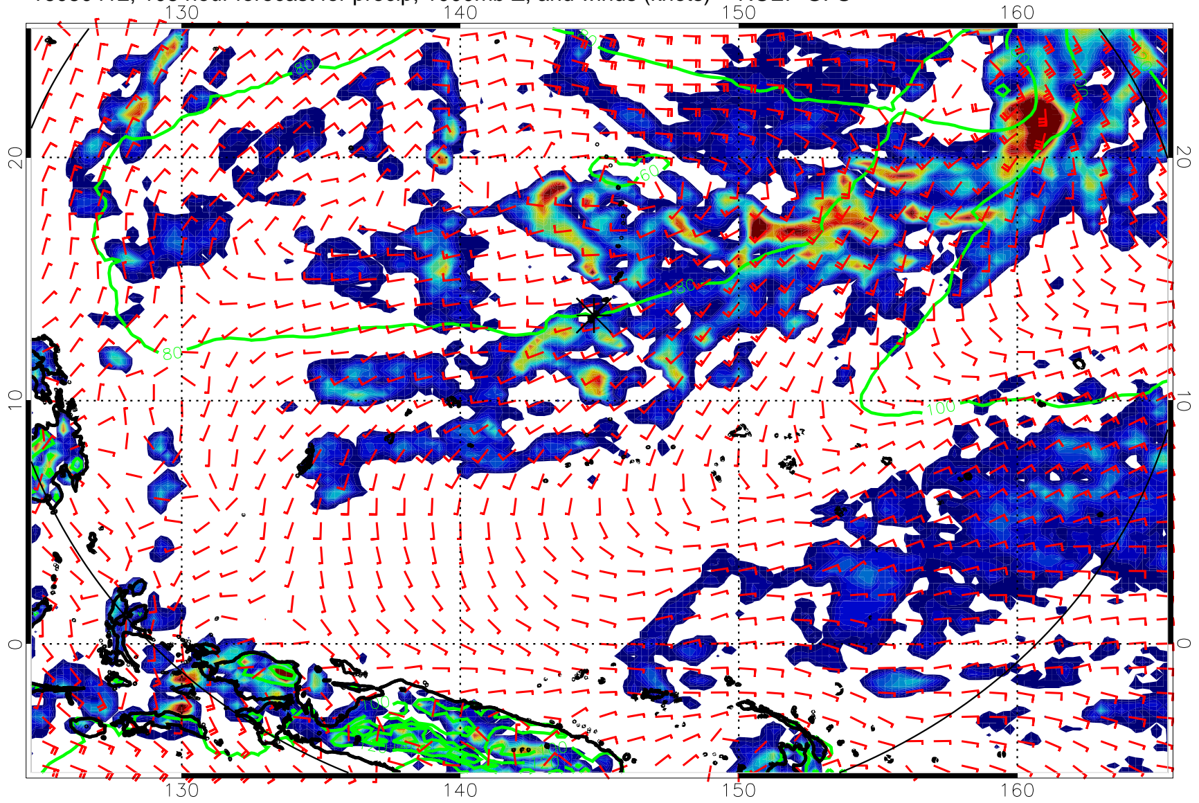
16080412, 108 hour forecast for precip, 1000mb Z, and winds (knots) -- NCEP GFS
