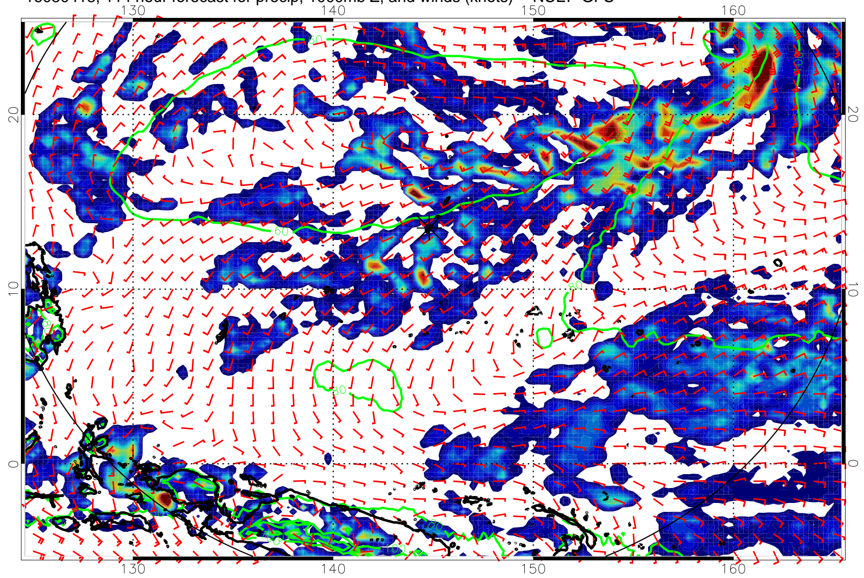
16080418, 114 hour forecast for precip, 1000mb Z, and winds (knots) -- NCEP GFS
