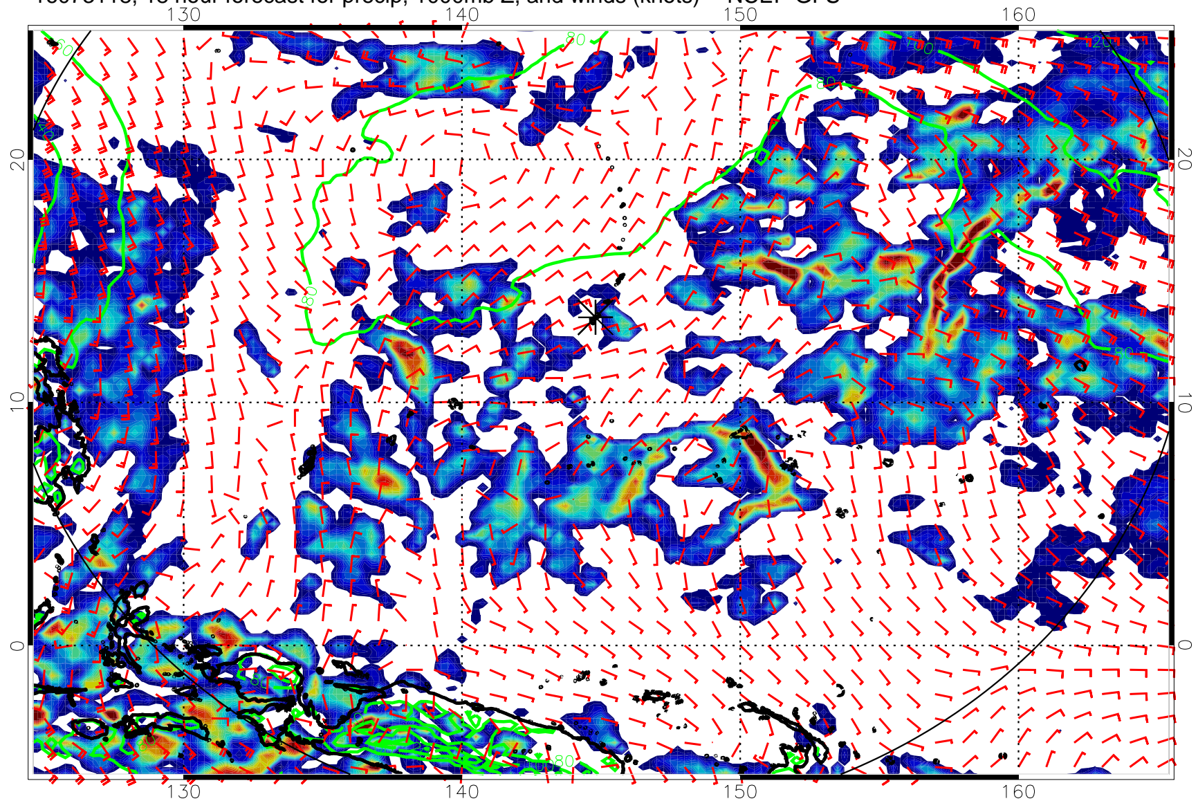
16073118, 18 hour forecast for precip, 1000mb Z, and winds (knots) -- NCEP GFS
