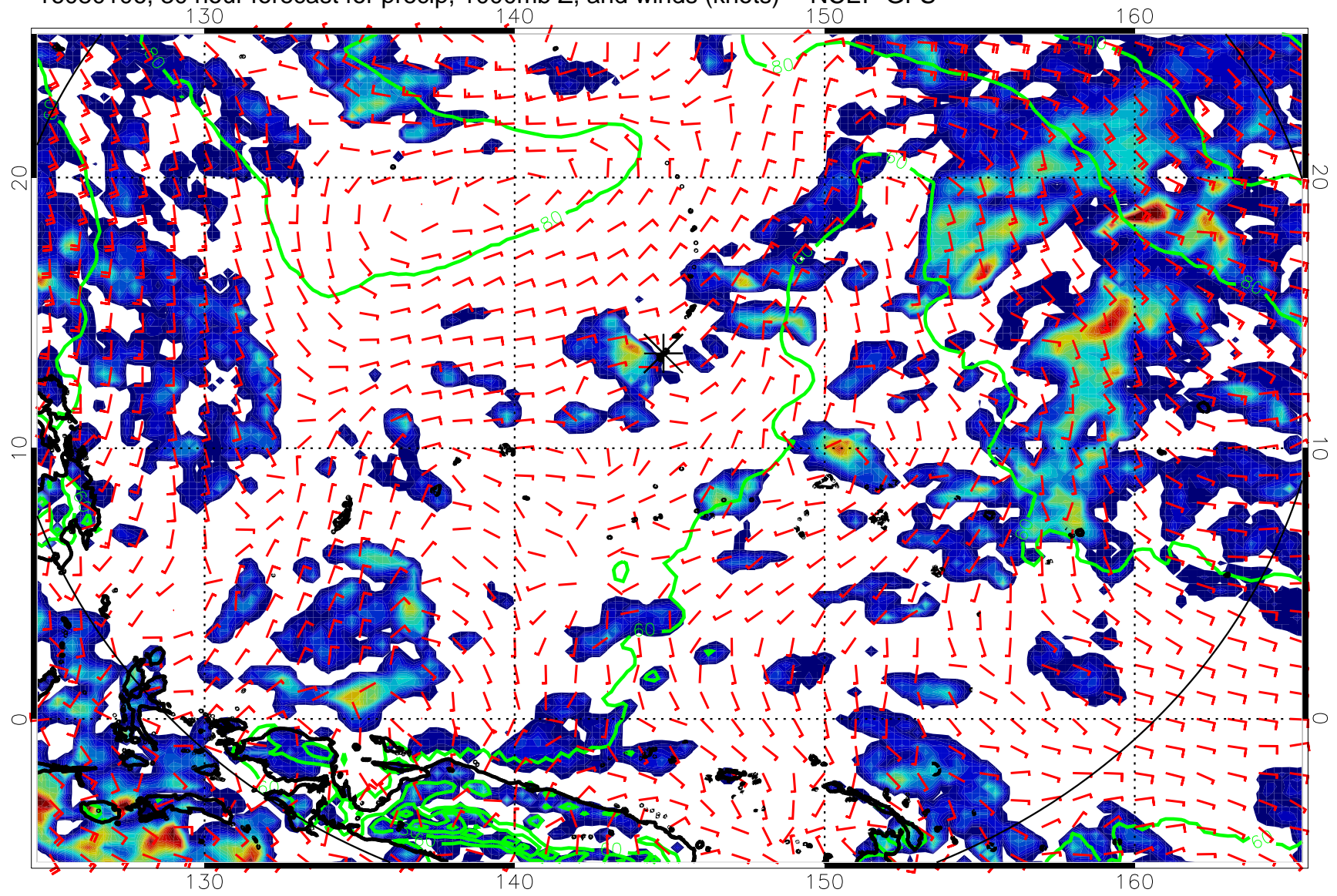
16080106, 30 hour forecast for precip, 1000mb Z, and winds (knots) -- NCEP GFS
