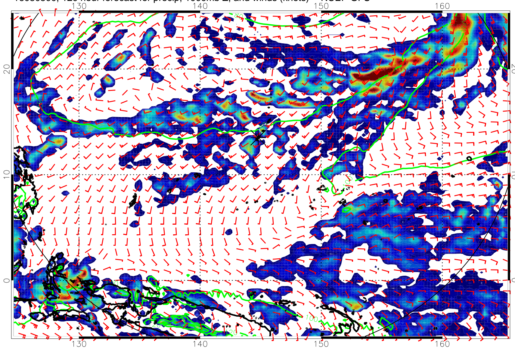
16080500, 120 hour forecast for precip, 1000mb Z, and winds (knots) -- NCEP GFS
