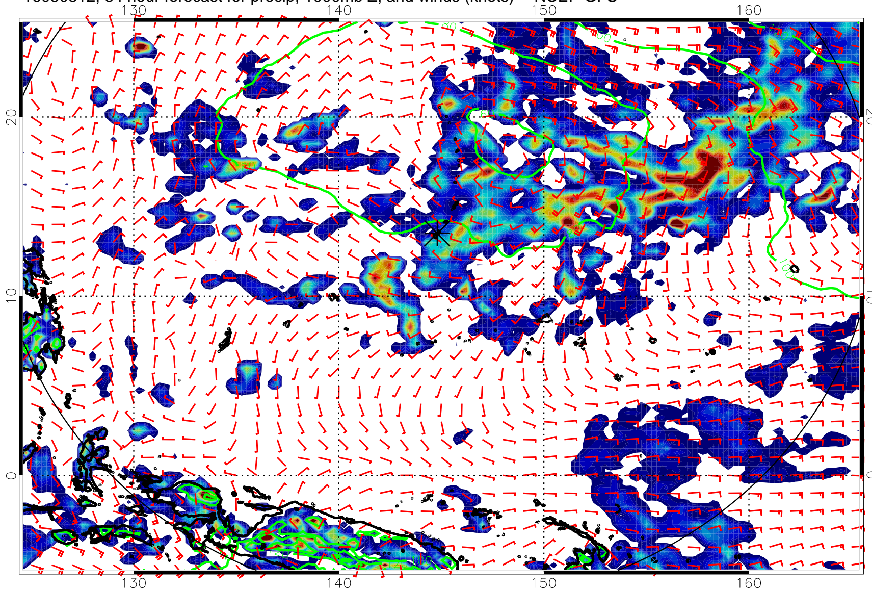
16080312, 84 hour forecast for precip, 1000mb Z, and winds (knots) -- NCEP GFS
