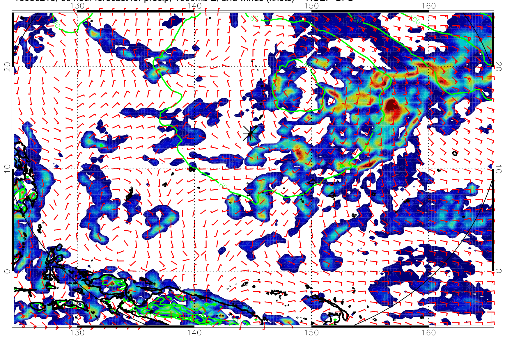
16080218, 66 hour forecast for precip, 1000mb Z, and winds (knots) -- NCEP GFS
