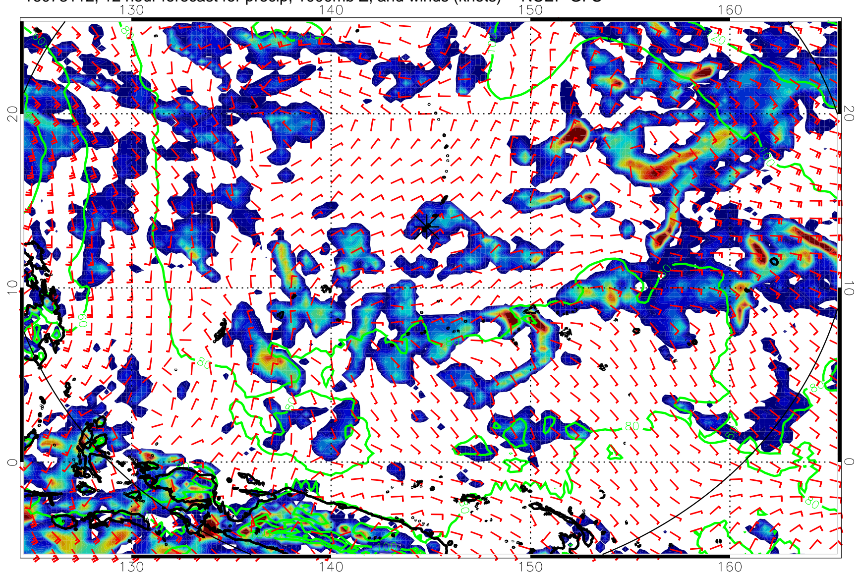
16073112, 12 hour forecast for precip, 1000mb Z, and winds (knots) -- NCEP GFS
