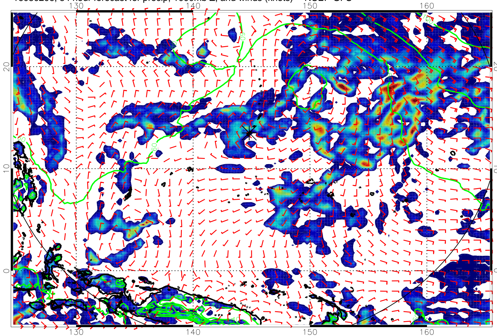
16080206, 54 hour forecast for precip, 1000mb Z, and winds (knots) -- NCEP GFS
