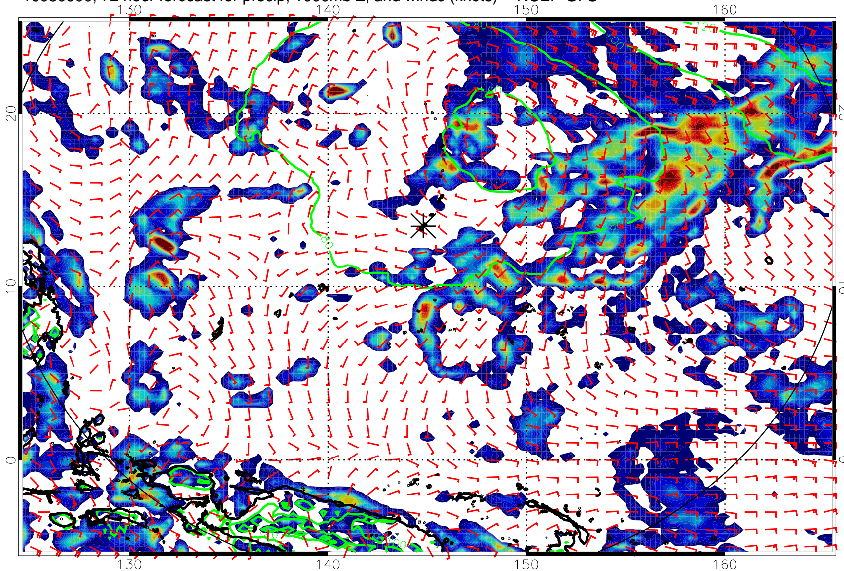
16080300, 72 hour forecast for precip, 1000mb Z, and winds (knots) -- NCEP GFS
