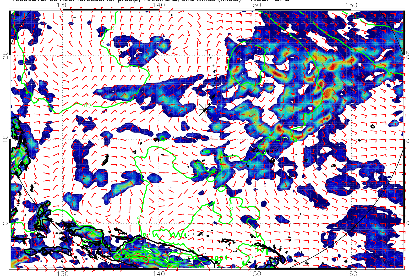
16080212, 60 hour forecast for precip, 1000mb Z, and winds (knots) -- NCEP GFS
