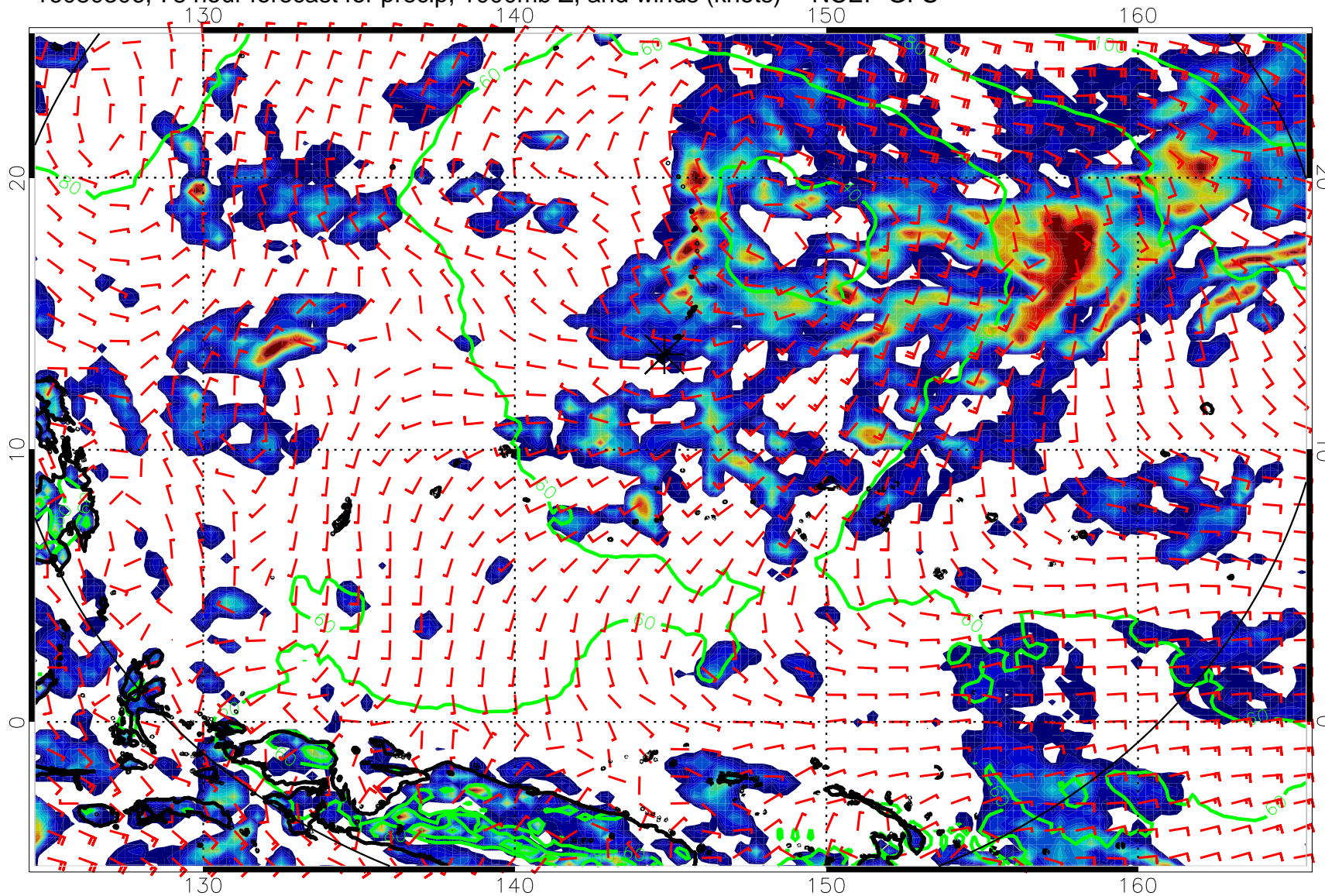
16080306, 78 hour forecast for precip, 1000mb Z, and winds (knots) -- NCEP GFS
