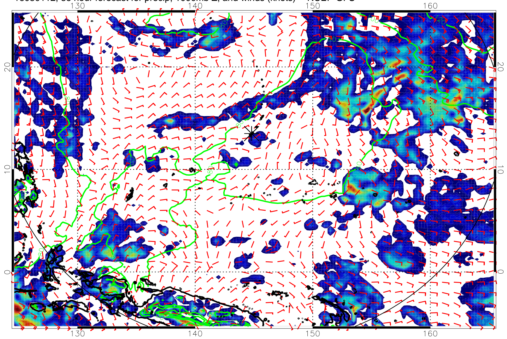
16080112, 36 hour forecast for precip, 1000mb Z, and winds (knots) -- NCEP GFS
