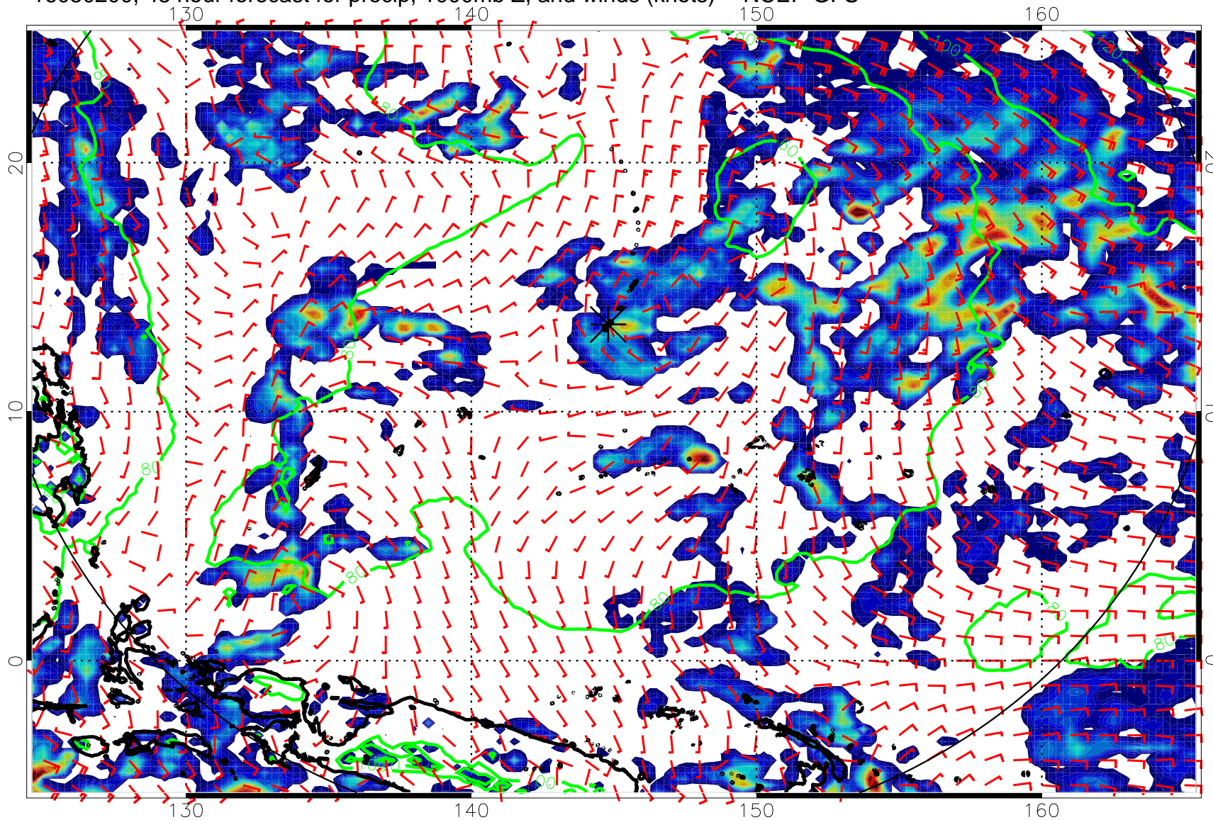
16080200, 48 hour forecast for precip, 1000mb Z, and winds (knots) -- NCEP GFS
