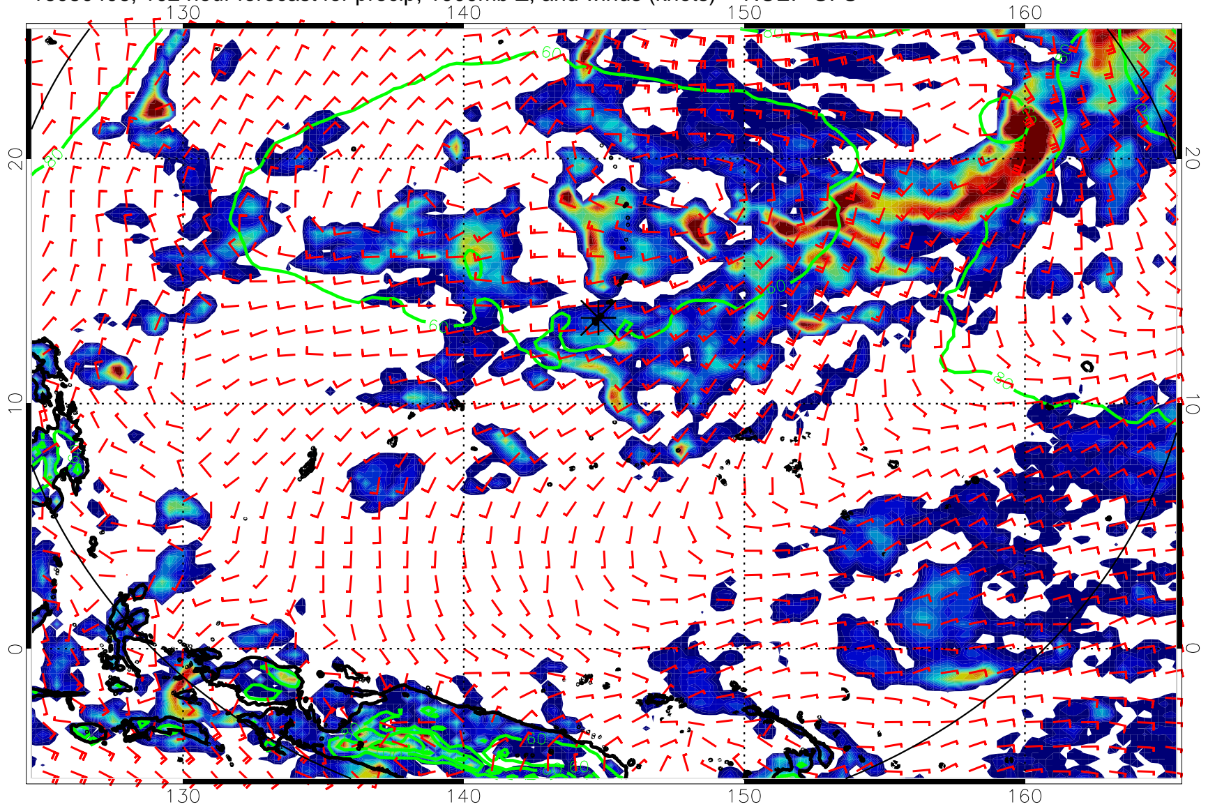
16080406, 102 hour forecast for precip, 1000mb Z, and winds (knots) -- NCEP GFS
