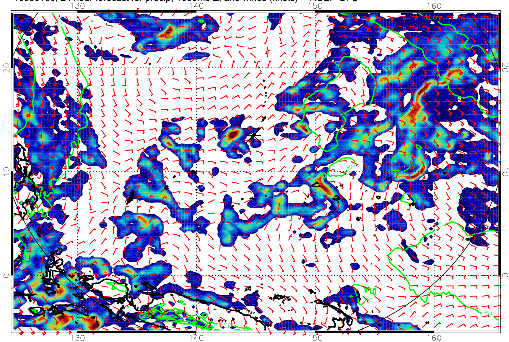
16080100, 24 hour forecast for precip, 1000mb Z, and winds (knots) -- NCEP GFS
