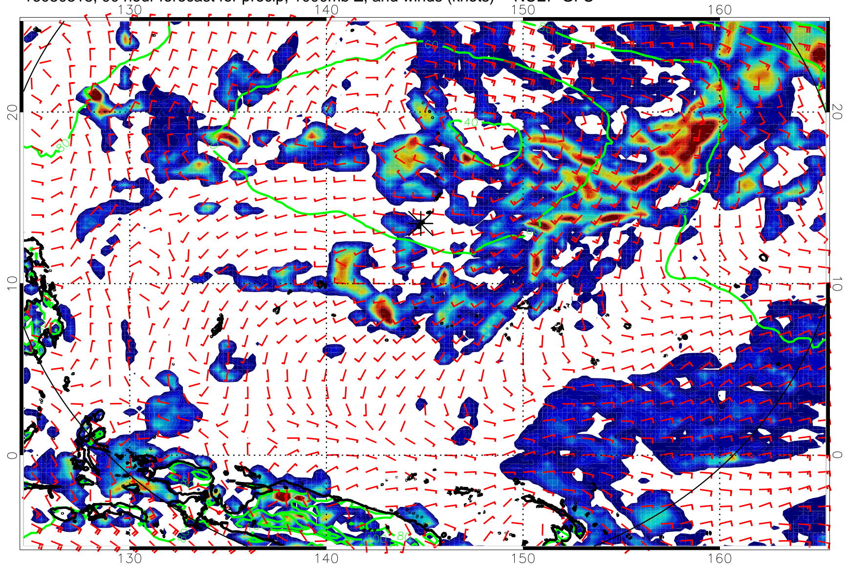
16080318, 90 hour forecast for precip, 1000mb Z, and winds (knots) -- NCEP GFS
