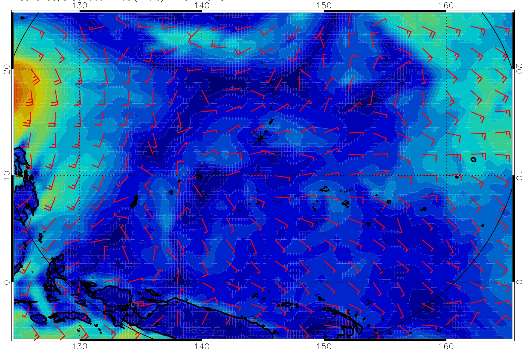
16073106, 6 Surface winds (knots) -- NCEP GFS
