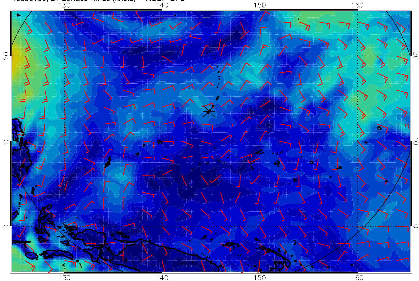
16080100, 24 Surface winds (knots) -- NCEP GFS
