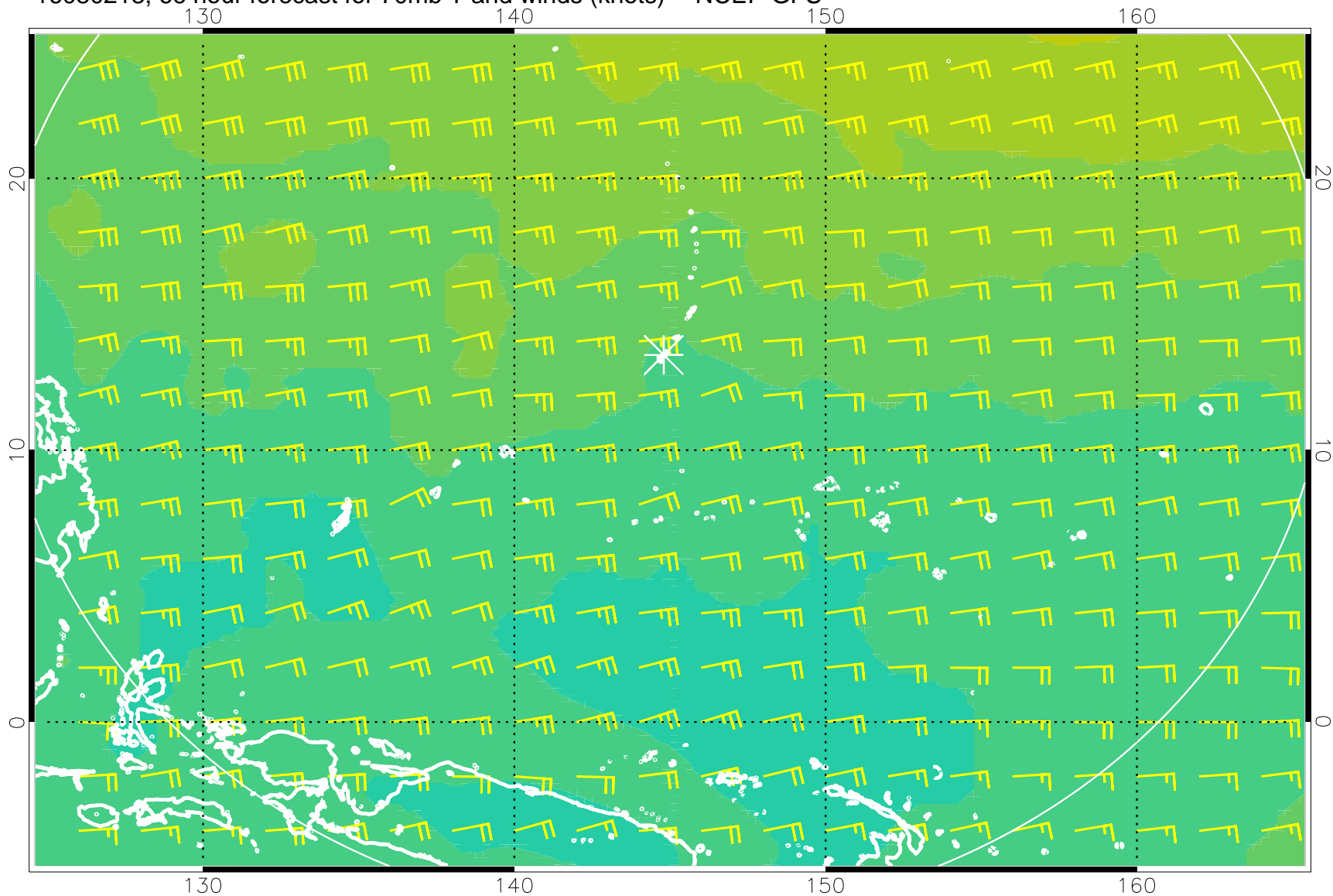
16080218, 66 hour forecast for 70mb T and winds (knots) -- NCEP GFS
