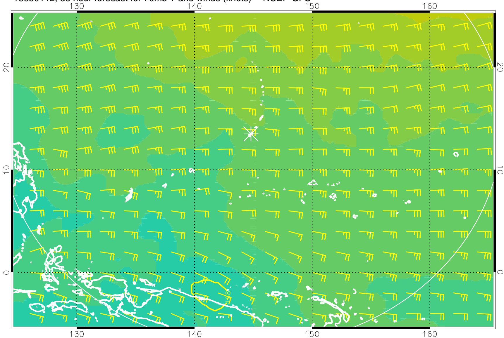
16080112, 36 hour forecast for 70mb T and winds (knots) -- NCEP GFS
