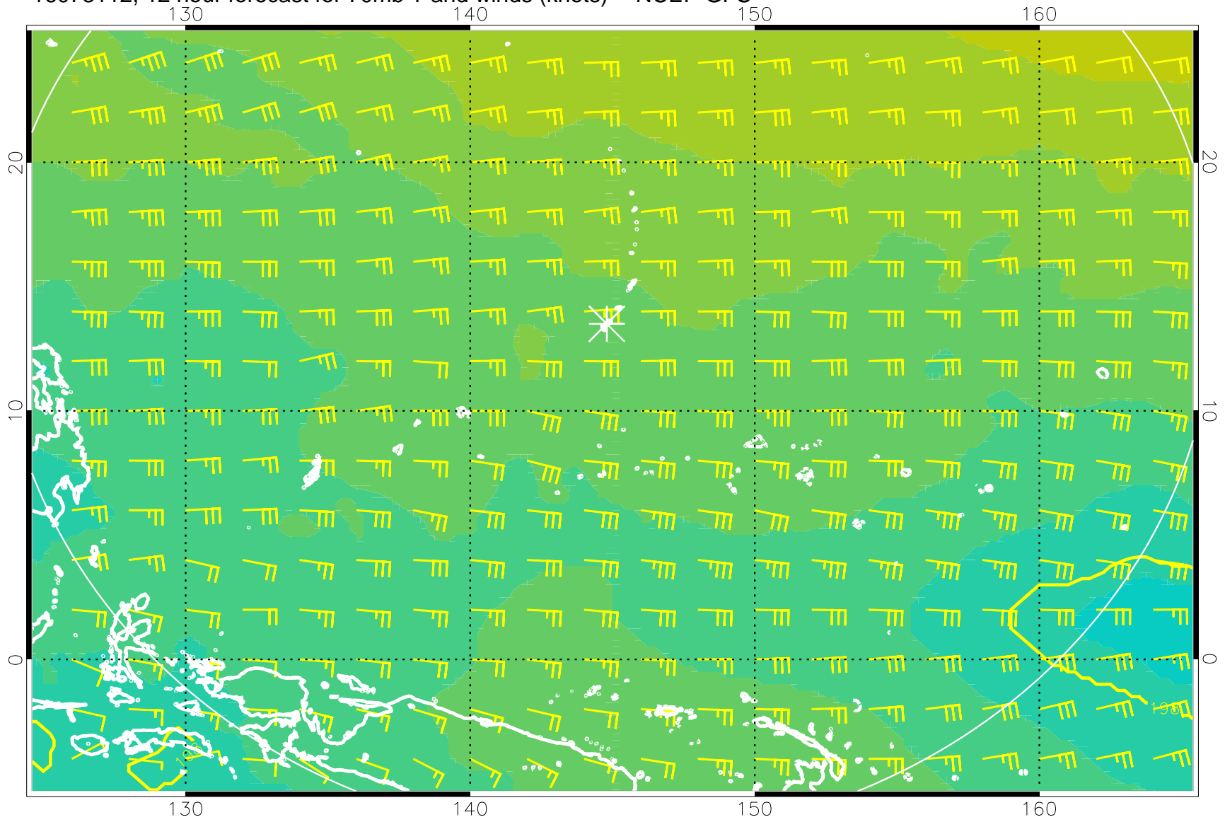
16073112, 12 hour forecast for 70mb T and winds (knots) -- NCEP GFS
