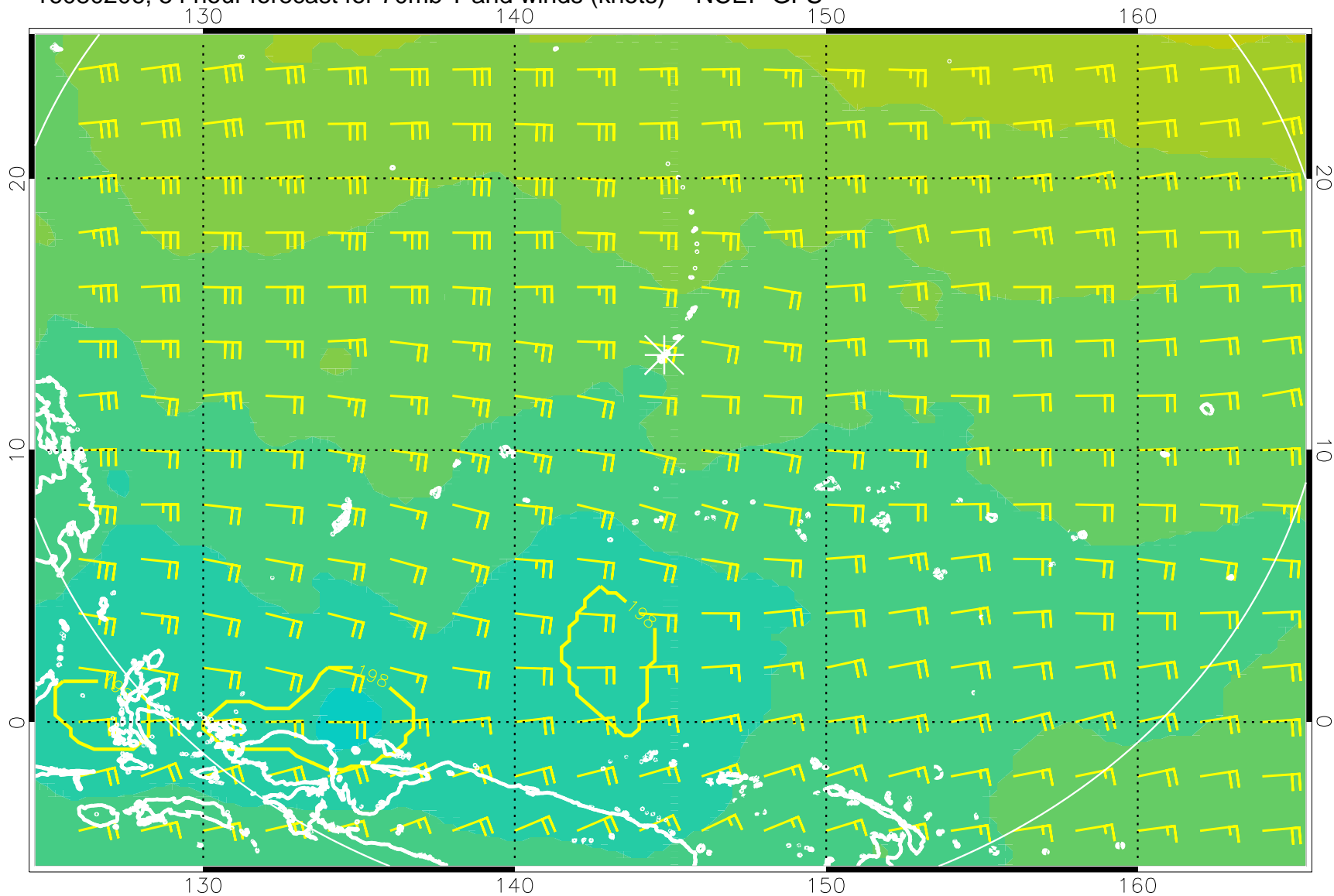
16080206, 54 hour forecast for 70mb T and winds (knots) -- NCEP GFS
