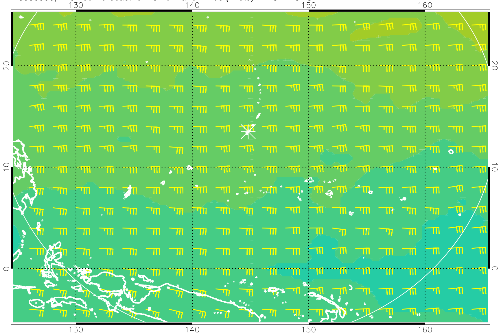
16080500, 120 hour forecast for 70mb T and winds (knots) -- NCEP GFS
