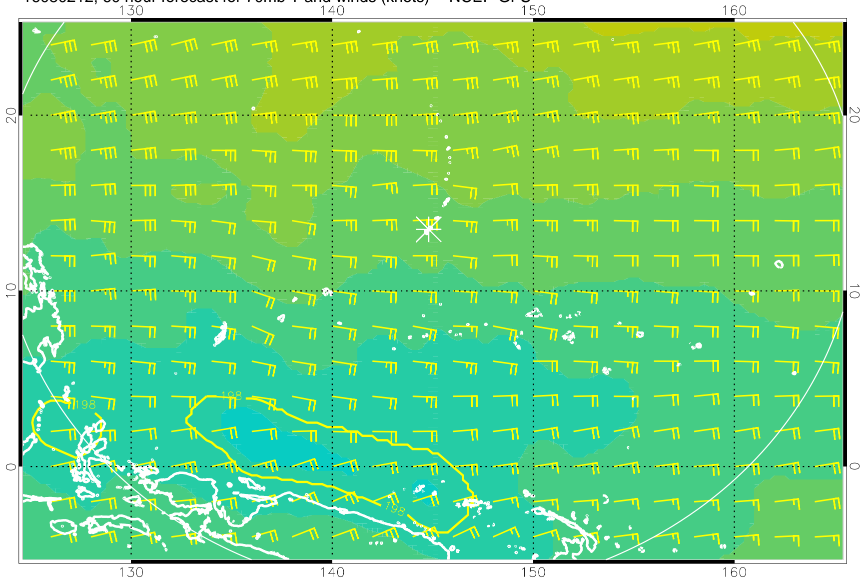
16080212, 60 hour forecast for 70mb T and winds (knots) -- NCEP GFS
