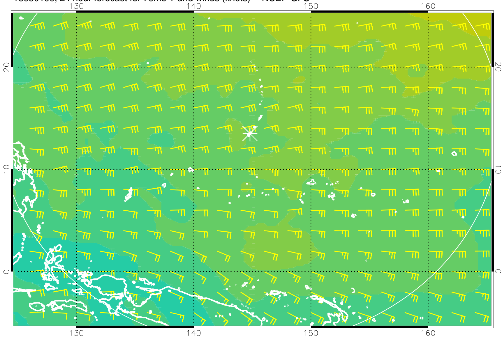
16080100, 24 hour forecast for 70mb T and winds (knots) -- NCEP GFS
