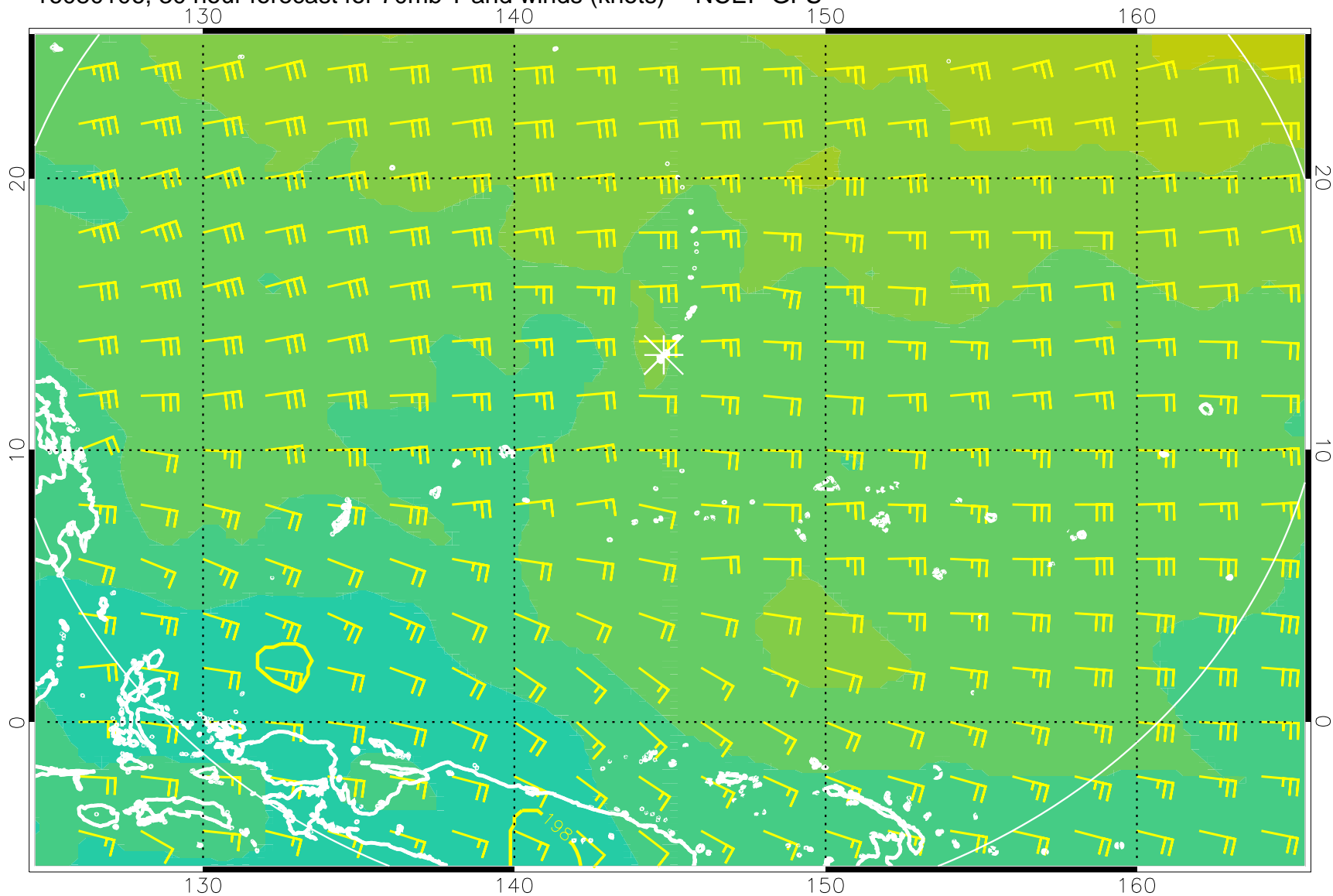
16080106, 30 hour forecast for 70mb T and winds (knots) -- NCEP GFS
