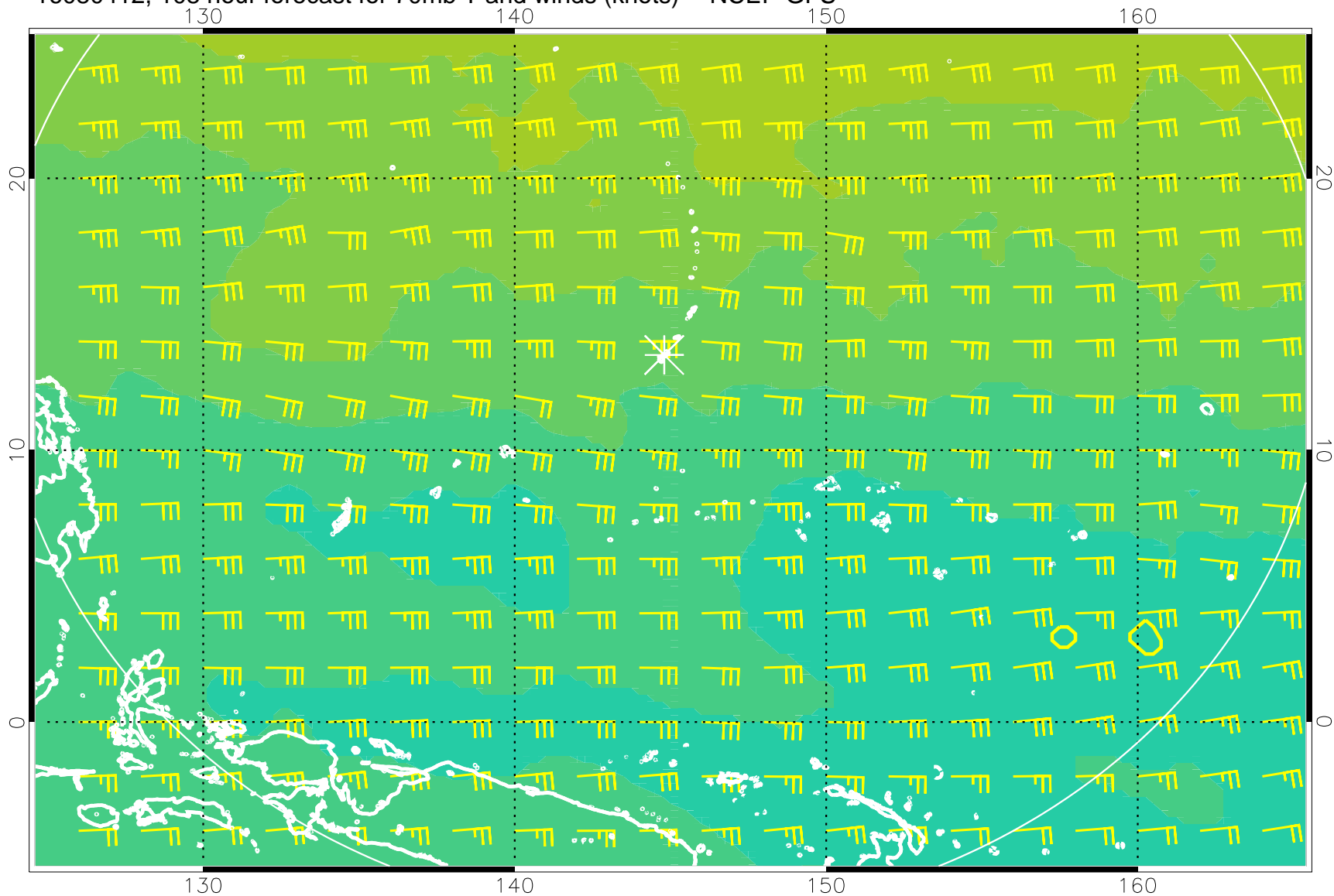
16080412, 108 hour forecast for 70mb T and winds (knots) -- NCEP GFS
