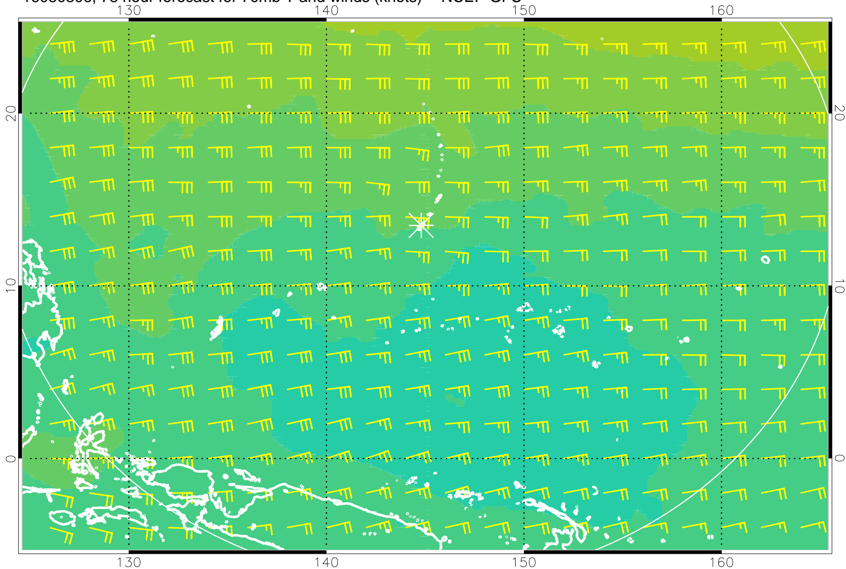
16080306, 78 hour forecast for 70mb T and winds (knots) -- NCEP GFS
