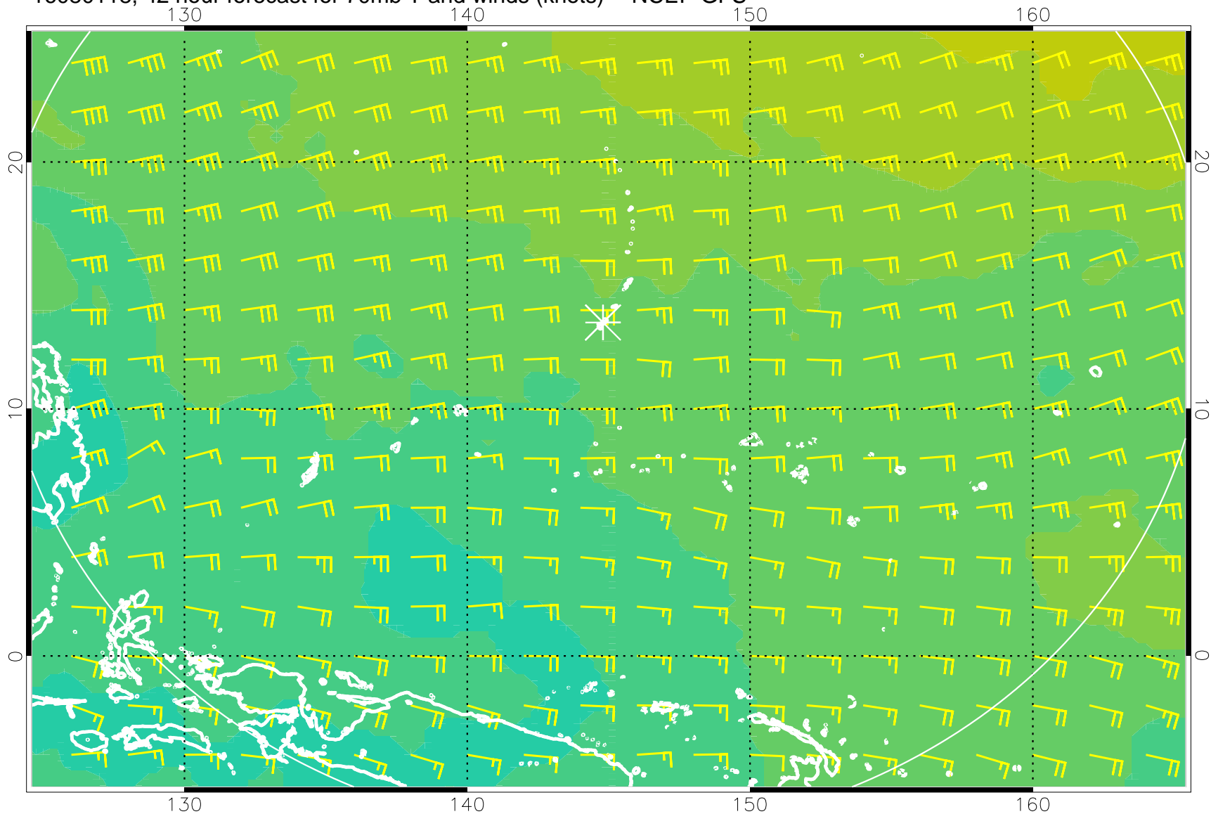
16080118, 42 hour forecast for 70mb T and winds (knots) -- NCEP GFS
