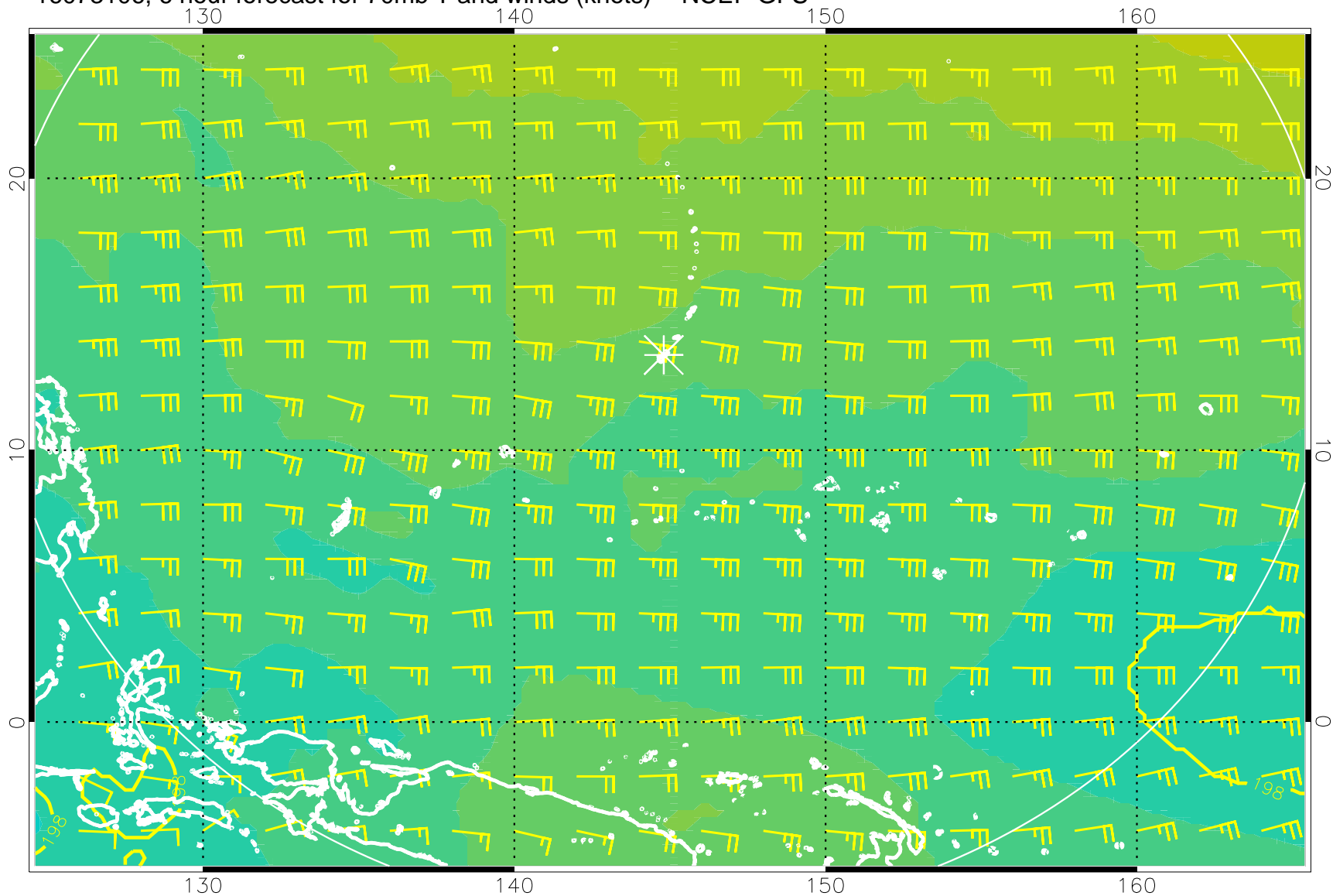
16073106, 6 hour forecast for 70mb T and winds (knots) -- NCEP GFS
