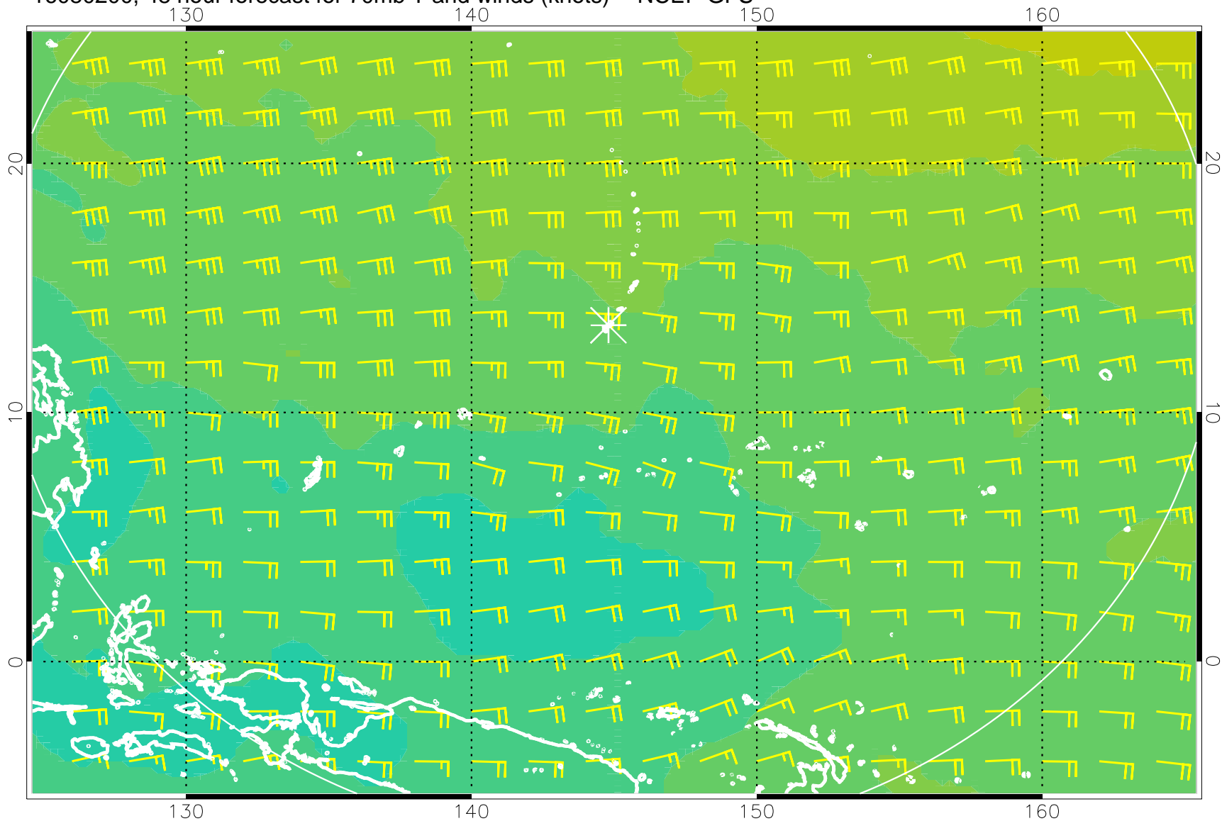
16080200, 48 hour forecast for 70mb T and winds (knots) -- NCEP GFS
