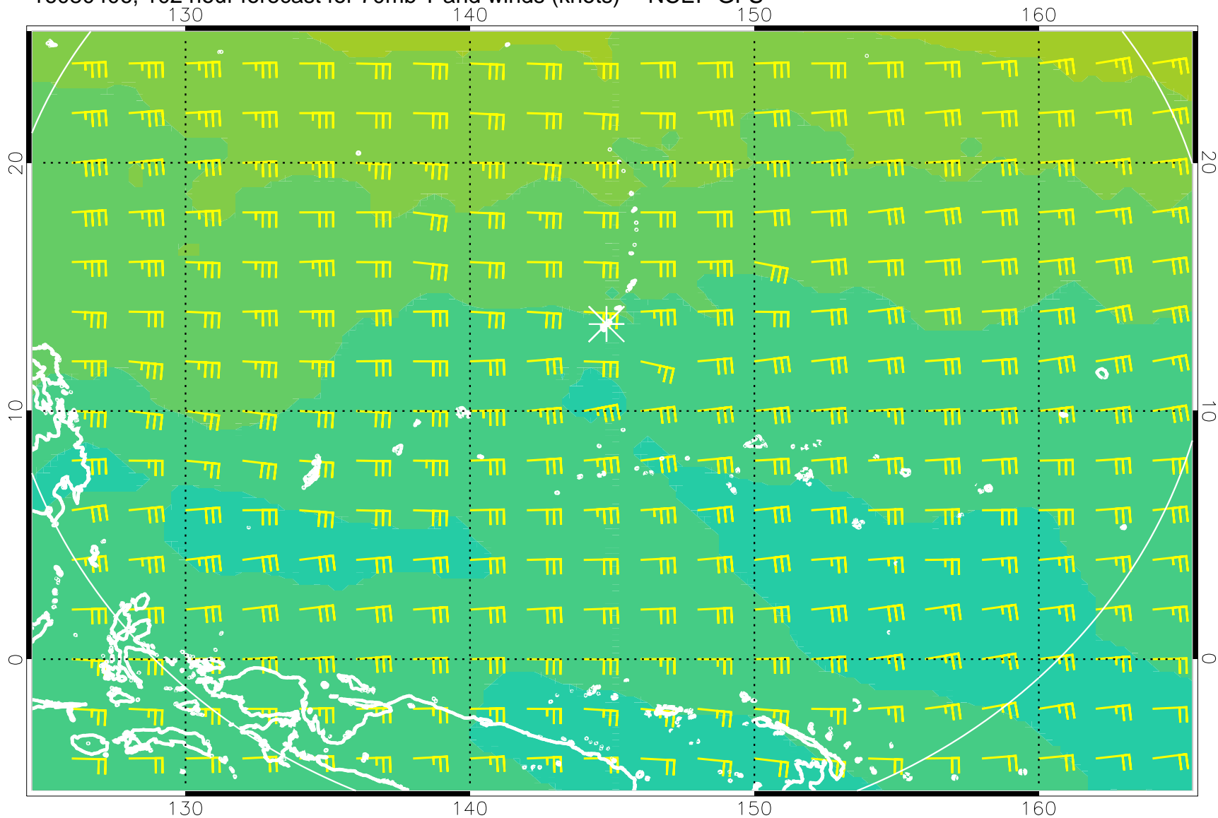
16080406, 102 hour forecast for 70mb T and winds (knots) -- NCEP GFS
