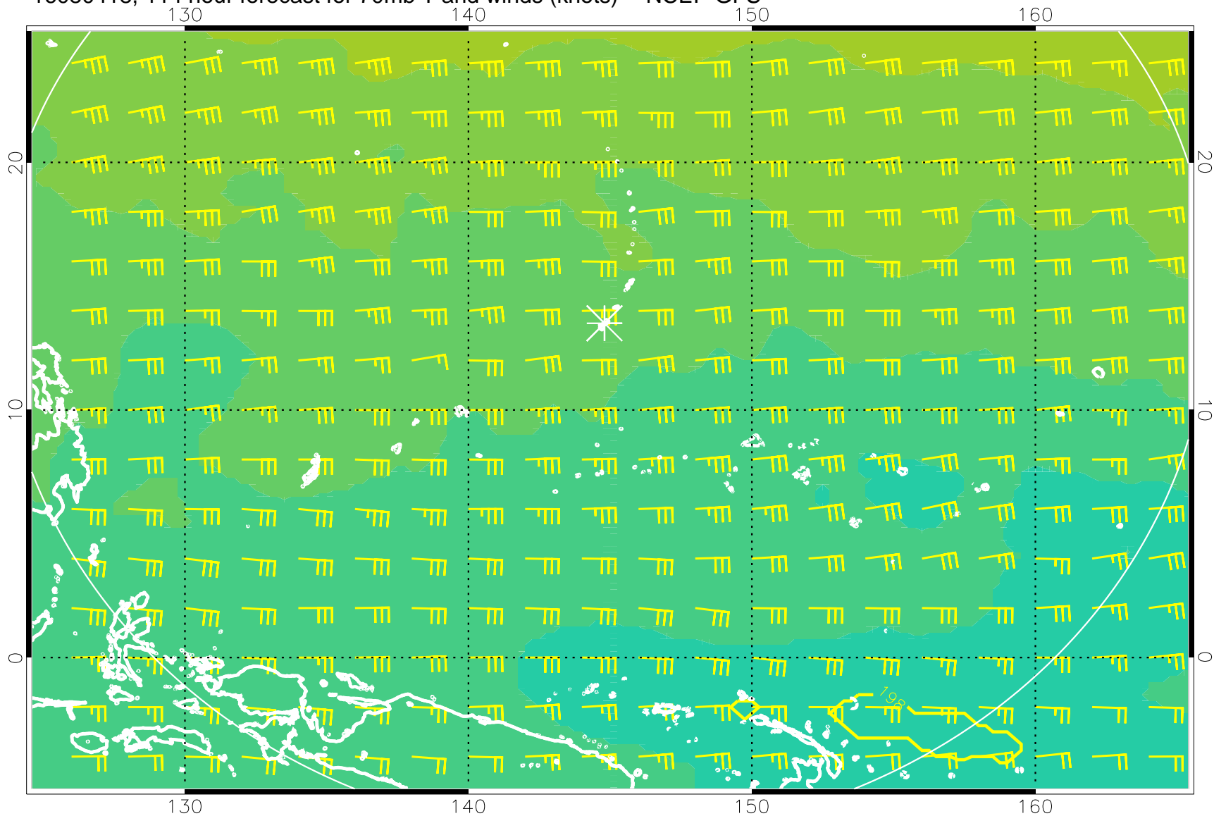
16080418, 114 hour forecast for 70mb T and winds (knots) -- NCEP GFS
