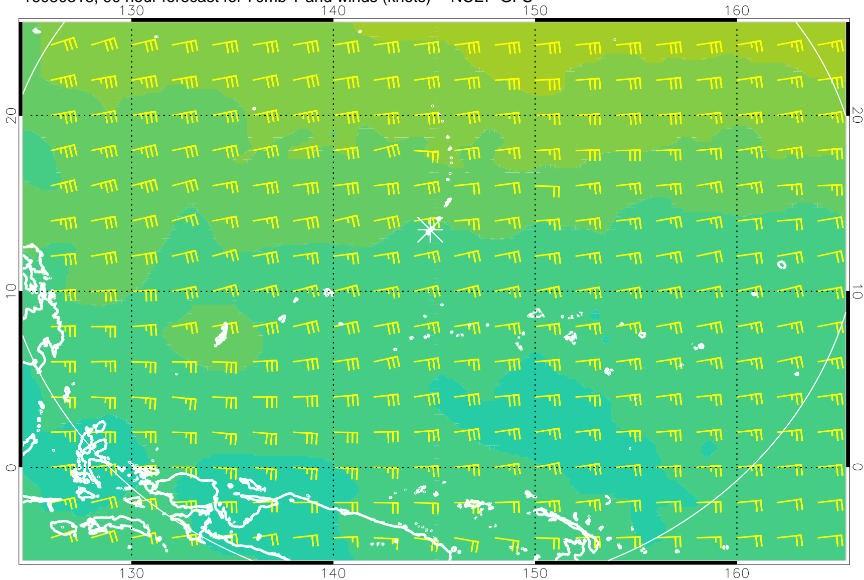
16080318, 90 hour forecast for 70mb T and winds (knots) -- NCEP GFS
