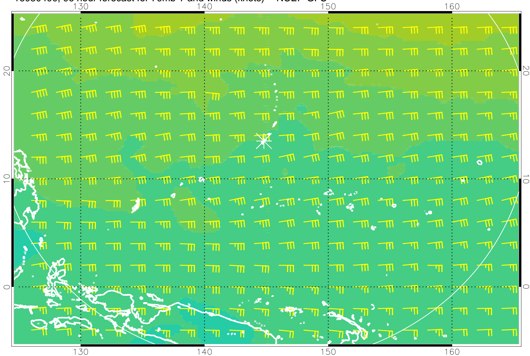
16080400, 96 hour forecast for 70mb T and winds (knots) -- NCEP GFS
