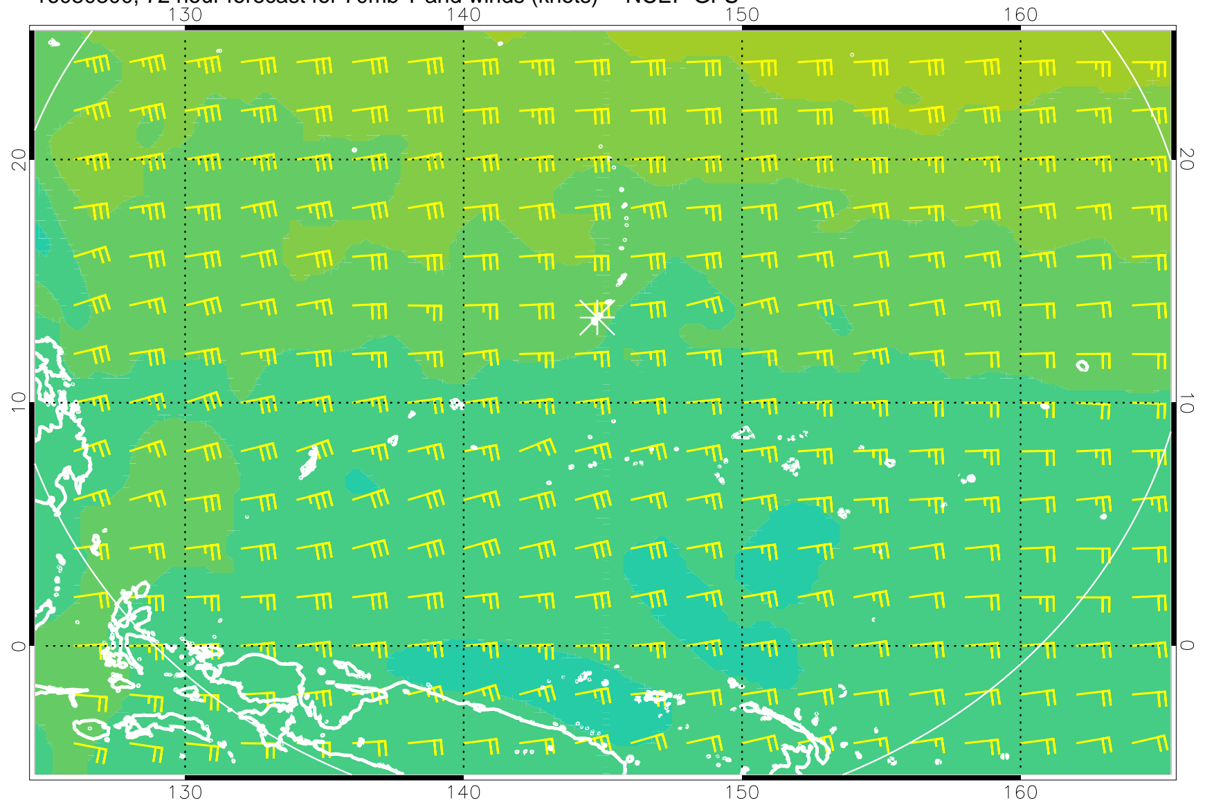
16080300, 72 hour forecast for 70mb T and winds (knots) -- NCEP GFS
