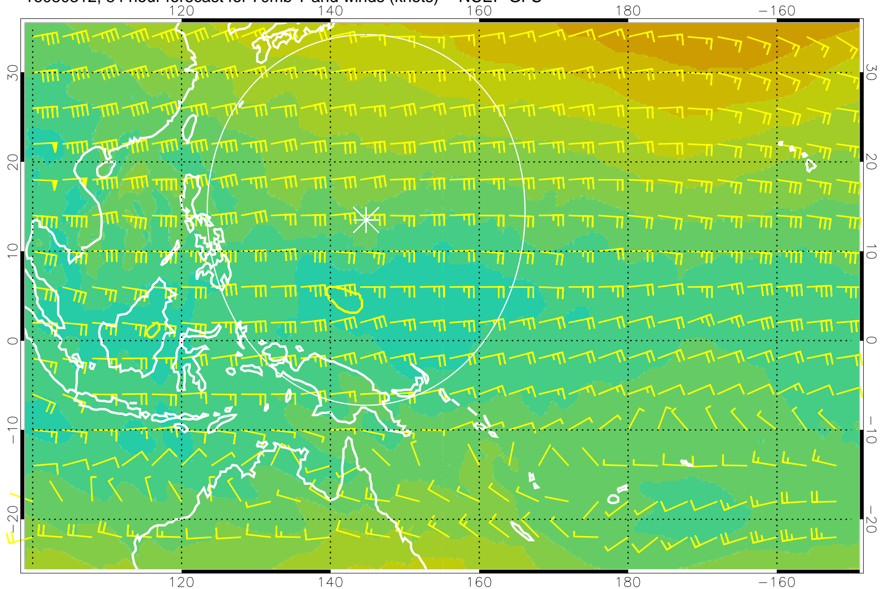
16080312, 84 hour forecast for 70mb T and winds (knots) -- NCEP GFS
