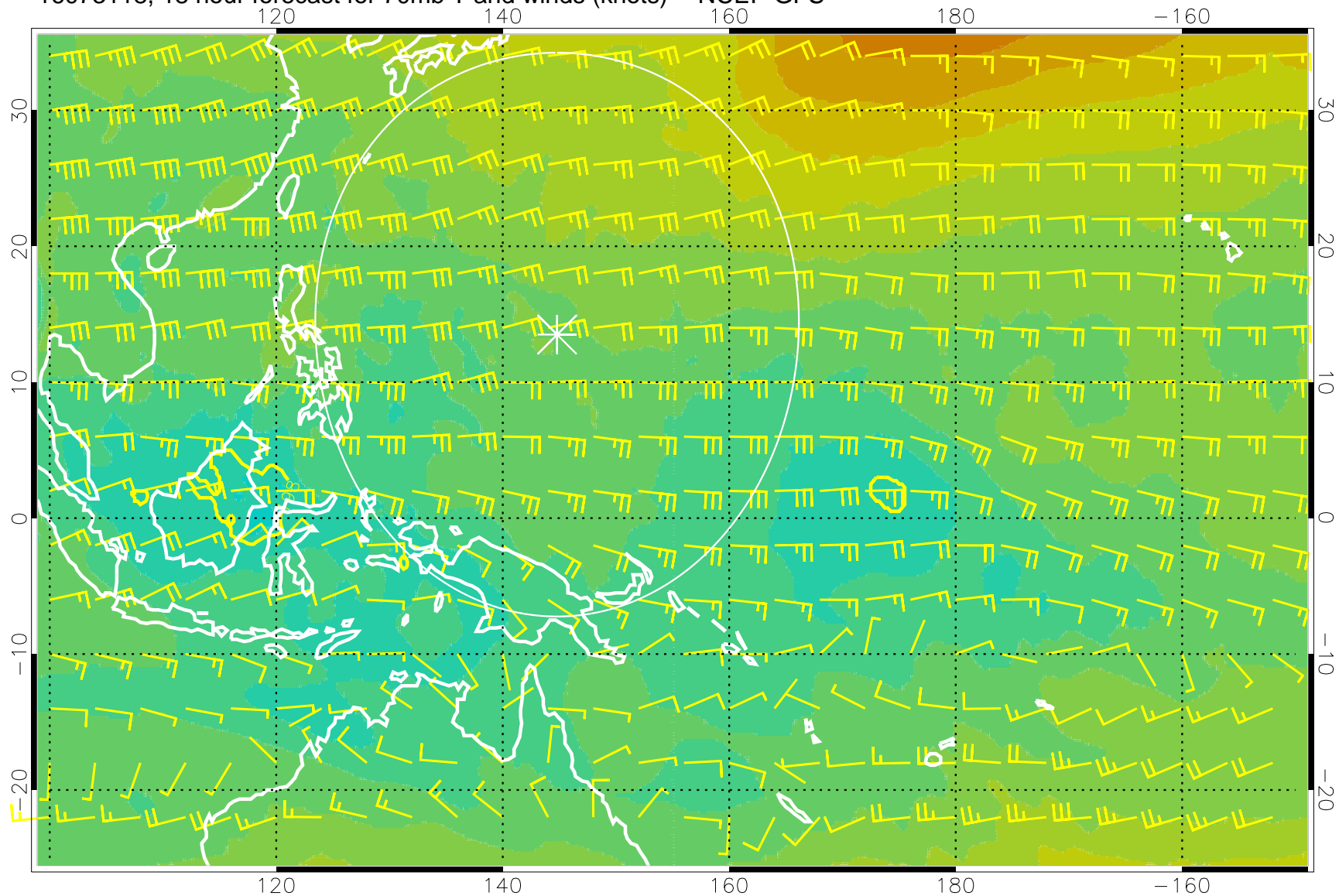
16073118, 18 hour forecast for 70mb T and winds (knots) -- NCEP GFS
