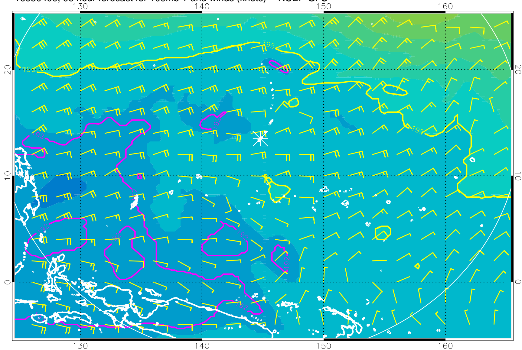
16080400, 96 hour forecast for 100mb T and winds (knots) -- NCEP GFS
