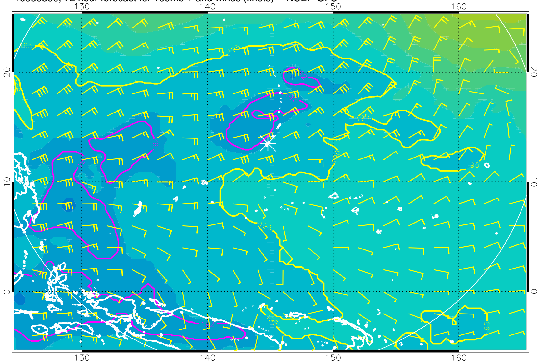
16080300, 72 hour forecast for 100mb T and winds (knots) -- NCEP GFS
