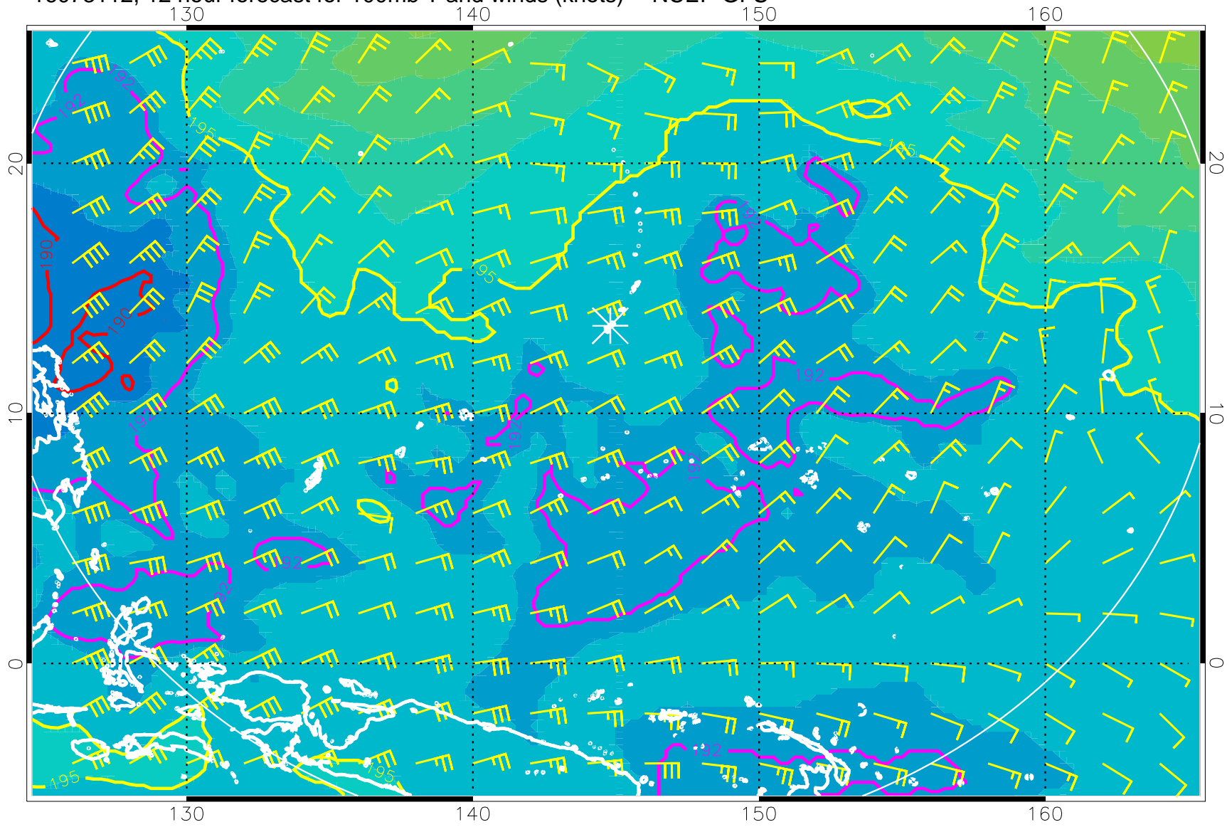
16073112, 12 hour forecast for 100mb T and winds (knots) -- NCEP GFS
