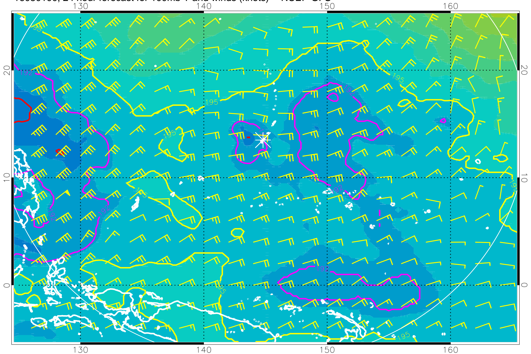
16080100, 24 hour forecast for 100mb T and winds (knots) -- NCEP GFS
