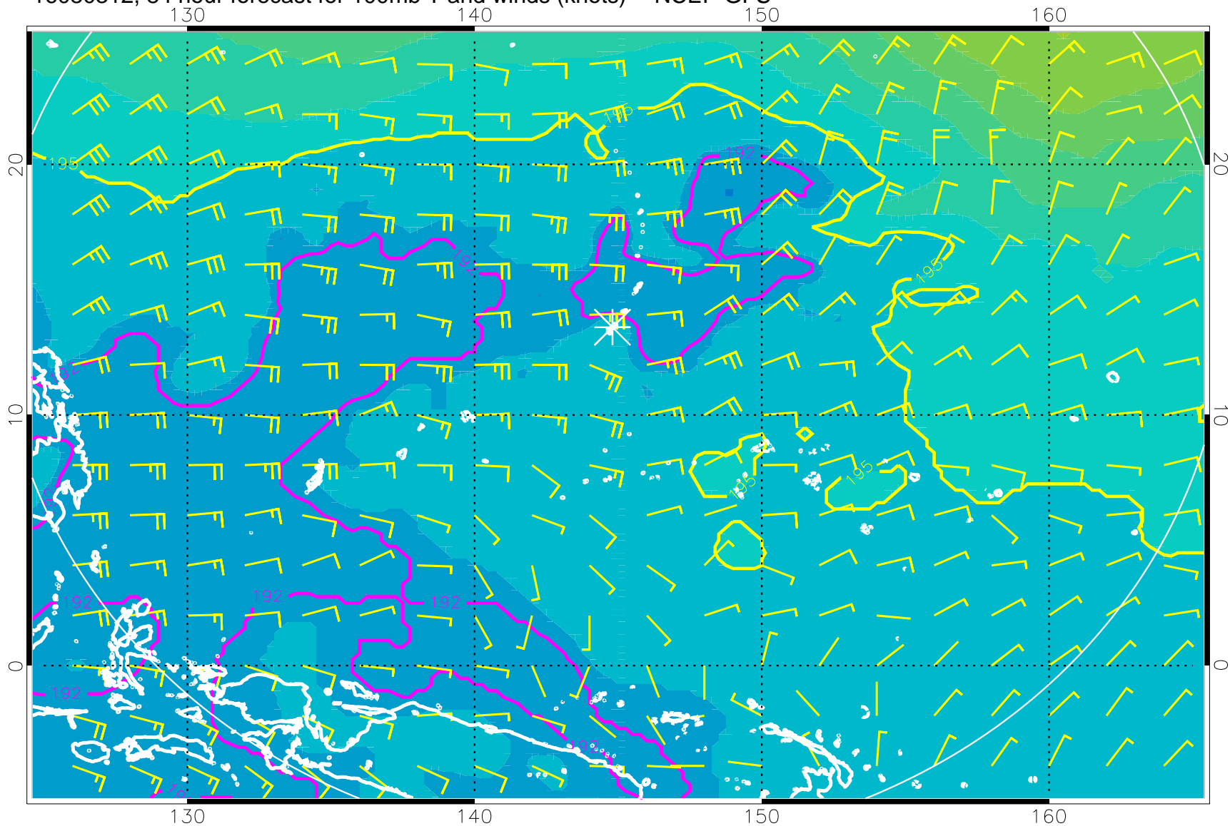
16080312, 84 hour forecast for 100mb T and winds (knots) -- NCEP GFS
