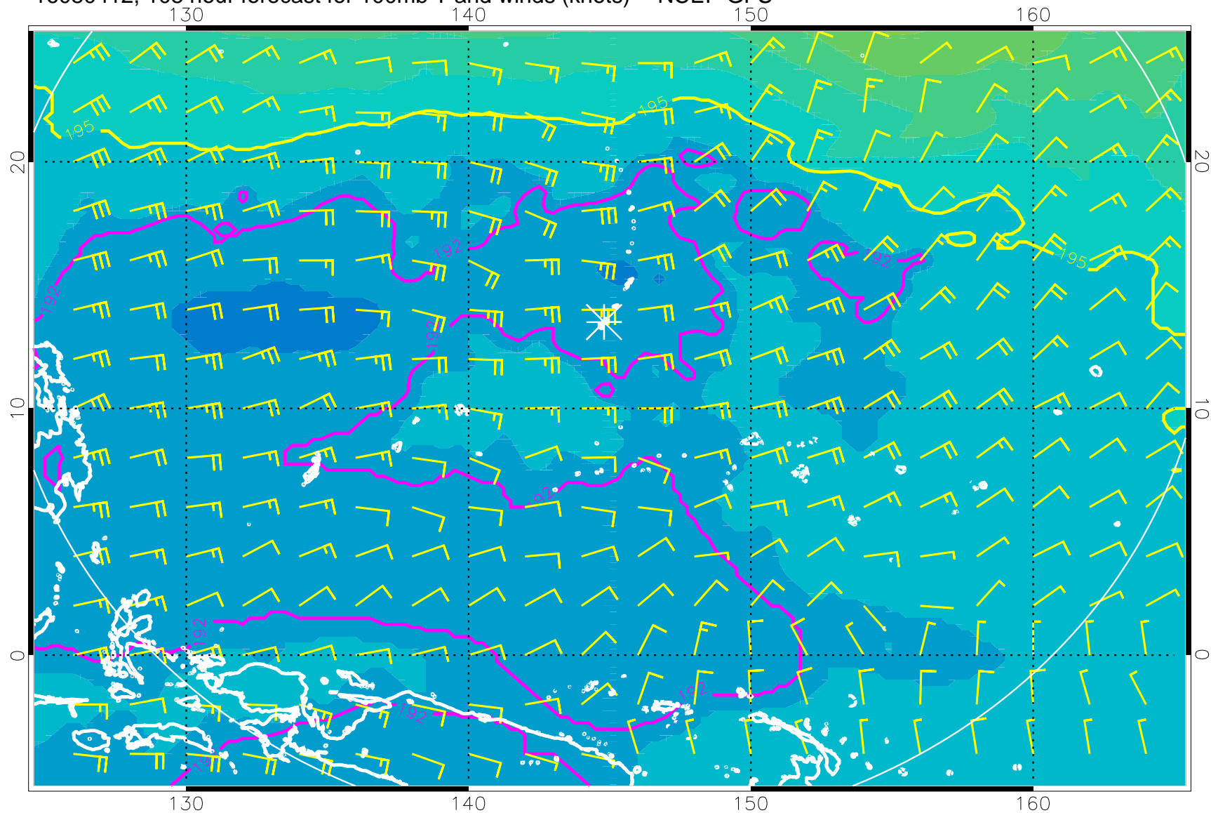
16080412, 108 hour forecast for 100mb T and winds (knots) -- NCEP GFS
