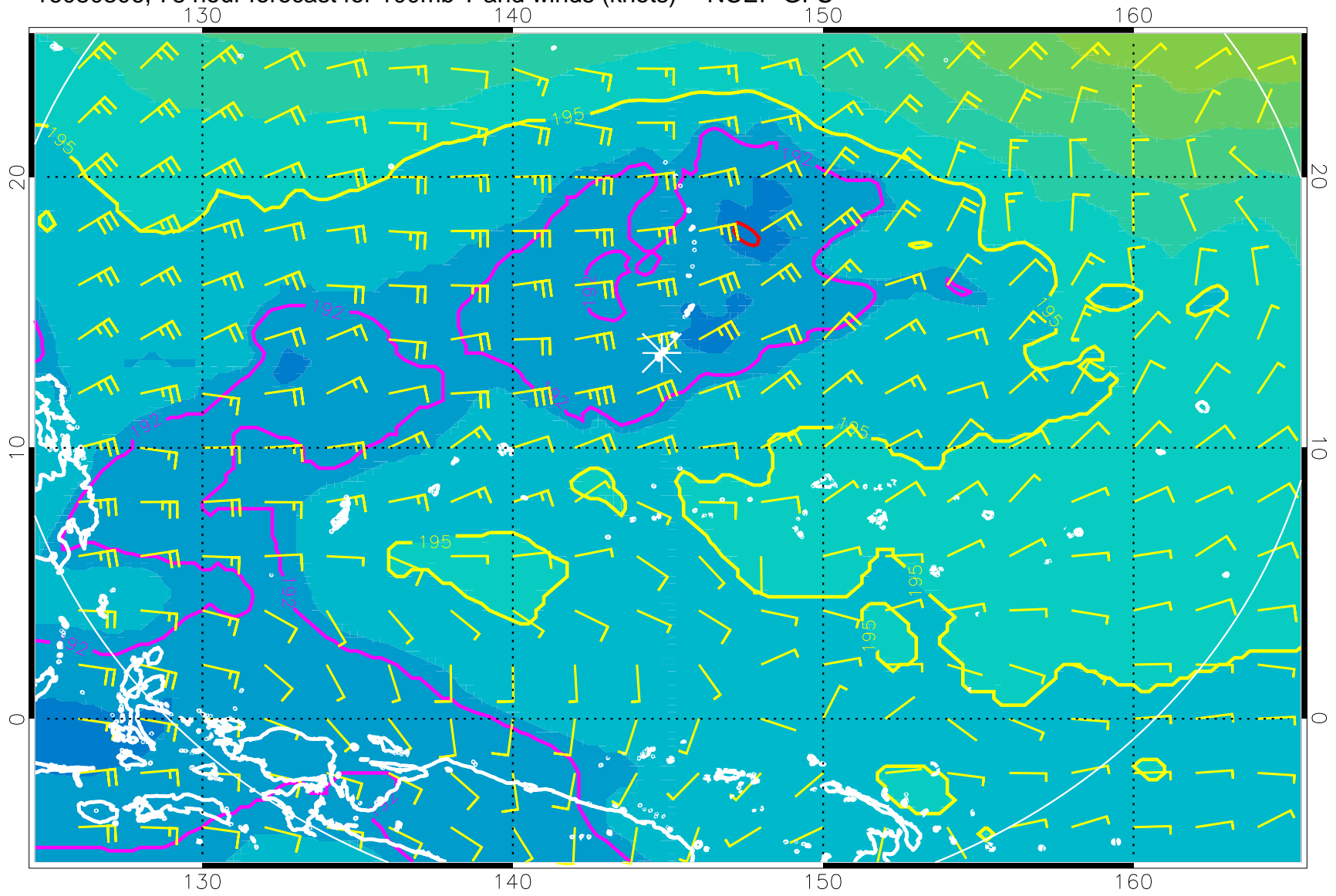
16080306, 78 hour forecast for 100mb T and winds (knots) -- NCEP GFS
