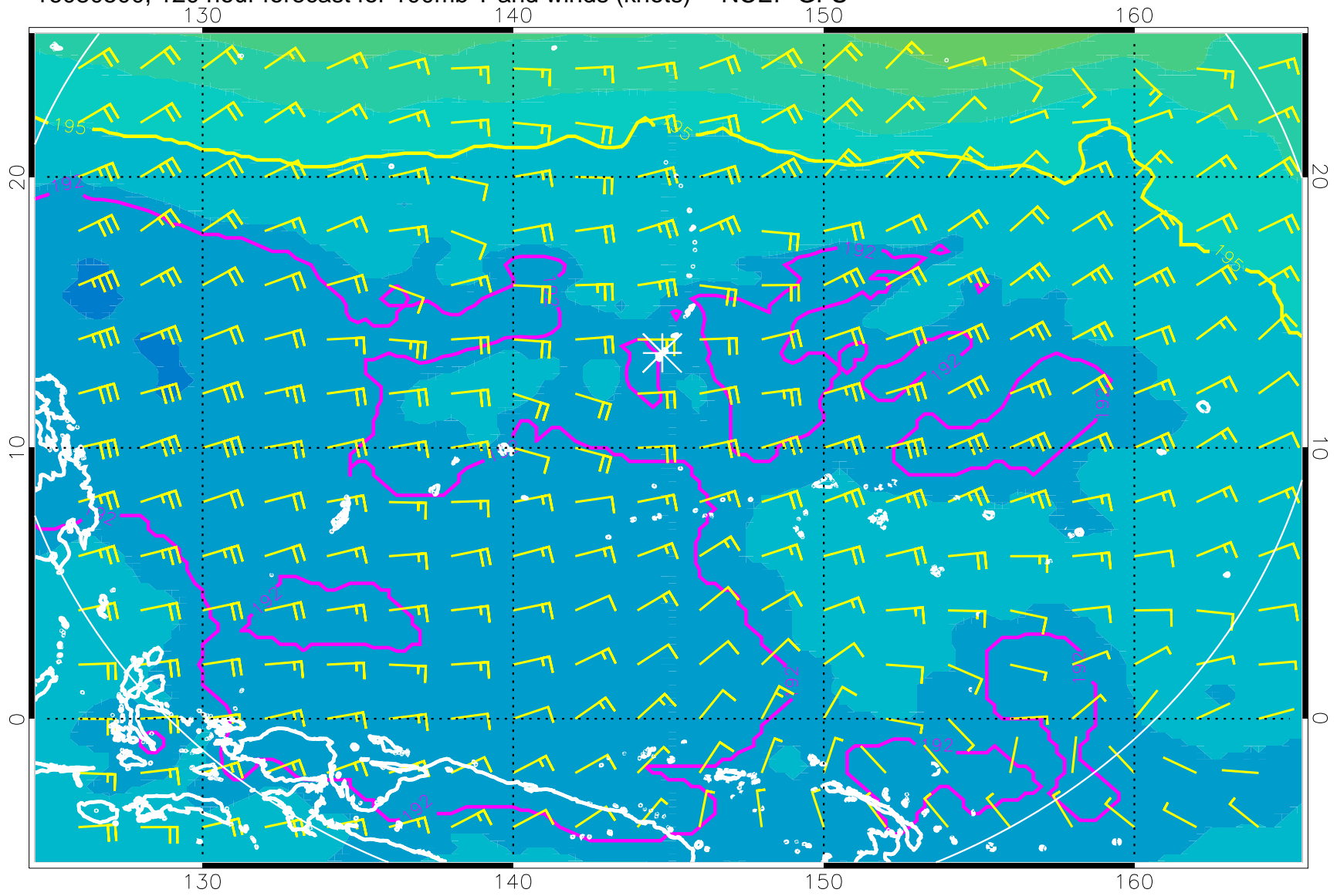
16080500, 120 hour forecast for 100mb T and winds (knots) -- NCEP GFS
