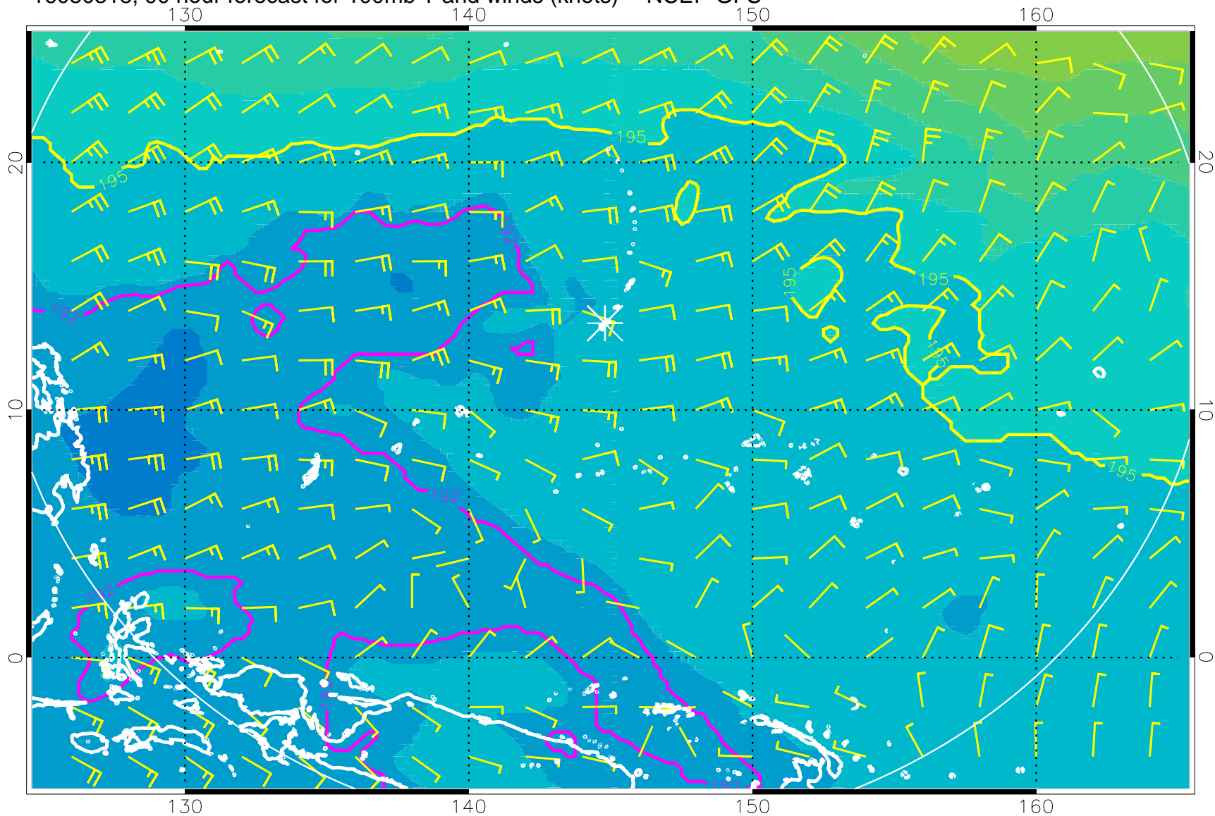
16080318, 90 hour forecast for 100mb T and winds (knots) -- NCEP GFS
