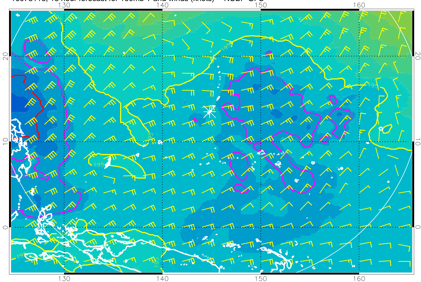
16073118, 18 hour forecast for 100mb T and winds (knots) -- NCEP GFS
