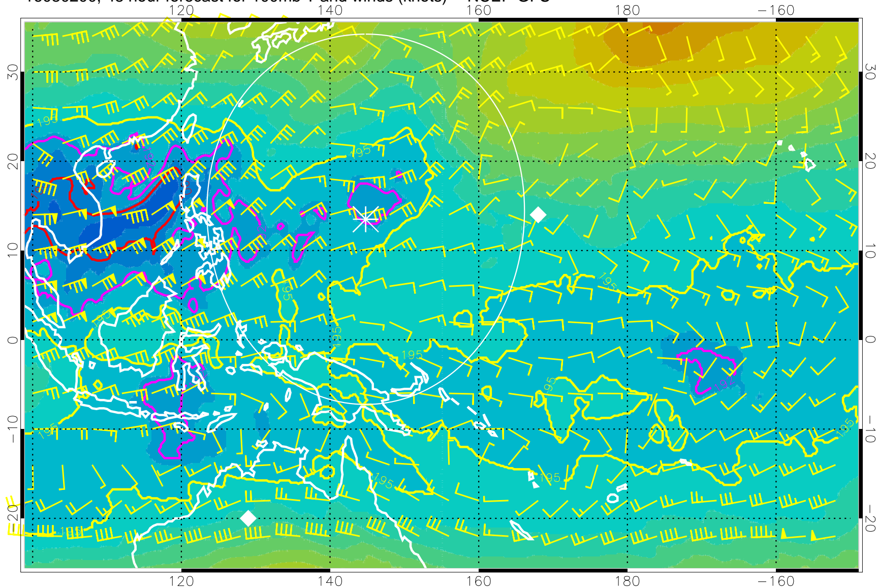
16080200, 48 hour forecast for 100mb T and winds (knots) -- NCEP GFS
