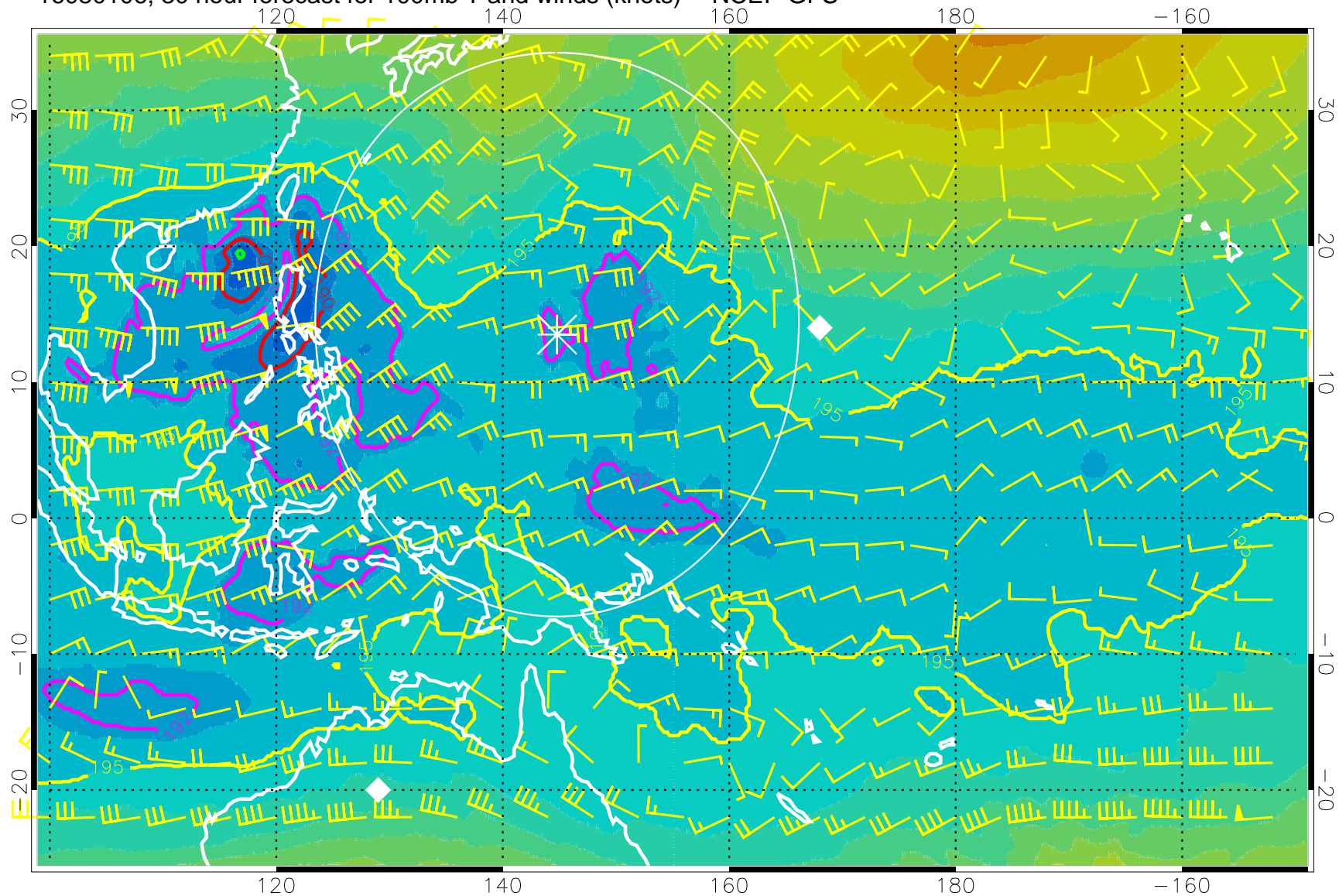
16080106, 30 hour forecast for 100mb T and winds (knots) -- NCEP GFS
