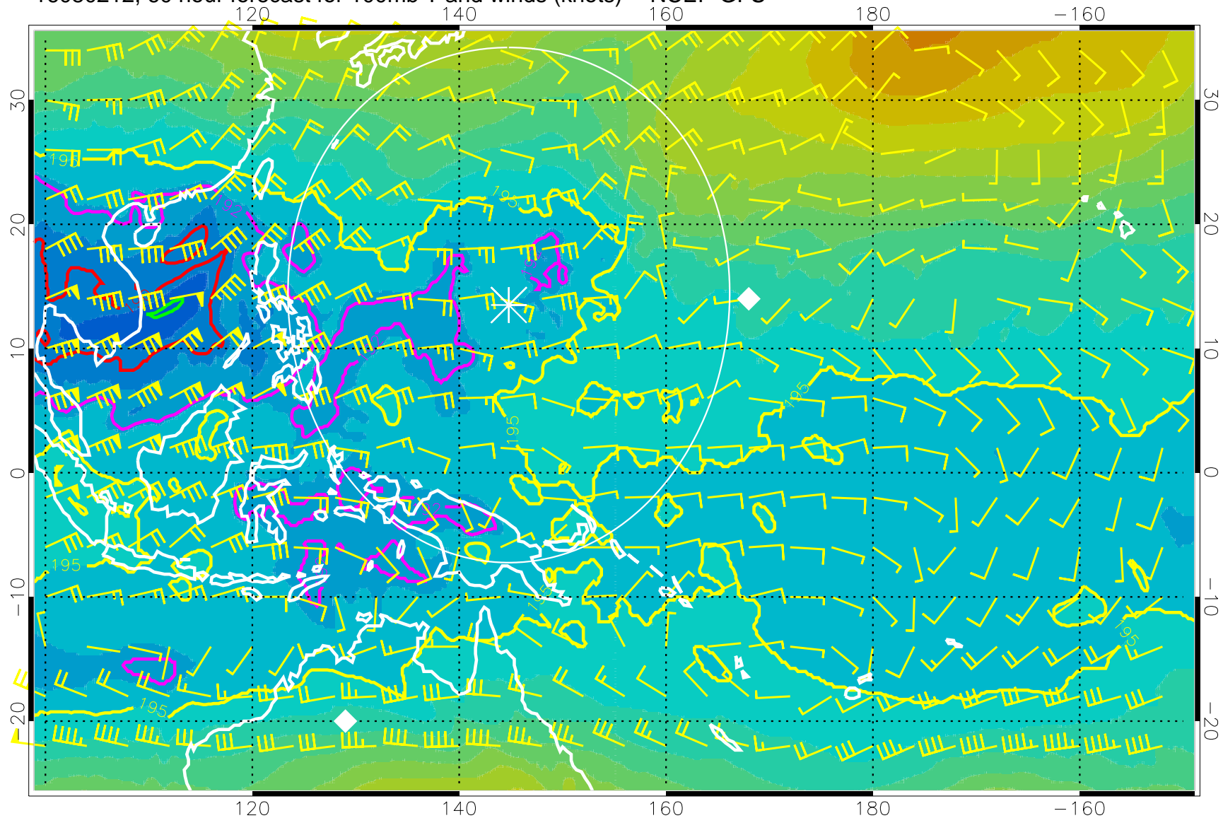
16080212, 60 hour forecast for 100mb T and winds (knots) -- NCEP GFS
