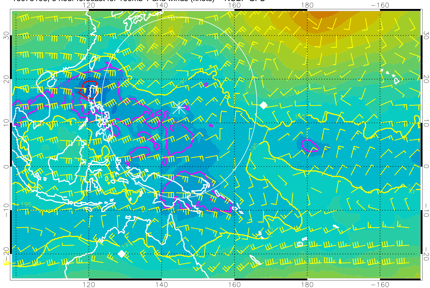
16073106, 6 hour forecast for 100mb T and winds (knots) -- NCEP GFS
