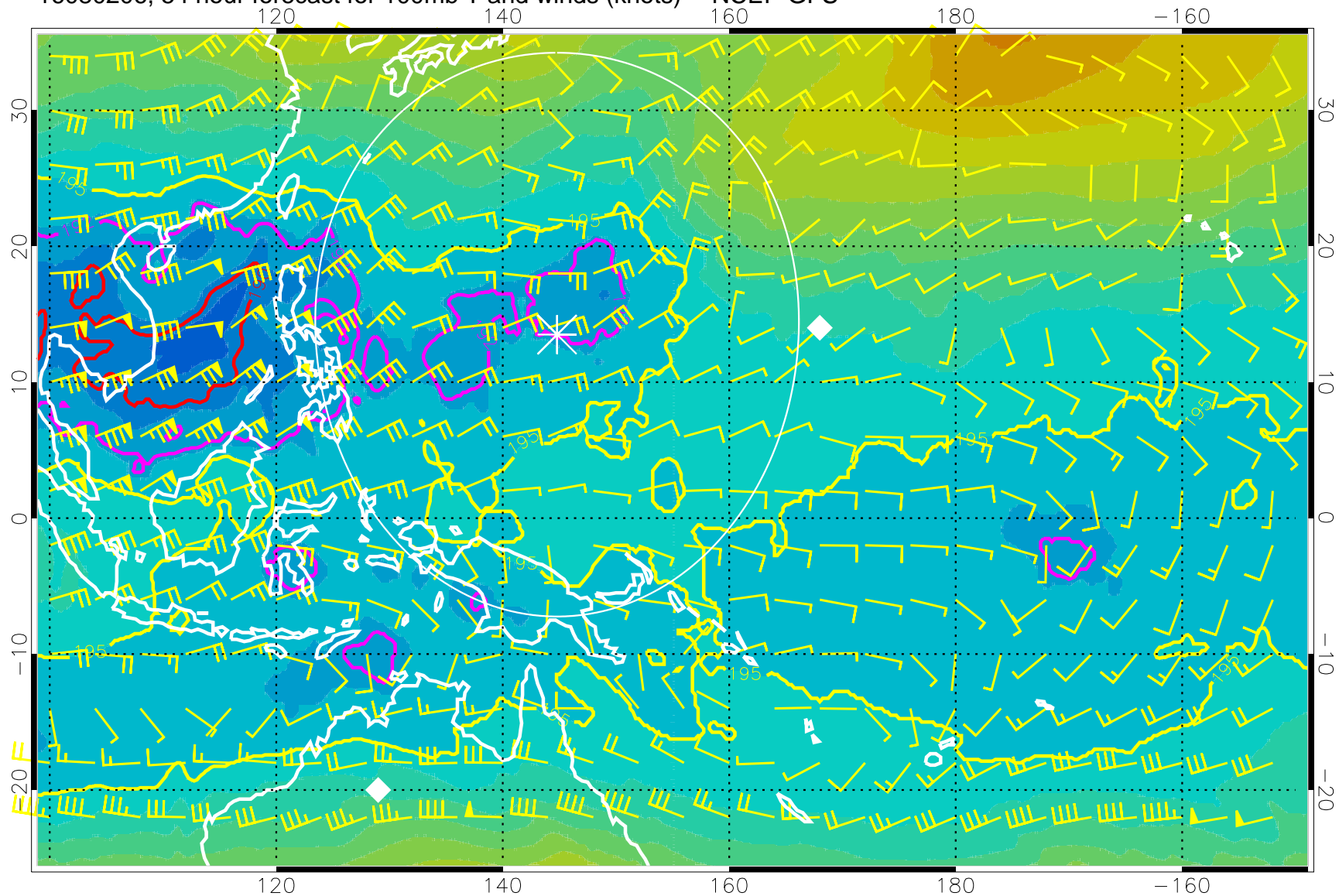
16080206, 54 hour forecast for 100mb T and winds (knots) -- NCEP GFS
