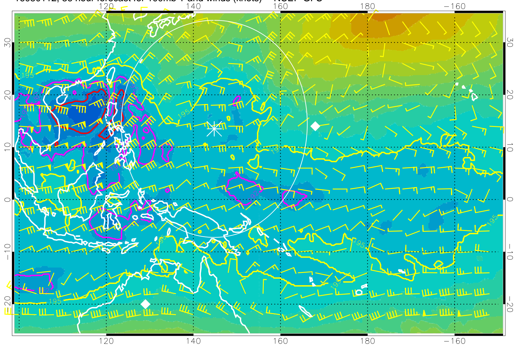
16080112, 36 hour forecast for 100mb T and winds (knots) -- NCEP GFS
