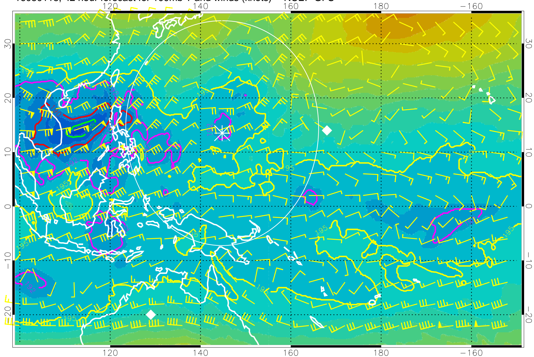
16080118, 42 hour forecast for 100mb T and winds (knots) -- NCEP GFS
