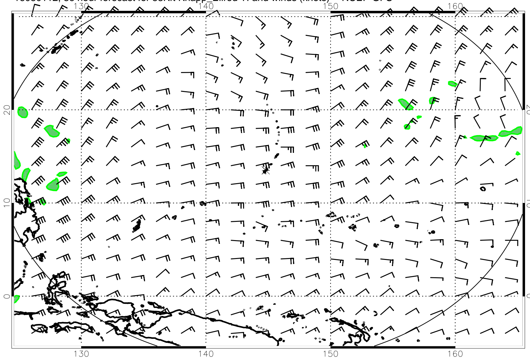
16080112, 36 hour forecast for 53Kft Knapp_Ellrod TI and winds (knots) -- NCEP GFS
