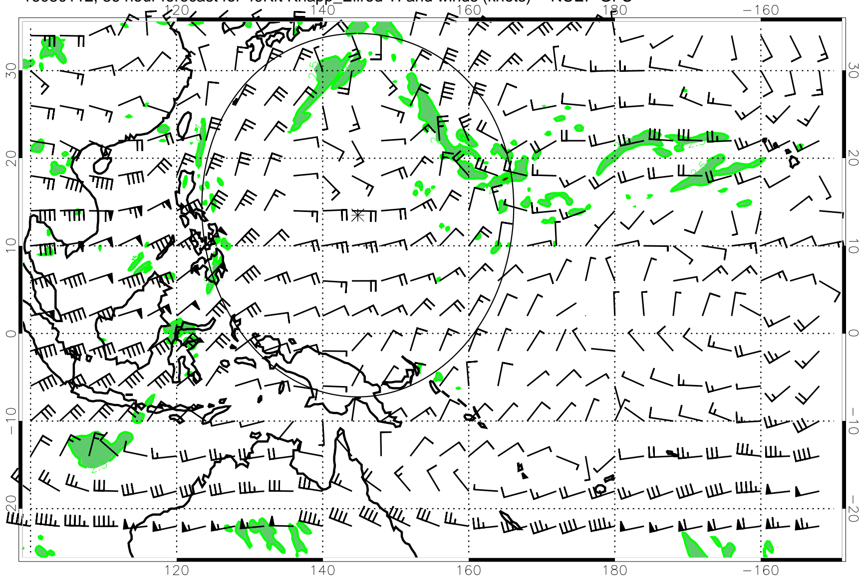
16080112, 36 hour forecast for 49Kft Knapp_Ellrod TI and winds (knots) -- NCEP GFS
