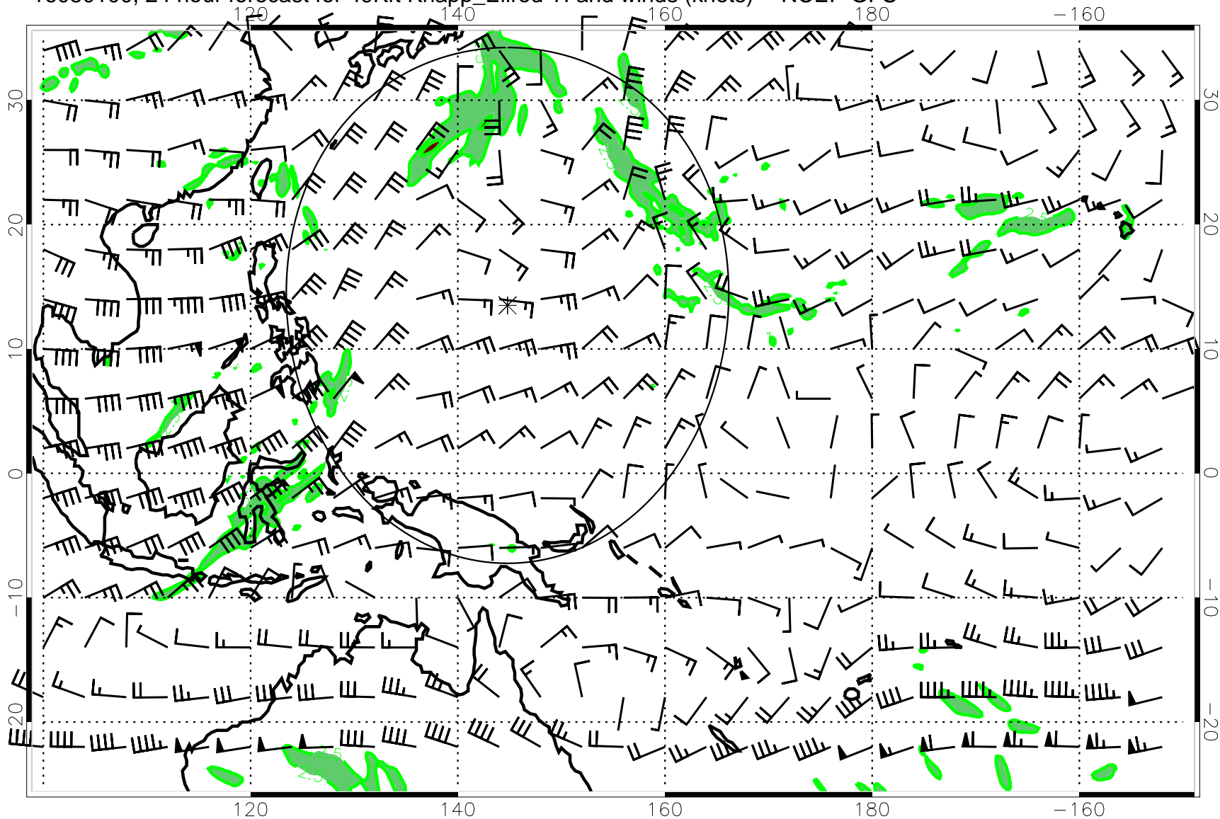
16080100, 24 hour forecast for 49Kft Knapp_Ellrod TI and winds (knots) -- NCEP GFS
