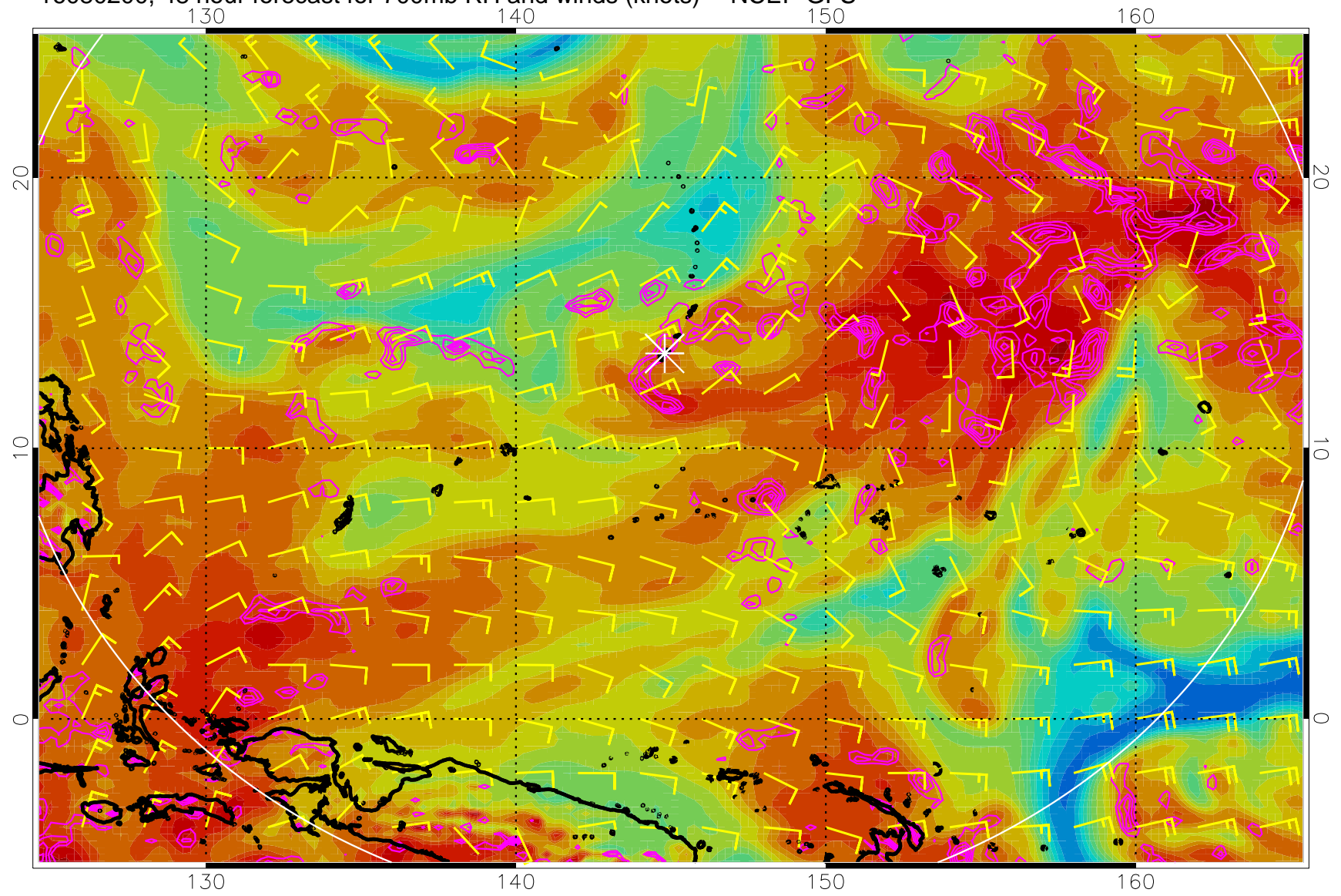
16080200, 48 hour forecast for 700mb RH and winds (knots) -- NCEP GFS
