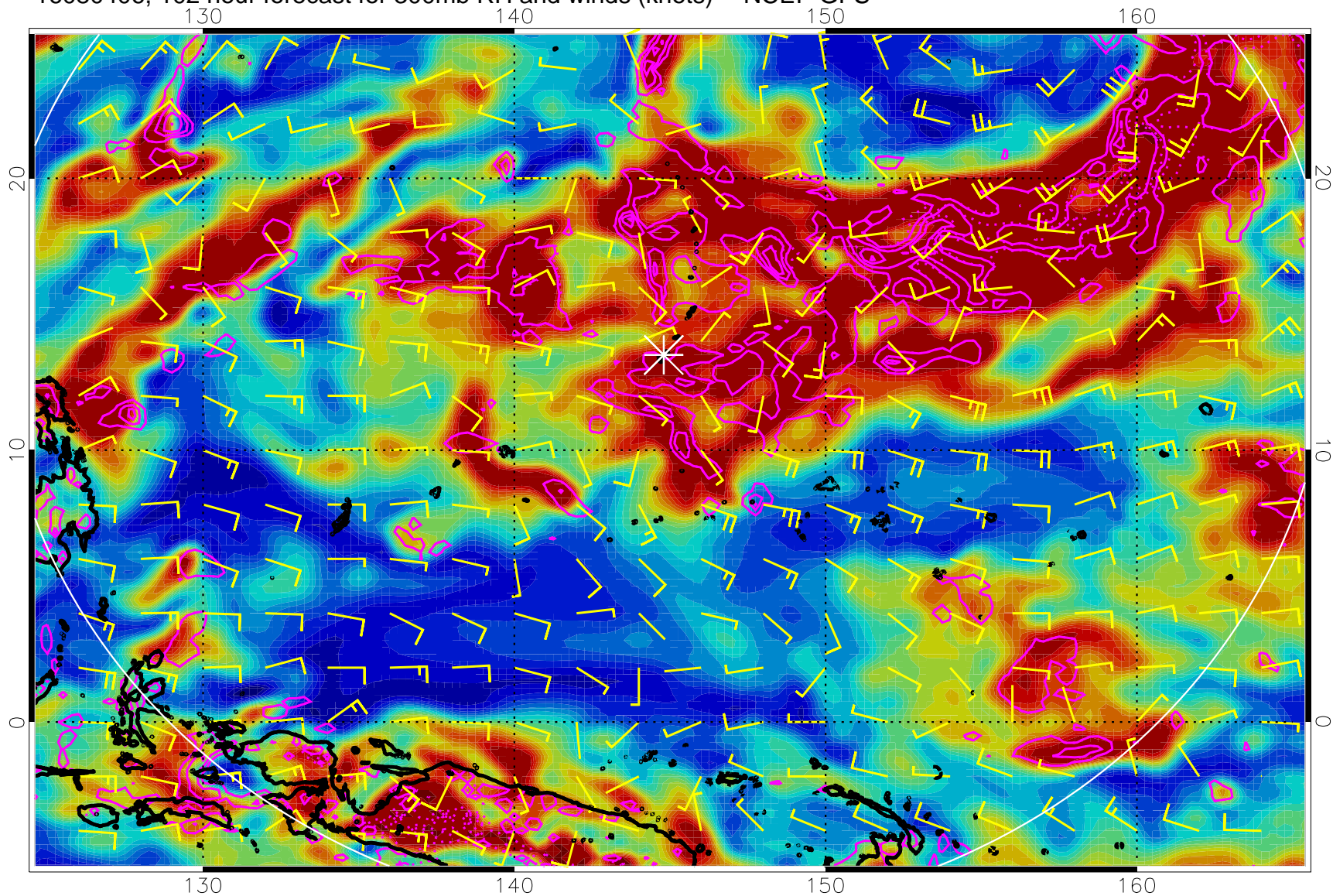
16080406, 102 hour forecast for 300mb RH and winds (knots) -- NCEP GFS
