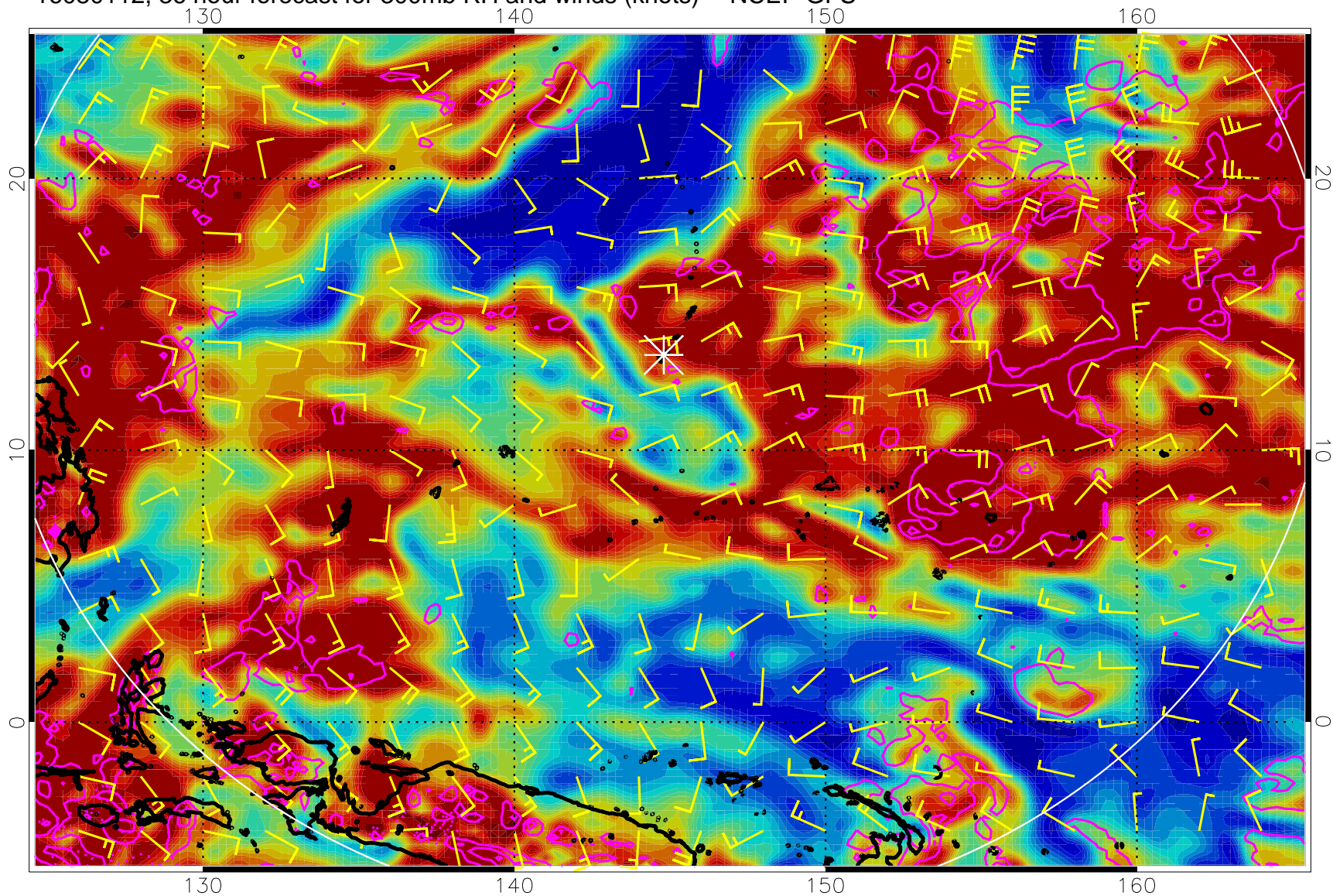
16080112, 36 hour forecast for 300mb RH and winds (knots) -- NCEP GFS
