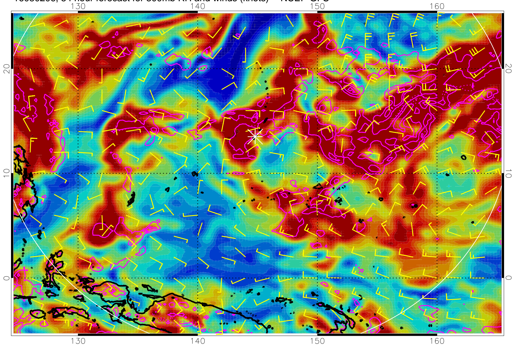
16080206, 54 hour forecast for 300mb RH and winds (knots) -- NCEP GFS
