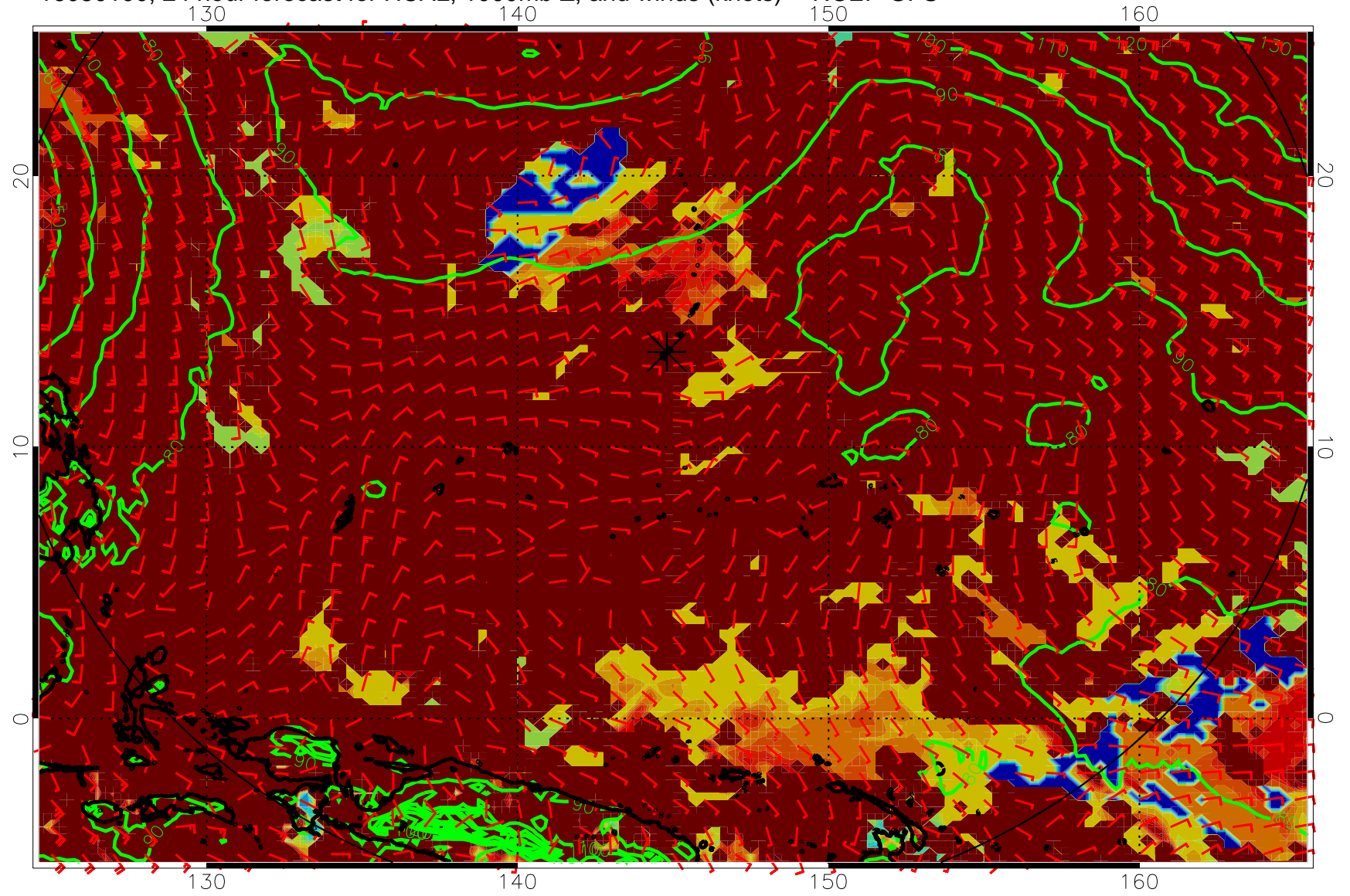
16080100, 24 hour forecast for HCAL, 1000mb Z, and winds (knots) -- NCEP GFS
