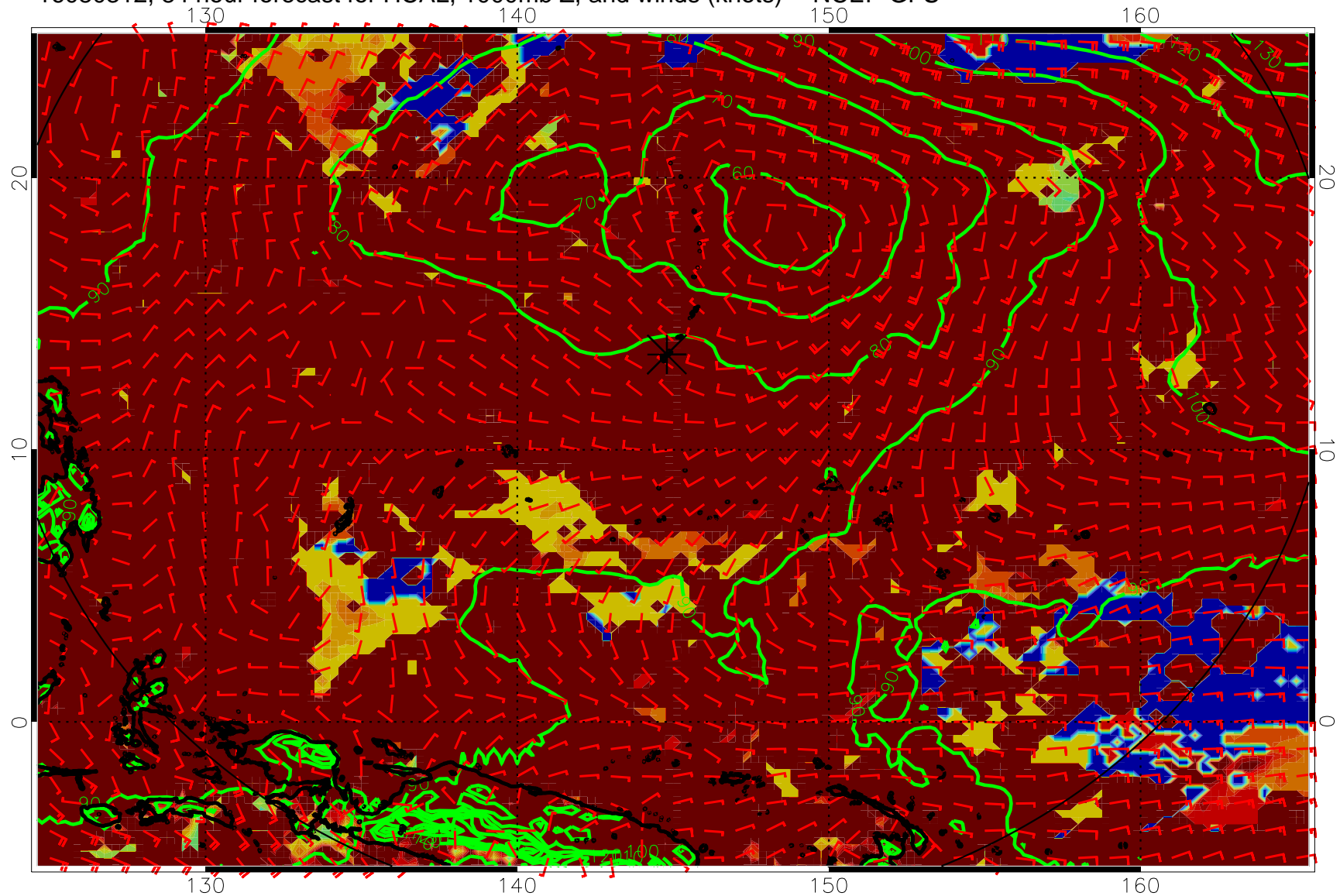
16080312, 84 hour forecast for HCAL, 1000mb Z, and winds (knots) -- NCEP GFS
