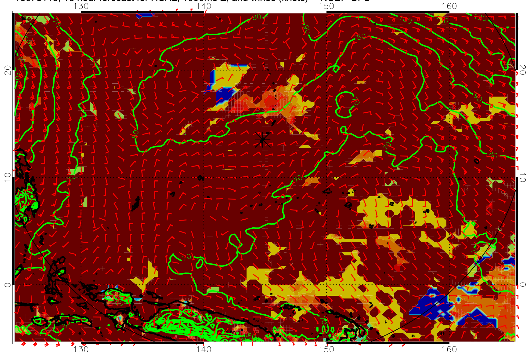
16073118, 18 hour forecast for HCAL, 1000mb Z, and winds (knots) -- NCEP GFS
