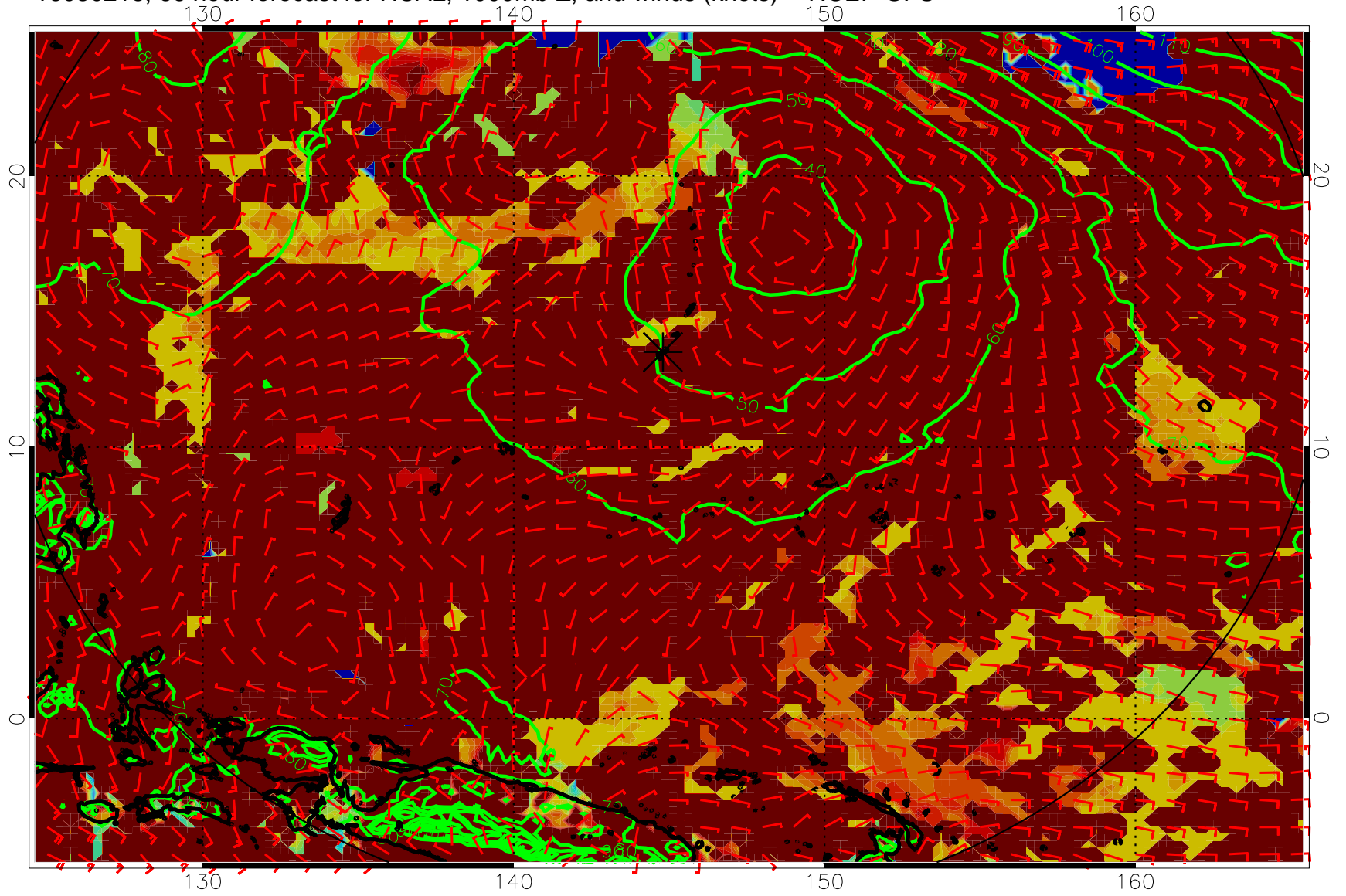
16080218, 66 hour forecast for HCAL, 1000mb Z, and winds (knots) -- NCEP GFS
