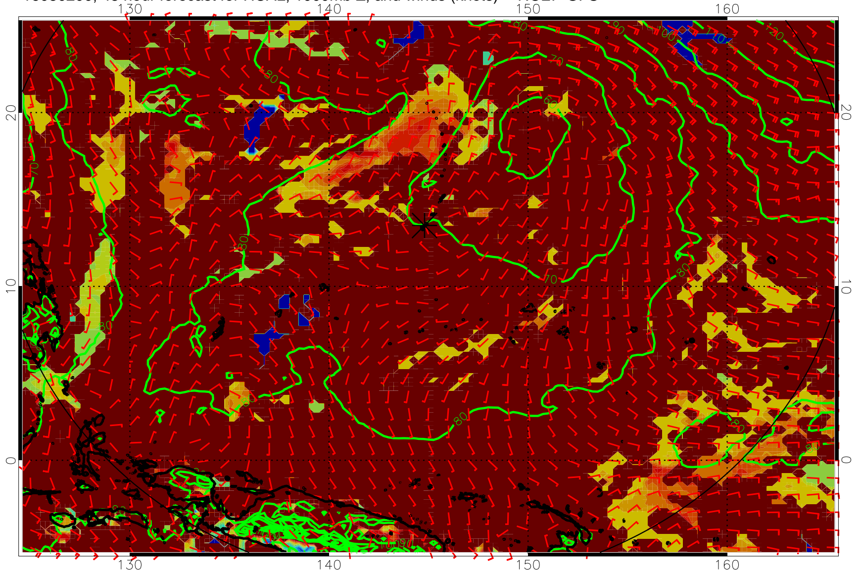
16080200, 48 hour forecast for HCAL, 1000mb Z, and winds (knots) -- NCEP GFS
