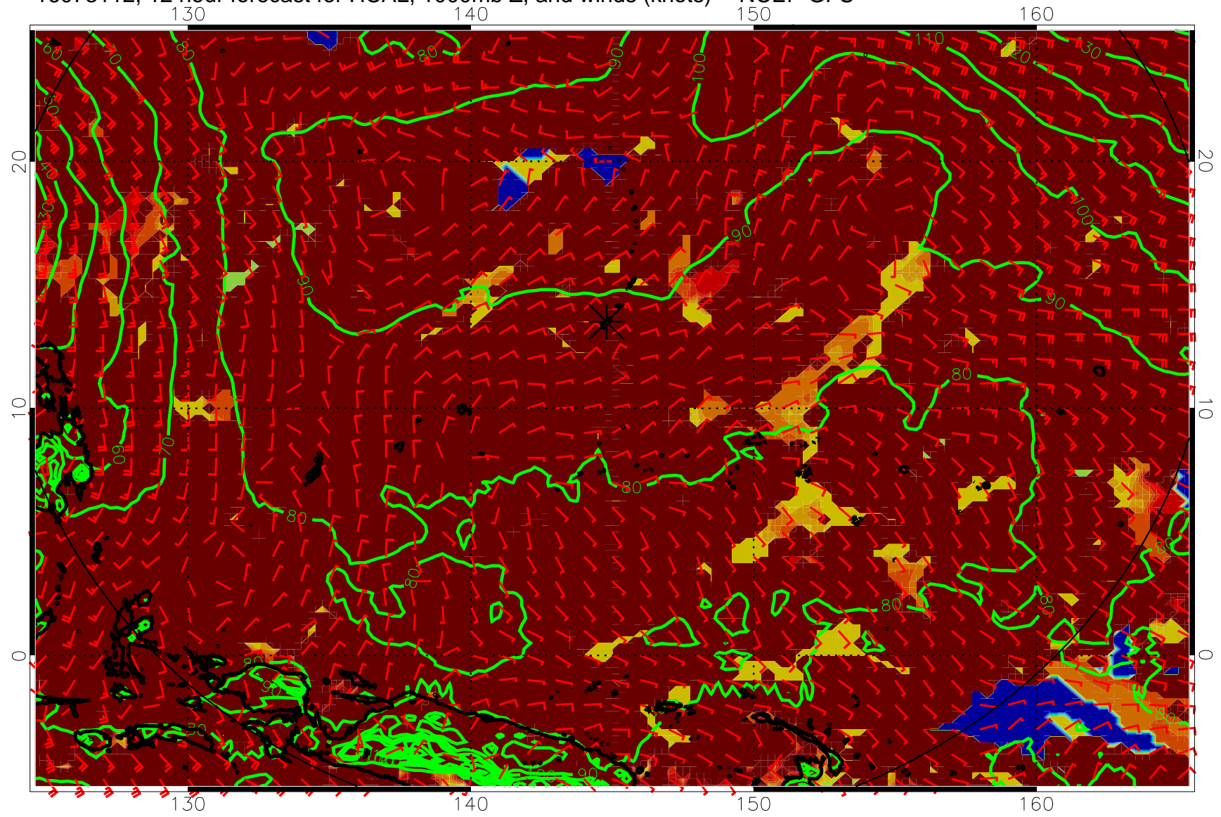
16073112, 12 hour forecast for HCAL, 1000mb Z, and winds (knots) -- NCEP GFS
