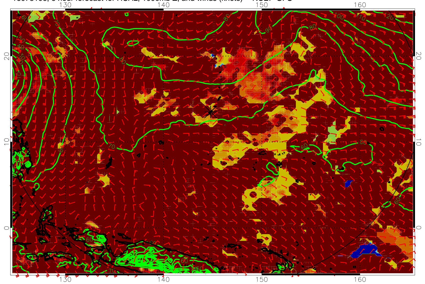
16073106, 6 hour forecast for HCAL, 1000mb Z, and winds (knots) -- NCEP GFS
