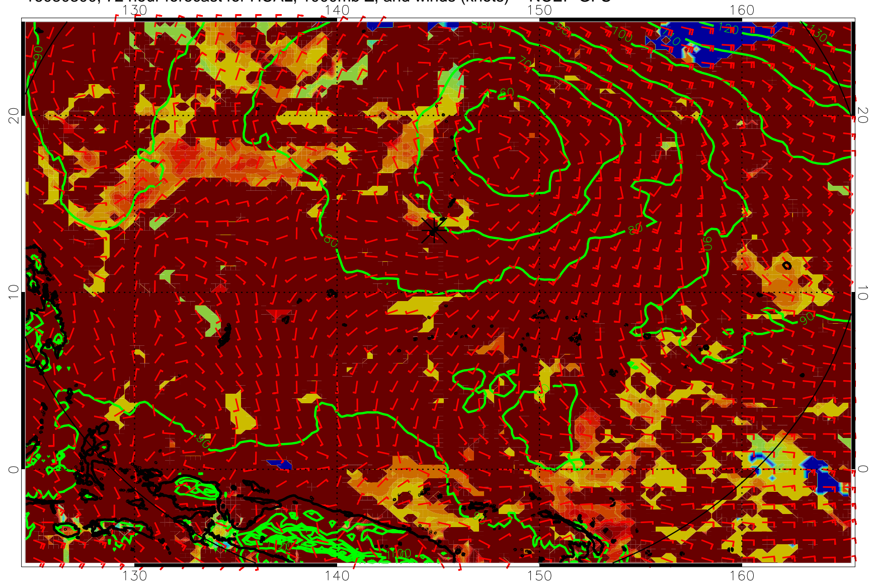
16080300, 72 hour forecast for HCAL, 1000mb Z, and winds (knots) -- NCEP GFS
