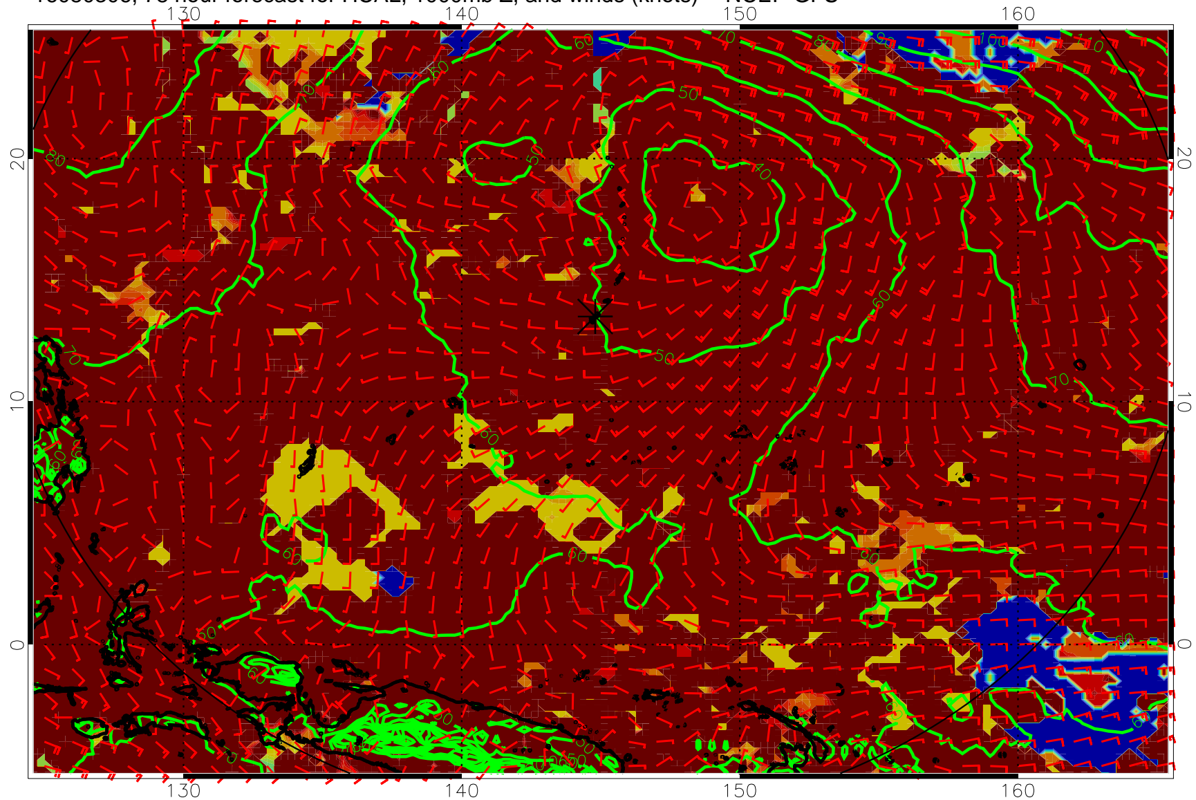
16080306, 78 hour forecast for HCAL, 1000mb Z, and winds (knots) -- NCEP GFS
