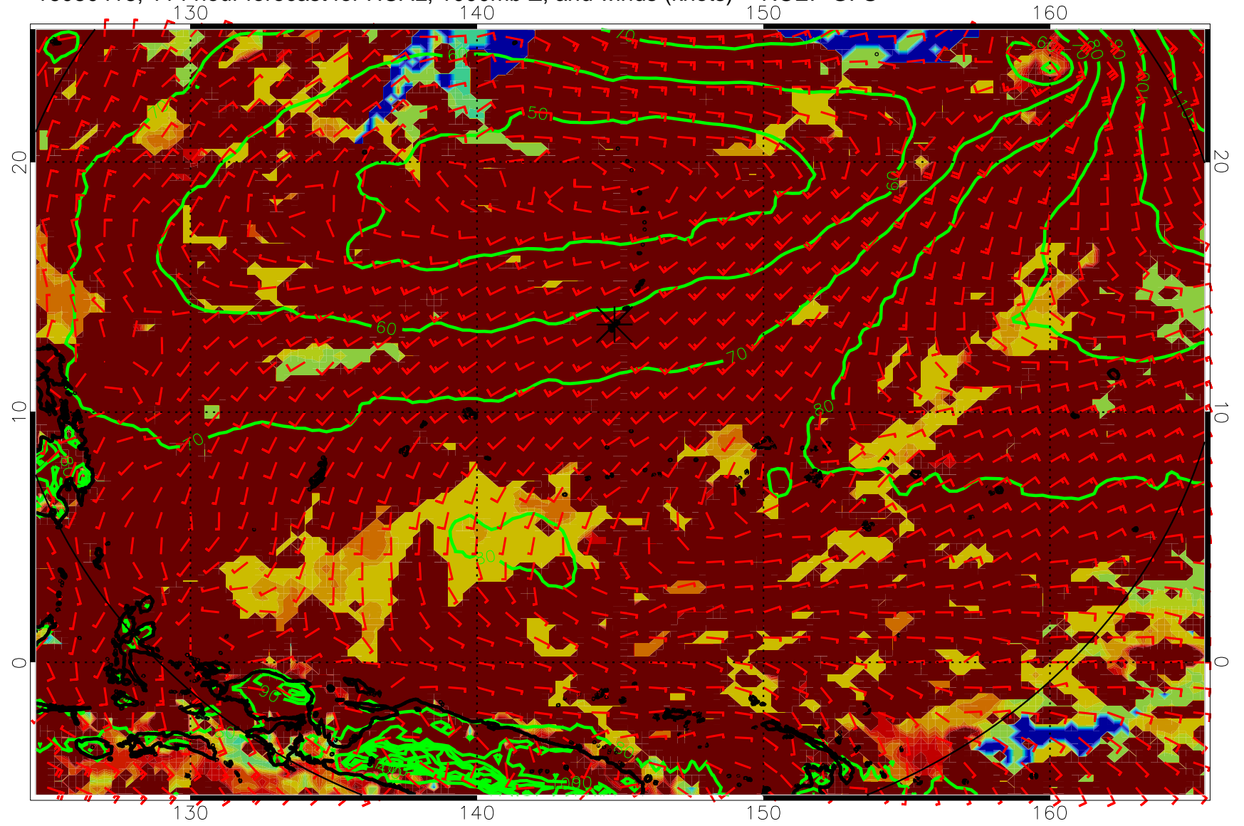
16080418, 114 hour forecast for HCAL, 1000mb Z, and winds (knots) -- NCEP GFS
