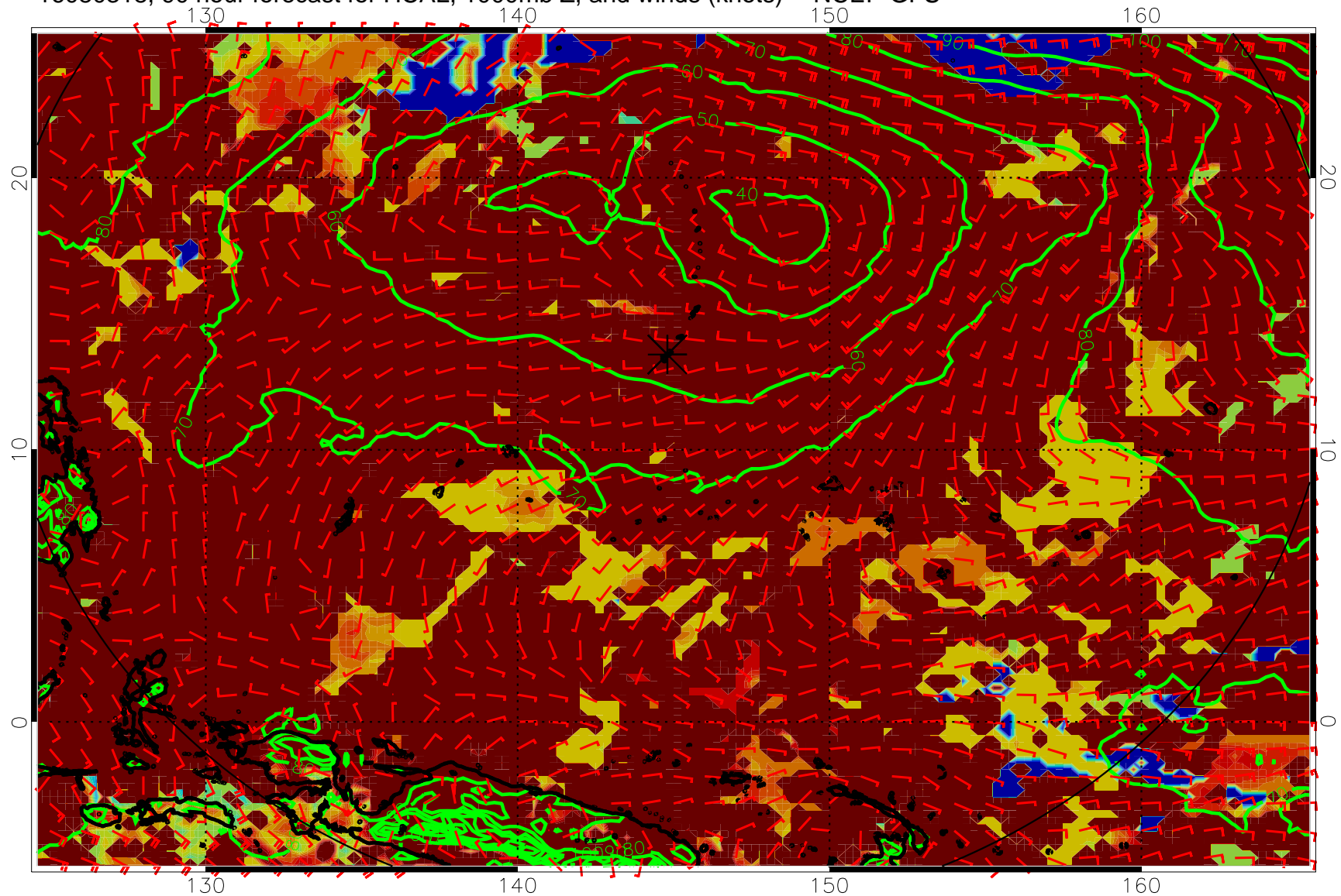
16080318, 90 hour forecast for HCAL, 1000mb Z, and winds (knots) -- NCEP GFS
