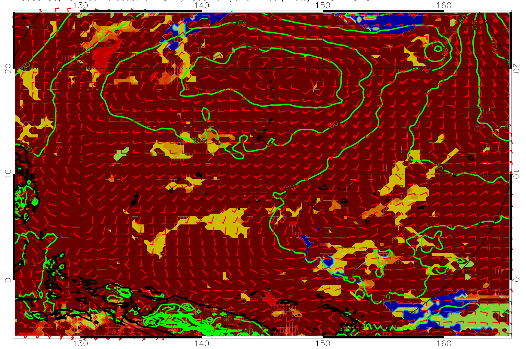
16080406, 102 hour forecast for HCAL, 1000mb Z, and winds (knots) -- NCEP GFS
