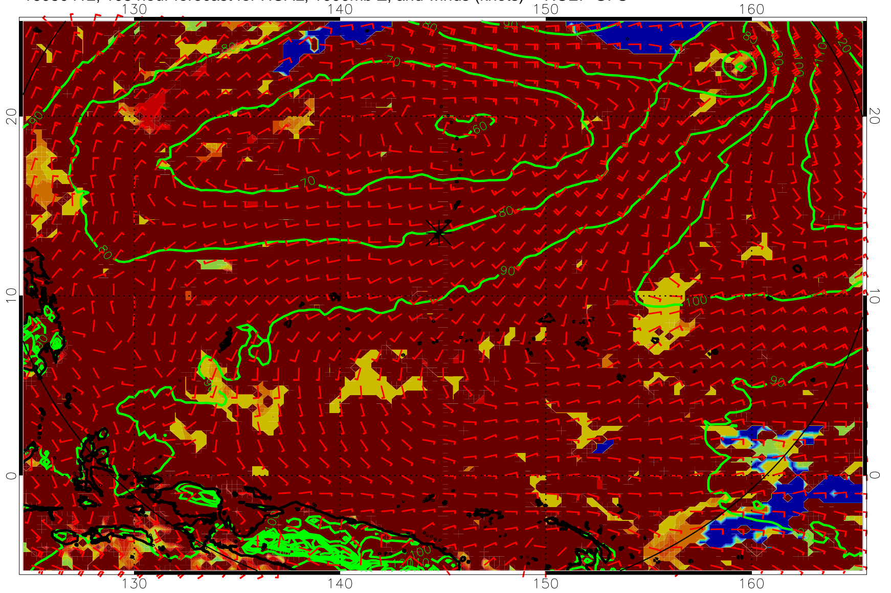
16080412, 108 hour forecast for HCAL, 1000mb Z, and winds (knots) -- NCEP GFS
