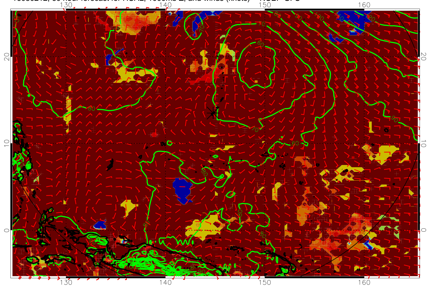
16080212, 60 hour forecast for HCAL, 1000mb Z, and winds (knots) -- NCEP GFS
