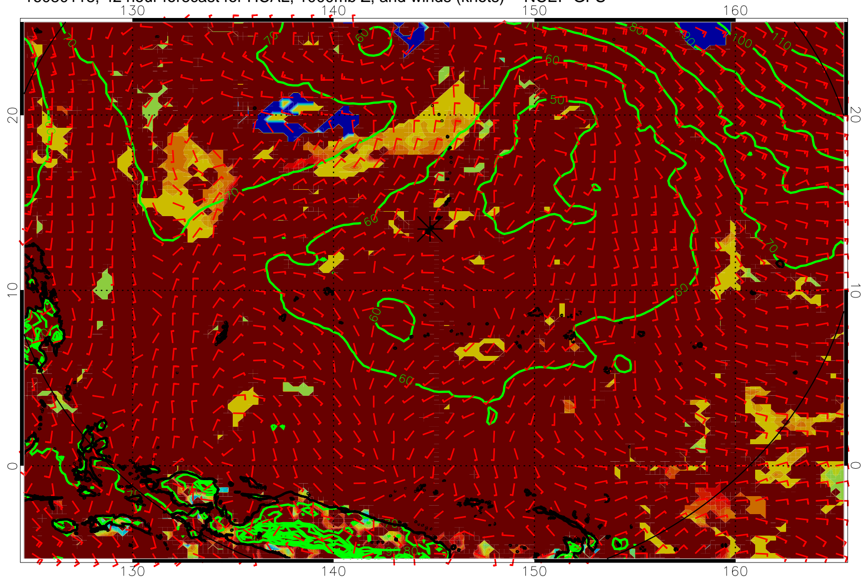
16080118, 42 hour forecast for HCAL, 1000mb Z, and winds (knots) -- NCEP GFS
