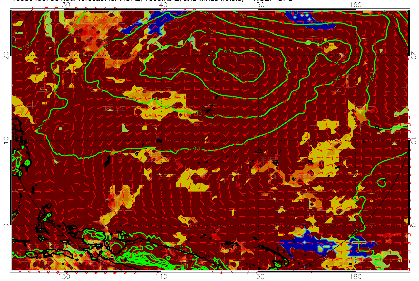
16080400, 96 hour forecast for HCAL, 1000mb Z, and winds (knots) -- NCEP GFS
