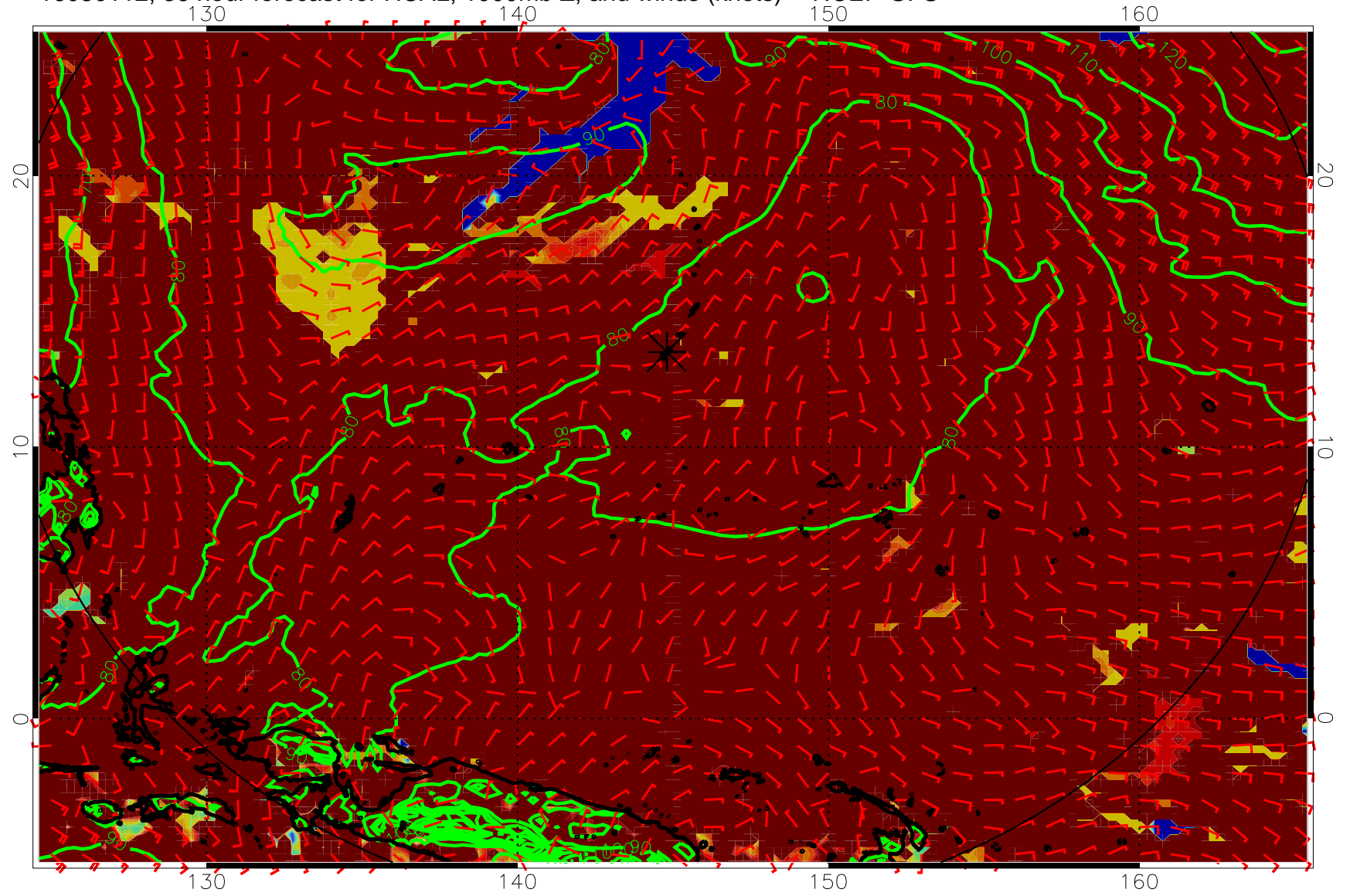
16080112, 36 hour forecast for HCAL, 1000mb Z, and winds (knots) -- NCEP GFS
