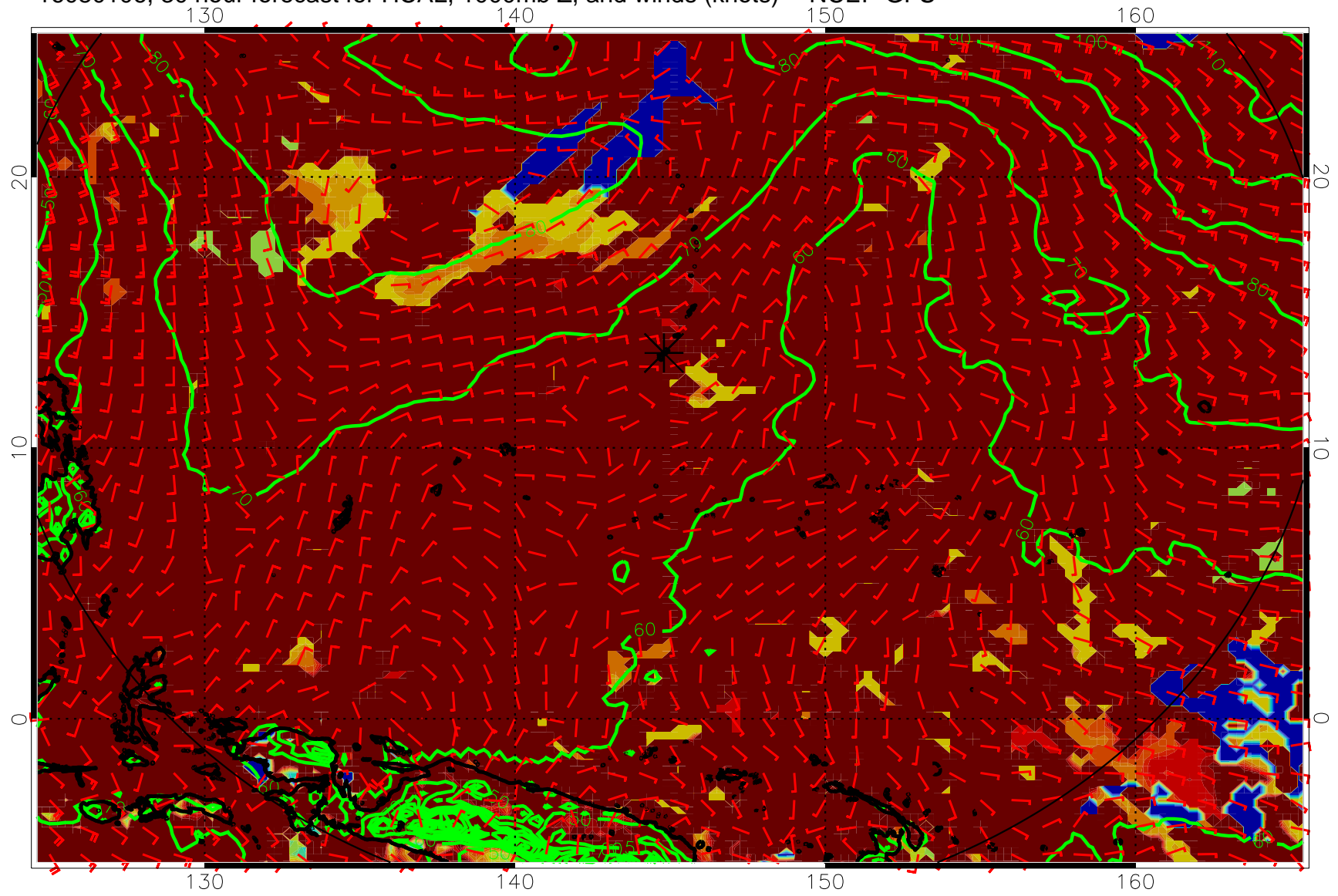
16080106, 30 hour forecast for HCAL, 1000mb Z, and winds (knots) -- NCEP GFS
