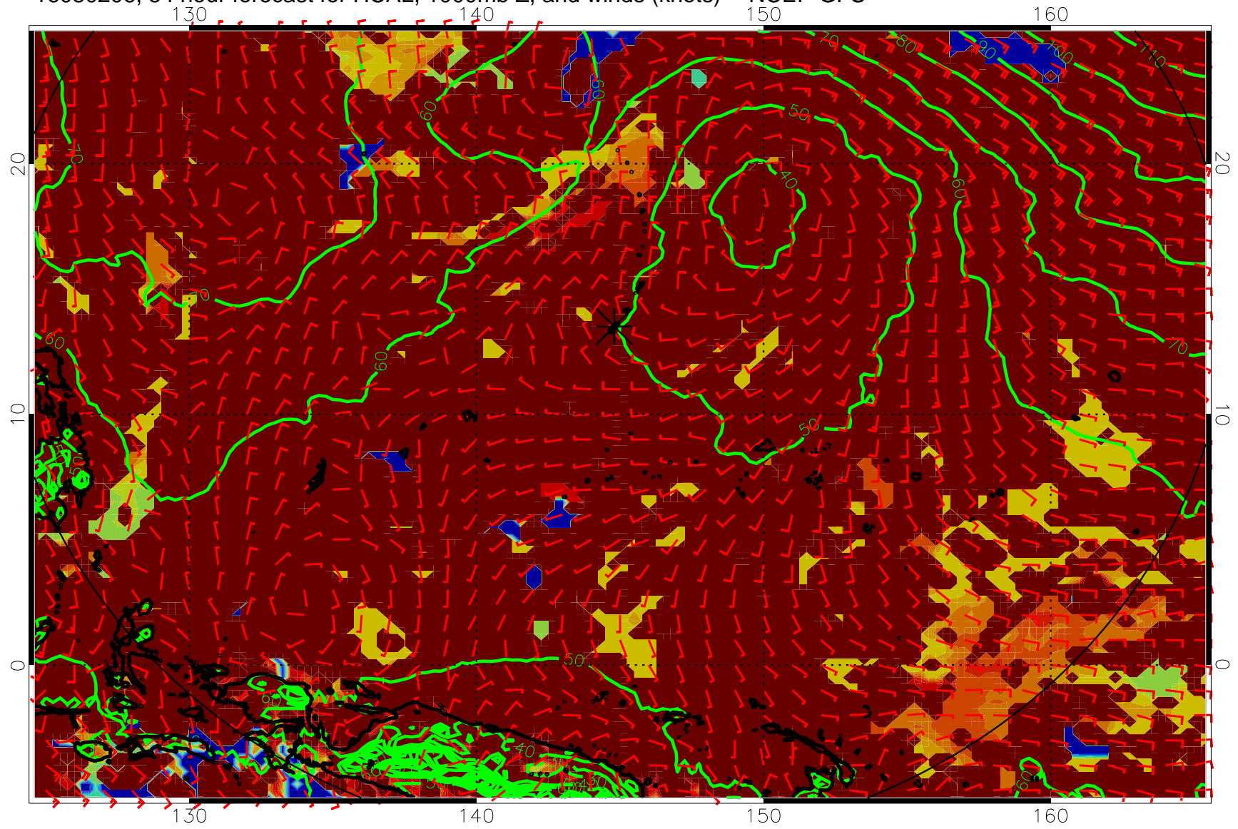
16080206, 54 hour forecast for HCAL, 1000mb Z, and winds (knots) -- NCEP GFS
