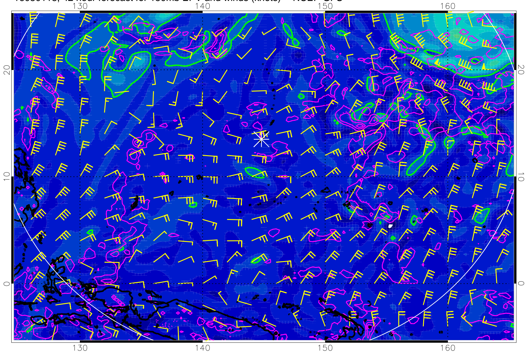
16080118, 42 hour forecast for 150mb EPV and winds (knots) -- NCEP GFS
