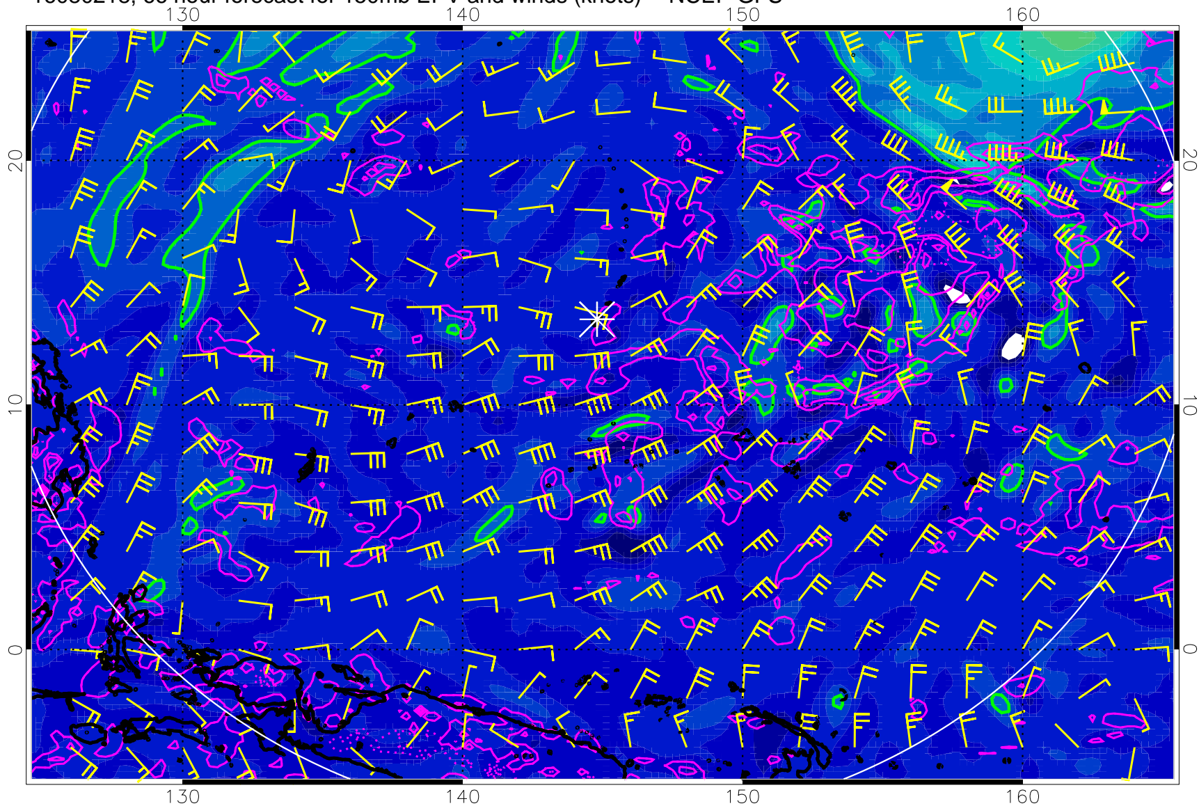
16080218, 66 hour forecast for 150mb EPV and winds (knots) -- NCEP GFS
