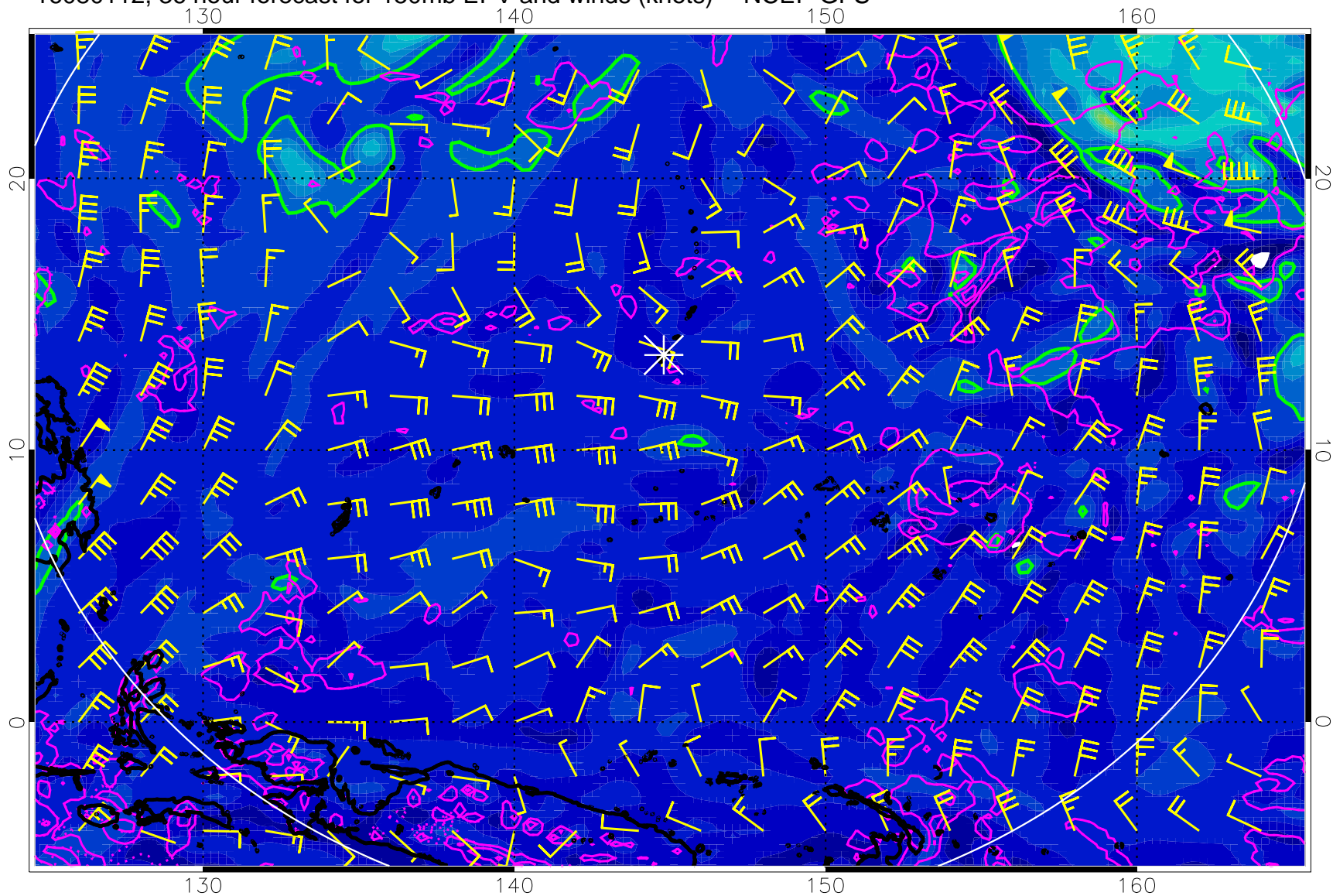
16080112, 36 hour forecast for 150mb EPV and winds (knots) -- NCEP GFS
