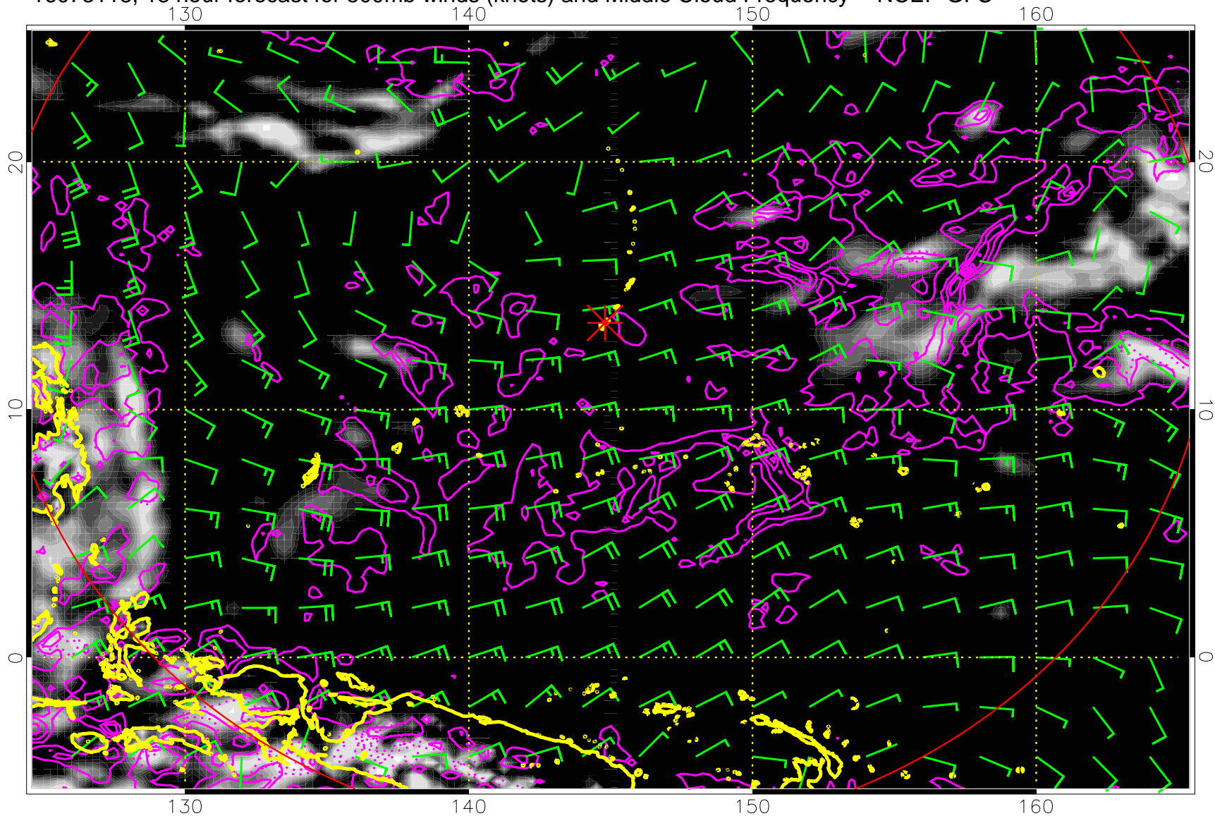
16073118, 18 hour forecast for 500mb winds (knots) and Middle Cloud Frequency -- NCEP GFS
