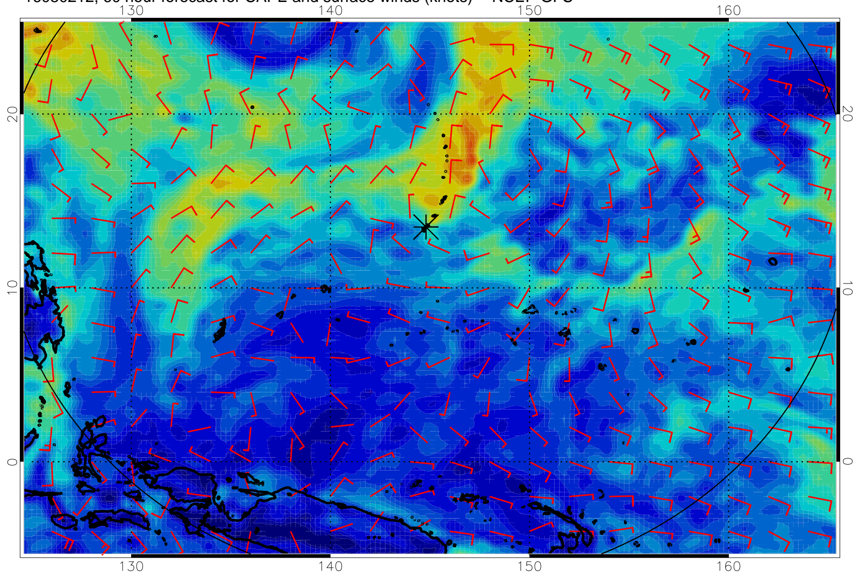
16080212, 60 hour forecast for CAPE and surface winds (knots) -- NCEP GFS
