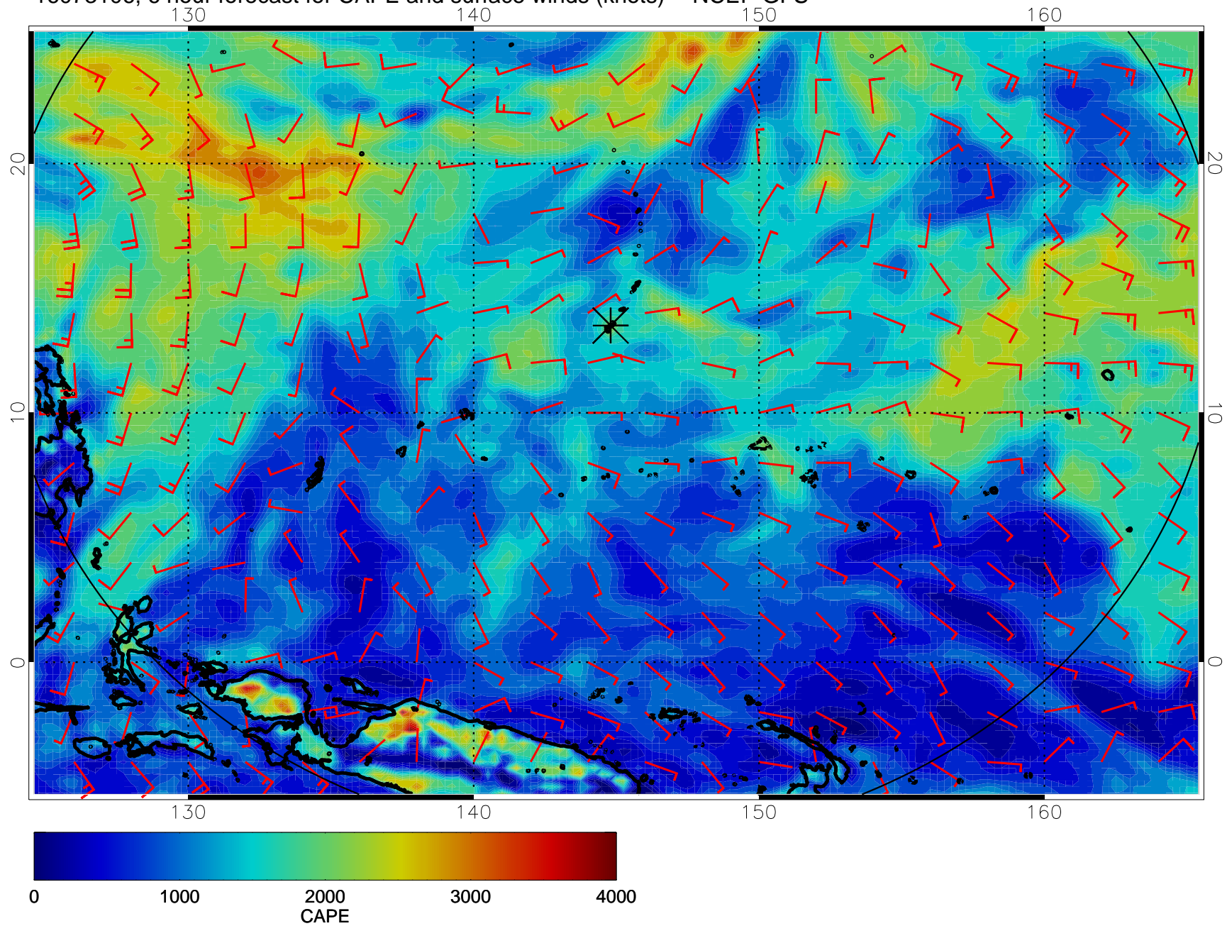
16073106, 6 hour forecast for CAPE and surface winds (knots) -- NCEP GFS
