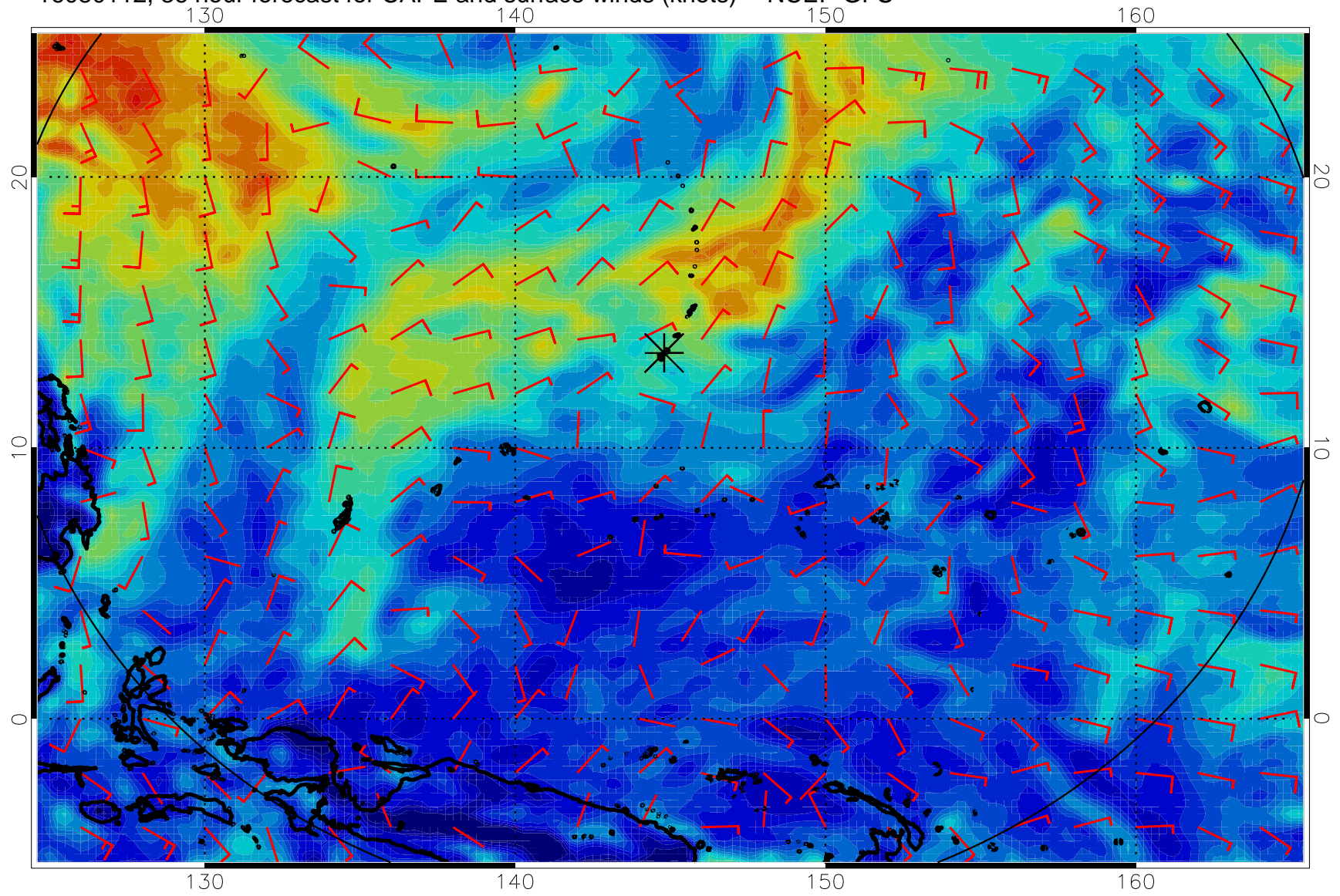
16080112, 36 hour forecast for CAPE and surface winds (knots) -- NCEP GFS
