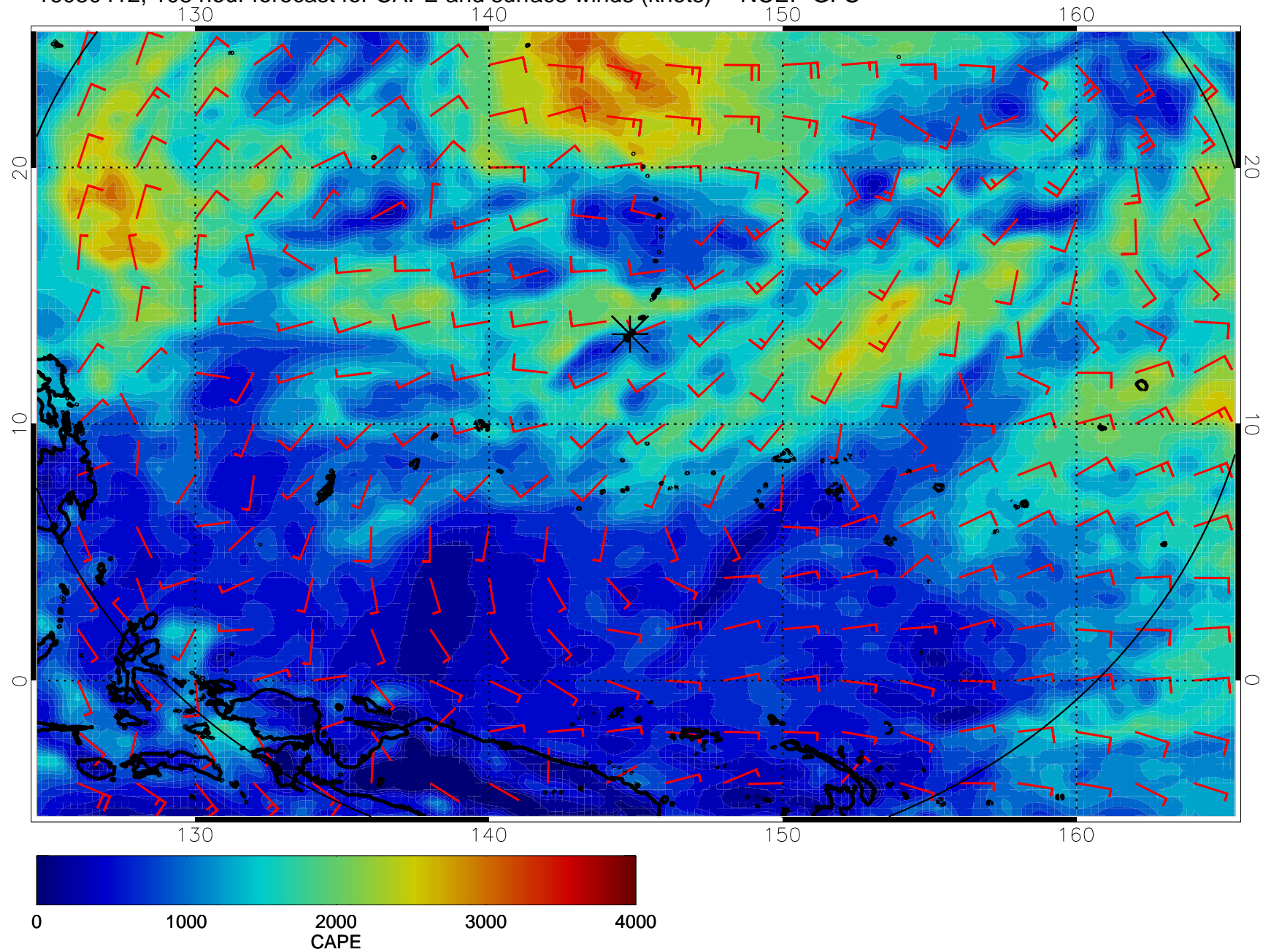
16080412, 108 hour forecast for CAPE and surface winds (knots) -- NCEP GFS
