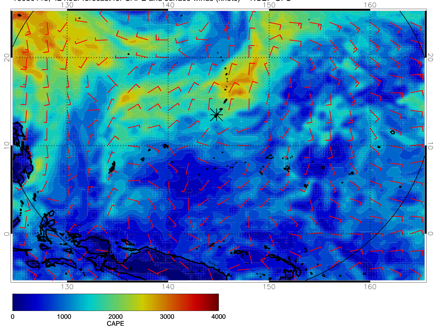
16080118, 42 hour forecast for CAPE and surface winds (knots) -- NCEP GFS
