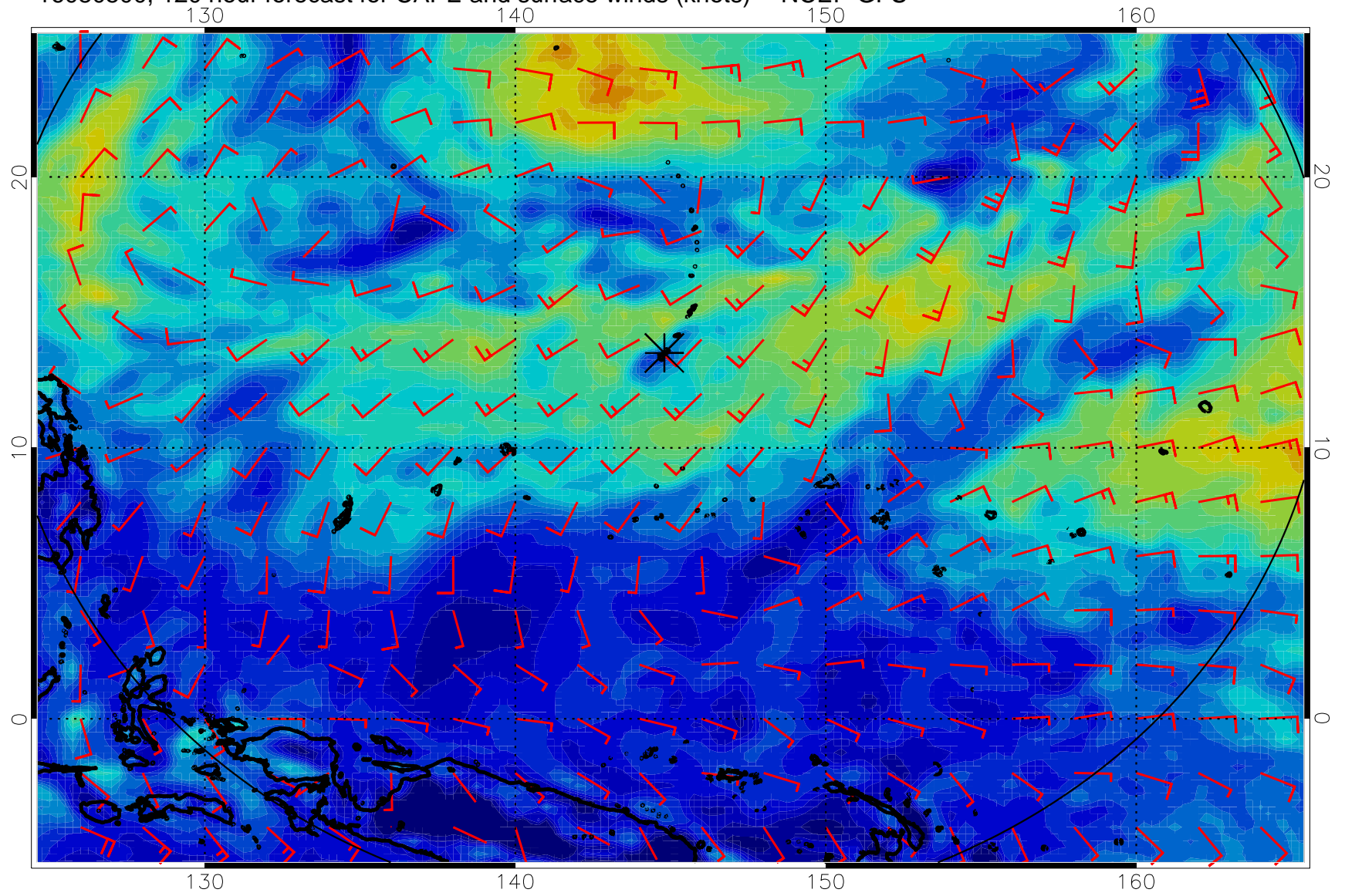
16080500, 120 hour forecast for CAPE and surface winds (knots) -- NCEP GFS
