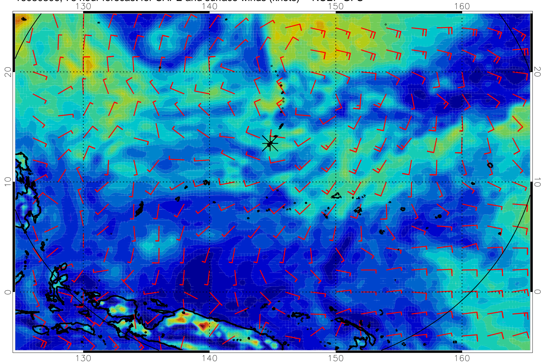
16080306, 78 hour forecast for CAPE and surface winds (knots) -- NCEP GFS
