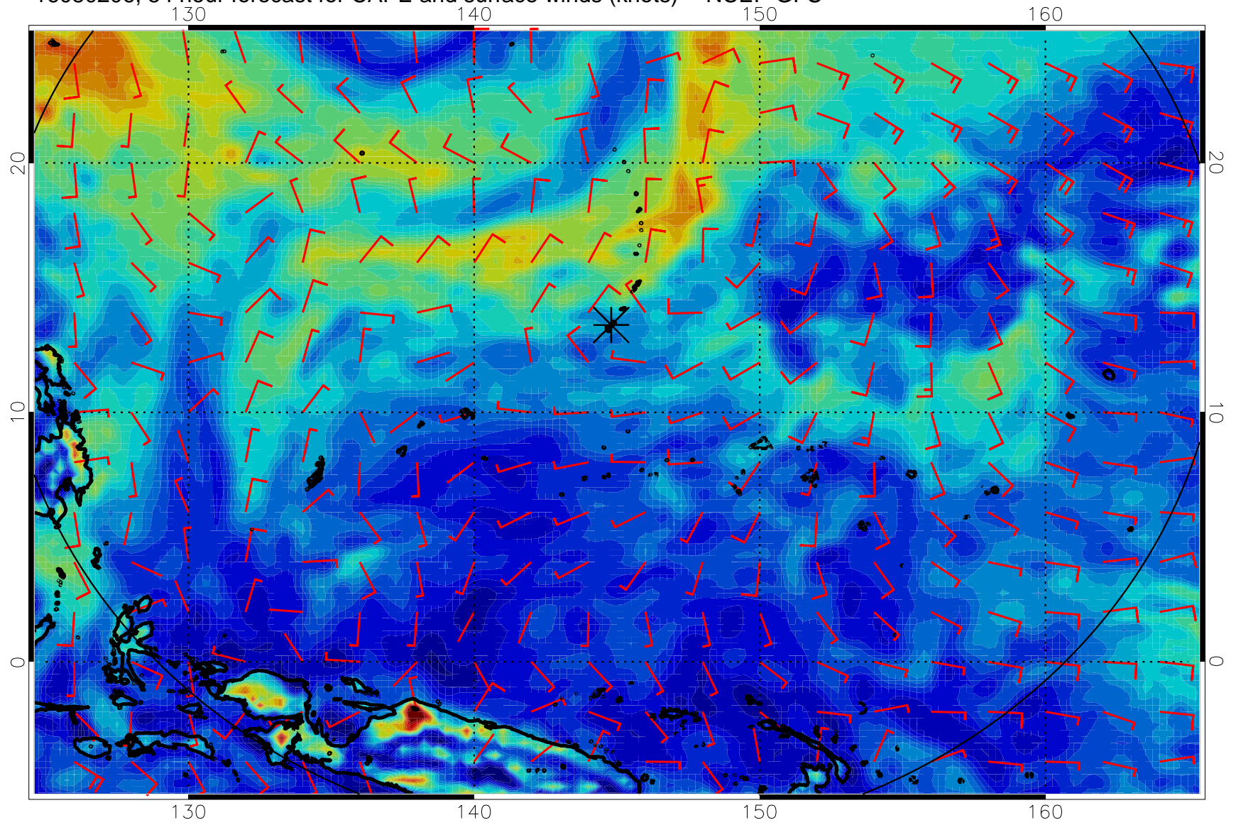
16080206, 54 hour forecast for CAPE and surface winds (knots) -- NCEP GFS
