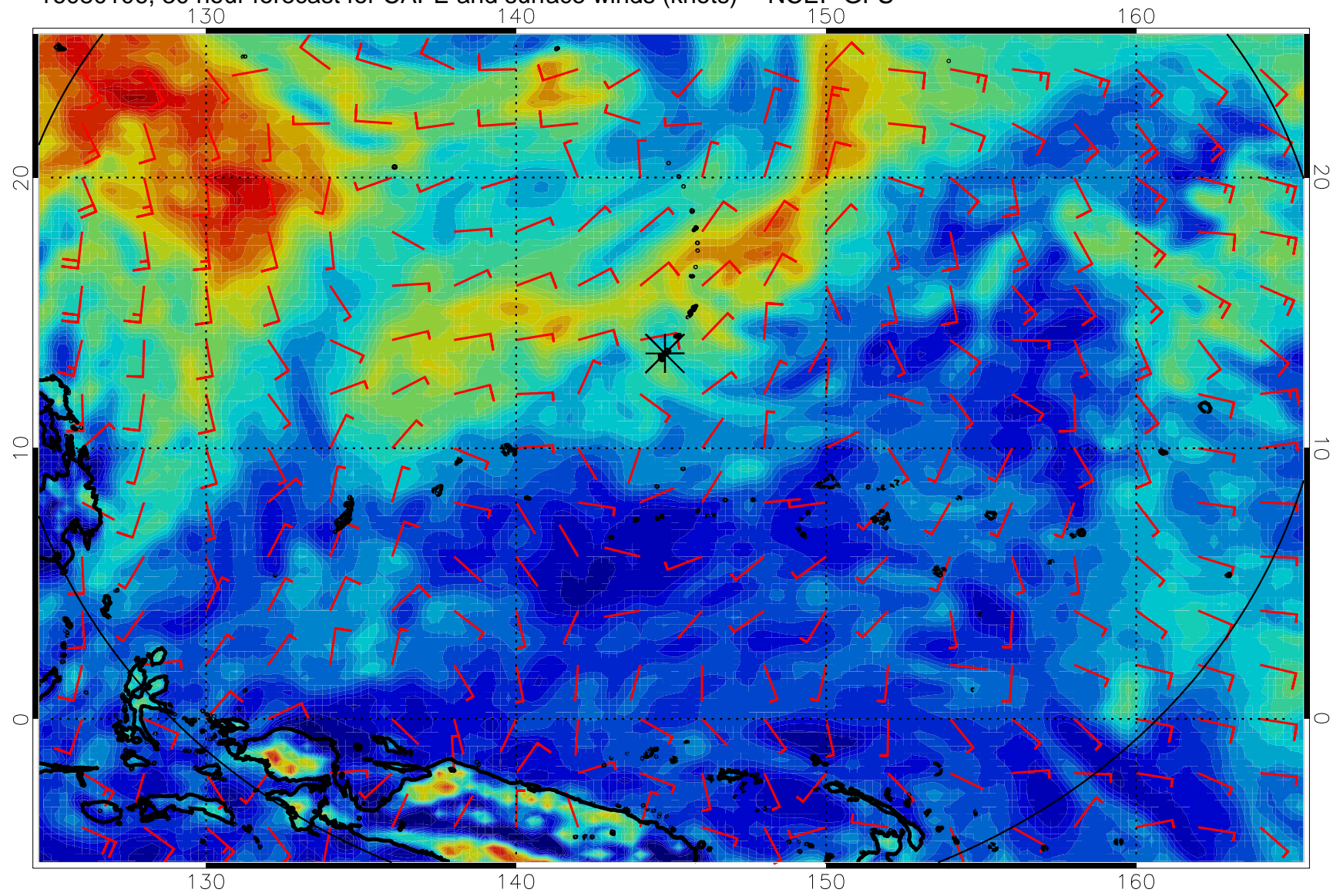
16080106, 30 hour forecast for CAPE and surface winds (knots) -- NCEP GFS
