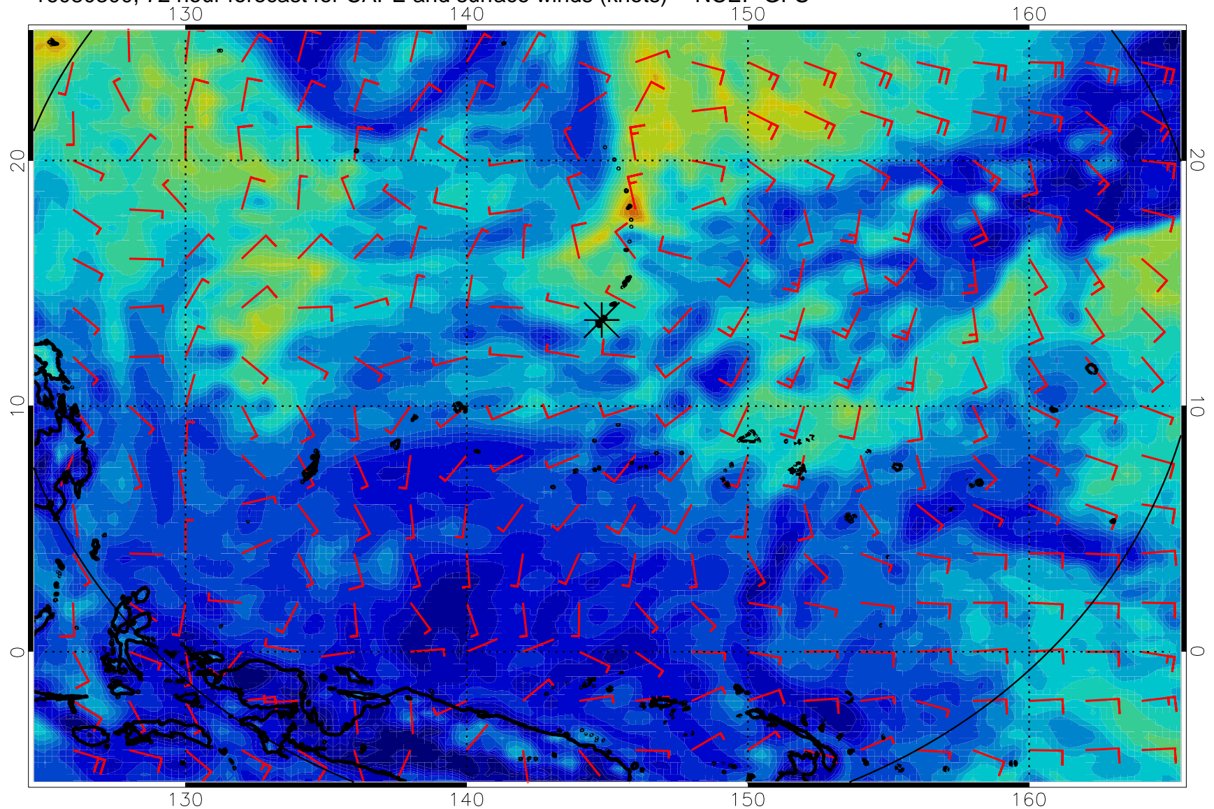
16080300, 72 hour forecast for CAPE and surface winds (knots) -- NCEP GFS
