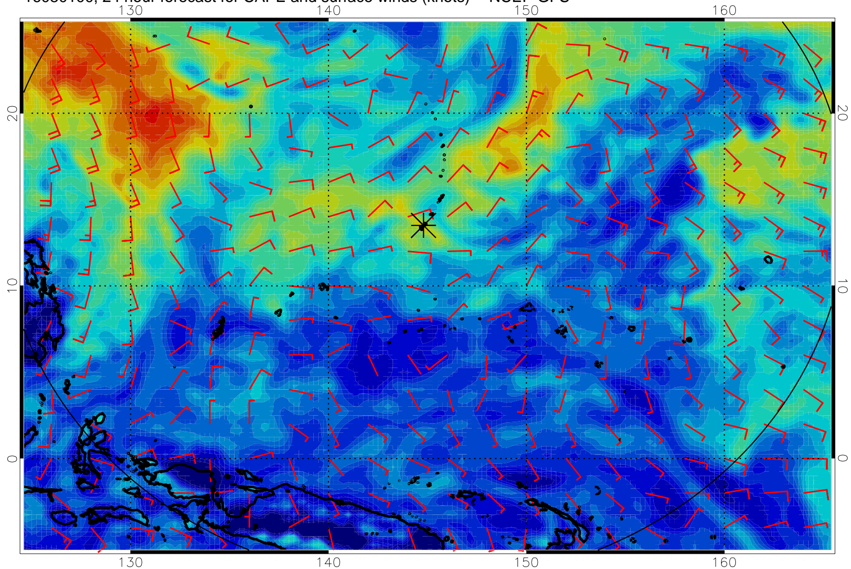
16080100, 24 hour forecast for CAPE and surface winds (knots) -- NCEP GFS
