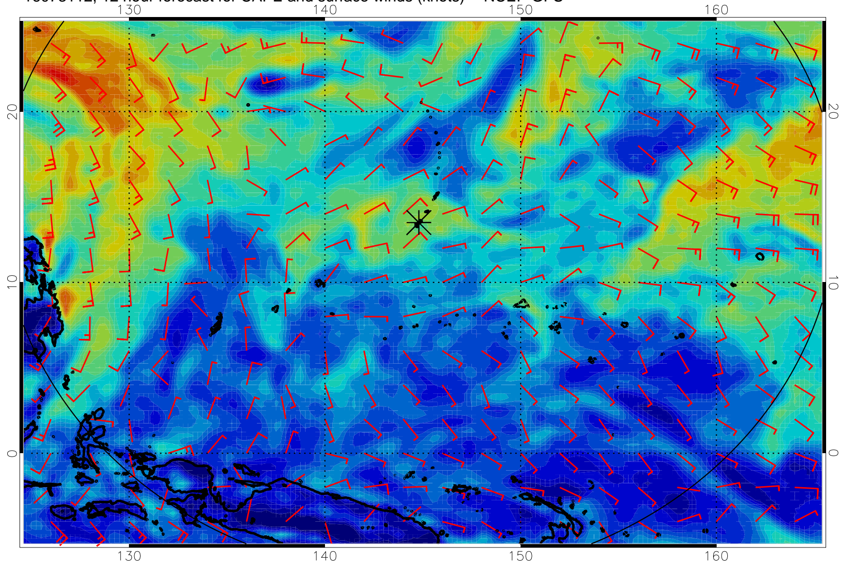
16073112, 12 hour forecast for CAPE and surface winds (knots) -- NCEP GFS
