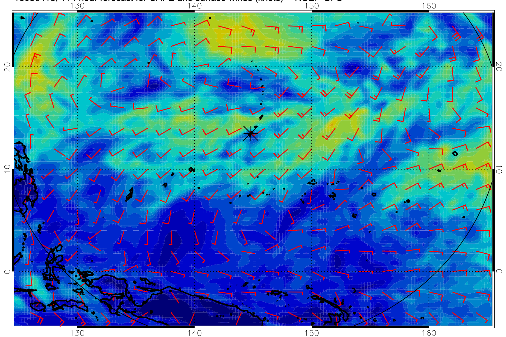
16080418, 114 hour forecast for CAPE and surface winds (knots) -- NCEP GFS
