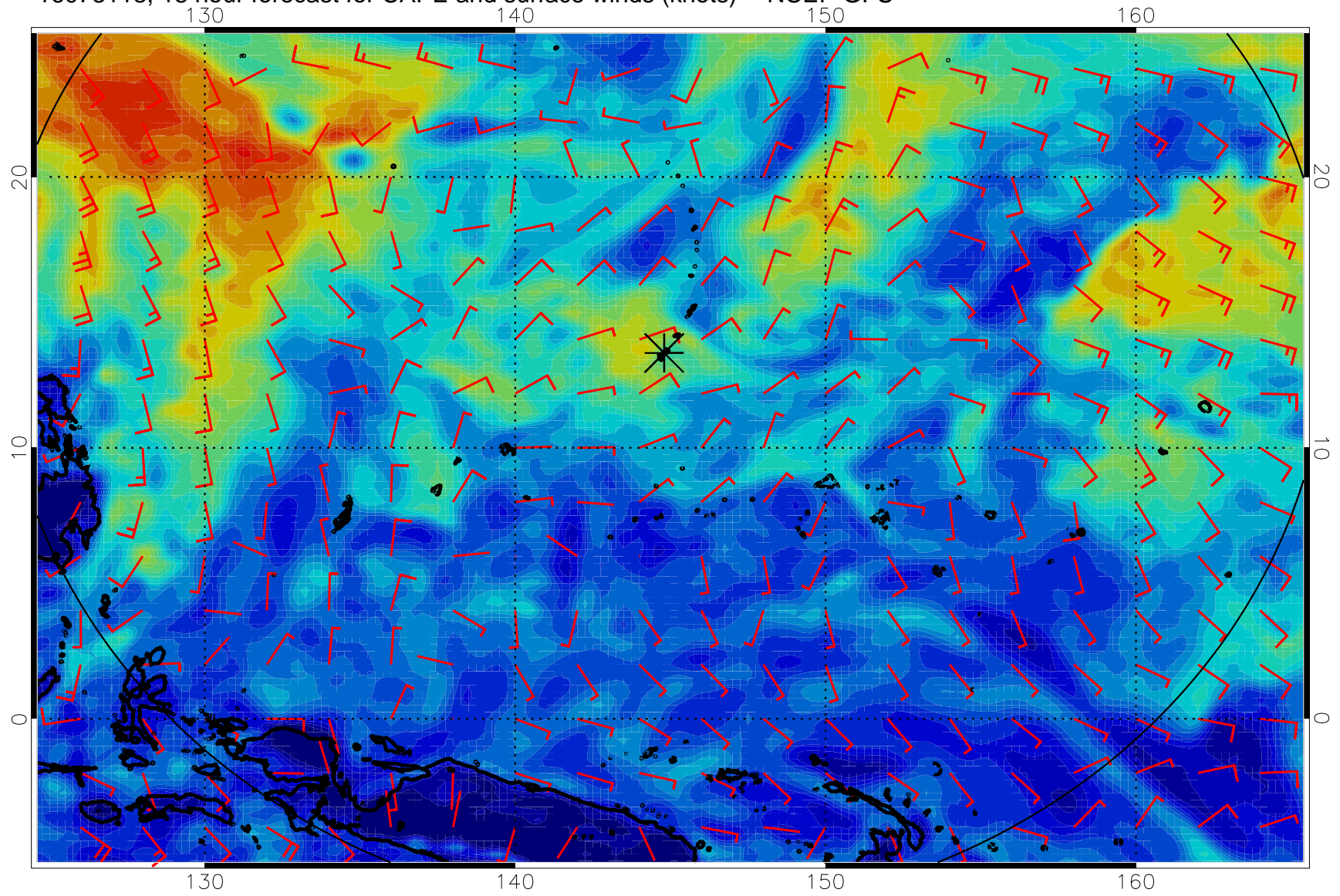
16073118, 18 hour forecast for CAPE and surface winds (knots) -- NCEP GFS
