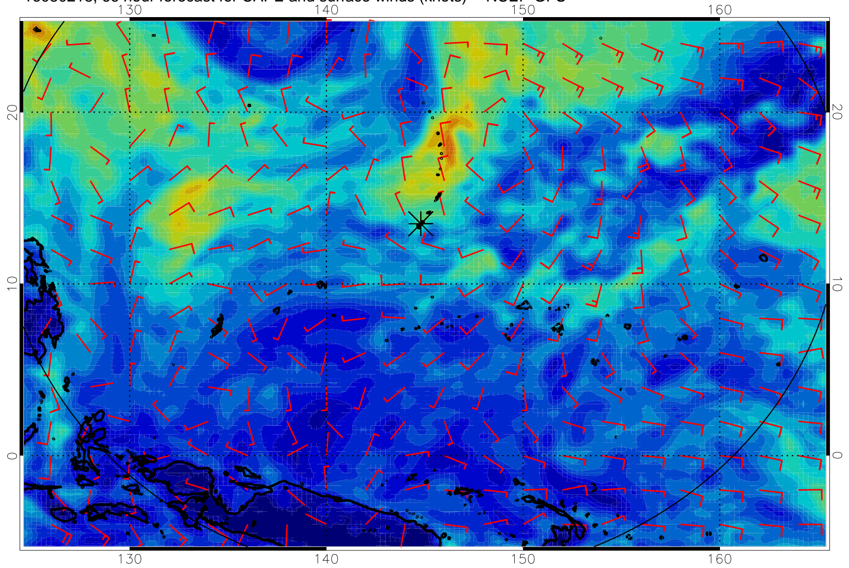
16080218, 66 hour forecast for CAPE and surface winds (knots) -- NCEP GFS
