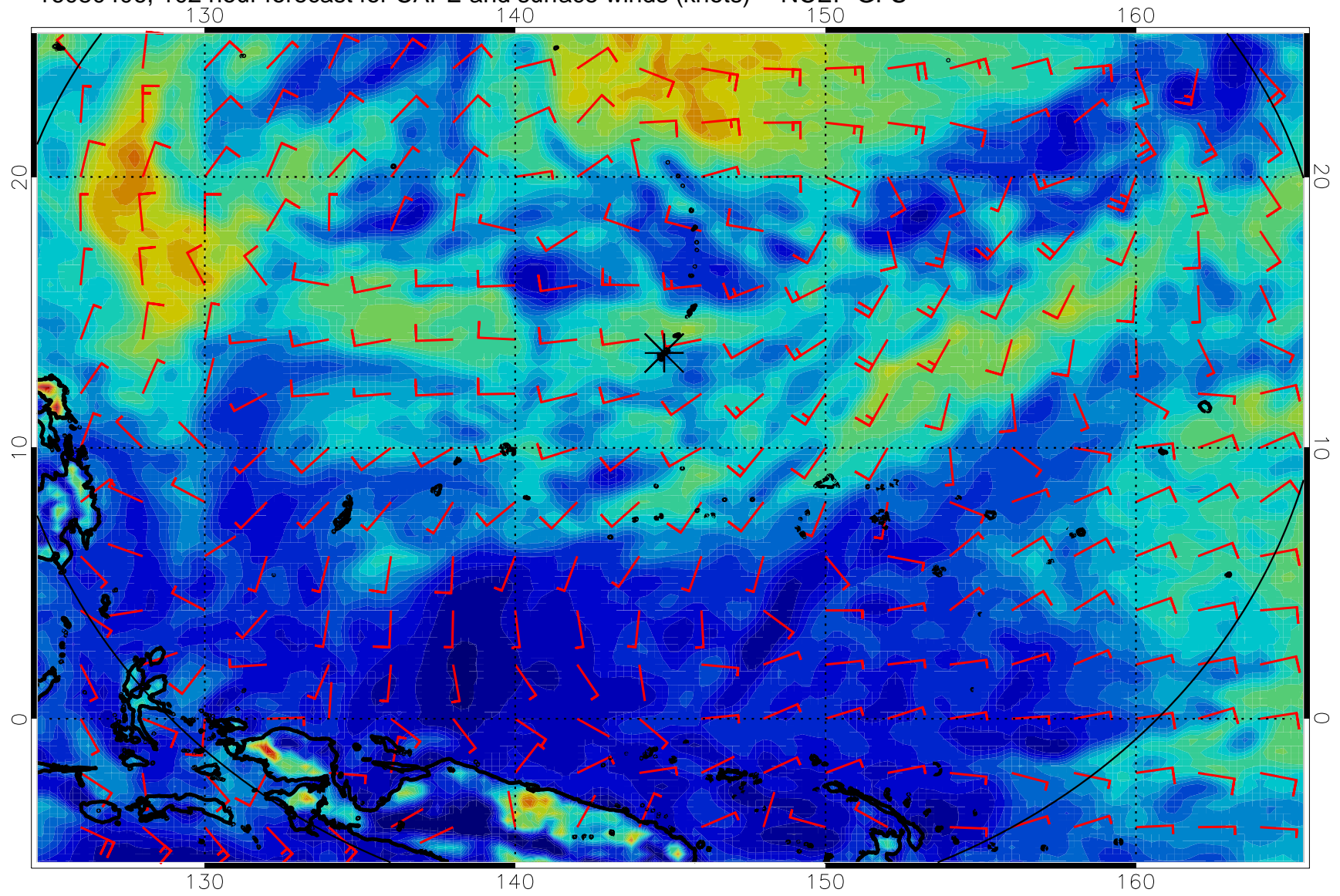
16080406, 102 hour forecast for CAPE and surface winds (knots) -- NCEP GFS
