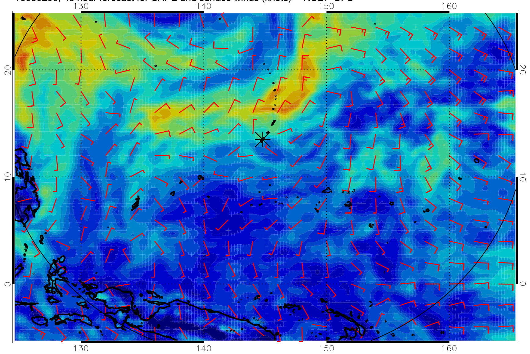
16080200, 48 hour forecast for CAPE and surface winds (knots) -- NCEP GFS
