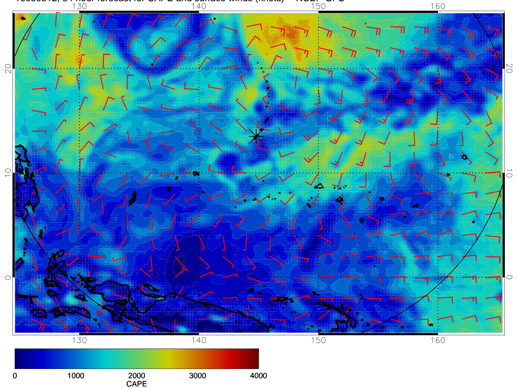
16080312, 84 hour forecast for CAPE and surface winds (knots) -- NCEP GFS
