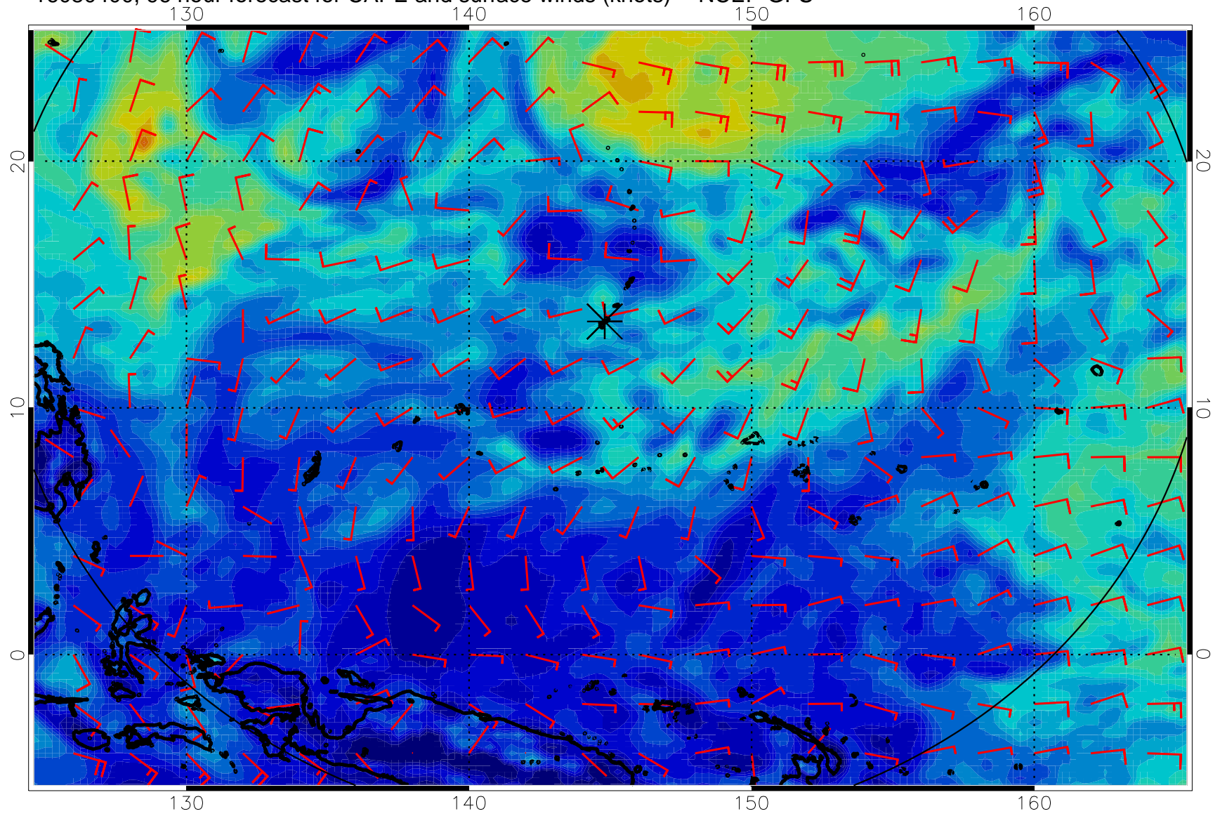
16080400, 96 hour forecast for CAPE and surface winds (knots) -- NCEP GFS
