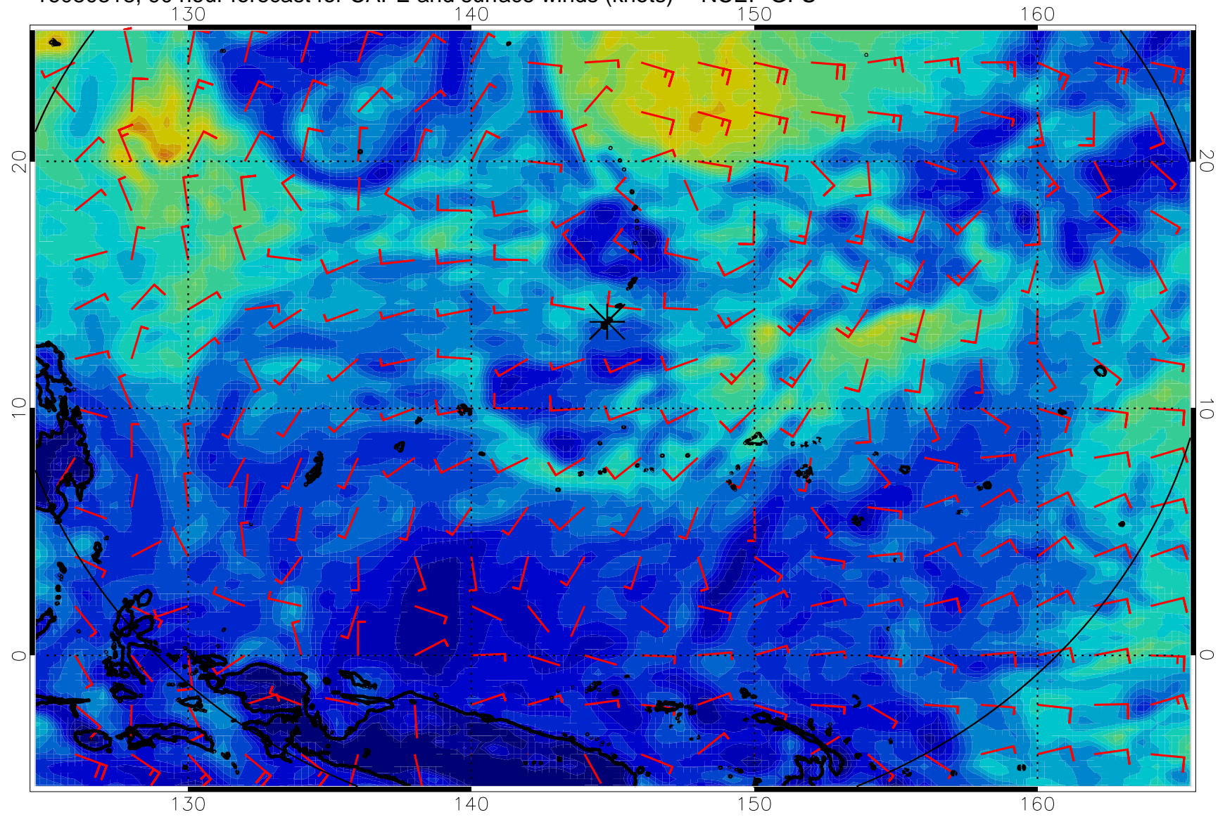
16080318, 90 hour forecast for CAPE and surface winds (knots) -- NCEP GFS
