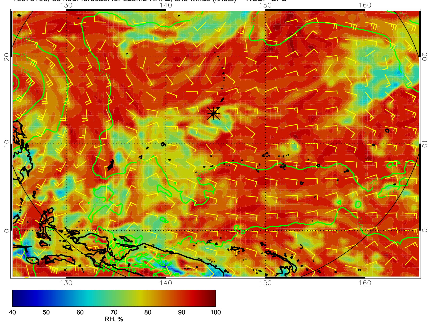
16073100, 36 hour forecast for 925mb RH, Z, and winds (knots) -- NCEP GFS
