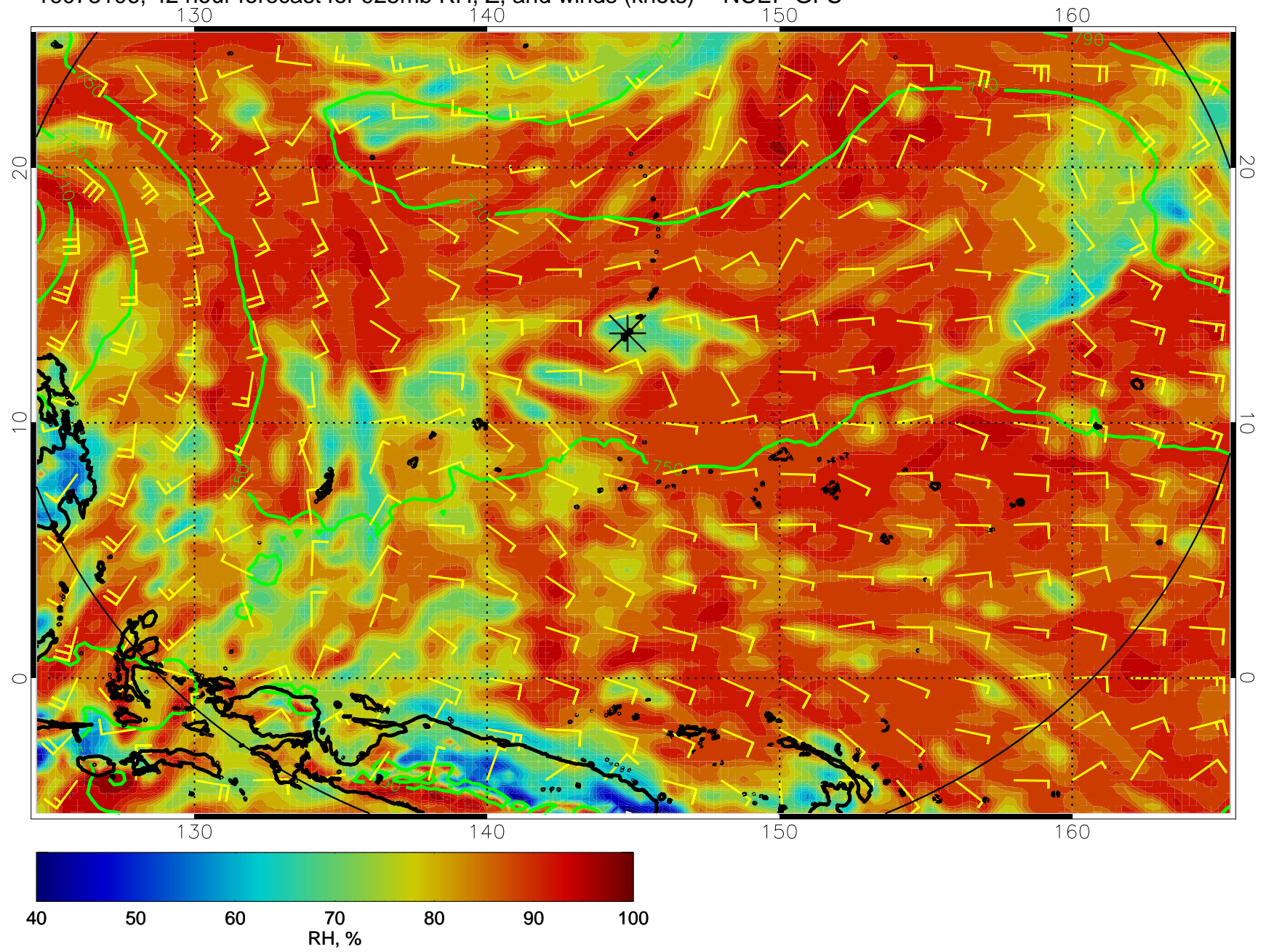
16073106, 42 hour forecast for 925mb RH, Z, and winds (knots) -- NCEP GFS
