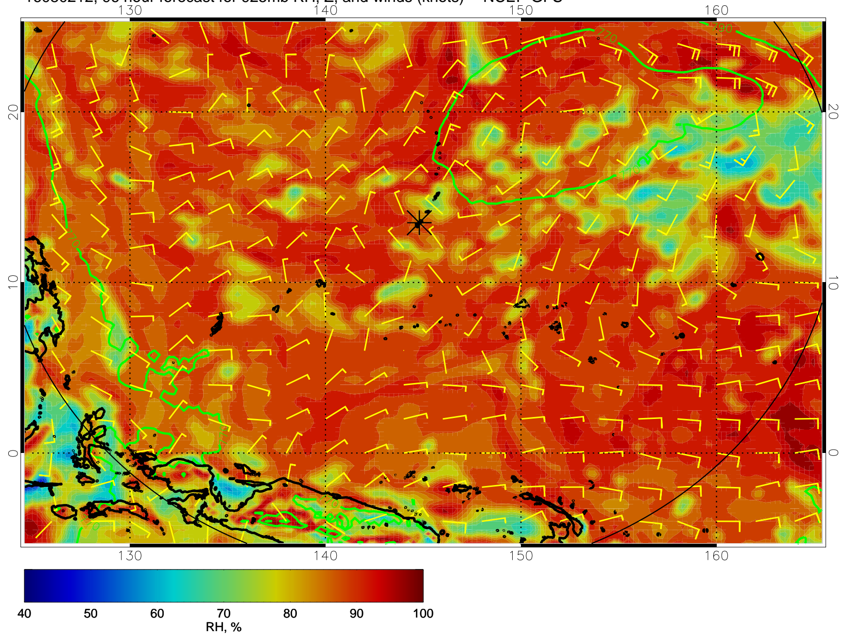
16080212, 96 hour forecast for 925mb RH, Z, and winds (knots) -- NCEP GFS
