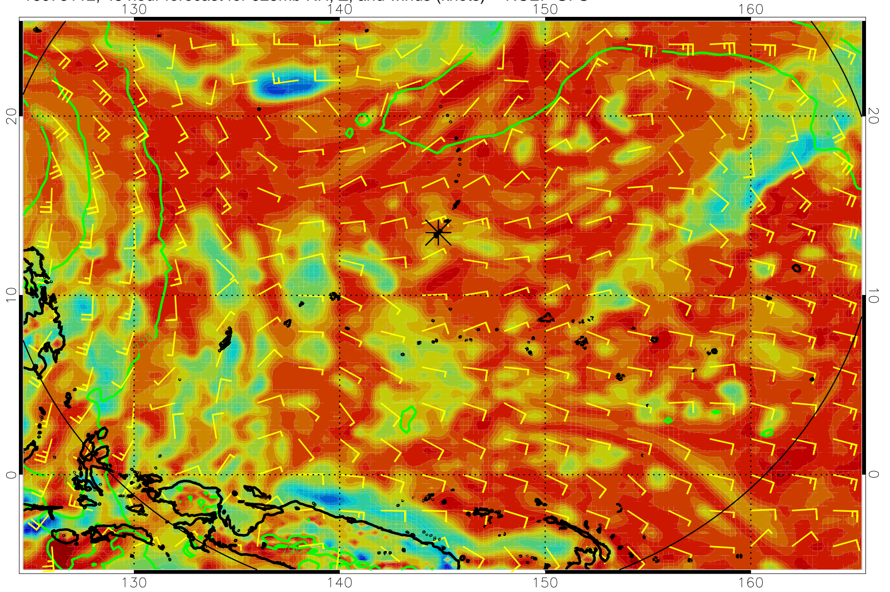
16073112, 48 hour forecast for 925mb RH, Z, and winds (knots) -- NCEP GFS
