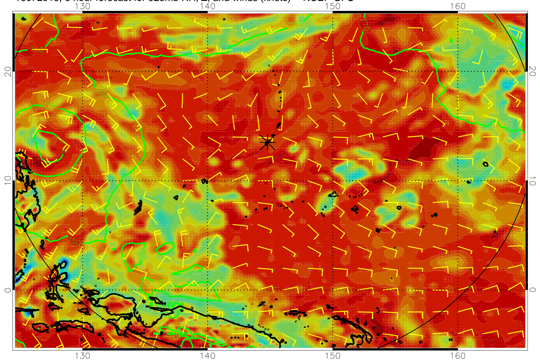
16072918, 6 hour forecast for 925mb RH, Z, and winds (knots) -- NCEP GFS
