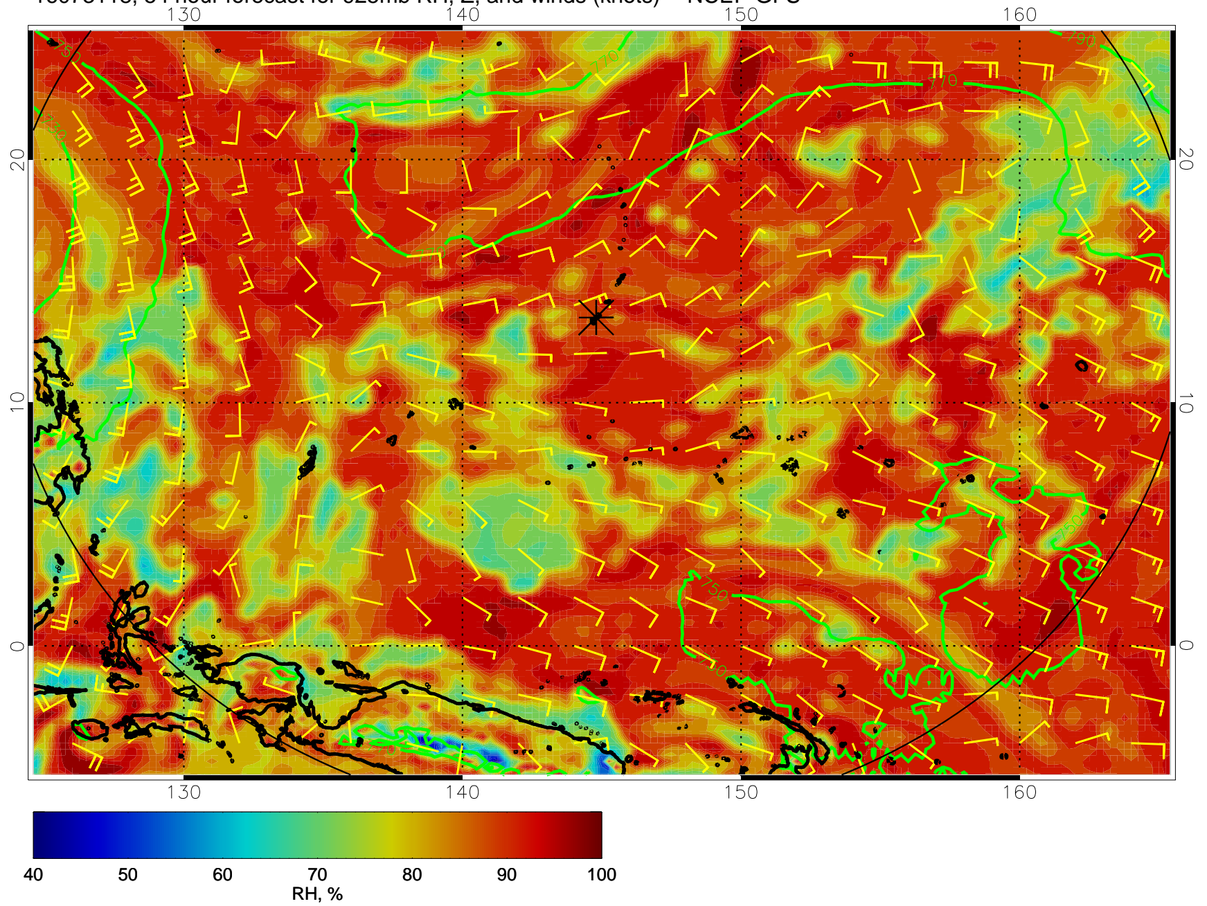
16073118, 54 hour forecast for 925mb RH, Z, and winds (knots) -- NCEP GFS
