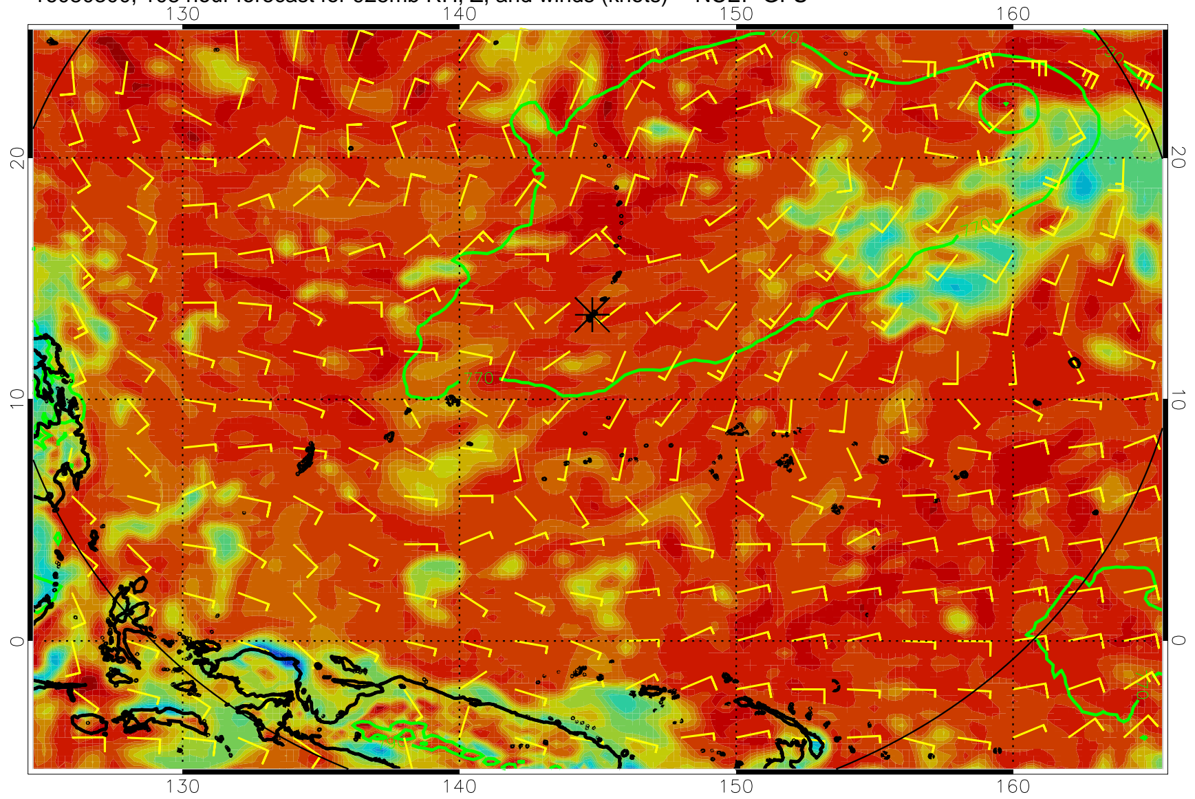
16080300, 108 hour forecast for 925mb RH, Z, and winds (knots) -- NCEP GFS
