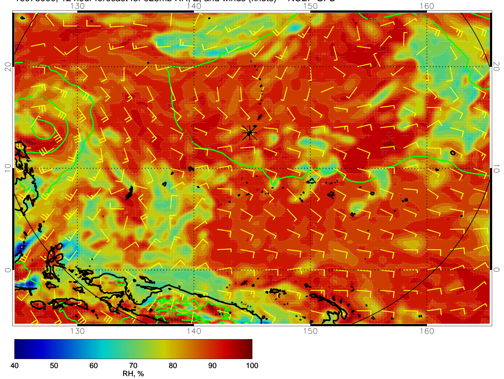
16073000, 12 hour forecast for 925mb RH, Z, and winds (knots) -- NCEP GFS
