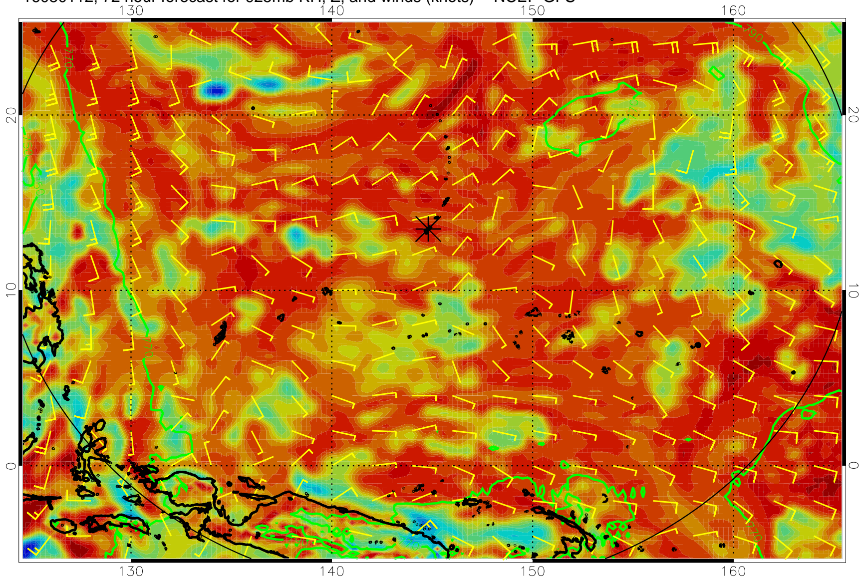
16080112, 72 hour forecast for 925mb RH, Z, and winds (knots) -- NCEP GFS
