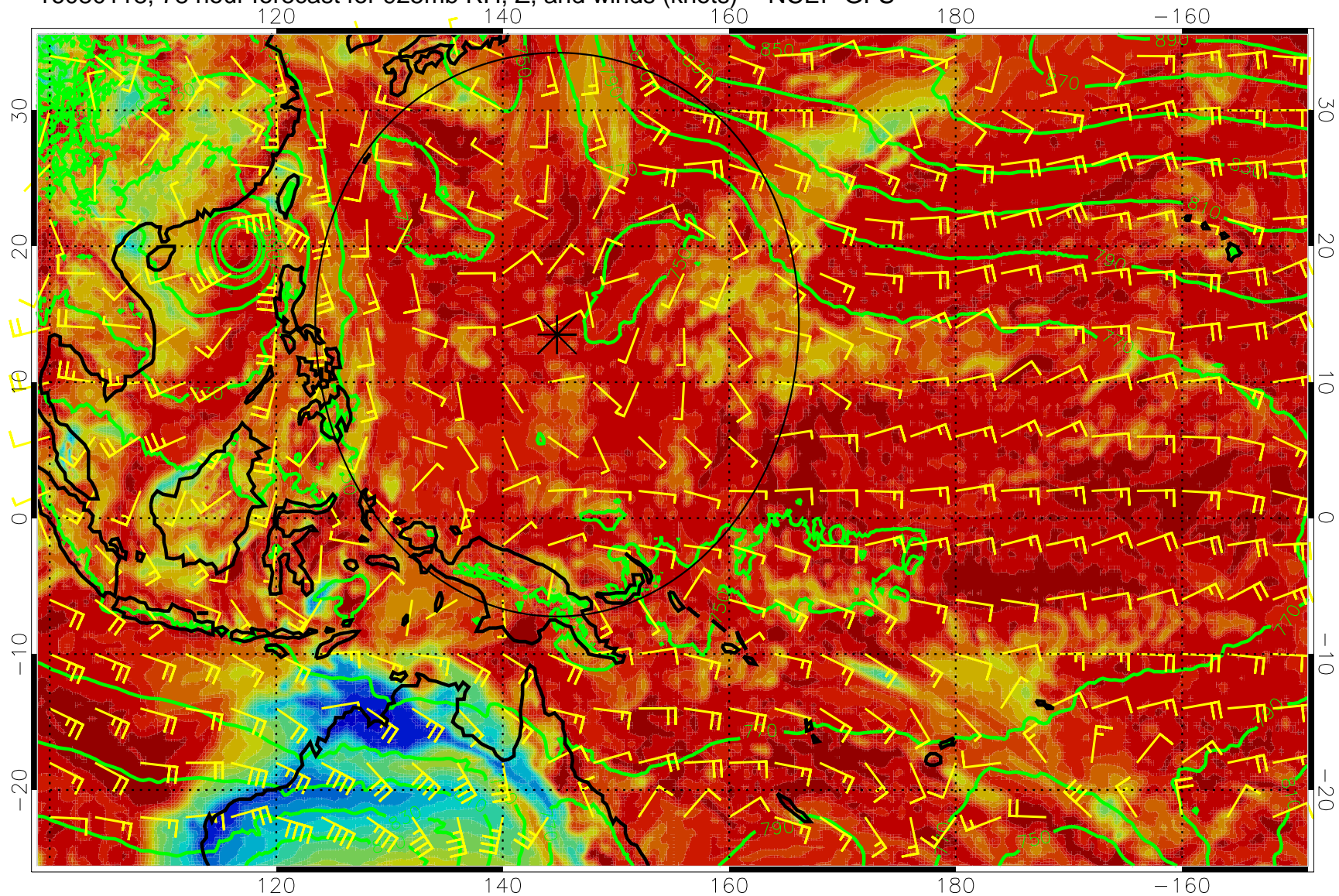
16080118, 78 hour forecast for 925mb RH, Z, and winds (knots) -- NCEP GFS
