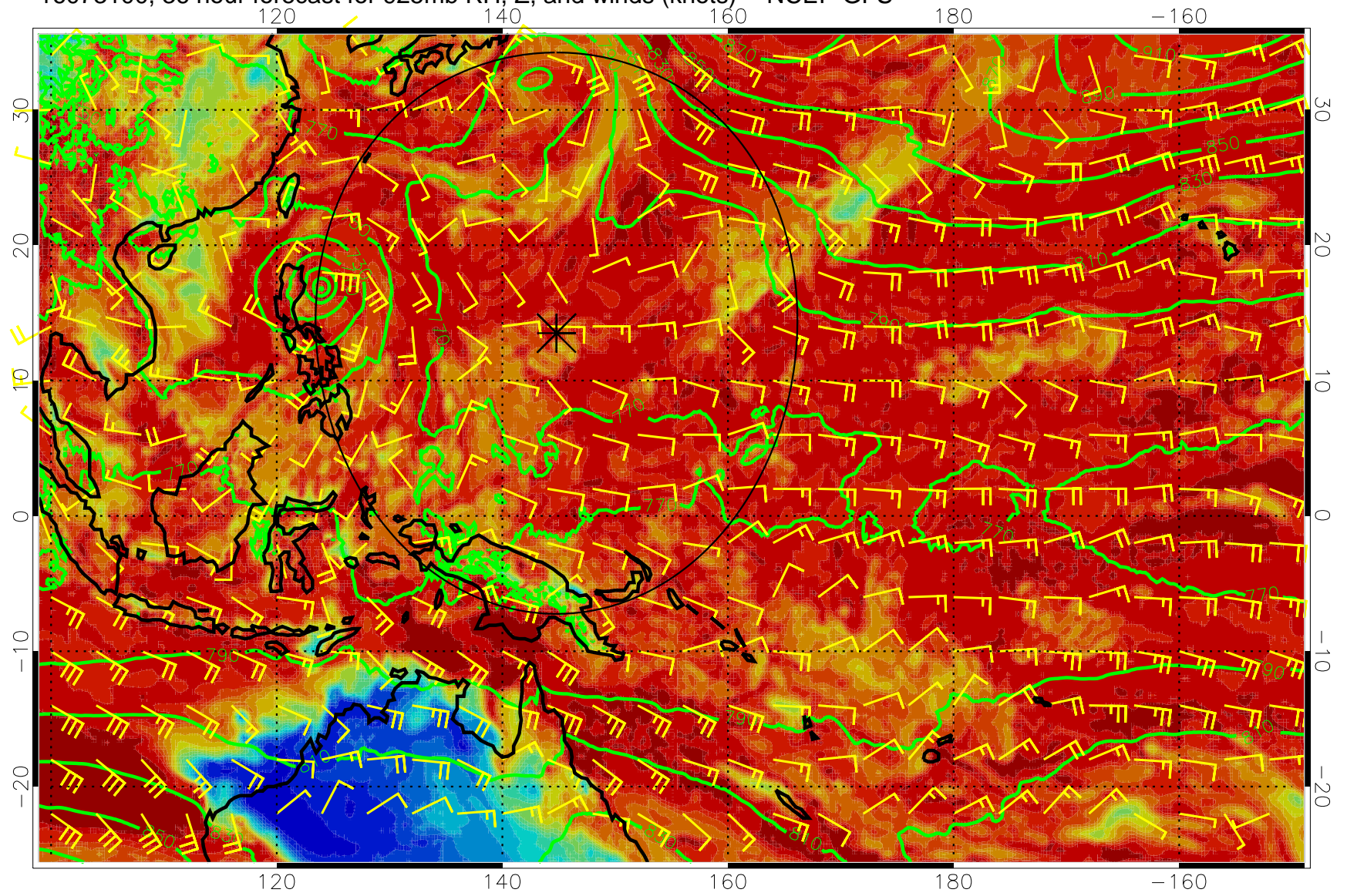
16073100, 36 hour forecast for 925mb RH, Z, and winds (knots) -- NCEP GFS
