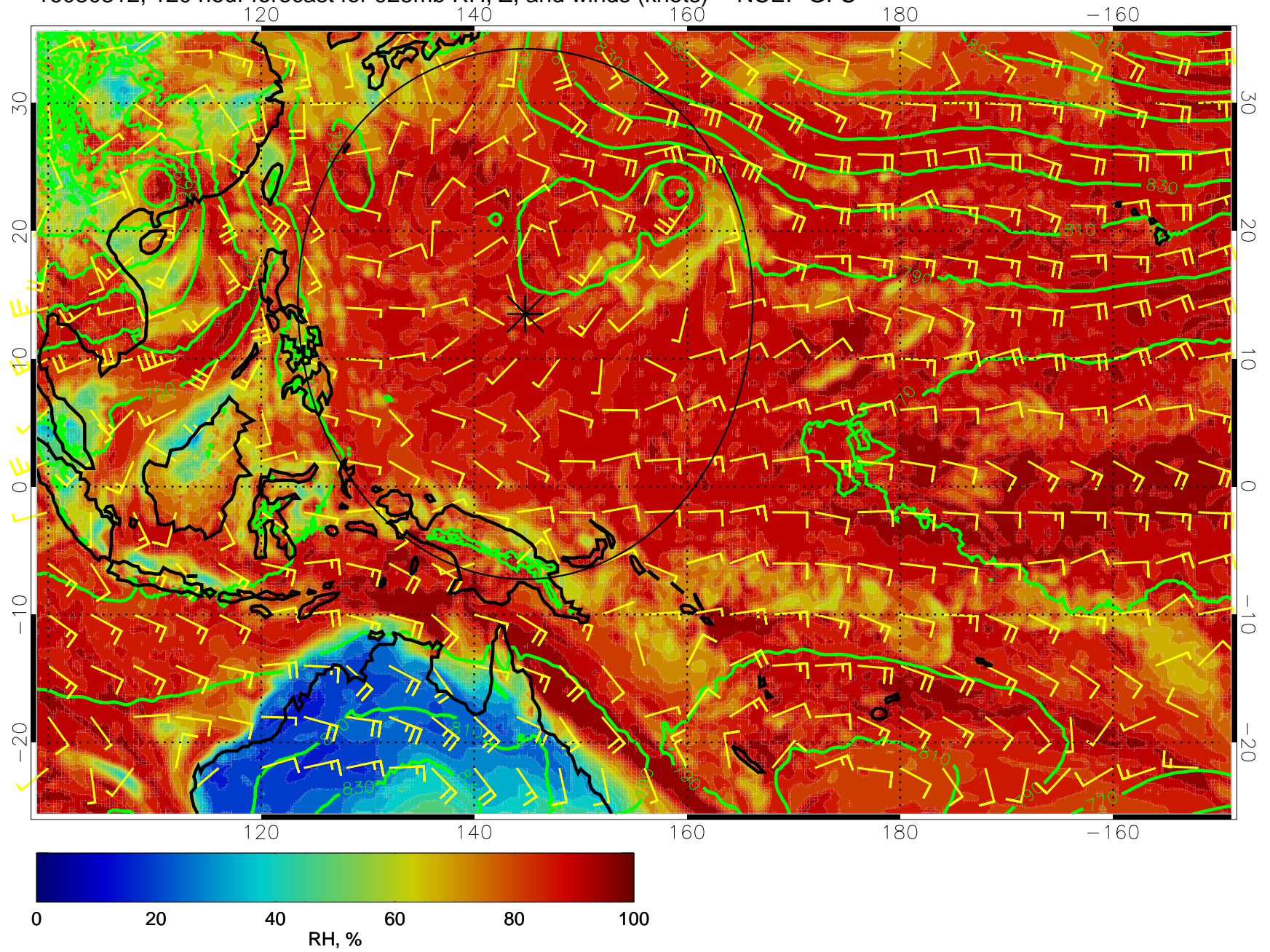
16080312, 120 hour forecast for 925mb RH, Z, and winds (knots) -- NCEP GFS
