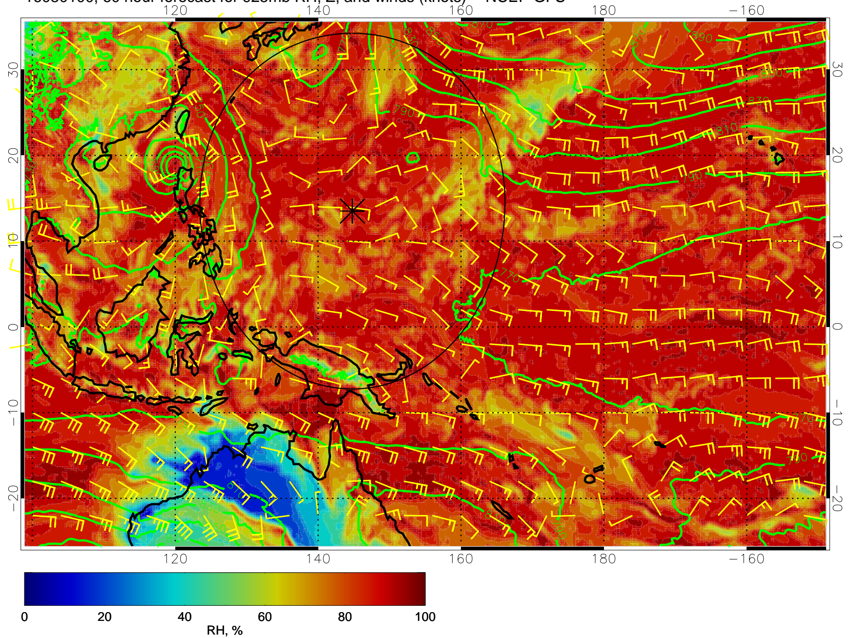
16080100, 60 hour forecast for 925mb RH, Z, and winds (knots) -- NCEP GFS
