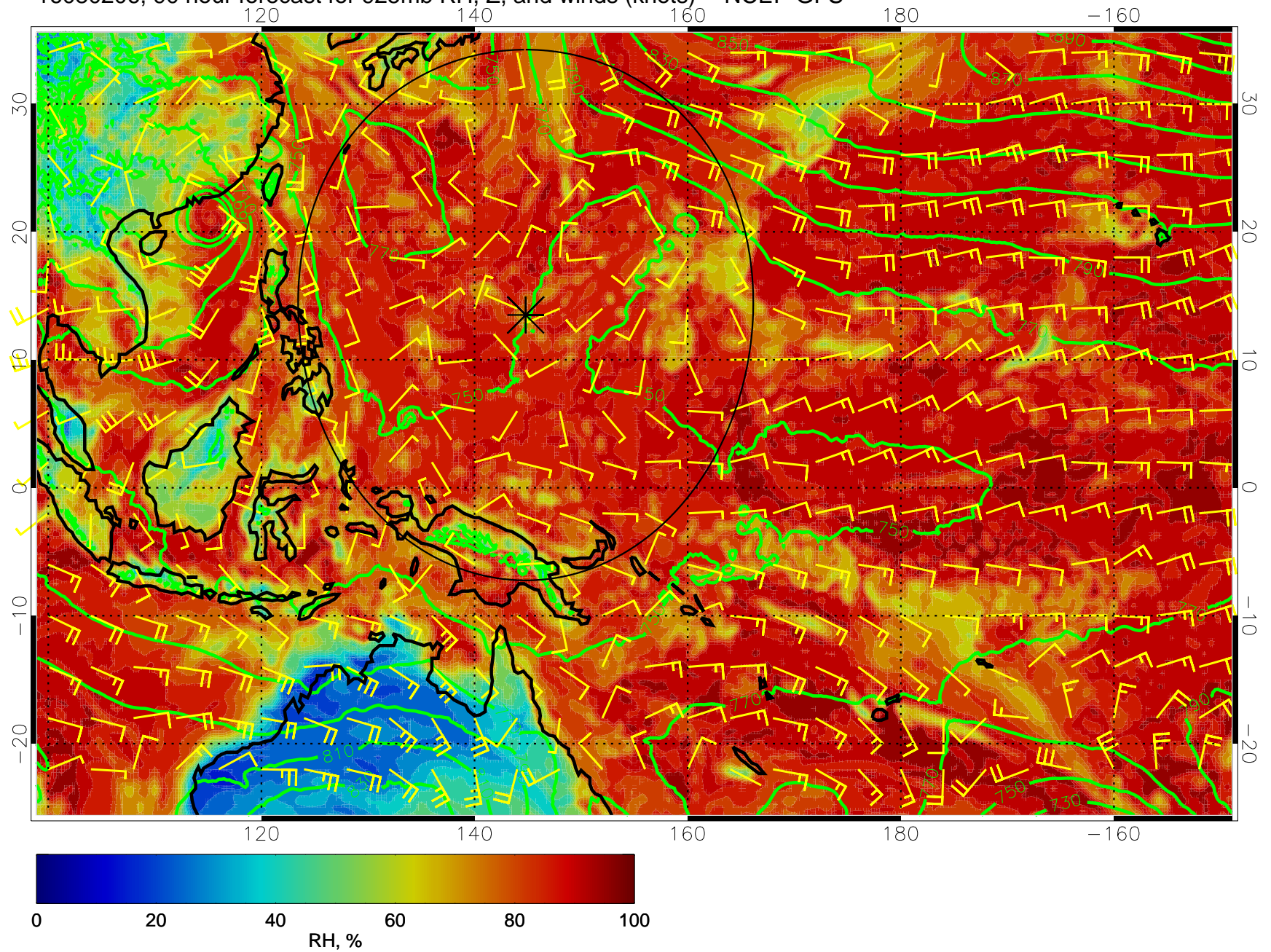
16080206, 90 hour forecast for 925mb RH, Z, and winds (knots) -- NCEP GFS
