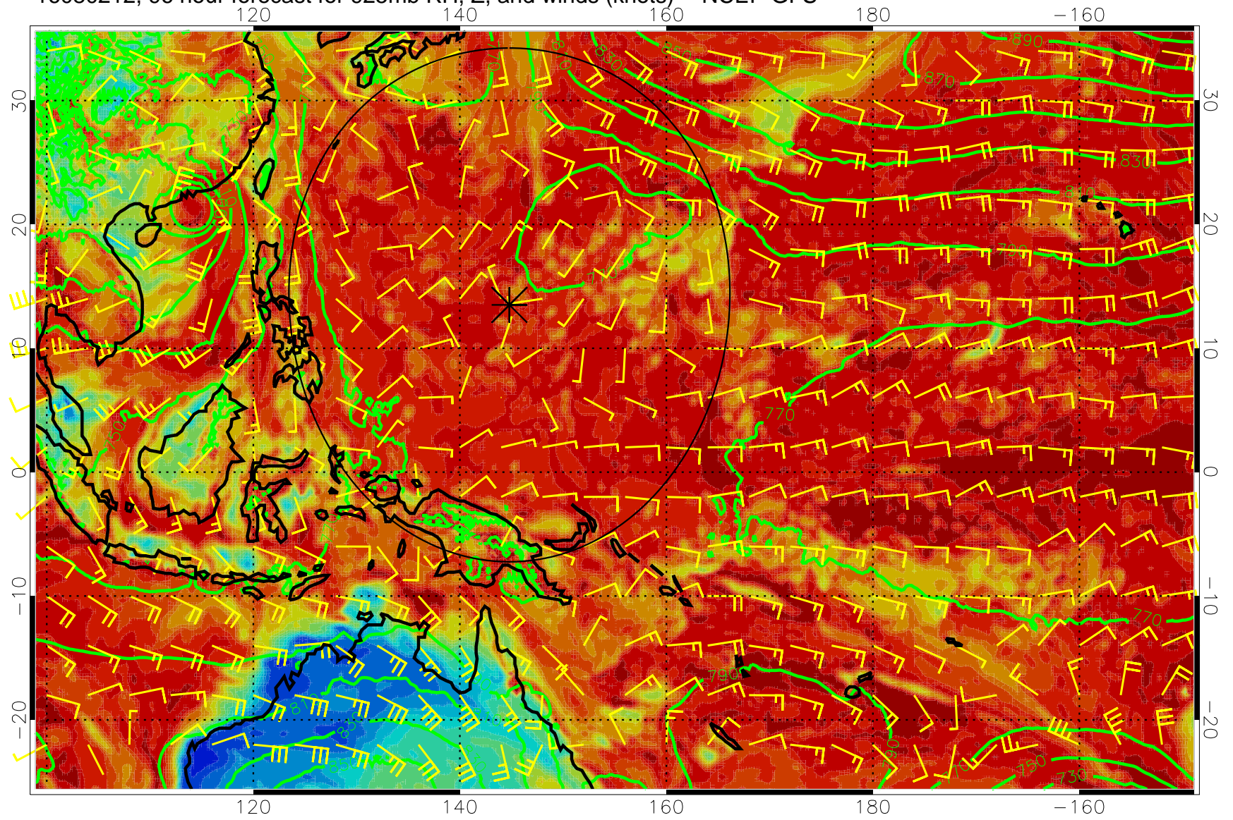
16080212, 96 hour forecast for 925mb RH, Z, and winds (knots) -- NCEP GFS
