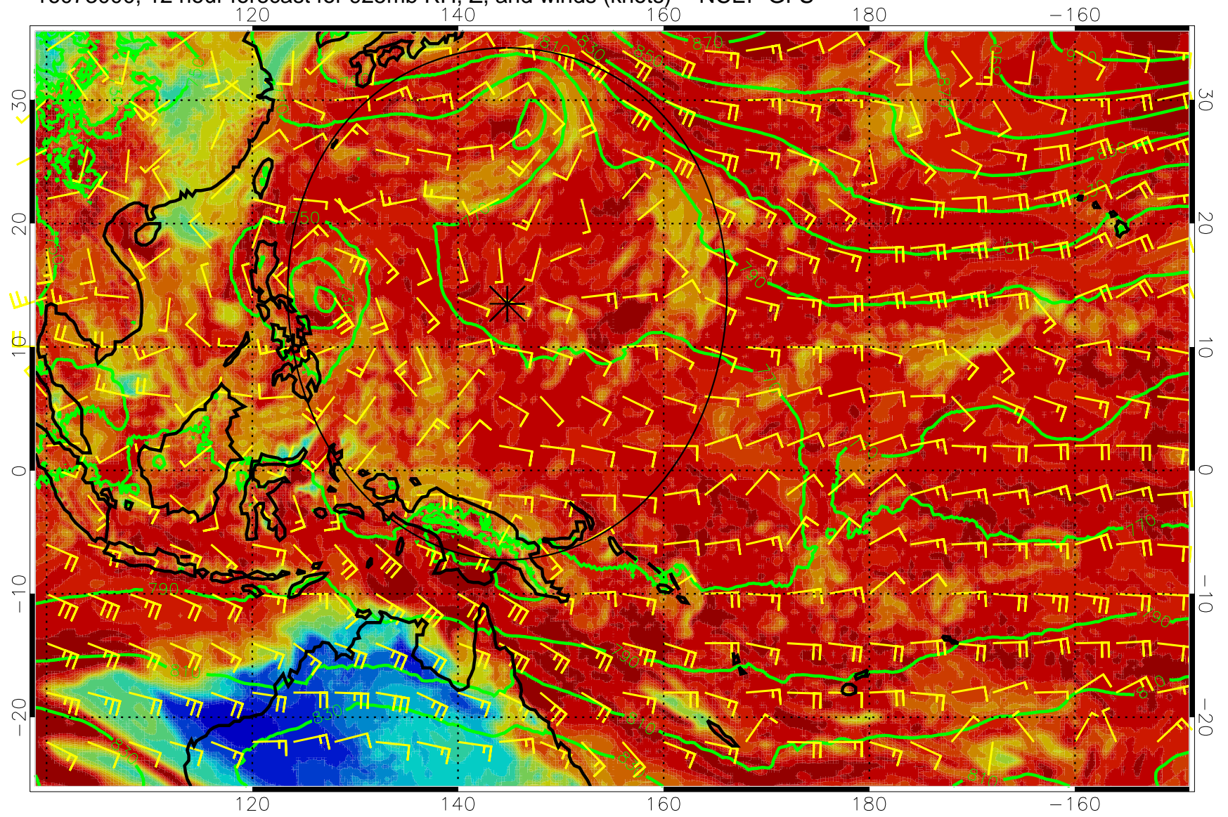
16073000, 12 hour forecast for 925mb RH, Z, and winds (knots) -- NCEP GFS
