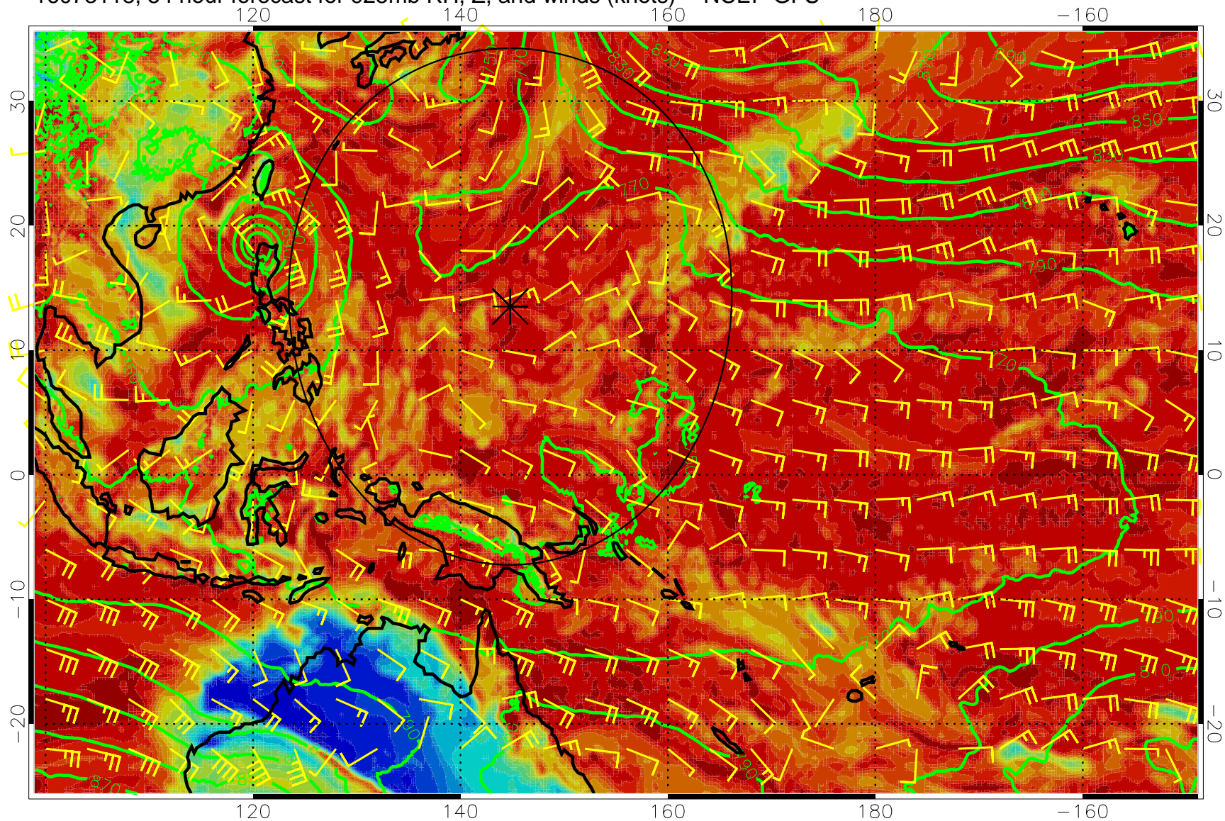
16073118, 54 hour forecast for 925mb RH, Z, and winds (knots) -- NCEP GFS
