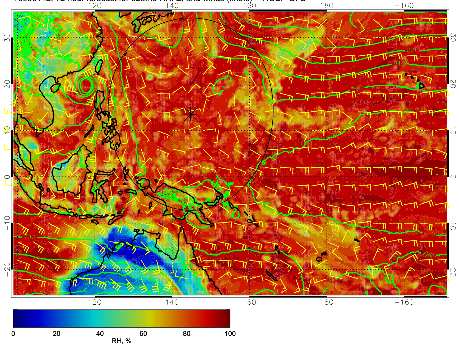
16080112, 72 hour forecast for 925mb RH, Z, and winds (knots) -- NCEP GFS
