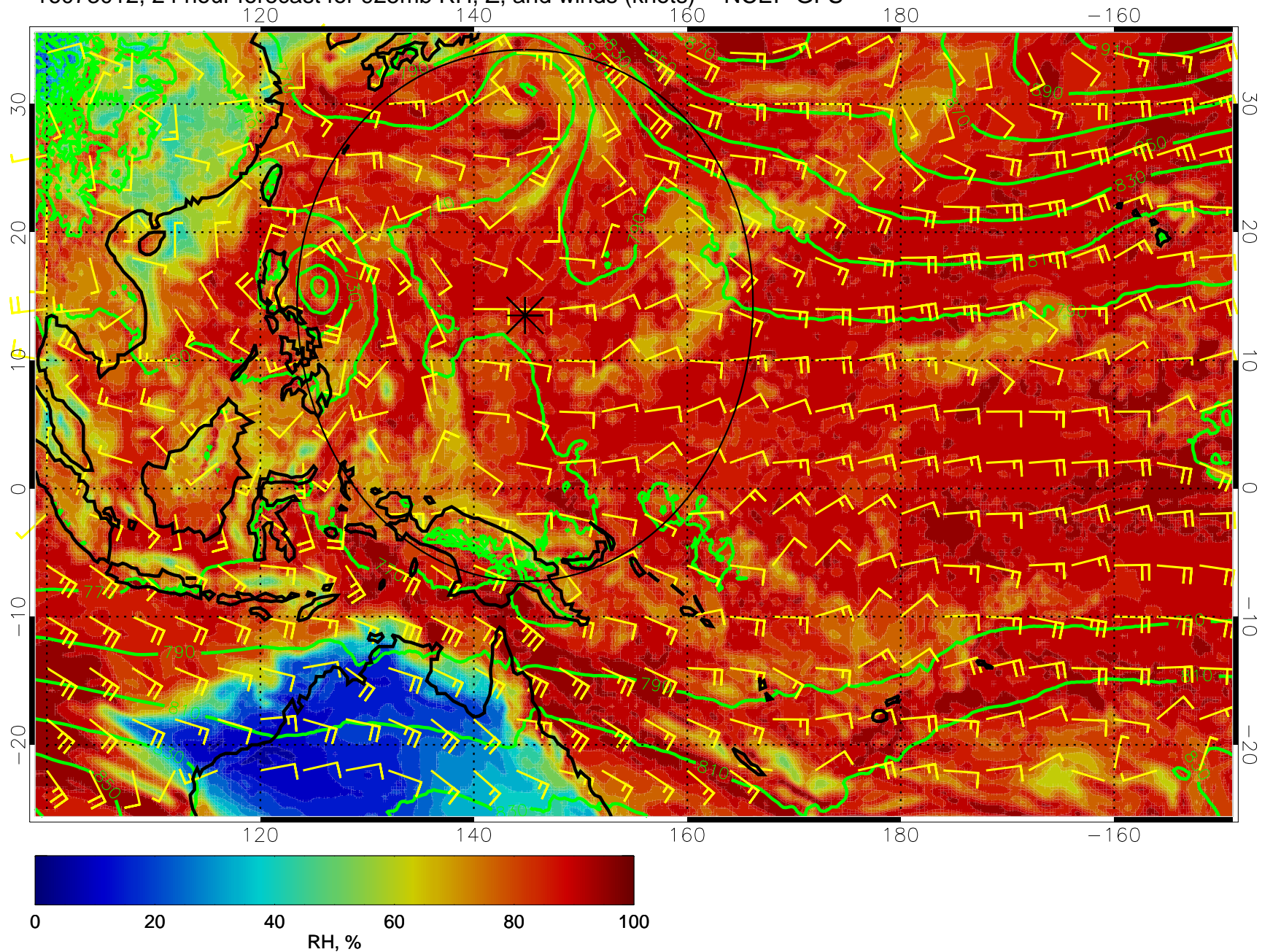
16073012, 24 hour forecast for 925mb RH, Z, and winds (knots) -- NCEP GFS
