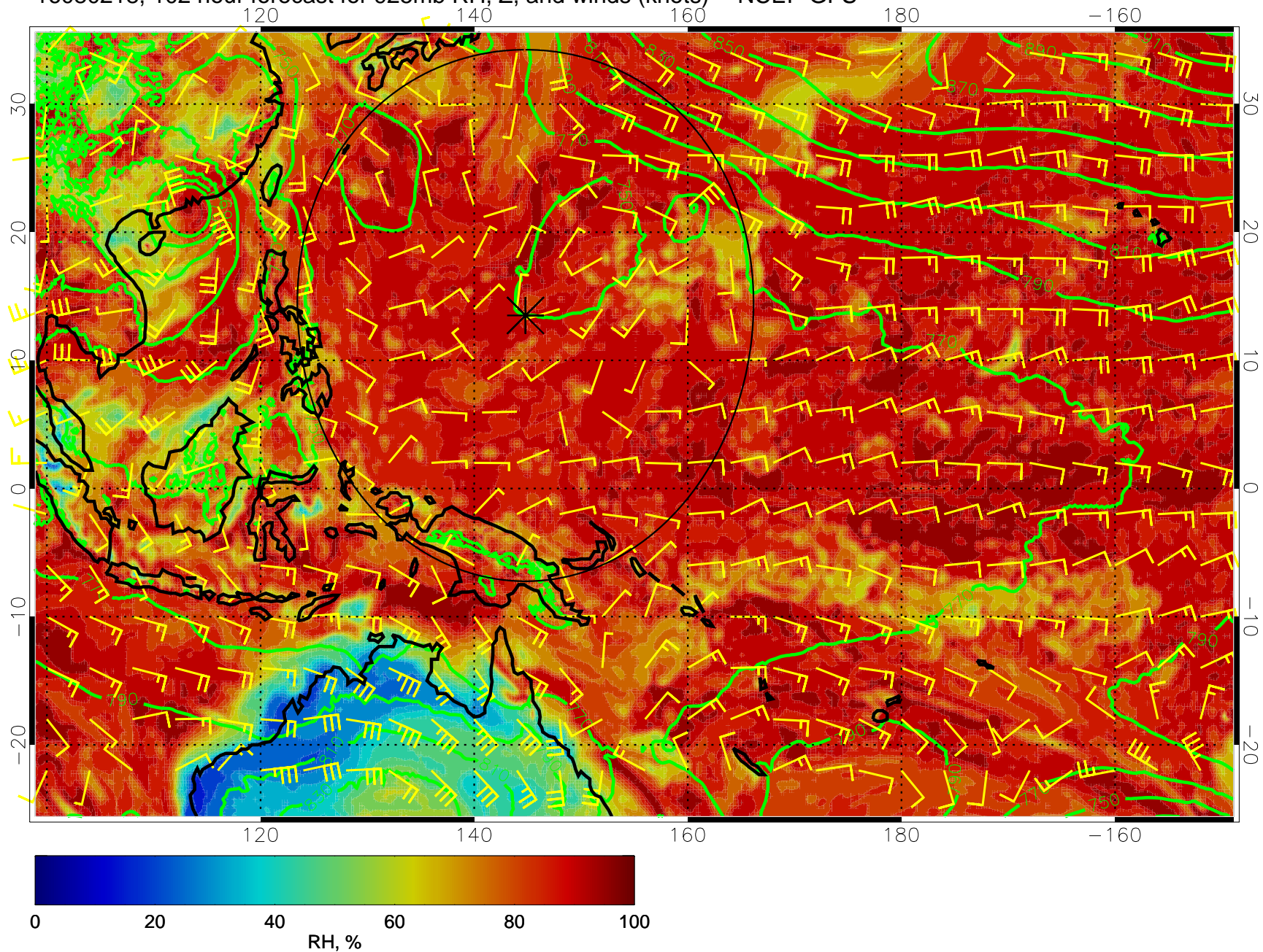
16080218, 102 hour forecast for 925mb RH, Z, and winds (knots) -- NCEP GFS
