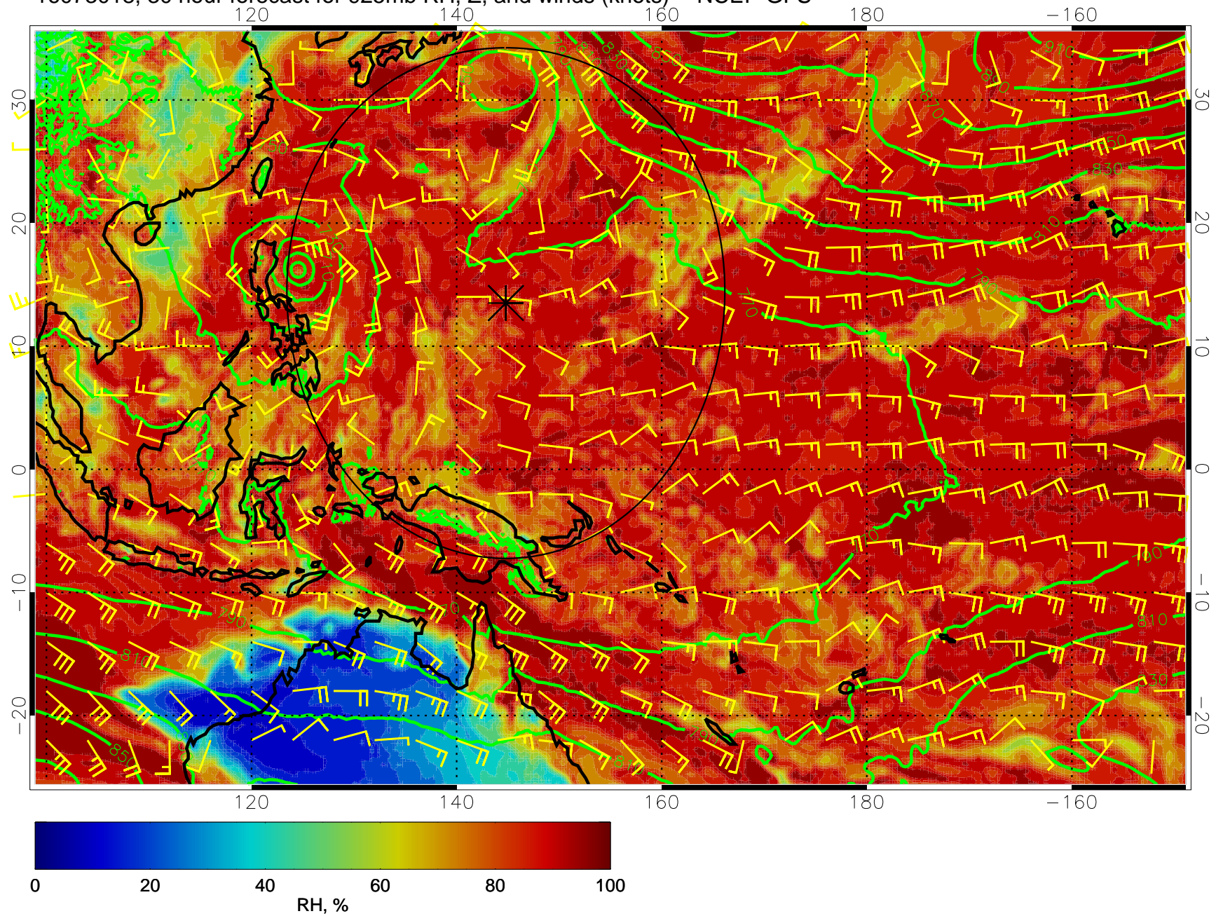
16073018, 30 hour forecast for 925mb RH, Z, and winds (knots) -- NCEP GFS
