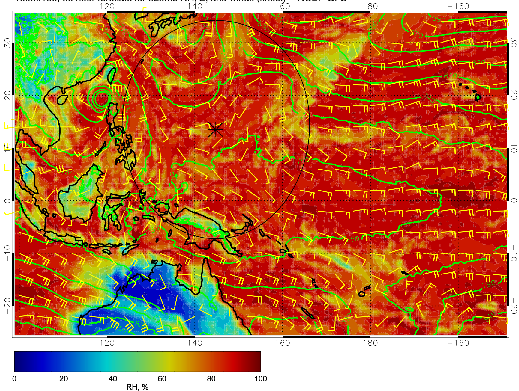
16080106, 66 hour forecast for 925mb RH, Z, and winds (knots) -- NCEP GFS
