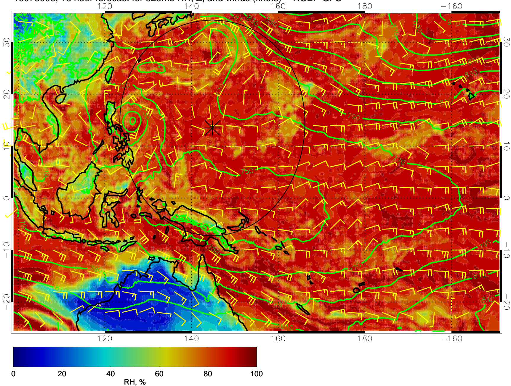
16073006, 18 hour forecast for 925mb RH, Z, and winds (knots) -- NCEP GFS
