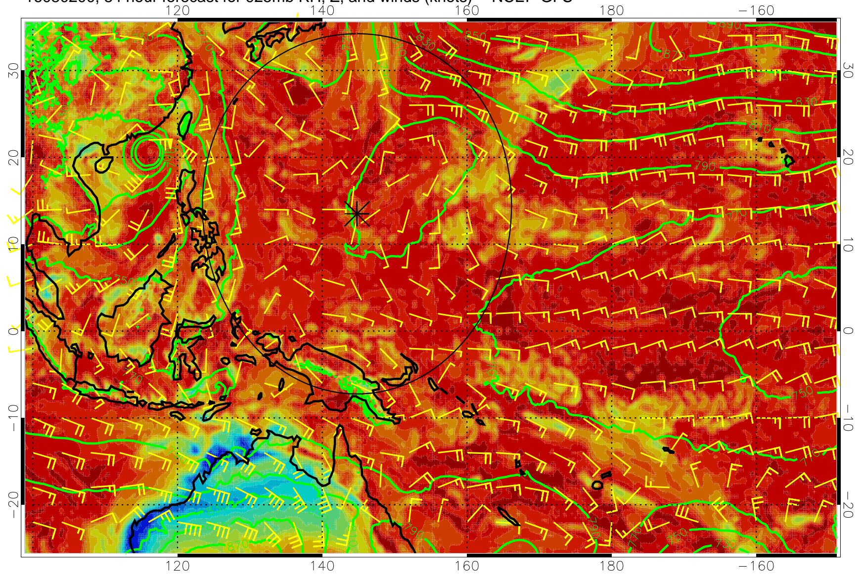
16080200, 84 hour forecast for 925mb RH, Z, and winds (knots) -- NCEP GFS
