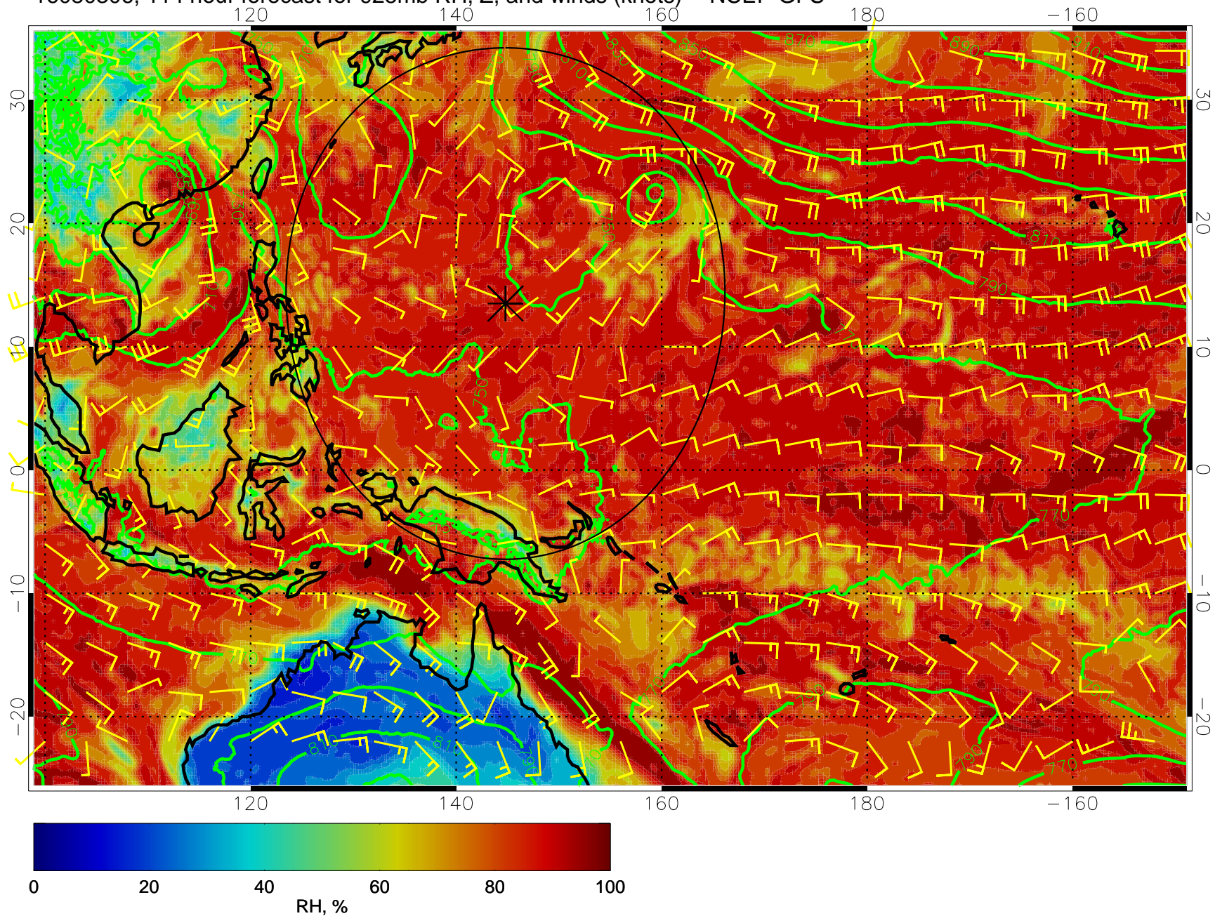
16080306, 114 hour forecast for 925mb RH, Z, and winds (knots) -- NCEP GFS
