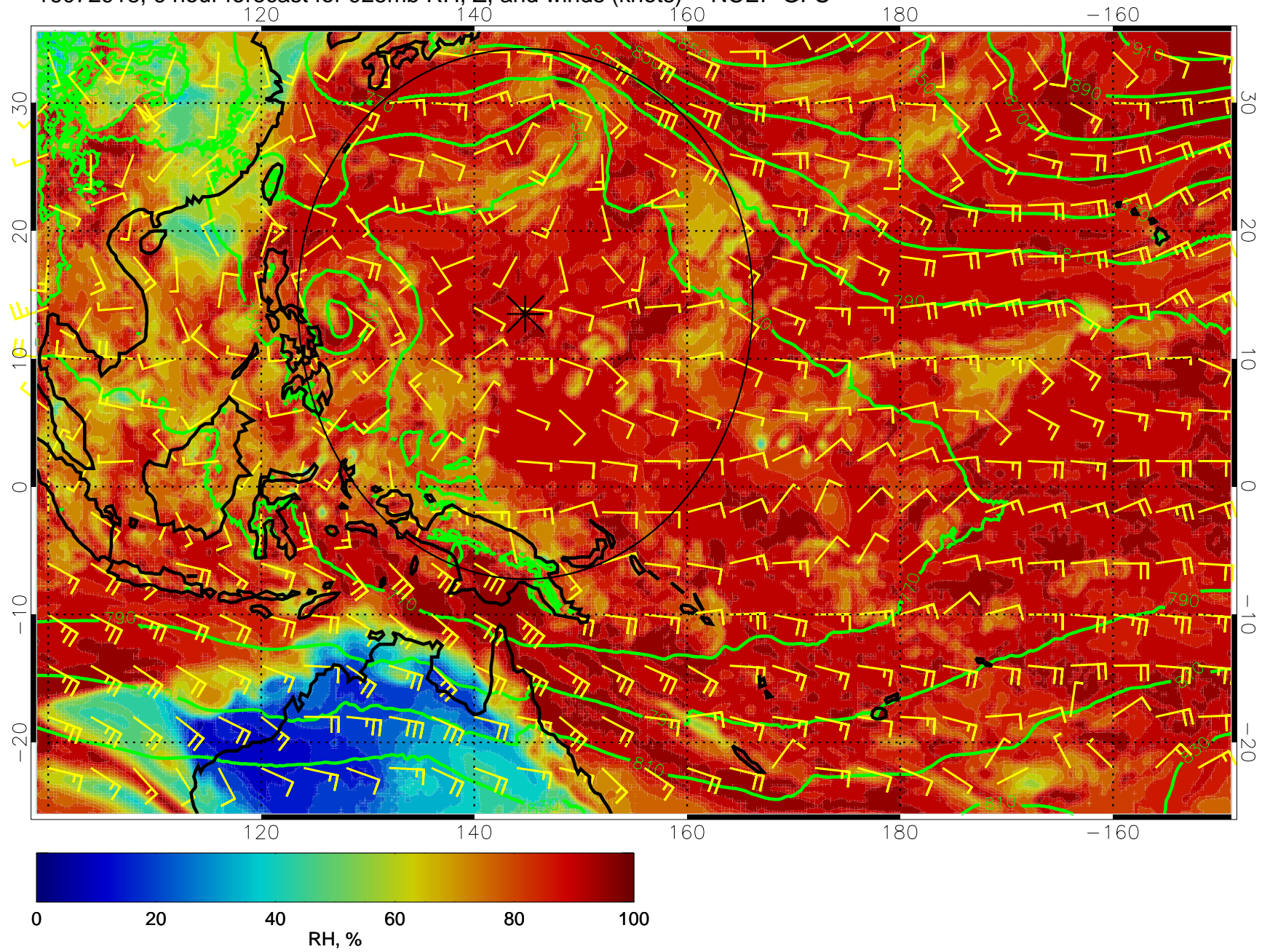
16072918, 6 hour forecast for 925mb RH, Z, and winds (knots) -- NCEP GFS
