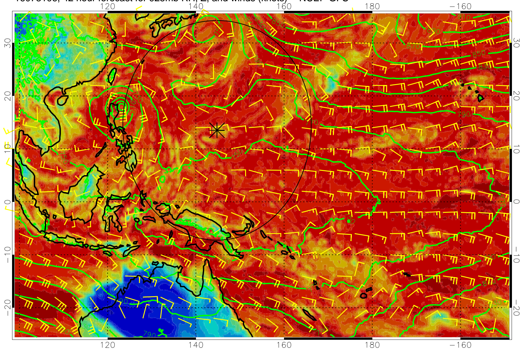
16073106, 42 hour forecast for 925mb RH, Z, and winds (knots) -- NCEP GFS
