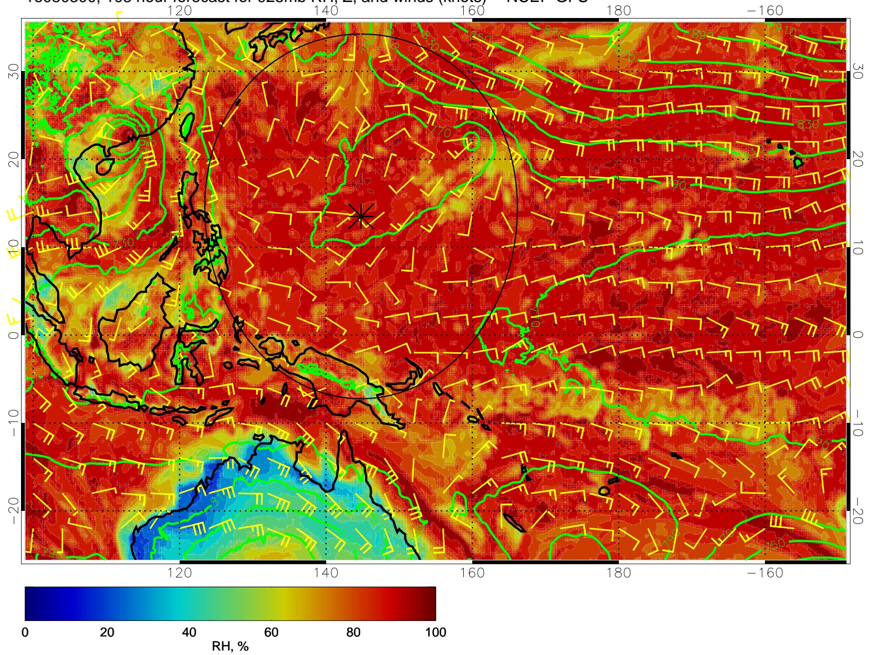
16080300, 108 hour forecast for 925mb RH, Z, and winds (knots) -- NCEP GFS
