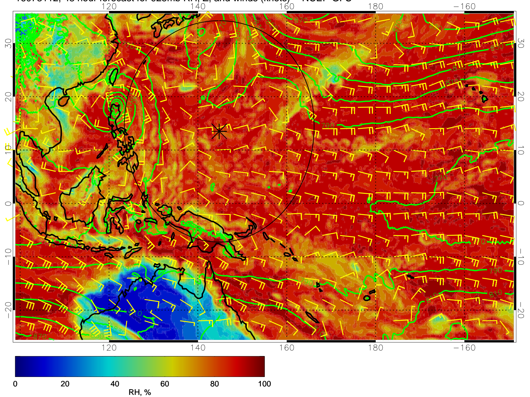
16073112, 48 hour forecast for 925mb RH, Z, and winds (knots) -- NCEP GFS
