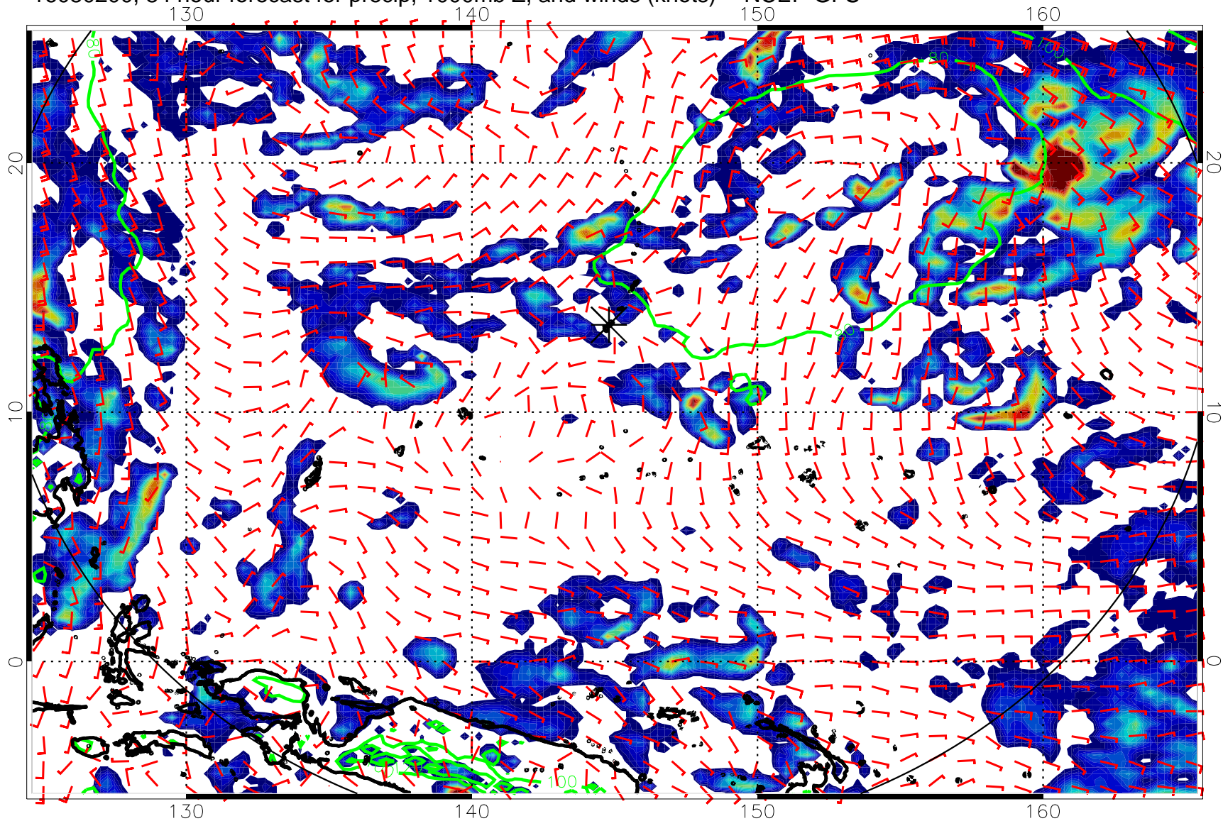
16080200, 84 hour forecast for precip, 1000mb Z, and winds (knots) -- NCEP GFS
