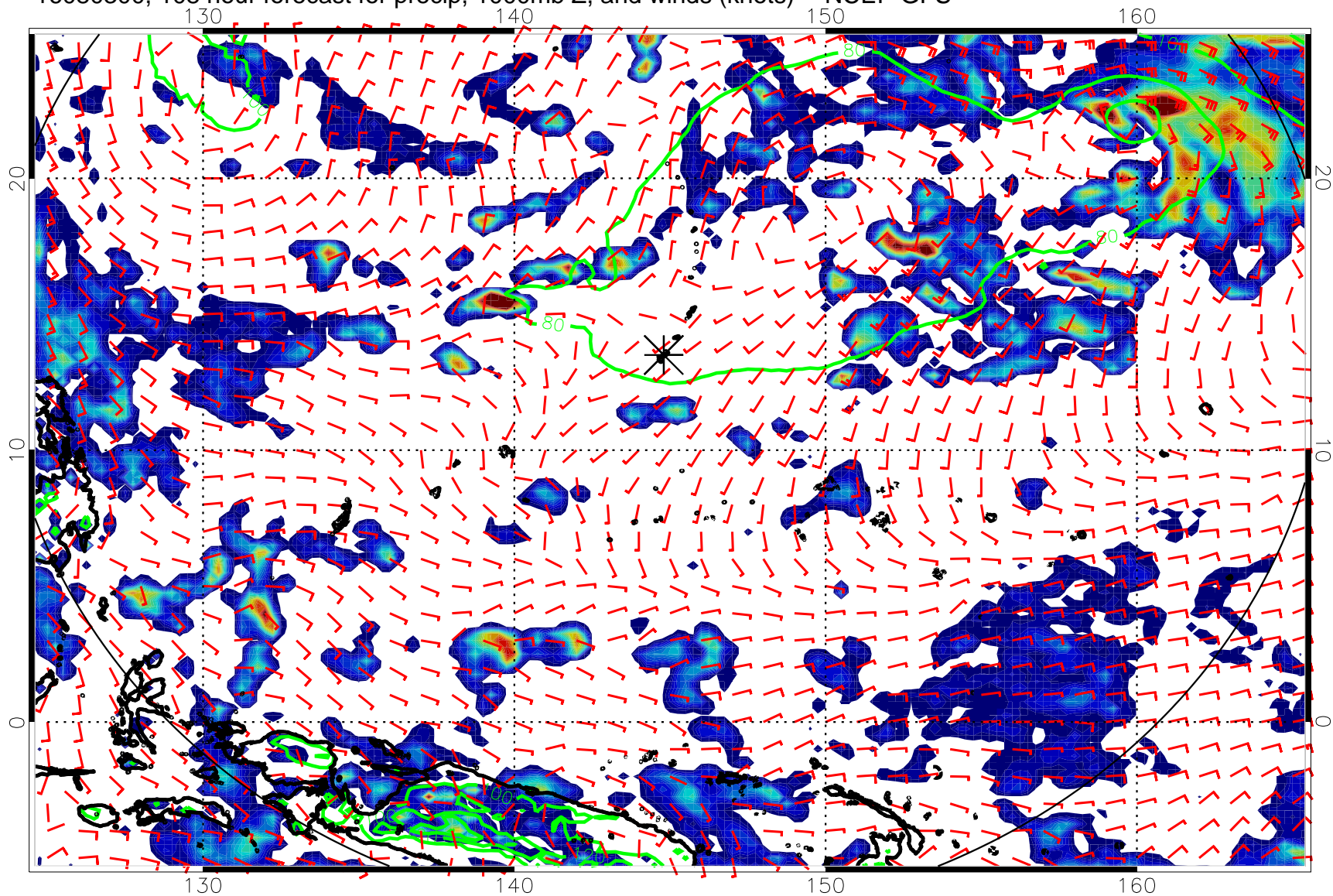
16080300, 108 hour forecast for precip, 1000mb Z, and winds (knots) -- NCEP GFS
