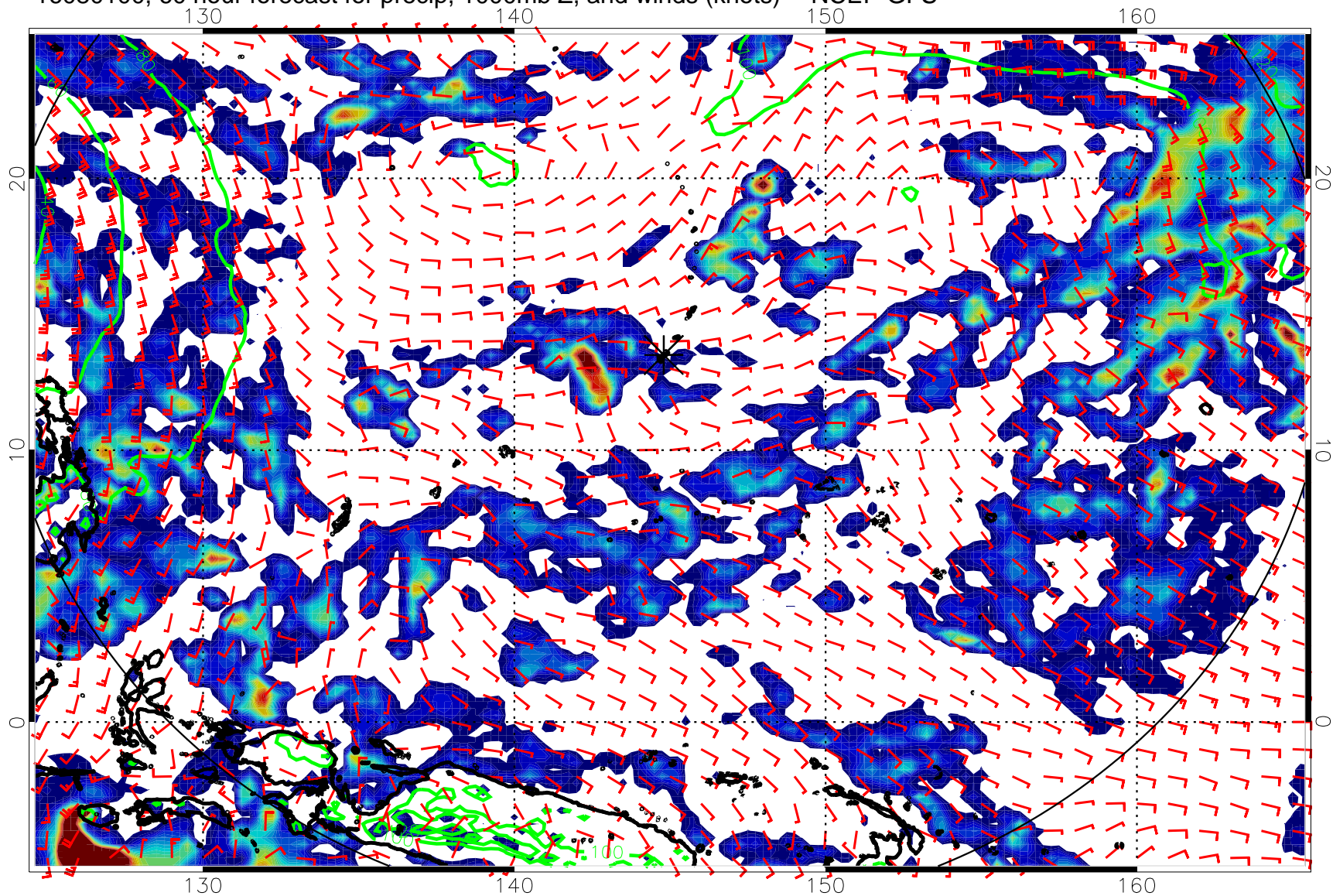
16080100, 60 hour forecast for precip, 1000mb Z, and winds (knots) -- NCEP GFS
