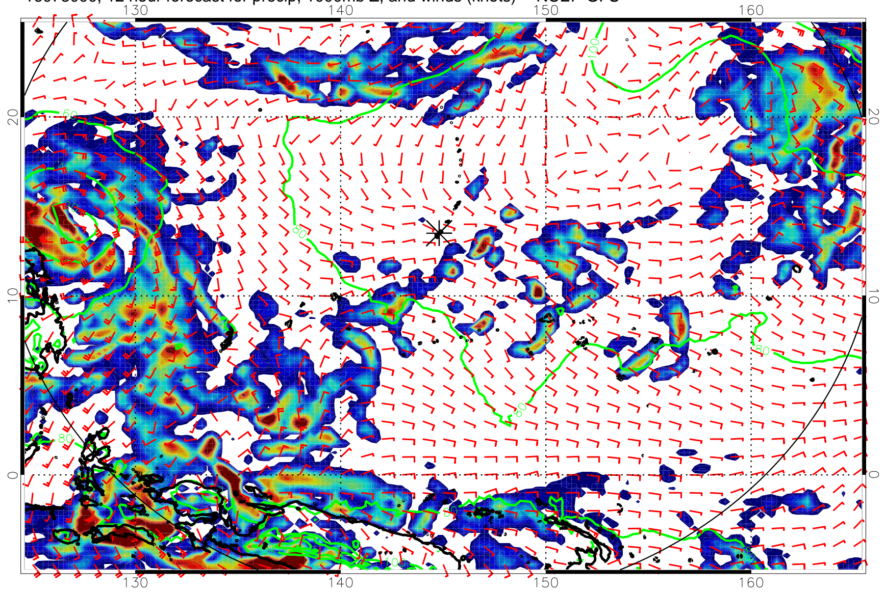
16073000, 12 hour forecast for precip, 1000mb Z, and winds (knots) -- NCEP GFS
