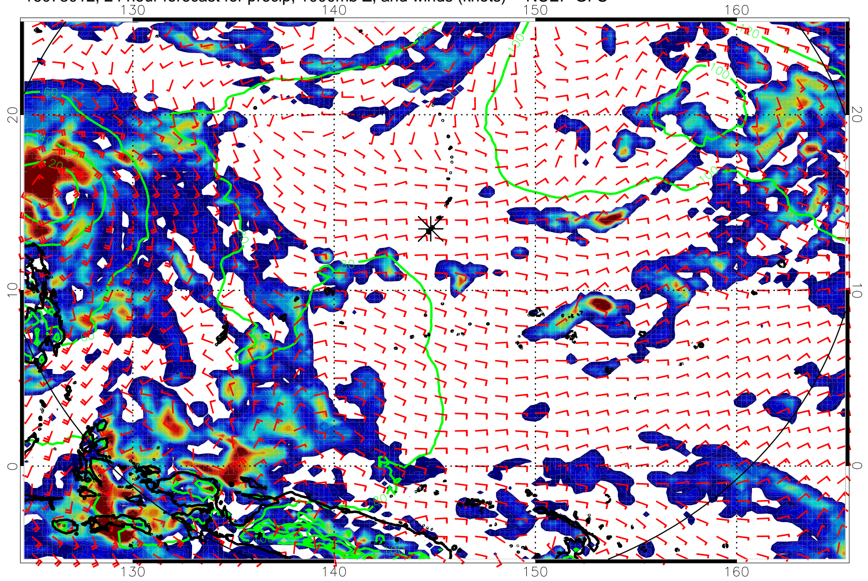
16073012, 24 hour forecast for precip, 1000mb Z, and winds (knots) -- NCEP GFS
