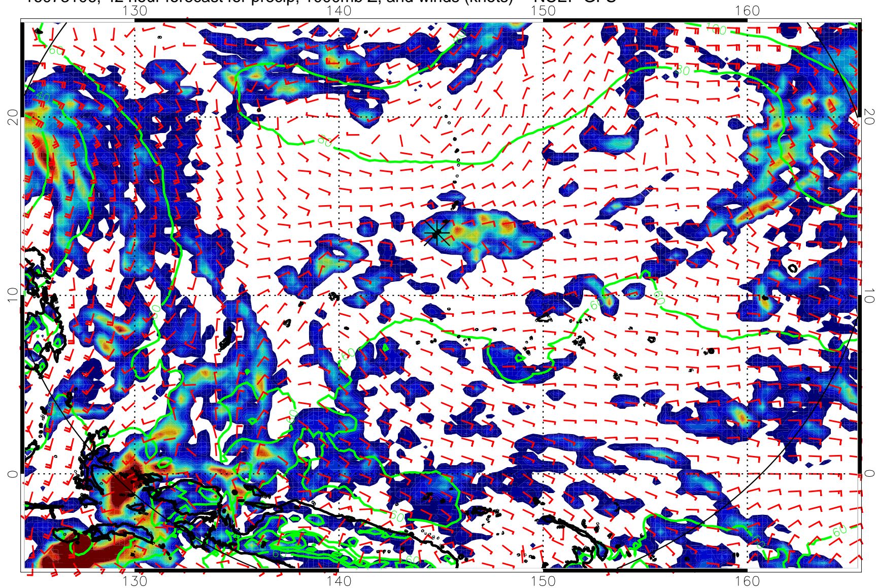
16073106, 42 hour forecast for precip, 1000mb Z, and winds (knots) -- NCEP GFS
