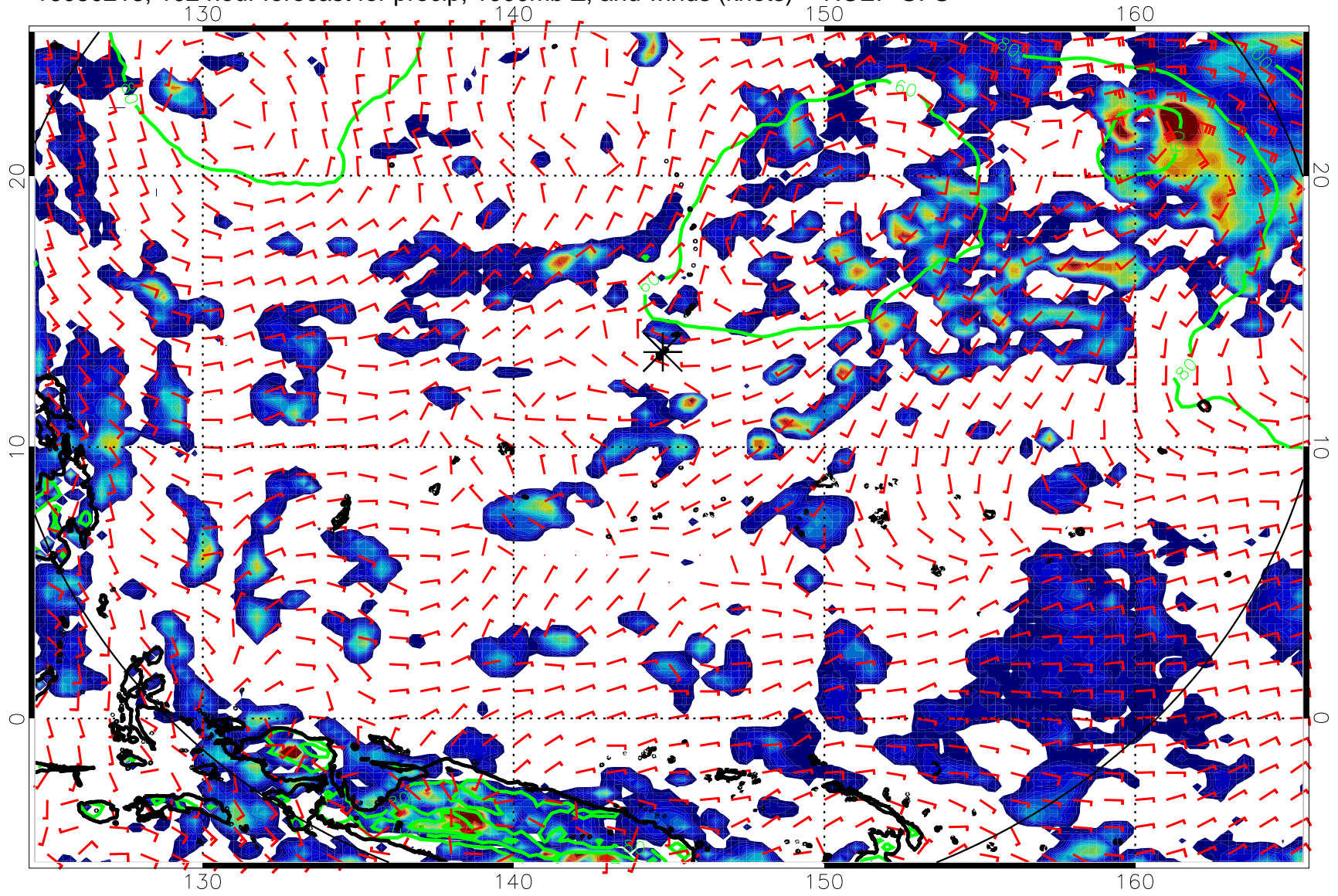
16080218, 102 hour forecast for precip, 1000mb Z, and winds (knots) -- NCEP GFS
