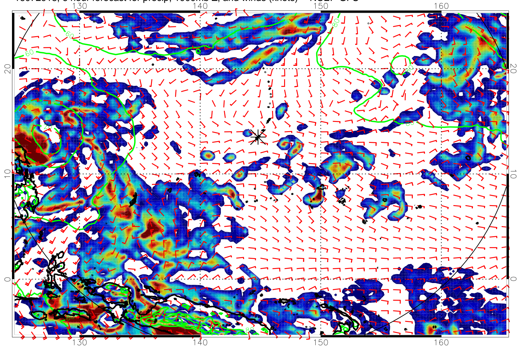
16072918, 6 hour forecast for precip, 1000mb Z, and winds (knots) -- NCEP GFS
