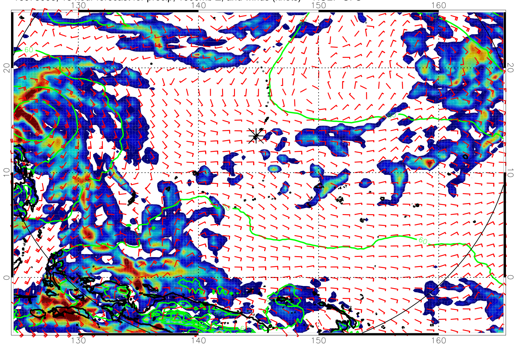
16073006, 18 hour forecast for precip, 1000mb Z, and winds (knots) -- NCEP GFS
