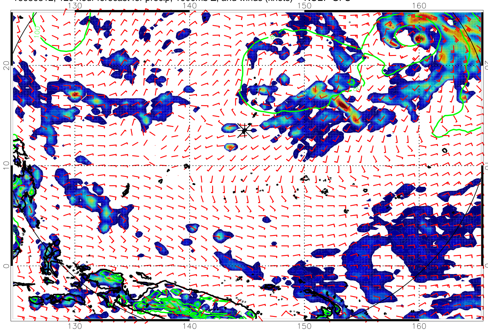
16080312, 120 hour forecast for precip, 1000mb Z, and winds (knots) -- NCEP GFS
