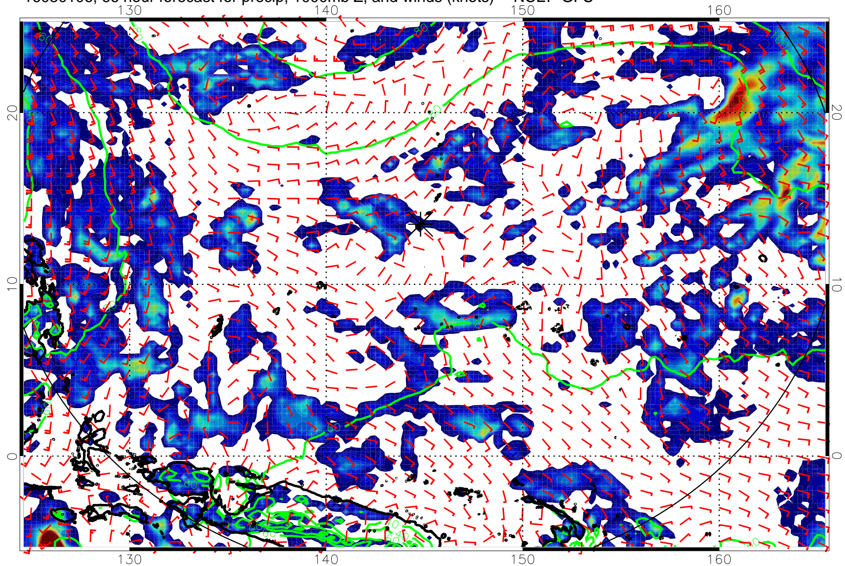
16080106, 66 hour forecast for precip, 1000mb Z, and winds (knots) -- NCEP GFS
