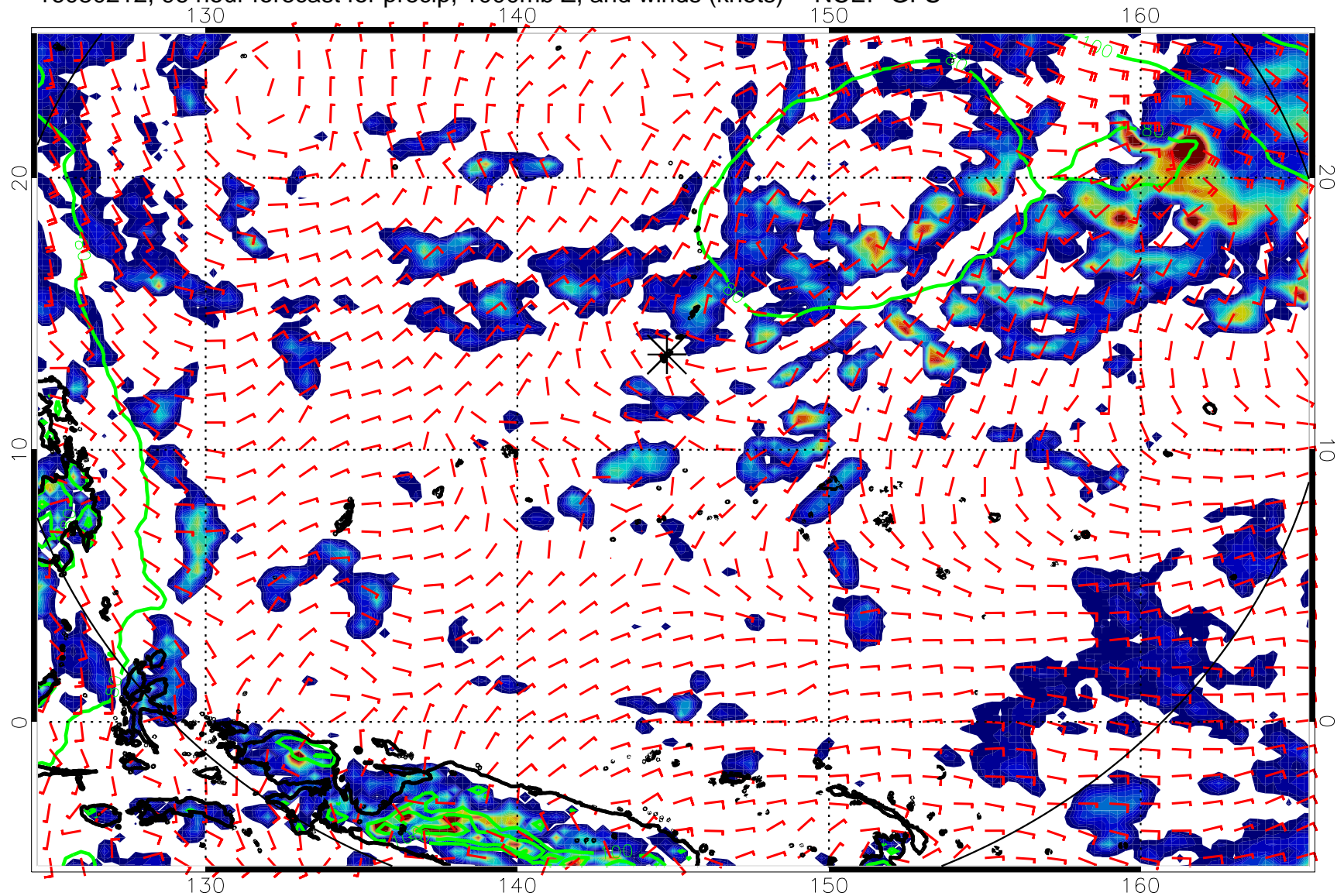
16080212, 96 hour forecast for precip, 1000mb Z, and winds (knots) -- NCEP GFS
