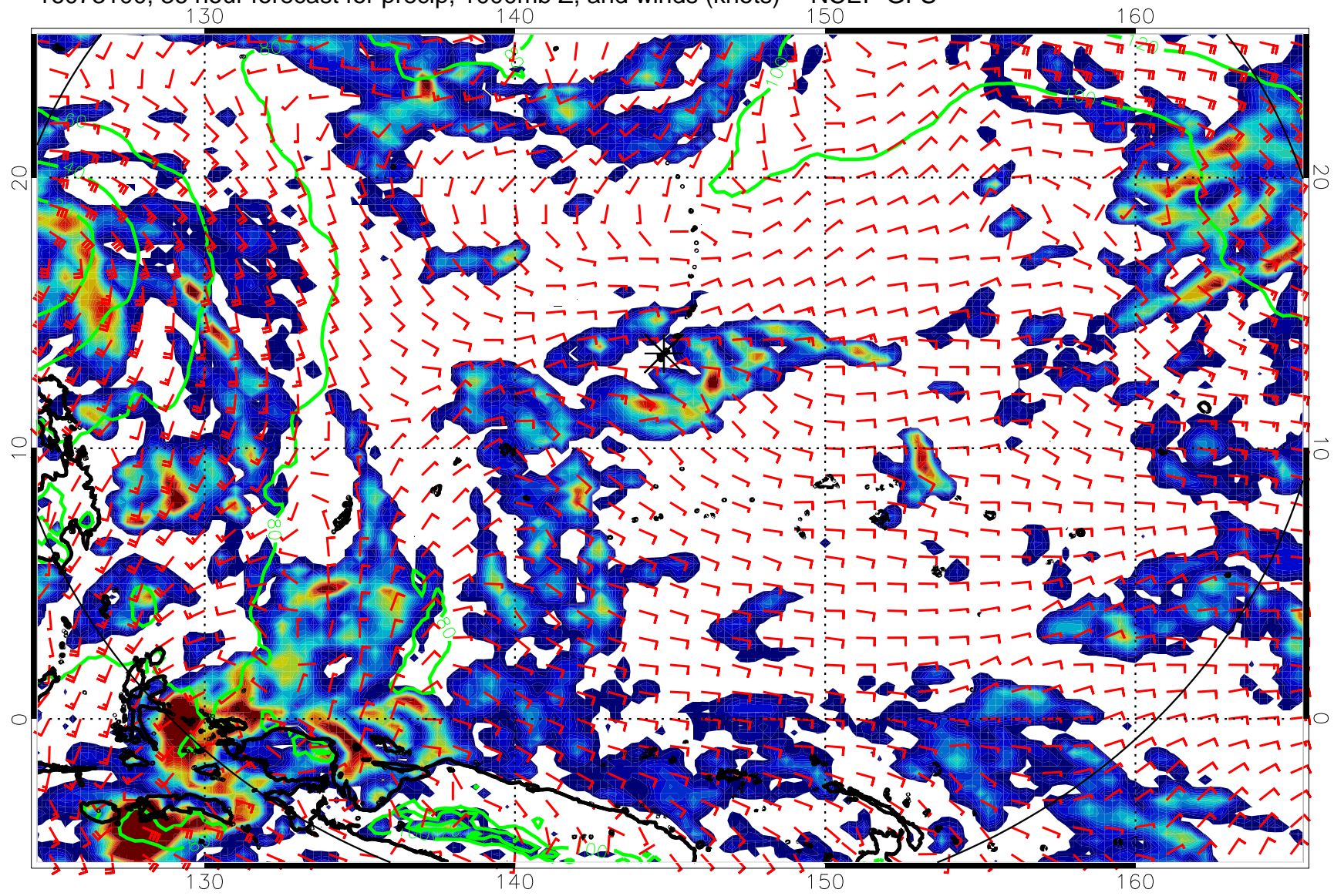
16073100, 36 hour forecast for precip, 1000mb Z, and winds (knots) -- NCEP GFS
