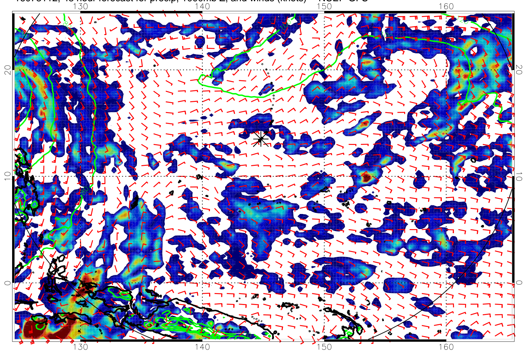
16073112, 48 hour forecast for precip, 1000mb Z, and winds (knots) -- NCEP GFS
