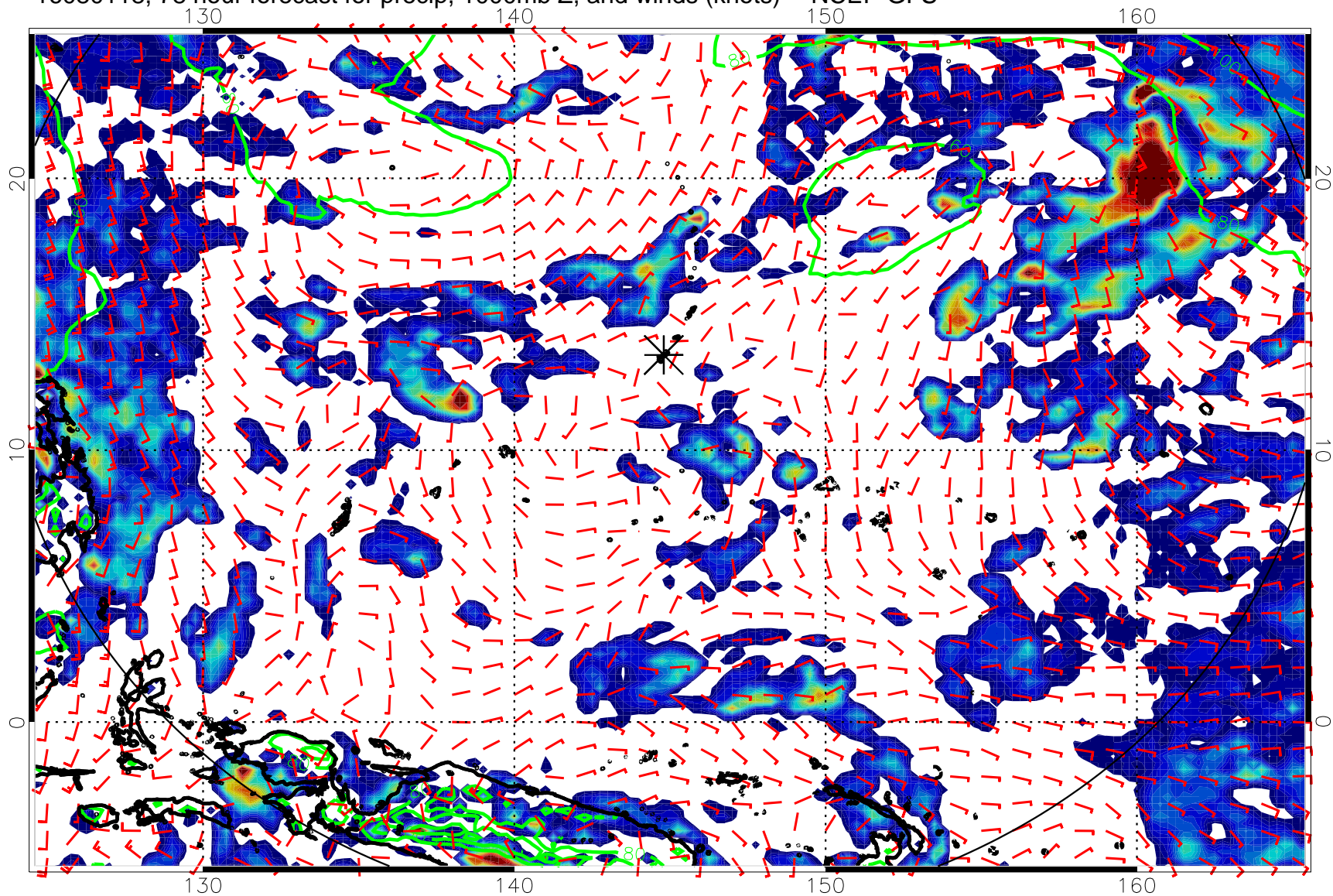
16080118, 78 hour forecast for precip, 1000mb Z, and winds (knots) -- NCEP GFS
