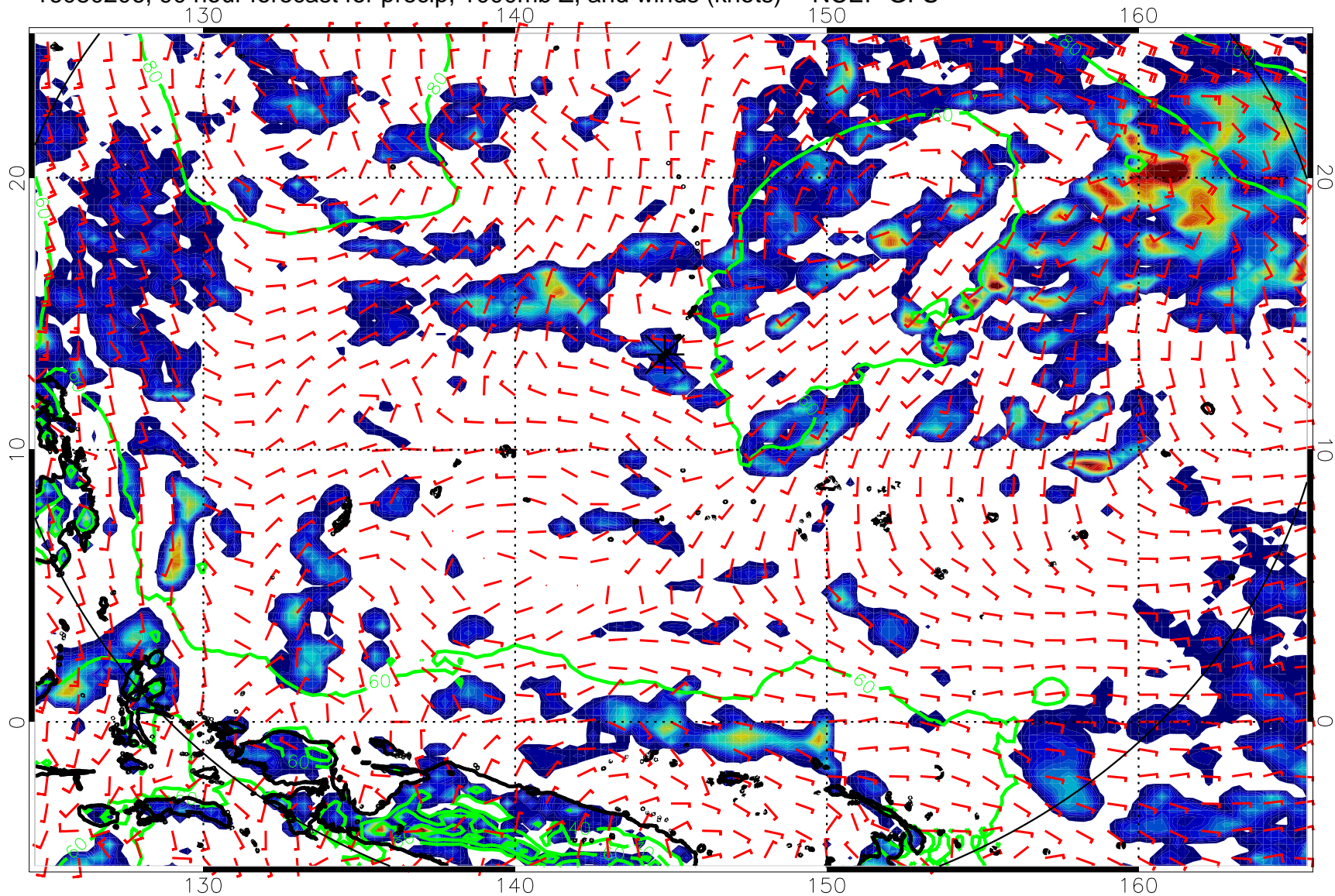
16080206, 90 hour forecast for precip, 1000mb Z, and winds (knots) -- NCEP GFS
