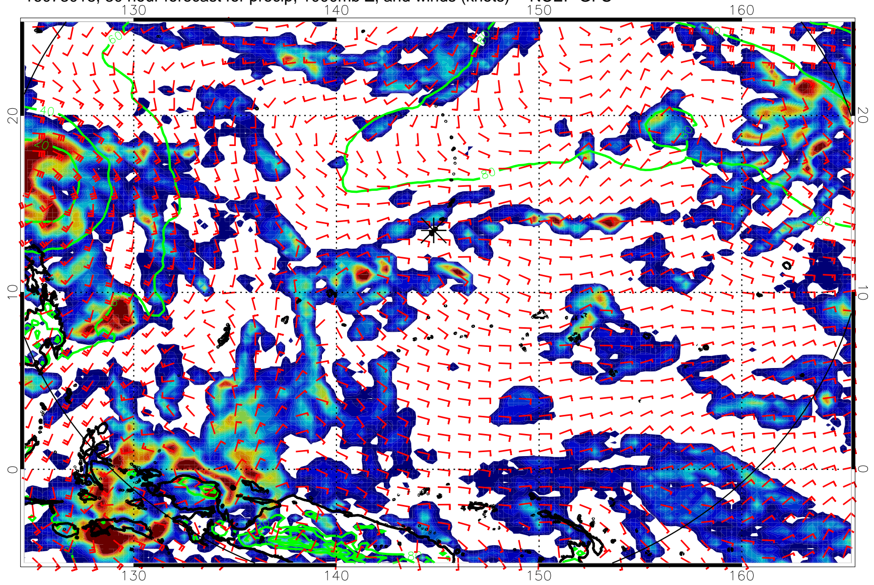
16073018, 30 hour forecast for precip, 1000mb Z, and winds (knots) -- NCEP GFS
