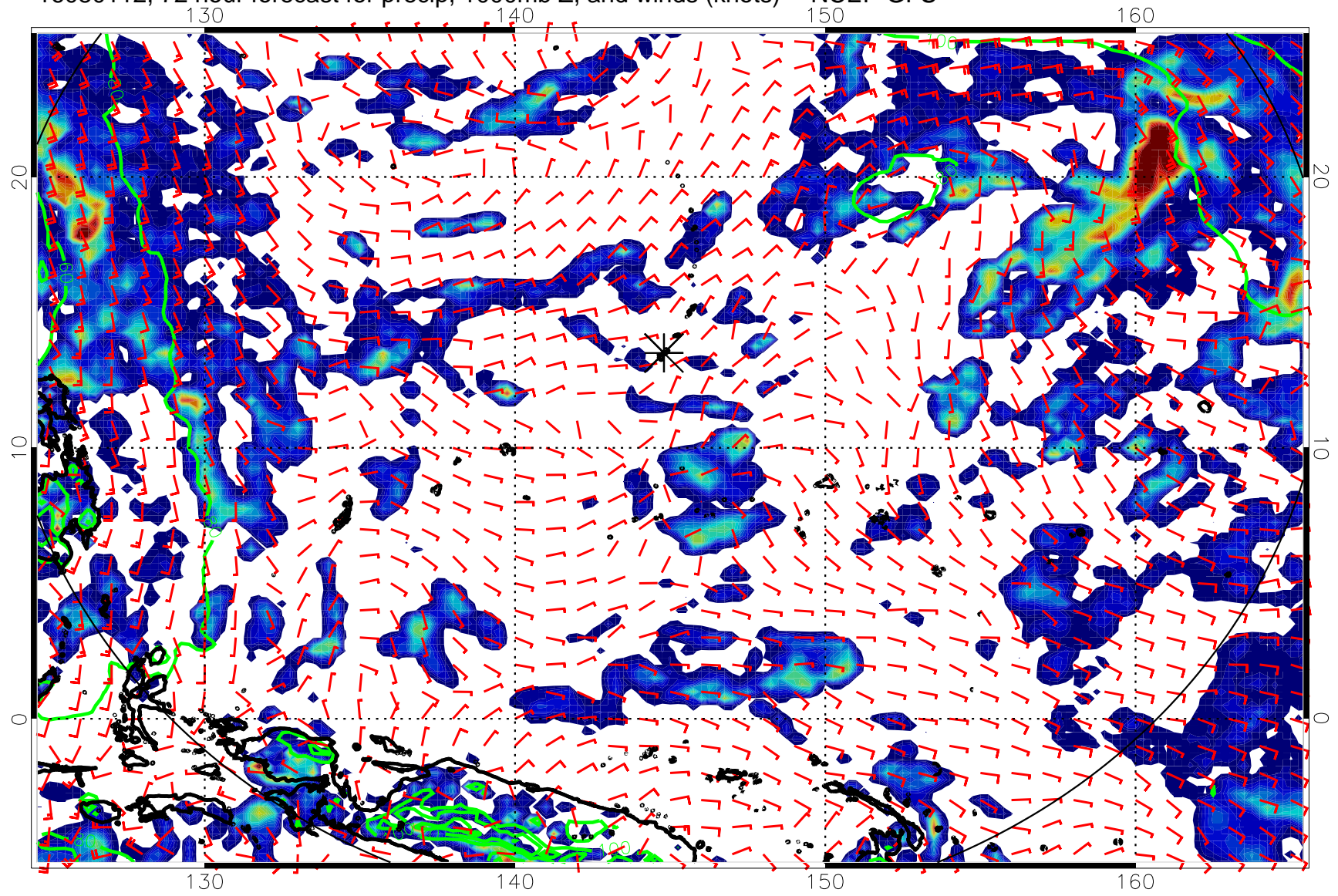
16080112, 72 hour forecast for precip, 1000mb Z, and winds (knots) -- NCEP GFS
