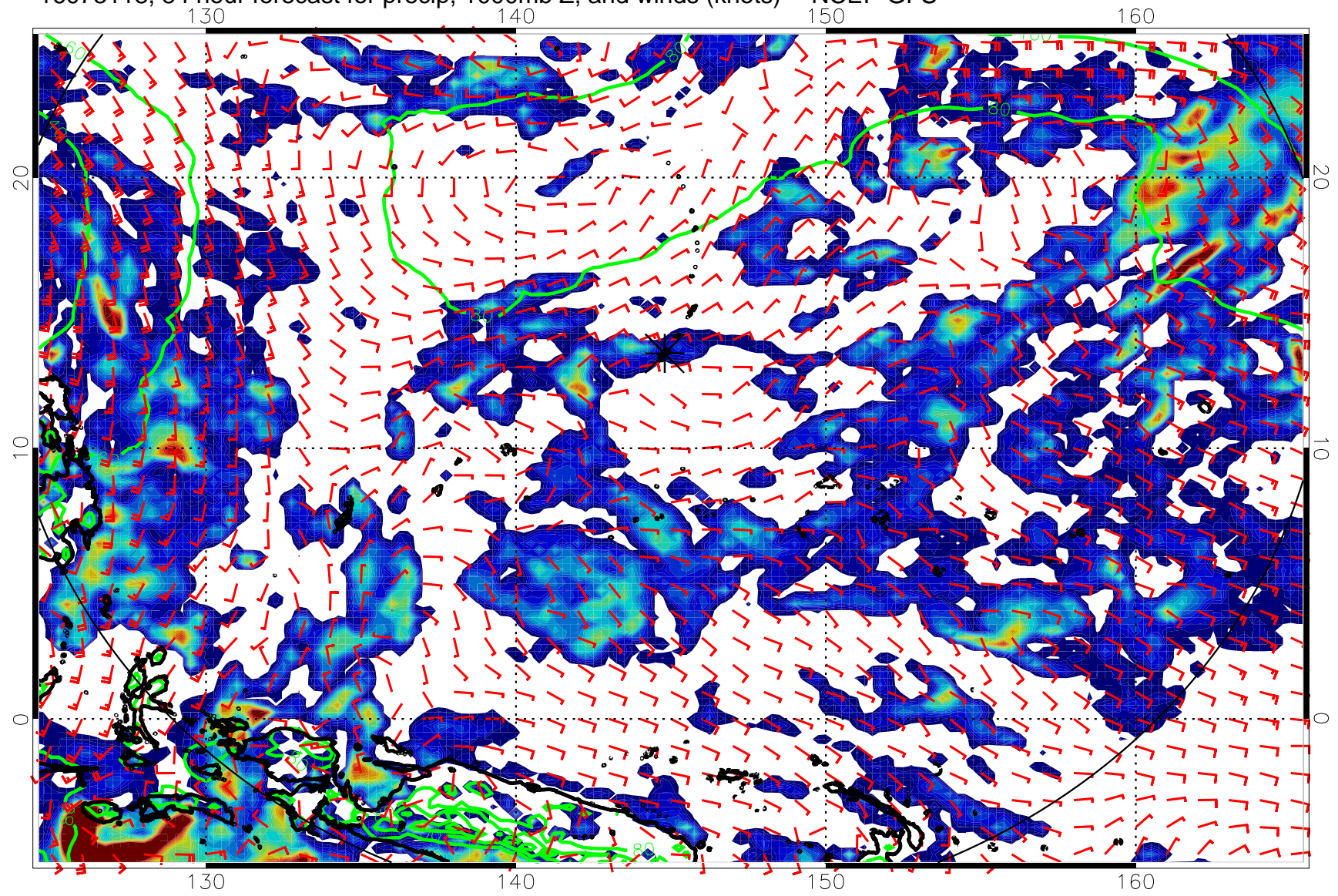
16073118, 54 hour forecast for precip, 1000mb Z, and winds (knots) -- NCEP GFS
