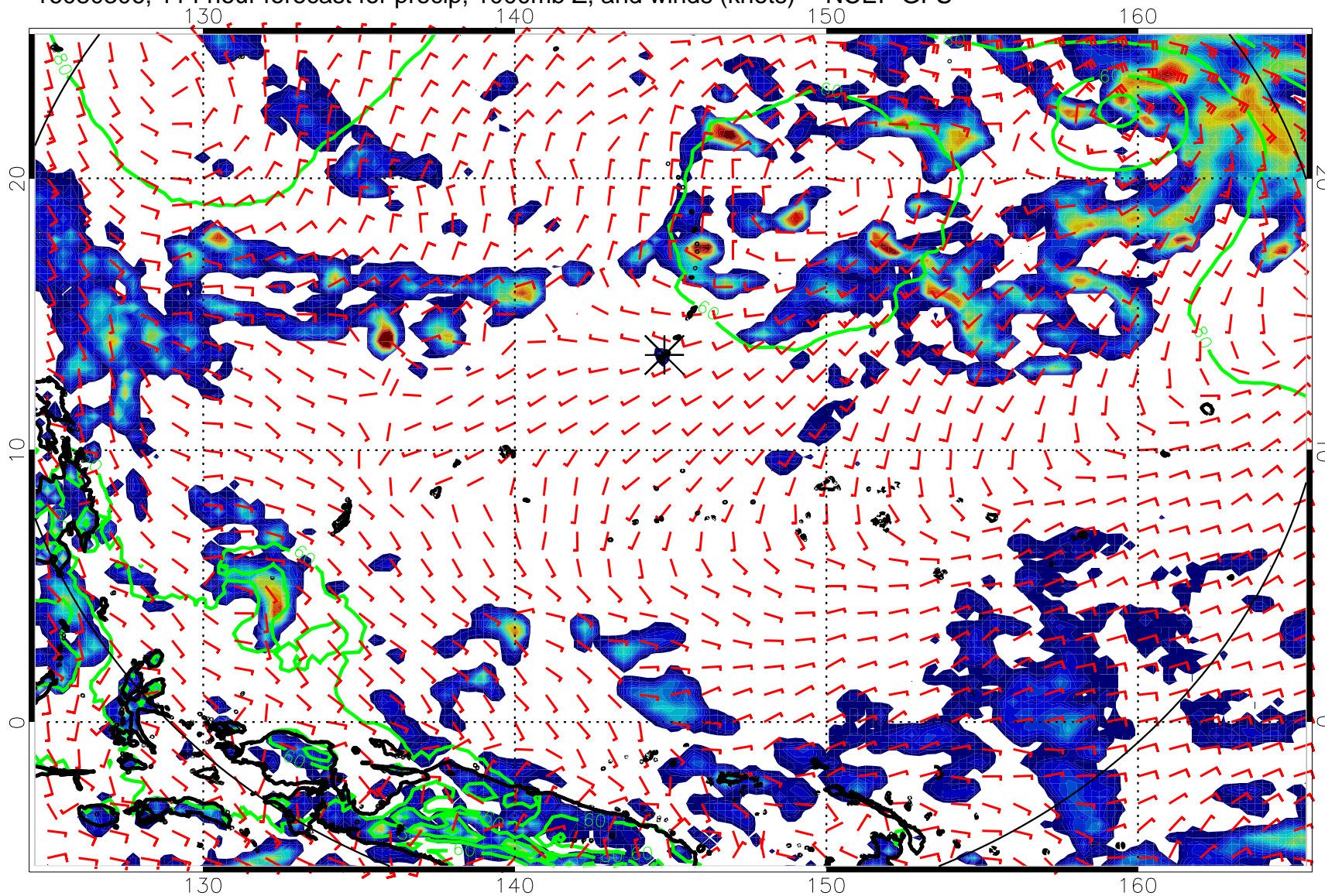
16080306, 114 hour forecast for precip, 1000mb Z, and winds (knots) -- NCEP GFS
