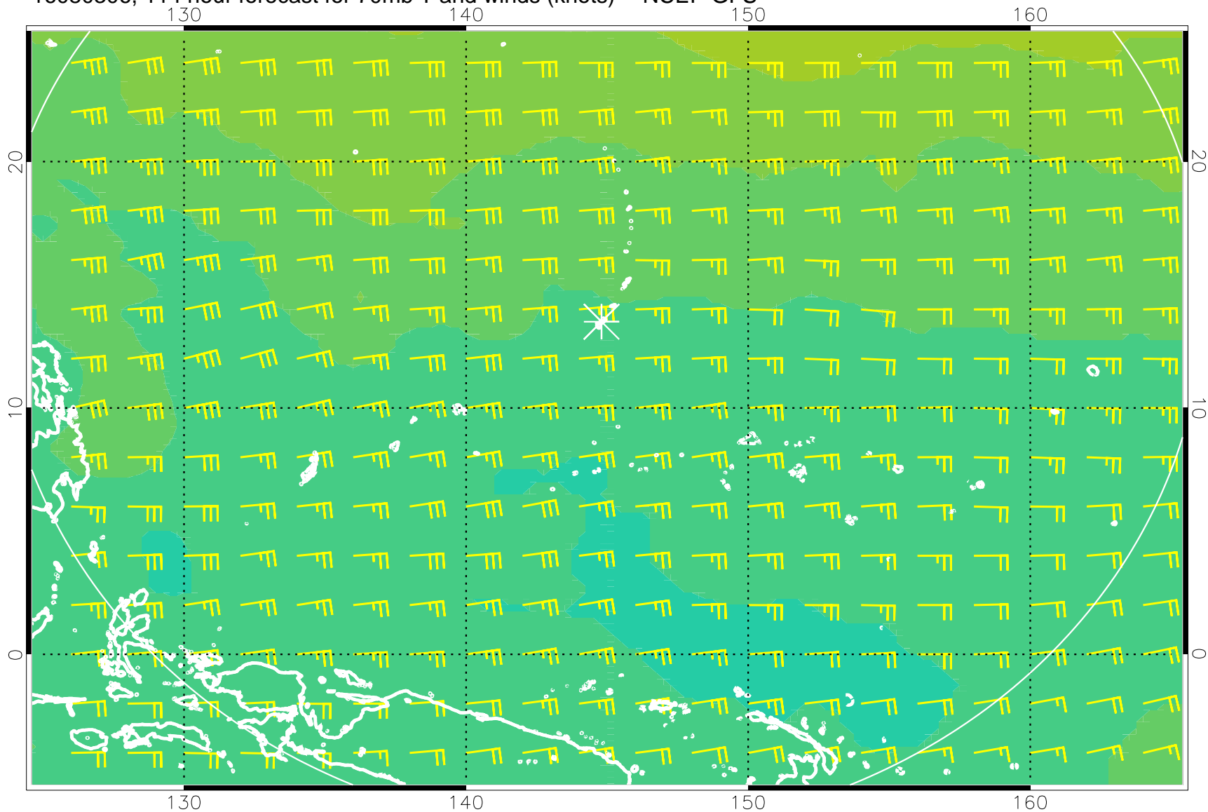
16080306, 114 hour forecast for 70mb T and winds (knots) -- NCEP GFS
