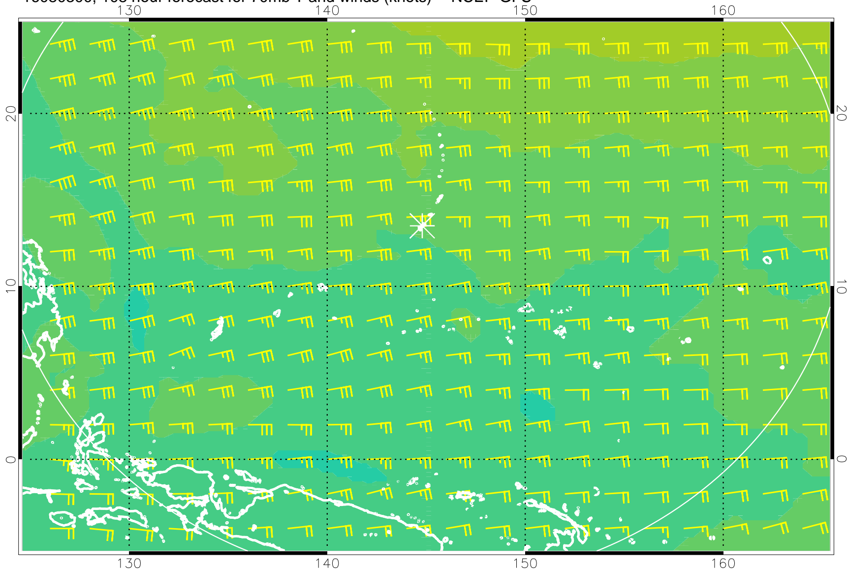
16080300, 108 hour forecast for 70mb T and winds (knots) -- NCEP GFS
