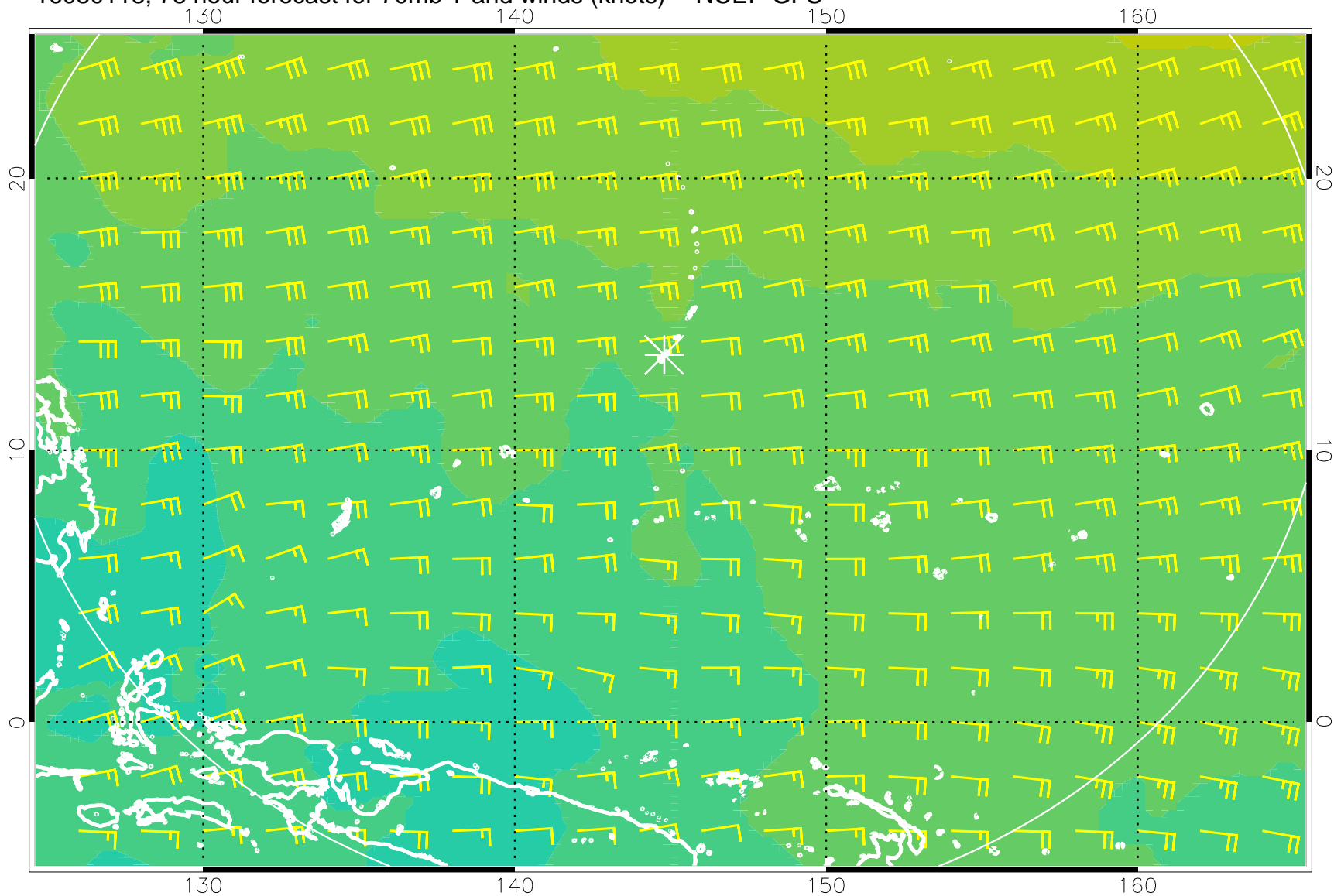
16080118, 78 hour forecast for 70mb T and winds (knots) -- NCEP GFS
