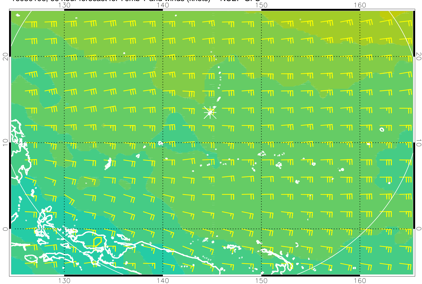
16080106, 66 hour forecast for 70mb T and winds (knots) -- NCEP GFS
