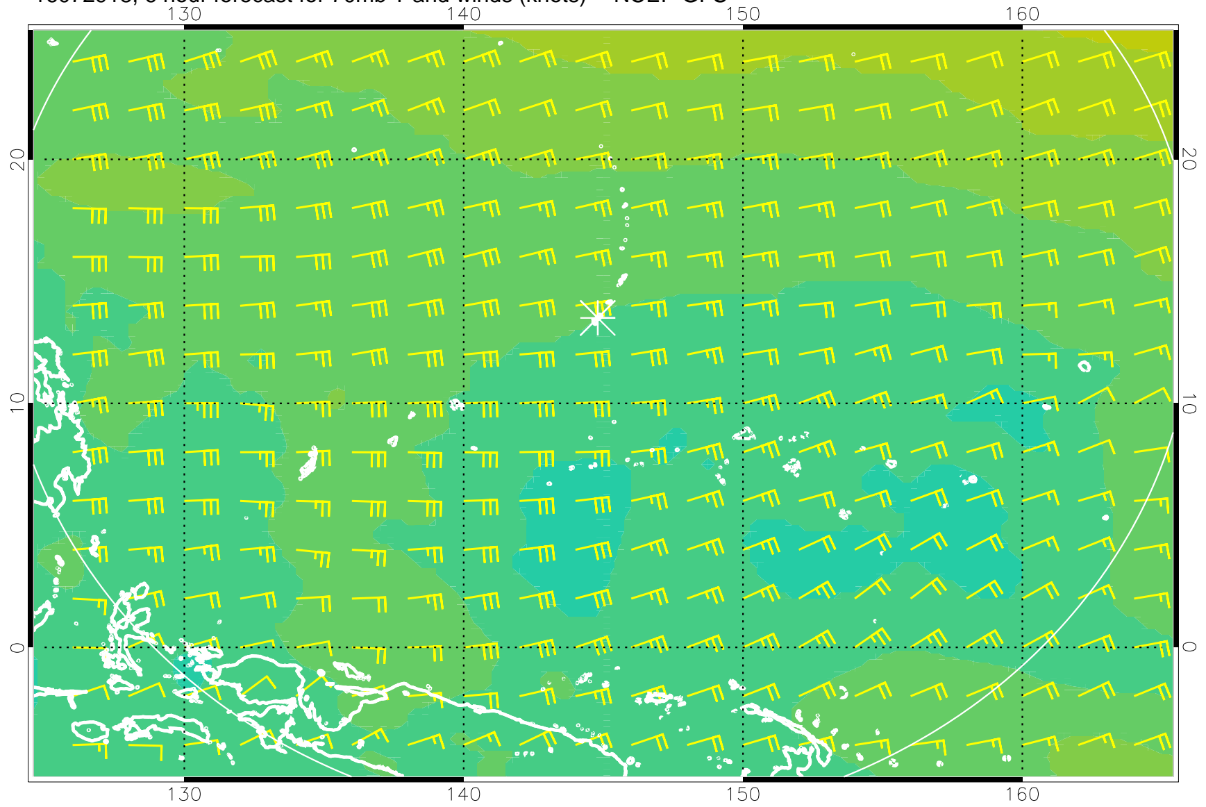
16072918, 6 hour forecast for 70mb T and winds (knots) -- NCEP GFS
