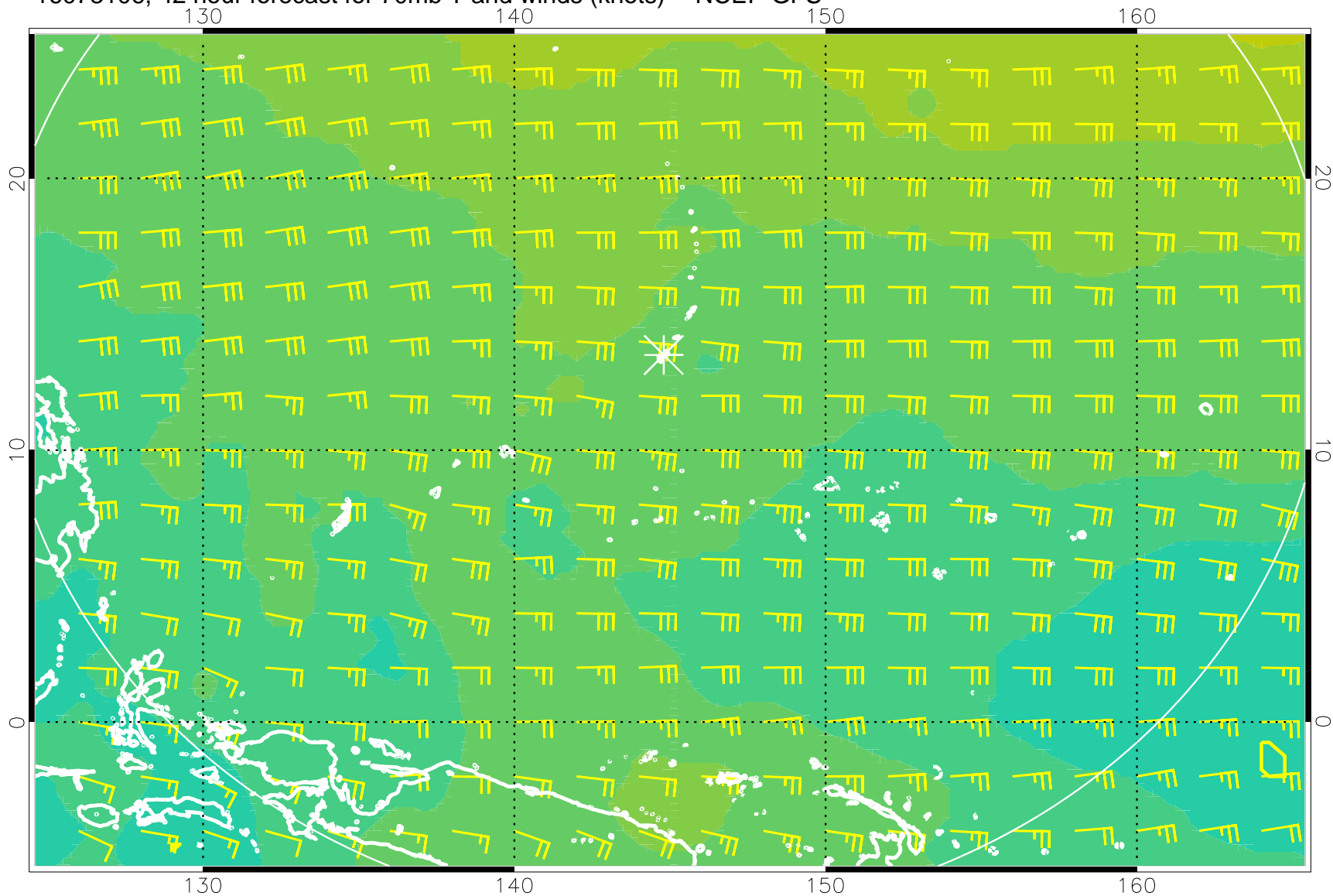
16073106, 42 hour forecast for 70mb T and winds (knots) -- NCEP GFS
