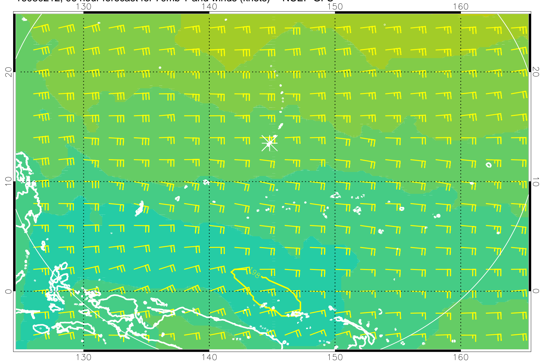
16080212, 96 hour forecast for 70mb T and winds (knots) -- NCEP GFS
