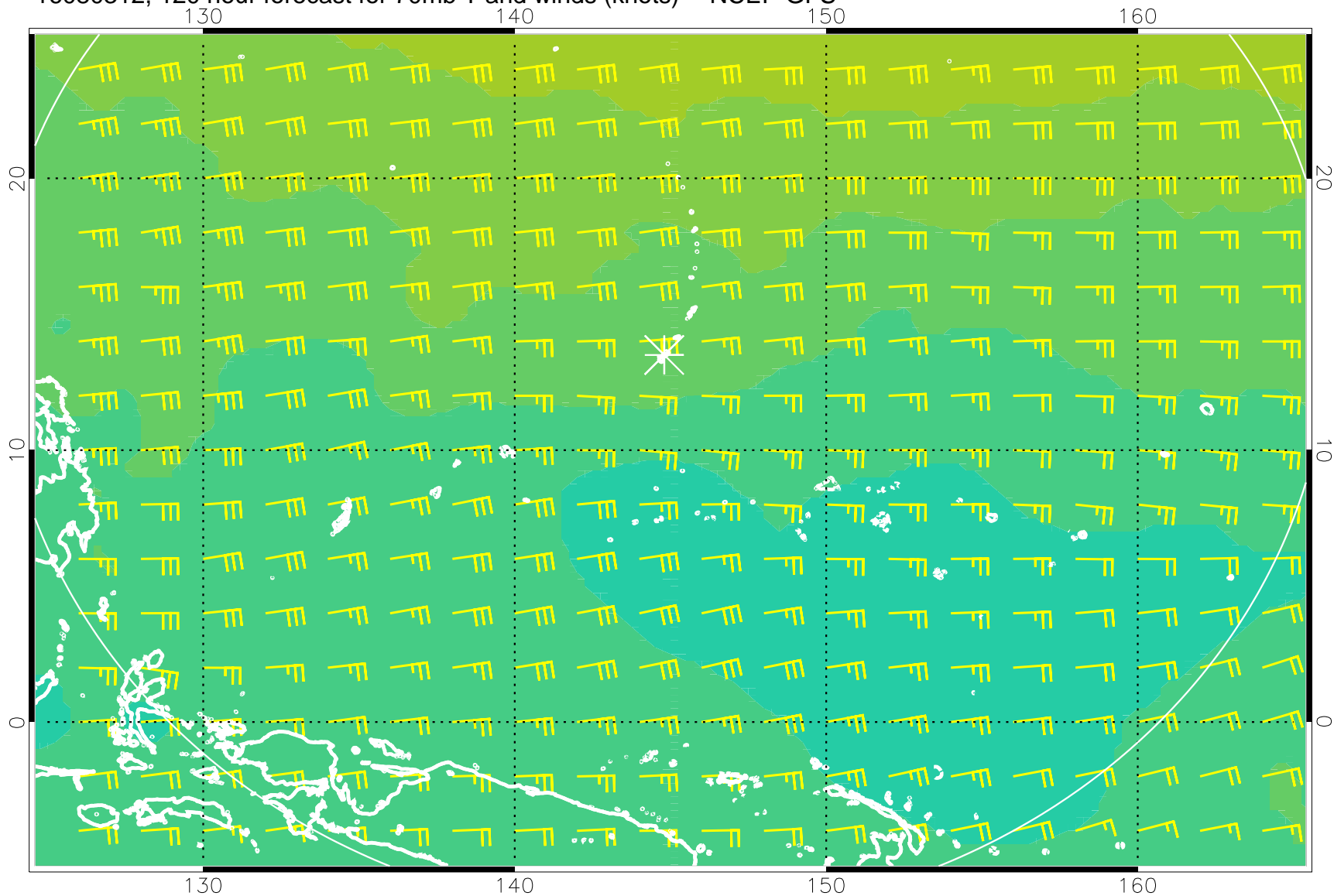
16080312, 120 hour forecast for 70mb T and winds (knots) -- NCEP GFS
