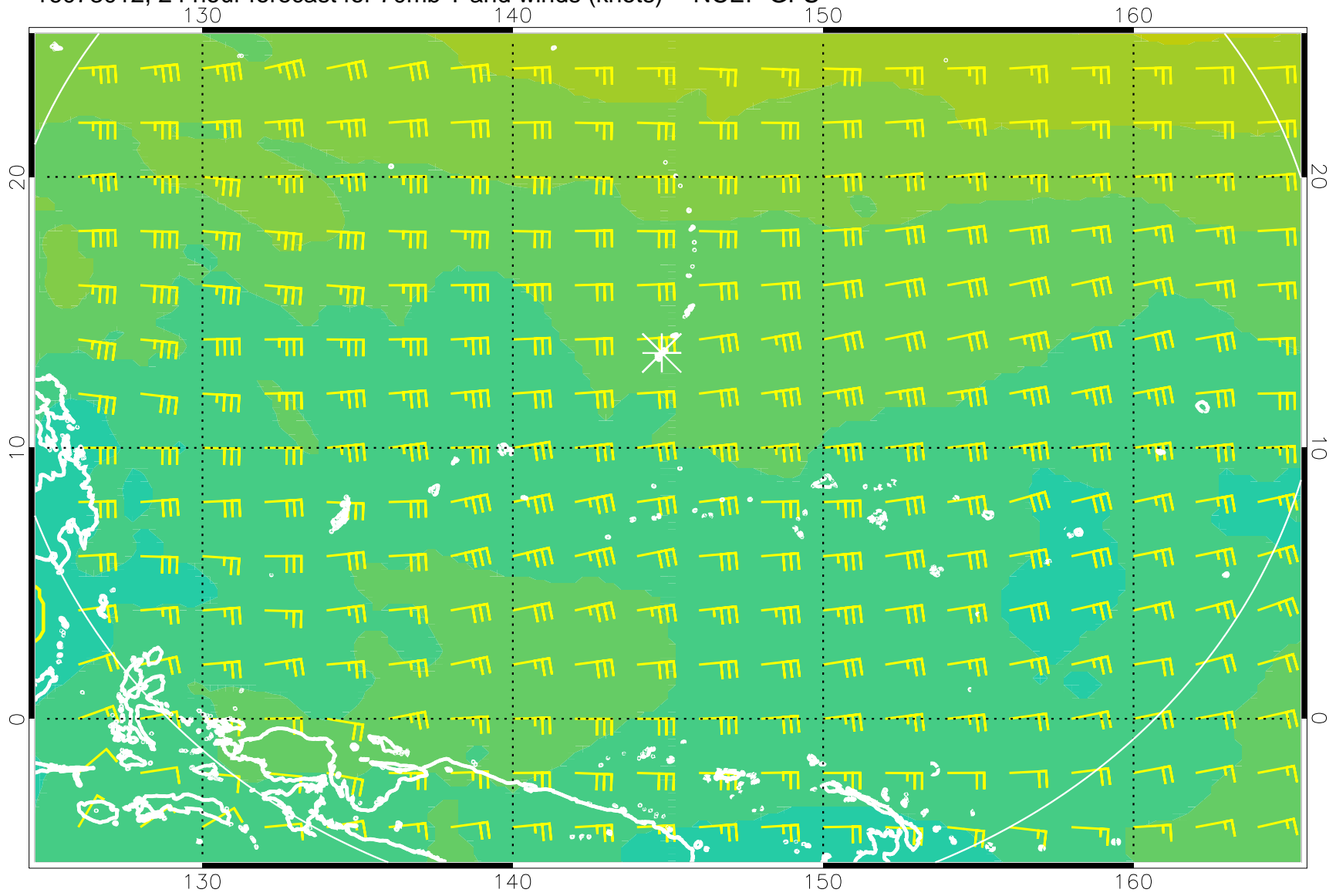
16073012, 24 hour forecast for 70mb T and winds (knots) -- NCEP GFS
