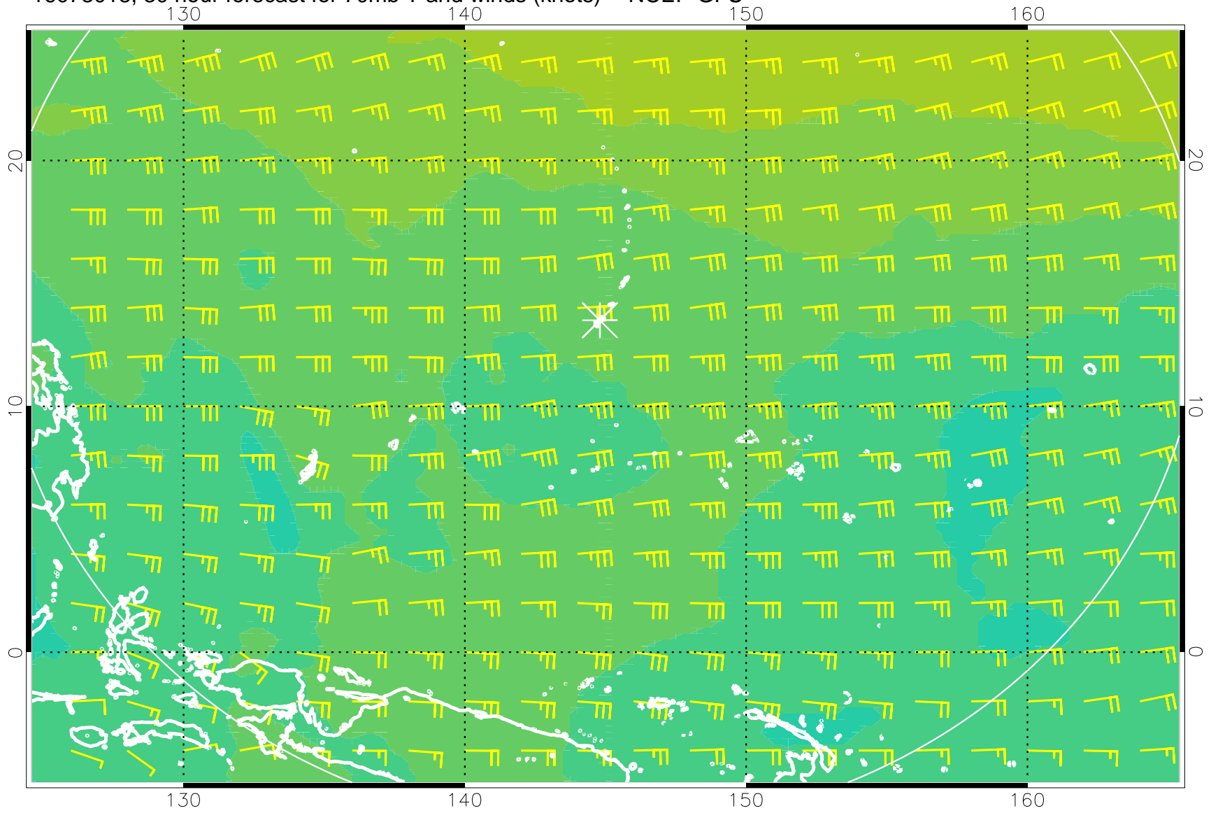
16073018, 30 hour forecast for 70mb T and winds (knots) -- NCEP GFS
