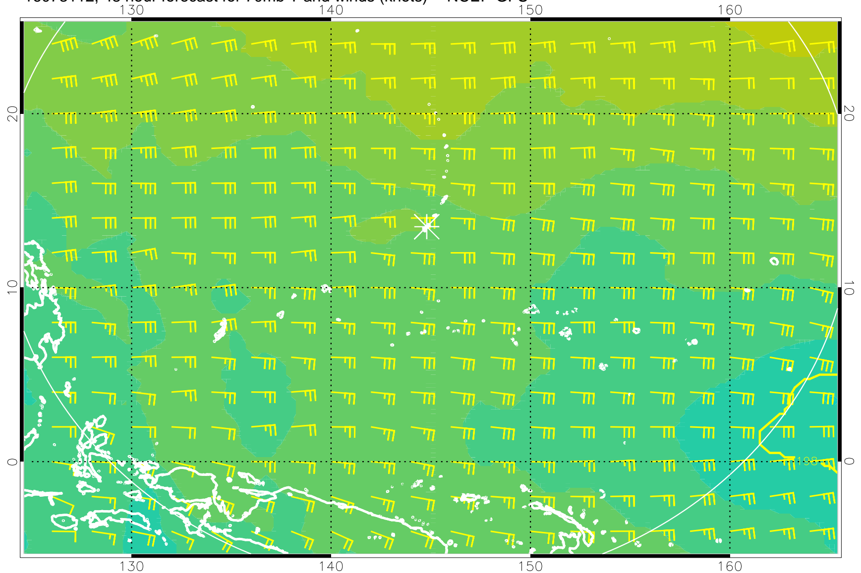
16073112, 48 hour forecast for 70mb T and winds (knots) -- NCEP GFS
