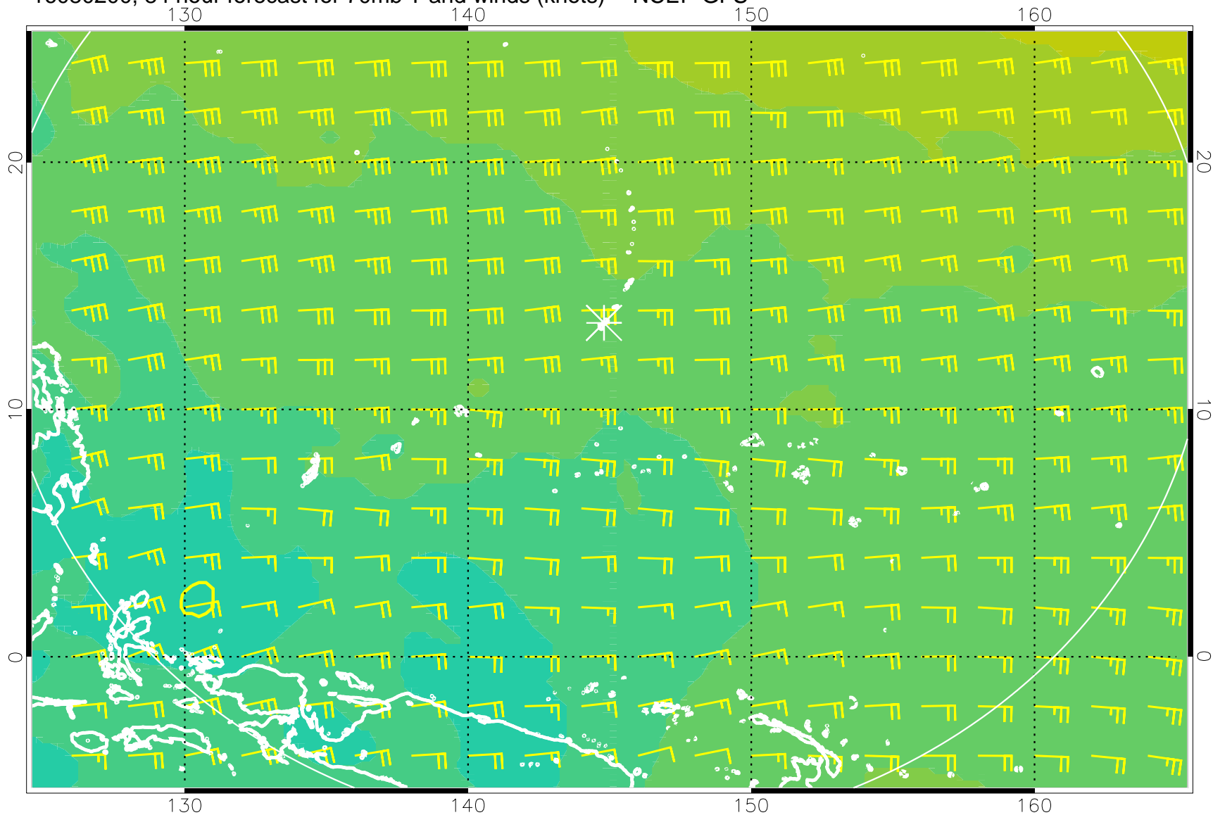
16080200, 84 hour forecast for 70mb T and winds (knots) -- NCEP GFS
