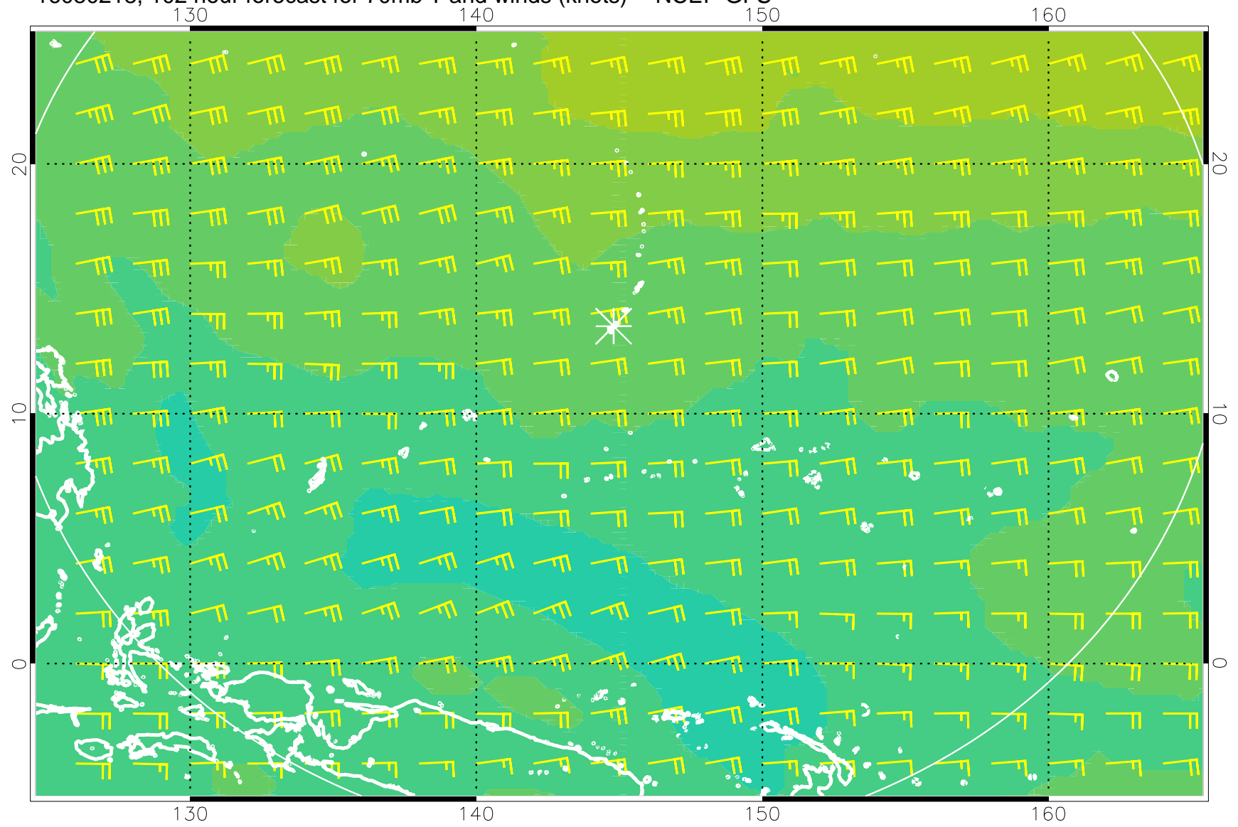
16080218, 102 hour forecast for 70mb T and winds (knots) -- NCEP GFS
