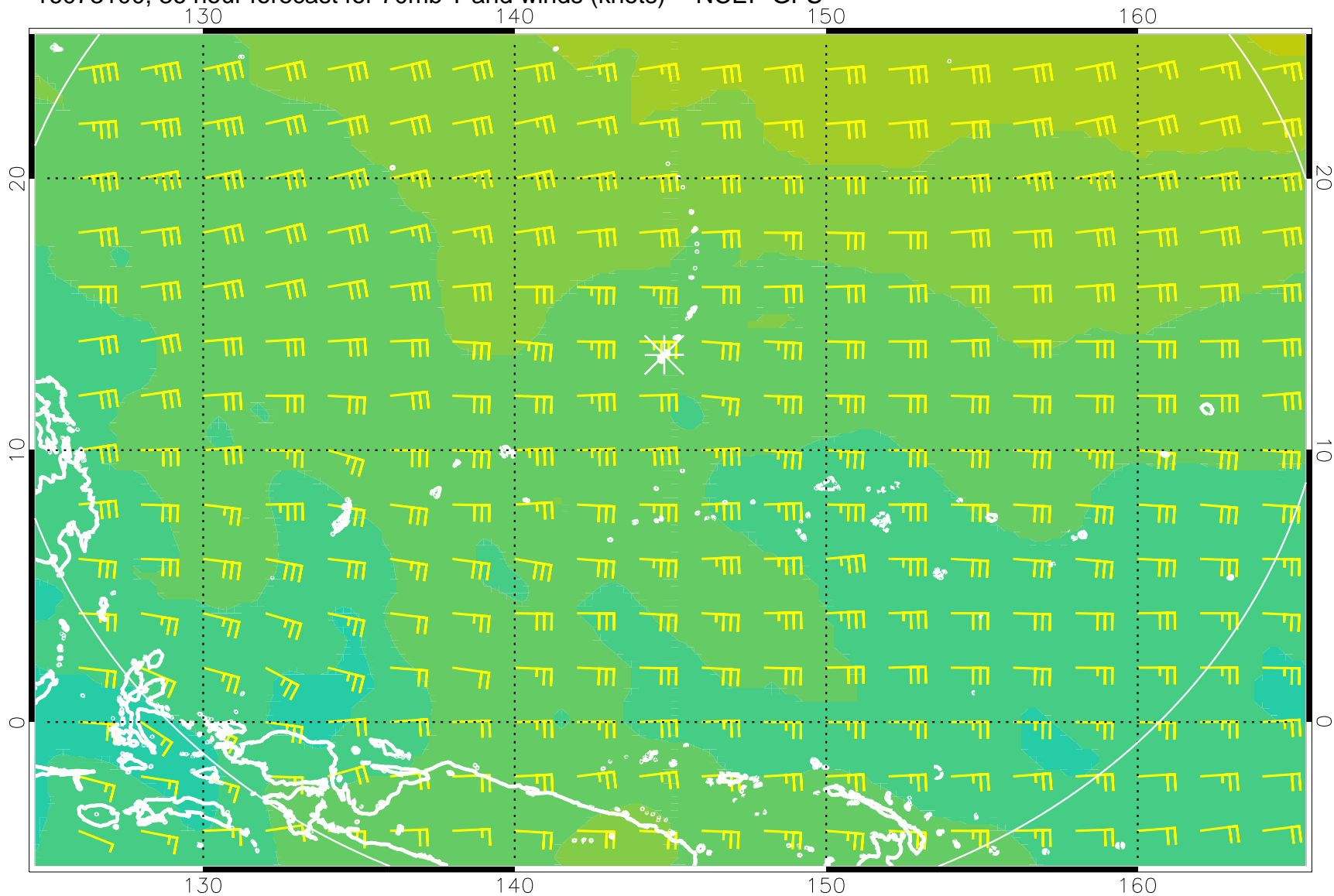
16073100, 36 hour forecast for 70mb T and winds (knots) -- NCEP GFS
