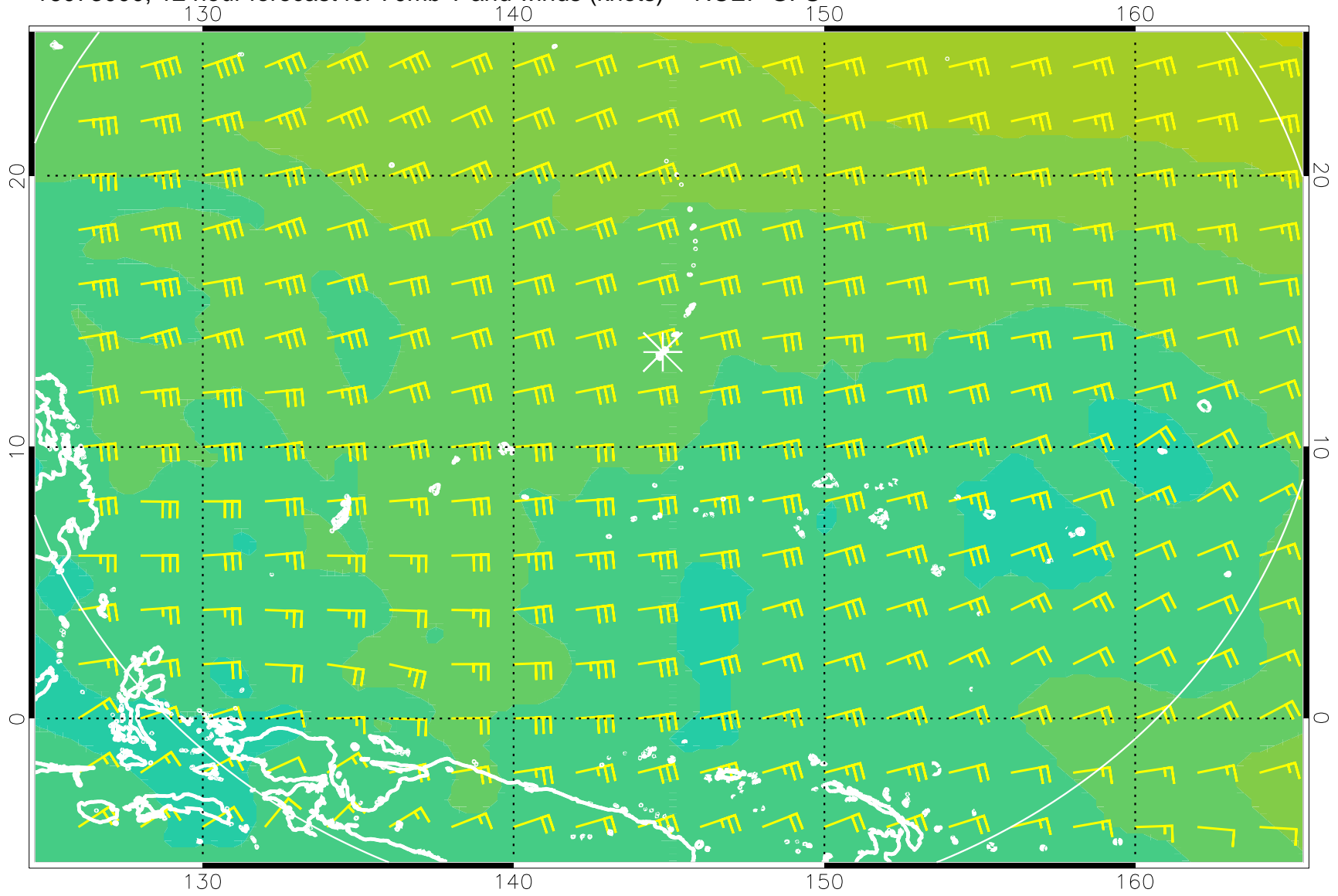
16073000, 12 hour forecast for 70mb T and winds (knots) -- NCEP GFS
