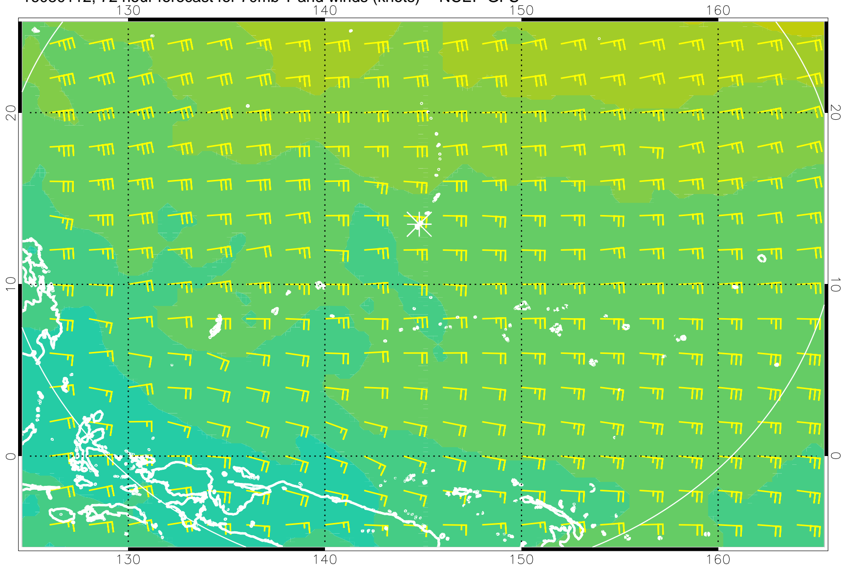
16080112, 72 hour forecast for 70mb T and winds (knots) -- NCEP GFS
