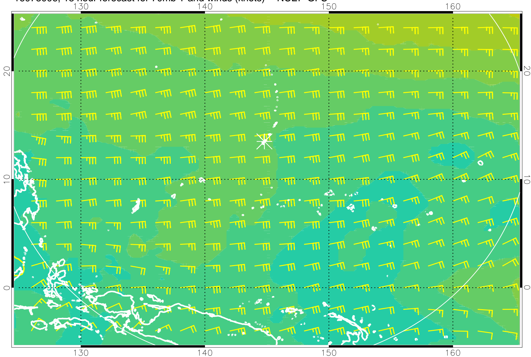
16073006, 18 hour forecast for 70mb T and winds (knots) -- NCEP GFS
