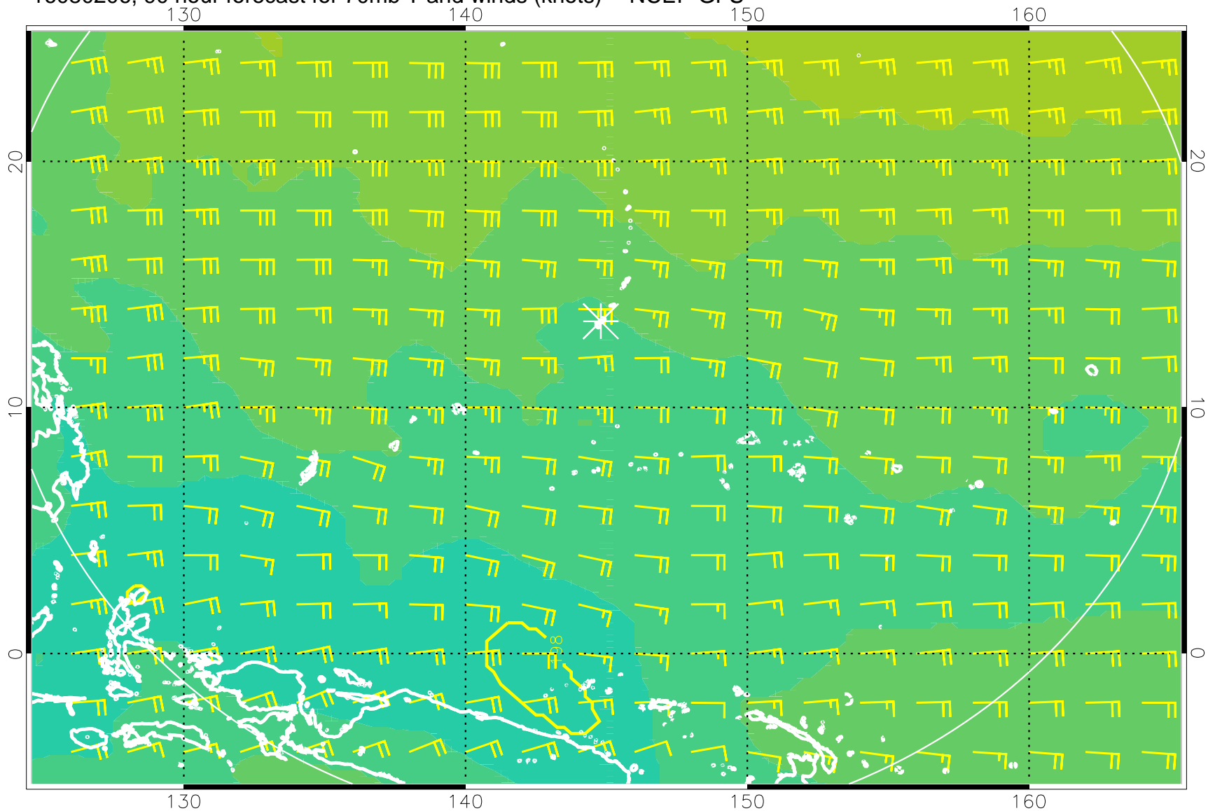
16080206, 90 hour forecast for 70mb T and winds (knots) -- NCEP GFS
