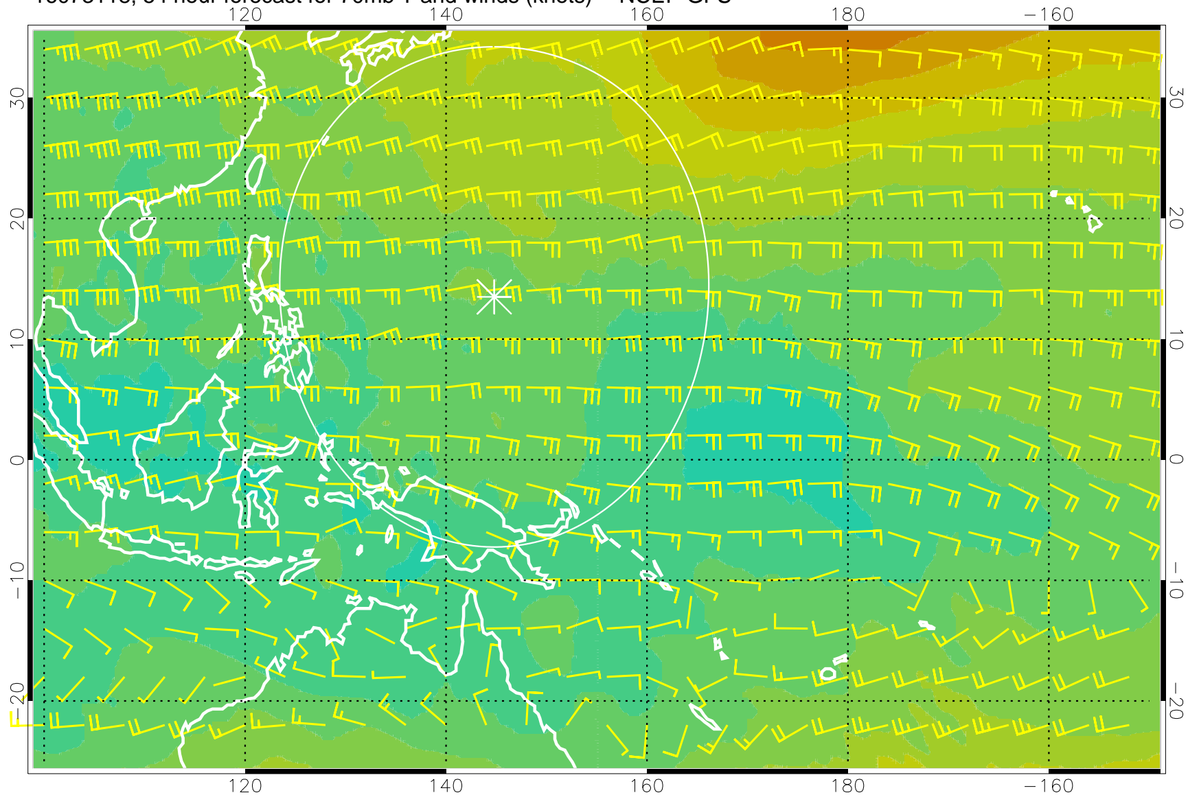
16073118, 54 hour forecast for 70mb T and winds (knots) -- NCEP GFS
