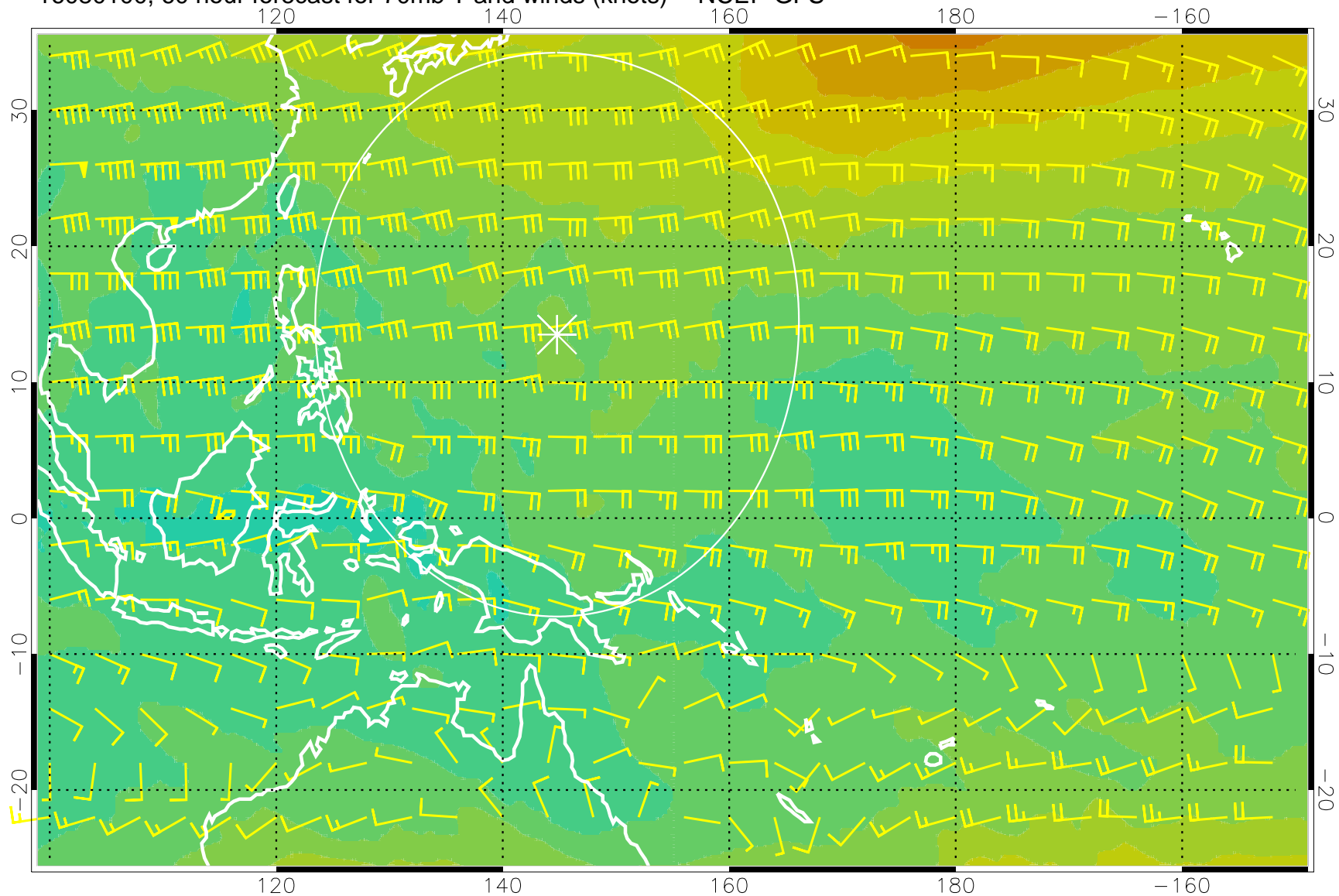
16080100, 60 hour forecast for 70mb T and winds (knots) -- NCEP GFS
