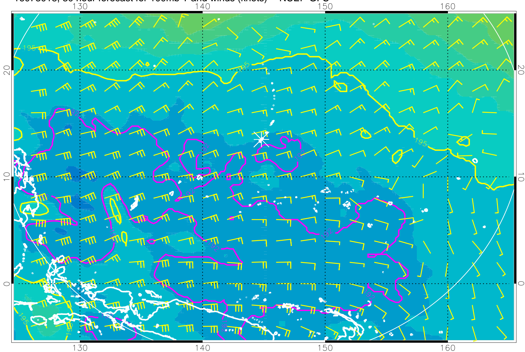
16073018, 30 hour forecast for 100mb T and winds (knots) -- NCEP GFS
