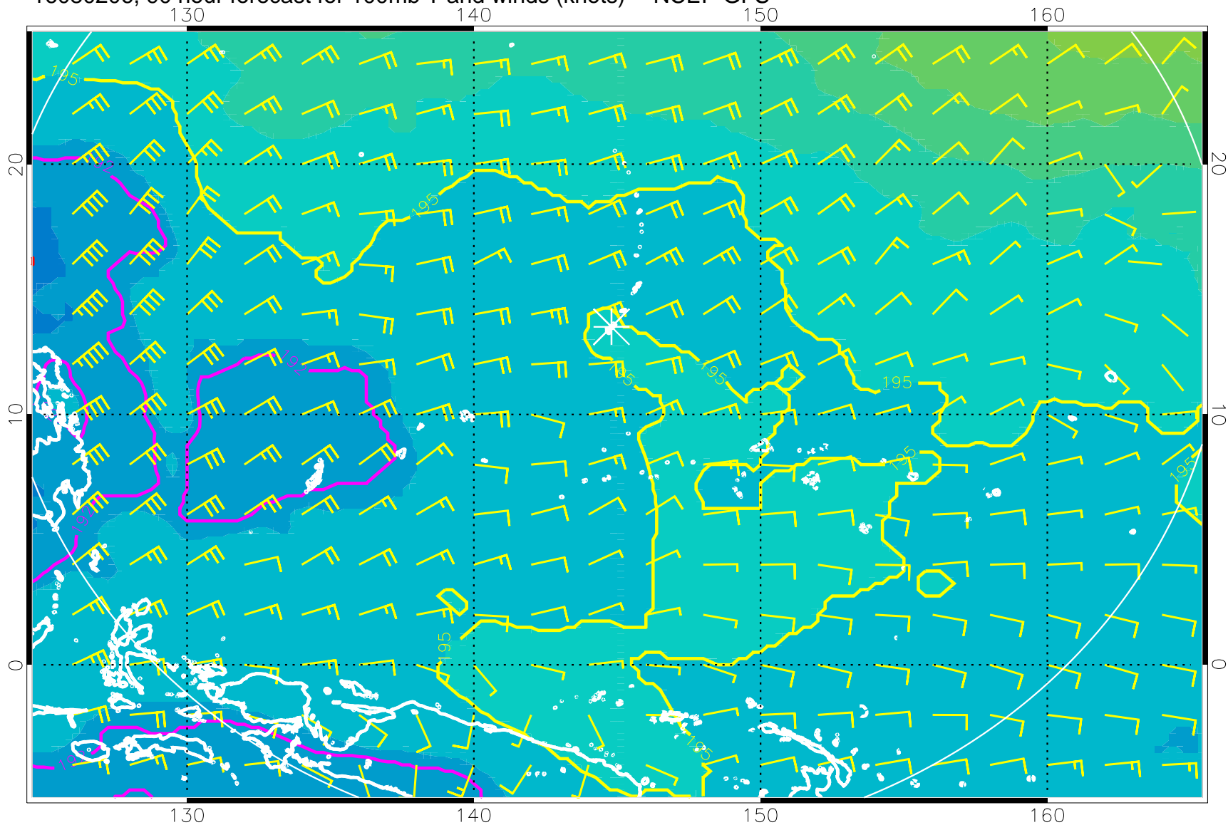
16080206, 90 hour forecast for 100mb T and winds (knots) -- NCEP GFS
