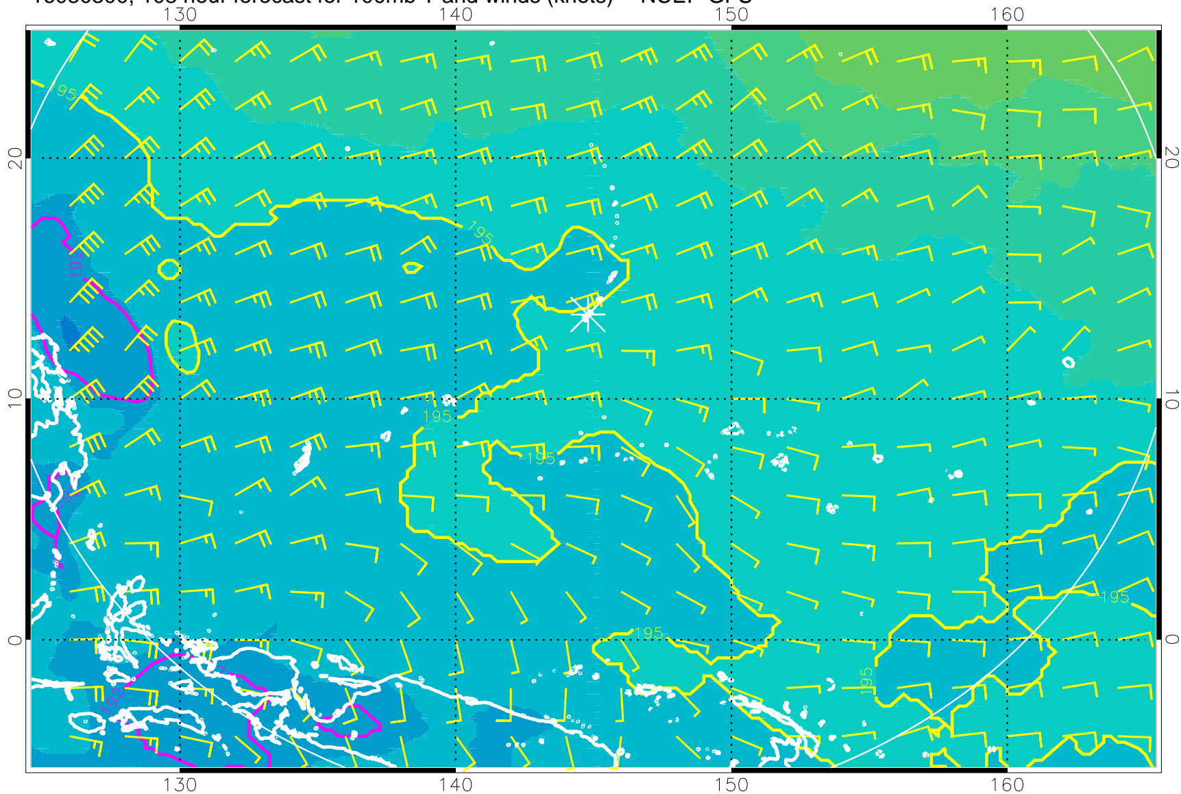
16080300, 108 hour forecast for 100mb T and winds (knots) -- NCEP GFS
