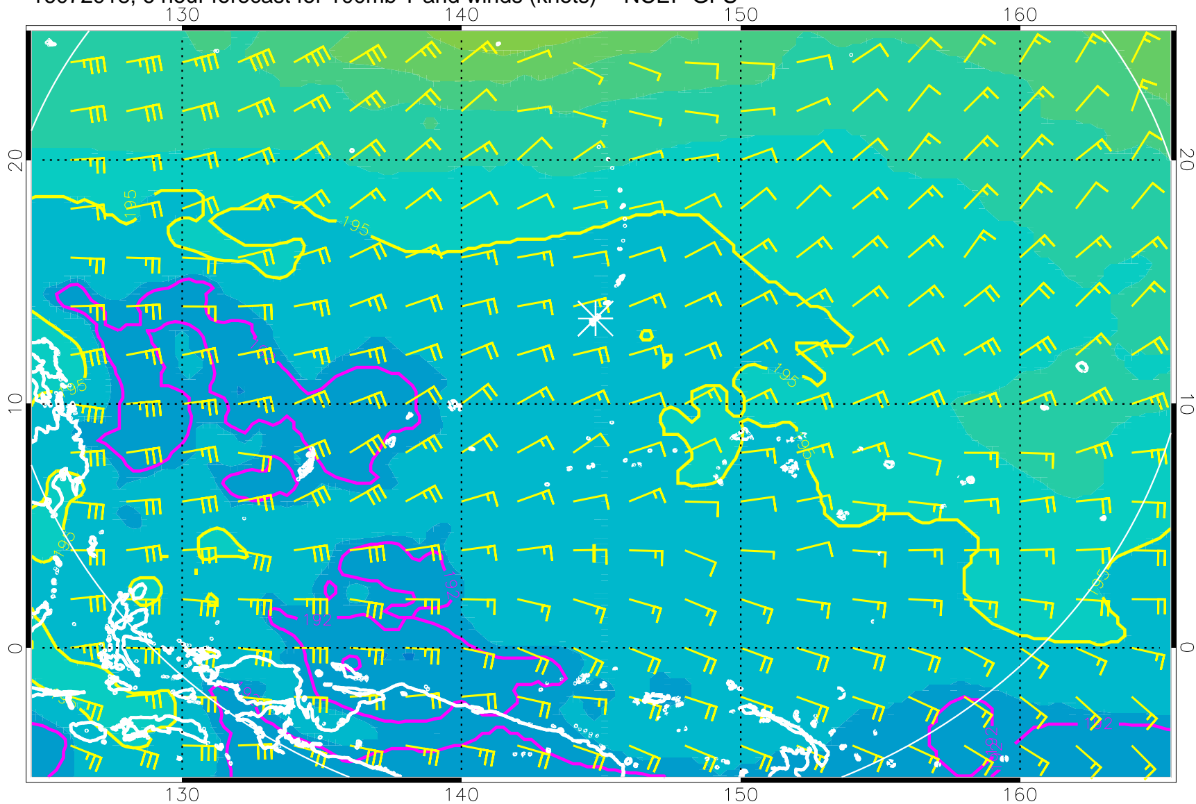
16072918, 6 hour forecast for 100mb T and winds (knots) -- NCEP GFS
