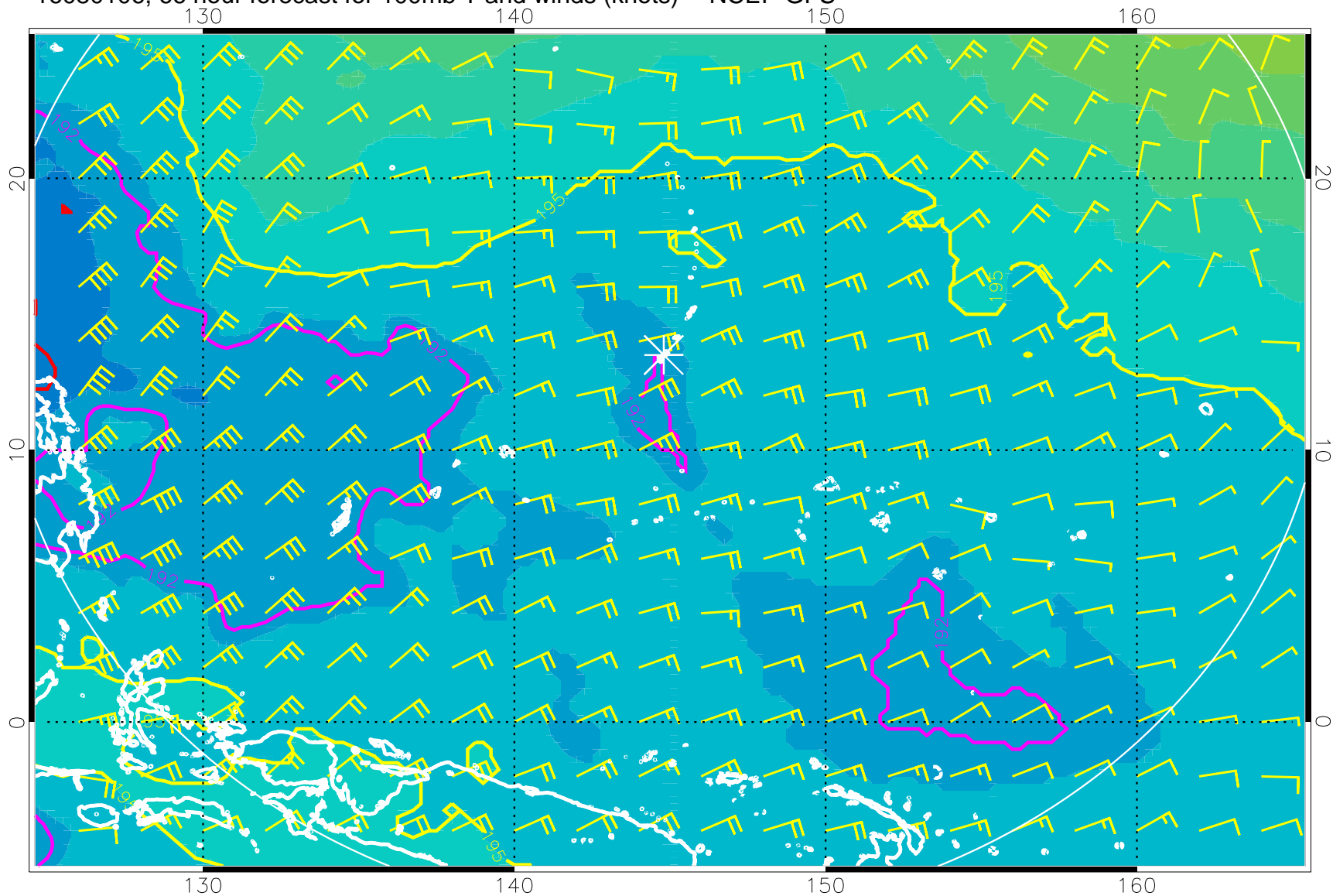
16080106, 66 hour forecast for 100mb T and winds (knots) -- NCEP GFS
