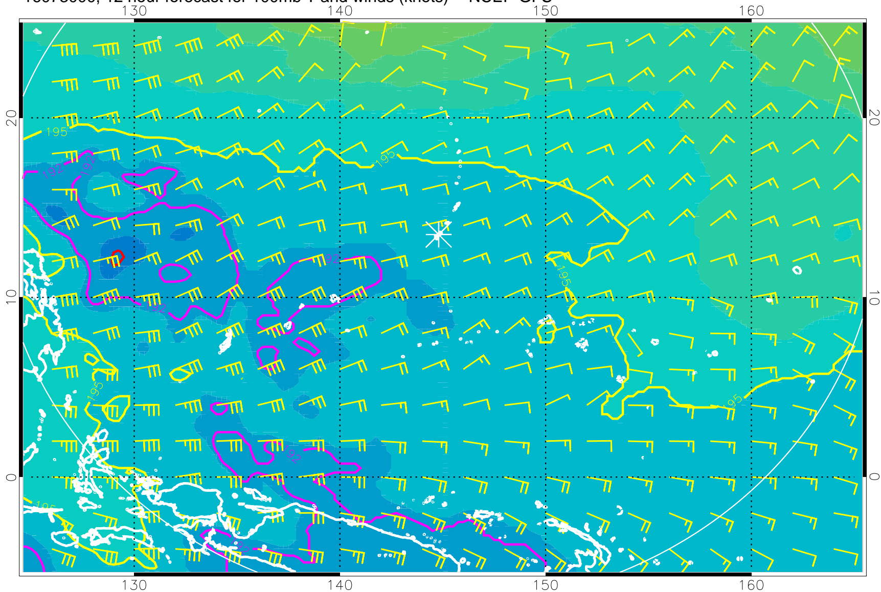
16073000, 12 hour forecast for 100mb T and winds (knots) -- NCEP GFS
