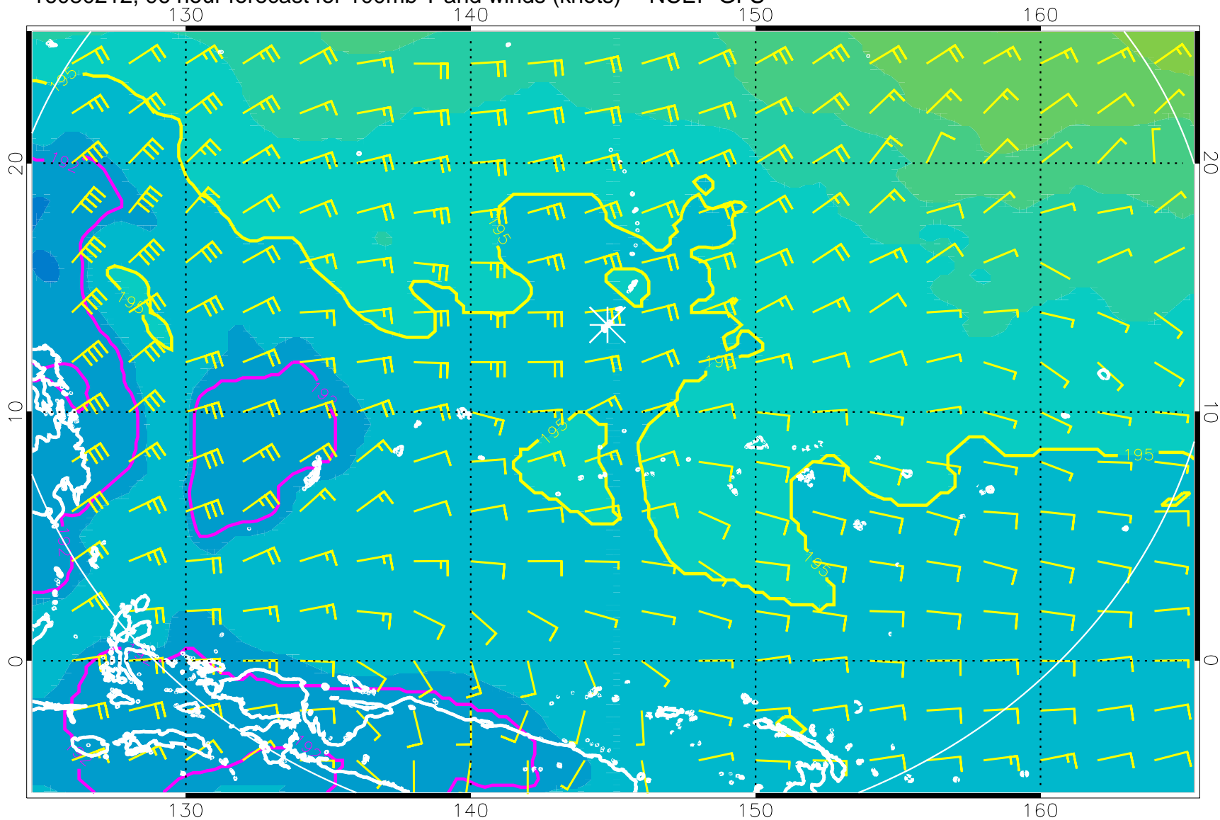
16080212, 96 hour forecast for 100mb T and winds (knots) -- NCEP GFS
