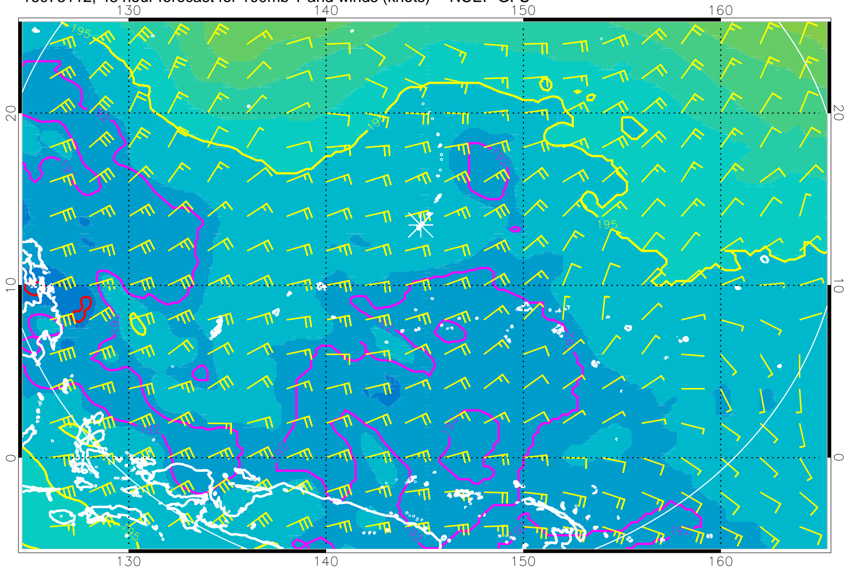
16073112, 48 hour forecast for 100mb T and winds (knots) -- NCEP GFS
