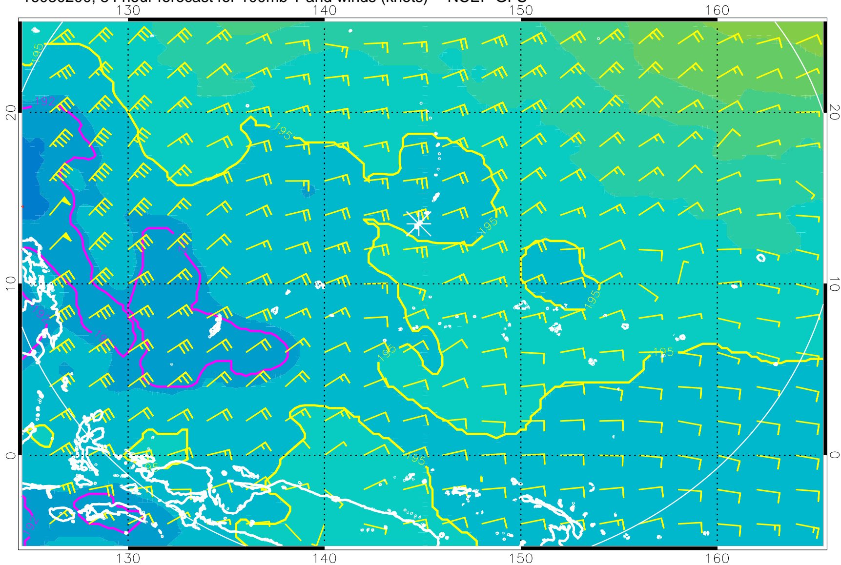
16080200, 84 hour forecast for 100mb T and winds (knots) -- NCEP GFS
