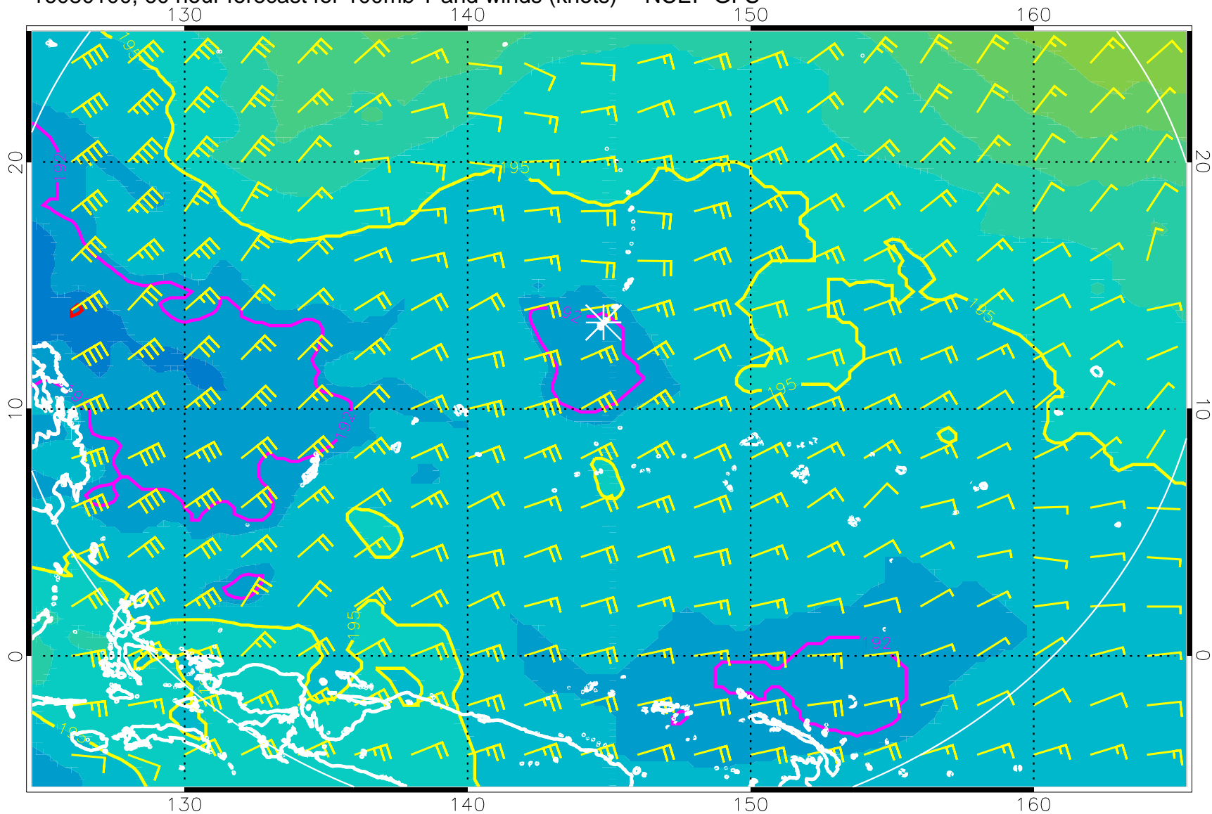
16080100, 60 hour forecast for 100mb T and winds (knots) -- NCEP GFS
