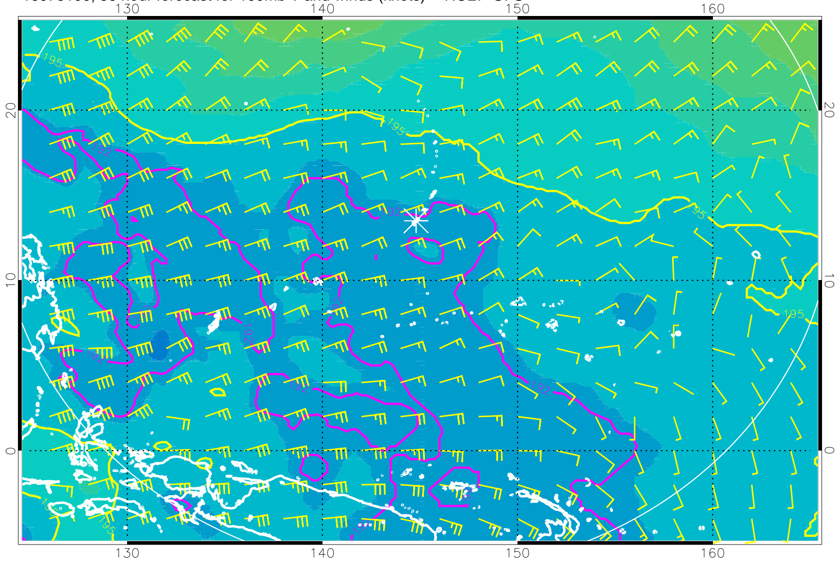
16073100, 36 hour forecast for 100mb T and winds (knots) -- NCEP GFS
