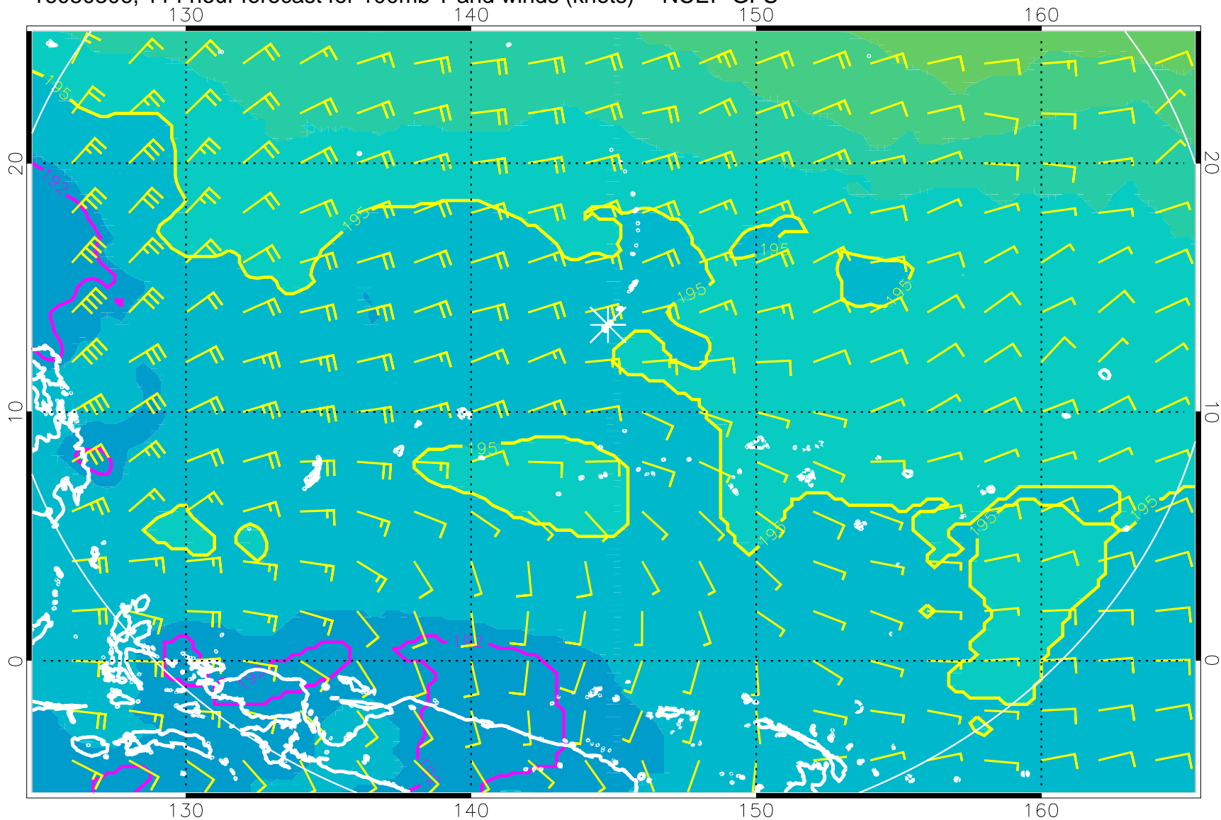
16080306, 114 hour forecast for 100mb T and winds (knots) -- NCEP GFS
