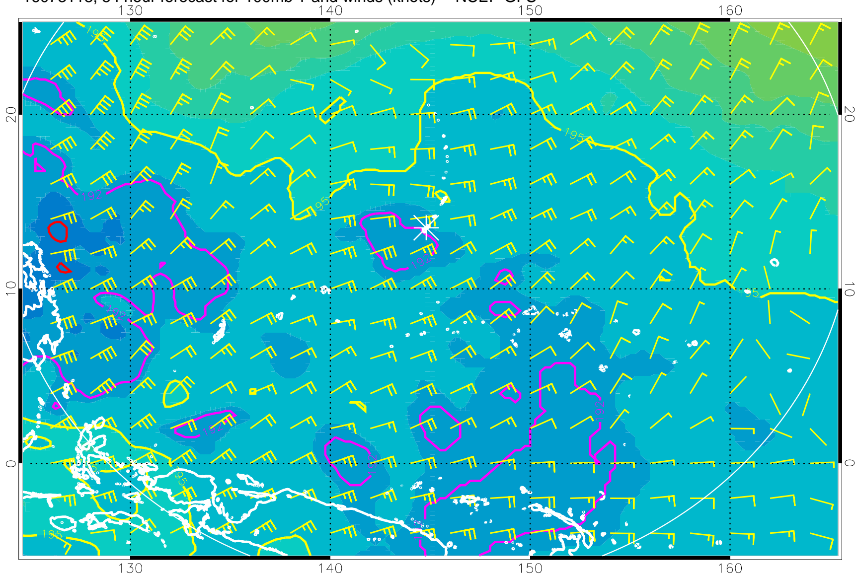
16073118, 54 hour forecast for 100mb T and winds (knots) -- NCEP GFS
