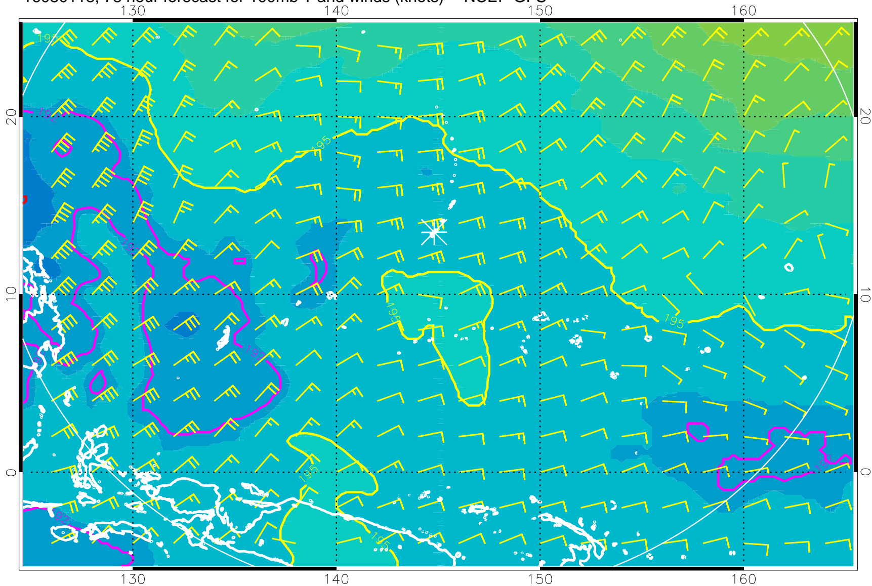
16080118, 78 hour forecast for 100mb T and winds (knots) -- NCEP GFS
