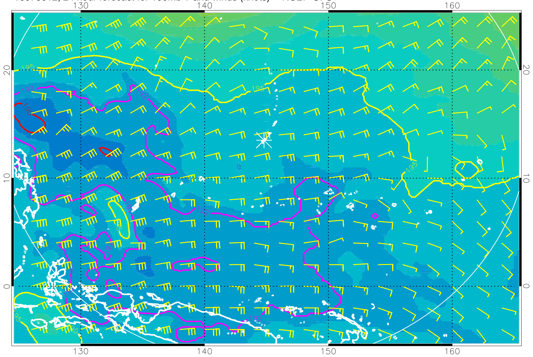
16073012, 24 hour forecast for 100mb T and winds (knots) -- NCEP GFS
