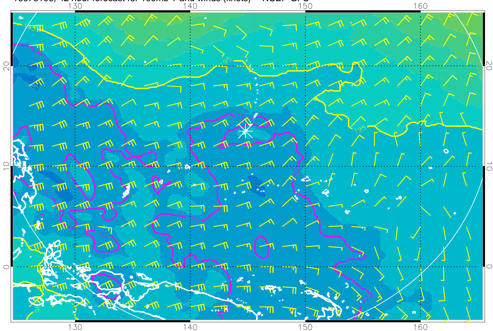
16073106, 42 hour forecast for 100mb T and winds (knots) -- NCEP GFS
