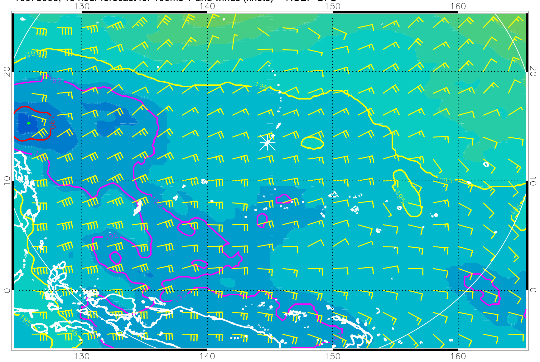
16073006, 18 hour forecast for 100mb T and winds (knots) -- NCEP GFS
