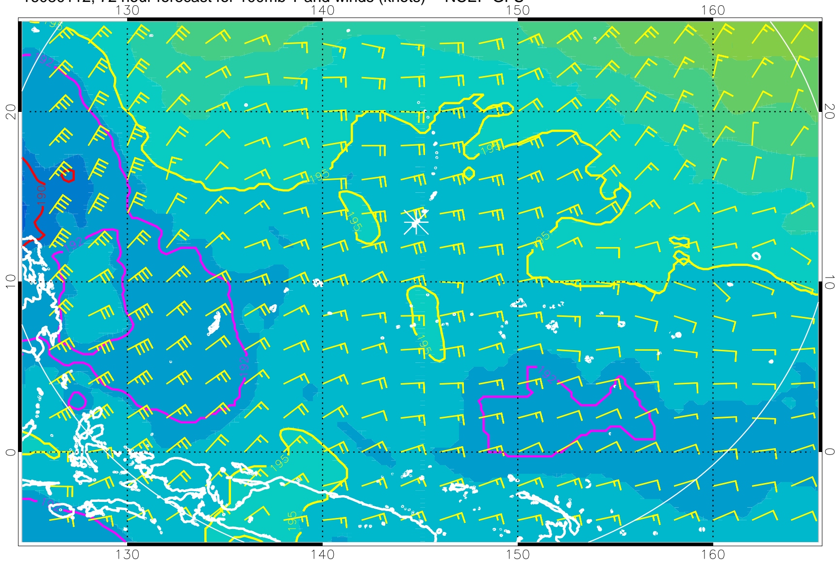
16080112, 72 hour forecast for 100mb T and winds (knots) -- NCEP GFS
