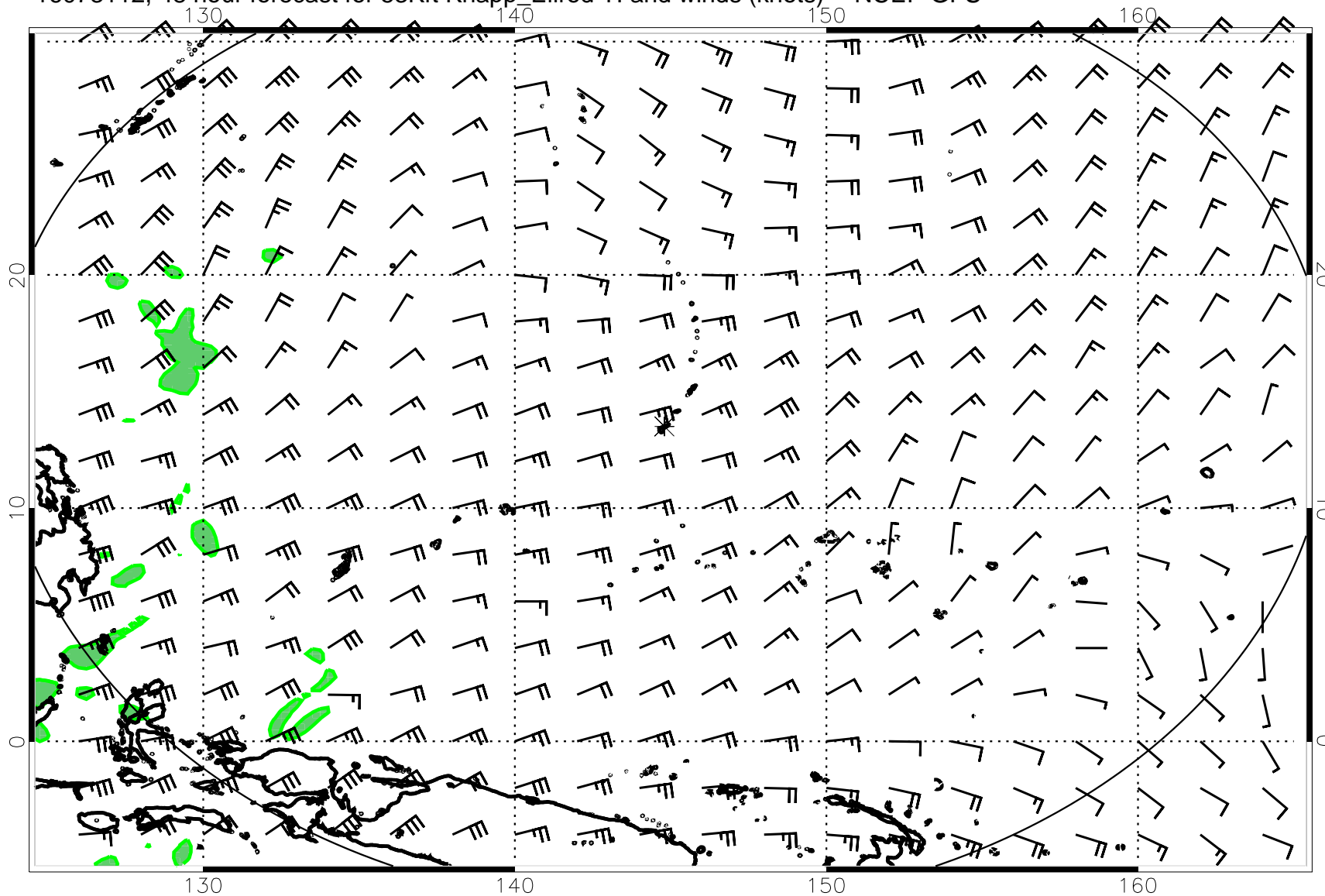
16073112, 48 hour forecast for 53Kft Knapp_Ellrod TI and winds (knots) -- NCEP GFS
