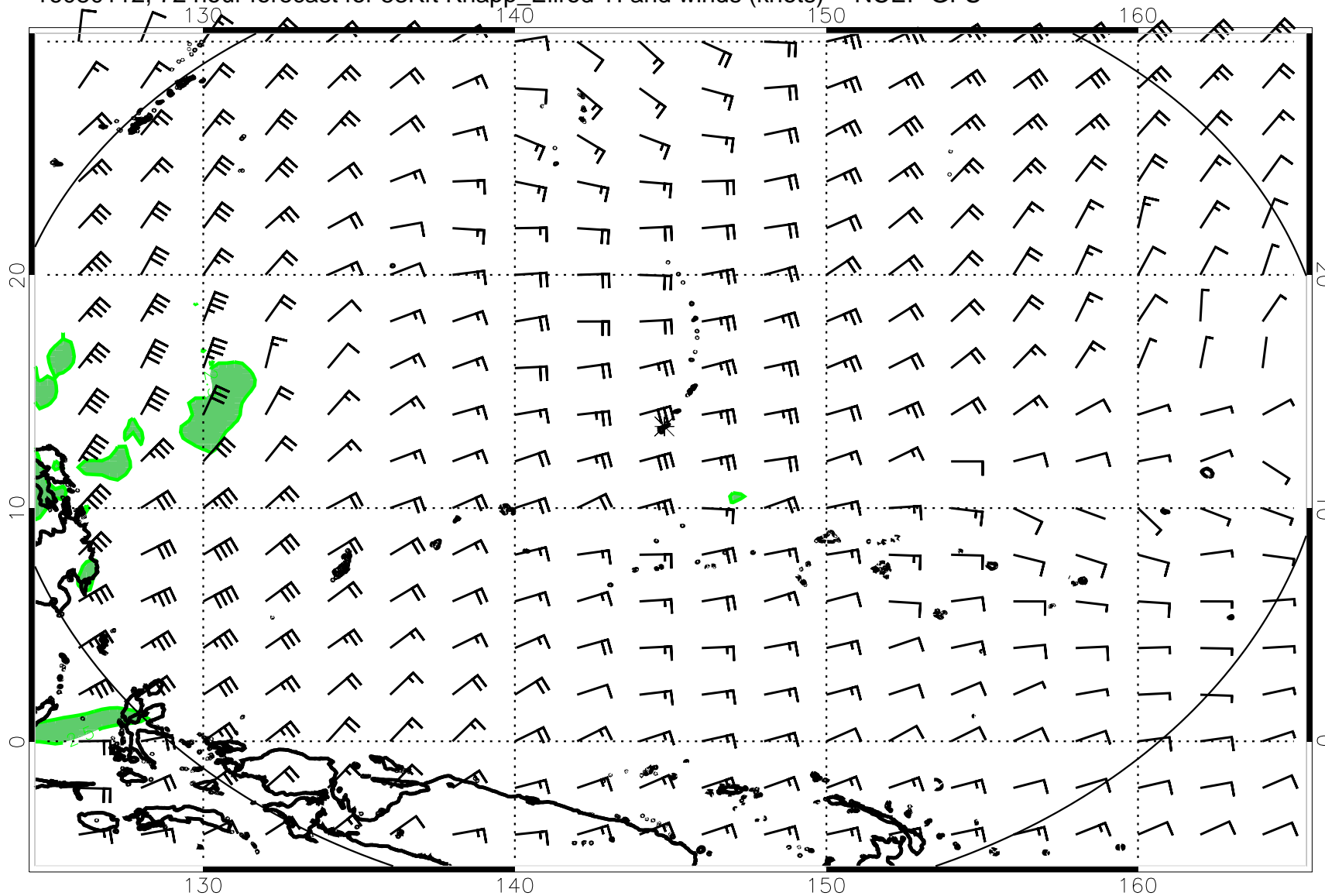
16080112, 72 hour forecast for 53Kft Knapp_Ellrod TI and winds (knots) -- NCEP GFS
