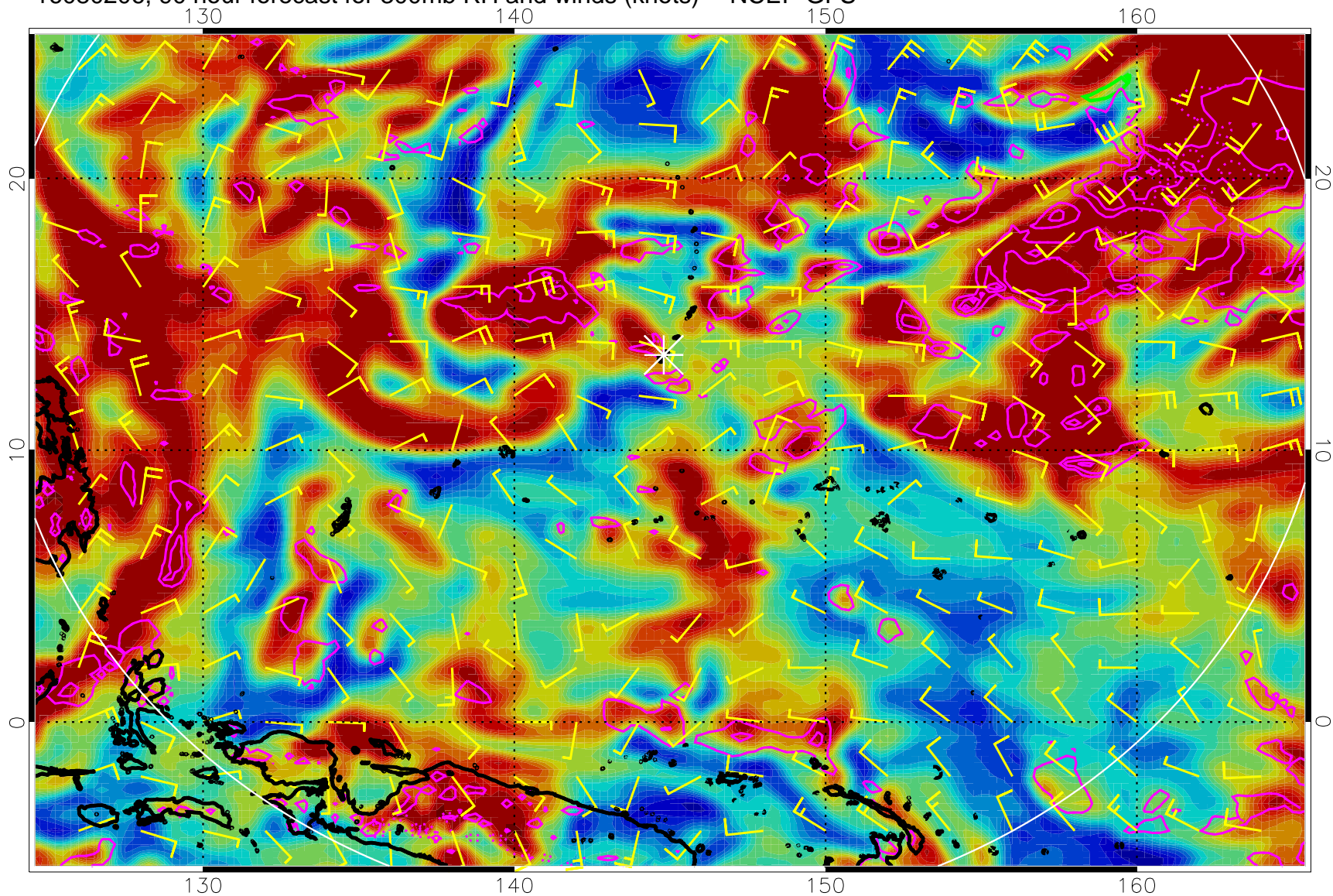
16080206, 90 hour forecast for 300mb RH and winds (knots) -- NCEP GFS
