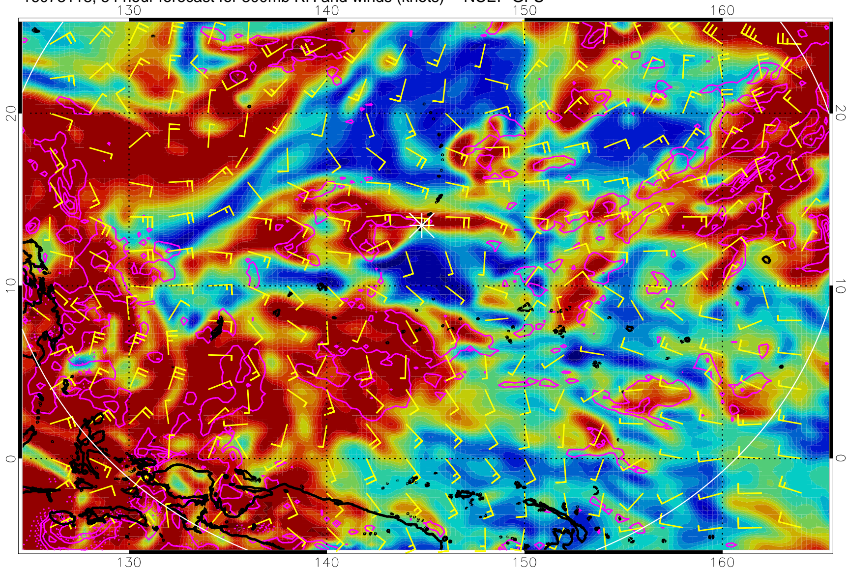
16073118, 54 hour forecast for 300mb RH and winds (knots) -- NCEP GFS
