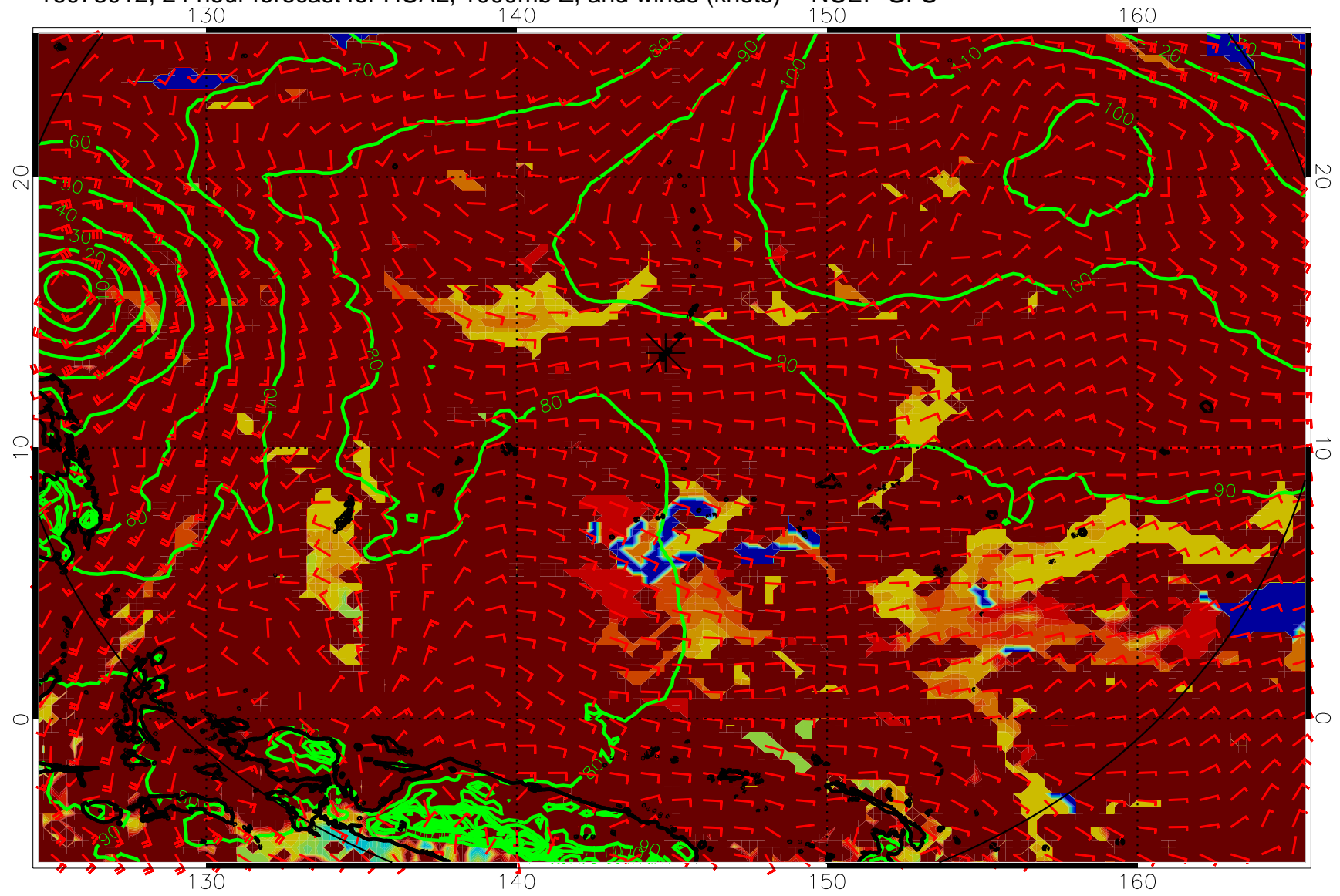
16073012, 24 hour forecast for HCAL, 1000mb Z, and winds (knots) -- NCEP GFS
