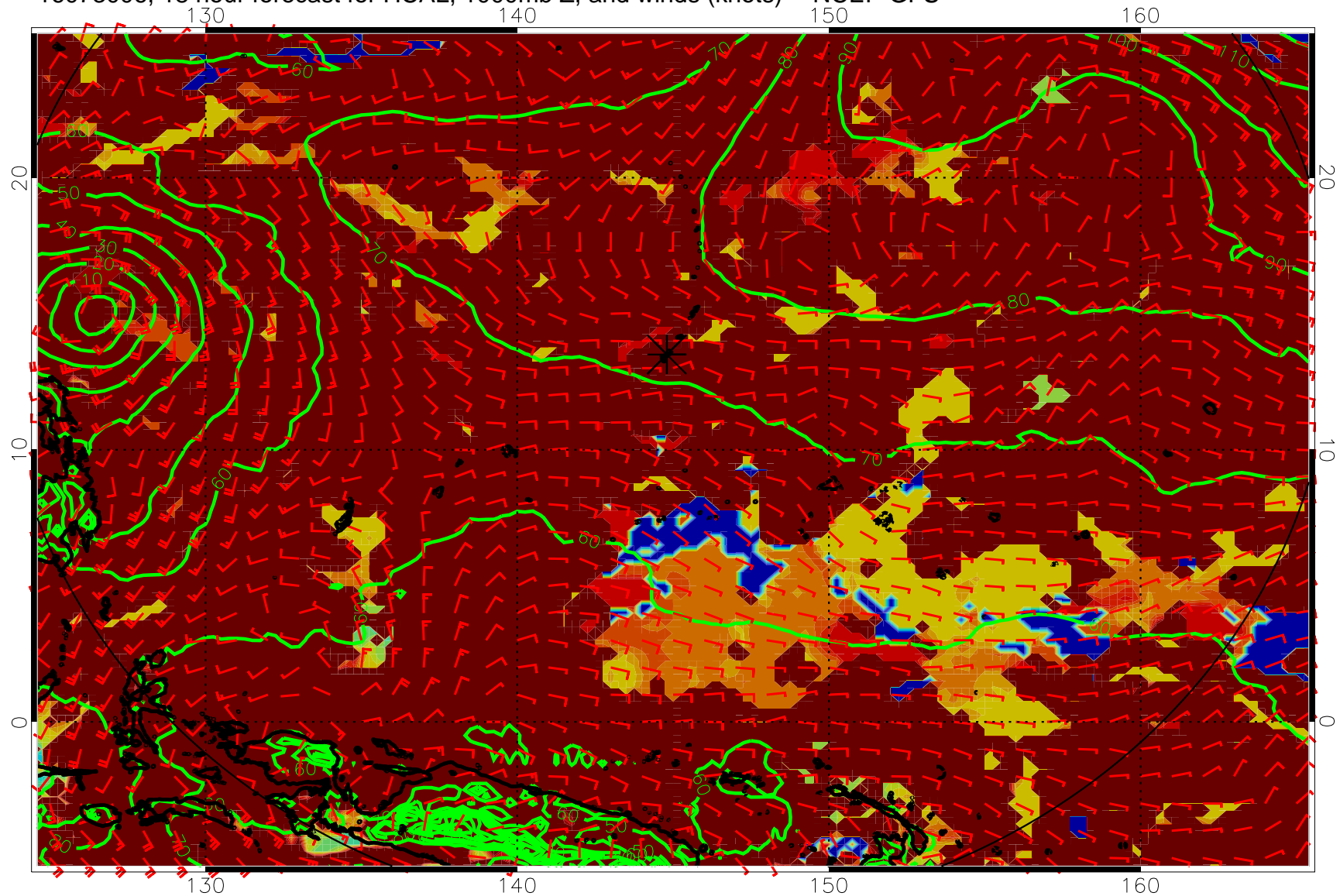
16073006, 18 hour forecast for HCAL, 1000mb Z, and winds (knots) -- NCEP GFS
