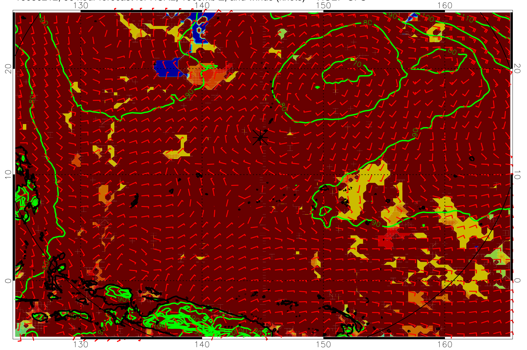
16080212, 96 hour forecast for HCAL, 1000mb Z, and winds (knots) -- NCEP GFS
