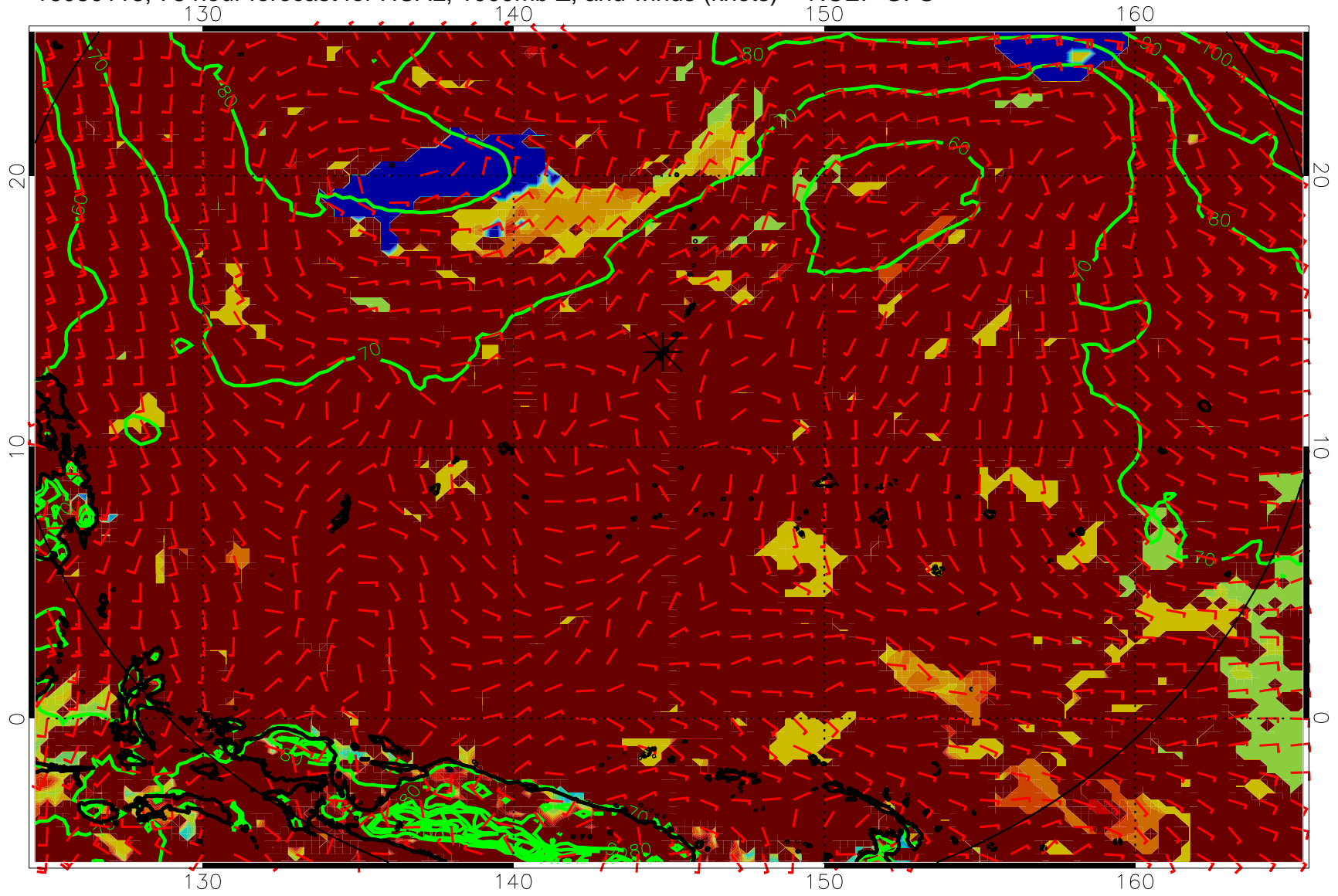
16080118, 78 hour forecast for HCAL, 1000mb Z, and winds (knots) -- NCEP GFS
