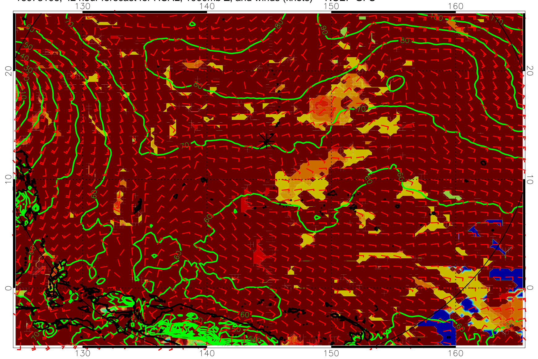
16073106, 42 hour forecast for HCAL, 1000mb Z, and winds (knots) -- NCEP GFS
