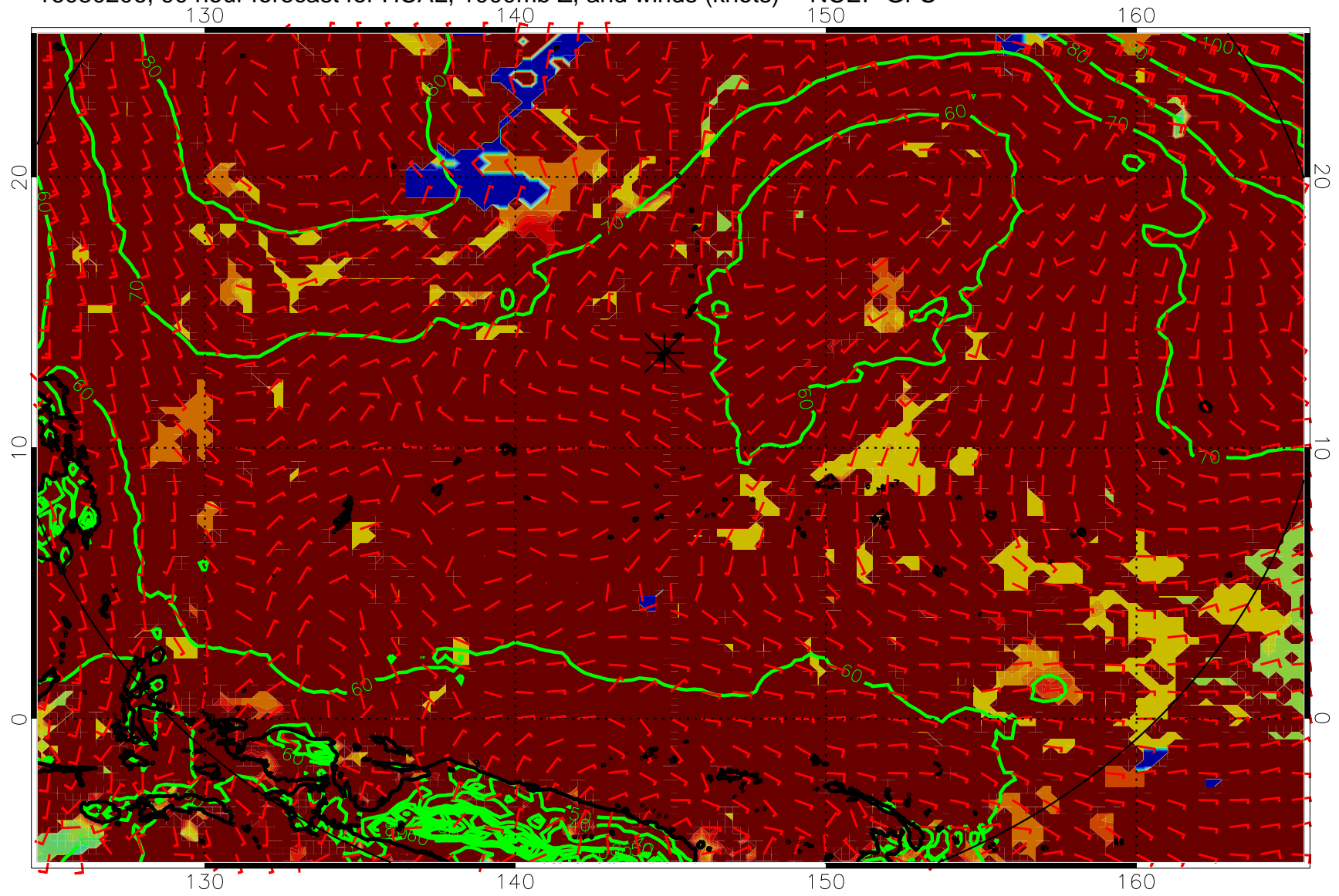
16080206, 90 hour forecast for HCAL, 1000mb Z, and winds (knots) -- NCEP GFS
