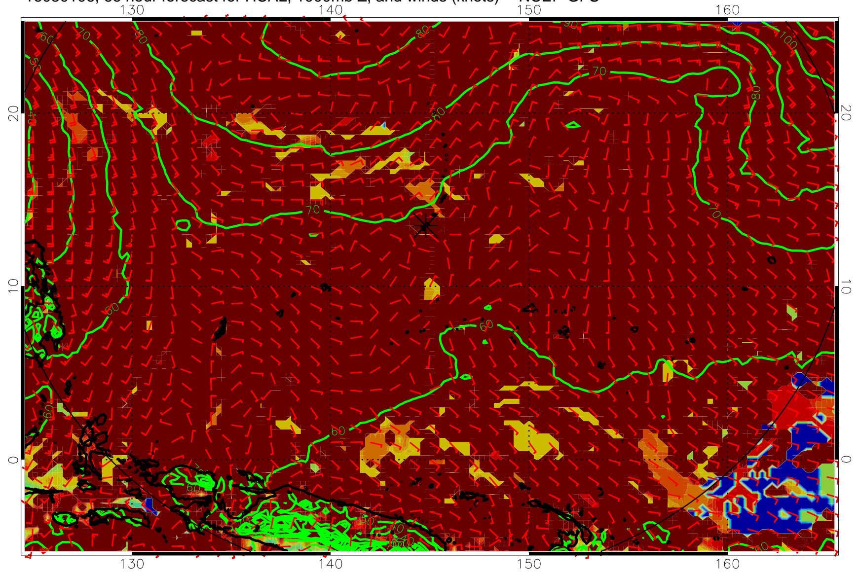
16080106, 66 hour forecast for HCAL, 1000mb Z, and winds (knots) -- NCEP GFS
