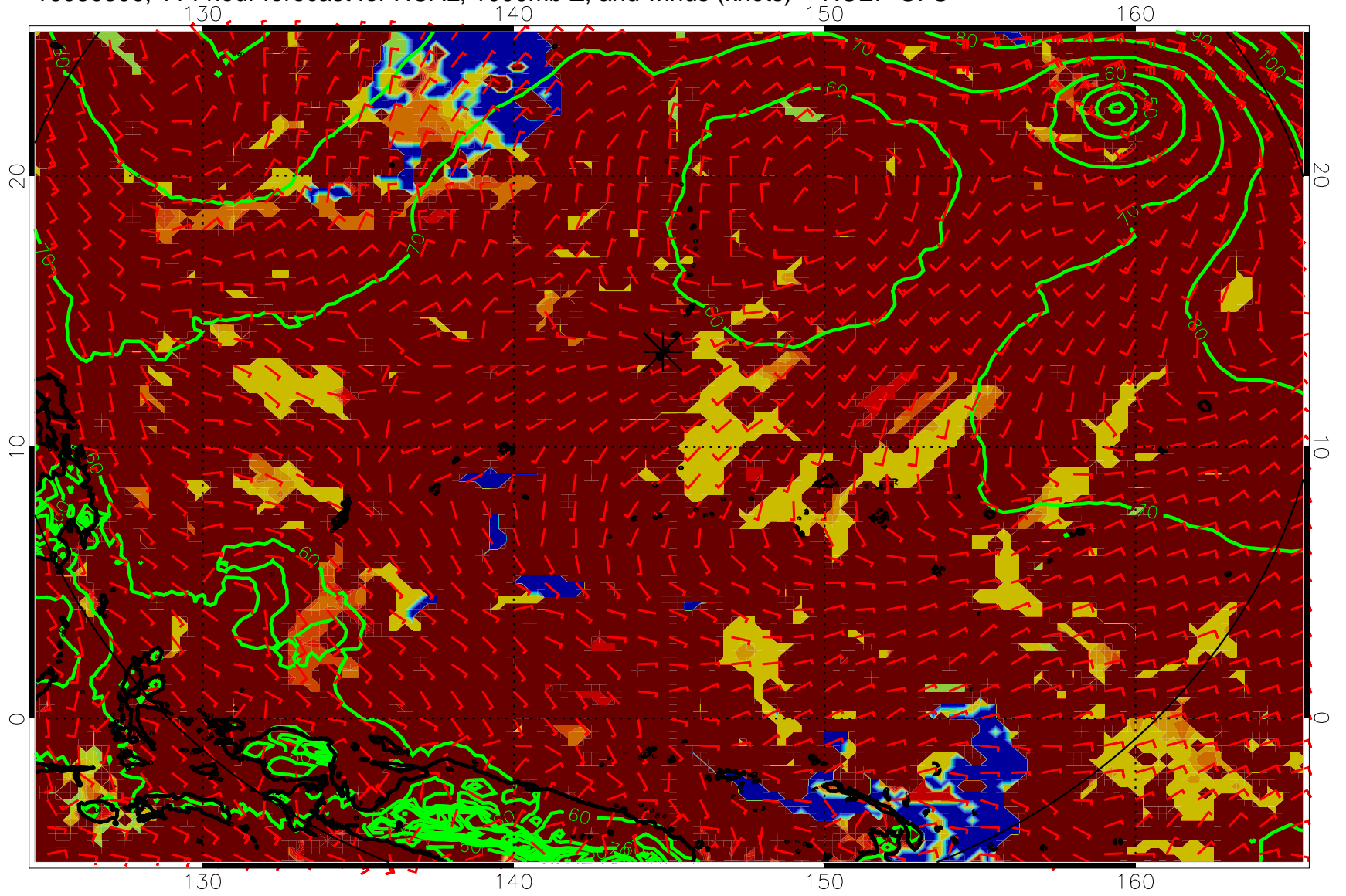
16080306, 114 hour forecast for HCAL, 1000mb Z, and winds (knots) -- NCEP GFS
