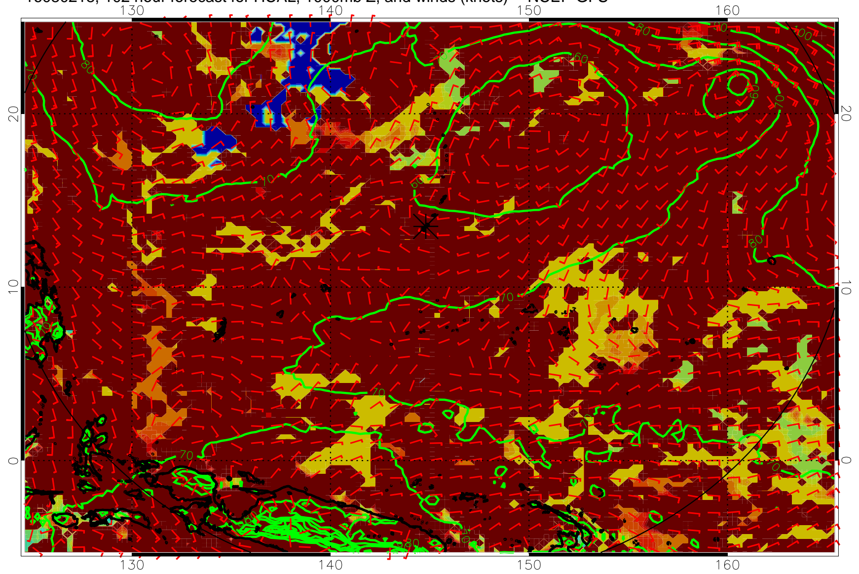
16080218, 102 hour forecast for HCAL, 1000mb Z, and winds (knots) -- NCEP GFS
