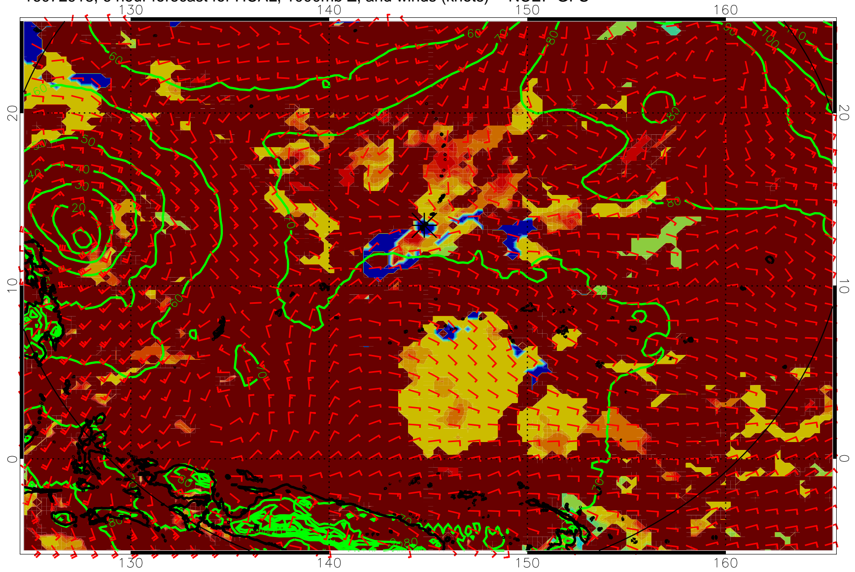
16072918, 6 hour forecast for HCAL, 1000mb Z, and winds (knots) -- NCEP GFS
