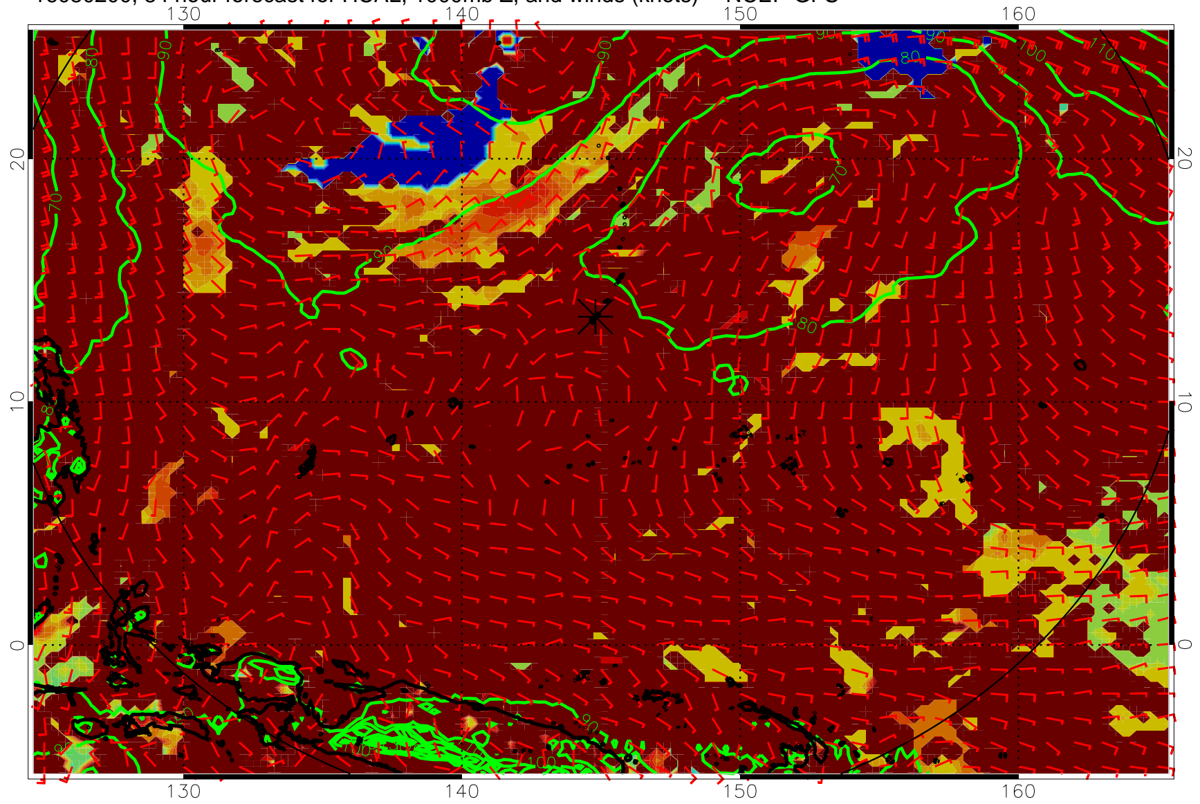
16080200, 84 hour forecast for HCAL, 1000mb Z, and winds (knots) -- NCEP GFS
