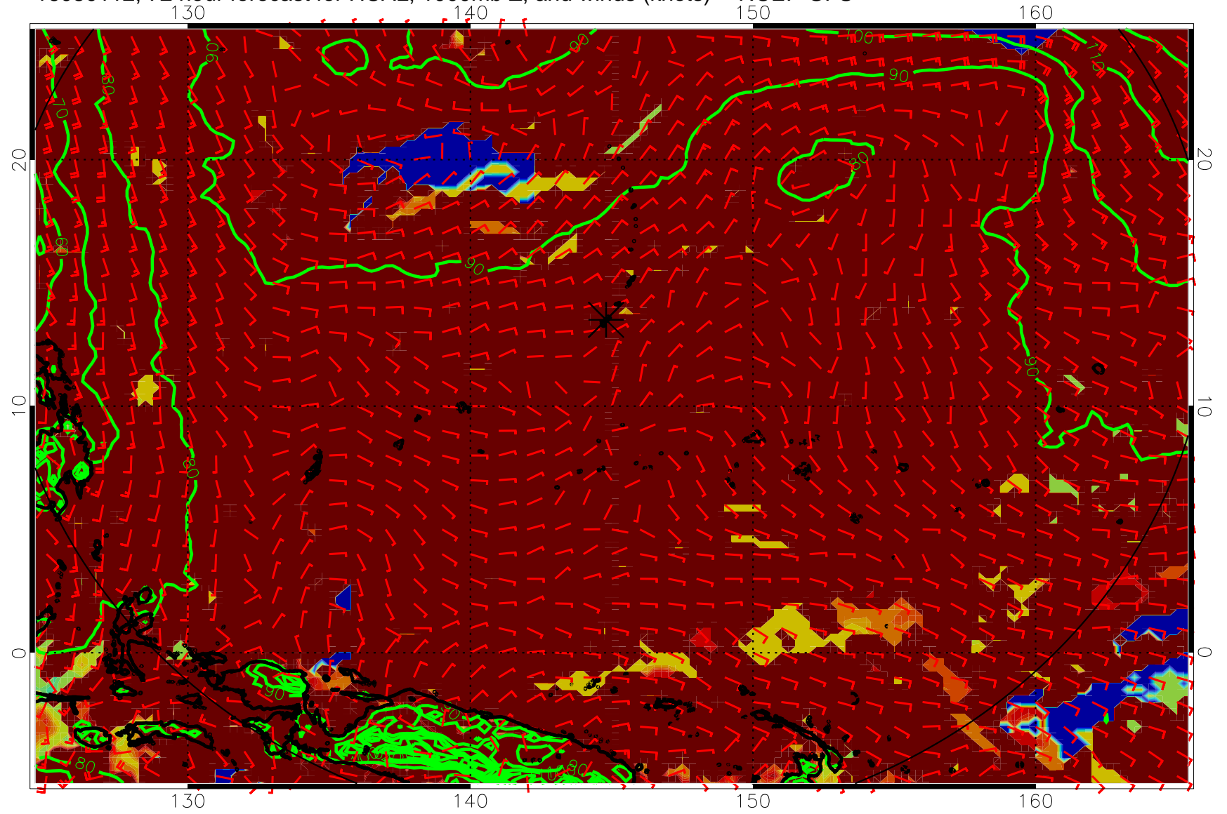
16080112, 72 hour forecast for HCAL, 1000mb Z, and winds (knots) -- NCEP GFS
