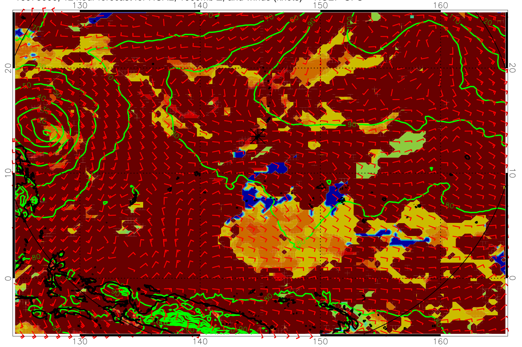
16073000, 12 hour forecast for HCAL, 1000mb Z, and winds (knots) -- NCEP GFS
