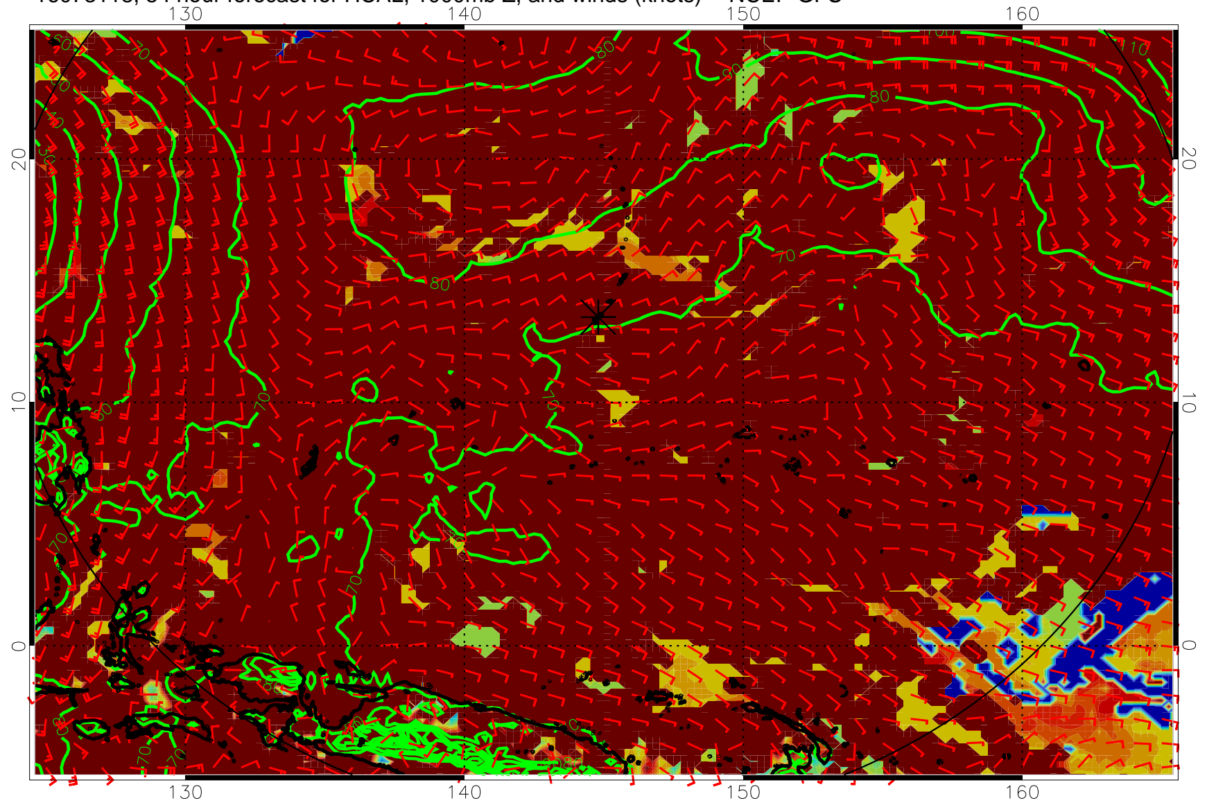
16073118, 54 hour forecast for HCAL, 1000mb Z, and winds (knots) -- NCEP GFS
