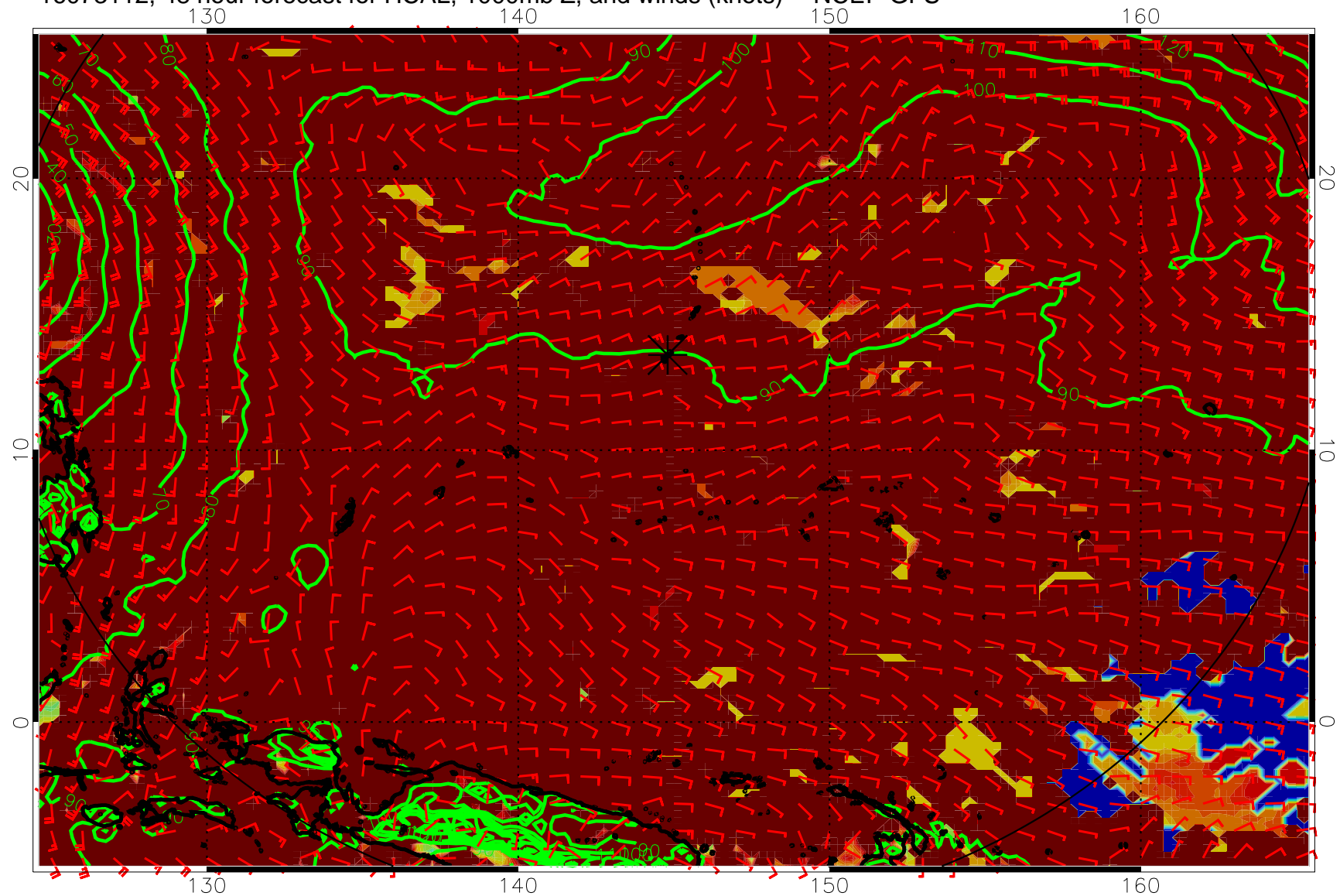
16073112, 48 hour forecast for HCAL, 1000mb Z, and winds (knots) -- NCEP GFS
