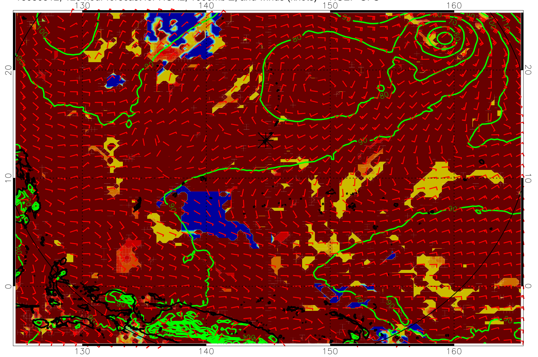
16080312, 120 hour forecast for HCAL, 1000mb Z, and winds (knots) -- NCEP GFS
