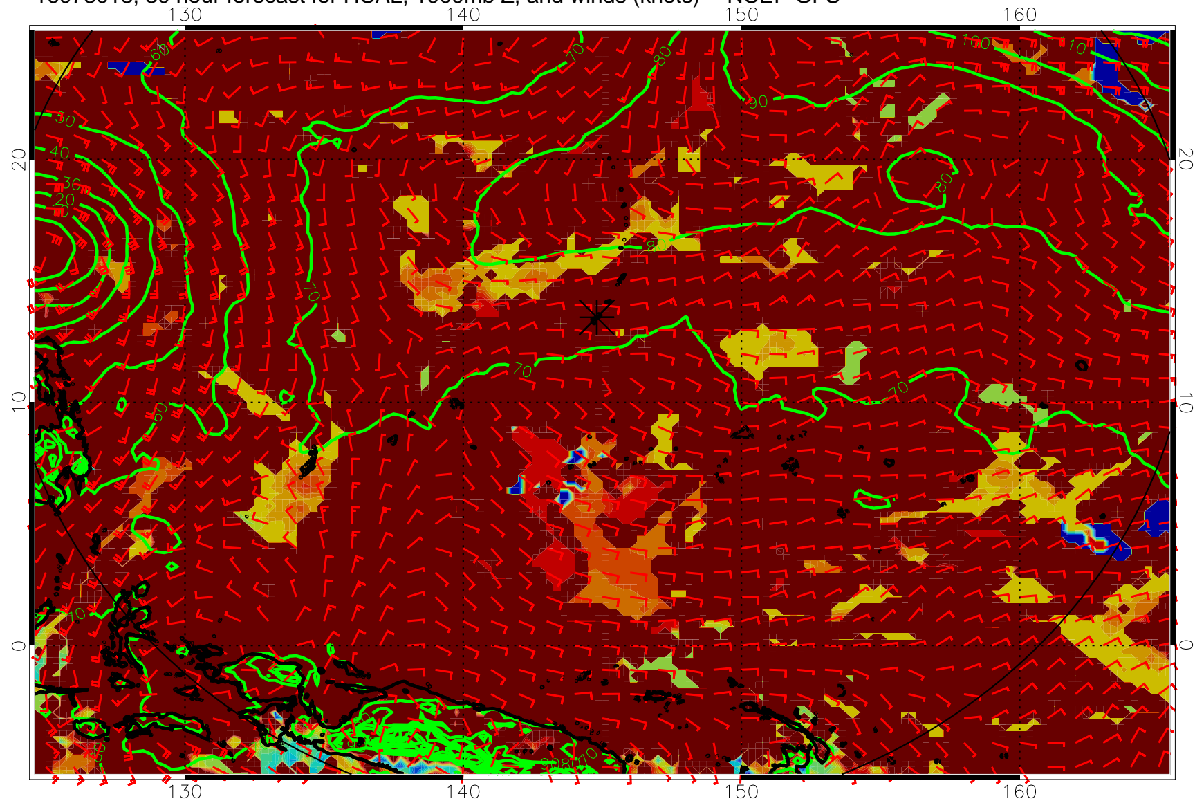
16073018, 30 hour forecast for HCAL, 1000mb Z, and winds (knots) -- NCEP GFS
