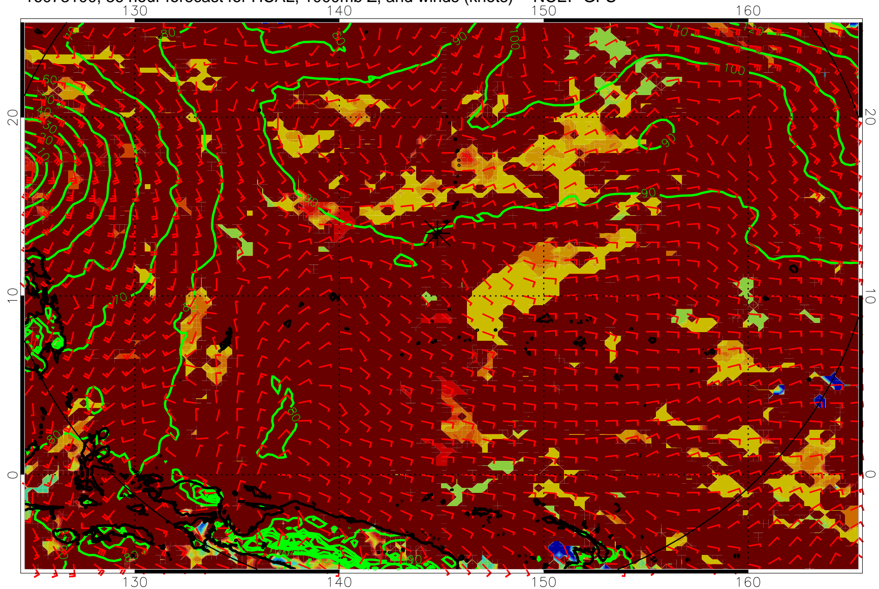
16073100, 36 hour forecast for HCAL, 1000mb Z, and winds (knots) -- NCEP GFS
