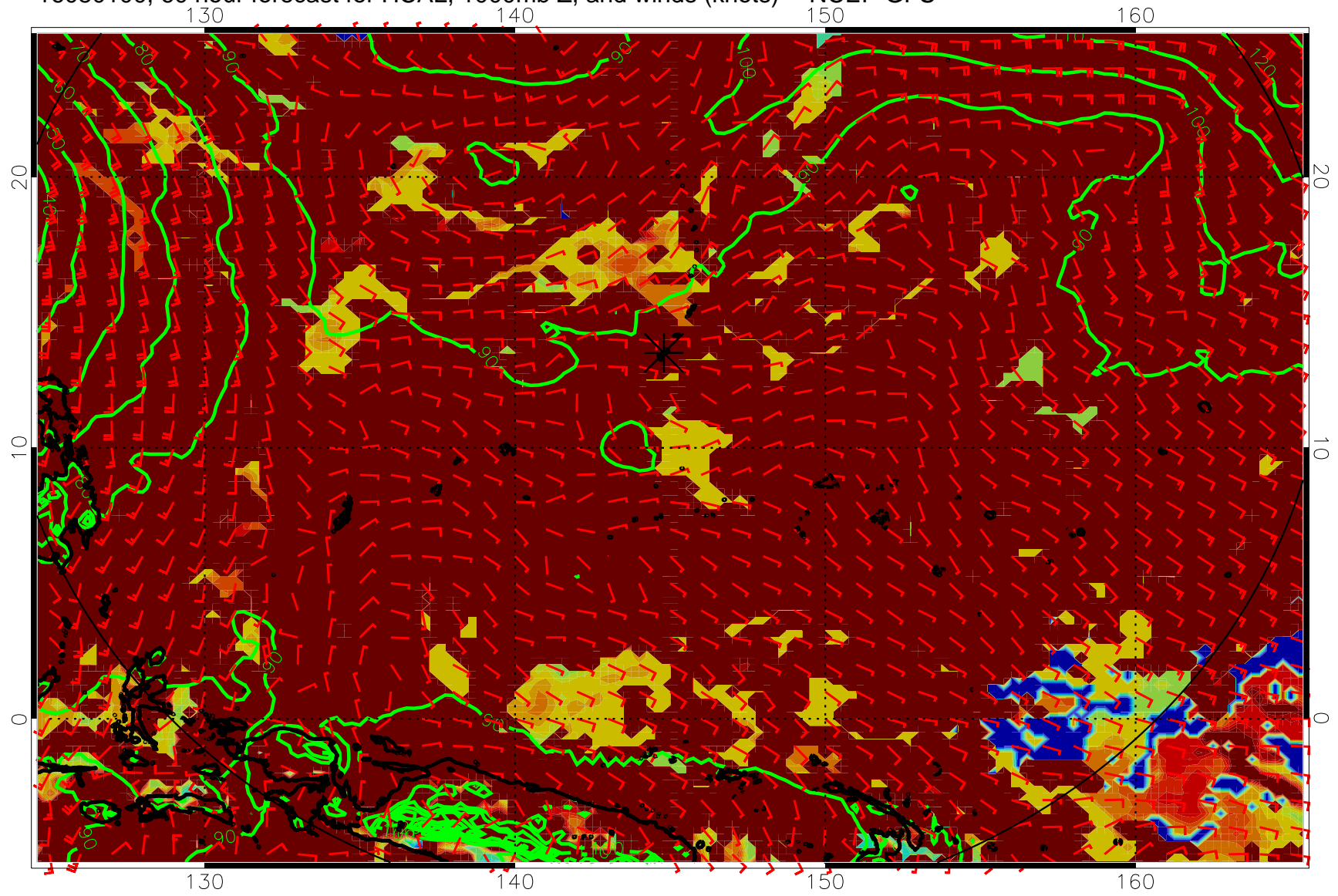
16080100, 60 hour forecast for HCAL, 1000mb Z, and winds (knots) -- NCEP GFS
