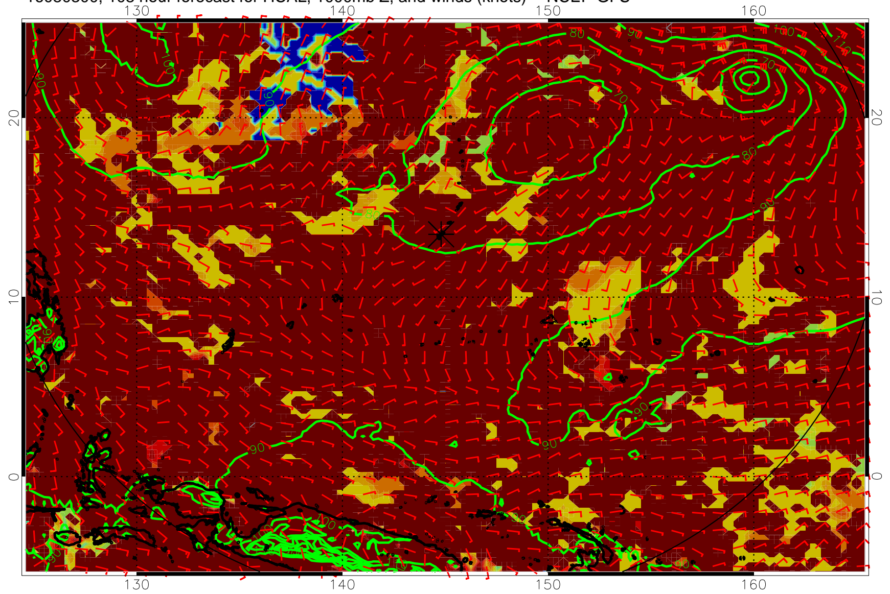
16080300, 108 hour forecast for HCAL, 1000mb Z, and winds (knots) -- NCEP GFS
